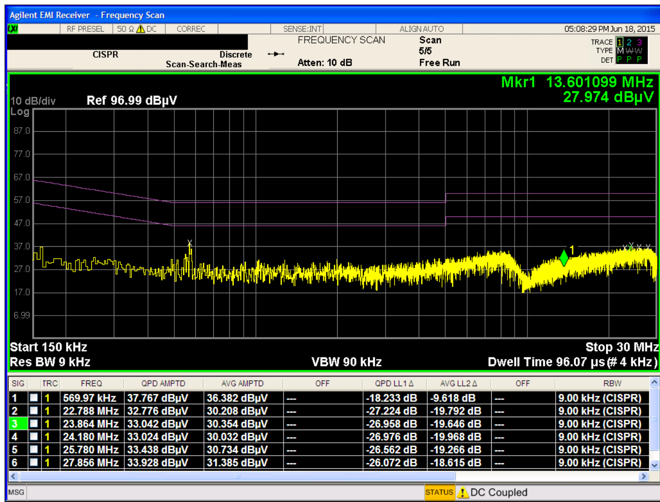
Plot 7-3. Line-Conducted Test Plot (L1) 50Ohm Terminated Antenna
