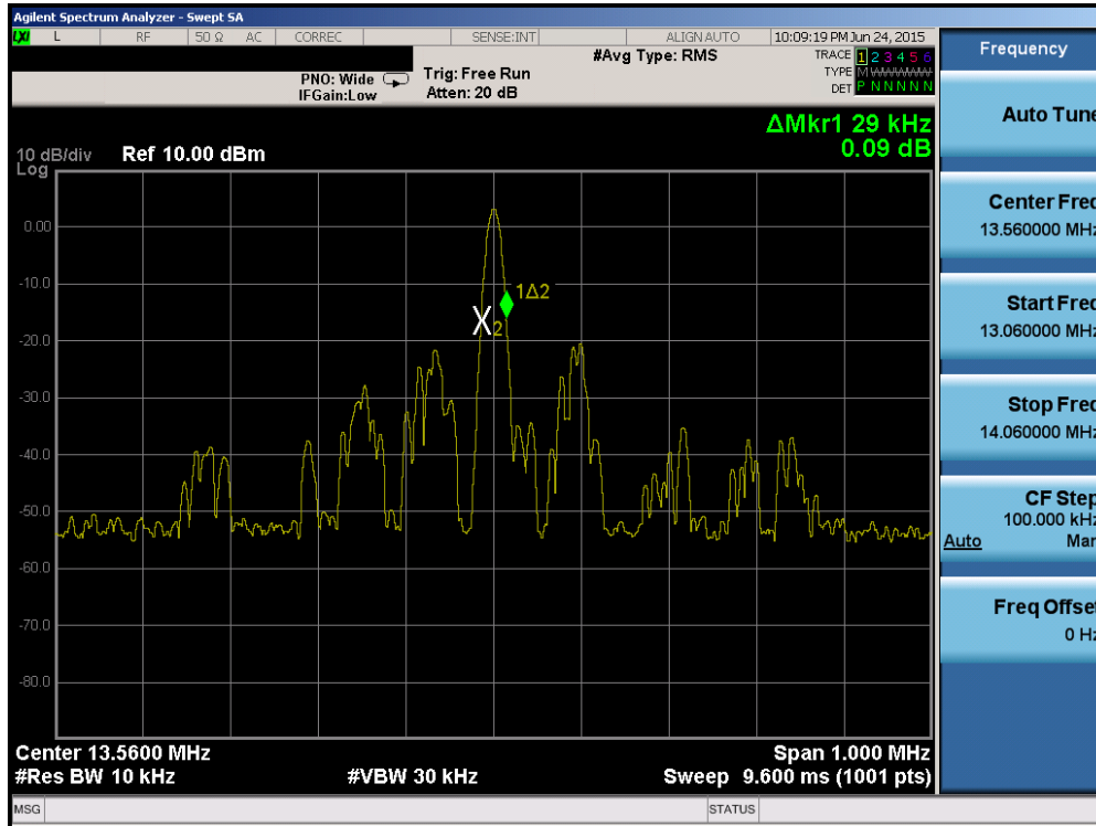
Figure 7-3. 20dB Bandwidth Plot with WCP
