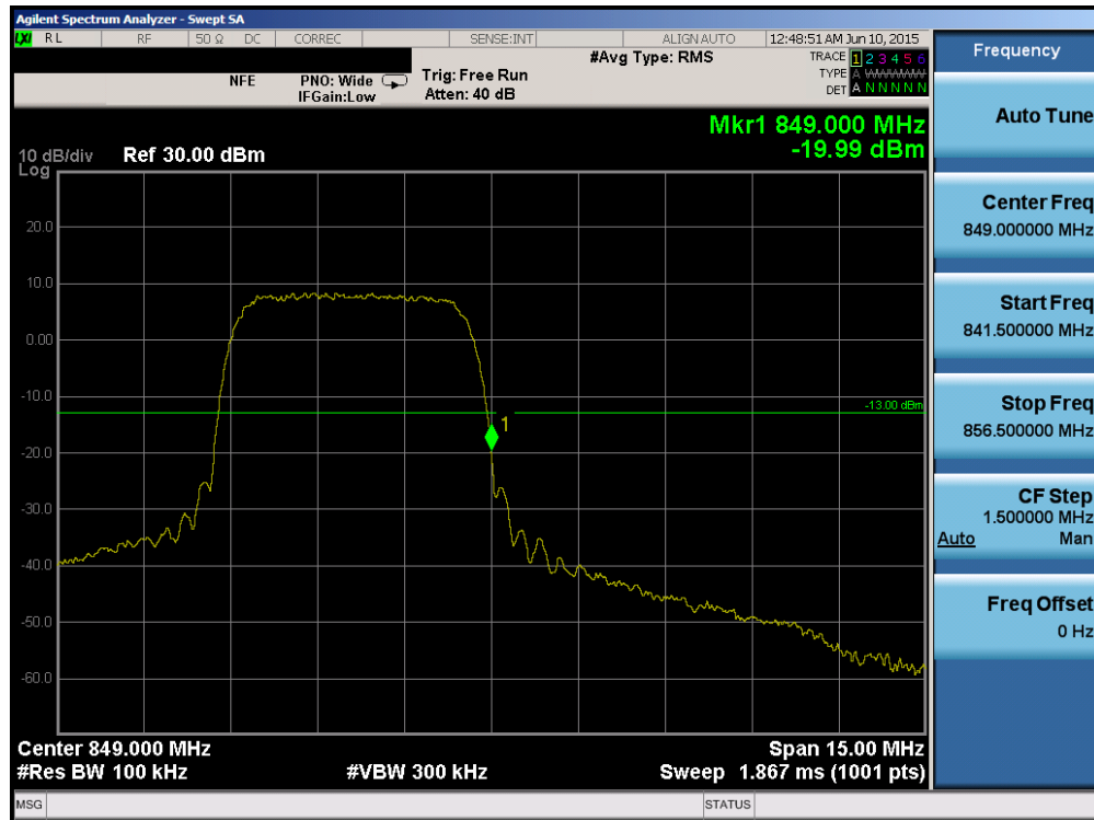
Plot 6-78. Band Edge Plot (Cellular WCDMA Mode – Ch. 4233)
