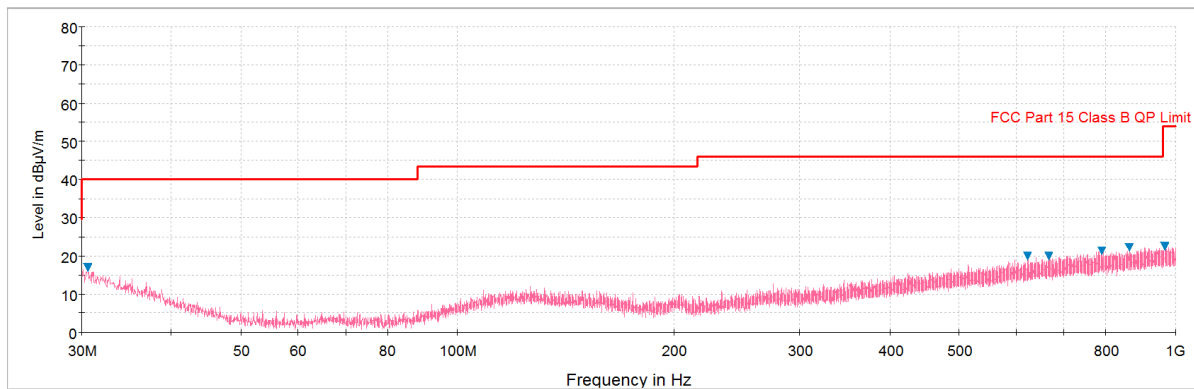
Plot 6-242. Radiated Spurious Plot below 1GHz (802.11a – U3 Ch. 157, Ant. Pol. V)
