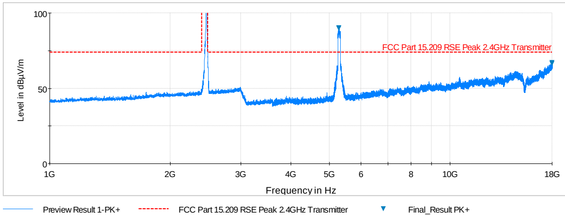
Plot 6-175. Radiated Spurious Plot above 1GHz (SIMULTANEOUS TX 5 GHz – 2.4 GHz, Ant. Pol. H)
