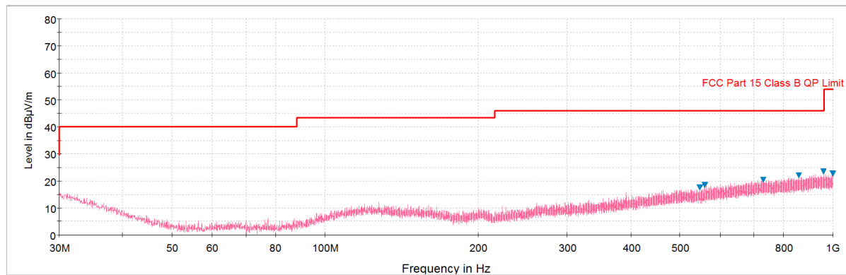
Plot 6-244. Radiated Spurious Plot below 1GHz (802.11a – U3 Ch. 157, Ant. Pol. V)
