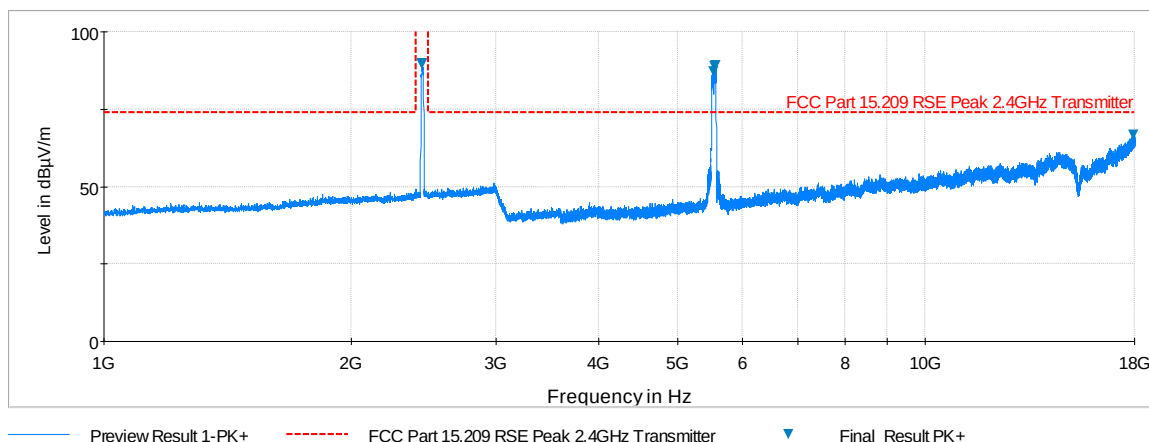
Plot 6-173. Radiated Spurious Plot above 1GHz (SIMULTANEOUS TX 2.4GHz – 5 GHz, Ant. Pol. H)
