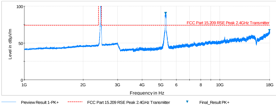
Plot 6-176. Radiated Spurious Plot above 1GHz (SIMULTANEOUS TX 5 GHz – 2.4 GHz, Ant. Pol. V)
