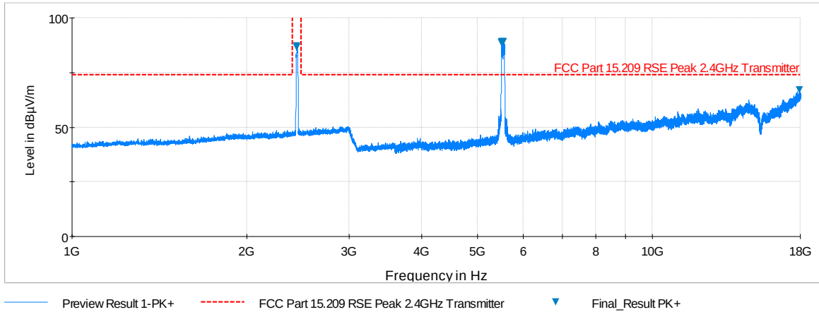
Plot 6-174. Radiated Spurious Plot above 1GHz (SIMULTANEOUS TX 2.4GHz – 5 GHz, Ant. Pol. V)
