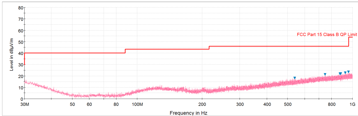
Plot 6-241. Radiated Spurious Plot below 1GHz (802.11a – U3 Ch. 157, Ant. Pol. H)
