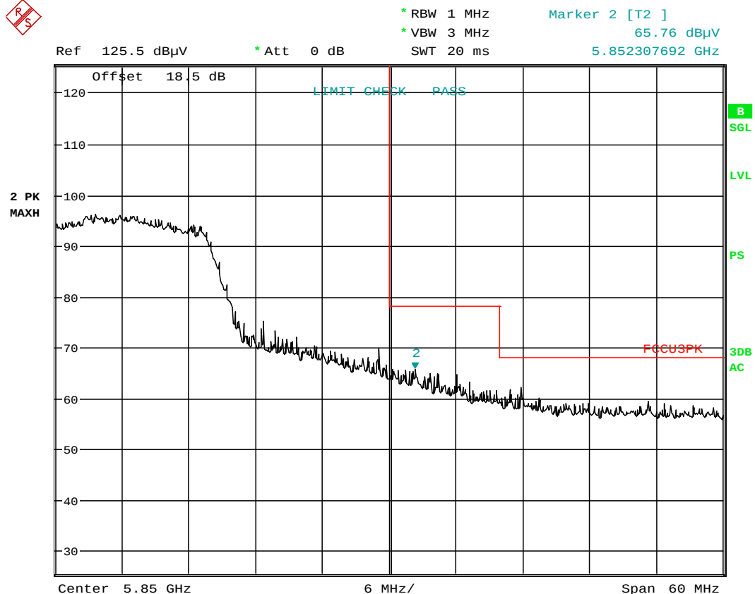
Plot 6-2. Radiated Restricted Upper Band Edge Plot (Peak – UNII Band 3)
