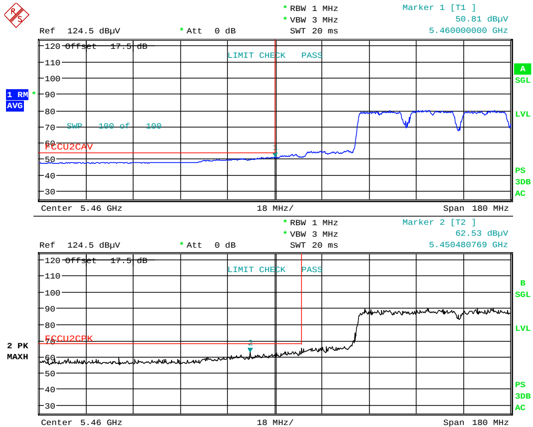
Plot 6-4. Radiated Restricted Lower Band Edge Plot (Average – UNII Band 2C)
