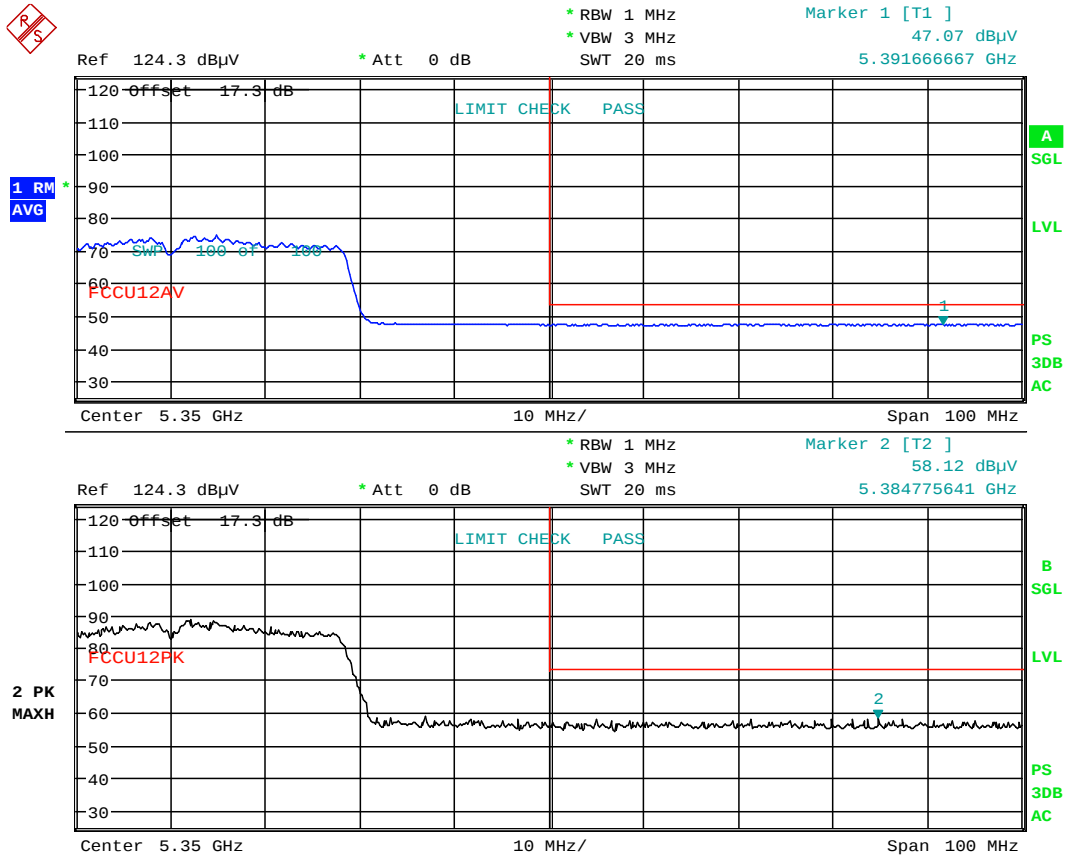
Plot 6-3. Radiated Restricted Upper Band Edge Plot (Average and Peak – UNII Band 2A)
