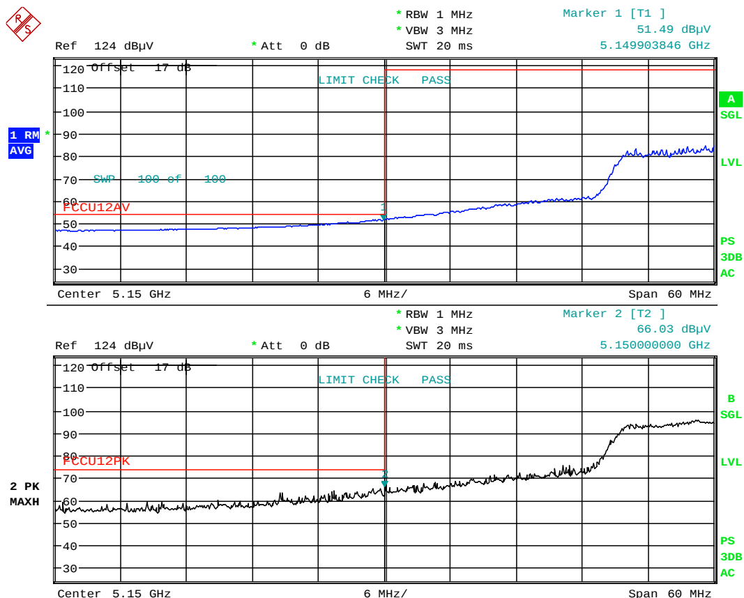
Plot 6-1. Radiated Restricted Lower Band Edge Plot (Average and Peak – UNII Band 1)
