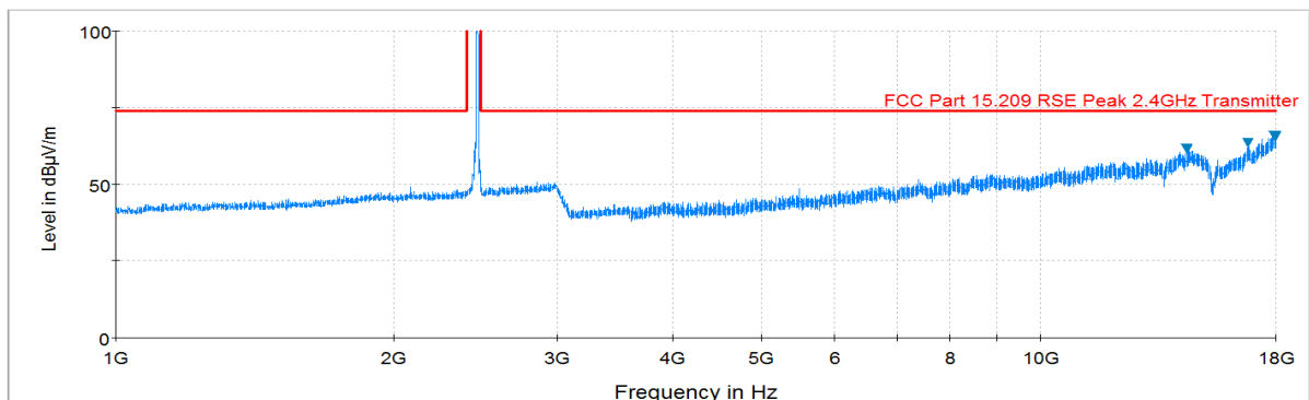
Plot 6-73. Radiated Spurious Plot above 1GHz (802.11b – Ch. 11, Ant. Pol. H)
