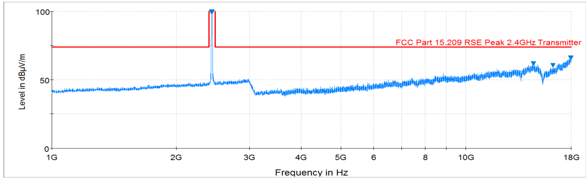
Plot 6-72. Radiated Spurious Plot above 1GHz (802.11b – Ch. 6, Ant. Pol. V)
