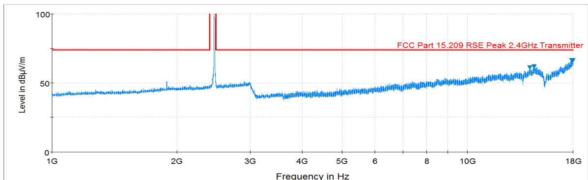
Plot 6-65. Radiated Spurious Plot above 1GHz (802.11b – Ch. 11, Ant. Pol. H)
