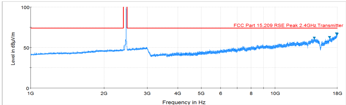
Plot 6-66. Radiated Spurious Plot above 1GHz (802.11b – Ch. 11, Ant. Pol. V)
