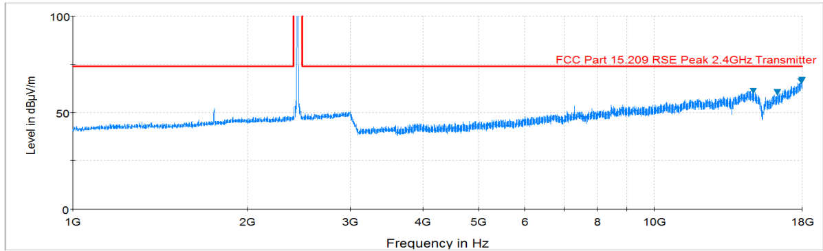
Plot 6-64. Radiated Spurious Plot above 1GHz (802.11b – Ch. 6, Ant. Pol. V)
