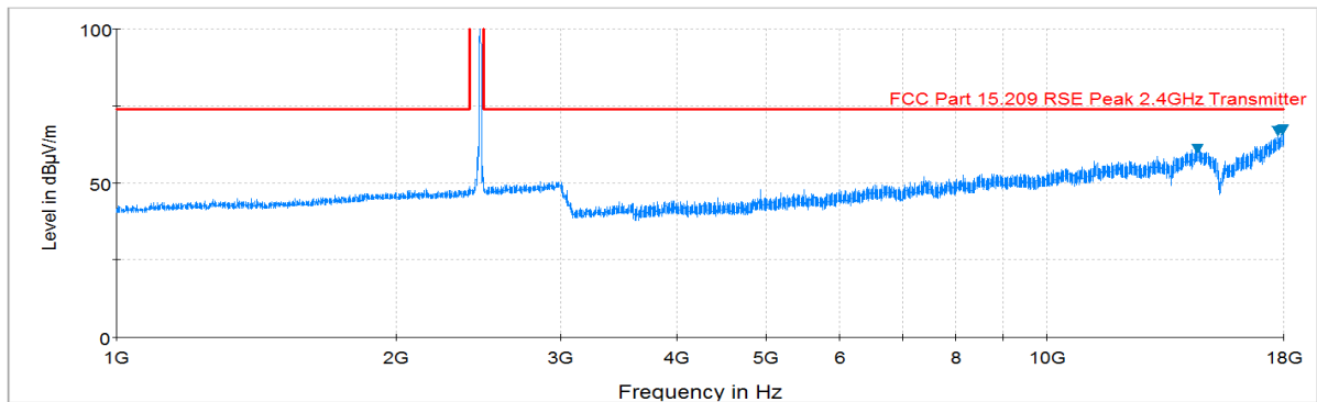
Plot 6-74. Radiated Spurious Plot above 1GHz (802.11b – Ch. 11, Ant. Pol. V)
