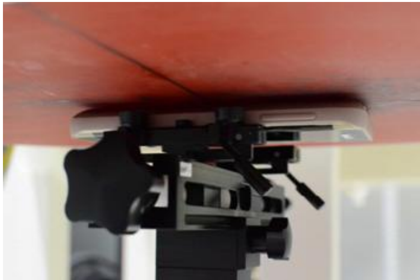
SAR Test Setup Photo 2- Back Side at 0.0 cm (Phablet)
