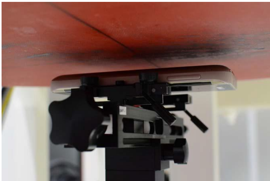
SAR Test Setup Photo 4 – Back Side at 1.5 cm (Body-worn)
