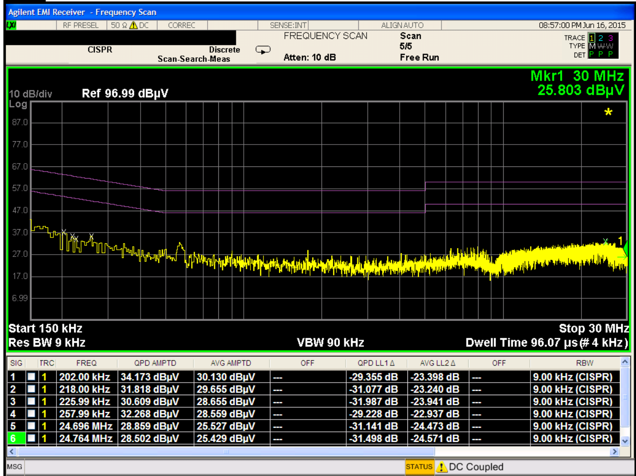
Plot 7-4. Line-Conducted Test Plot (N) – NF50Ohm Terminated Antenna
