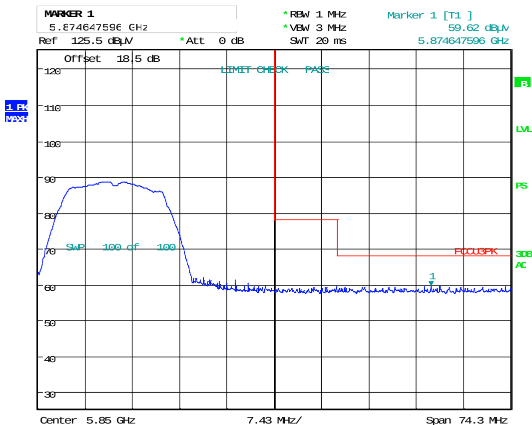
Plot 6-7. Radiated Upper Band Edge Plot (Peak – UNII Band 3)
