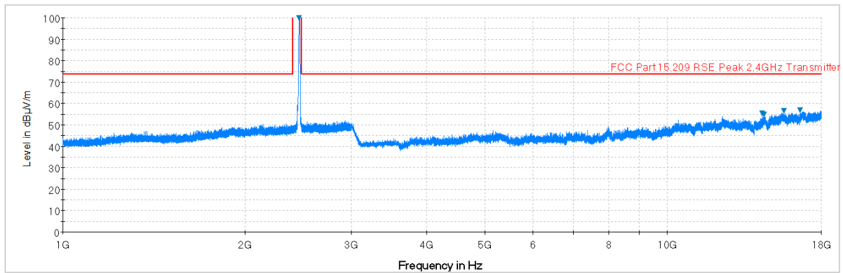
Plot 6-73. Radiated Spurious Plot above 1GHz (802.11b – Ch. 11, Ant. Pol. H)
