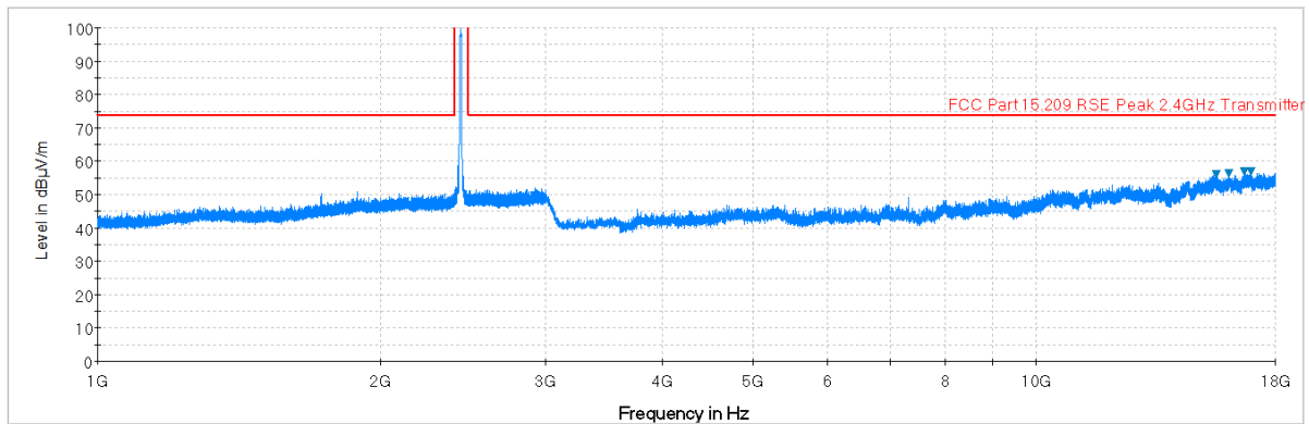
Plot 6-71. Radiated Spurious Plot above 1GHz (802.11b – Ch. 6, Ant. Pol. H)
