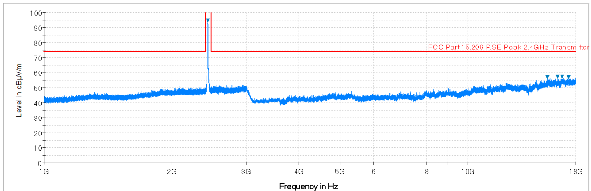
Plot 6-63. Radiated Spurious Plot above 1GHz (802.11b – Ch. 6, Ant. Pol. H)
