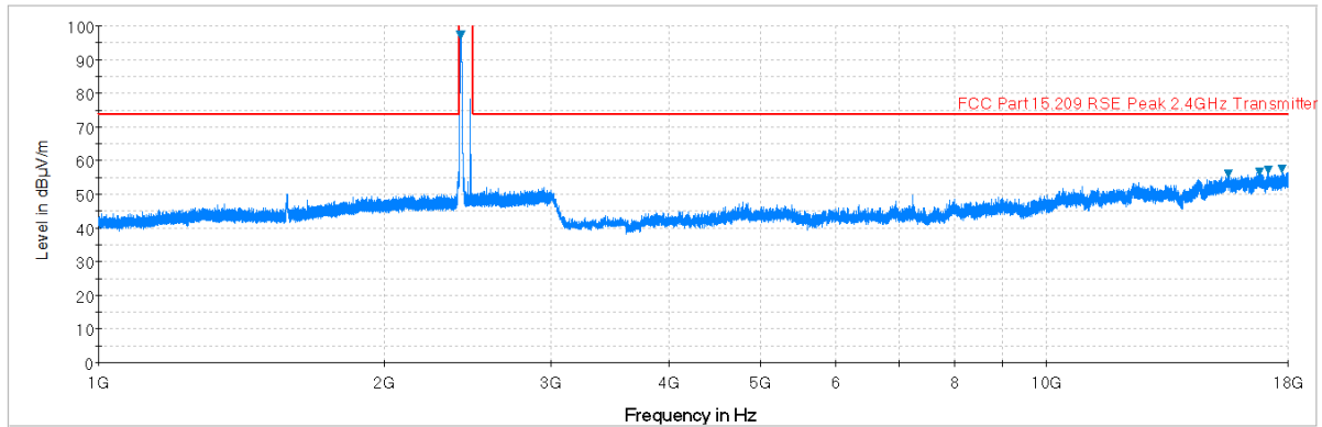
Plot 6-70. Radiated Spurious Plot above 1GHz (802.11b – Ch. 1, Ant. Pol. V)
