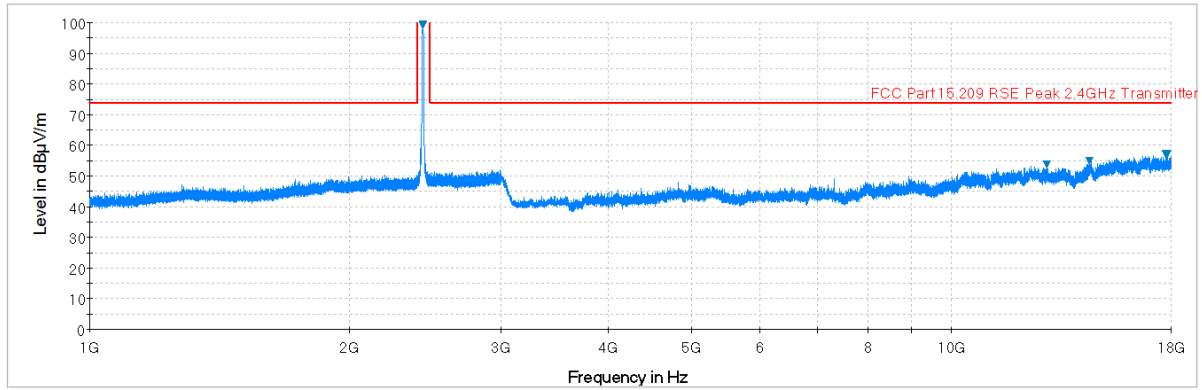
Plot 6-72. Radiated Spurious Plot above 1GHz (802.11b – Ch. 6, Ant. Pol. V)
