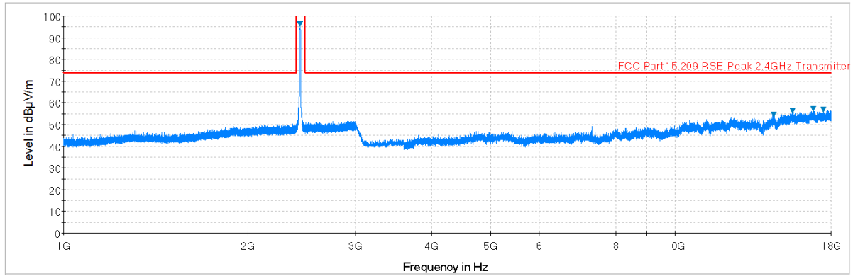
Plot 6-64. Radiated Spurious Plot above 1GHz (802.11b – Ch. 6, Ant. Pol. V)
