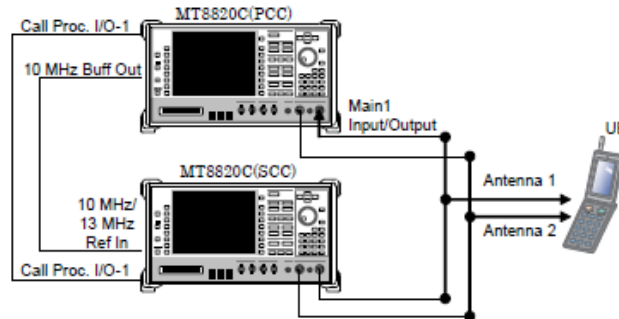
Figure 9-4 Power Measurement Setup
