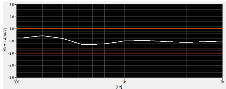
Figure 8-7 Helmholtz Coil Validation for Frequency Response
