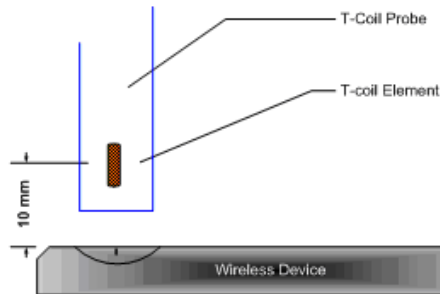
Figure 5-10 Measurement Distance
