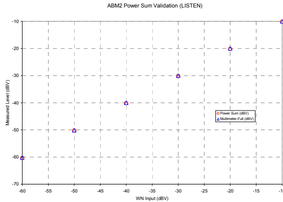
Figure 5-9 ABM2 Power Sum Validation
