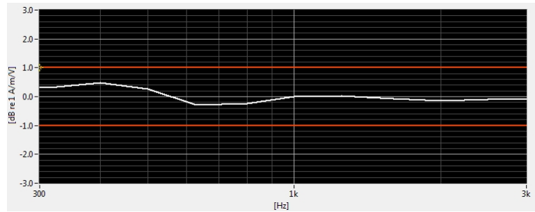
Figure 8-6 Helmholtz Coil Validation for Frequency Response
