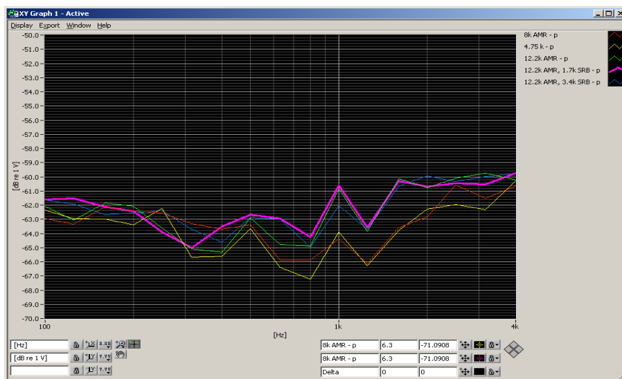
Figure 7-2 UMTS Audio Band Magnetic Noise
