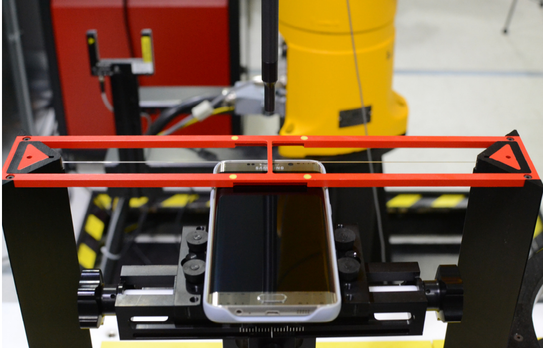
Figure 15-1 Ear Reference Point HAC Phantom Alignment
