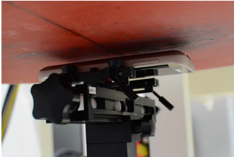
SAR Test Setup Photo 2 – Back Side at 1.0 cm (Hotspot)
