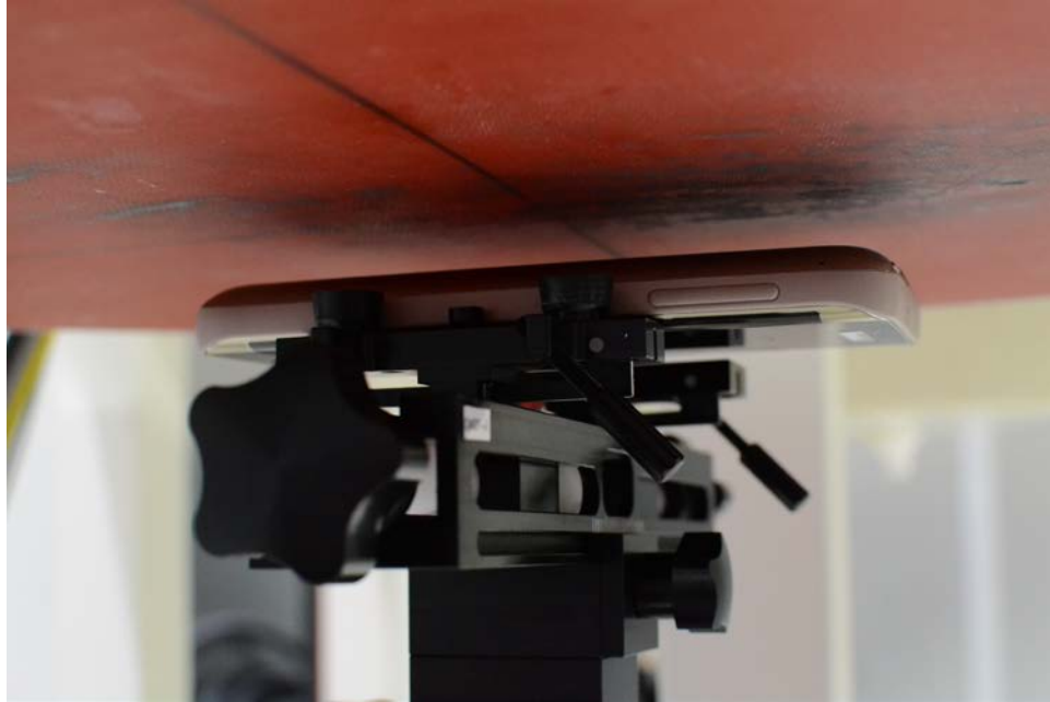
SAR Test Setup Photo 3 – Back Side at 1.5 cm (Body-worn)
