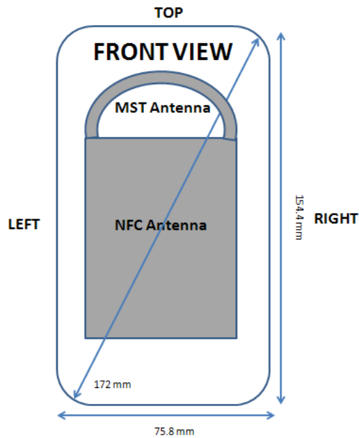
Figure F-1 DUT Antenna Locations
