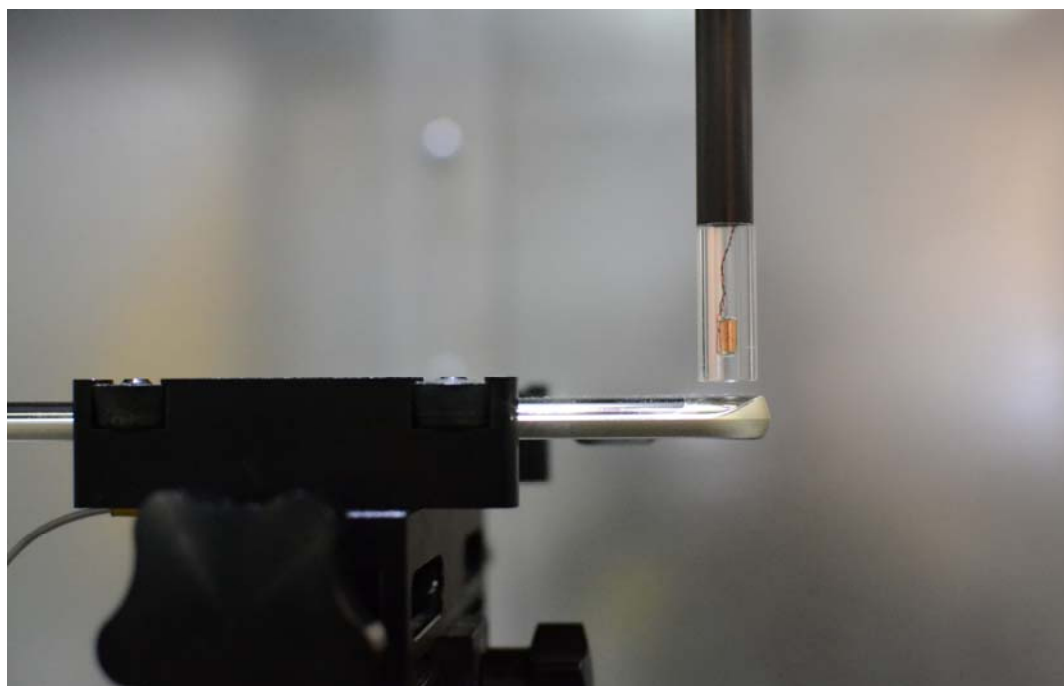
Figure 14-2 Test Setup for Wireless Device
