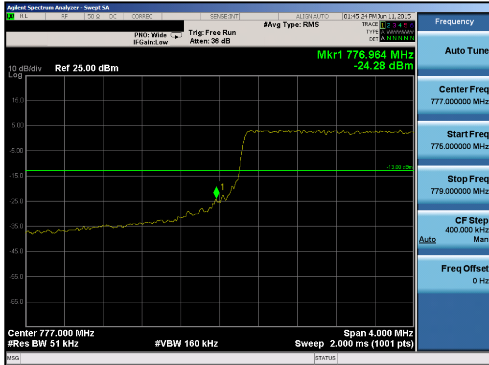
Plot 6-111. Lower Band Edge Plot (Band 13 – 5.0MHz QPSK – RB Size 25)
