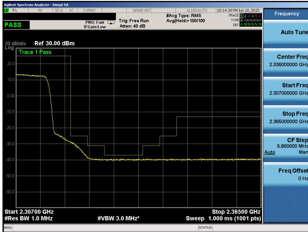
Plot 6-187. Upper Extended Band Edge Plot (Band 30 – 10.0MHz QPSK – RB Size 50)
