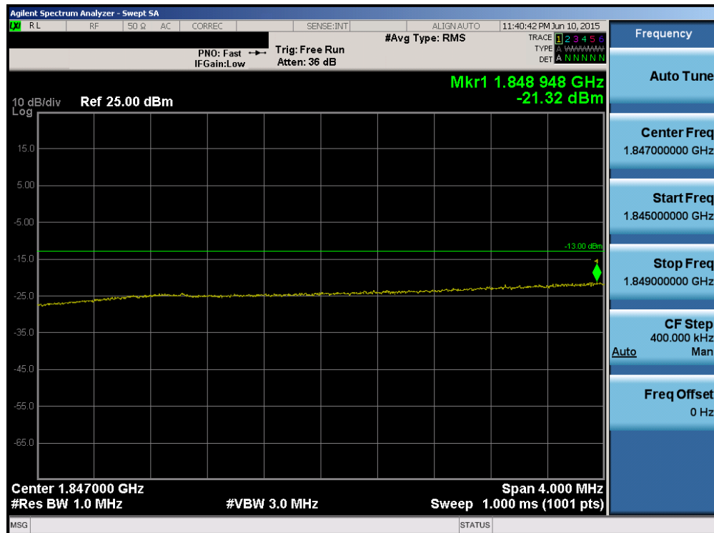
Plot 6-172. Lower Extended Band Edge Plot (Band 2 – 15.0MHz QPSK – RB Size 75)
