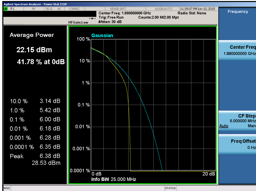
Plot 6-197. PAR Plot (Band 2 – 15.0MHz 16-QAM – RB Size 75)
