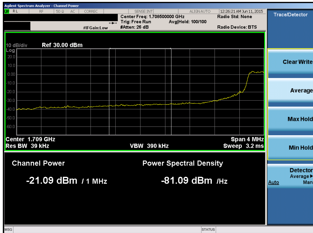
Plot 6-140. Lower Extended Band Edge Plot (Band 4 – 5.0MHz QPSK – RB Size 25)
