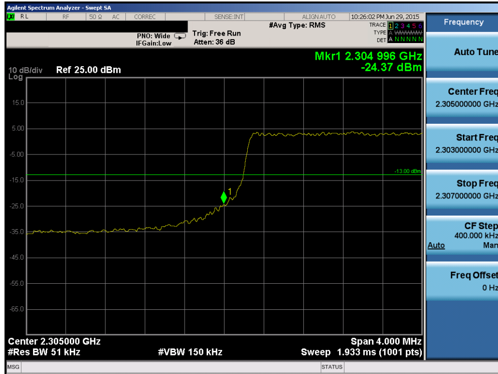
Plot 6-179. Lower Band Edge Plot (Band 30 – 5.0MHz QPSK – RB Size 25)
