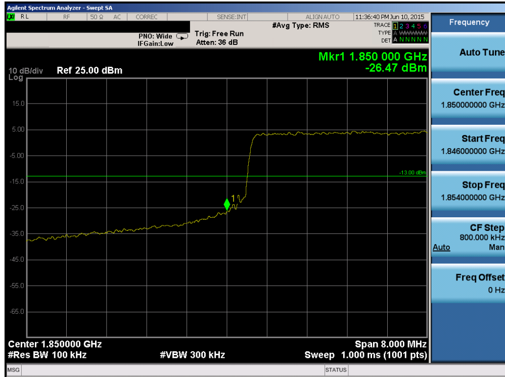
Plot 6-167. Lower Band Edge Plot (Band 2 – 10.0MHz QPSK – RB Size 50)
