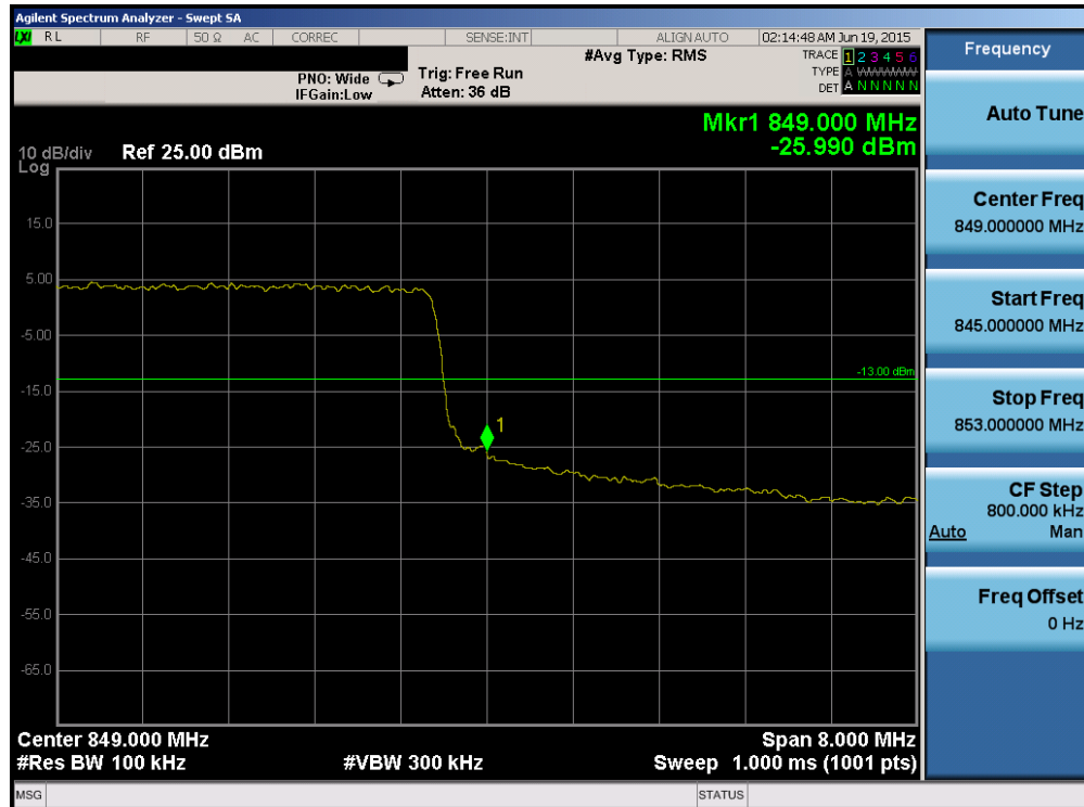
Plot 6-130. Upper Band Edge Plot (Band 5 – 10.0MHz QPSK – RB Size 50)
