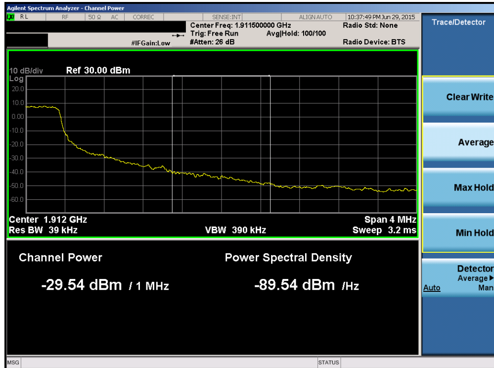
Plot 6-158. Upper Extended Band Edge Plot (Band 2 – 1.4MHz QPSK – RB Size 6)
