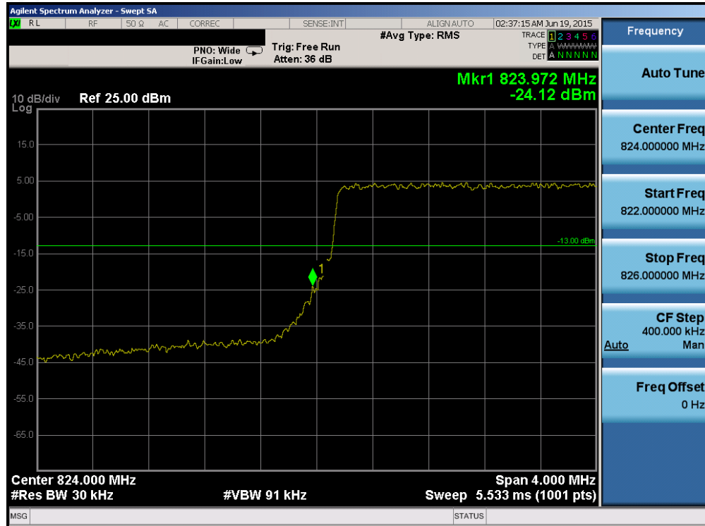
Plot 6-121. Lower Band Edge Plot (Band 5 – 3.0MHz QPSK – RB Size 15)
