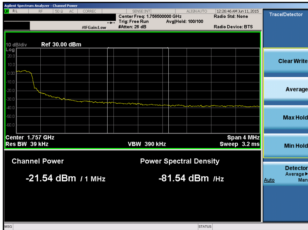
Plot 6-142. Upper Extended Band Edge Plot (Band 4 – 5.0MHz QPSK – RB Size 25)
