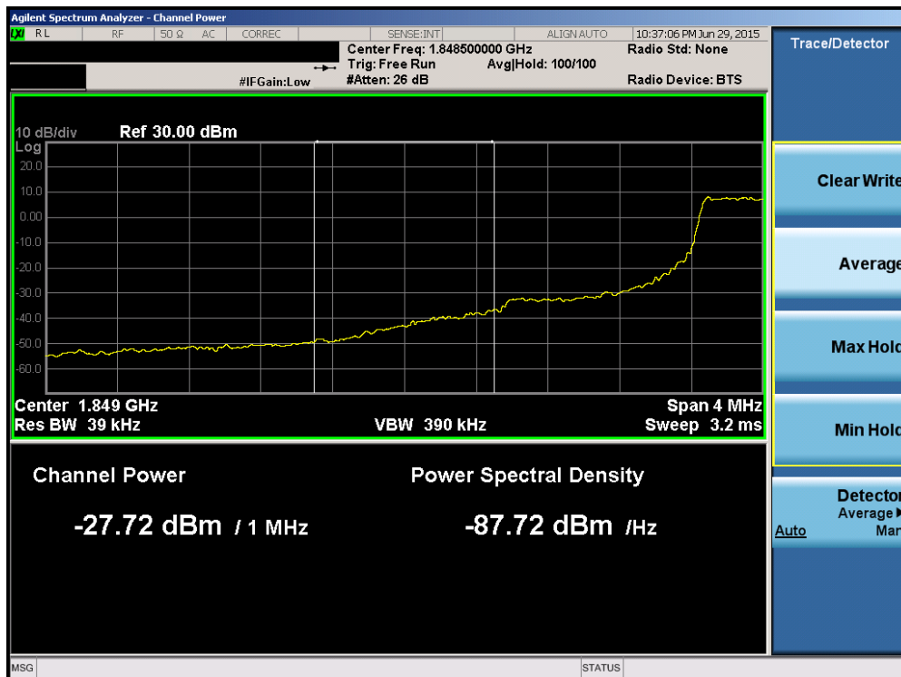
Plot 6-156. Lower Extended Band Edge Plot (Band 2 – 1.4MHz QPSK – RB Size 6)
