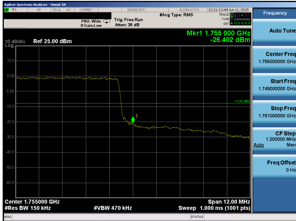
Plot 6-149. Upper Band Edge Plot (Band 4 – 15.0MHz QPSK – RB Size 75)
