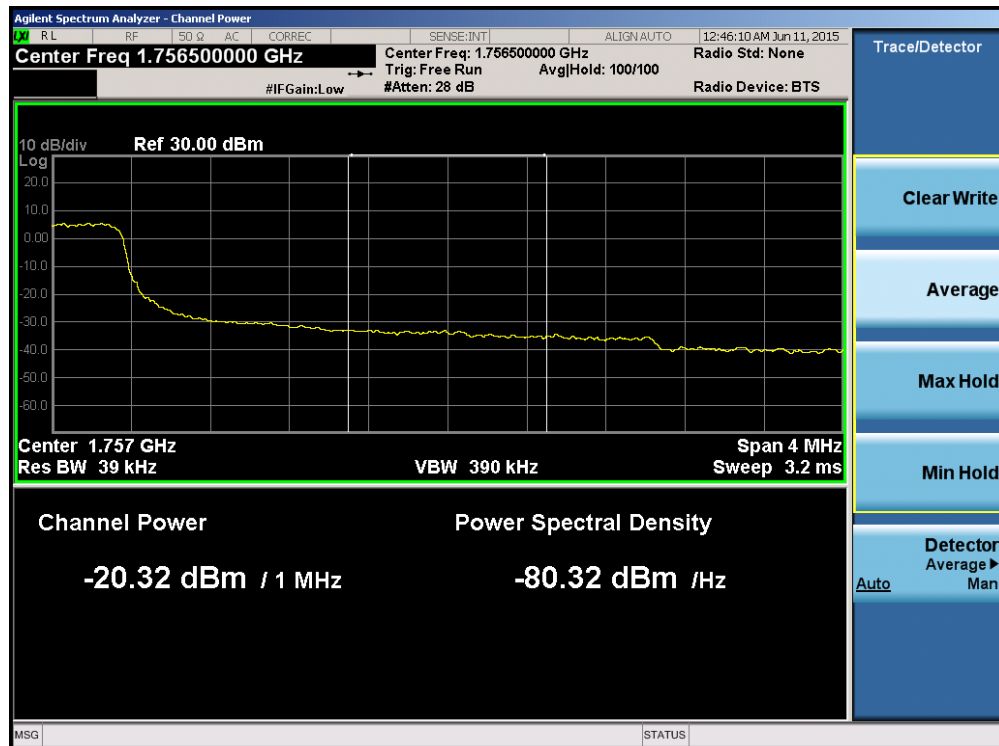
Plot 6-138. Upper Extended Band Edge Plot (Band 4 – 3.0MHz QPSK – RB Size 15)
