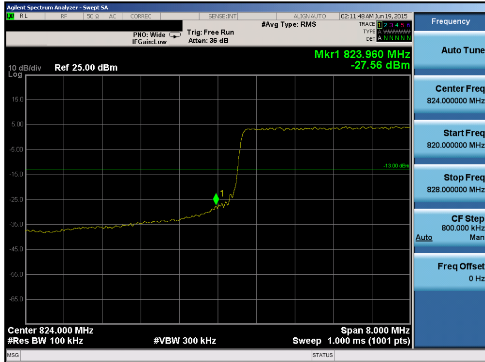
Plot 6-129. Lower Band Edge Plot (Band 5 – 10.0MHz QPSK – RB Size 50)
