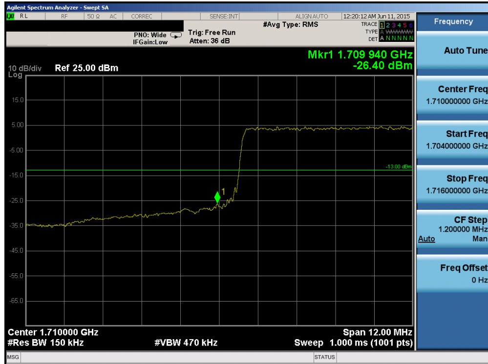
Plot 6-147. Lower Band Edge Plot (Band 4 – 15.0MHz QPSK – RB Size 75)
