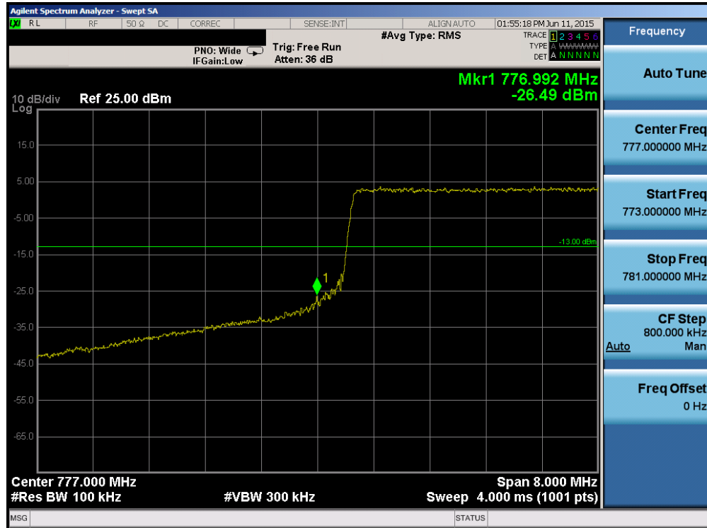
Plot 6-115. Lower Band Edge Plot (Band 13 – 10.0MHz QPSK – RB Size 50)
