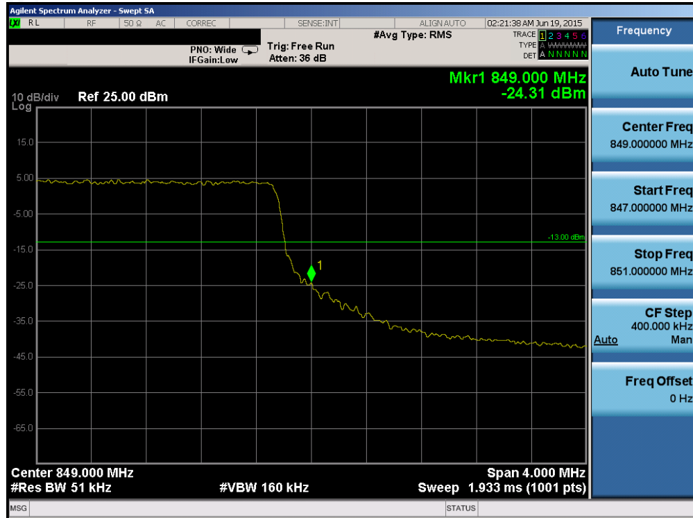
Plot 6-127. Upper Band Edge Plot (Band 5 – 5.0MHz QPSK – RB Size 25)
