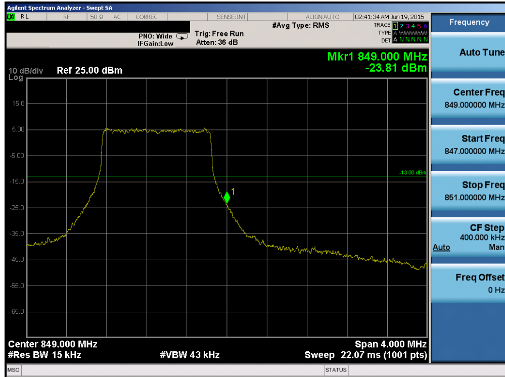
Plot 6-119. Upper Band Edge Plot (Band 5 – 1.4MHz QPSK – RB Size 6)
