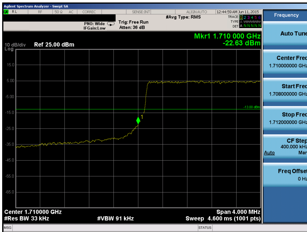
Plot 6-135. Lower Band Edge Plot (Band 4 – 3.0MHz QPSK – RB Size 15)
