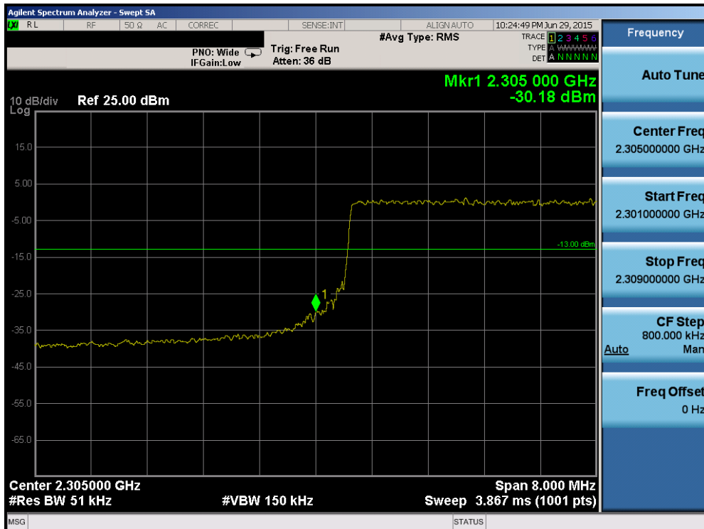
Plot 6-184. Lower Band Edge Plot (Band 30 – 10.0MHz QPSK – RB Size 50)
