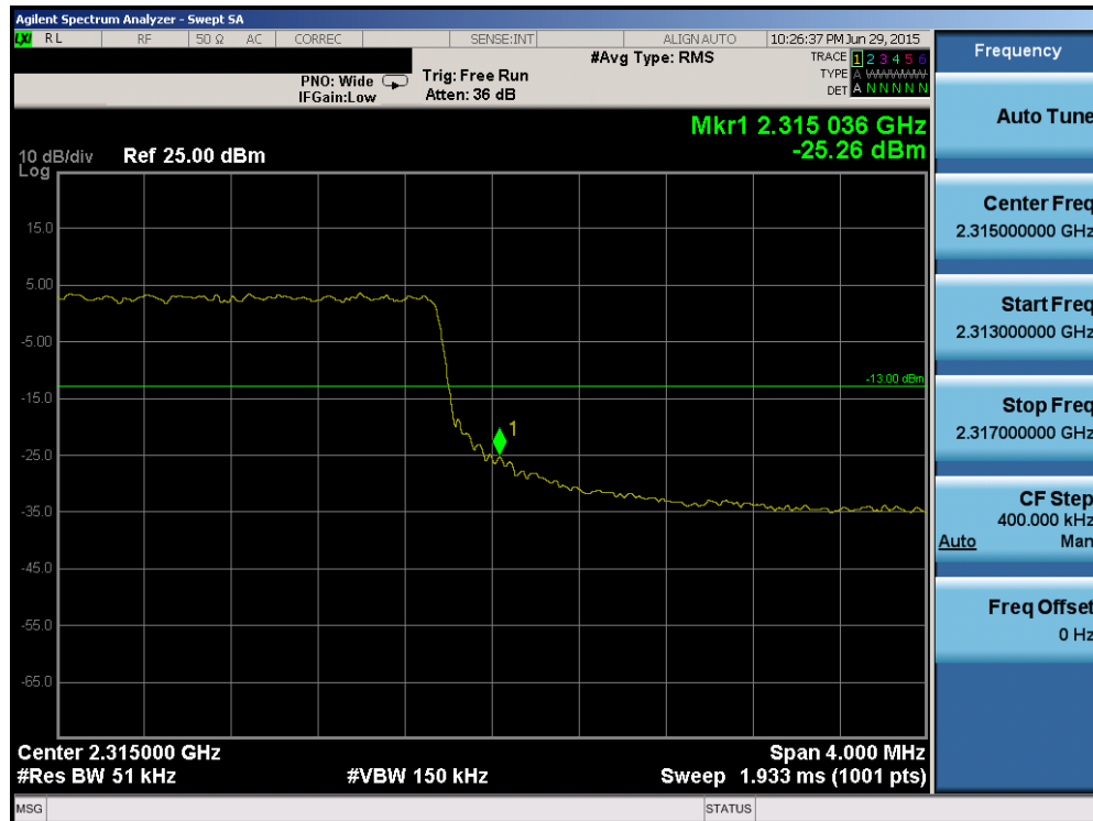
Plot 6-182. Upper Band Edge Plot (Band 30 – 5.0MHz QPSK – RB Size 25)
