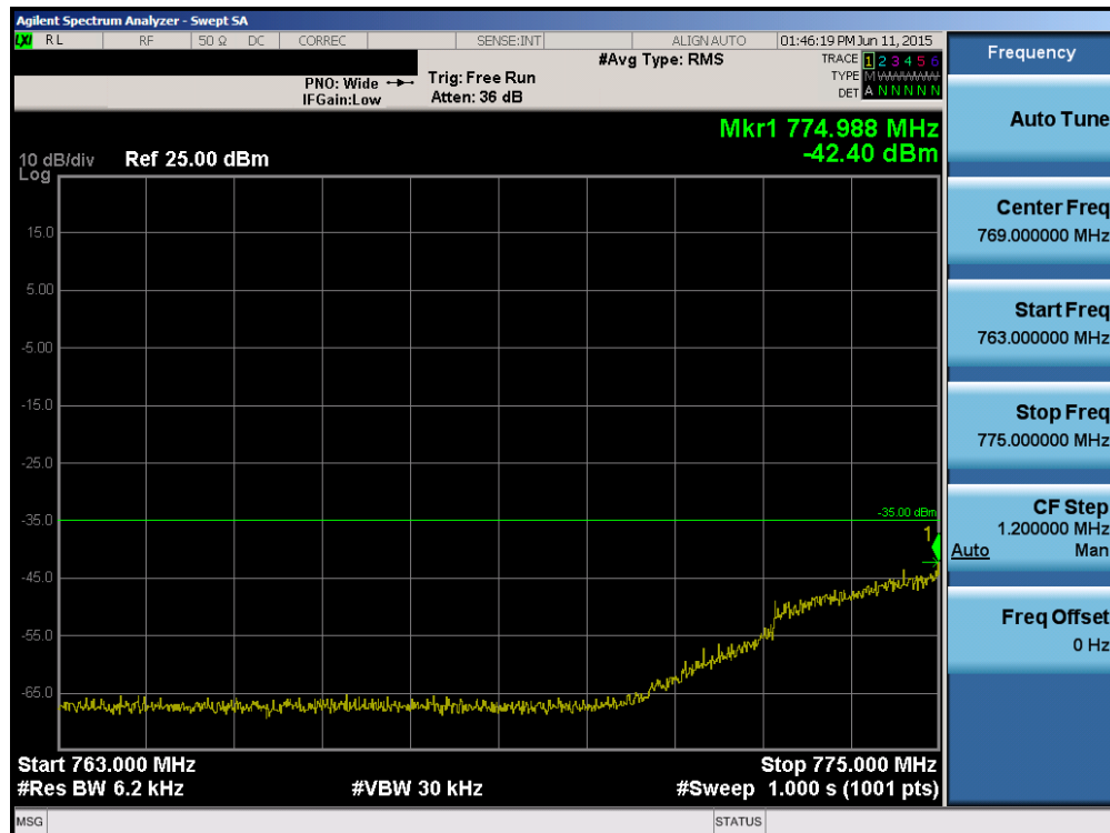
Plot 6-112. Lower Emission Mask Edge Plot (Band 13 – 5.0MHz QPSK – RB Size 25)
