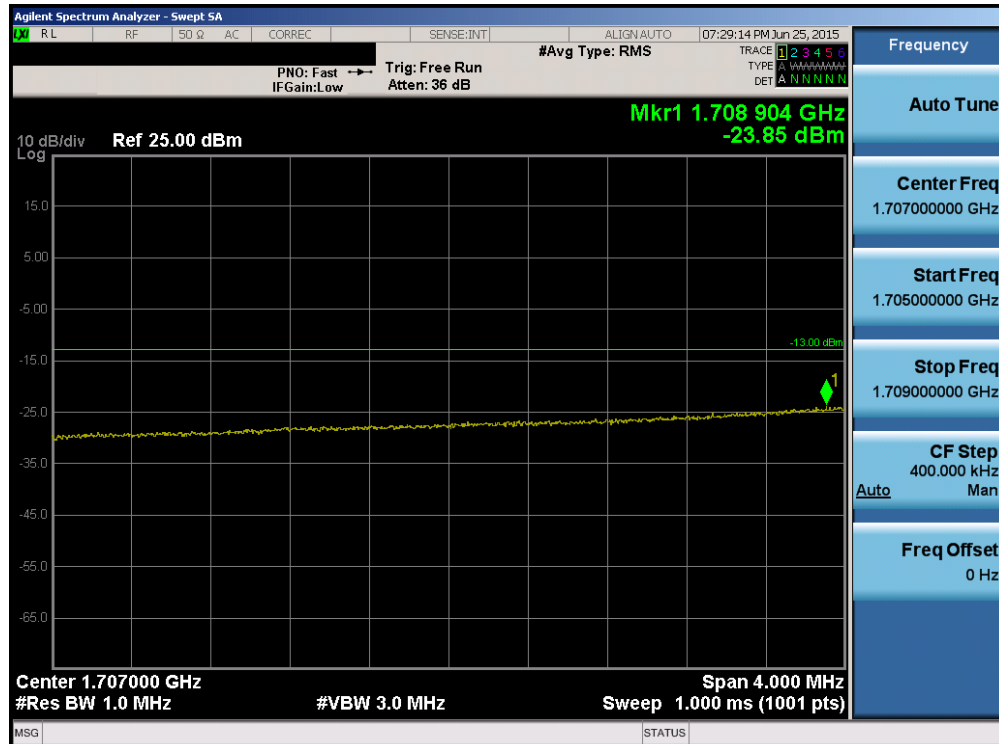
Plot 6-152. Lower Extended Band Edge Plot (Band 4 – 20.0MHz QPSK – RB Size 100)
