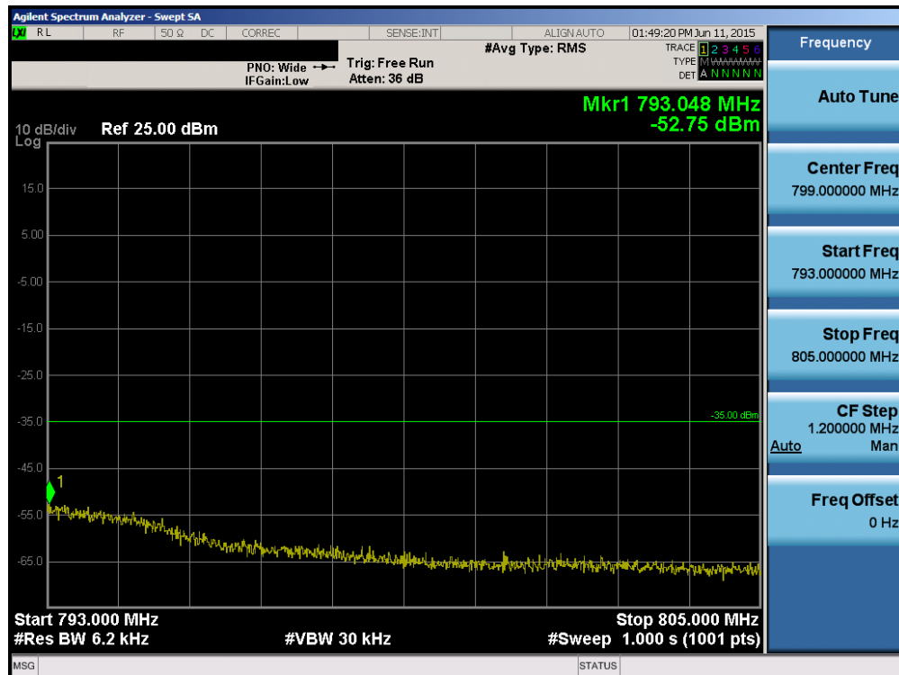
Plot 6-114. Upper Emission Mask Edge Plot (Band 13 – 5.0MHz QPSK – RB Size 25)
