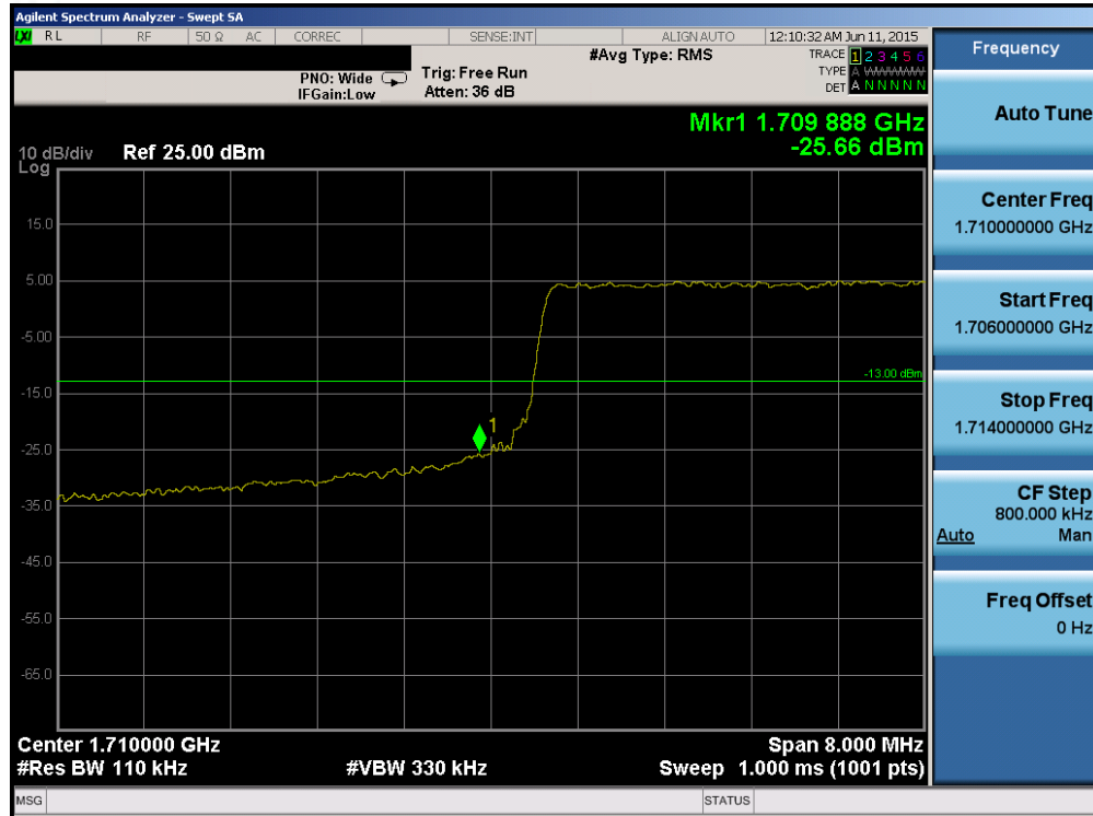
Plot 6-143. Lower Band Edge Plot (Band 4 – 10.0MHz QPSK – RB Size 50)
