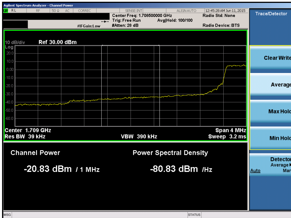
Plot 6-136. Lower Extended Band Edge Plot (Band 4 – 3.0MHz QPSK – RB Size 15)
