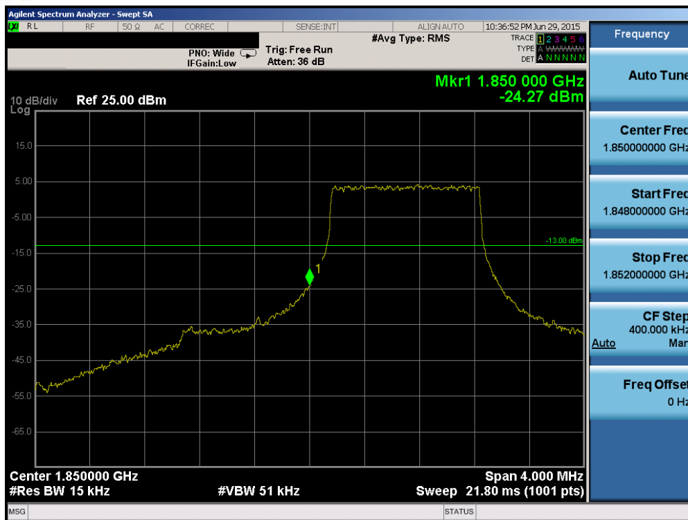
Plot 6-155. Lower Band Edge Plot (Band 2 – 1.4MHz QPSK – RB Size 6)
