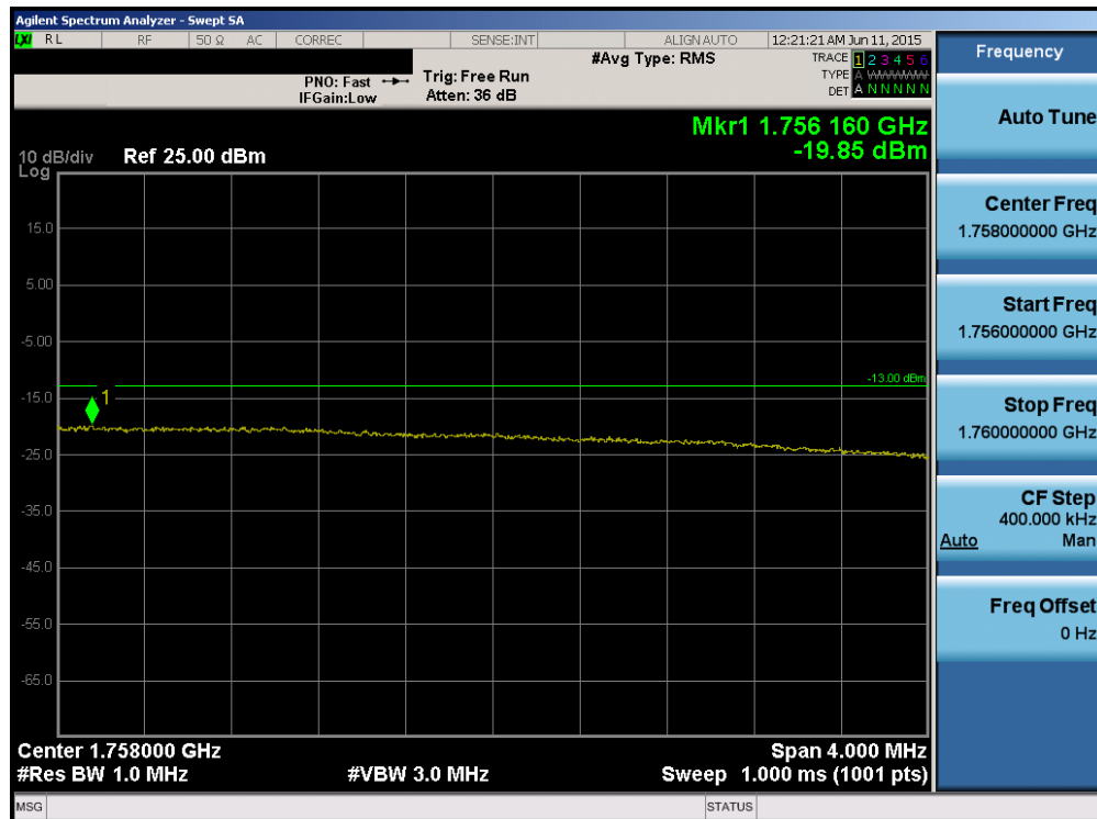
Plot 6-150. Upper Extended Band Edge Plot (Band 4 – 15.0MHz QPSK – RB Size 75)
