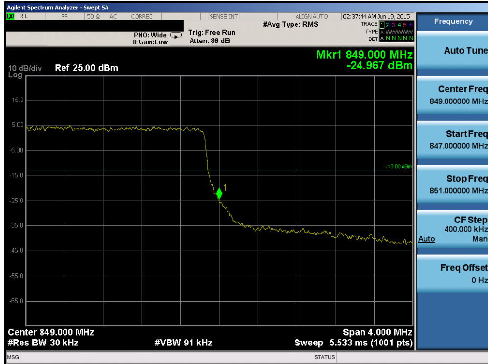
Plot 6-123. Upper Band Edge Plot (Band 5 – 3.0MHz QPSK – RB Size 15)
