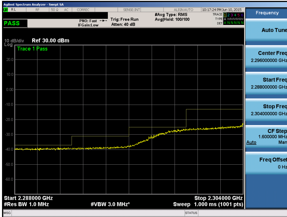
Plot 6-185. Lower Extended Band Edge Plot (Band 30 – 10.0MHz QPSK – RB Size 50)
