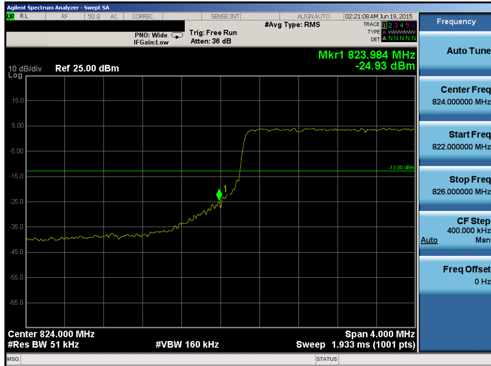
Plot 6-125. Lower Band Edge Plot (Band 5 – 5.0MHz QPSK – RB Size 25)
