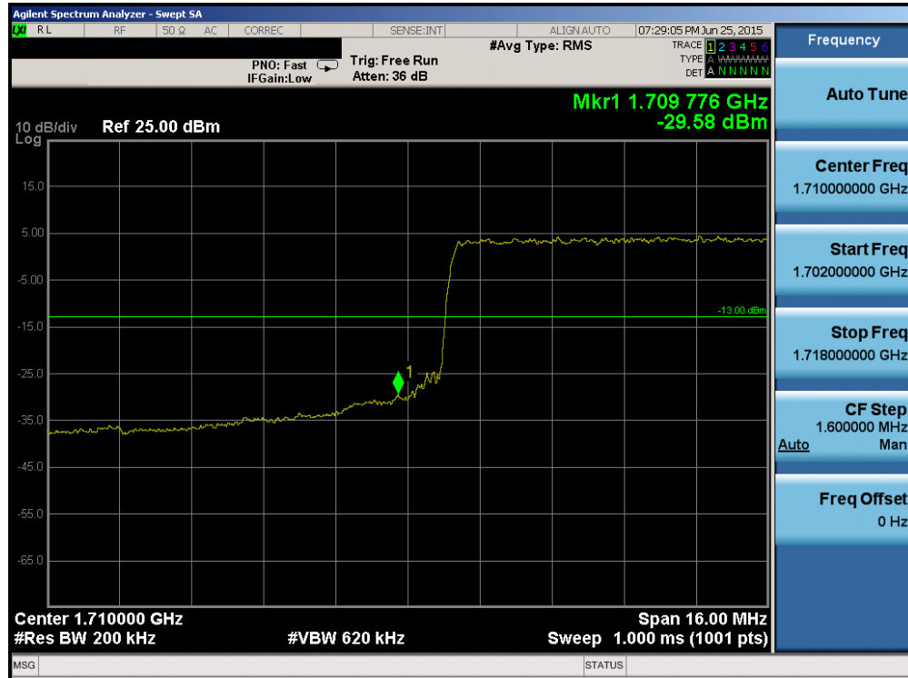
Plot 6-151. Lower Band Edge Plot (Band 4 – 20.0MHz QPSK – RB Size 100)
