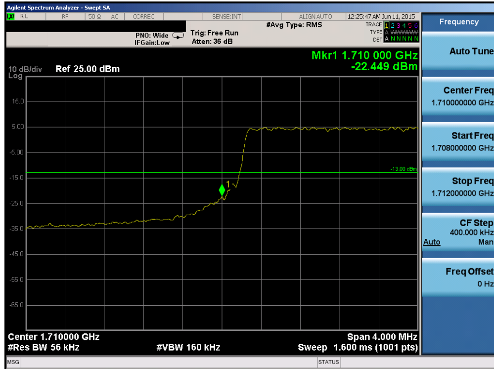
Plot 6-139. Lower Band Edge Plot (Band 4 – 5.0MHz QPSK – RB Size 25)
