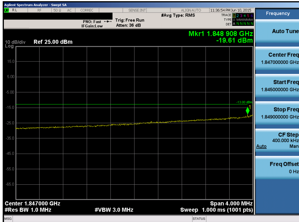
Plot 6-168. Lower Extended Band Edge Plot (Band 2 – 10.0MHz QPSK – RB Size 50)
