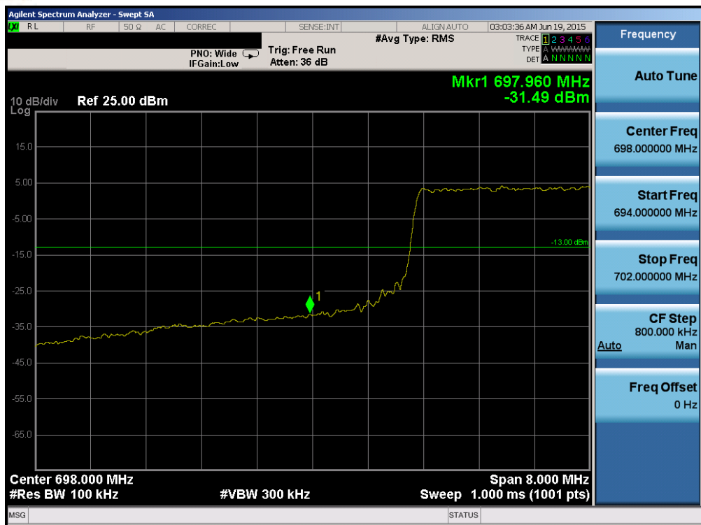
Plot 6-109. Lower Band Edge Plot (Band 12/17 - 10.0MHz QPSK - RB Size 50)
