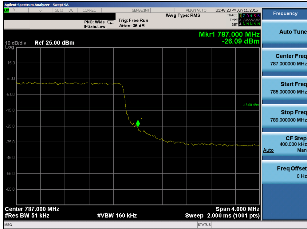
Plot 6-113. Upper Band Edge Plot (Band 13 – 5.0MHz QPSK – RB Size 25)
