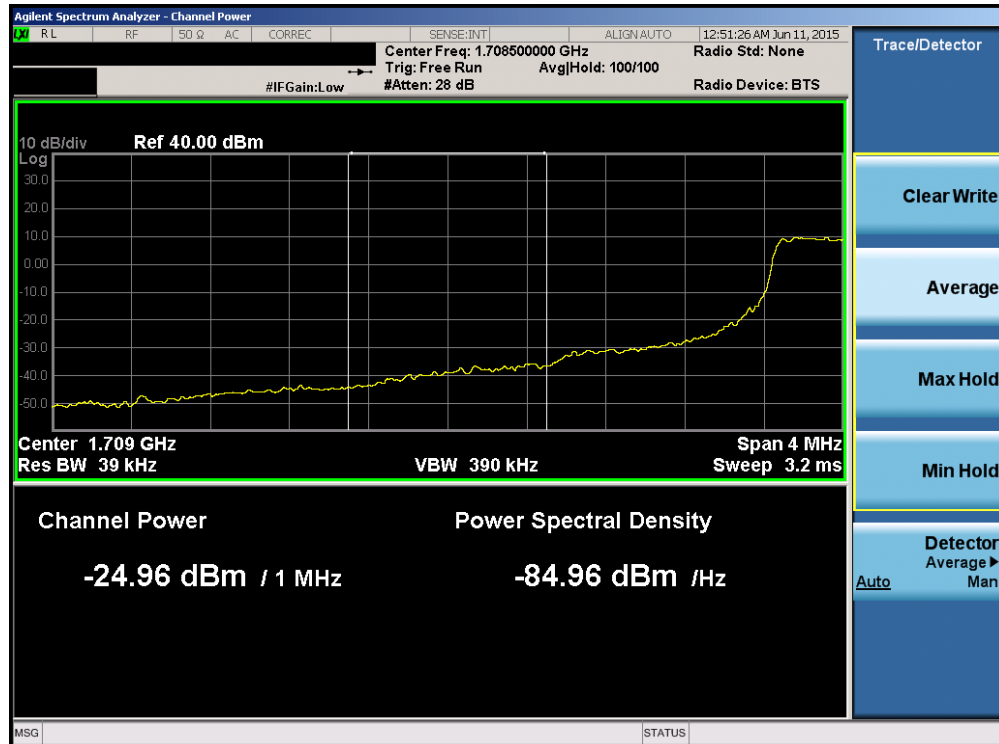
Plot 6-132. Lower Extended Band Edge Plot (Band 4 – 1.4MHz QPSK – RB Size 6)
