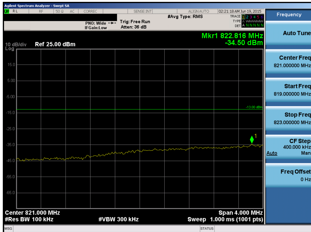
Plot 6-126. Lower Extended Band Edge Plot (Band 5 – 5.0MHz QPSK – RB Size 25)
