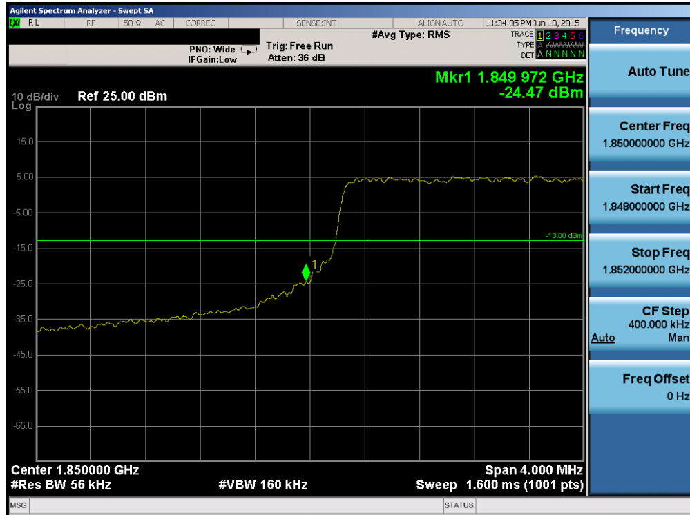
Plot 6-163. Lower Band Edge Plot (Band 2 – 5.0MHz QPSK – RB Size 25)
