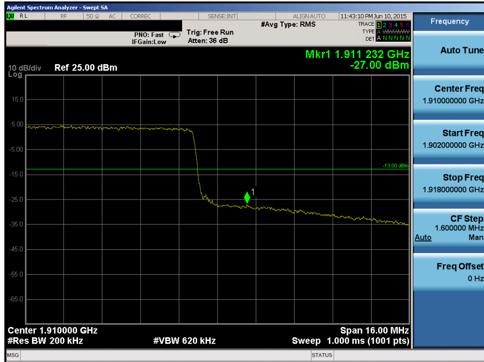
Plot 6-177. Upper Band Edge Plot (Band 2 – 20.0MHz QPSK – RB Size 100)
