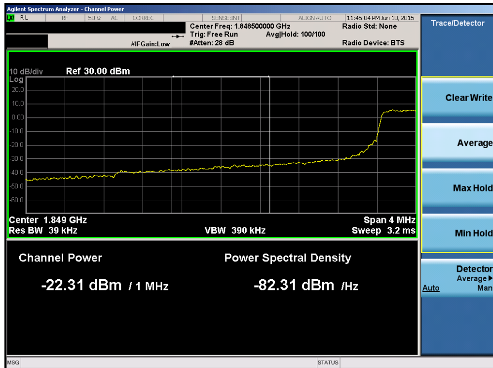
Plot 6-160. Lower Extended Band Edge Plot (Band 2 – 3.0MHz QPSK – RB Size 15)
