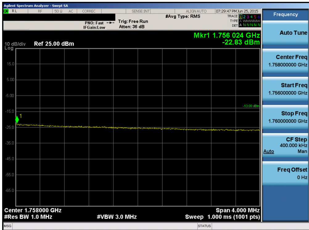
Plot 6-154. Upper Extended Band Edge Plot (Band 4 – 20.0MHz QPSK – RB Size 100)
