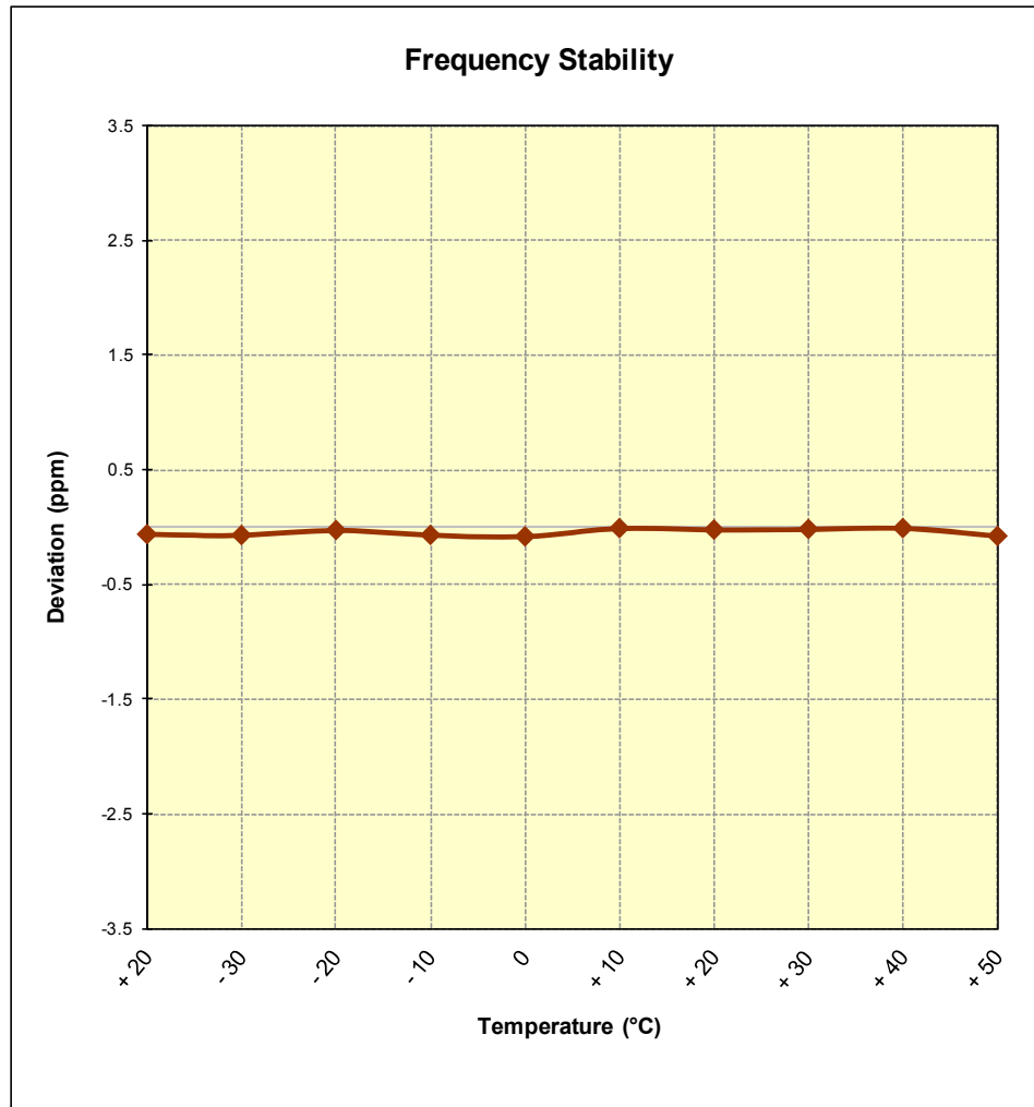
Figure 6-12. Frequency Stability Graph (Band 30)
