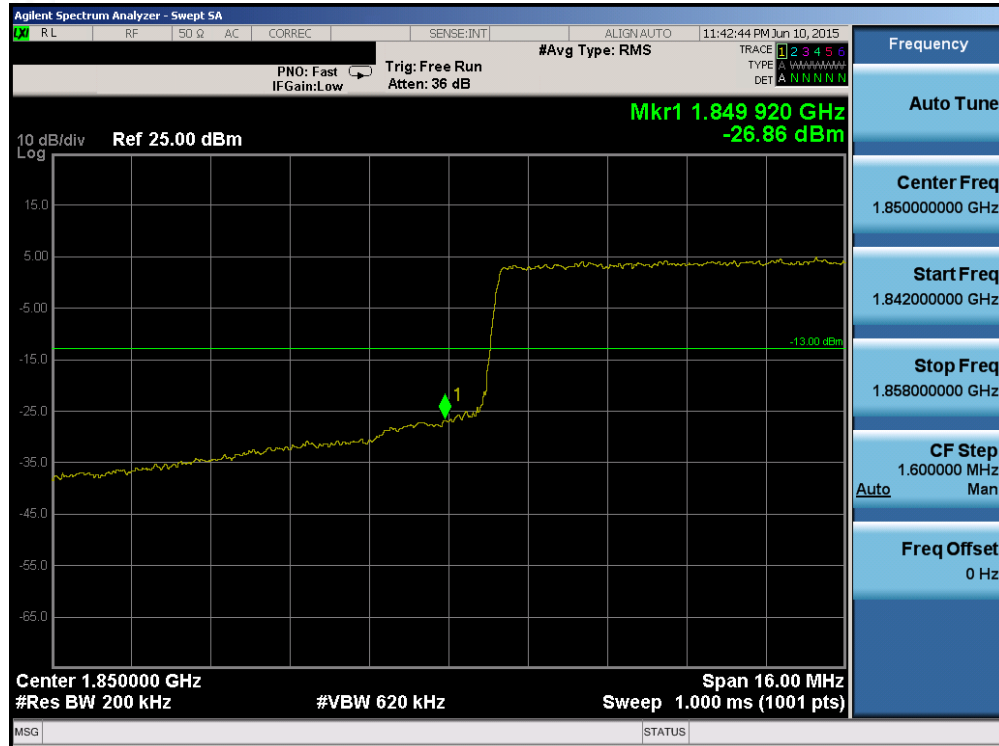
Plot 6-175. Lower Band Edge Plot (Band 2 – 20.0MHz QPSK – RB Size 100)
