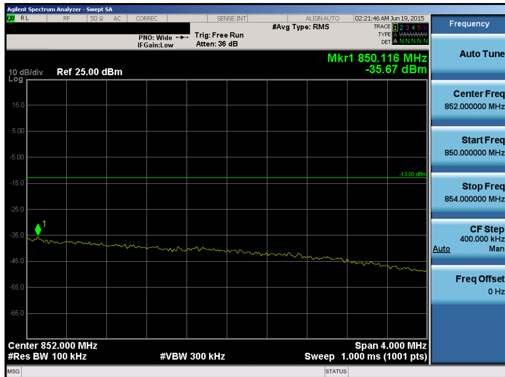
Plot 6-128. Upper Extended Band Edge Plot (Band 5 – 5.0MHz QPSK – RB Size 25)
