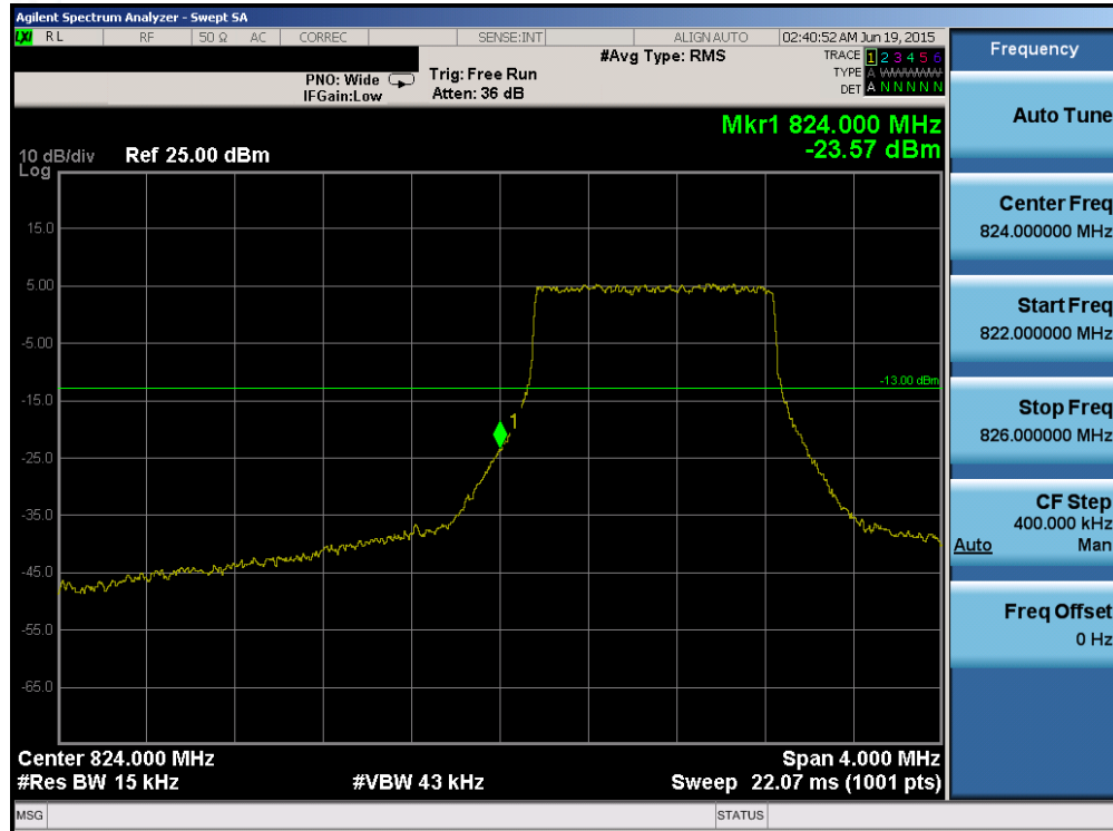
Plot 6-117. Lower Band Edge Plot (Band 5 – 1.4MHz QPSK – RB Size 6)
