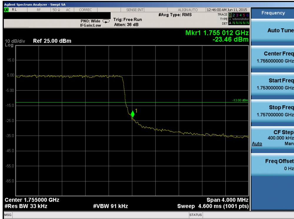
Plot 6-137. Upper Band Edge Plot (Band 4 – 3.0MHz QPSK – RB Size 15)
