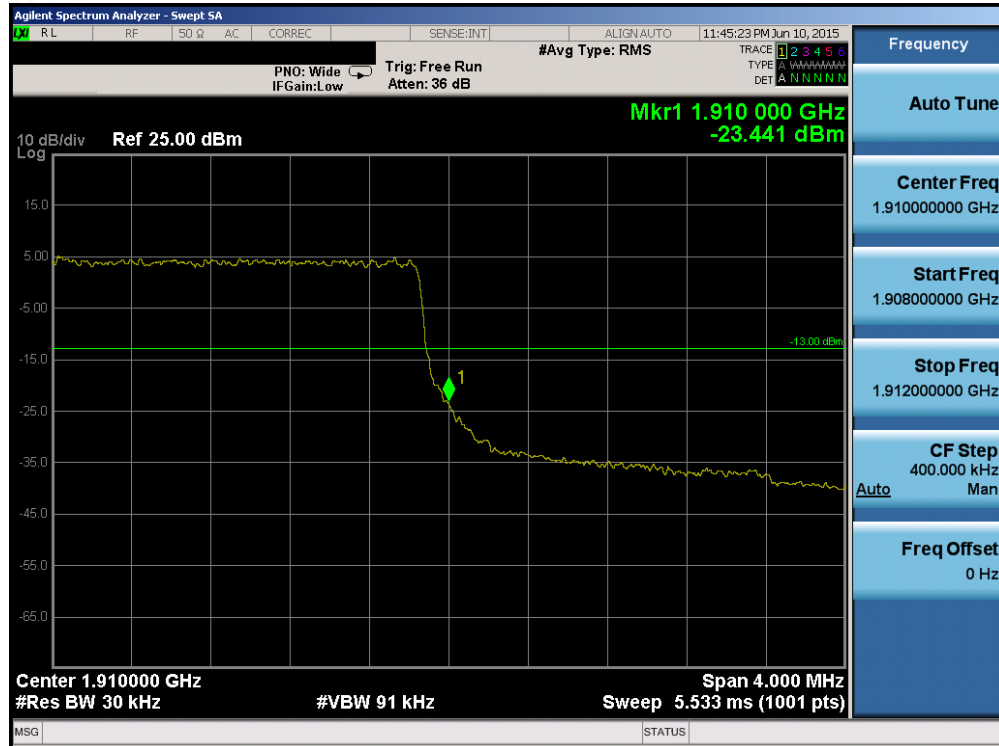
Plot 6-161. Upper Band Edge Plot (Band 2 – 3.0MHz QPSK – RB Size 15)
