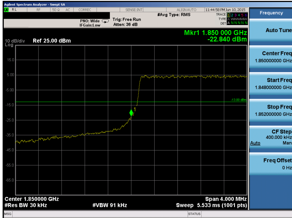
Plot 6-159. Lower Band Edge Plot (Band 2 – 3.0MHz QPSK – RB Size 15)
