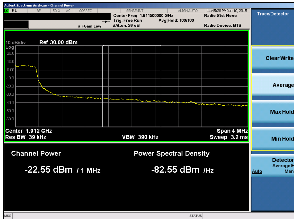
Plot 6-162. Upper Extended Band Edge Plot (Band 2 – 3.0MHz QPSK – RB Size 15)
