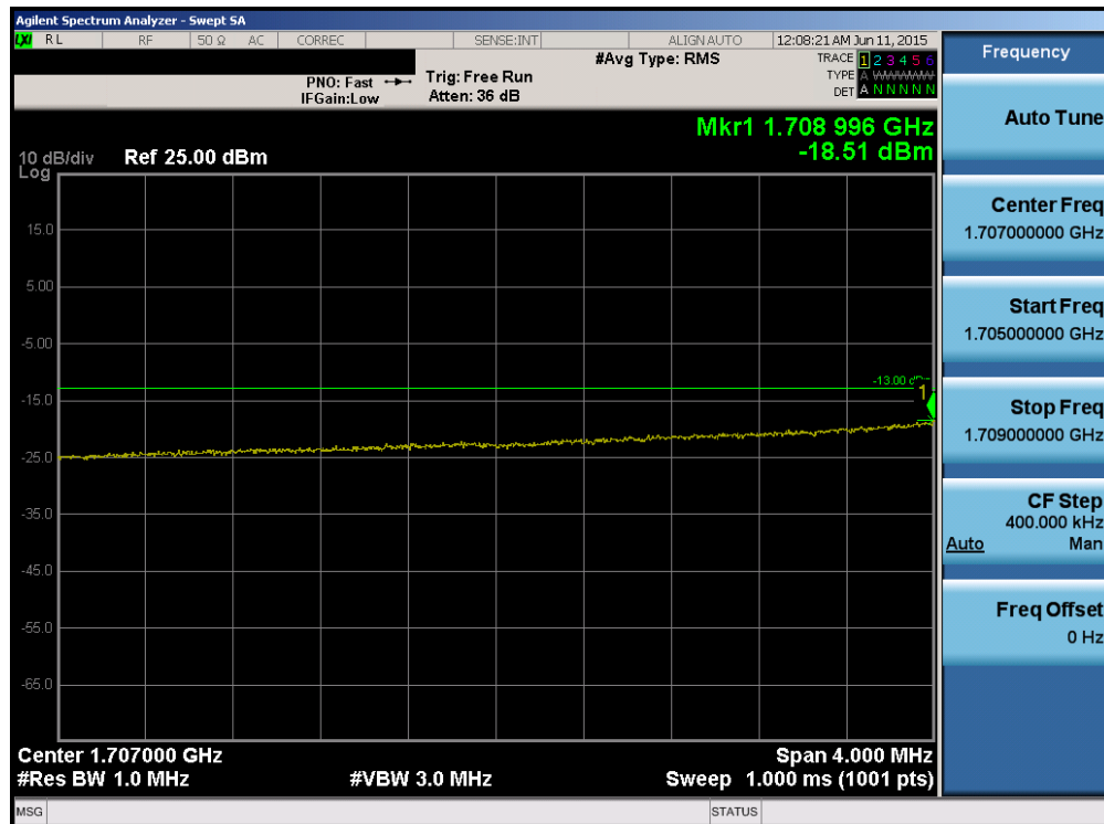
Plot 6-144. Lower Extended Band Edge Plot (Band 4 – 10.0MHz QPSK – RB Size 50)
