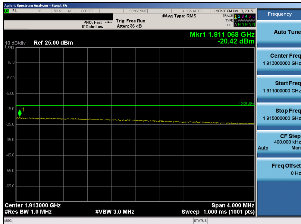
Plot 6-178. Upper Extended Band Edge Plot (Band 2 – 20.0MHz QPSK – RB Size 100)
