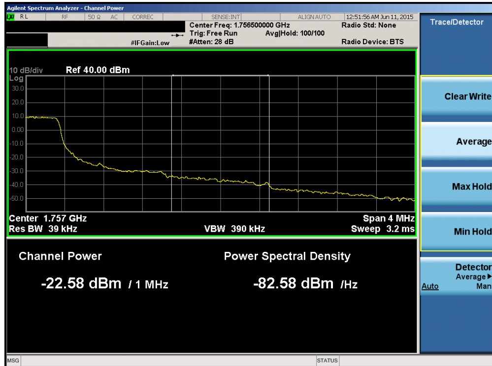
Plot 6-134. Upper Extended Band Edge Plot (Band 4 – 1.4MHz QPSK – RB Size 6)
