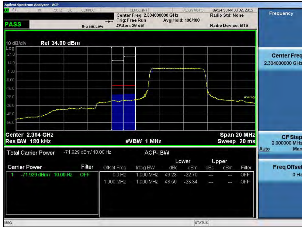
Plot 6-181. Lower Extended Band Edge Plot (Band 30 – 5.0MHz QPSK – RB Size 25)
