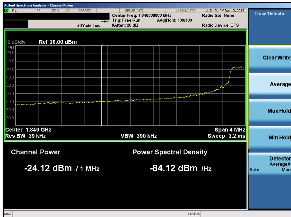
Plot 6-164. Lower Extended Band Edge Plot (Band 2 – 5.0MHz QPSK – RB Size 25)
