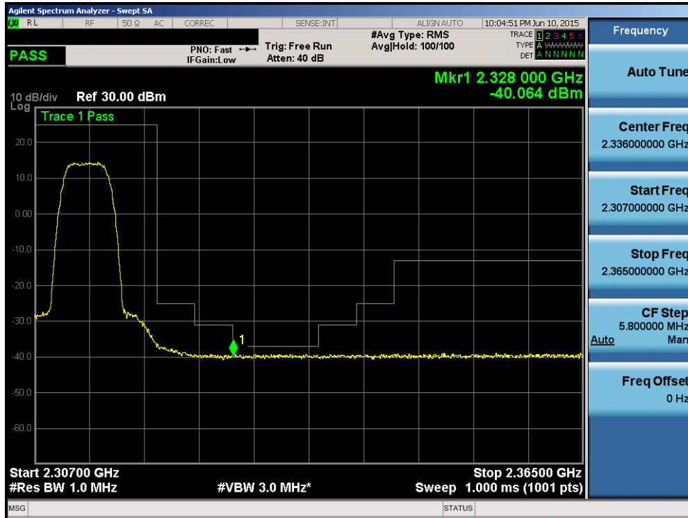
Plot 6-183. Upper Extended Band Edge Plot (Band 30 – 5.0MHz QPSK – RB Size 25)
