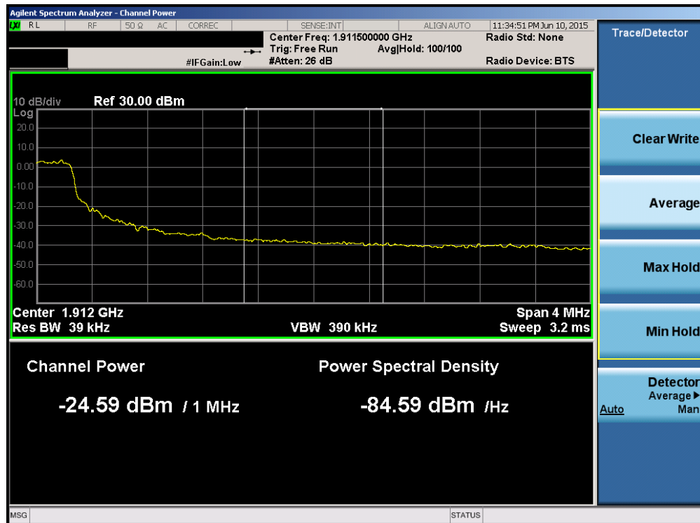
Plot 6-166. Upper Extended Band Edge Plot (Band 2 – 5.0MHz QPSK – RB Size 25)
