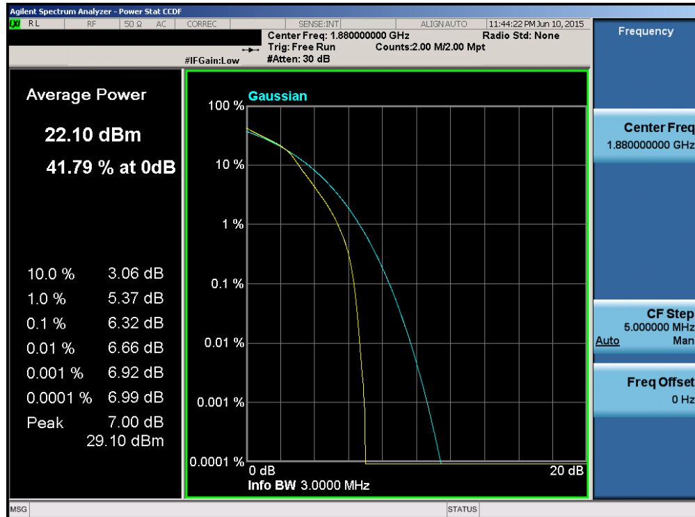
Plot 6-191. PAR Plot (Band 2 – 3.0MHz 16-QAM – RB Size 15)
