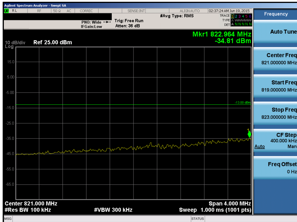
Plot 6-122. Lower Extended Band Edge Plot (Band 5 – 3.0MHz QPSK – RB Size 15)
