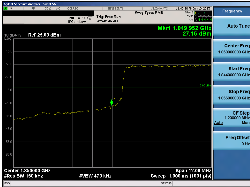
Plot 6-171. Lower Band Edge Plot (Band 2 – 15.0MHz QPSK – RB Size 75)
