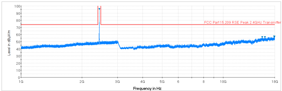
Plot 6-44. Radiated Spurious Plot above 1GHz (BT – Ch. 39, Ant. Pol. H)
