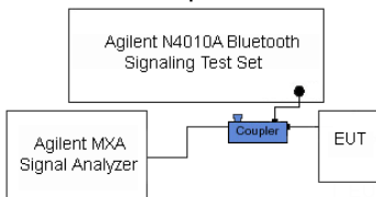
Figure 6-2. Test Instrument & Measurement Setup
