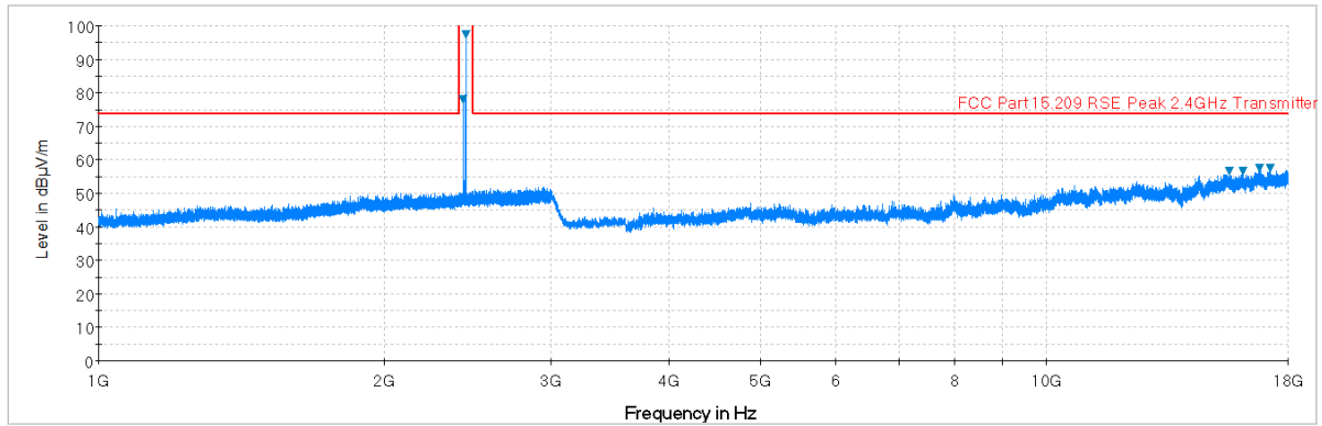
Plot 6-45. Radiated Spurious Plot above 1GHz (BT – Ch. 39, Ant. Pol. V)
