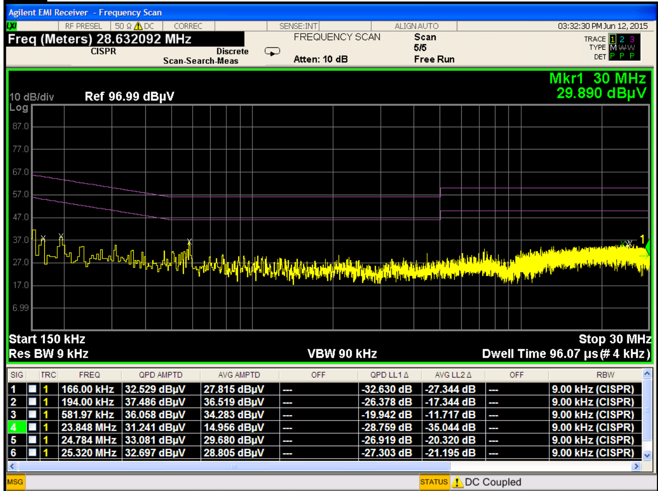
Plot 6-55. Line-Conducted Test Plot (N)
