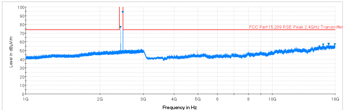
Plot 6-47. Radiated Spurious Plot above 1GHz (BT – Ch. 78, Ant. Pol. V)
