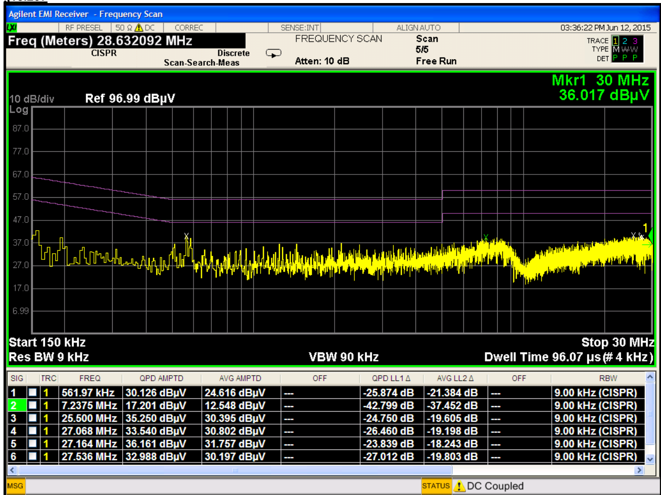
Plot 6-54. Line-Conducted Test Plot (L1)
