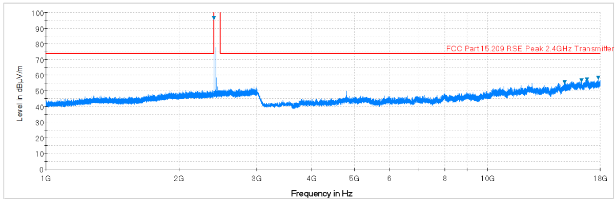
Plot 6-43. Radiated Spurious Plot above 1GHz (BT – Ch. 0, Ant. Pol. V)
