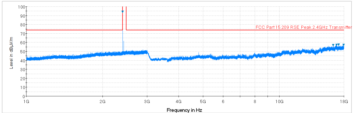
Plot 6-42. Radiated Spurious Plot above 1GHz (BT – Ch. 0, Ant. Pol. H)
