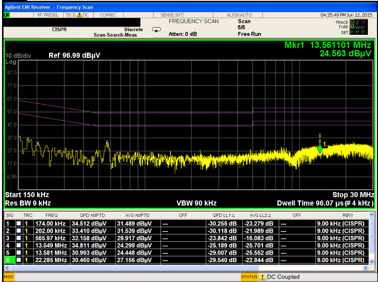
Plot 6-229. Line Conducted Plot with 802.11a UNII Band 2C (N)
