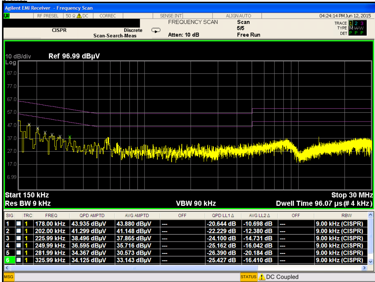
Plot 6-226. Line Conducted Plot with 802.11a UNII Band 2A (L1)
