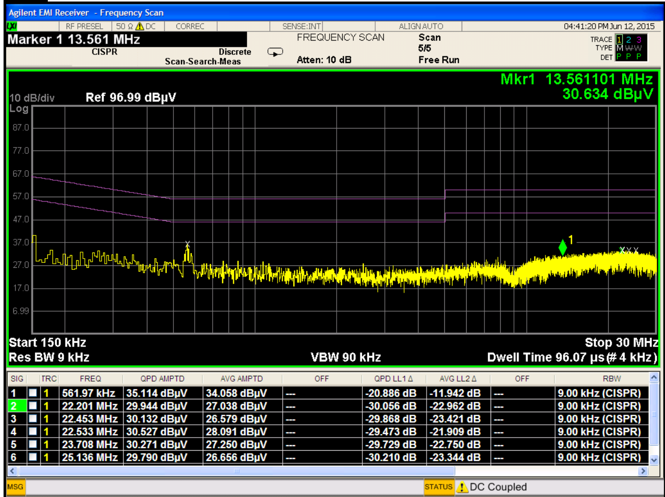
Plot 6-225. Line Conducted Plot with 802.11a UNII Band 1 (N)
