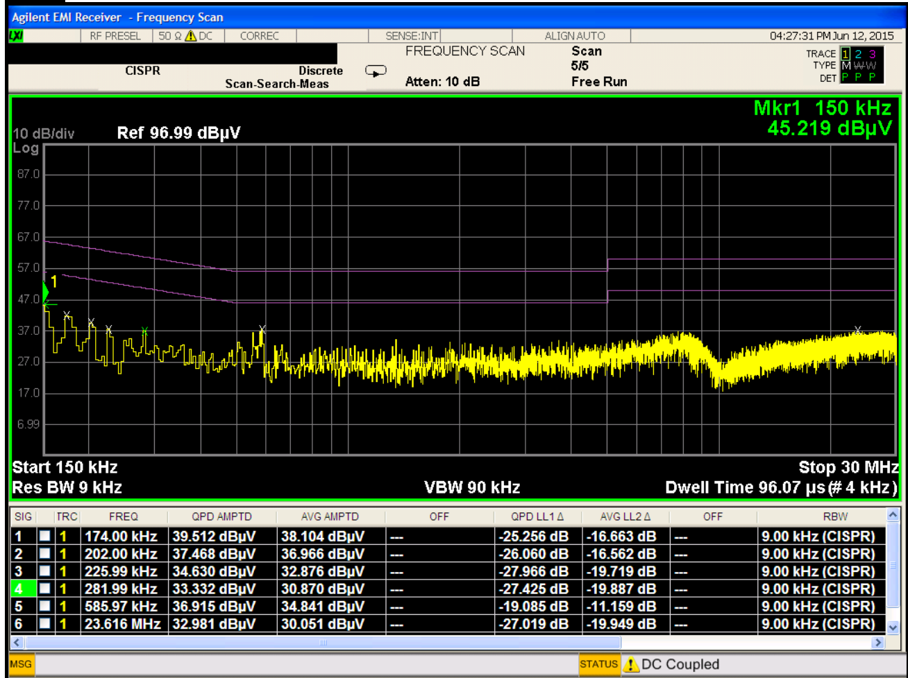
Plot 6-228. Line Conducted Plot with 802.11a UNII Band 2C (L1)
