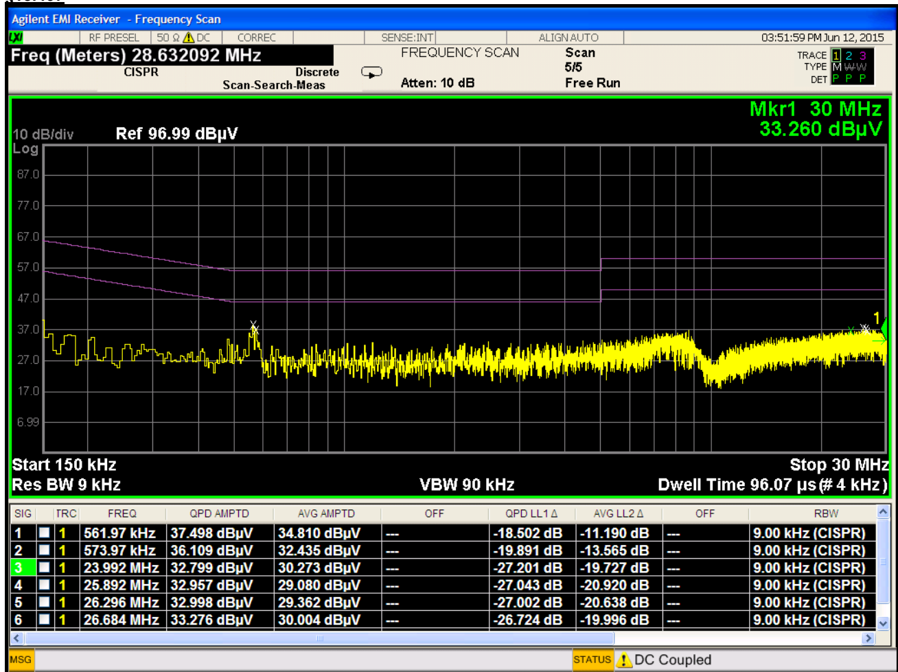
Plot 6-224. Line Conducted Plot with 802.11a UNII Band 1 (L1)
