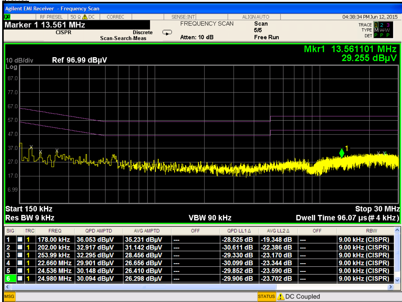
Plot 6-227. Line Conducted Plot with 802.11a UNII Band 2A (N)
