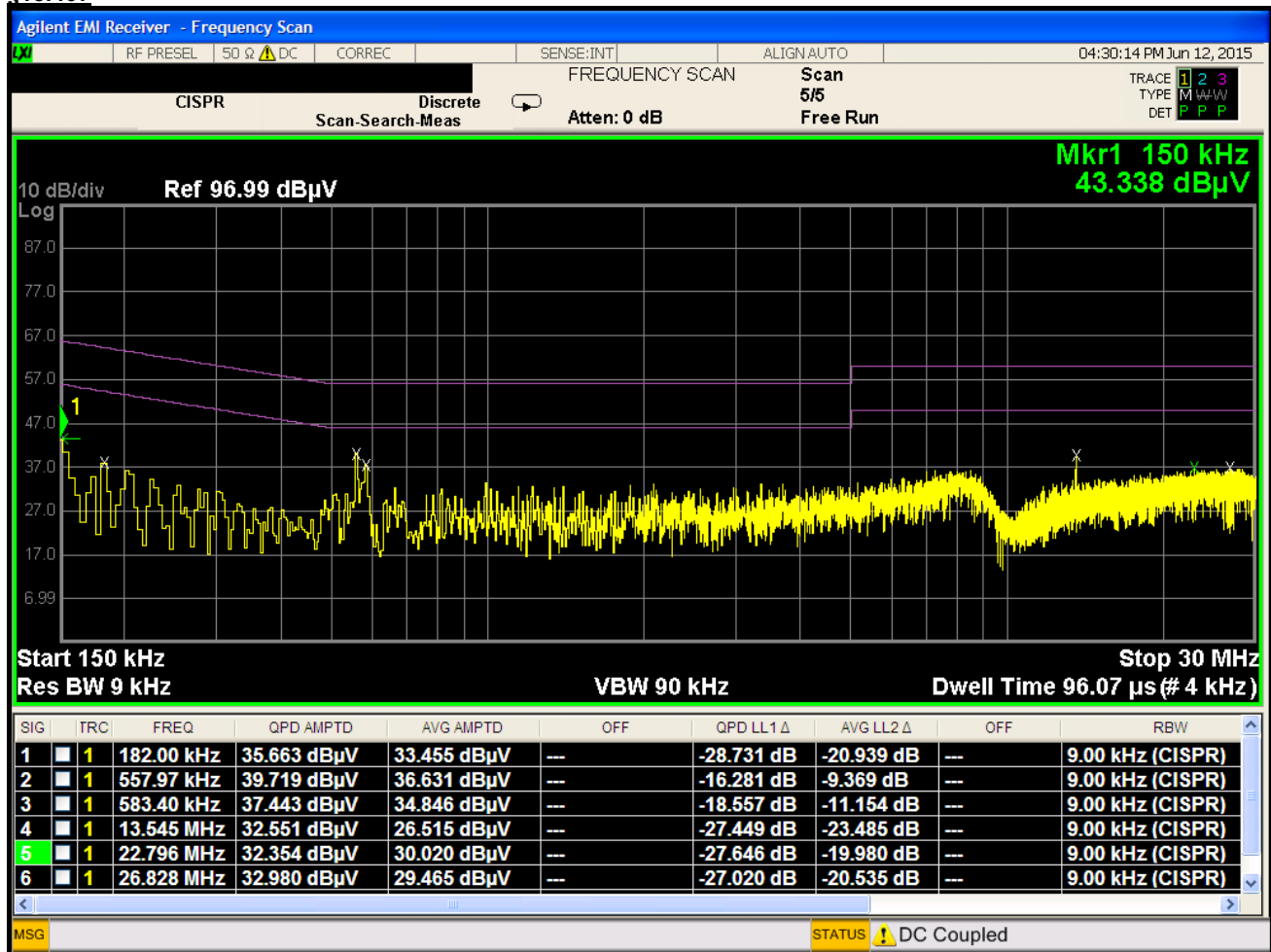
Plot 6-230. Line Conducted Plot with 802.11a UNII Band 3 (L1)
