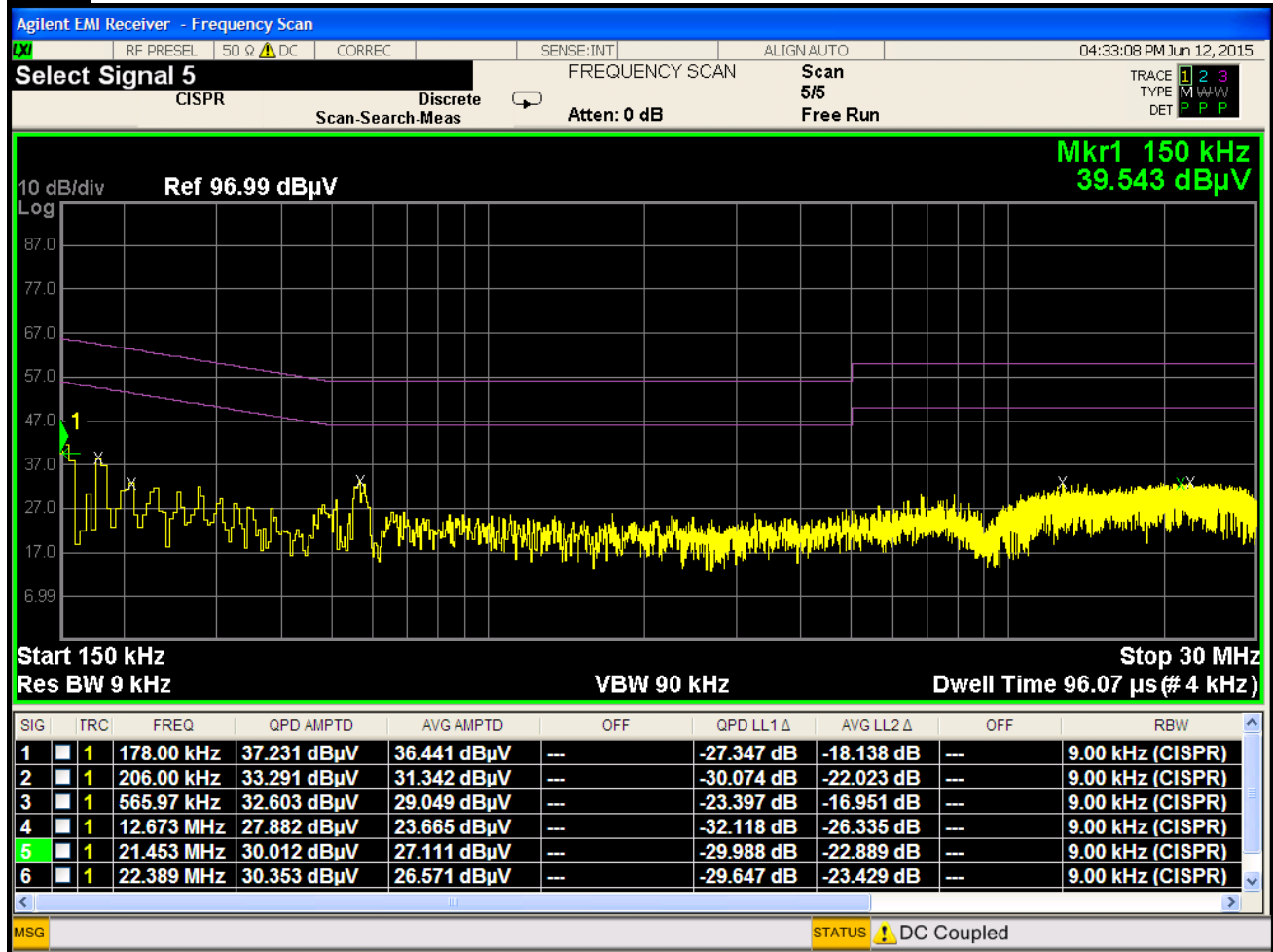
Plot 6-231. Line Conducted Plot with 802.11a UNII Band 3 (N)
