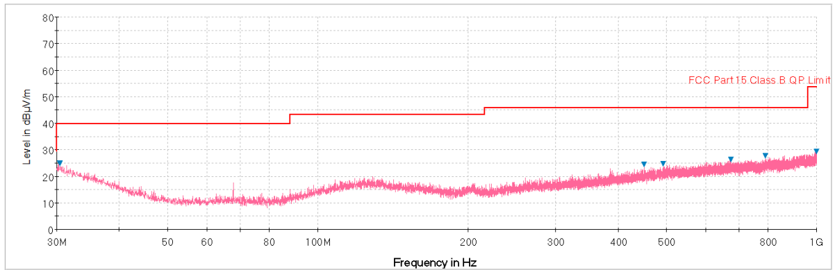
Plot 6-86. Radiated Spurious Plot below 1GHz (Pol. V)
