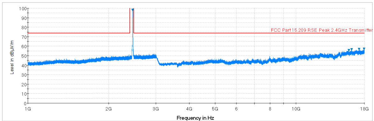
Plot 6-65. Radiated Spurious Plot above 1GHz (802.11b – Ch. 11, Ant. Pol. H)
