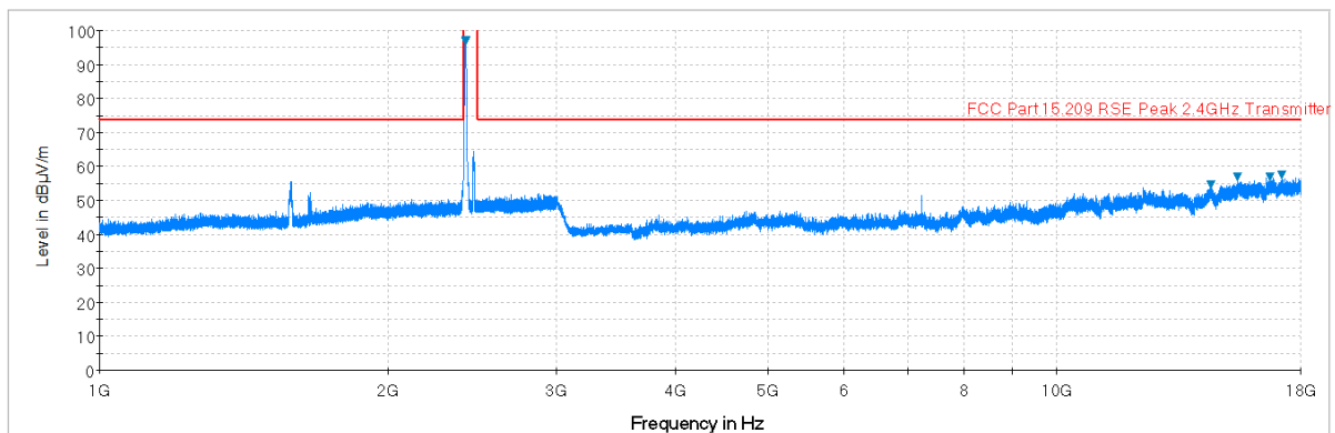
Plot 6-62. Radiated Spurious Plot above 1GHz (802.11b – Ch. 1, Ant. Pol. V)
