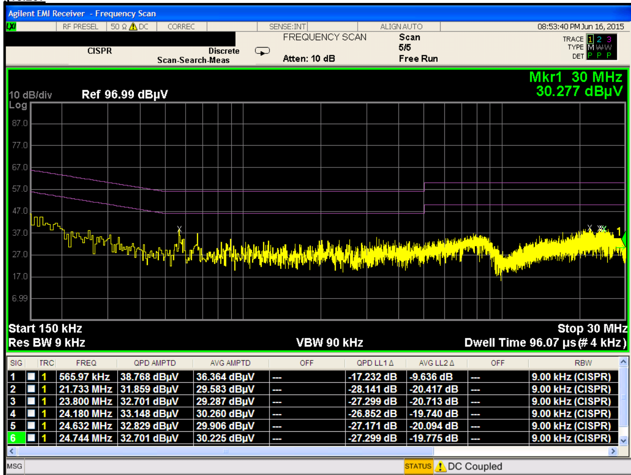
Plot 7-3. Line-Conducted Test Plot (L1) 50 Ohm Terminated Antenna
