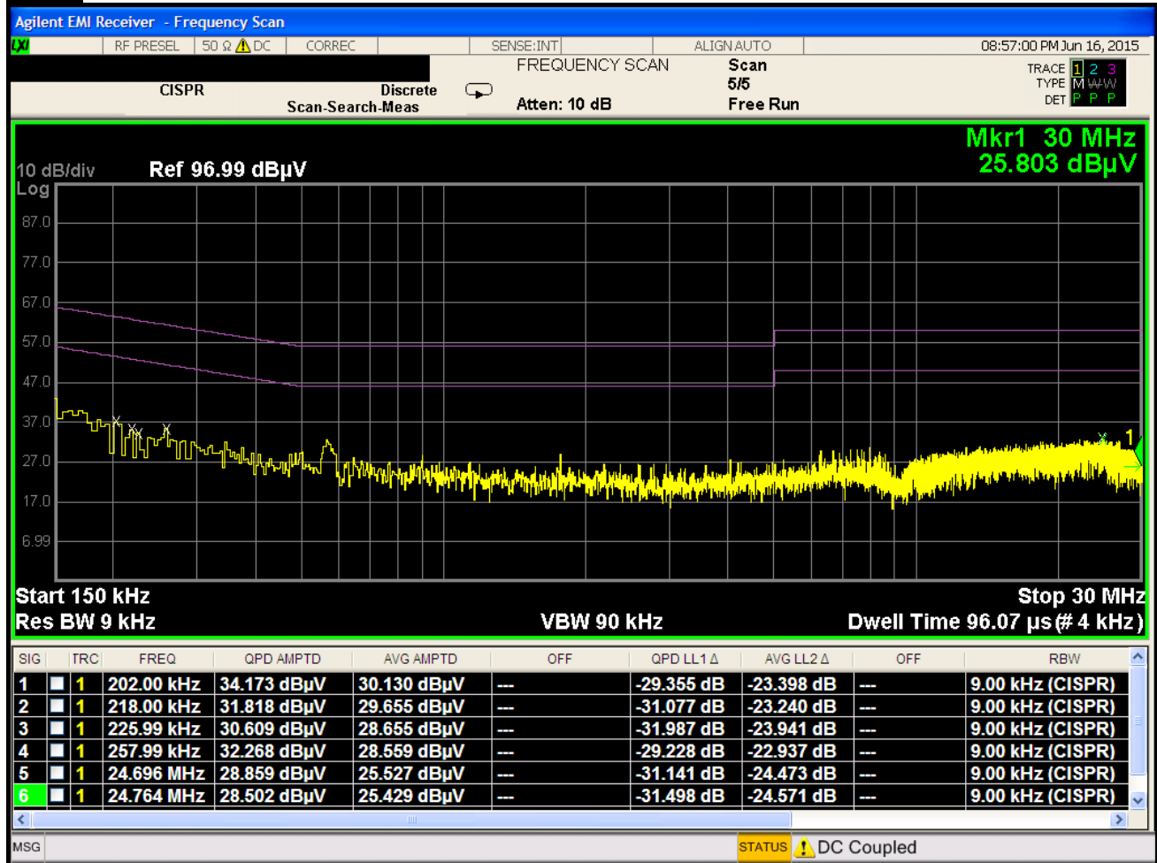
Plot 7-4. Line-Conducted Test Plot (N) 50Ohm Terminated Antenna
