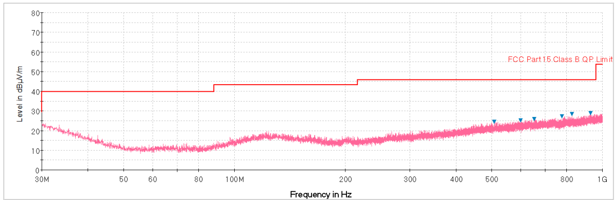
Plot 6-220. Radiated Spurious Plot below 1GHz (802.11a – U3 Ch. 157, Ant. Pol. H)
