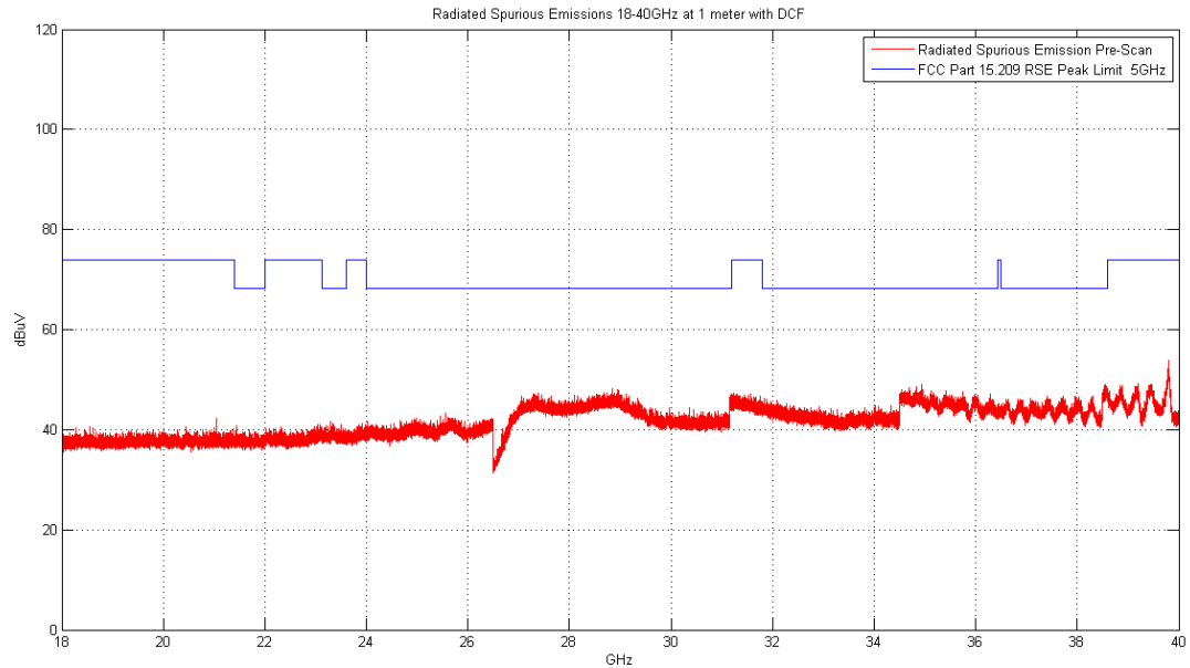
Plot 6-179. Radiated Spurious Plot above 18GHz (SIMULTANEOUS TX Config-2, Ant. Pol. H)
