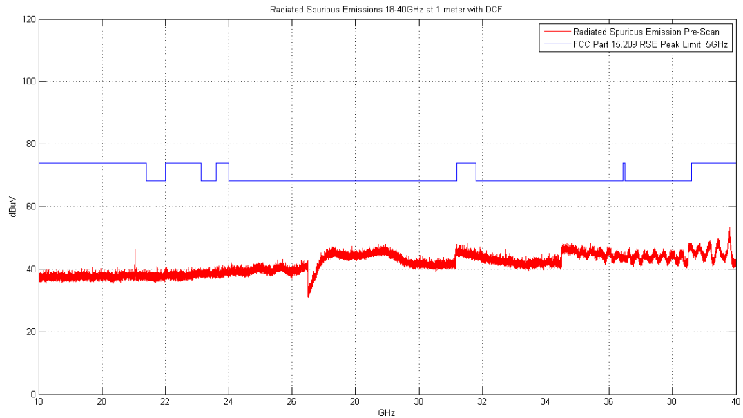
Plot 6-178. Radiated Spurious Plot above 18GHz (SIMULTANEOUS TX Config-1, Ant. Pol. V)
