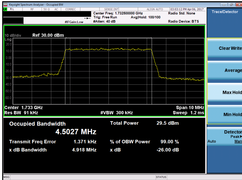
Plot 7-6. Occupied Bandwidth Plot (Band 4 – 5.0MHz 16-QAM – RB Size 25)
