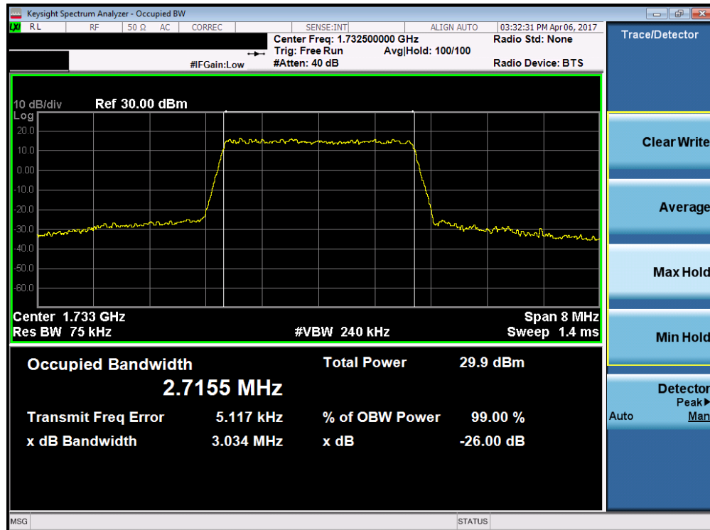
Plot 7-4. Occupied Bandwidth Plot (Band 4 – 3.0MHz 16-QAM – RB Size 15)
