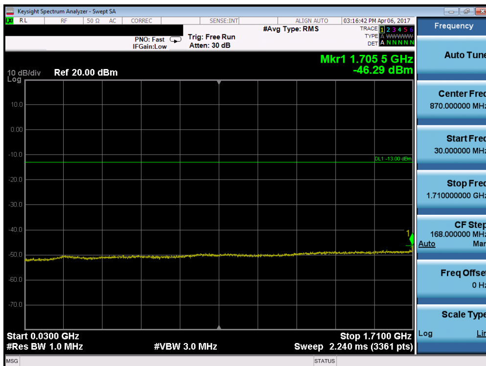
Plot 7-24. Conducted Spurious Plot (Band 4 – 5.0MHz QPSK – RB Size 1, RB Offset 0 – Mid Channel)
