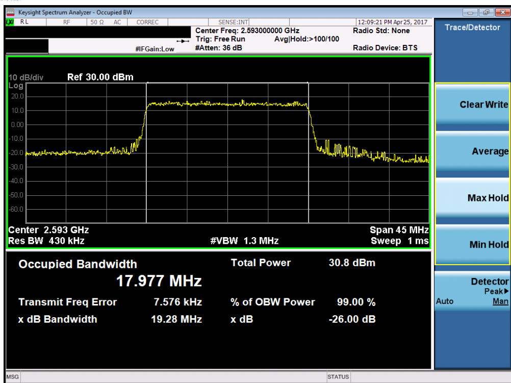
Plot 7-19. Occupied Bandwidth Plot (Band 41 – 20.0MHz QPSK – RB Size 100)
