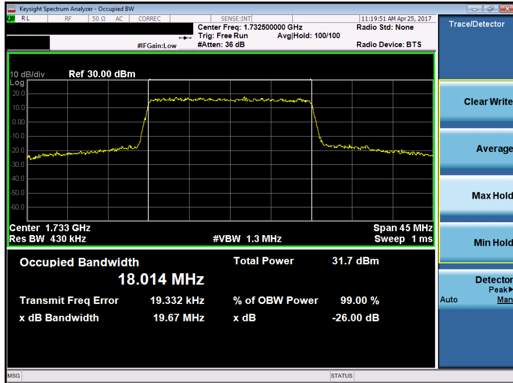
Plot 7-11. Occupied Bandwidth Plot (Band 4 – 20.0MHz QPSK – RB Size 100)
