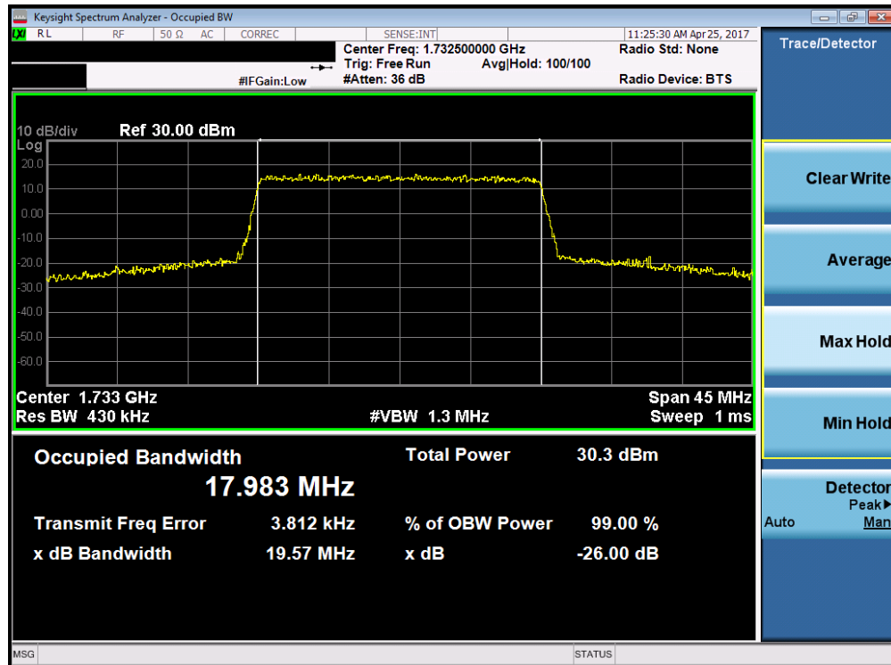
Plot 7-12. Occupied Bandwidth Plot (Band 4 – 20.0MHz 16-QAM – RB Size 100)
