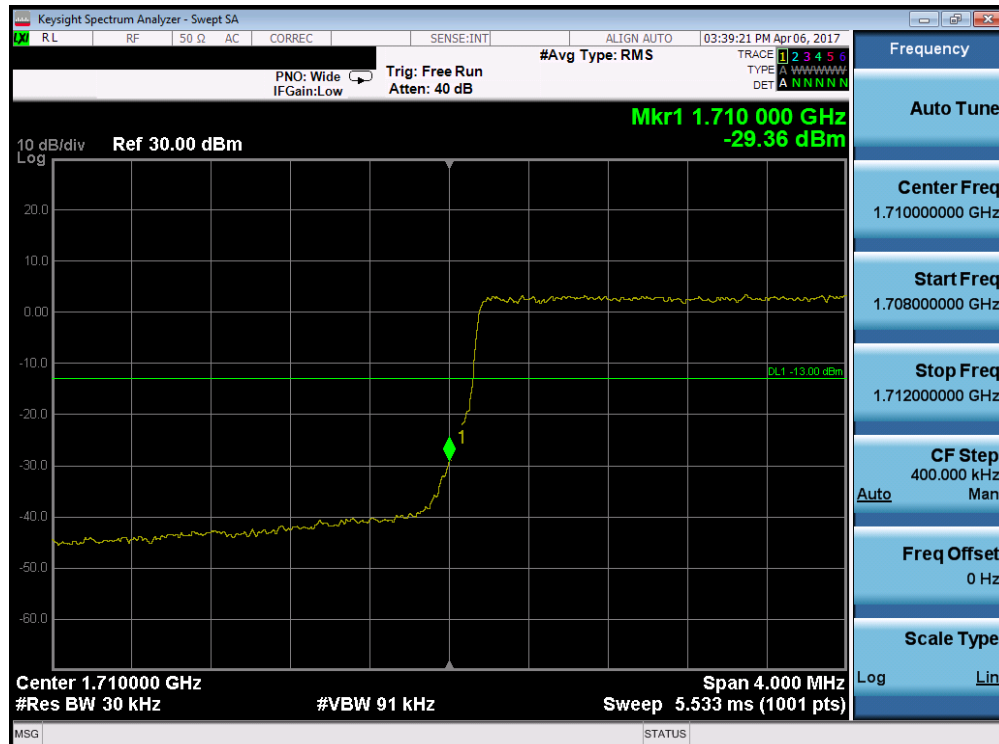
Plot 7-43. Lower Band Edge Plot (Band 4 – 3.0MHz QPSK – RB Size 15)
