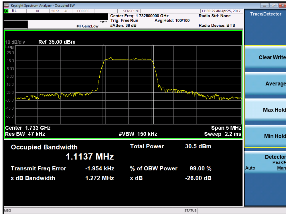
Plot 7-2. Occupied Bandwidth Plot (Band 4 – 1.4MHz 16-QAM – RB Size 6)
