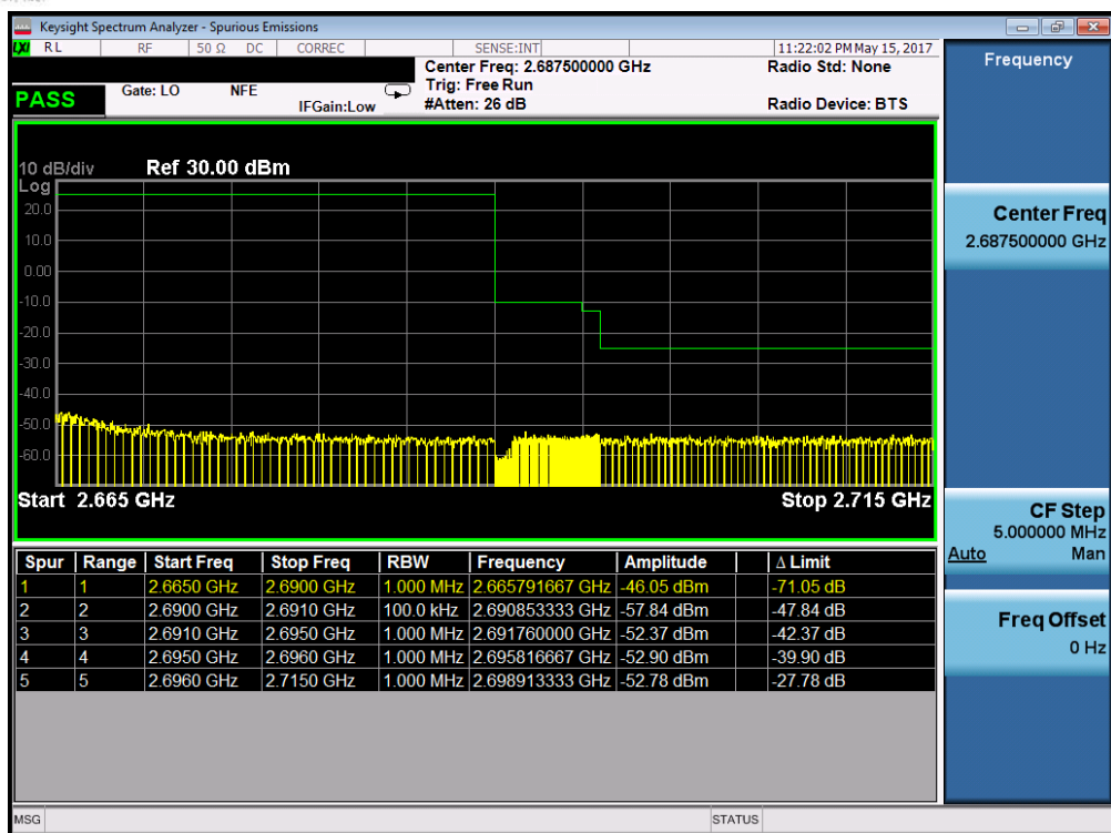
Plot 7-64. Upper ACP Plot (Band 41 – 5.0MHz QPSK – RB Size 25)
