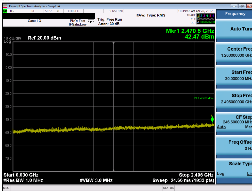
Plot 7-33. Conducted Spurious Plot (Band 41 – 20.0MHz QPSK – RB Size 1, RB Offset 0 – Mid Channel)
