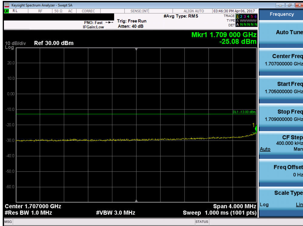
Plot 7-52. Lower Extended Band Edge Plot (Band 4 – 10.0MHz QPSK – RB Size 50)
