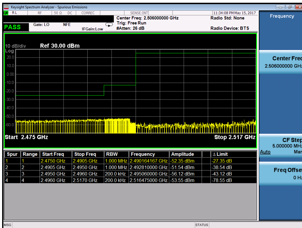
Plot 7-69. Lower ACP Plot (Band 41 – 20.0MHz QPSK – RB Size 100)
