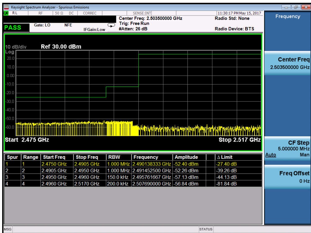
Plot 7-67. Lower ACP Plot (Band 41 – 15.0MHz QPSK – RB Size 75)
