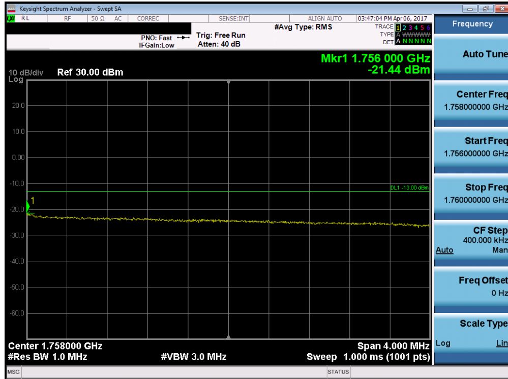
Plot 7-54. Upper Extended Band Edge Plot (Band 4 – 10.0MHz QPSK – RB Size 50)
