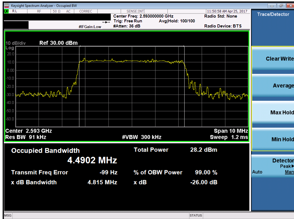
Plot 7-14. Occupied Bandwidth Plot (Band 41 – 5.0MHz 16-QAM – RB Size 25)
