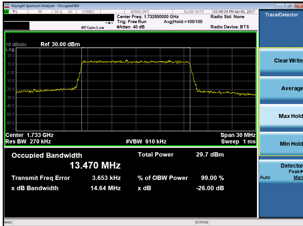
Plot 7-10. Occupied Bandwidth Plot (Band 4 – 15.0MHz 16-QAM – RB Size 75)
