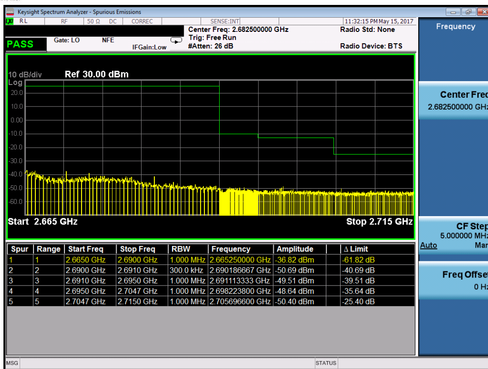
Plot 7-68. Upper ACP Plot (Band 41 – 15.0MHz QPSK – RB Size 75)
