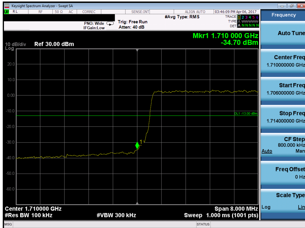
Plot 7-51. Lower Band Edge Plot (Band 4 – 10.0MHz QPSK – RB Size 50)
