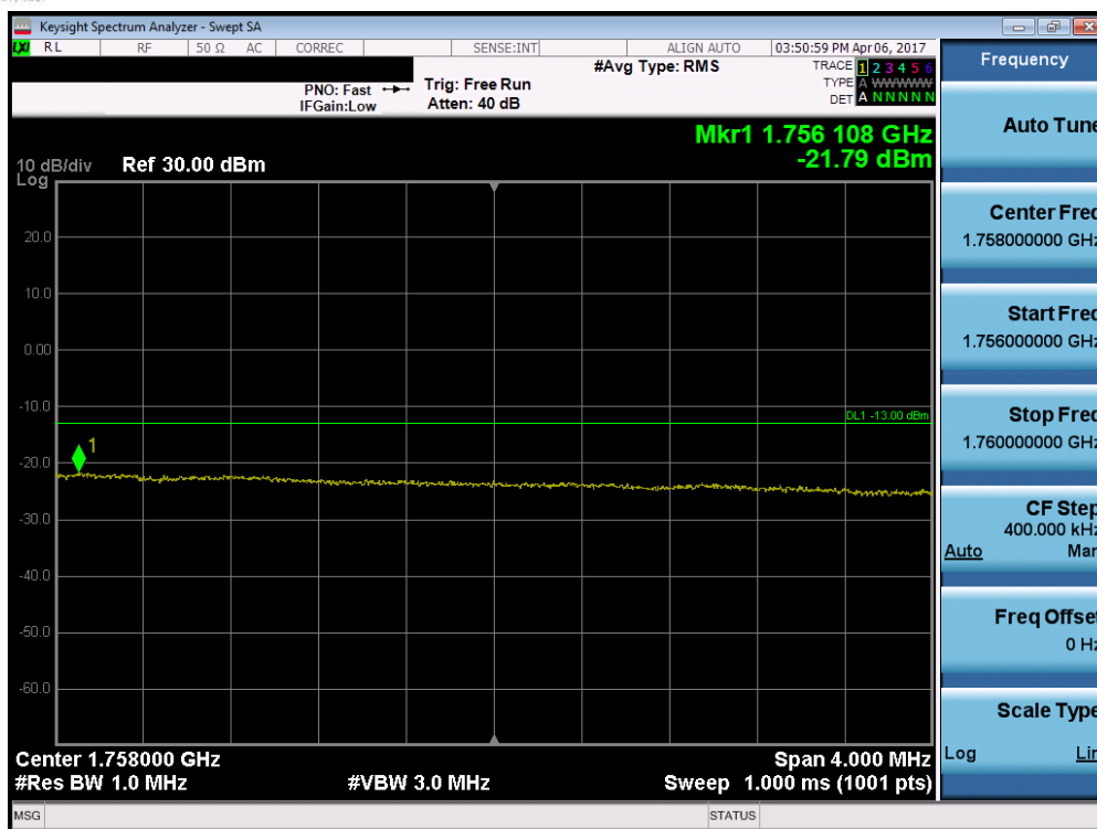
Plot 7-58. Upper Extended Band Edge Plot (Band 4 - 15.0MHz QPSK - RB Size 75)
