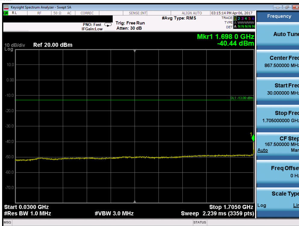
Plot 7-21. Conducted Spurious Plot (Band 4 – 5.0MHz QPSK – RB Size 1, RB Offset 0 – Low Channel)
