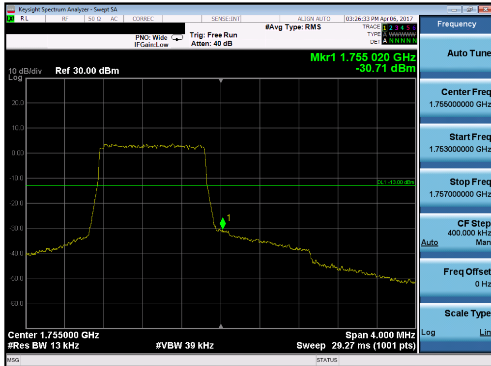
Plot 7-41. Upper Band Edge Plot (Band 4 – 1.4MHz QPSK – RB Size 6)
