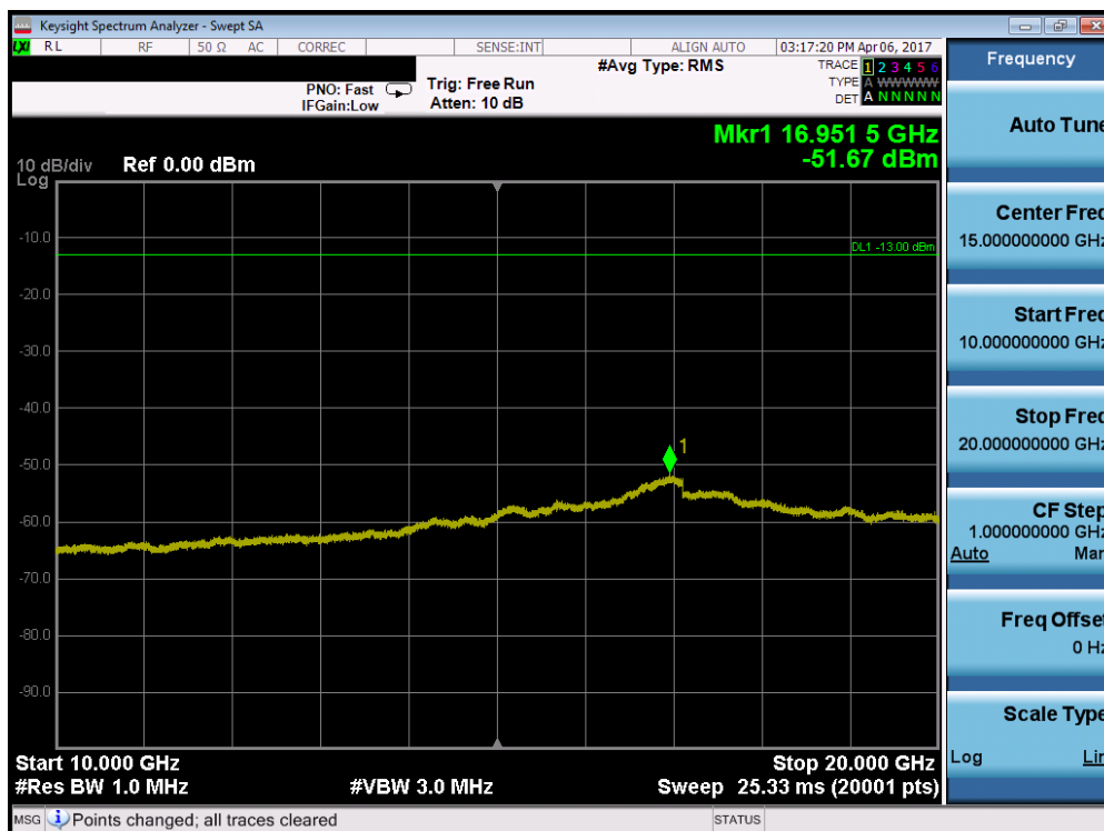
Plot 7-26. Conducted Spurious Plot (Band 4 – 5.0MHz QPSK – RB Size 1, RB Offset 0 – Mid Channel)
