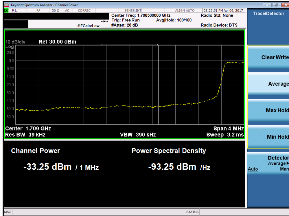
Plot 7-40. Lower Extended Band Edge Plot (Band 4 – 1.4MHz QPSK – RB Size 6)
