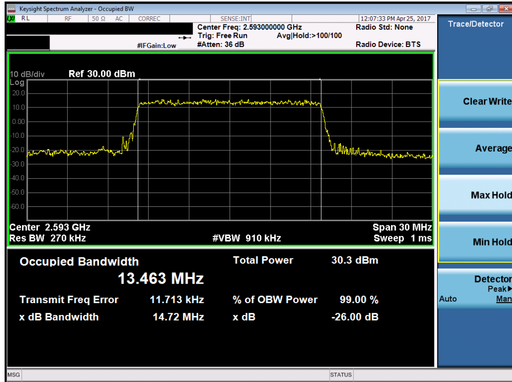
Plot 7-17. Occupied Bandwidth Plot (Band 41 – 15.0MHz QPSK – RB Size 75)
