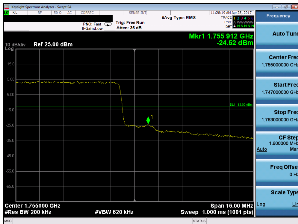
Plot 7-61. Upper Band Edge Plot (Band 4 – 20.0MHz QPSK – RB Size 100)
