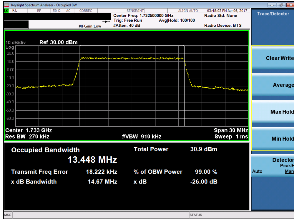
Plot 7-9. Occupied Bandwidth Plot (Band 4 – 15.0MHz QPSK – RB Size 75)
