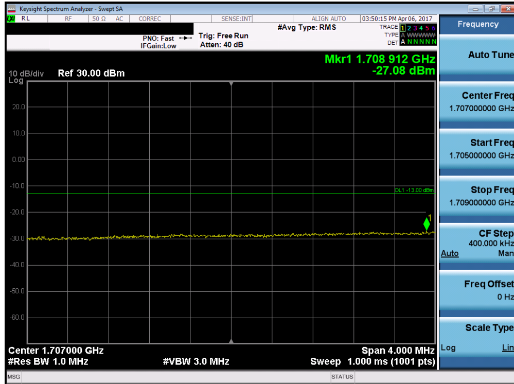
Plot 7-56. Lower Extended Band Edge Plot (Band 4 – 15.0MHz QPSK – RB Size 75)
