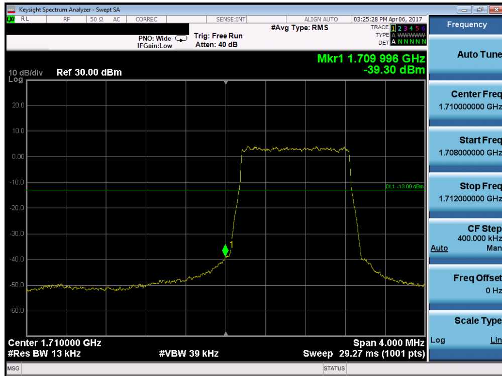
Plot 7-39. Lower Band Edge Plot (Band 4 – 1.4MHz QPSK – RB Size 6)
