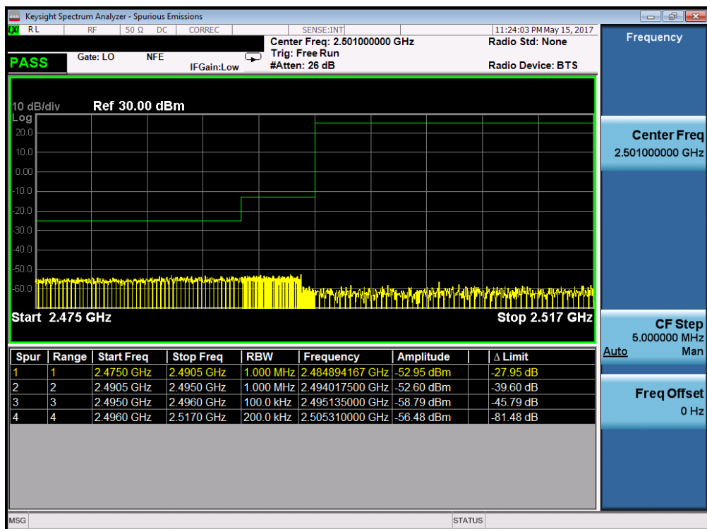
Plot 7-65. Lower ACP Plot (Band 41 – 10.0MHz QPSK – RB Size 50)
