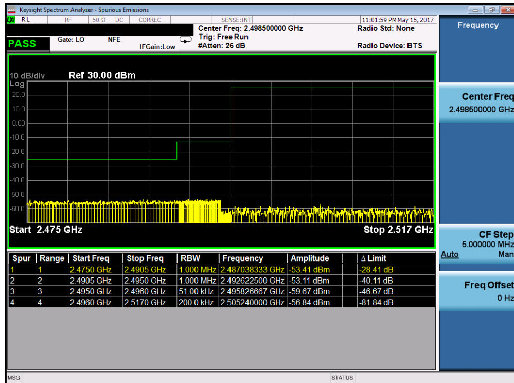
Plot 7-63. Lower ACP Plot (Band 41 – 5.0MHz QPSK – RB Size 25)
