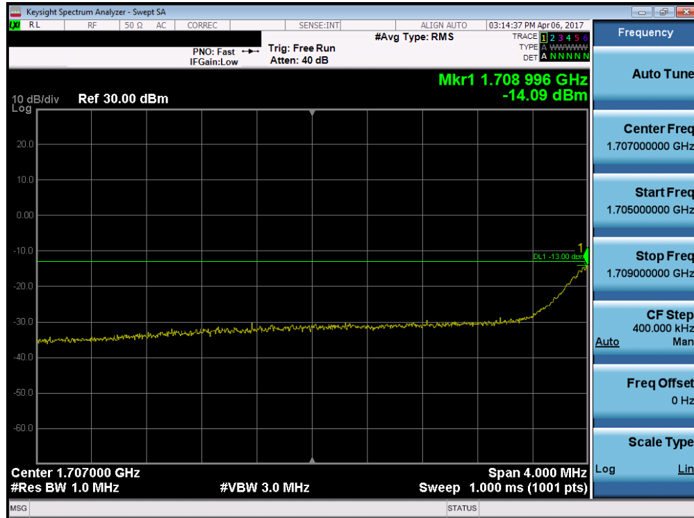
Plot 7-48. Lower Extended Band Edge Plot (Band 4 – 5.0MHz QPSK – RB Size 25)
