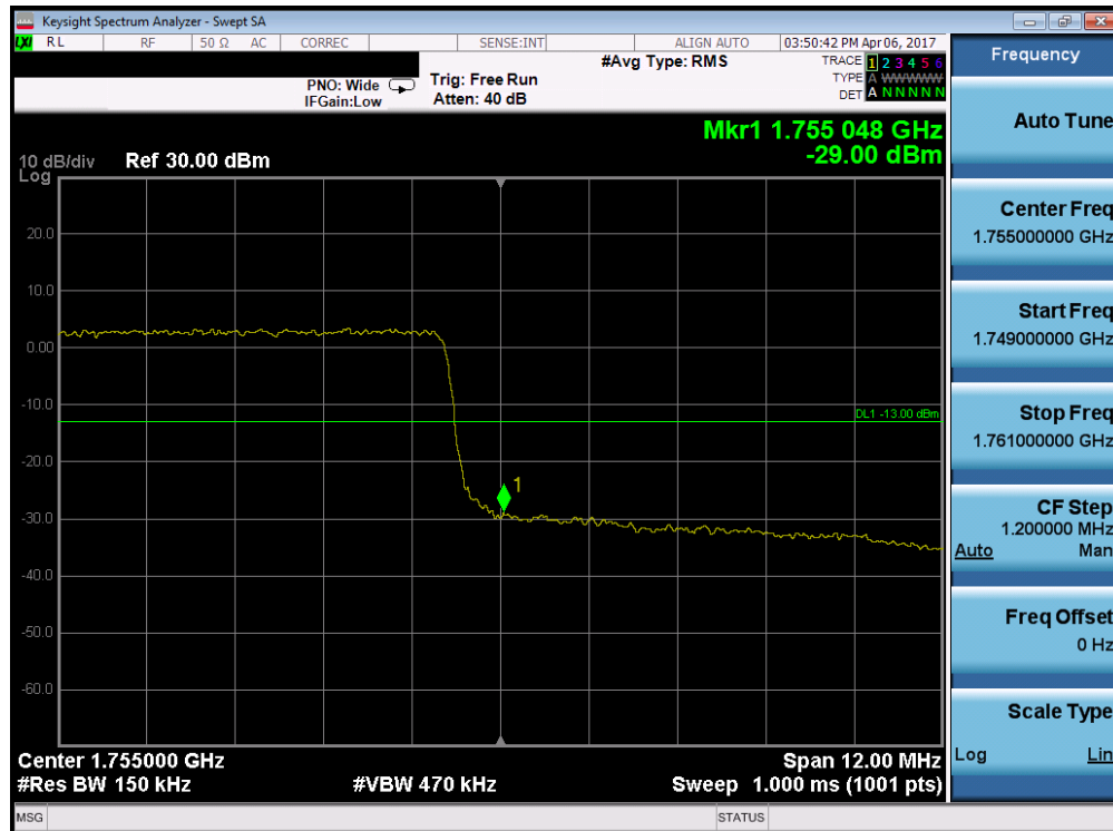
Plot 7-57. Upper Band Edge Plot (Band 4 – 15.0MHz QPSK – RB Size 75)
