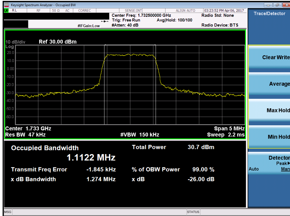
Plot 7-1. Occupied Bandwidth Plot (Band 4 – 1.4MHz QPSK – RB Size 6)
