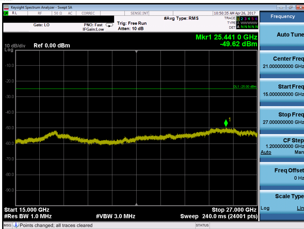
Plot 7-35. Conducted Spurious Plot (Band 41 – 20.0MHz QPSK – RB Size 1, RB Offset 0 – Mid Channel)
