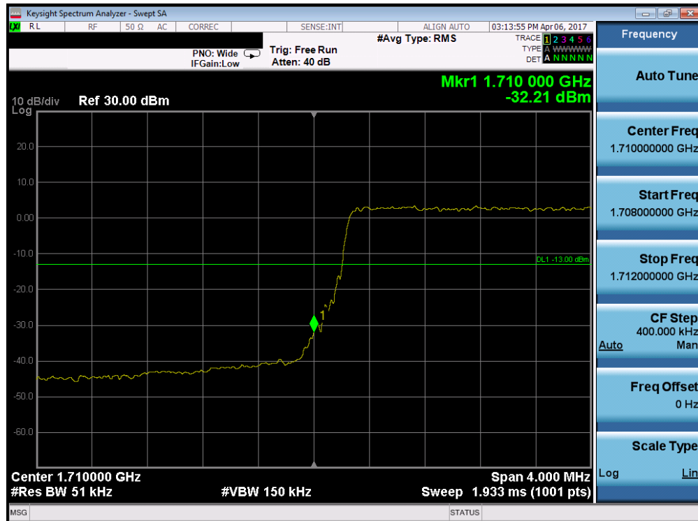
Plot 7-47. Lower Band Edge Plot (Band 4 – 5.0MHz QPSK – RB Size 25)
