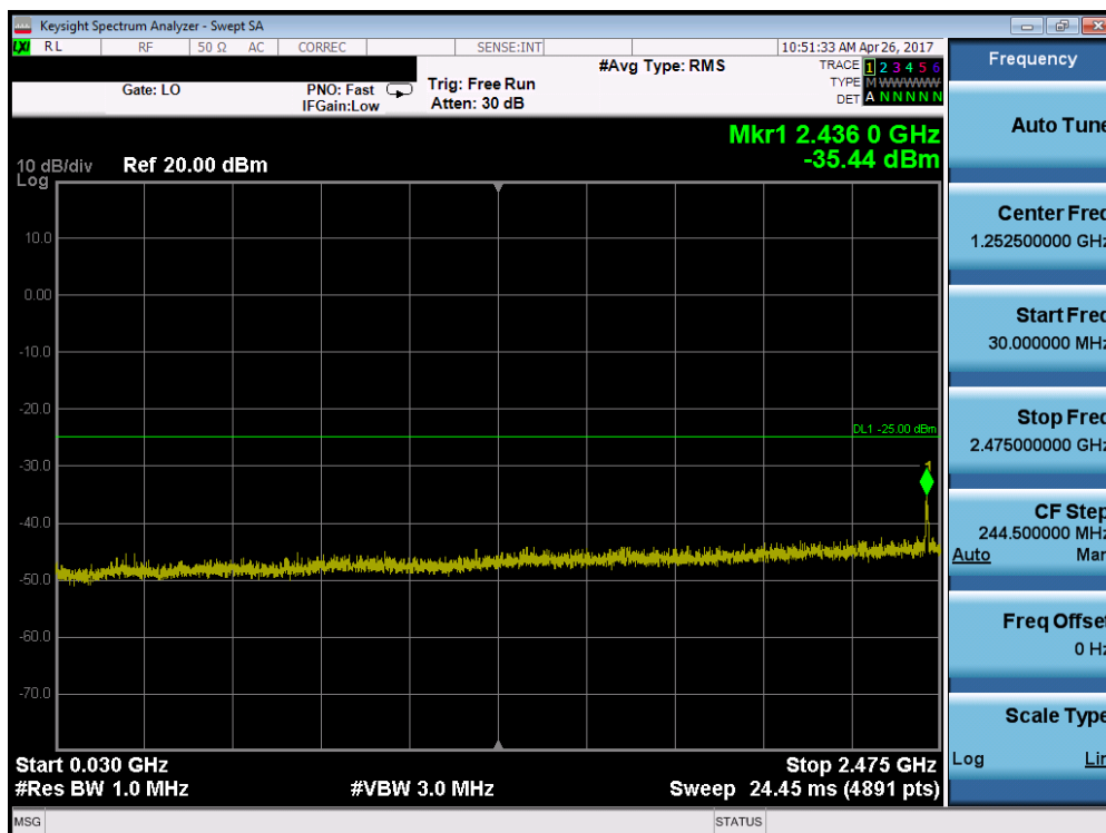
Plot 7-30. Conducted Spurious Plot (Band 41 – 20.0MHz QPSK – RB Size 1, RB Offset 0– Low Channel)
