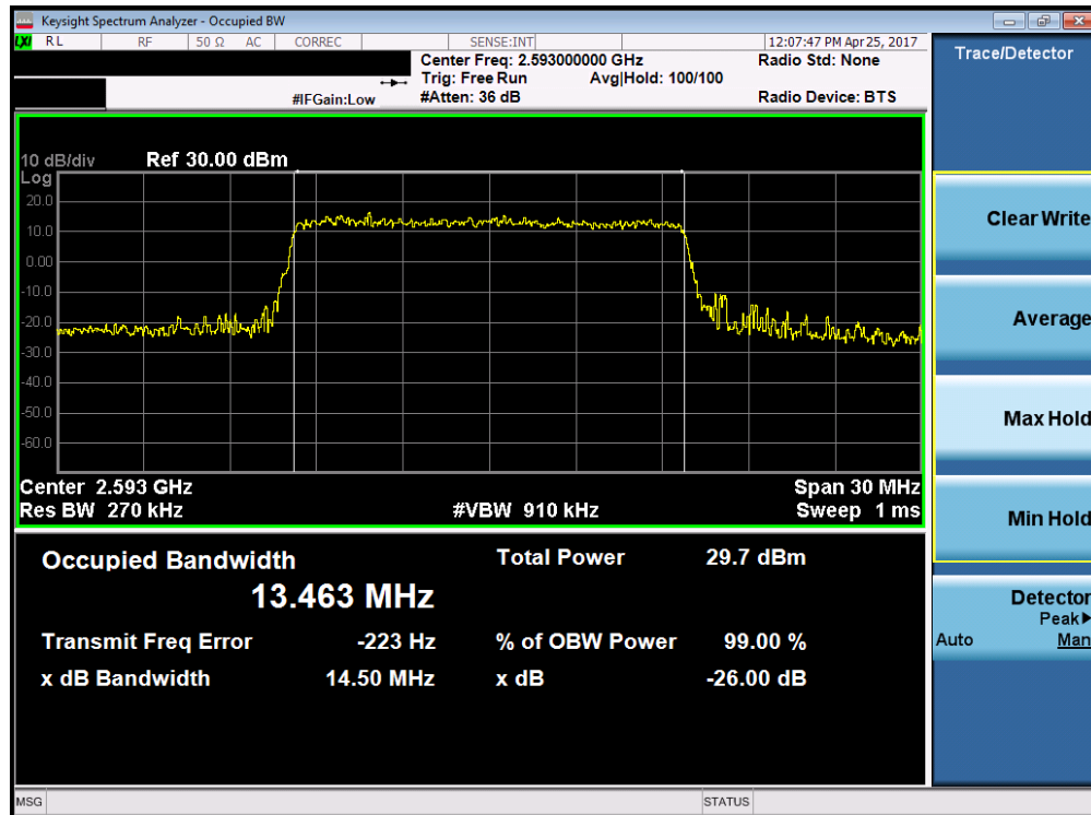
Plot 7-18. Occupied Bandwidth Plot (Band 41 – 15.0MHz 16-QAM – RB Size 75)
