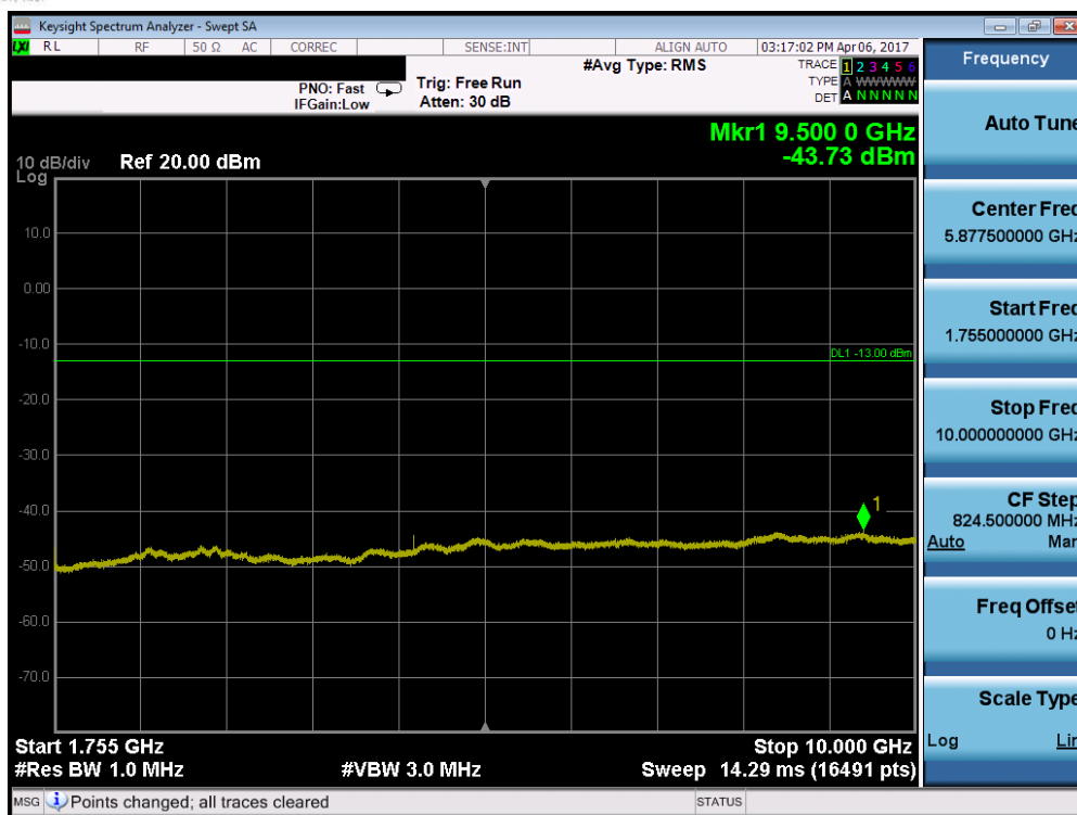
Plot 7-25. Conducted Spurious Plot (Band 4 – 5.0MHz QPSK – RB Size 1, RB Offset 0 – Mid Channel)
