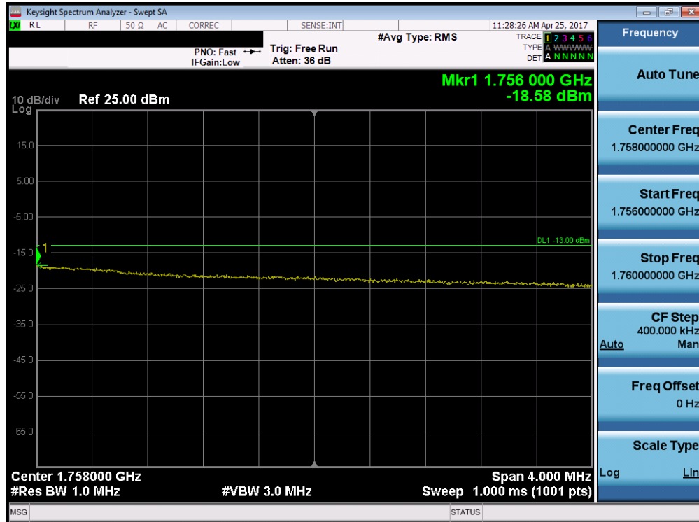
Plot 7-62. Upper Extended Band Edge Plot (Band 4 – 20.0MHz QPSK – RB Size 100)
