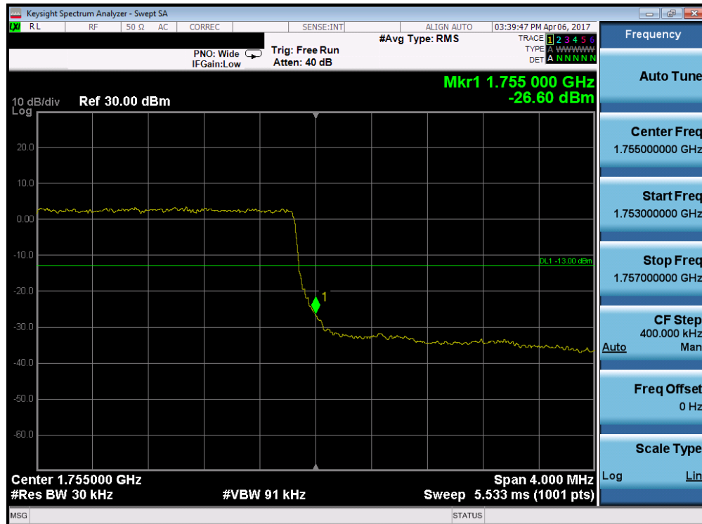
Plot 7-45. Upper Band Edge Plot (Band 4 – 3.0MHz QPSK – RB Size 15)
