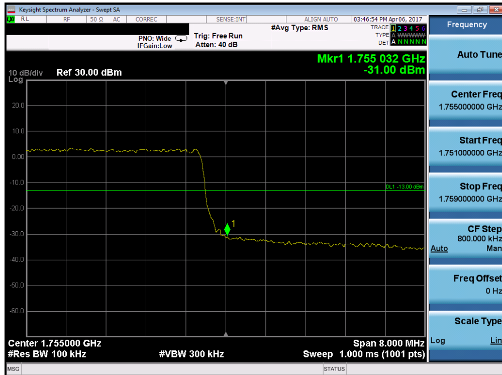
Plot 7-53. Upper Band Edge Plot (Band 4 – 10.0MHz QPSK – RB Size 50)
