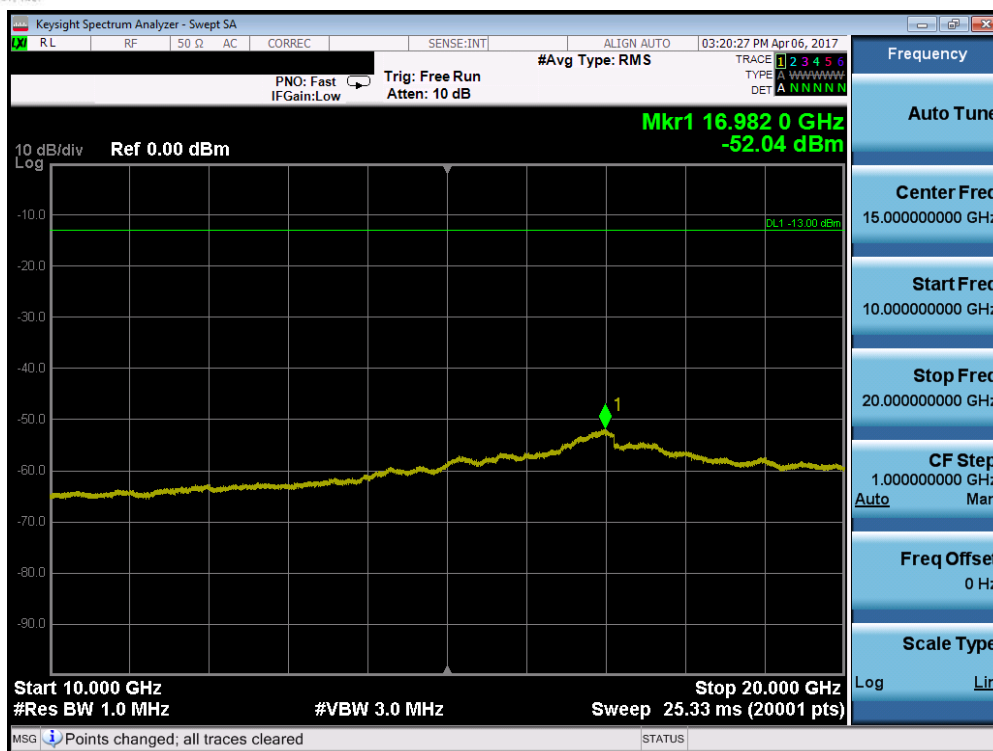
Plot 7-29. Conducted Spurious Plot (Band 4 – 5.0MHz QPSK – RB Size 1, RB Offset 0 – High Channel)
