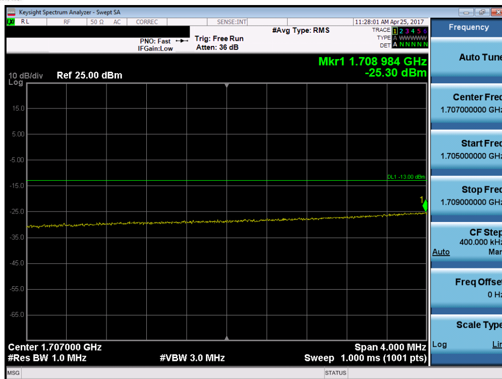
Plot 7-60. Lower Extended Band Edge Plot (Band 4 – 20.0MHz QPSK – RB Size 100)
