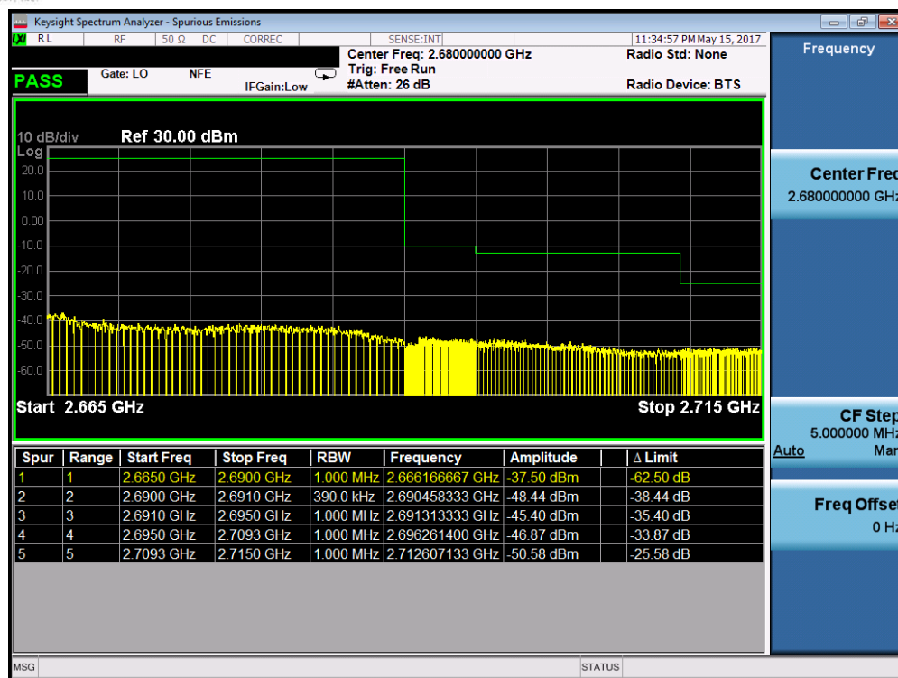
Plot 7-70. Upper ACP Plot (Band 41 – 20.0MHz QPSK – RB Size 100)
