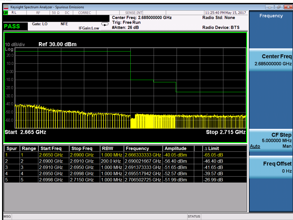
Plot 7-66. Upper ACP Plot (Band 41 – 10.0MHz QPSK – RB Size 50)
