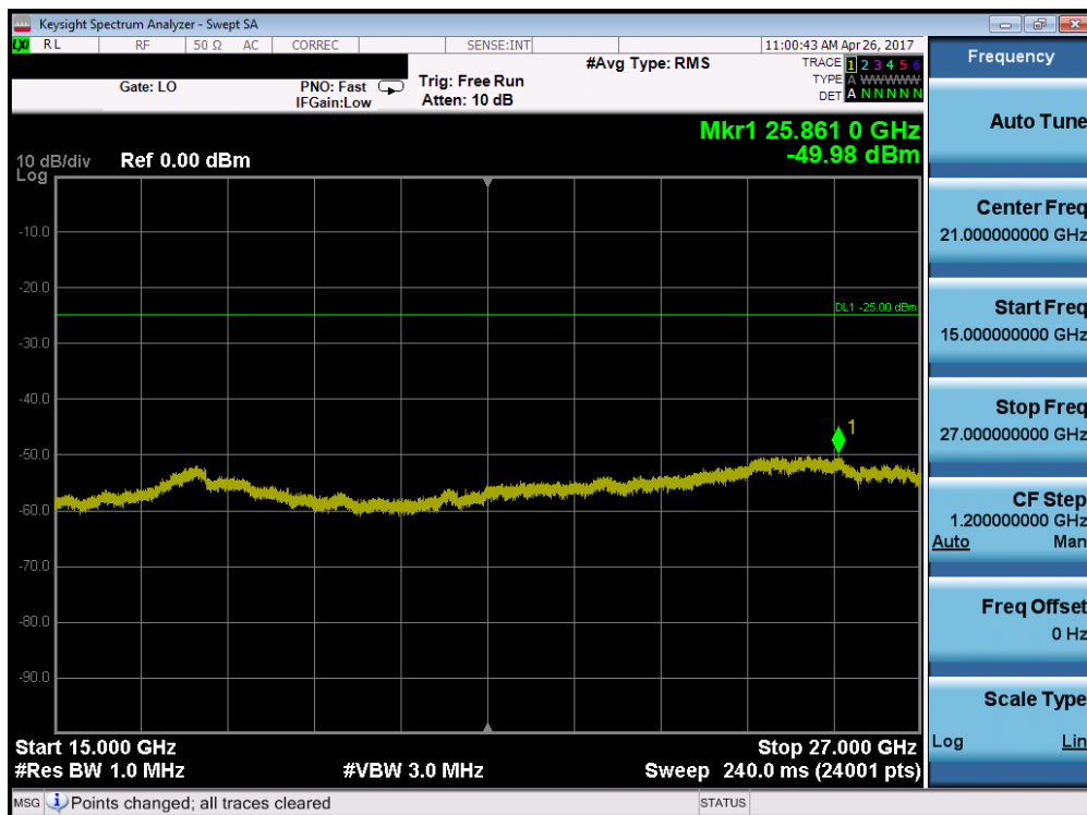
Plot 7-38. Conducted Spurious Plot (Band 41 – 20.0MHz QPSK – RB Size 1, RB Offset 0 – High Channel)
