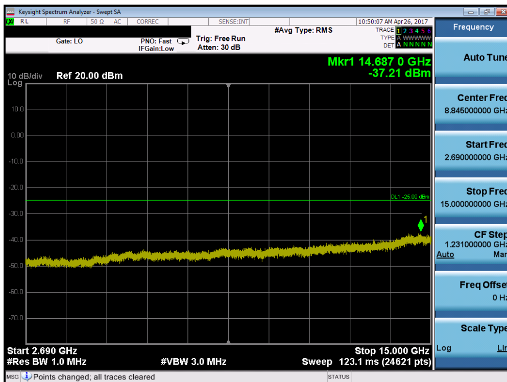
Plot 7-34. Conducted Spurious Plot (Band 41 – 20.0MHz QPSK – RB Size 1, RB Offset 0 – Mid Channel)
