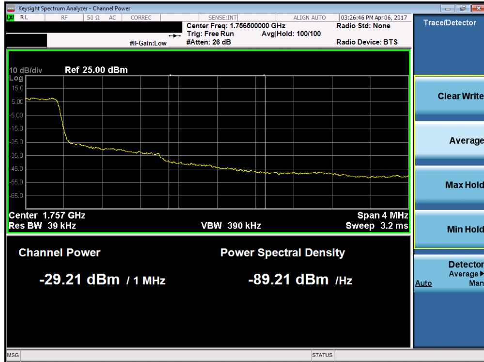
Plot 7-42. Upper Extended Band Edge Plot (Band 4 – 1.4MHz QPSK – RB Size 6)
