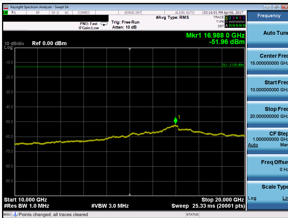
Plot 7-23. Conducted Spurious Plot (Band 4 – 5.0MHz QPSK – RB Size 1, RB Offset 0 – Low Channel)
