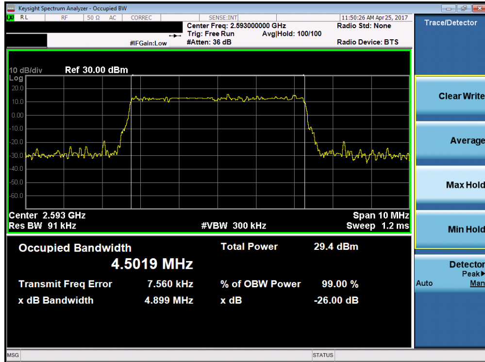
Plot 7-13. Occupied Bandwidth Plot (Band 41 – 5.0MHz QPSK – RB Size 25)
