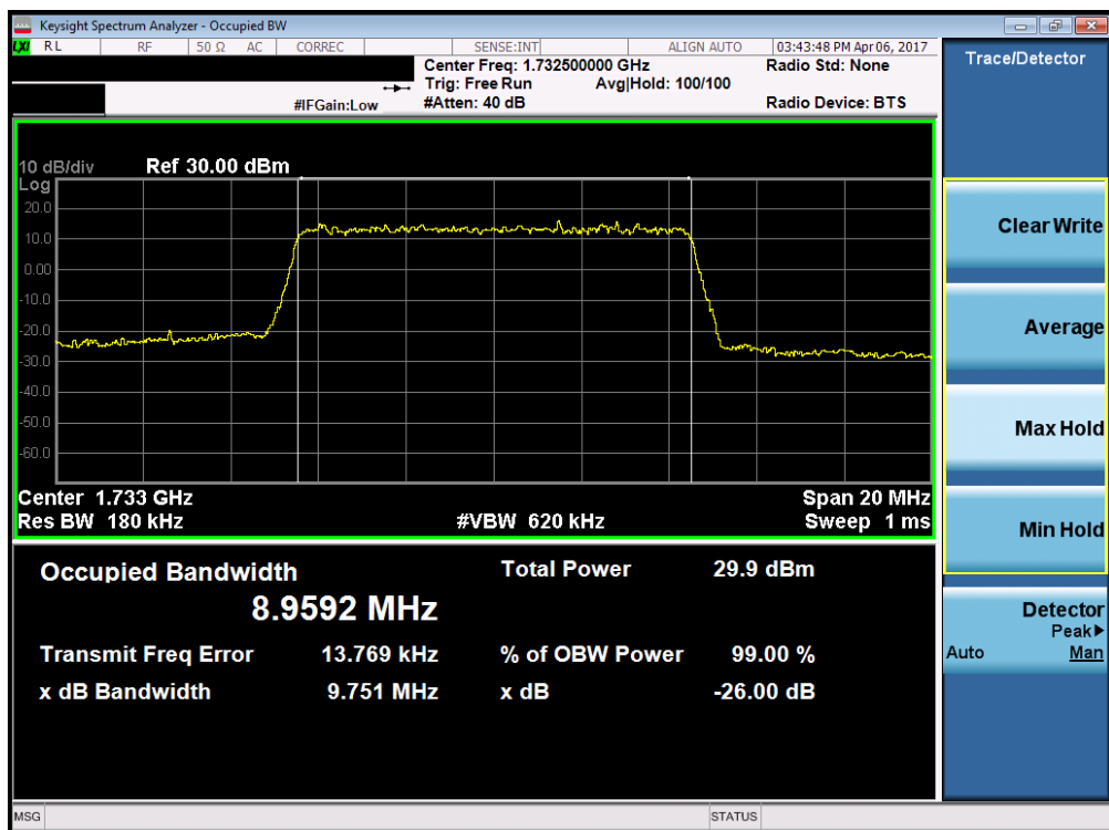
Plot 7-8. Occupied Bandwidth Plot (Band 4 – 10.0MHz 16-QAM – RB Size 50)
