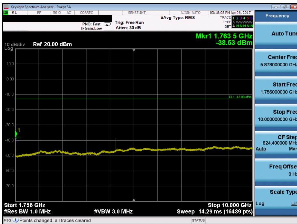
Plot 7-28. Conducted Spurious Plot (Band 4 – 5.0MHz QPSK – RB Size 1, RB Offset 0 – High Channel)
