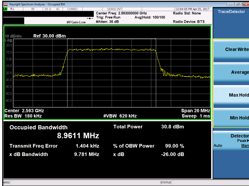
Plot 7-15. Occupied Bandwidth Plot (Band 41 – 10.0MHz QPSK – RB Size 50)
