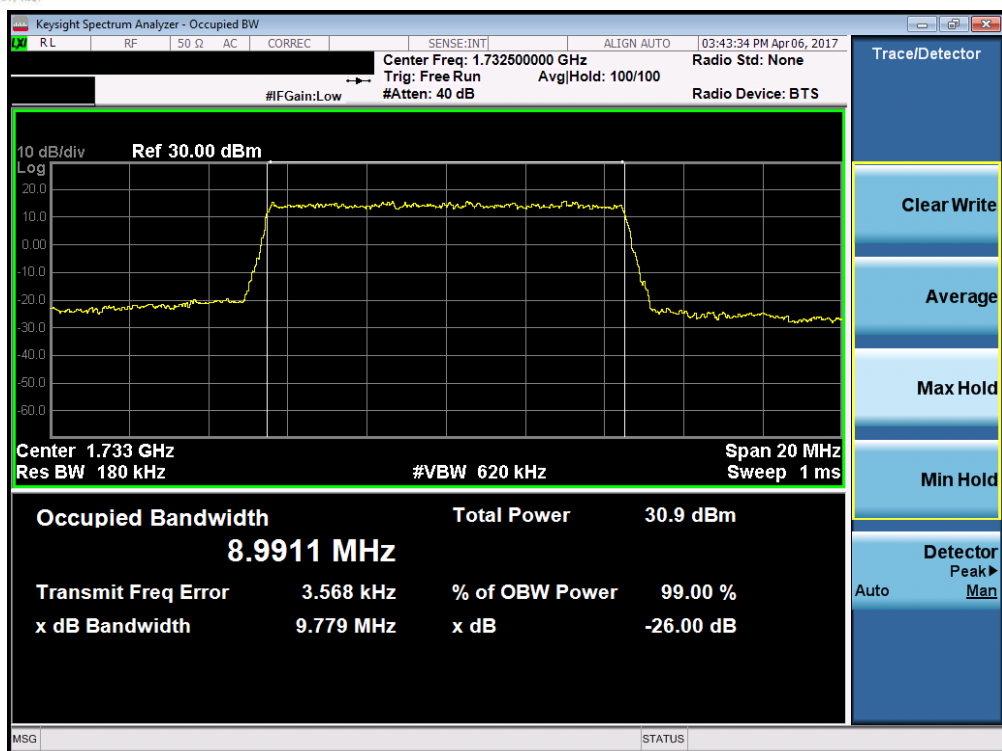
Plot 7-7. Occupied Bandwidth Plot (Band 4 – 10.0MHz QPSK – RB Size 50)
