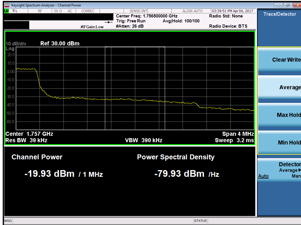
Plot 7-46. Upper Extended Band Edge Plot (Band 4 – 3.0MHz QPSK – RB Size 15)
