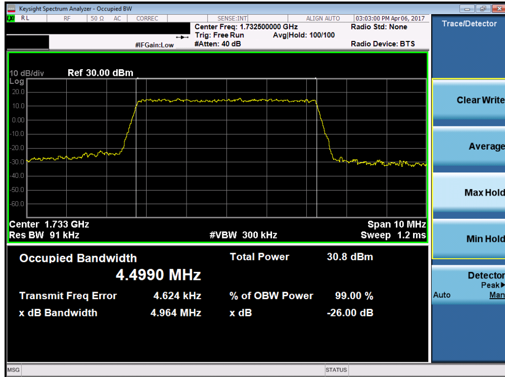
Plot 7-5. Occupied Bandwidth Plot (Band 4 – 5.0MHz QPSK – RB Size 25)
