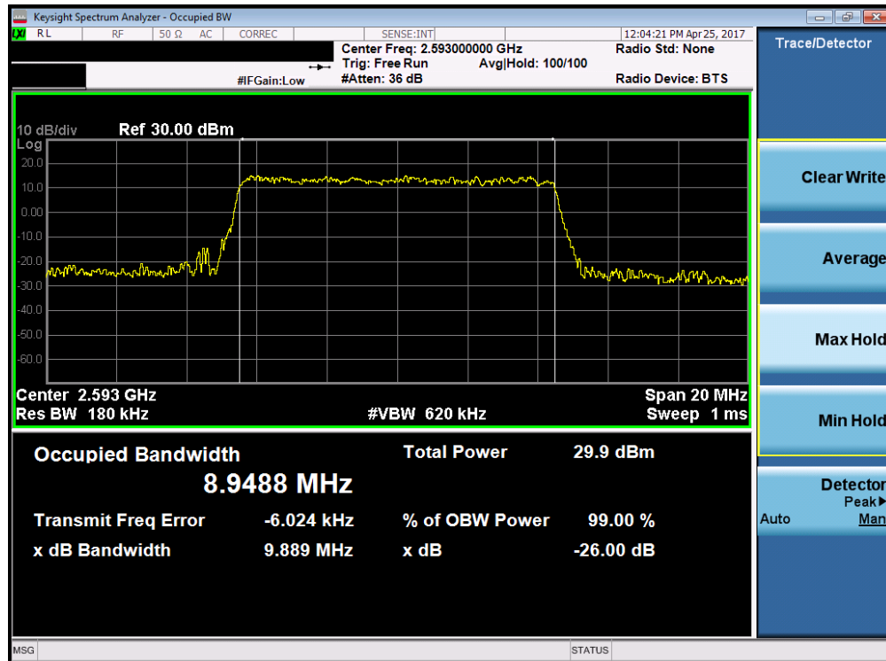
Plot 7-16. Occupied Bandwidth Plot (Band 41 – 10.0MHz 16-QAM – RB Size 50)
