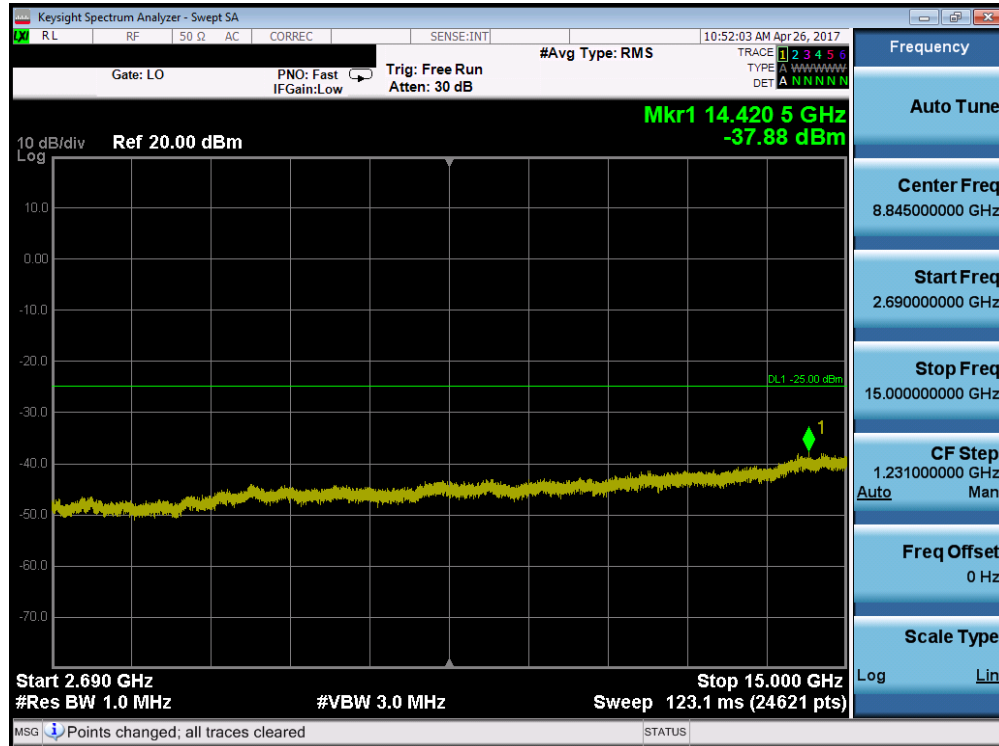
Plot 7-31. Conducted Spurious Plot (Band 41 – 20.0MHz QPSK – RB Size 1, RB Offset 0 – Low Channel)
