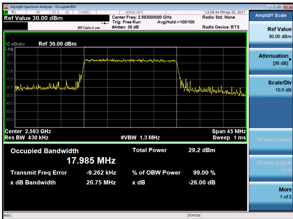
Plot 7-20. Occupied Bandwidth Plot (Band 41 – 20.0MHz 16-QAM – RB Size 100)
