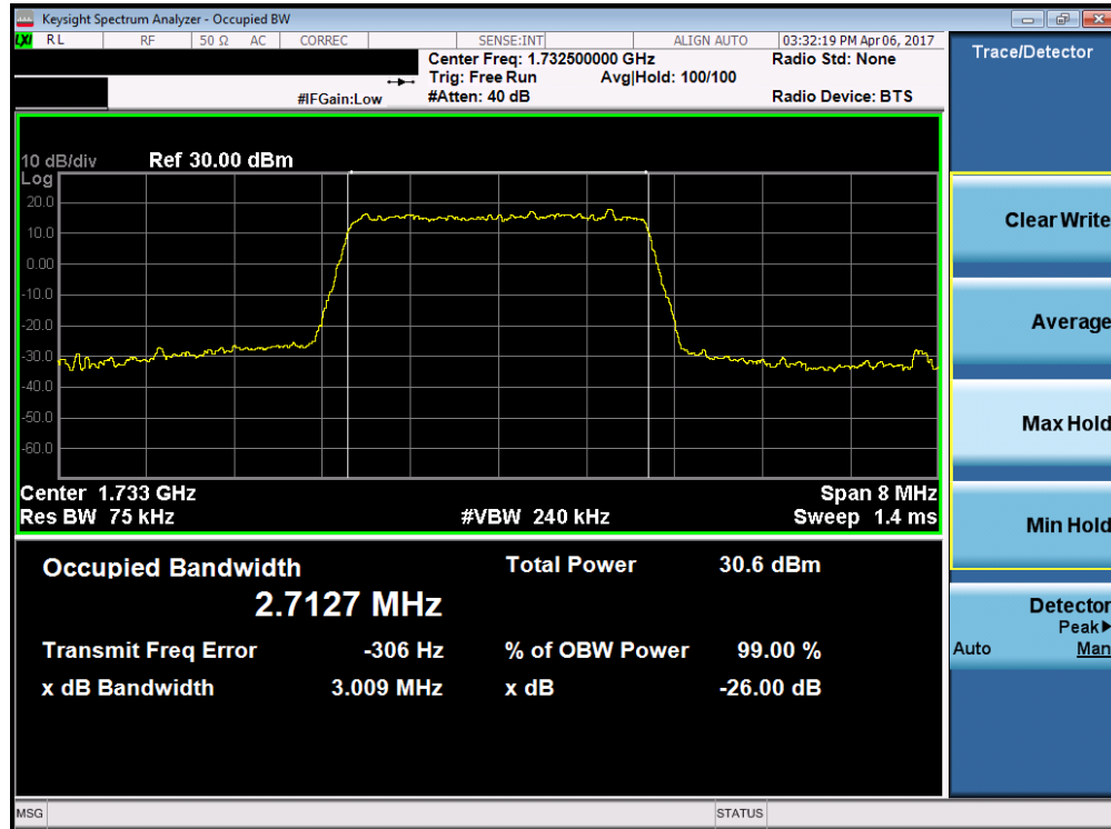
Plot 7-3. Occupied Bandwidth Plot (Band 4 – 3.0MHz QPSK – RB Size 15)
