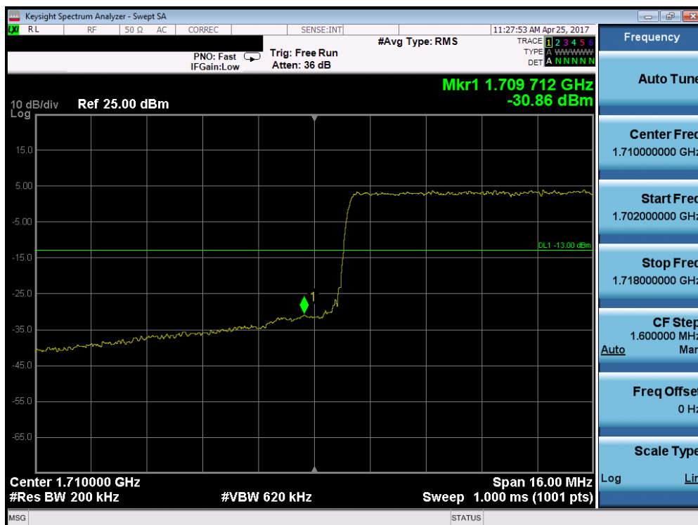
Plot 7-59. Lower Band Edge Plot (Band 4 - 20.0MHz QPSK - RB Size 100)
