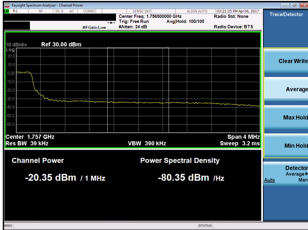
Plot 7-50. Upper Extended Band Edge Plot (Band 4 – 5.0MHz QPSK – RB Size 25)
