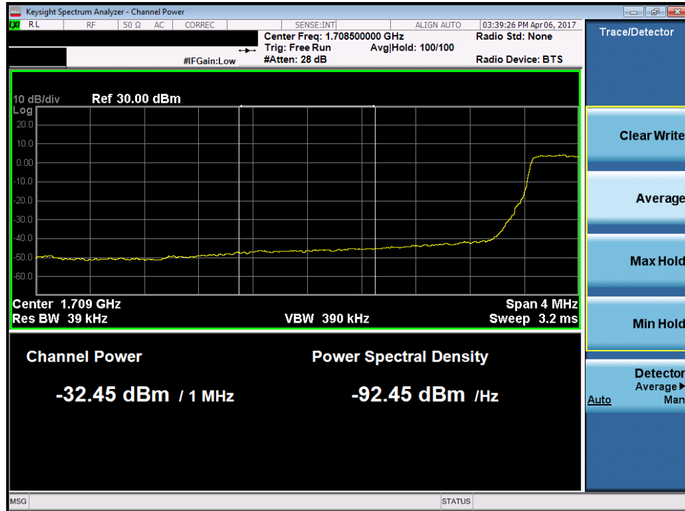
Plot 7-44. Lower Extended Band Edge Plot (Band 4 – 3.0MHz QPSK – RB Size 15)
