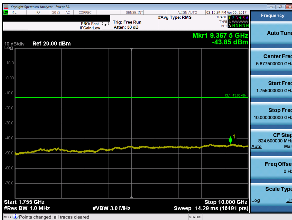
Plot 7-22. Conducted Spurious Plot (Band 4 – 5.0MHz QPSK – RB Size 1, RB Offset 0 – Low Channel)
