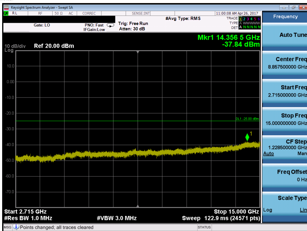
Plot 7-37. Conducted Spurious Plot (Band 41 – 20.0MHz QPSK – RB Size 1, RB Offset 0 – High Channel)
