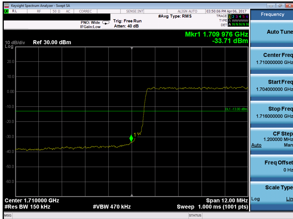
Plot 7-55. Lower Band Edge Plot (Band 4 – 15.0MHz QPSK – RB Size 75)
