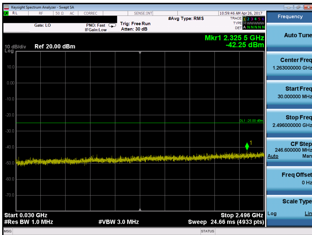
Plot 7-36. Conducted Spurious Plot (Band 41 – 20.0MHz QPSK – RB Size 1, RB Offset 0 – High Channel)
