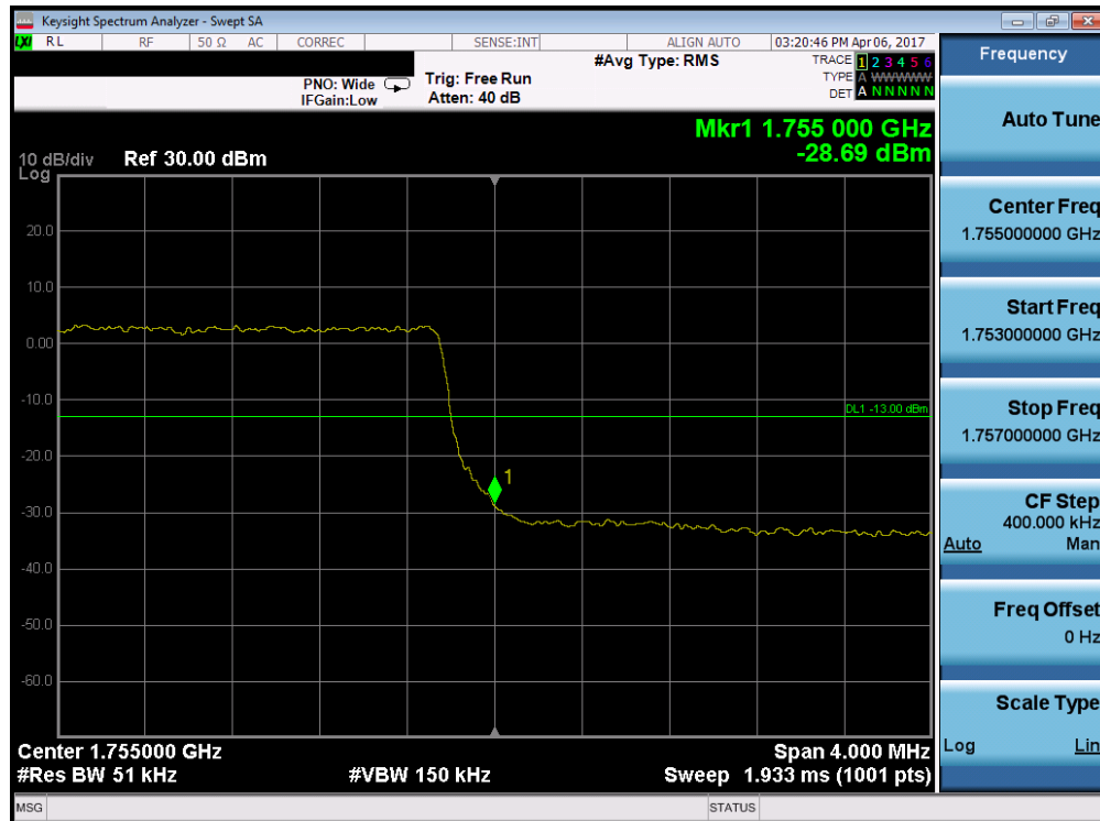
Plot 7-49. Upper Band Edge Plot (Band 4 – 5.0MHz QPSK – RB Size 25)
