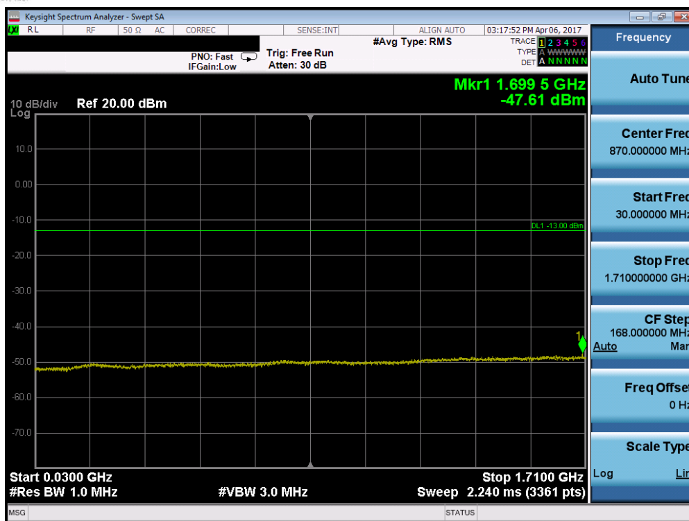
Plot 7-27. Conducted Spurious Plot (Band 4 – 5.0MHz QPSK – RB Size 1, RB Offset 0 – High Channel)
