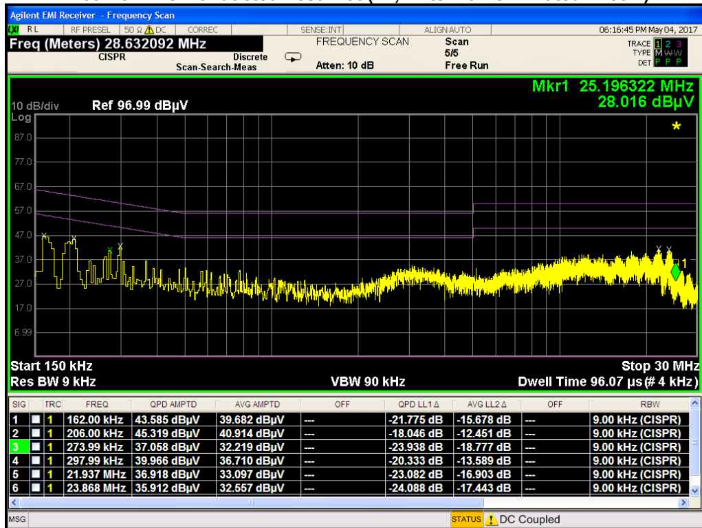
Plot 7-4. Line-Conducted Test Plot (N, Antenna Terminated in 50 \Omega )
