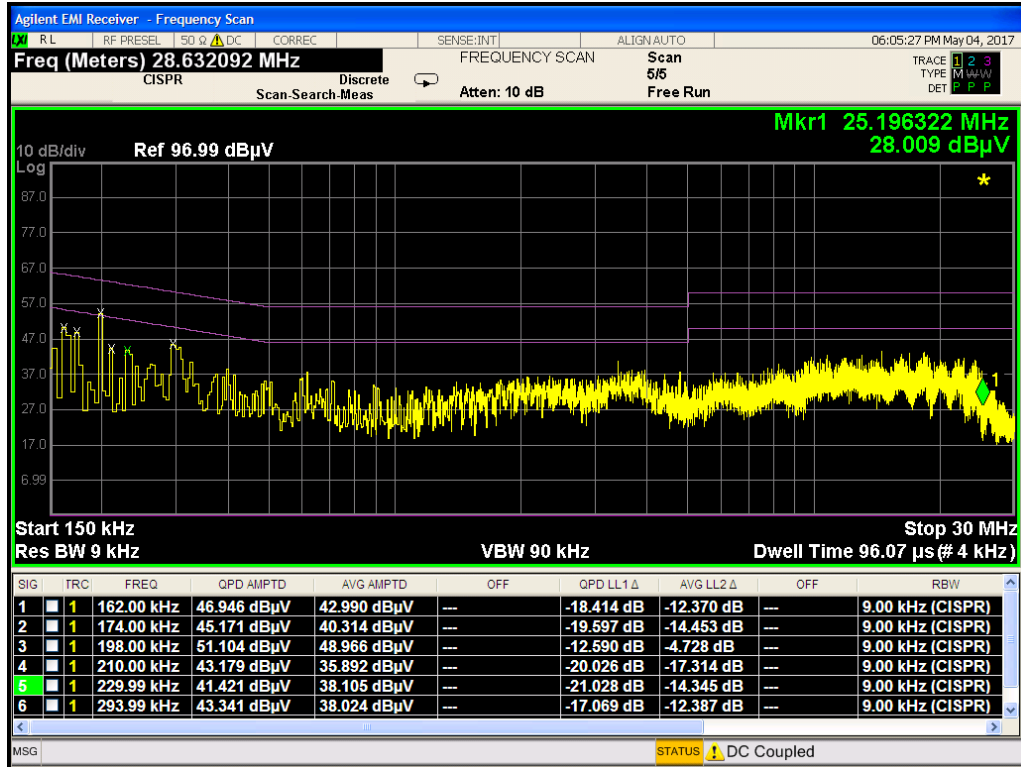
Plot 7-3. Line-Conducted Test Plot (L1, Antenna Terminated in 50 \Omega )
