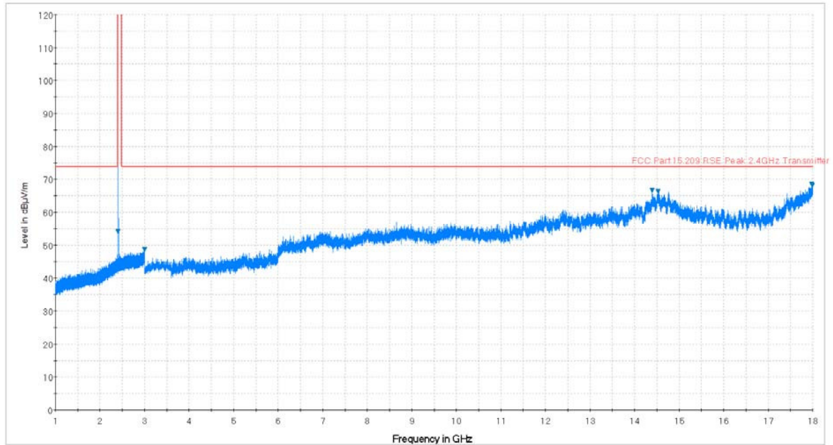
Plot 7-42. Radiated Spurious Plot above 1GHz (BT – Ch. 0, Ant. Pol. H)
