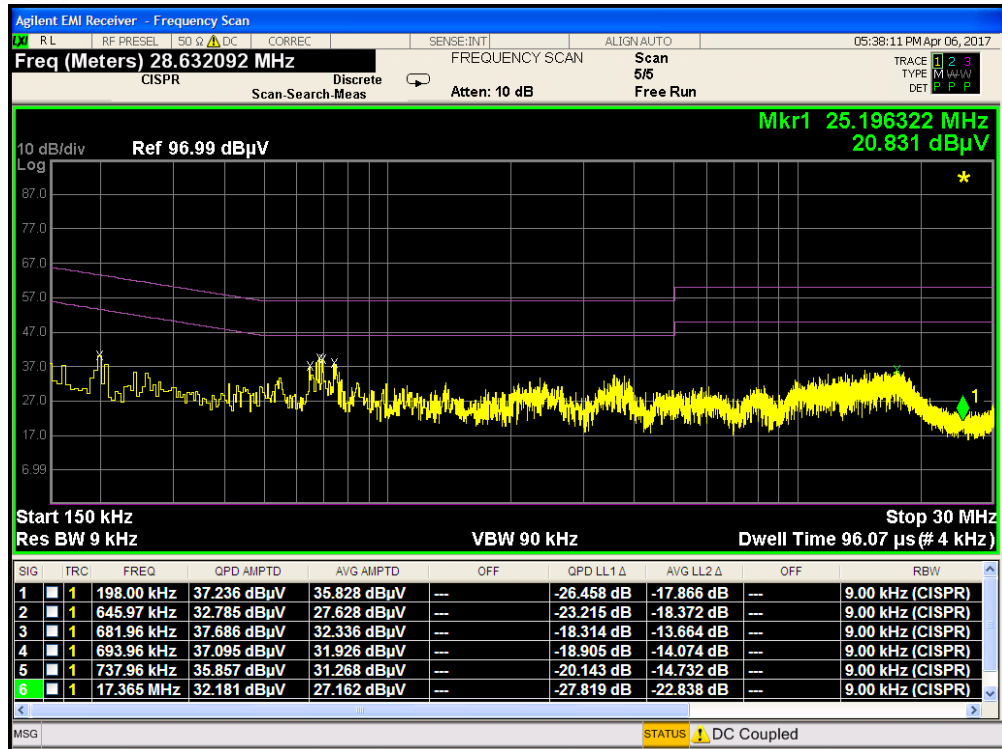
Plot 7-122. Line Conducted Plot with 802.11a UNII Band 2A (L1)
