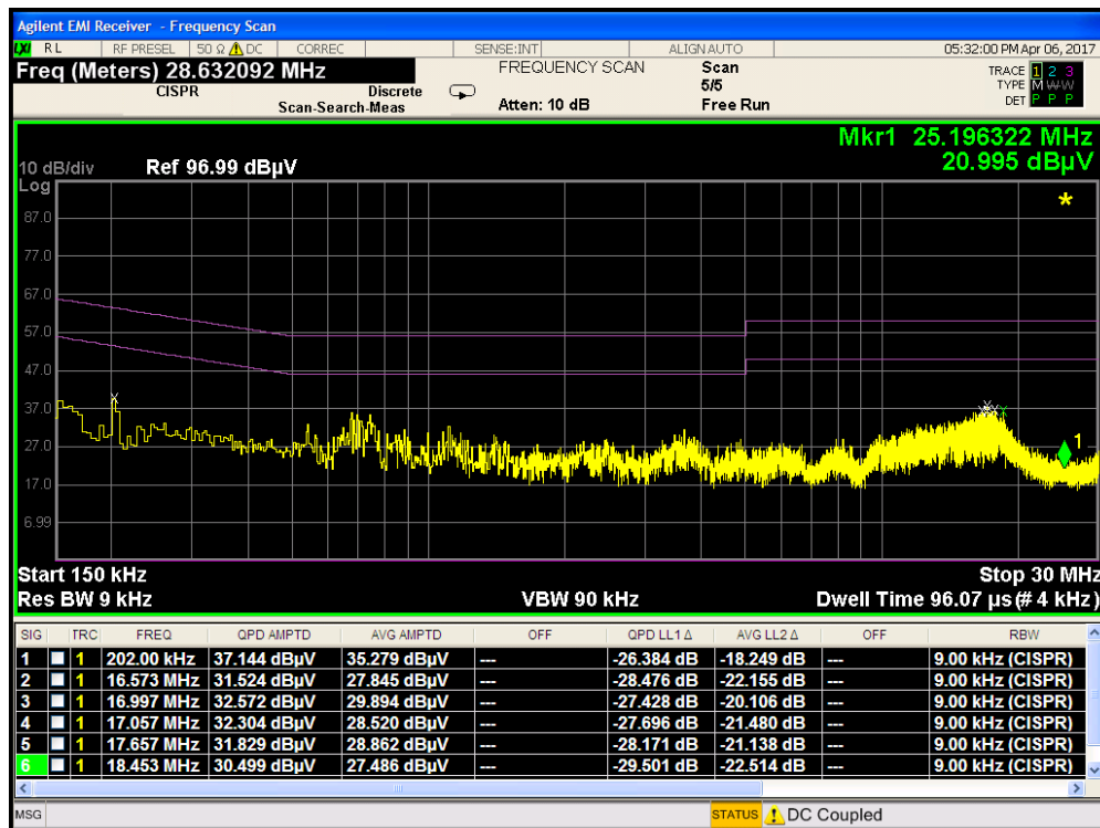
Plot 7-121. Line Conducted Plot with 802.11a UNII Band 1 (N)
