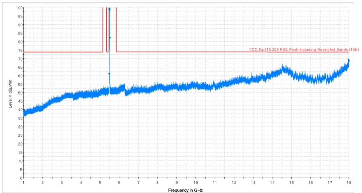
Plot 7-84. Radiated Spurious Plot above 1GHz (802.11a – U2C Ch. 120, Ant. Pol. V)
