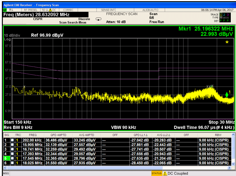
Plot 7-127. Line Conducted Plot with 802.11a UNII Band 3 (N)
