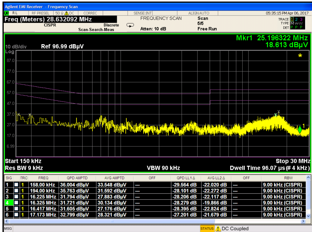
Plot 7-123. Line Conducted Plot with 802.11a UNII Band 2A (N)
