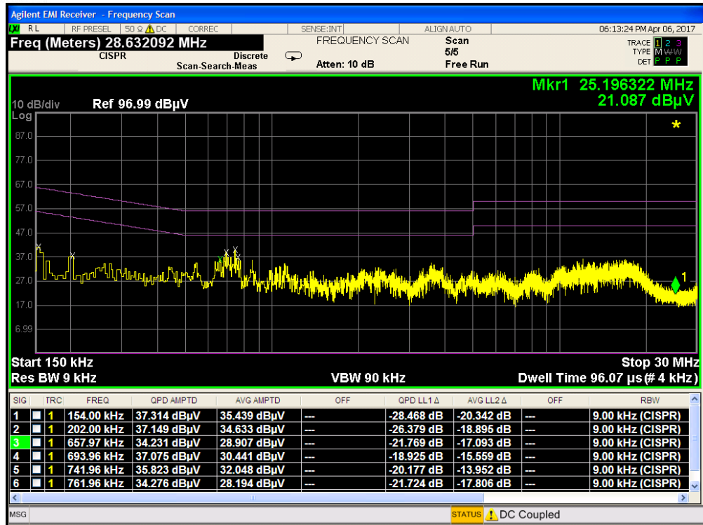
Plot 7-126. Line Conducted Plot with 802.11a UNII Band 3 (L1)
