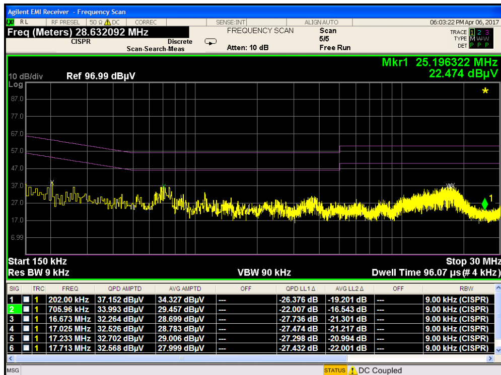
Plot 7-125. Line Conducted Plot with 802.11a UNII Band 2C (N)
