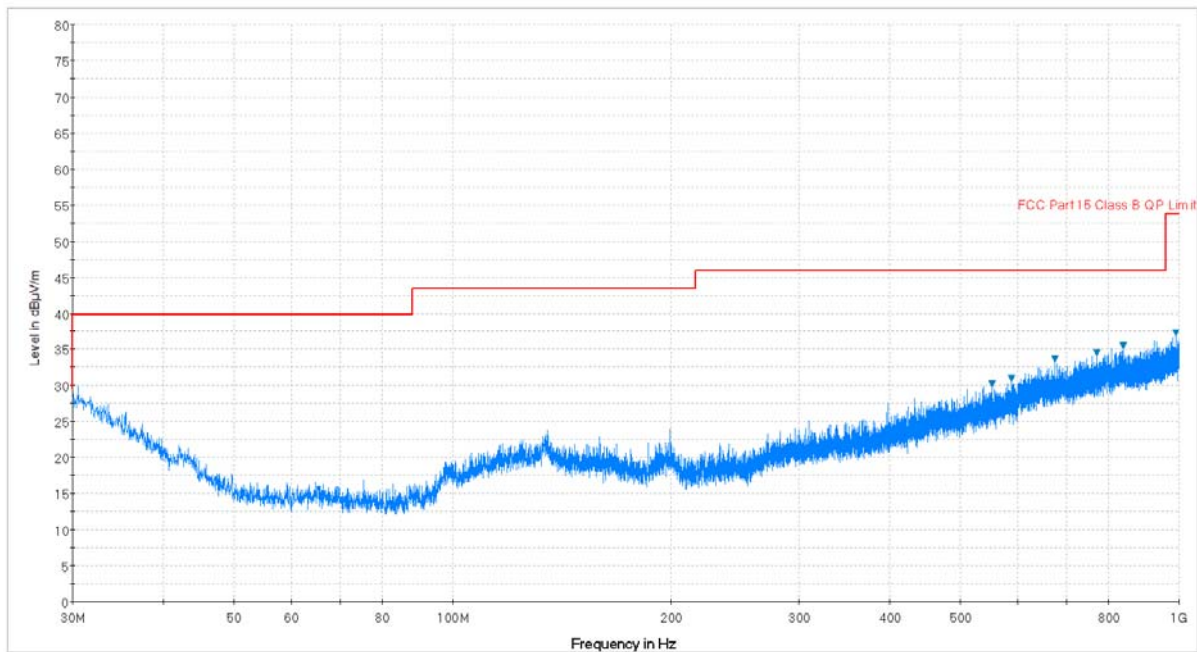
Plot 7-119. Radiated Spurious Plot below 1GHz (802.11a – U3 Ch. 157, Ant. Pol. V)
