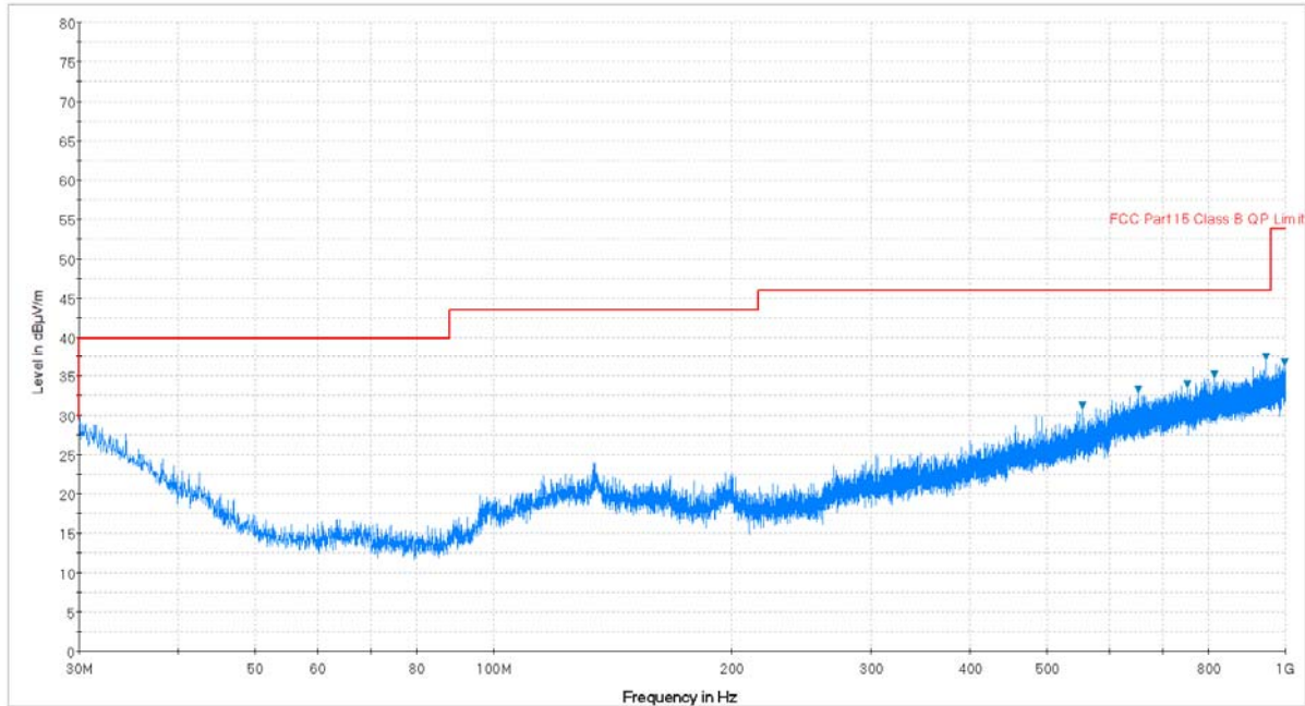
Plot 7-118. Radiated Spurious Plot below 1GHz (802.11a – U3 Ch. 157, Ant. Pol. H)
