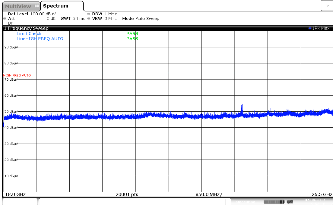
Plot 7-87. Radiated Spurious Plot 18GHz - 26.5GHz (802.11a – Ant. Pol. H)
