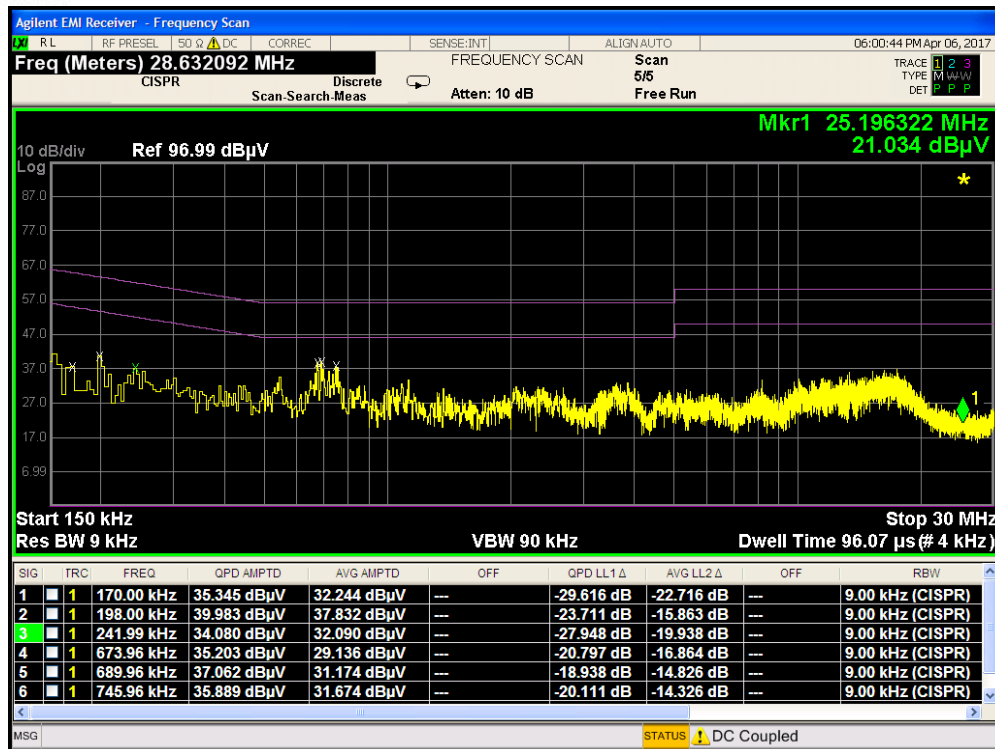
Plot 7-124. Line Conducted Plot with 802.11a UNII Band 2C (L1)
