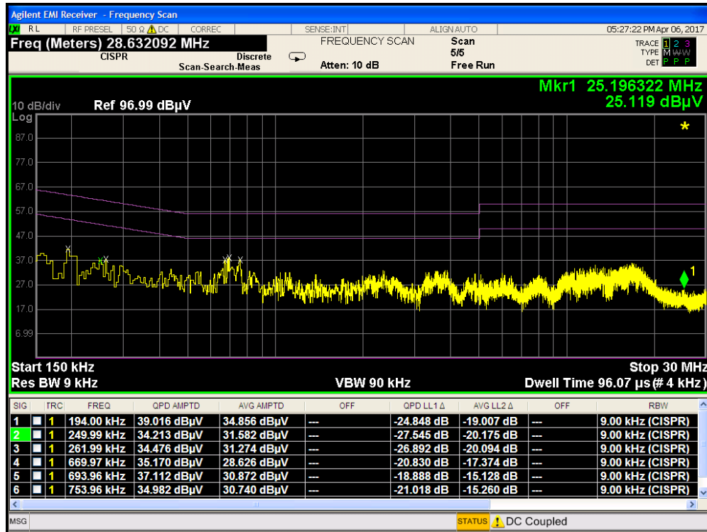
Plot 7-120. Line Conducted Plot with 802.11a UNII Band 1 (L1)
