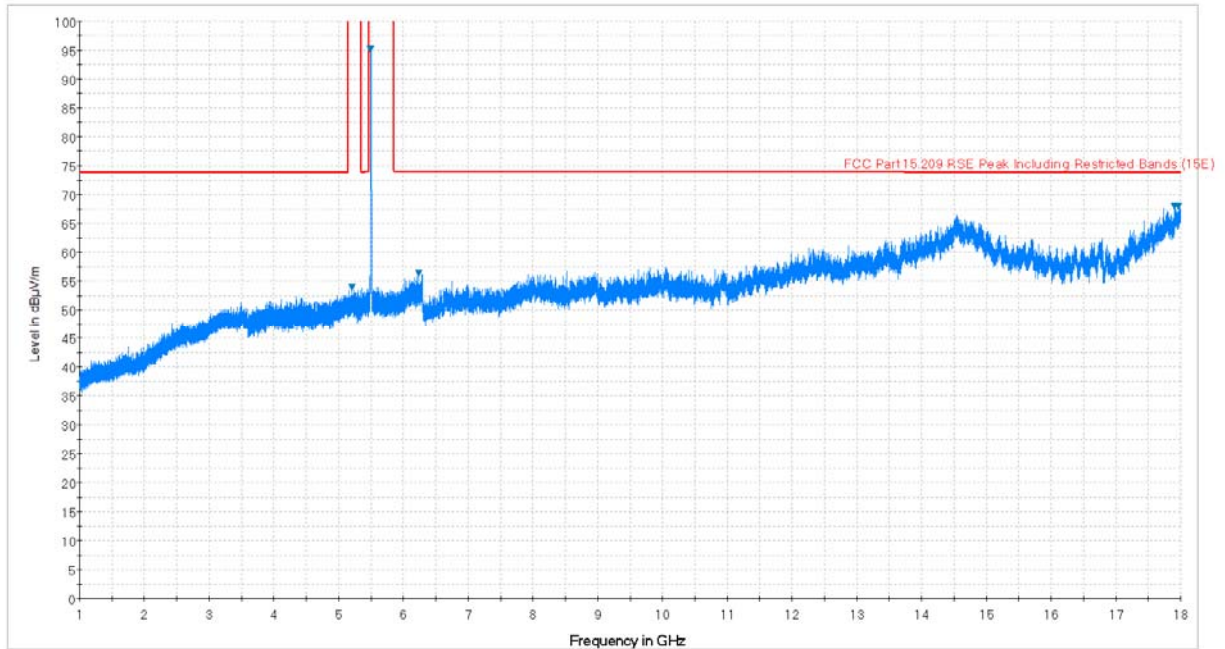
Plot 7-83. Radiated Spurious Plot above 1GHz (802.11a – U2C Ch. 120, Ant. Pol. H)
