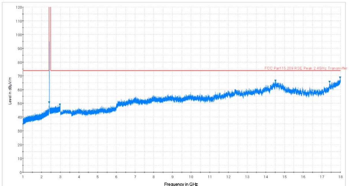
Plot 7-32. Radiated Spurious Plot above 1GHz (802.11b – Ch. 1, Ant. Pol. V)
