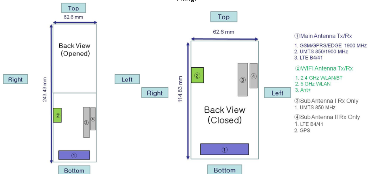
Figure F-1 DUT Antenna Locations
