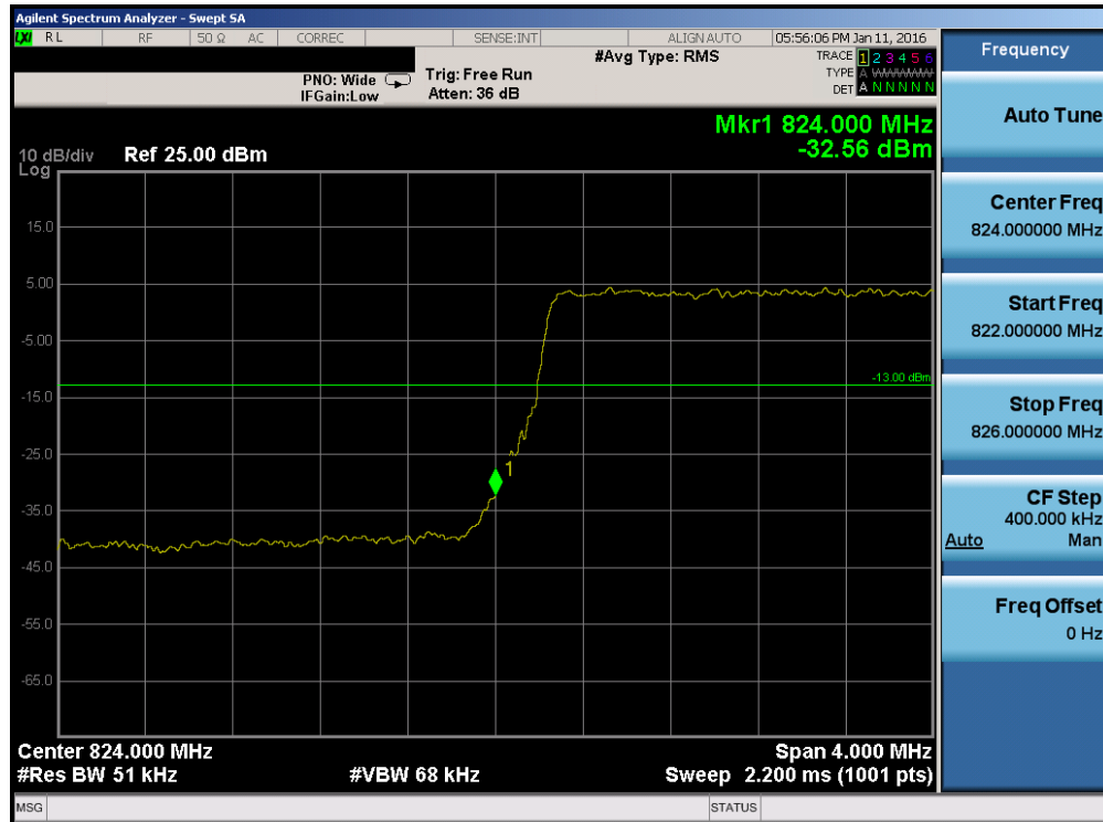
Plot 7-137. Lower Band Edge Plot (Band 5/26 – 5.0MHz QPSK – RB Size 25)
