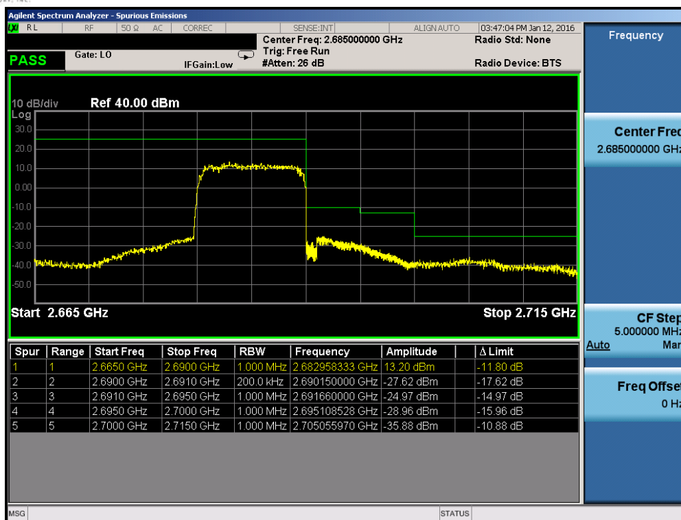
Plot 7-196. Upper ACP Plot (Band 41 – 10.0MHz QPSK – RB Size 50)
