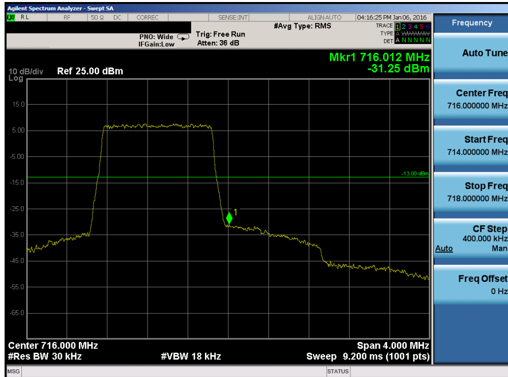
Plot 7-111. Upper Band Edge Plot (Band 12 – 1.4MHz QPSK – RB Size 6)
