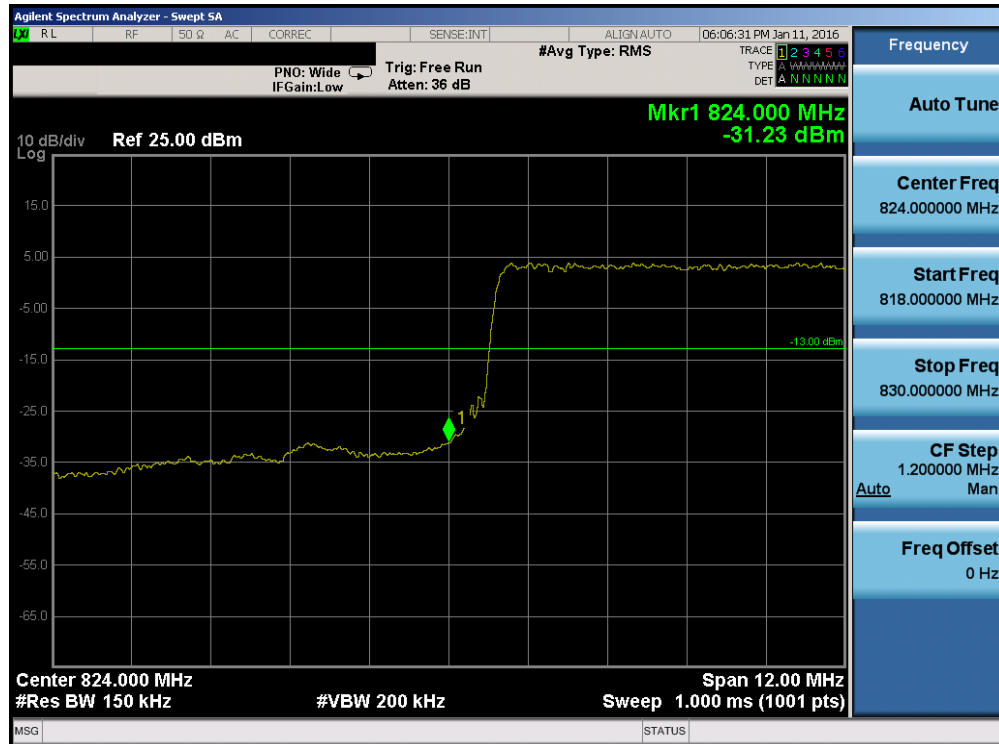
Plot 7-143. Lower Band Edge Plot (Band 26 – 15.0MHz QPSK – RB Size 75)
