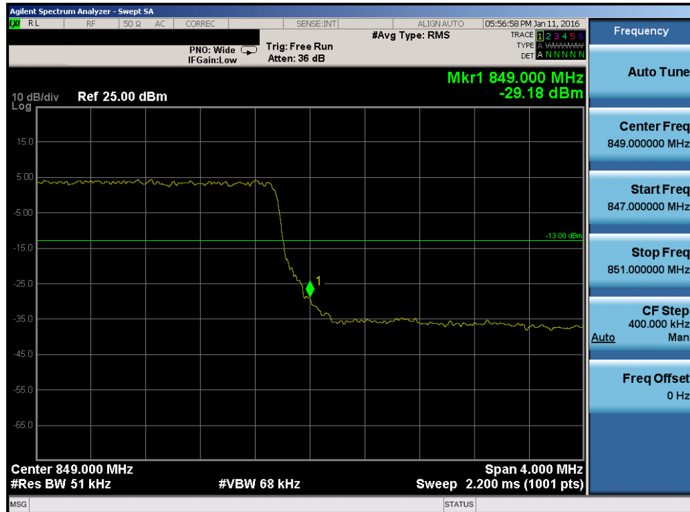
Plot 7-139. Upper Band Edge Plot (Band 5/26 - 5.0MHz QPSK - RB Size 25)
