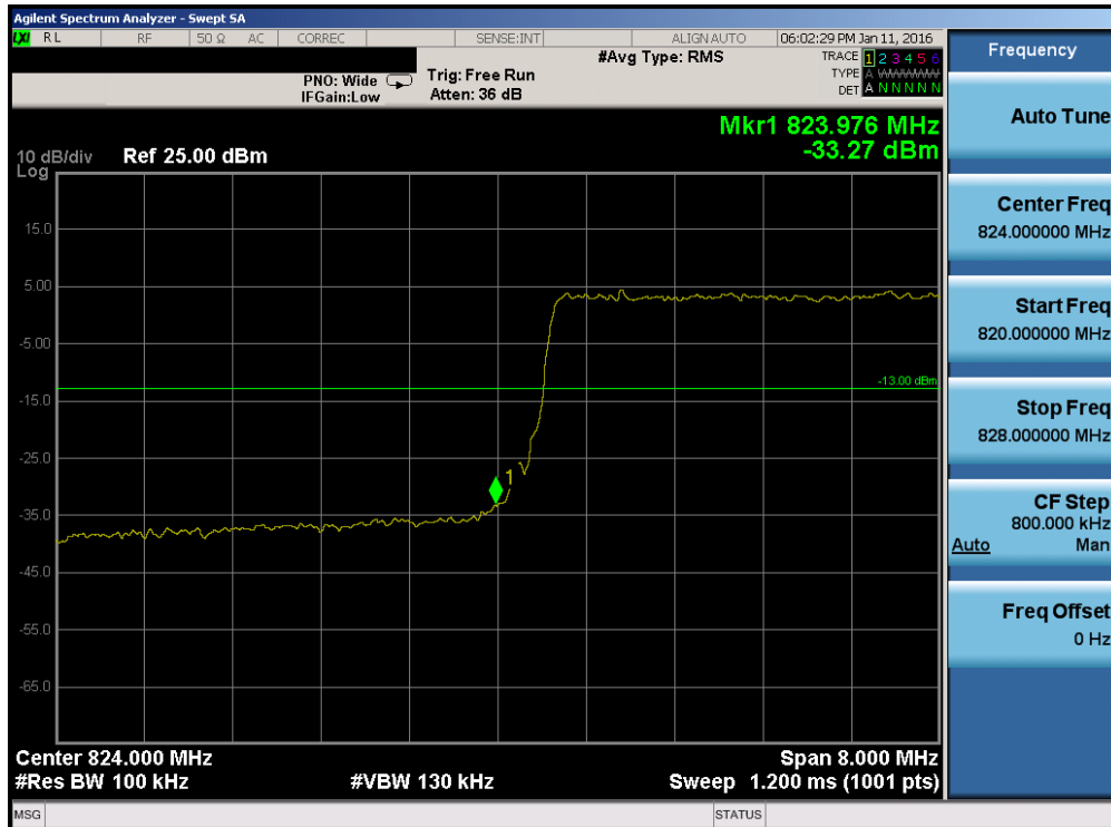
Plot 7-141. Lower Band Edge Plot (Band 5/26 - 10.0MHz QPSK - RB Size 50)
