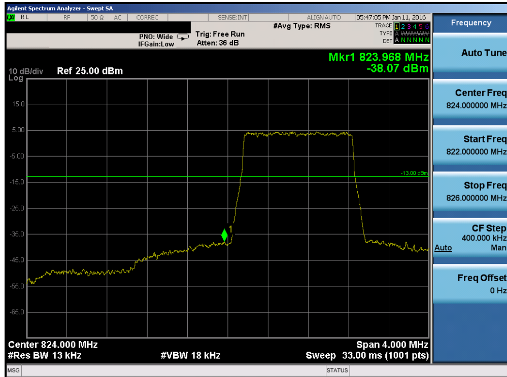
Plot 7-129. Lower Band Edge Plot (Band 5/26 – 1.4MHz QPSK – RB Size 6)
