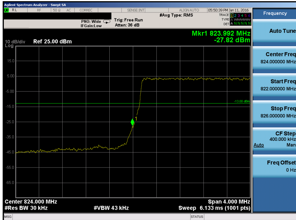
Plot 7-133. Lower Band Edge Plot (Band 5/26 - 3.0MHz QPSK - RB Size 15)
