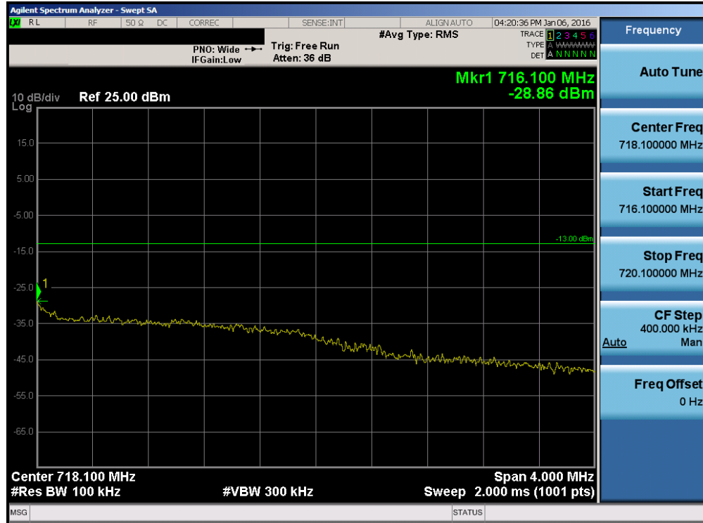
Plot 7-116. Upper Extended Band Edge Plot (Band 12 – 3.0MHz QPSK – RB Size 15)
