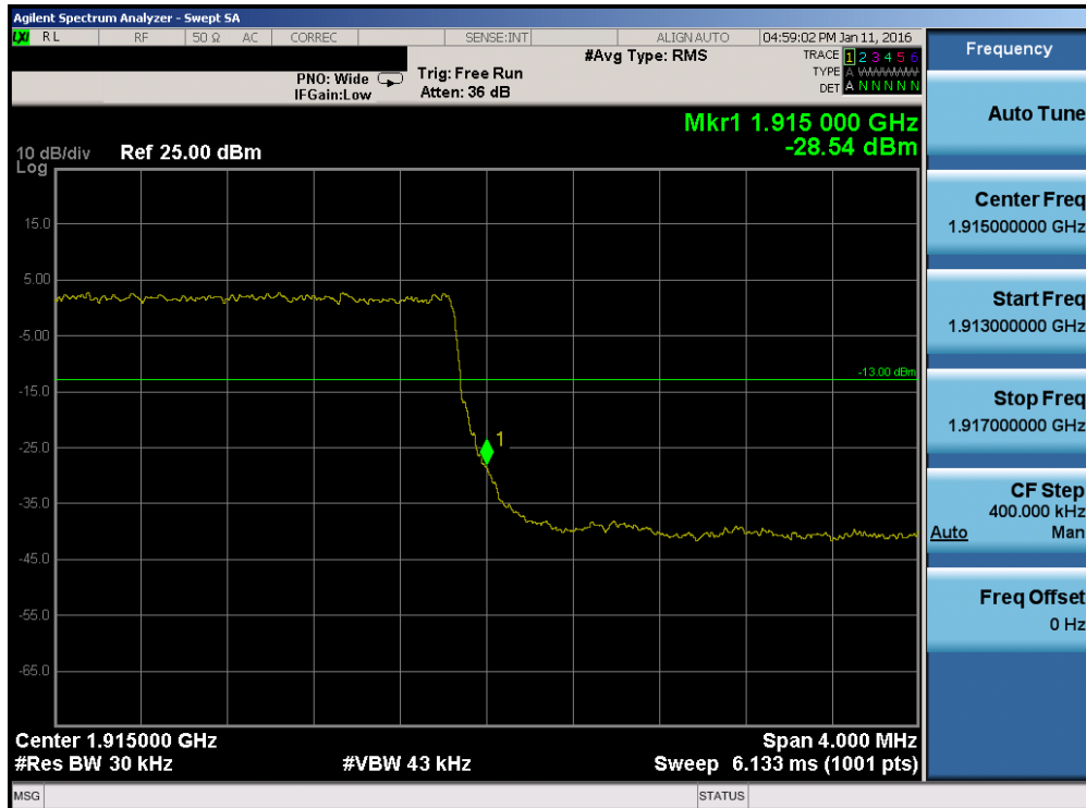
Plot 7-175. Upper Band Edge Plot (Band 2/25 – 3.0MHz QPSK – RB Size 15)
