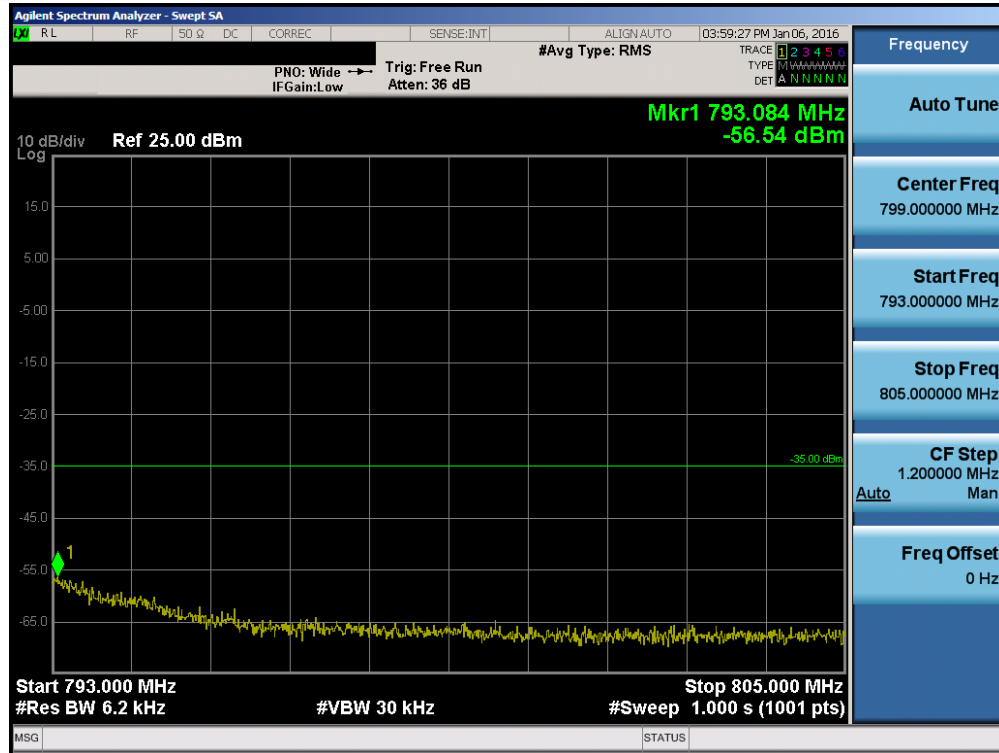
Plot 7-126. Upper Emission Mask Edge Plot (Band 13 - 5.0MHz QPSK - RB Size 25)
