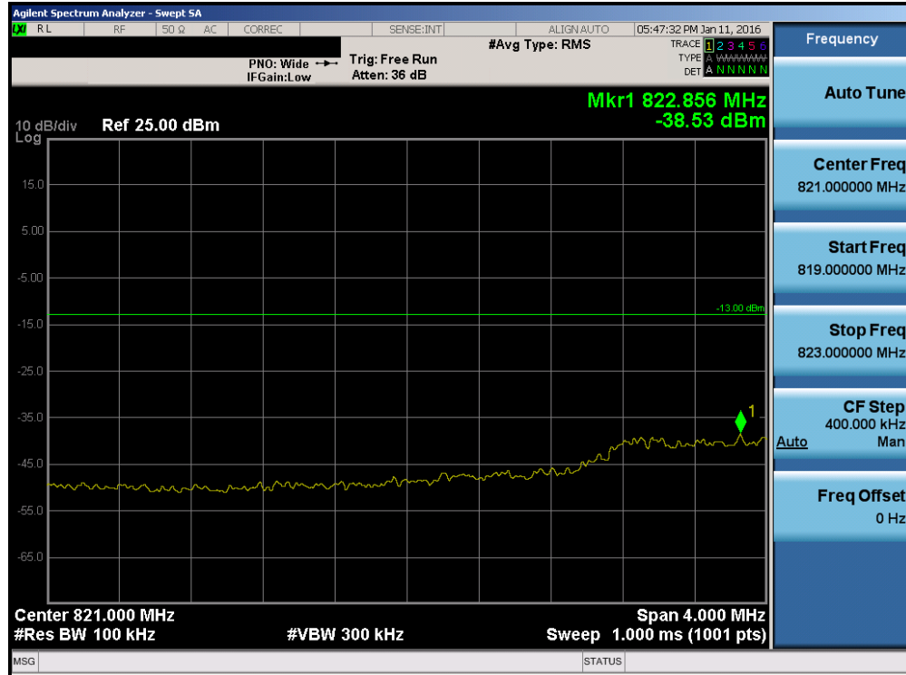
Plot 7-130. Lower Extended Band Edge Plot (Band 5/26 – 1.4MHz QPSK – RB Size 6)
