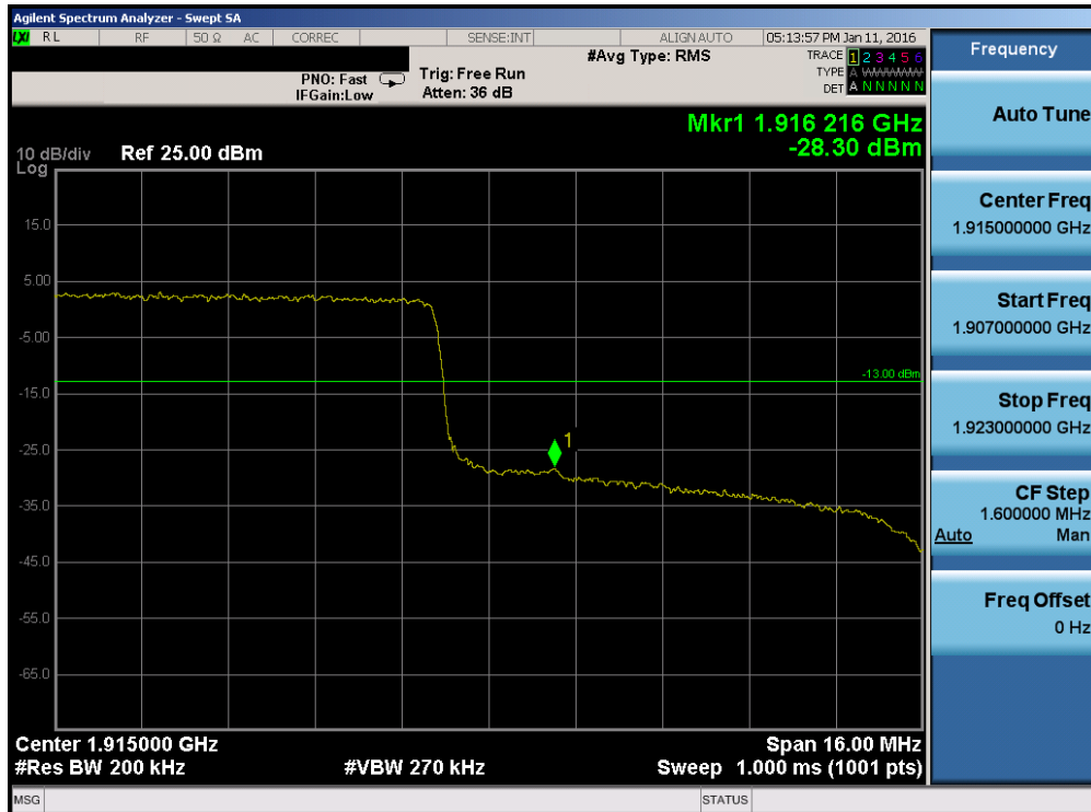
Plot 7-191. Upper Band Edge Plot (Band 2/25 – 20.0MHz QPSK – RB Size 100)
