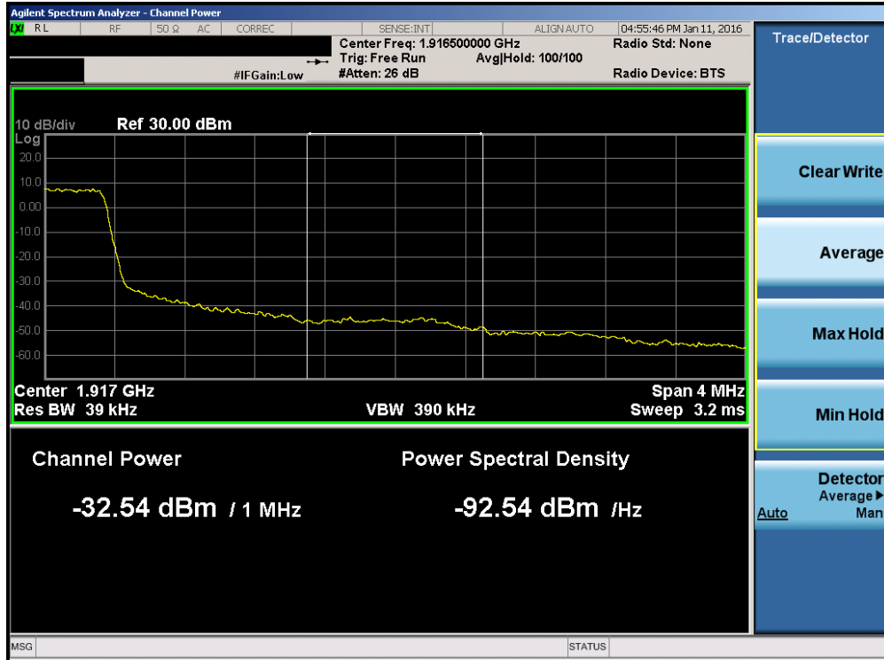
Plot 7-172. Upper Extended Band Edge Plot (Band 2/25 – 1.4MHz QPSK – RB Size 6)
