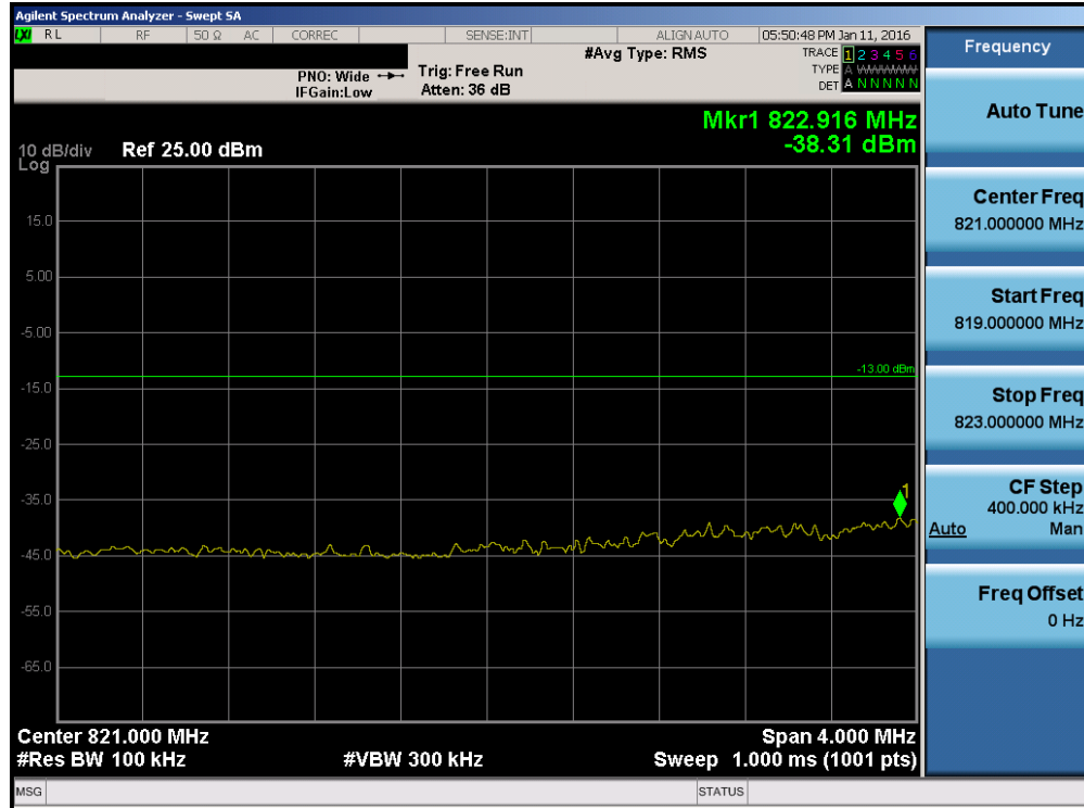
Plot 7-134. Lower Extended Band Edge Plot (Band 5/26 - 3.0MHz QPSK - RB Size 15)
