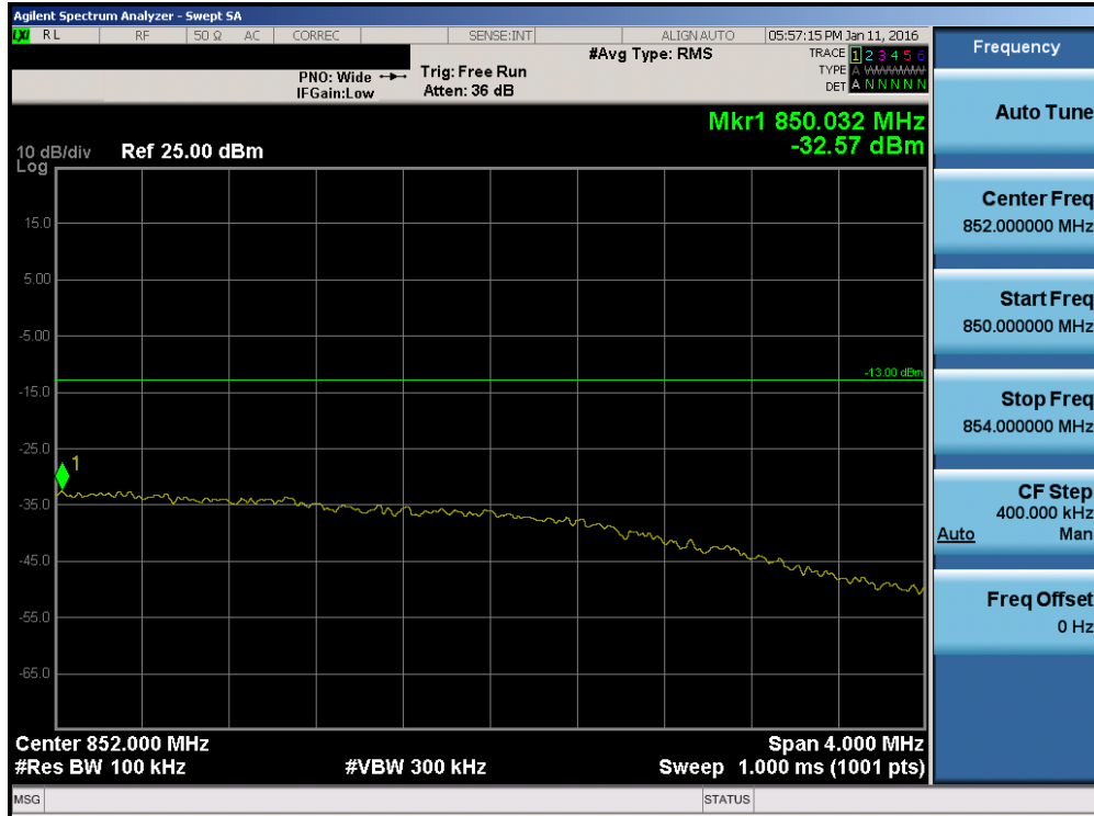
Plot 7-140. Upper Extended Band Edge Plot (Band 5/26 - 5.0MHz QPSK - RB Size 25)
