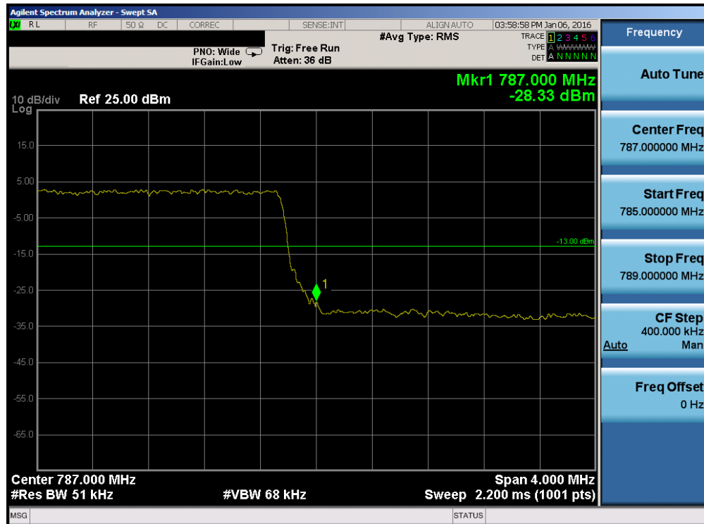
Plot 7-125. Upper Band Edge Plot (Band 13 – 5.0MHz QPSK – RB Size 25)
