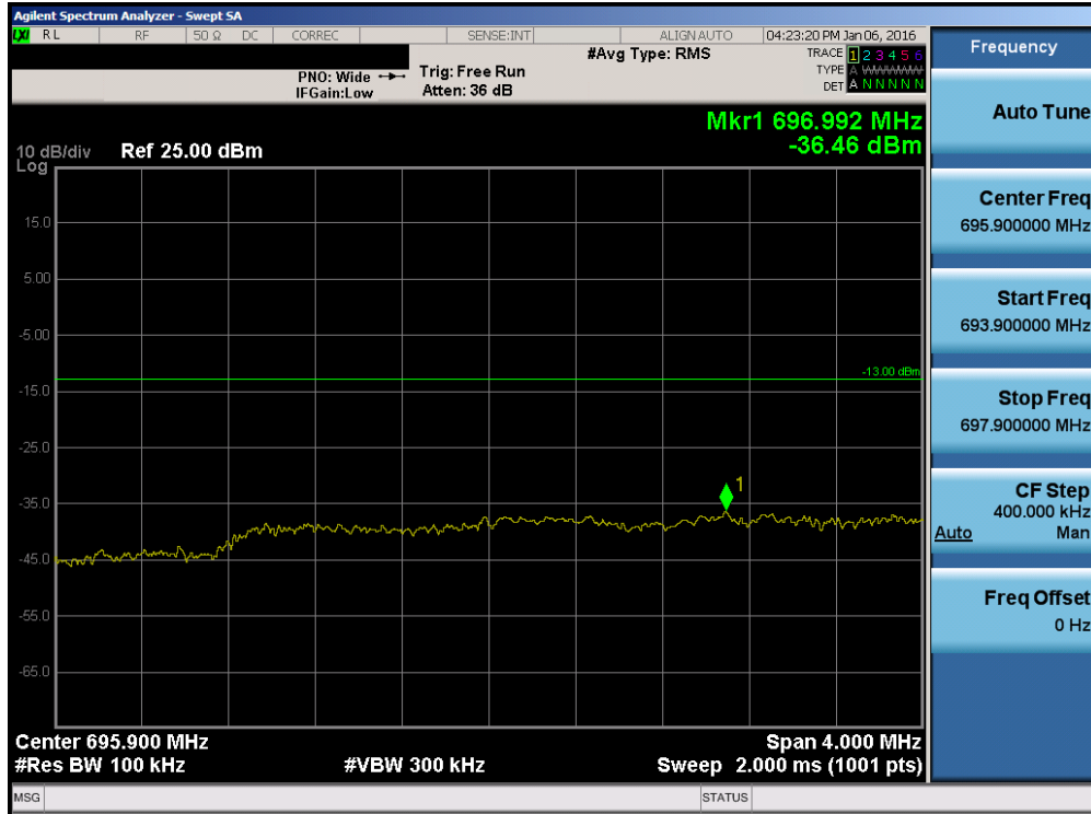
Plot 7-118. Lower Extended Band Edge Plot (Band 12/17 - 5.0MHz QPSK - RB Size 25)
