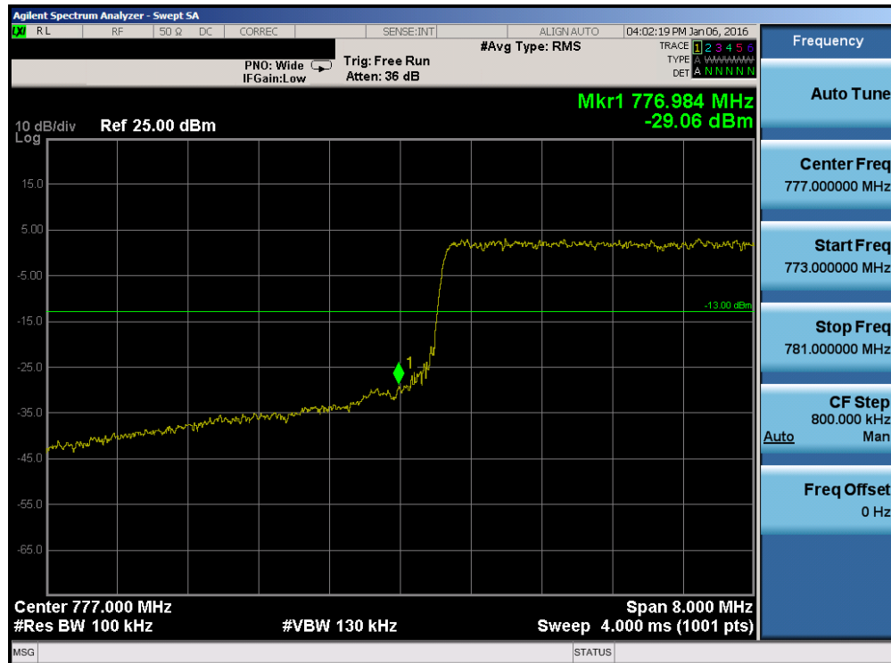
Plot 7-127. Lower Band Edge Plot (Band 13 - 10.0MHz QPSK - RB Size 50)
