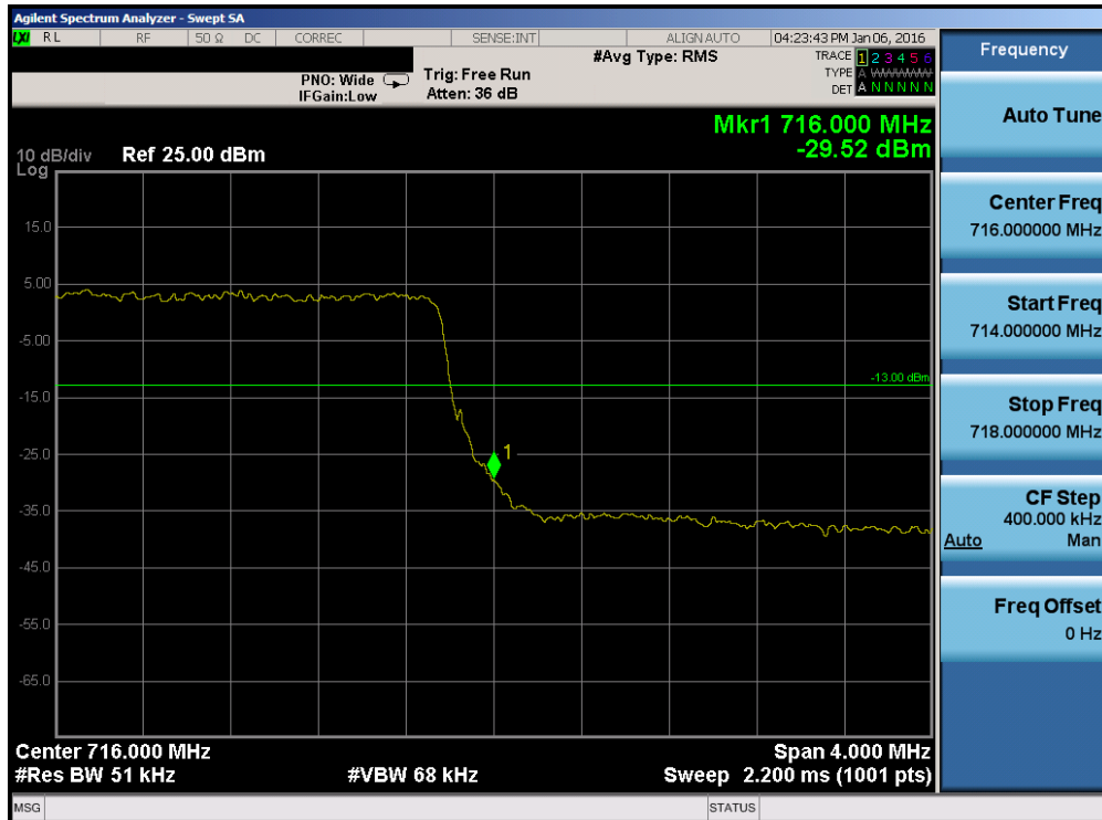
Plot 7-119. Upper Band Edge Plot (Band 12/17 - 5.0MHz QPSK - RB Size 25)
