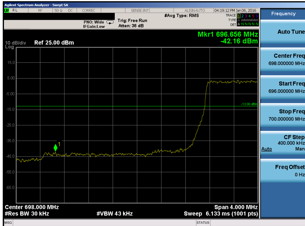
Plot 7-113. Lower Band Edge Plot (Band 12 – 3.0MHz QPSK – RB Size 15)
