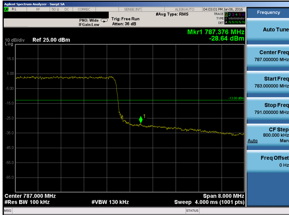
Plot 7-128. Upper Band Edge Plot (Band 13 – 10.0MHz QPSK – RB Size 50)
