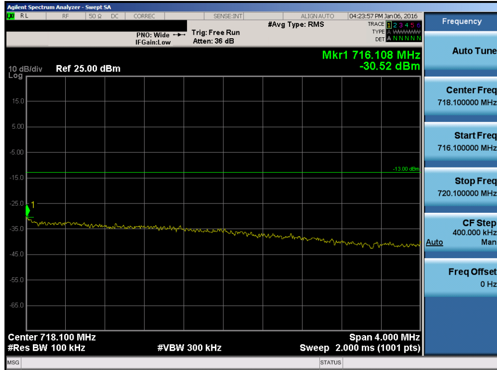
Plot 7-120. Upper Extended Band Edge Plot (Band 12/17 - 5.0MHz QPSK - RB Size 25)
