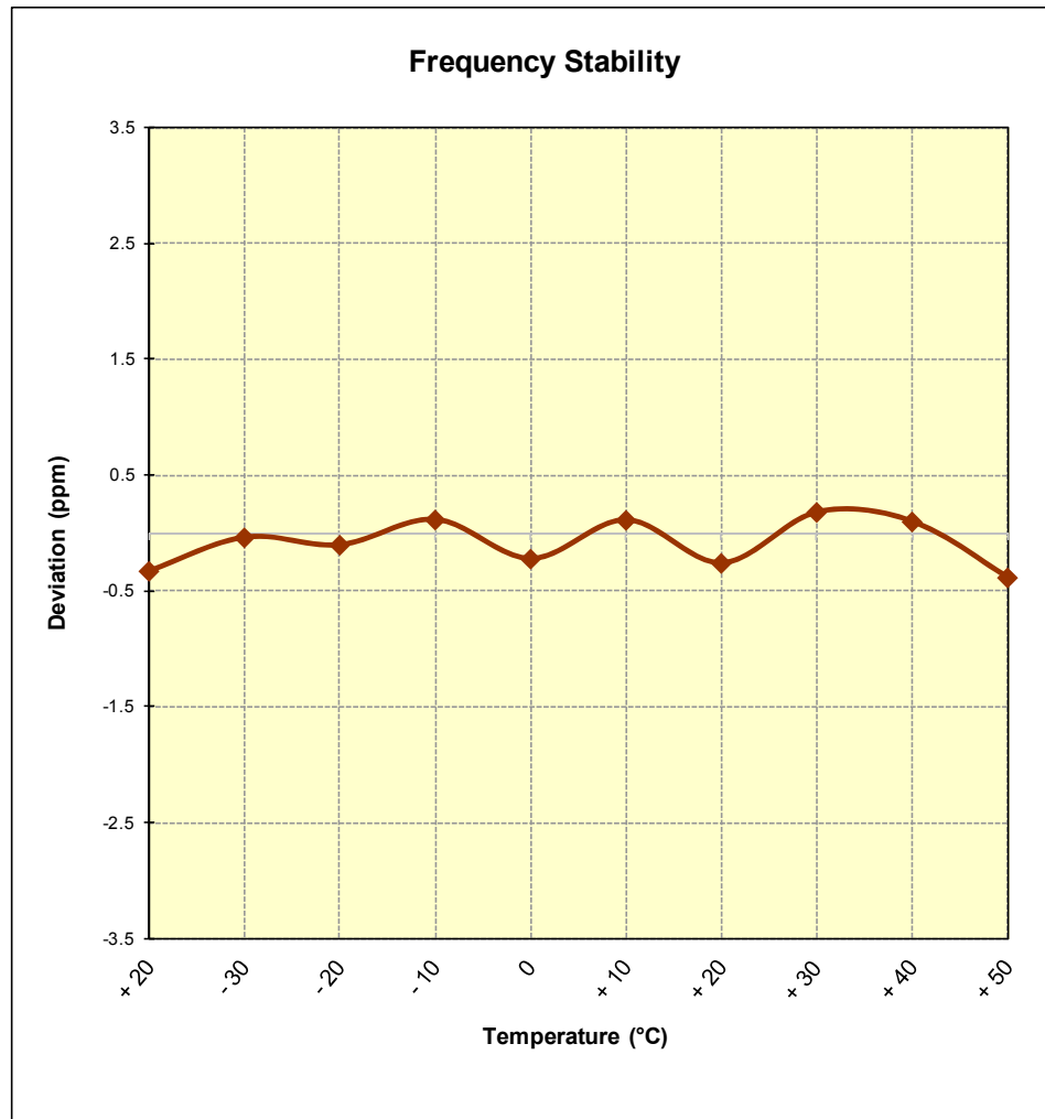
Figure 7-10. Frequency Stability Graph (Band 5/26)
