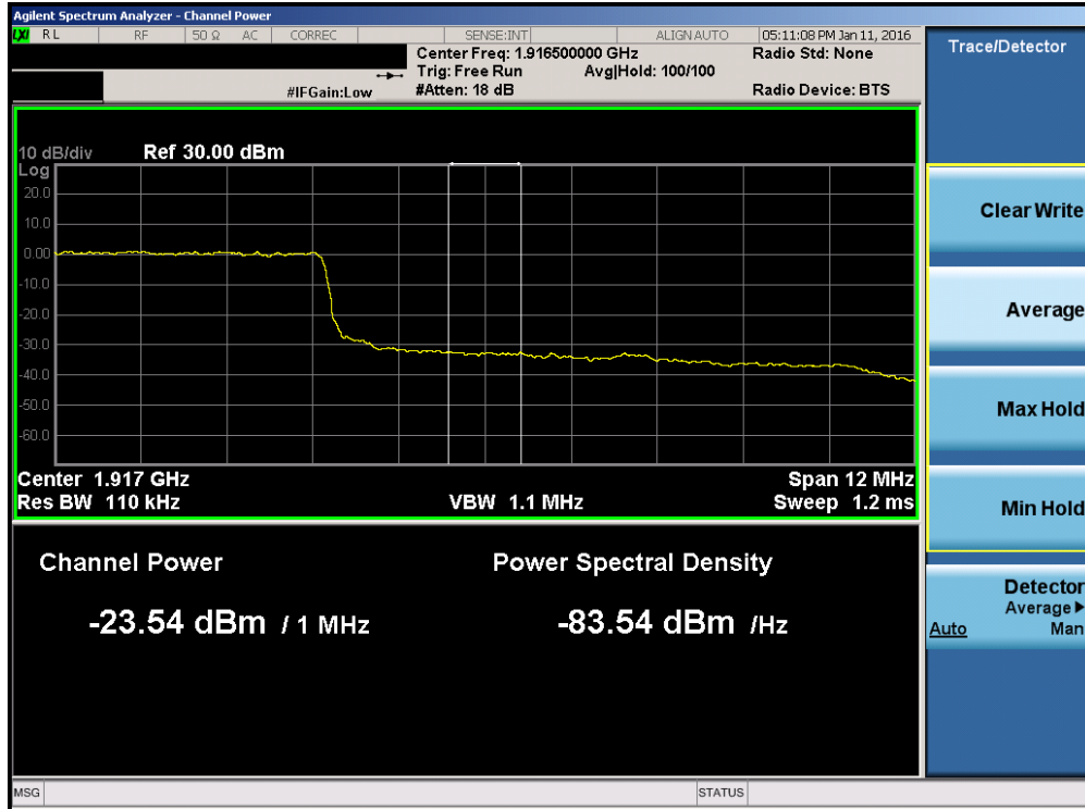
Plot 7-188. Upper Extended Band Edge Plot (Band 2/25 – 15.0MHz QPSK – RB Size 75)
