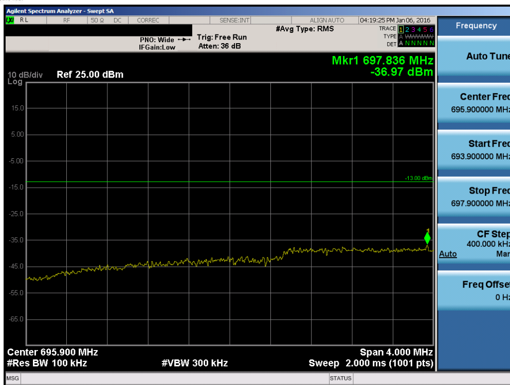
Plot 7-114. Lower Extended Band Edge Plot (Band 12 – 3.0MHz QPSK – RB Size 15)
