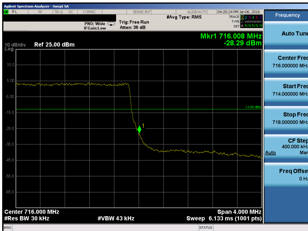
Plot 7-115. Upper Band Edge Plot (Band 12 – 3.0MHz QPSK – RB Size 15)
