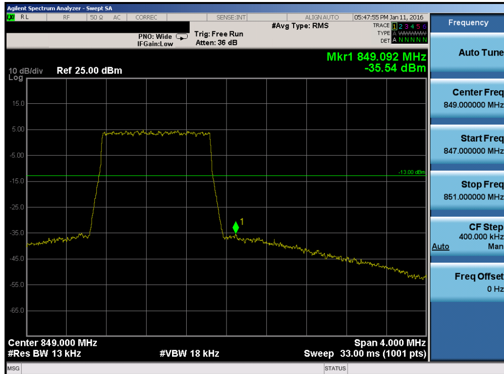
Plot 7-131. Upper Band Edge Plot (Band 5/26 – 1.4MHz QPSK – RB Size 6)
