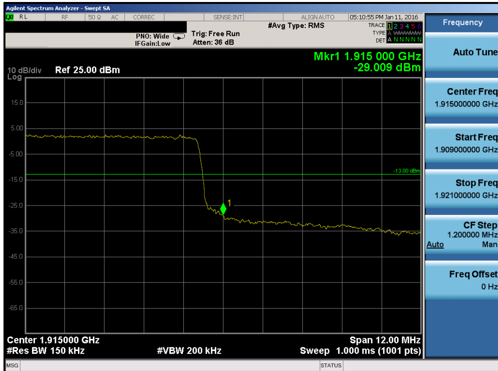
Plot 7-187. Upper Band Edge Plot (Band 2/25 – 15.0MHz QPSK – RB Size 75)
