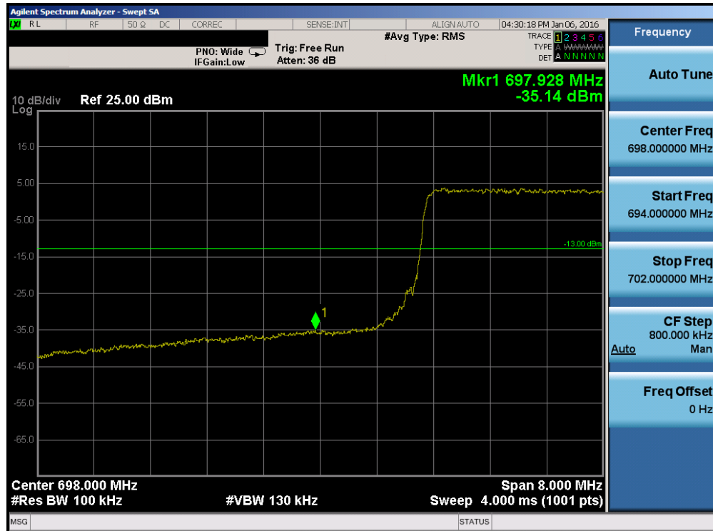
Plot 7-121. Lower Band Edge Plot (Band 12/17 - 10.0MHz QPSK - RB Size 50)
