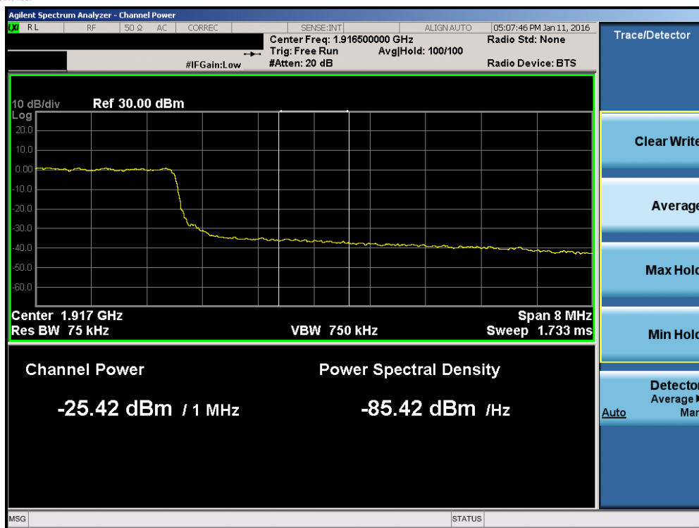
Plot 7-184. Upper Extended Band Edge Plot (Band 2/25 – 10.0MHz QPSK – RB Size 50)
