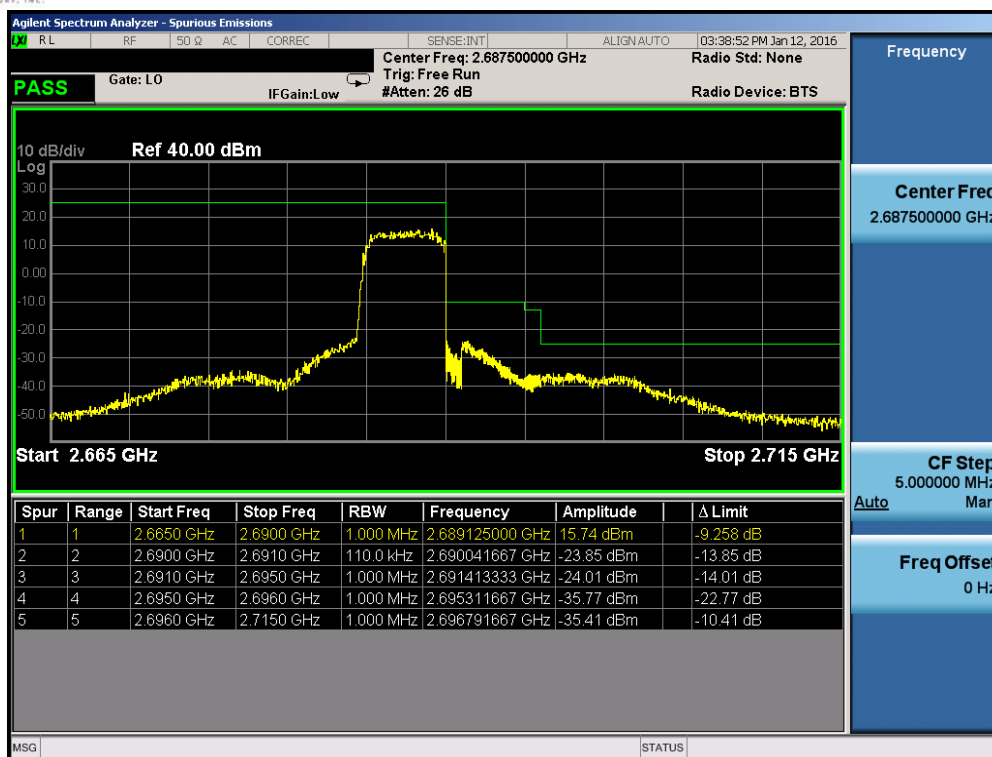
Plot 7-194. Upper ACP Plot (Band 41 – 5.0MHz QPSK – RB Size 25)
