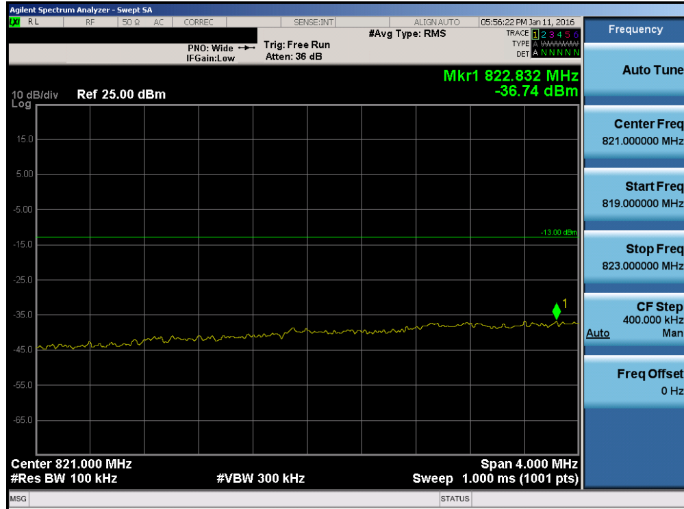
Plot 7-138. Lower Extended Band Edge Plot (Band 5/26 - 5.0MHz QPSK - RB Size 25)
