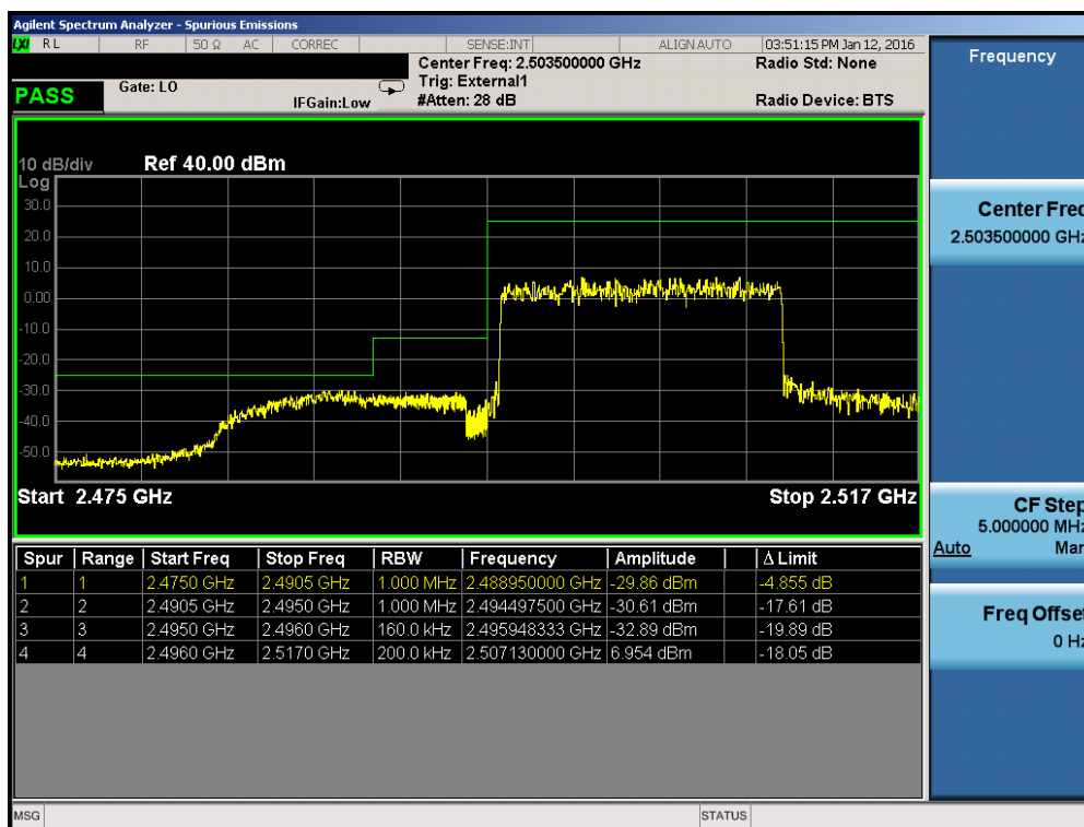
Plot 7-197. Lower ACP Plot (Band 41 – 15.0MHz QPSK – RB Size 75)
