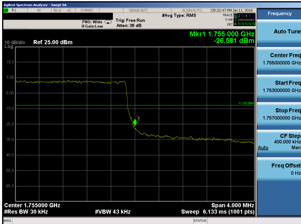
Plot 7-151. Upper Band Edge Plot (Band 4 – 3.0MHz QPSK – RB Size 15)
