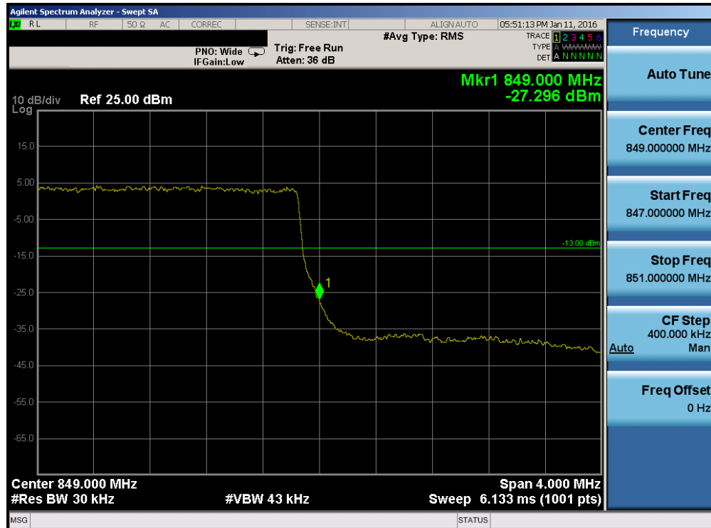
Plot 7-135. Upper Band Edge Plot (Band 5/26 - 3.0MHz QPSK - RB Size 15)
