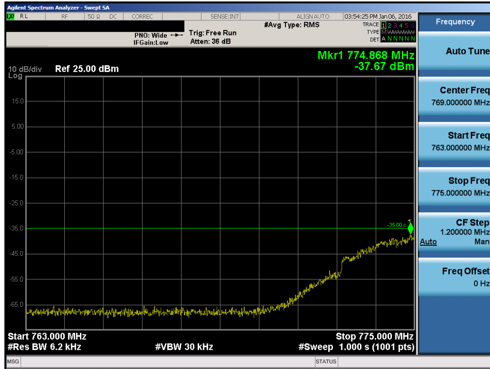
Plot 7-124. Lower Emission Mask Edge Plot (Band 13 – 5.0MHz QPSK – RB Size 25)
