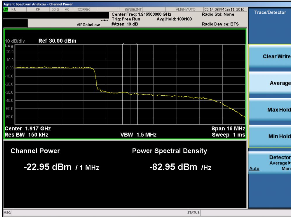
Plot 7-192. Upper Extended Band Edge Plot (Band 2/25 – 20.0MHz QPSK – RB Size 100)
