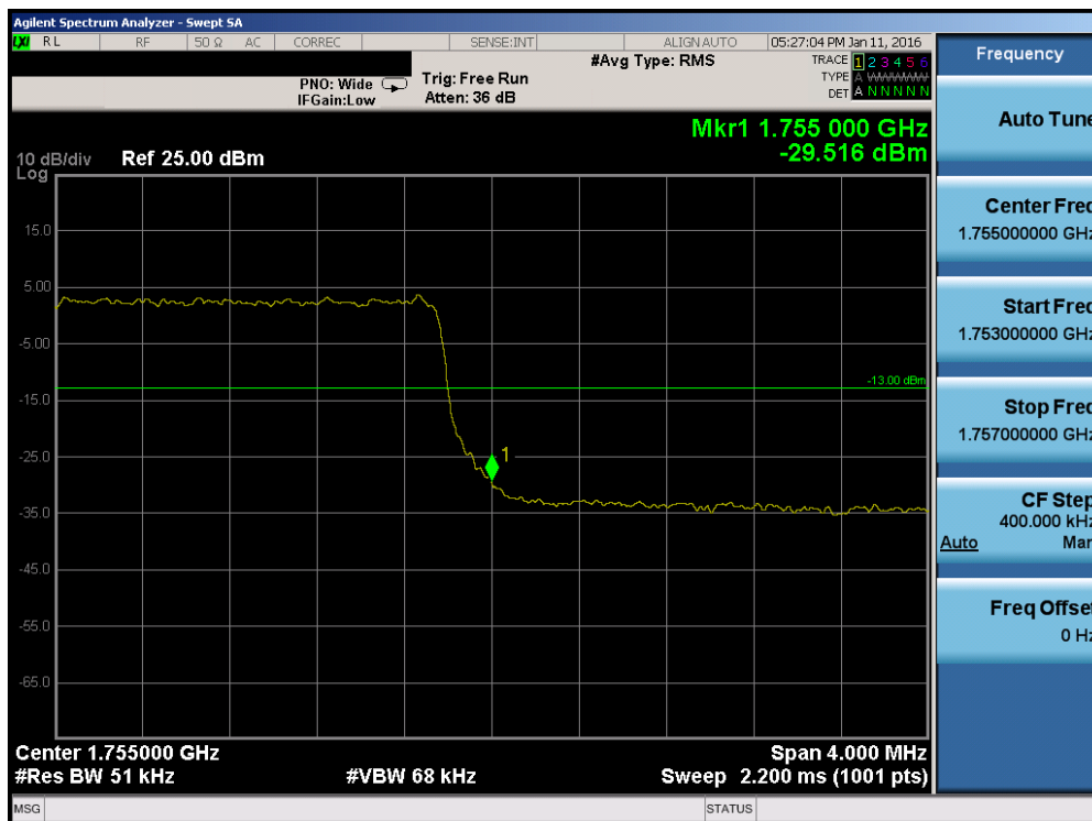
Plot 7-155. Upper Band Edge Plot (Band 4 – 5.0MHz QPSK – RB Size 25)
