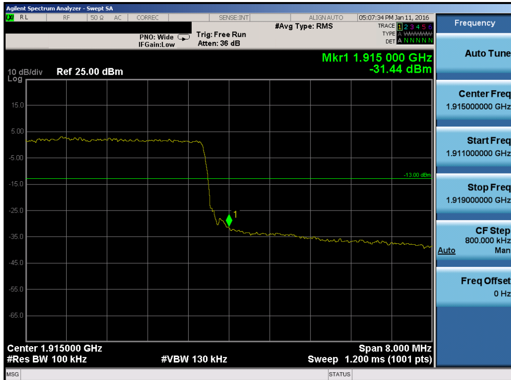
Plot 7-183. Upper Band Edge Plot (Band 2/25 – 10.0MHz QPSK – RB Size 50)
