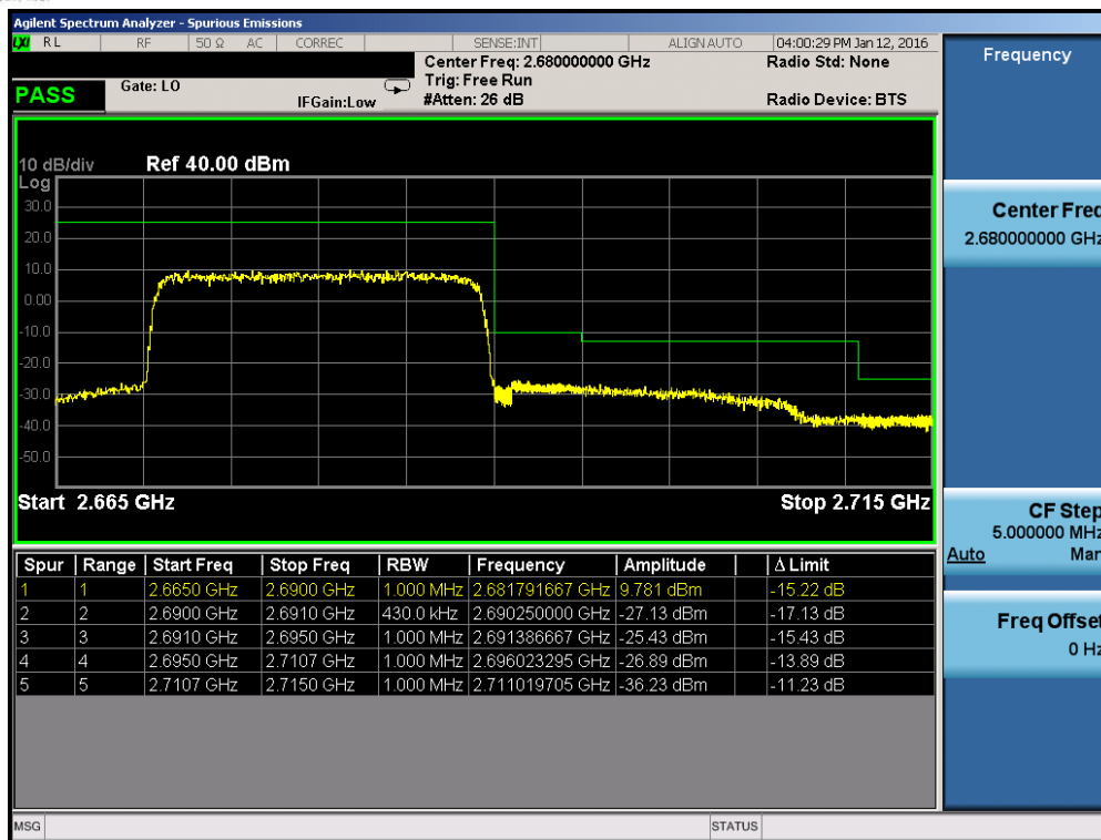
Plot 7-200. Upper ACP Plot (Band 41 – 20.0MHz QPSK – RB Size 100)
