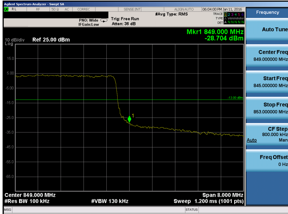
Plot 7-142. Upper Band Edge Plot (Band 5/26 – 10.0MHz QPSK – RB Size 50)
