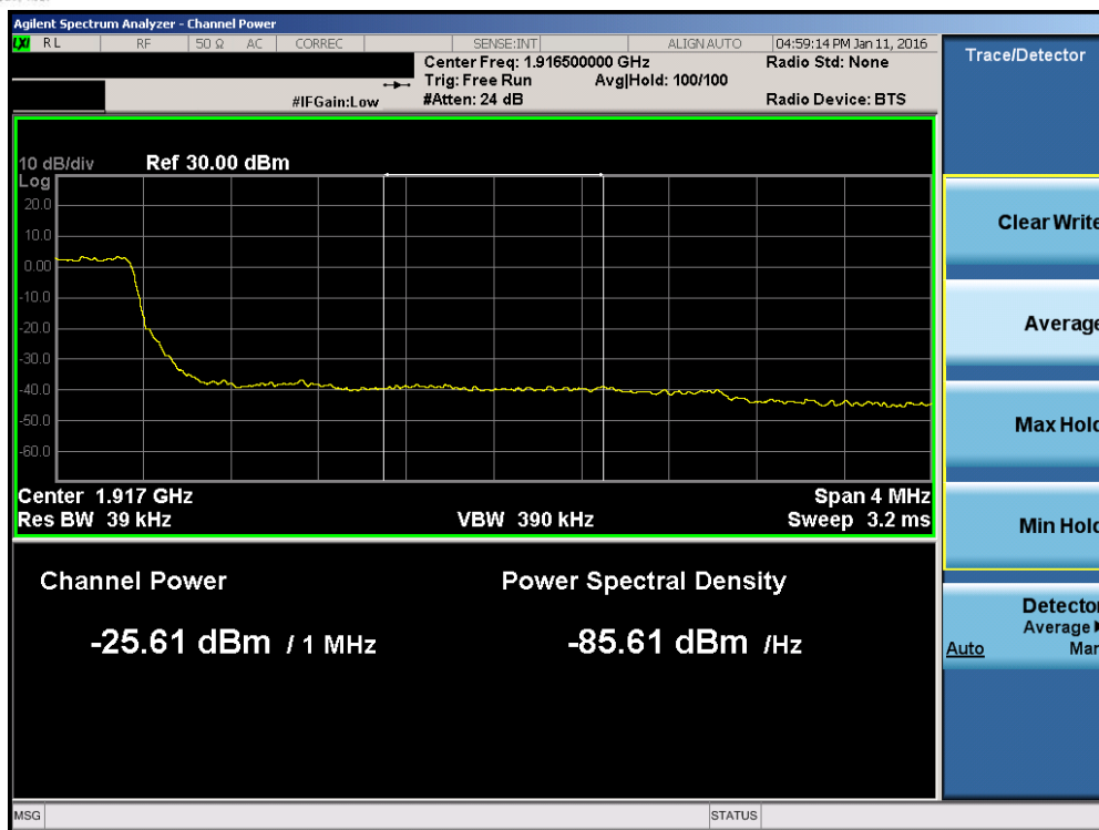
Plot 7-176. Upper Extended Band Edge Plot (Band 2/25 – 3.0MHz QPSK – RB Size 15)
