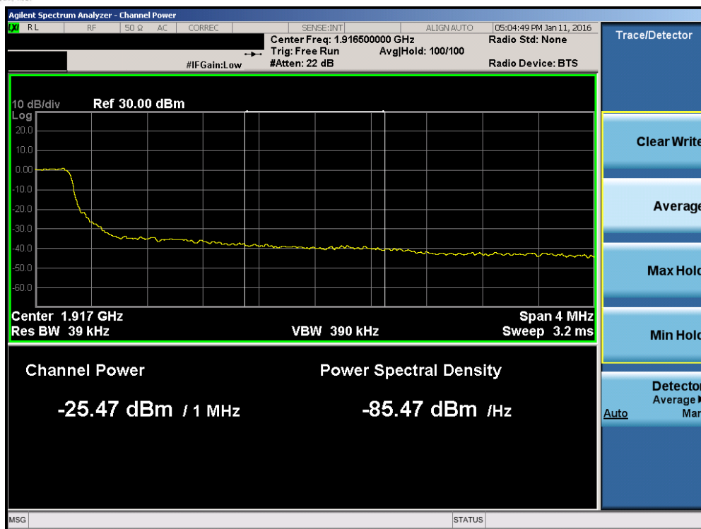
Plot 7-180. Upper Extended Band Edge Plot (Band 2/25 – 5.0MHz QPSK – RB Size 25)
