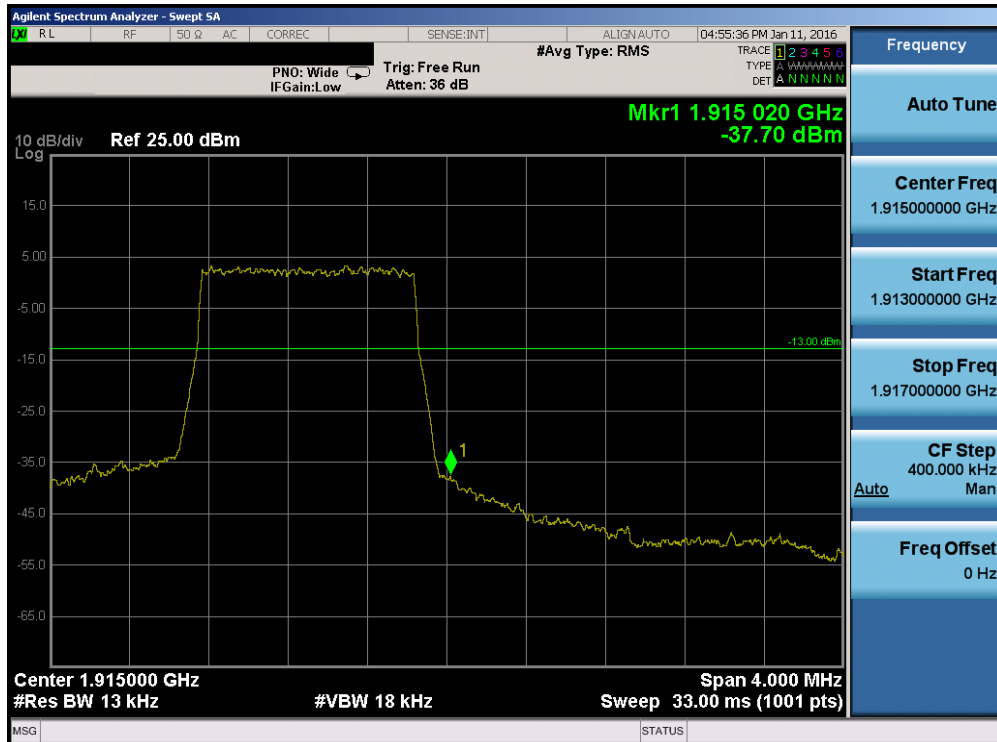
Plot 7-171. Upper Band Edge Plot (Band 2/25 – 1.4MHz QPSK – RB Size 6)
