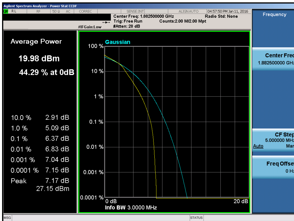
Plot 7-204. PAR Plot (Band 2/25 – 3.0MHz 16-QAM – RB Size 15)
