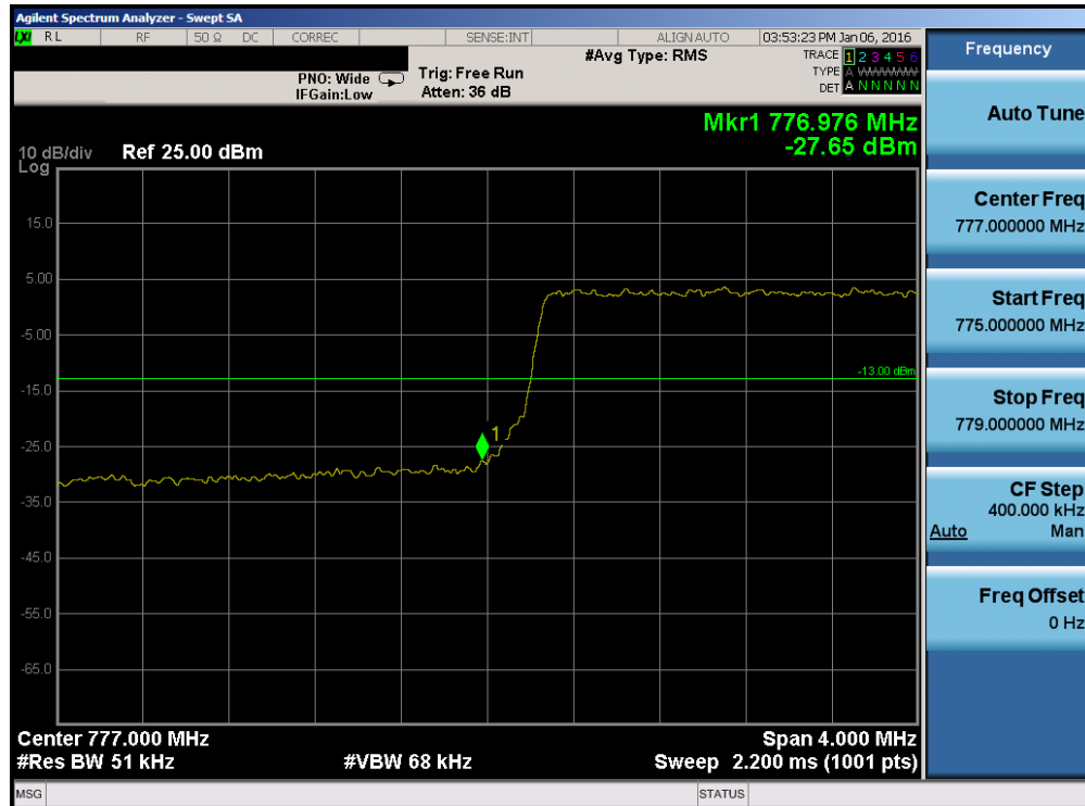
Plot 7-123. Lower Band Edge Plot (Band 13 – 5.0MHz QPSK – RB Size 25)
