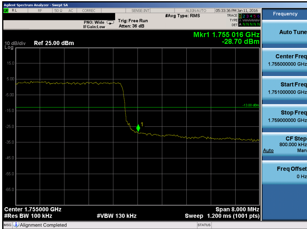
Plot 7-159. Upper Band Edge Plot (Band 4 – 10.0MHz QPSK – RB Size 50)
