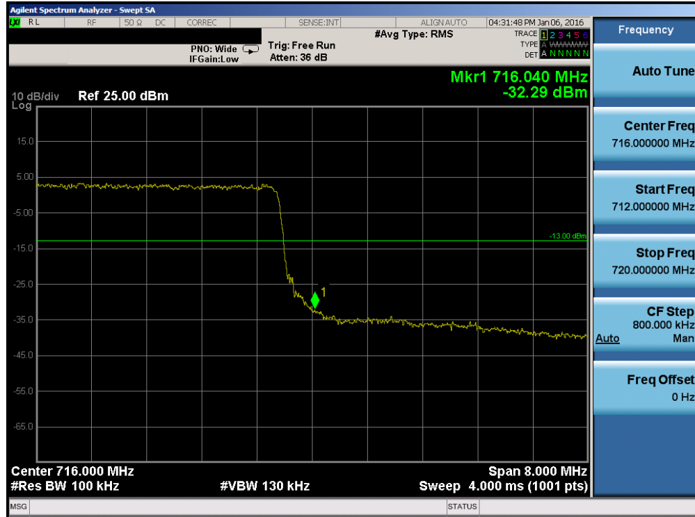
Plot 7-122. Upper Band Edge Plot (Band 12/17 – 10.0MHz QPSK – RB Size 50)
