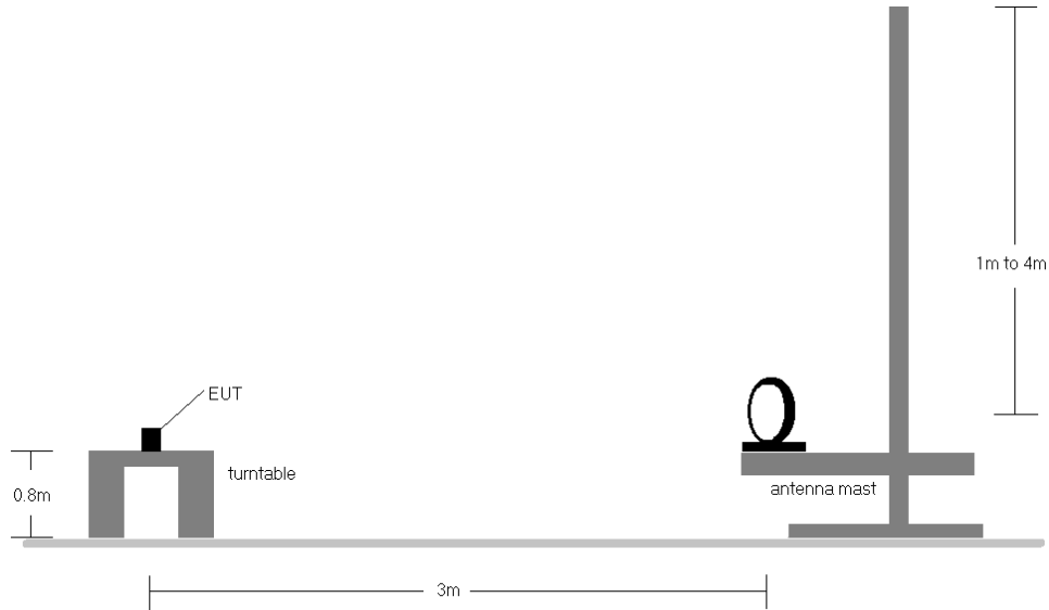
Figure 8-5. Radiated Test Setup
