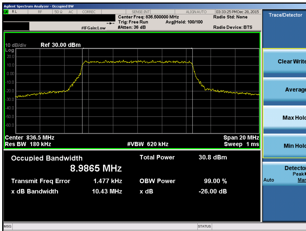
Plot 7-27. Occupied Bandwidth Plot (Band 26 – 10.0MHz QPSK – RB Size 50)
