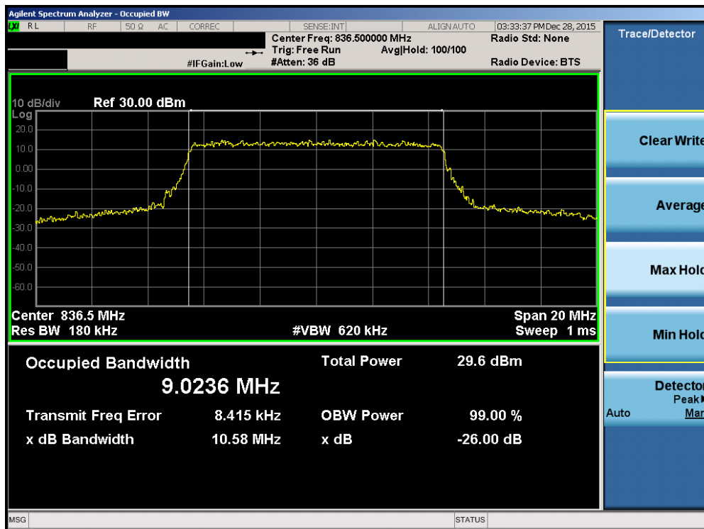
Plot 7-28. Occupied Bandwidth Plot (Band 26 – 10.0MHz 16-QAM – RB Size 50)
