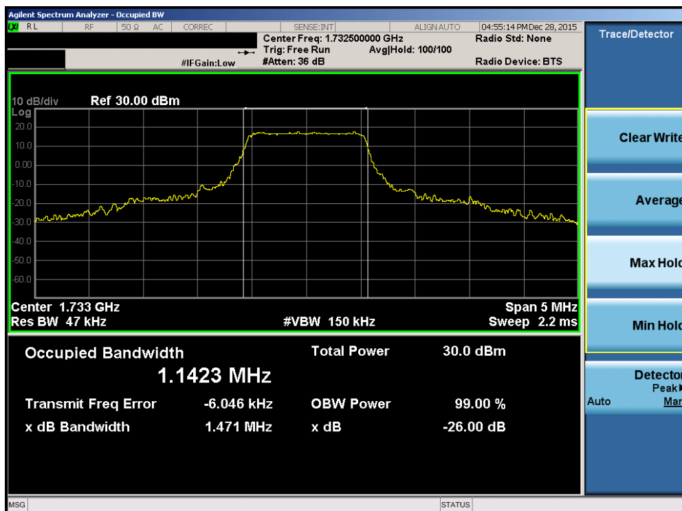
Plot 7-32. Occupied Bandwidth Plot (Band 4 – 1.4MHz 16-QAM – RB Size 6)
