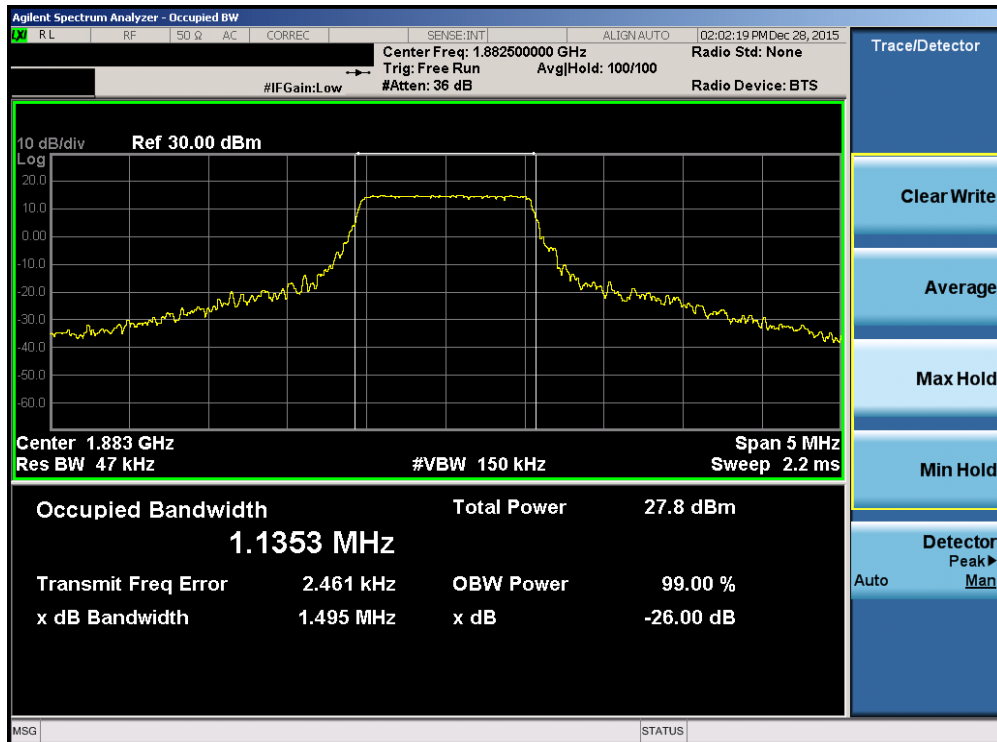
Plot 7-44. Occupied Bandwidth Plot (Band 2/25 – 1.4MHz 16-QAM – RB Size 6)
