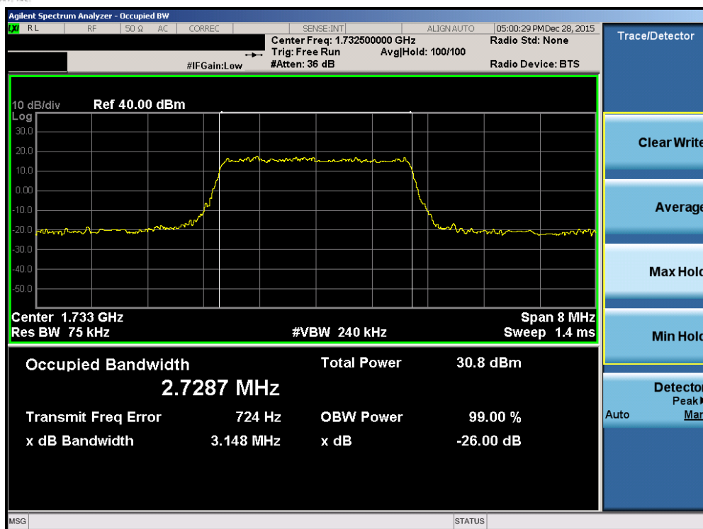
Plot 7-33. Occupied Bandwidth Plot (Band 4 – 3.0MHz QPSK – RB Size 15)
