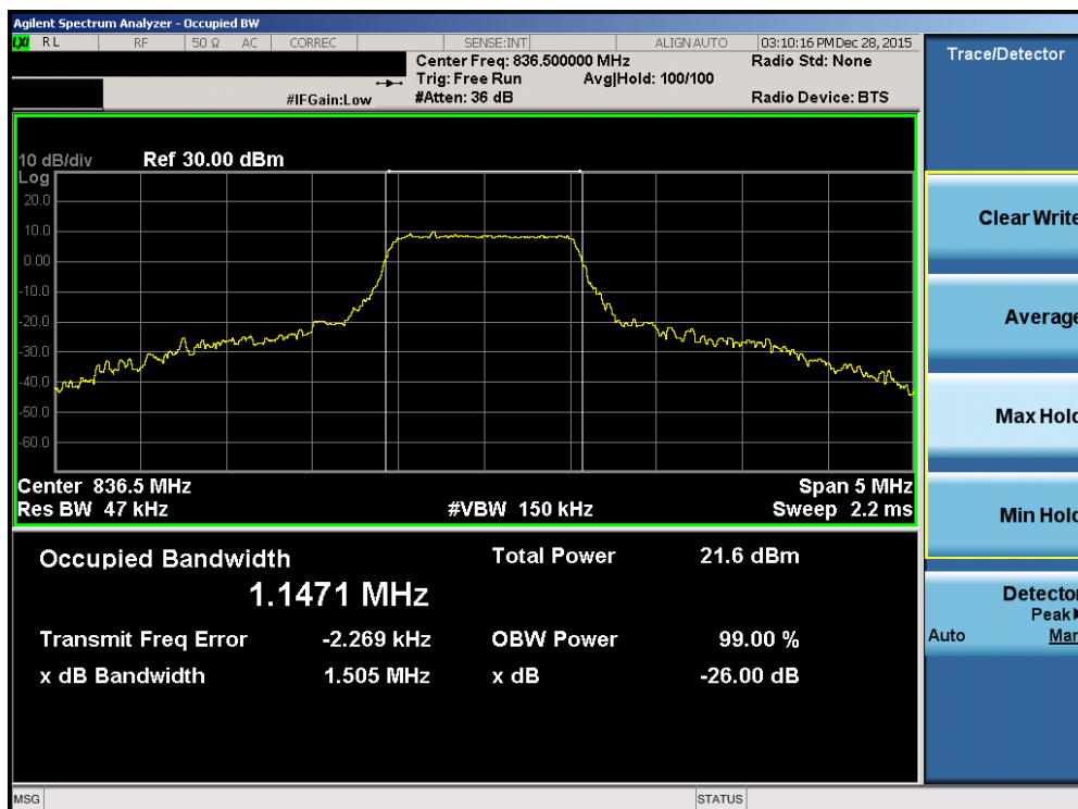
Plot 7-22. Occupied Bandwidth Plot (Band 26 – 1.4MHz 16-QAM – RB Size 6)
