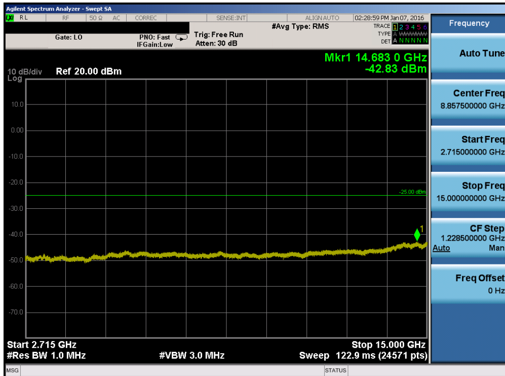
Plot 7-124. Conducted Spurious Plot (Band 41 – 15.0MHz QPSK – RB Size 1, RB Offset 0 – High Channel)
