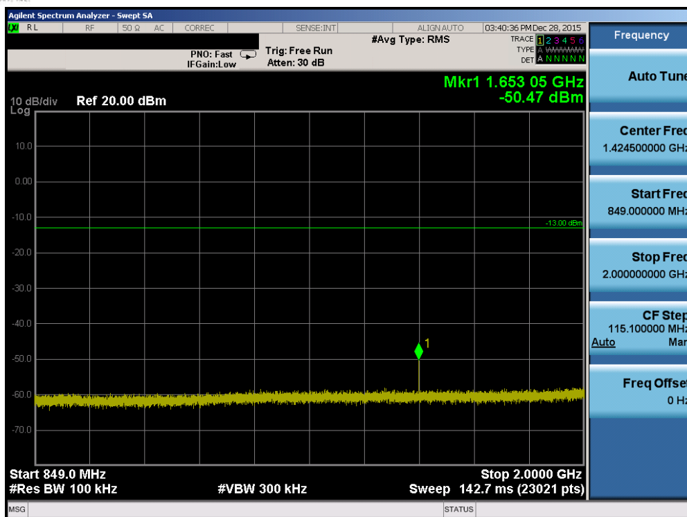
Plot 7-91. Conducted Spurious Plot (Band 26 – 5.0MHz QPSK – RB Size 1, RB Offset 0 – Low Channel)
