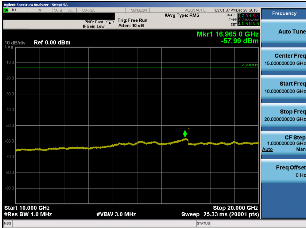
Plot 7-113. Conducted Spurious Plot (Band 2/25 – 5.0MHz QPSK – RB Size 1, RB Offset 0 – Mid Channel)
