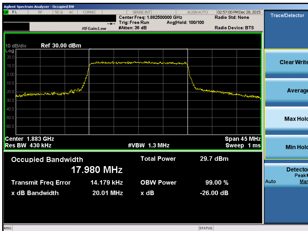
Plot 7-54. Occupied Bandwidth Plot (Band 2/25 – 20.0MHz 16-QAM – RB Size 100)
