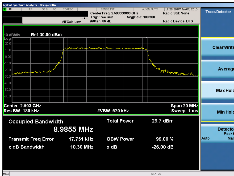
Plot 7-58. Occupied Bandwidth Plot (Band 41 – 10.0MHz 16-QAM – RB Size 50)
