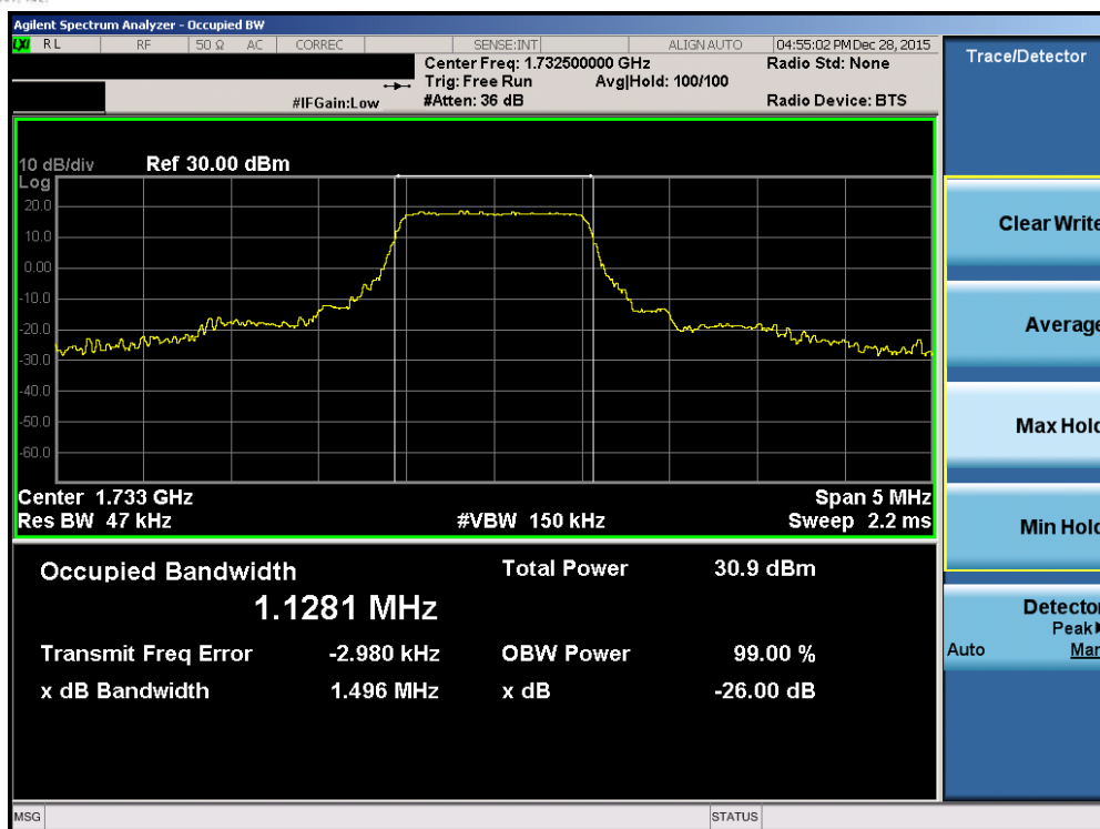
Plot 7-31. Occupied Bandwidth Plot (Band 4 – 1.4MHz QPSK – RB Size 6)
