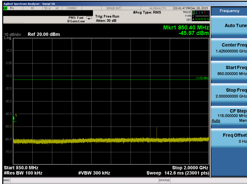
Plot 7-97. Conducted Spurious Plot (Band 26 – 5.0MHz QPSK – RB Size 1, RB Offset 0 – High Channel)
