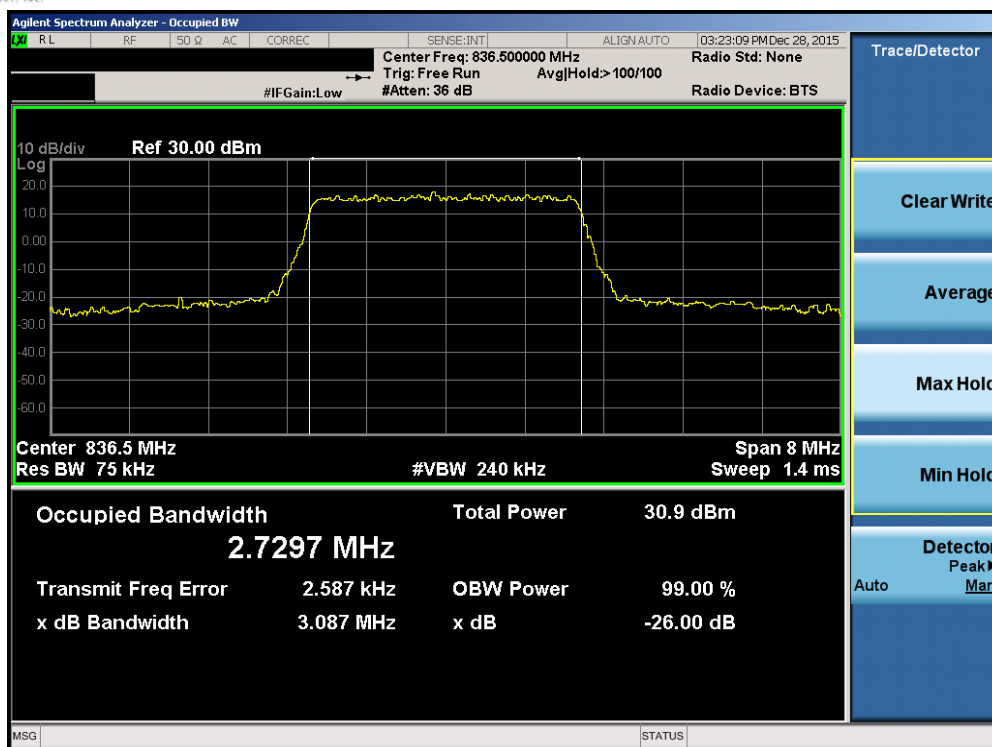
Plot 7-23. Occupied Bandwidth Plot (Band 26 – 3.0MHz QPSK – RB Size 15)
