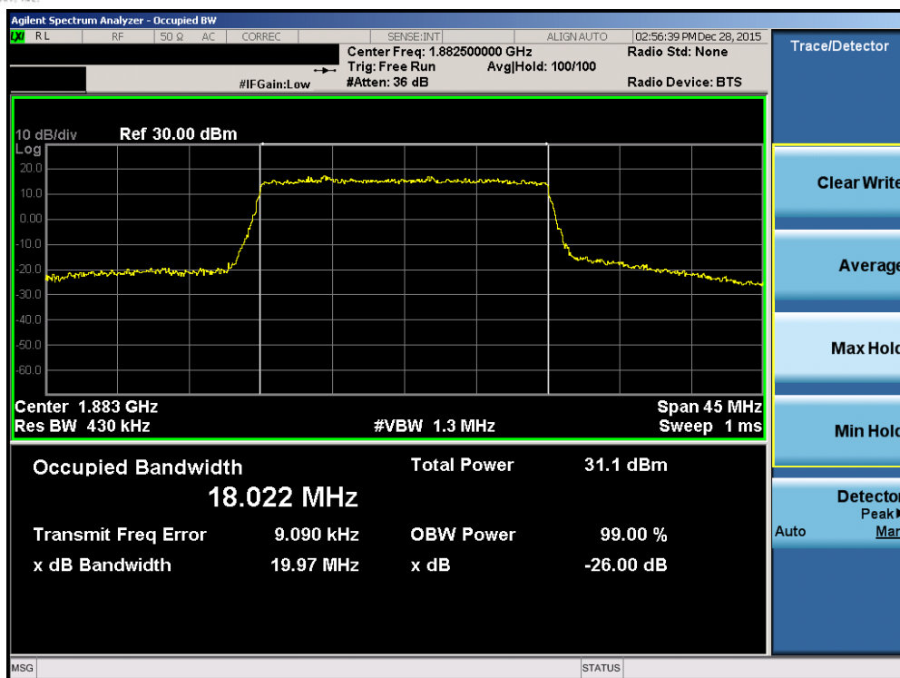
Plot 7-53. Occupied Bandwidth Plot (Band 2/25 – 20.0MHz QPSK – RB Size 100)
