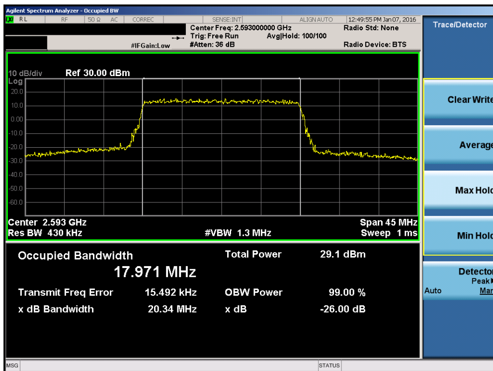
Plot 7-62. Occupied Bandwidth Plot (Band 41 – 20.0MHz 16-QAM – RB Size 100)
