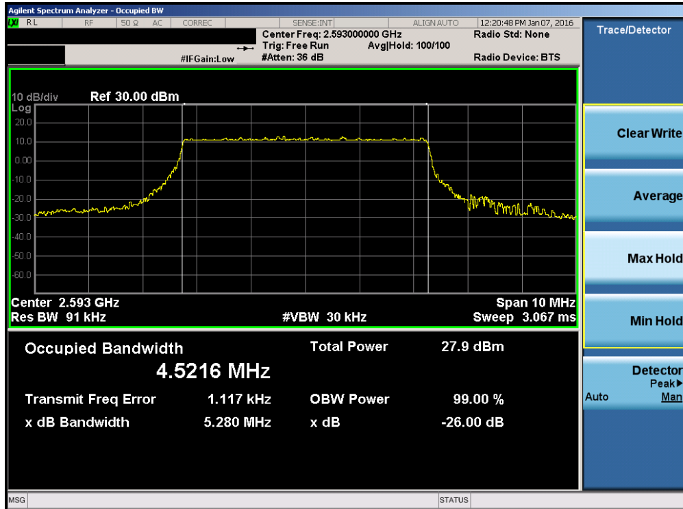
Plot 7-56. Occupied Bandwidth Plot (Band 41 – 5.0MHz 16-QAM – RB Size 25)
