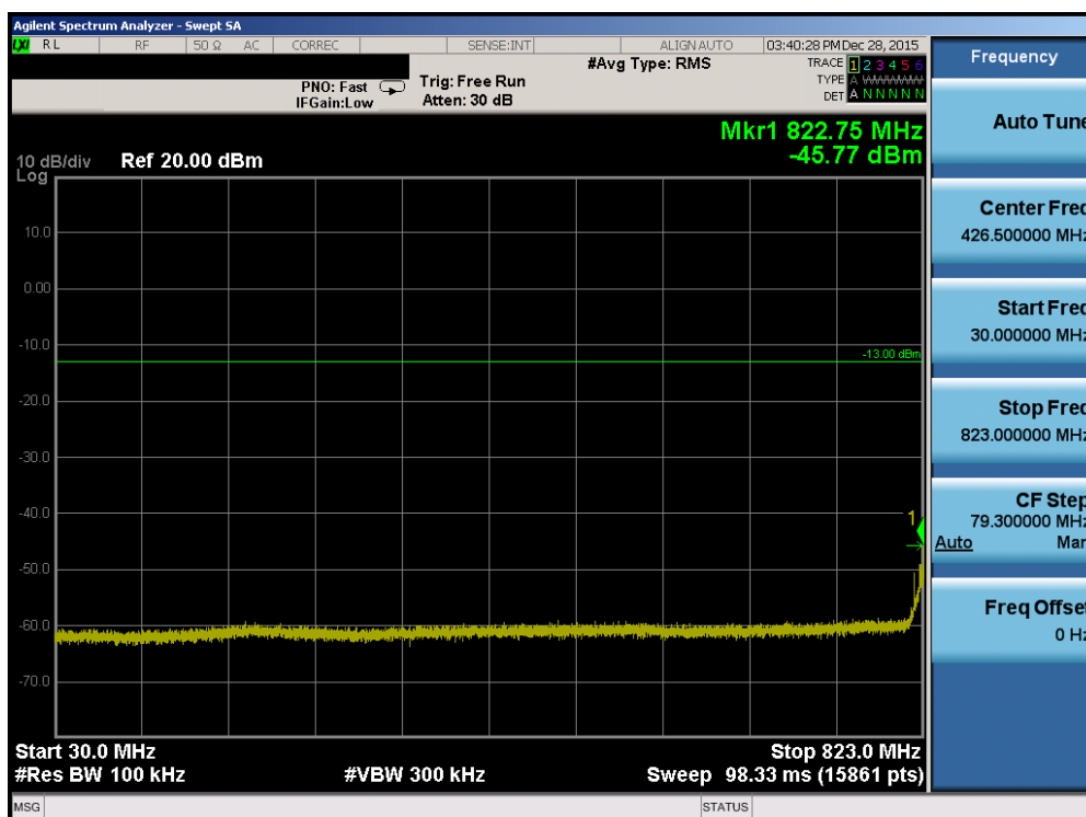
Plot 7-90. Conducted Spurious Plot (Band 26 – 5.0MHz QPSK – RB Size 1, RB Offset 0 – Low Channel)
