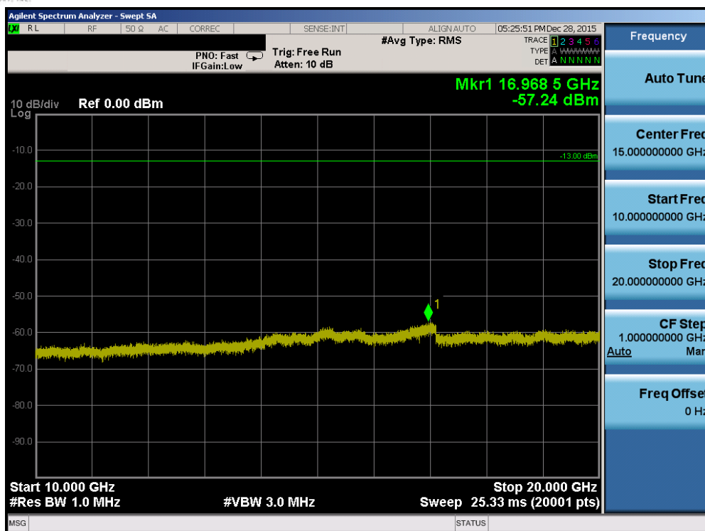
Plot 7-107. Conducted Spurious Plot (Band 4 – 10.0MHz QPSK – RB Size 1, RB Offset 0 – High Channel)
