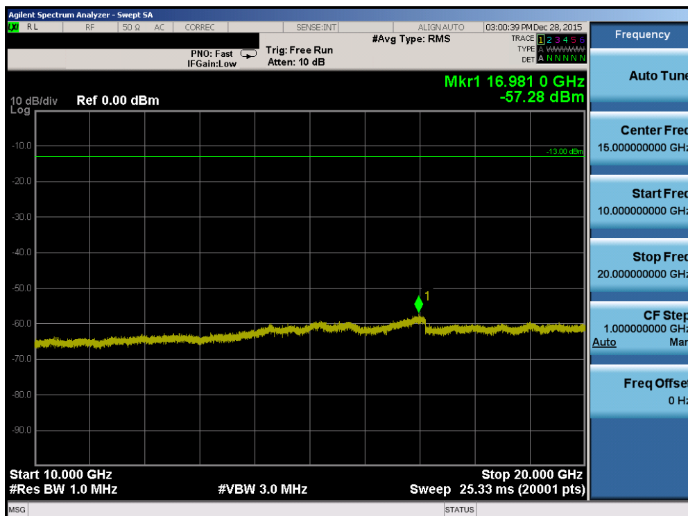
Plot 7-110. Conducted Spurious Plot (Band 2/25 – 5.0MHz QPSK – RB Size 1, RB Offset 0 – Low Channel)
