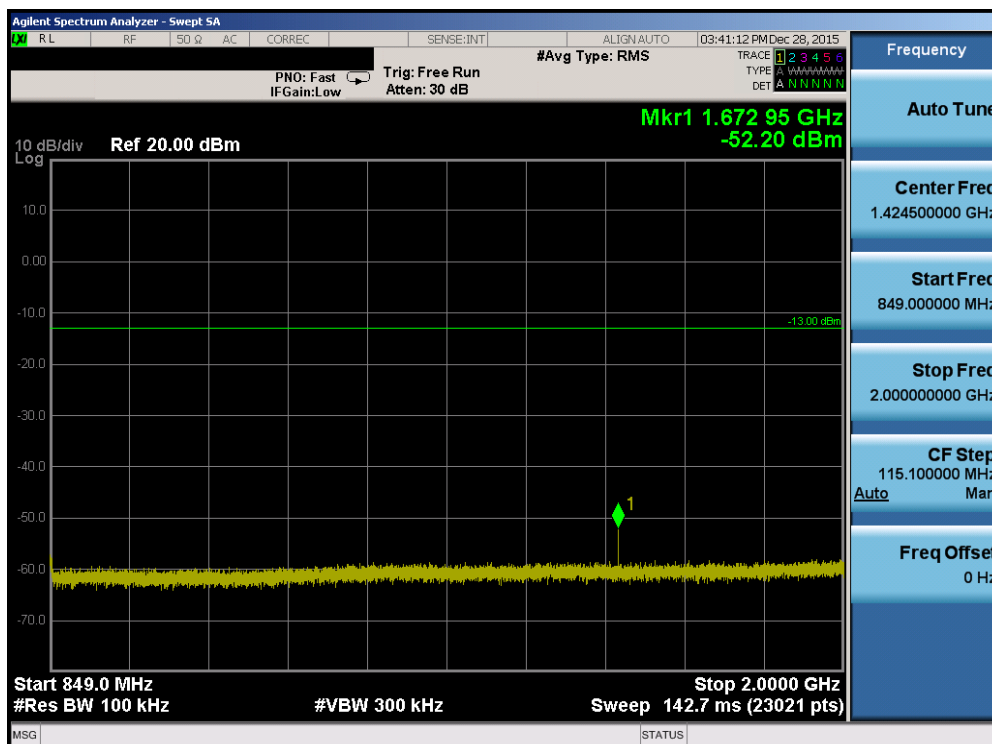
Plot 7-94. Conducted Spurious Plot (Band 26 – 5.0MHz QPSK – RB Size 1, RB Offset 0 – Mid Channel)
