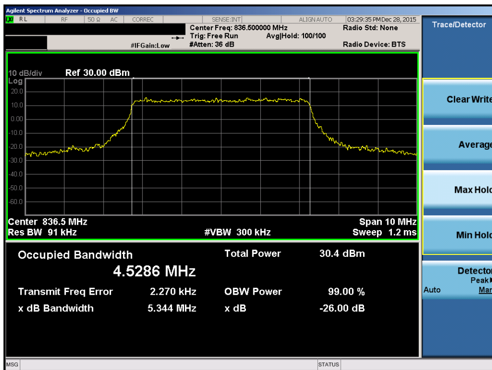
Plot 7-26. Occupied Bandwidth Plot (Band 26 – 5.0MHz 16-QAM – RB Size 25)
