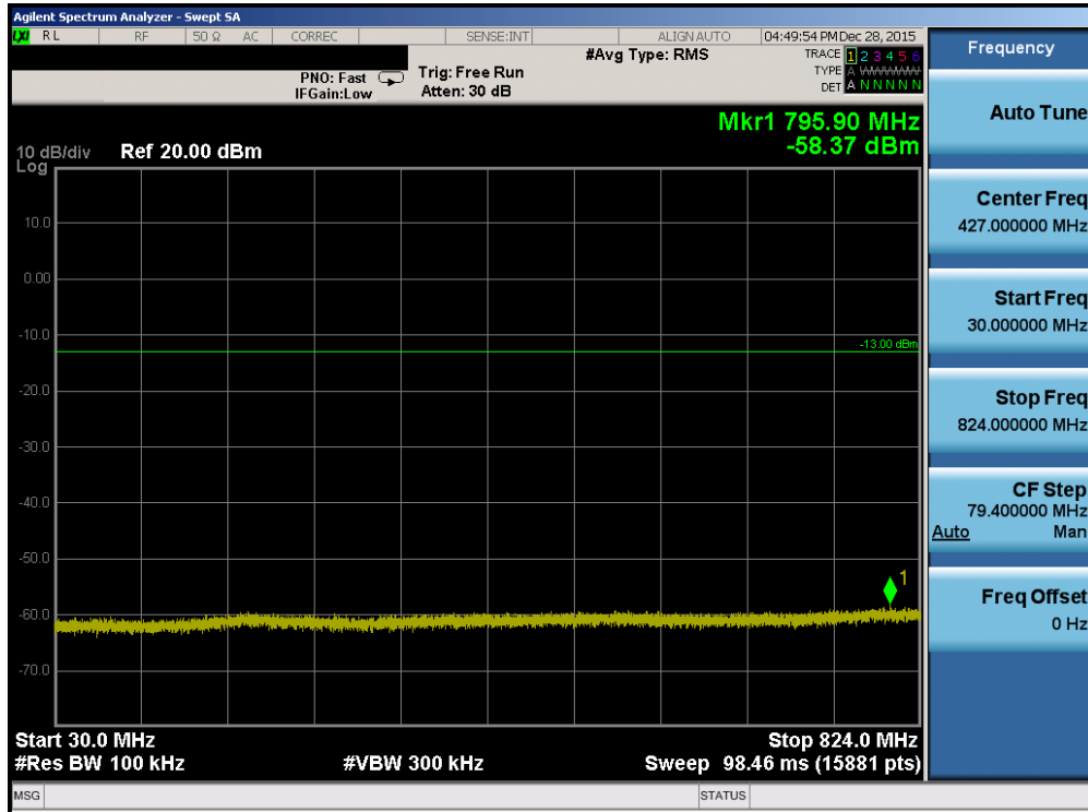
Plot 7-87. Conducted Spurious Plot (Band 5 – 3.0MHz QPSK – RB Size 1, RB Offset 0 – High Channel)
