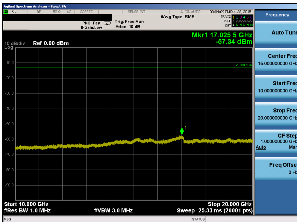
Plot 7-116. Conducted Spurious Plot (Band 2/25 – 5.0MHz QPSK – RB Size 1, RB Offset 0 – High Channel)
