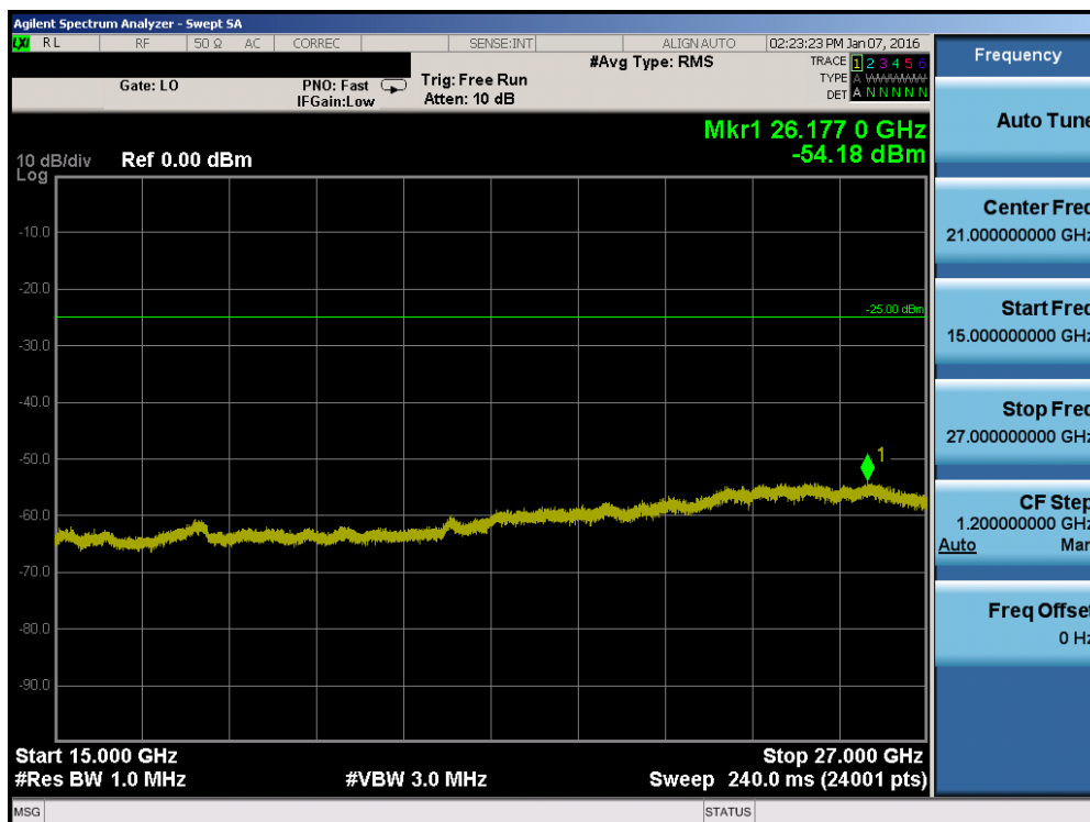
Plot 7-122. Conducted Spurious Plot (Band 41 – 15.0MHz QPSK – RB Size 1, RB Offset 0 – Mid Channel)
