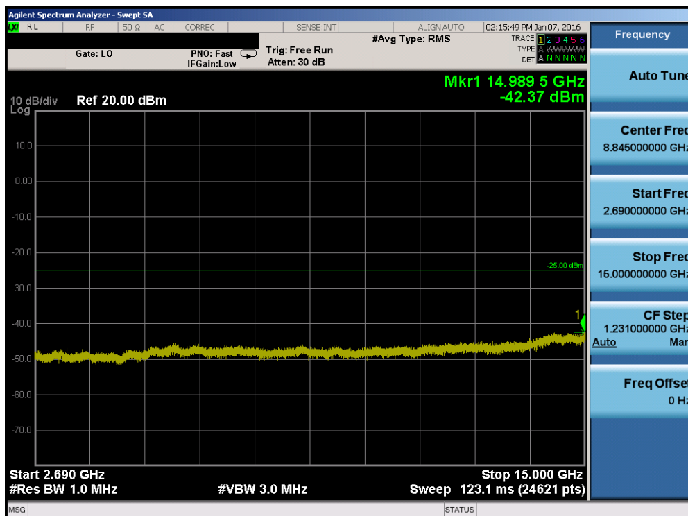
Plot 7-118. Conducted Spurious Plot (Band 41 – 15.0MHz QPSK – RB Size 1, RB Offset 0 – Low Channel)
