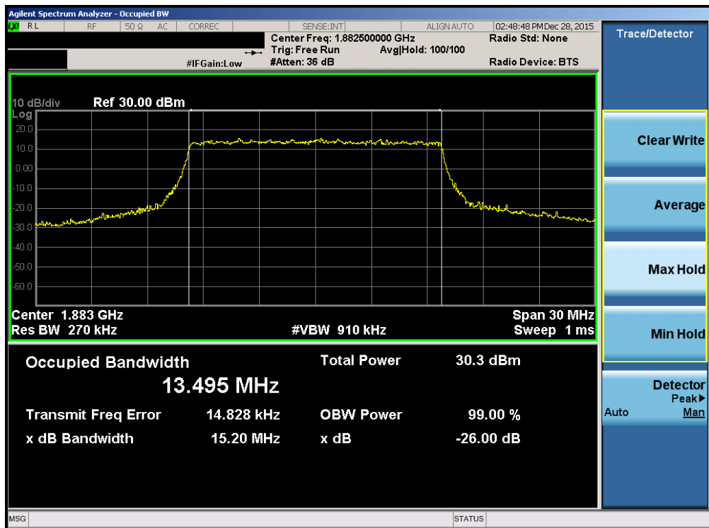
Plot 7-52. Occupied Bandwidth Plot (Band 2/25 – 15.0MHz 16-QAM – RB Size 75)
