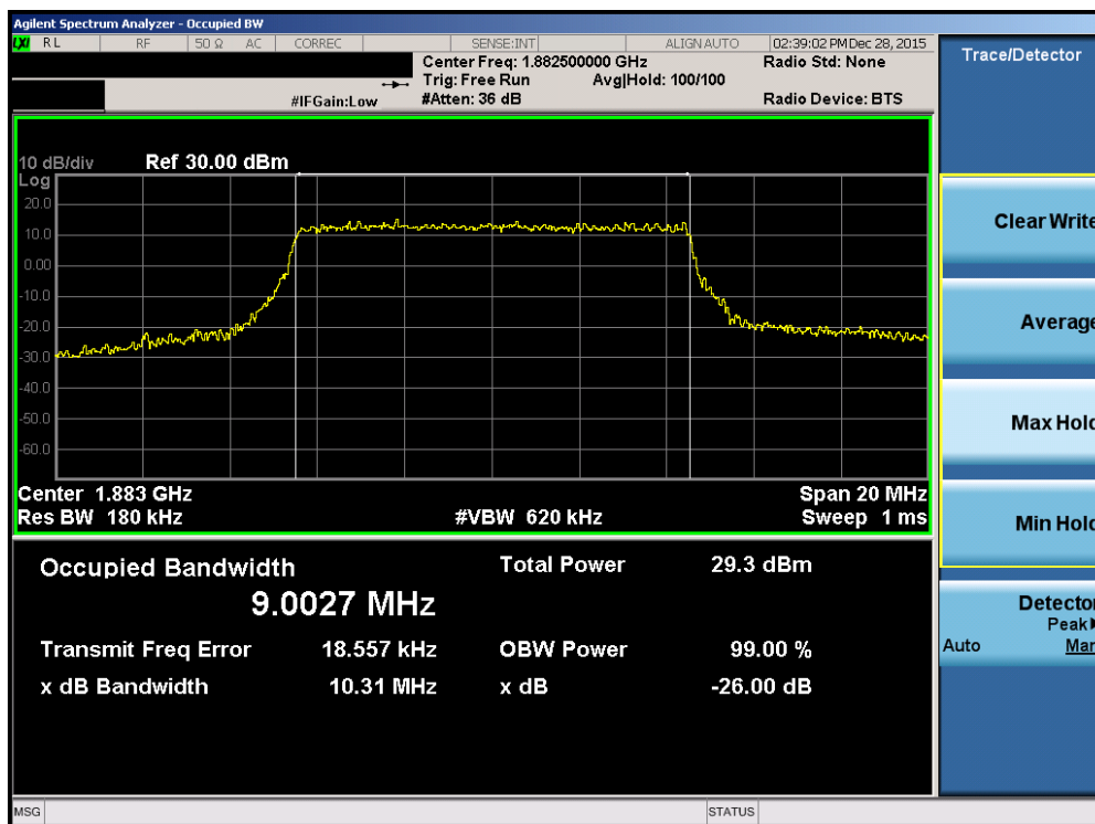
Plot 7-50. Occupied Bandwidth Plot (Band 2/25 – 10.0MHz 16-QAM – RB Size 50)
