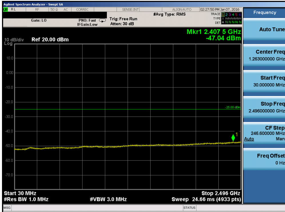
Plot 7-123. Conducted Spurious Plot (Band 41 – 15.0MHz QPSK – RB Size 1, RB Offset 0 – High Channel)
