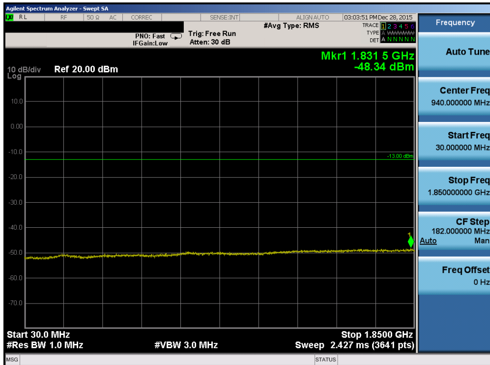
Plot 7-114. Conducted Spurious Plot (Band 2/25 – 5.0MHz QPSK – RB Size 1, RB Offset 0 – High Channel)
