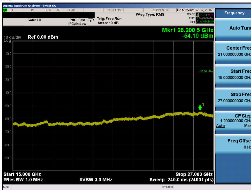
Plot 7-119. Conducted Spurious Plot (Band 41 – 15.0MHz QPSK – RB Size 1, RB Offset 0 – Low Channel)
