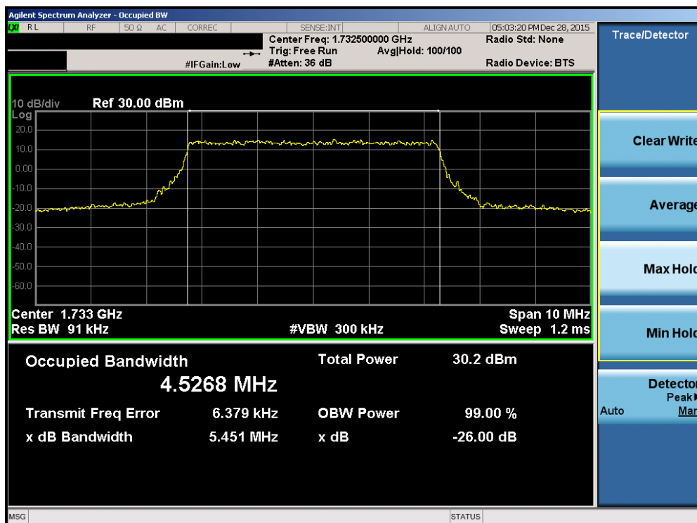
Plot 7-36. Occupied Bandwidth Plot (Band 4 – 5.0MHz 16-QAM – RB Size 25)
