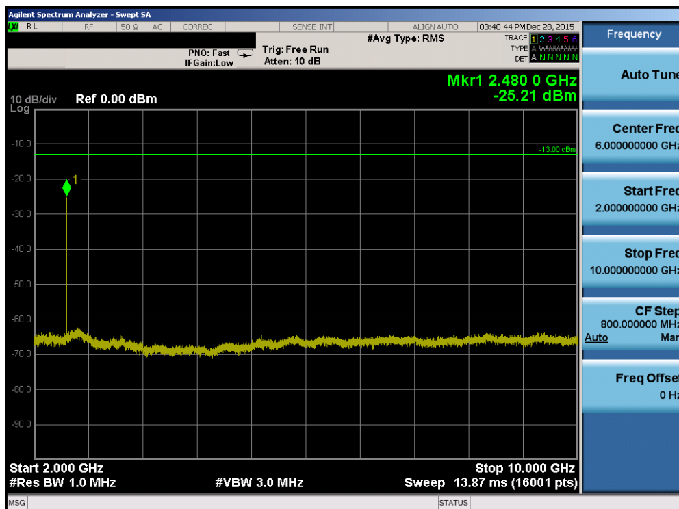
Plot 7-92. Conducted Spurious Plot (Band 26 – 5.0MHz QPSK – RB Size 1, RB Offset 0 – Low Channel)
