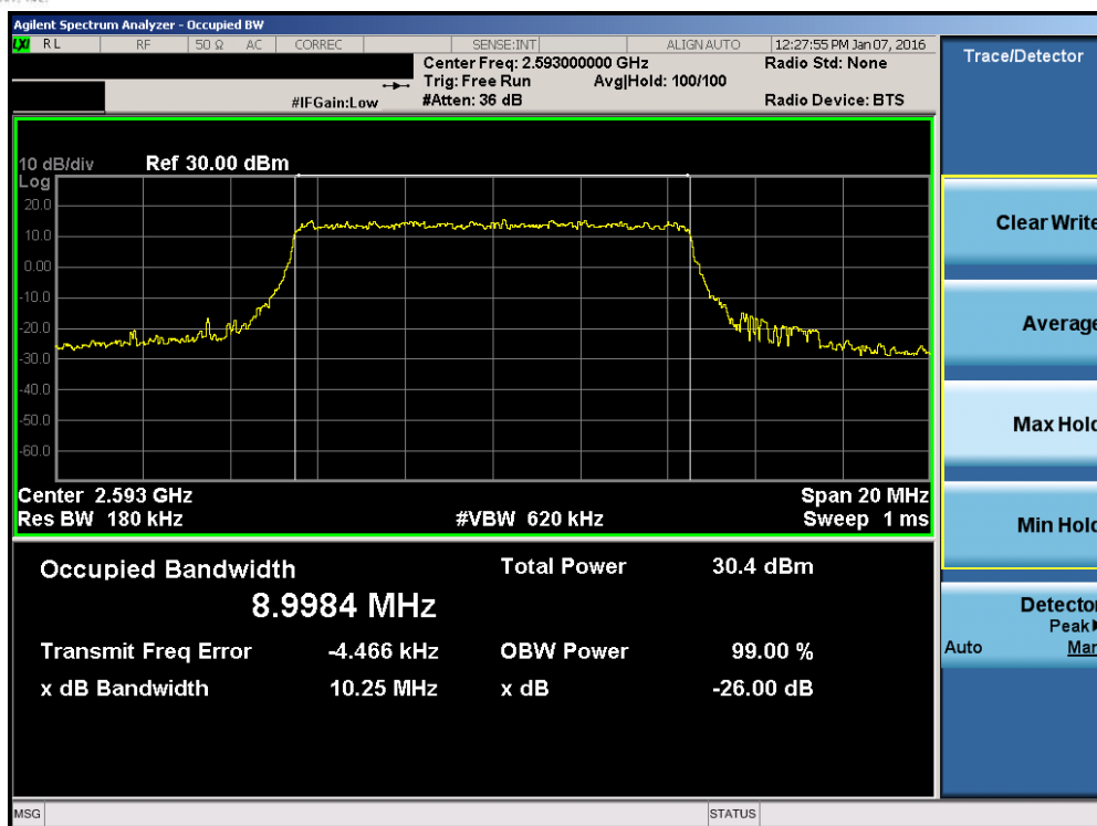
Plot 7-57. Occupied Bandwidth Plot (Band 41 – 10.0MHz QPSK – RB Size 50)
