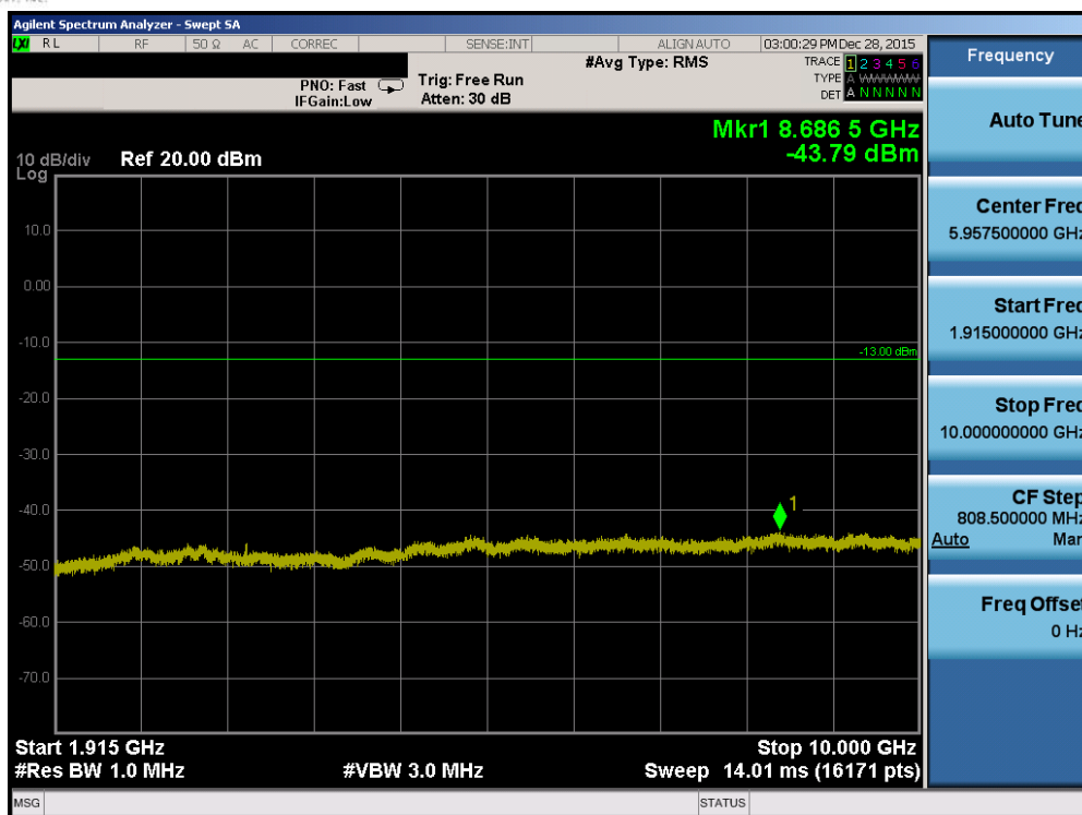
Plot 7-109. Conducted Spurious Plot (Band 2/25 – 5.0MHz QPSK – RB Size 1, RB Offset 0 – Low Channel)
