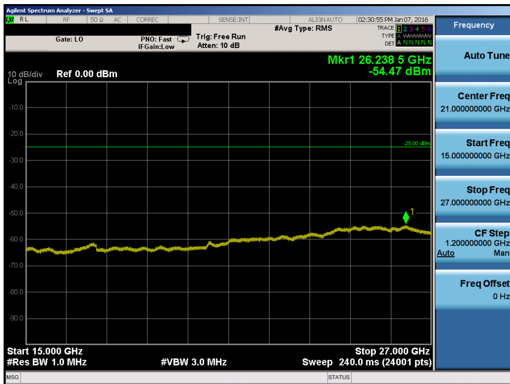
Plot 7-125. Conducted Spurious Plot (Band 41 – 15.0MHz QPSK – RB Size 1, RB Offset 0 – High Channel)
