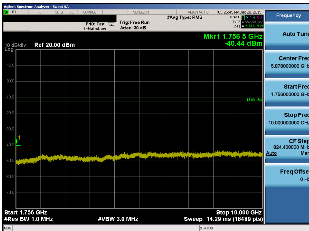
Plot 7-106. Conducted Spurious Plot (Band 4 – 10.0MHz QPSK – RB Size 1, RB Offset 0 – High Channel)
