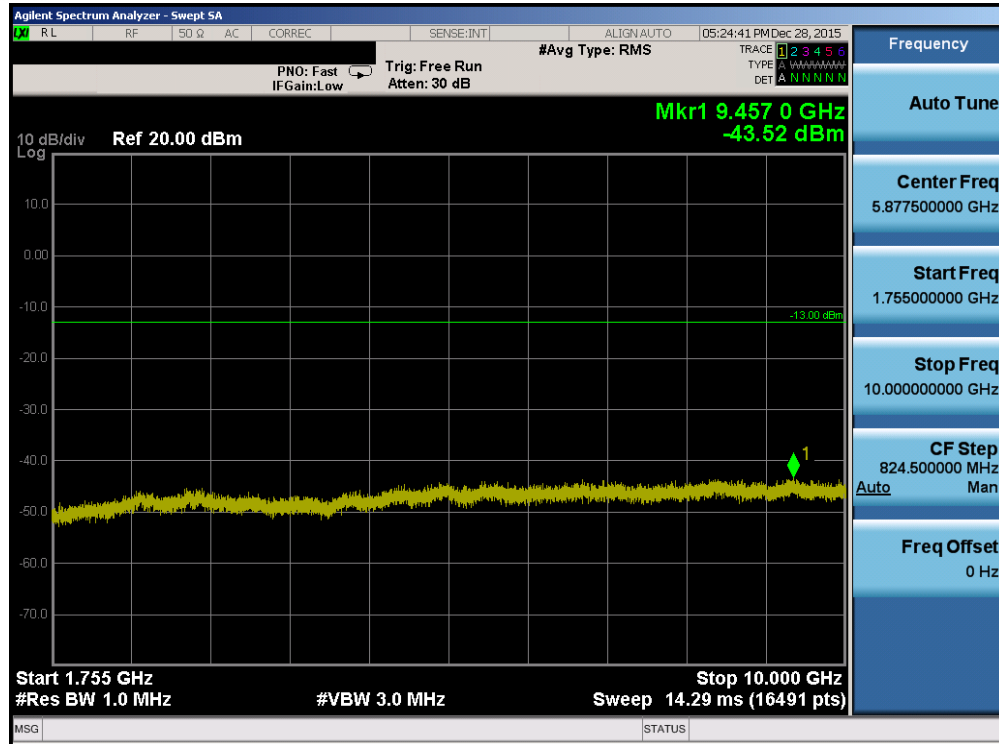
Plot 7-103. Conducted Spurious Plot (Band 4 – 10.0MHz QPSK – RB Size 1, RB Offset 0 – Mid Channel)
