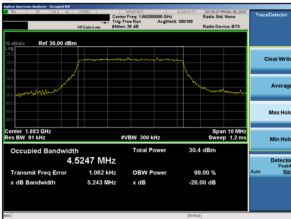
Plot 7-47. Occupied Bandwidth Plot (Band 2/25 – 5.0MHz QPSK – RB Size 25)
