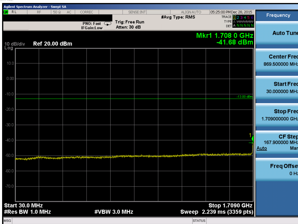
Plot 7-99. Conducted Spurious Plot (Band 4 – 10.0MHz QPSK – RB Size 1, RB Offset 0– Low Channel)
