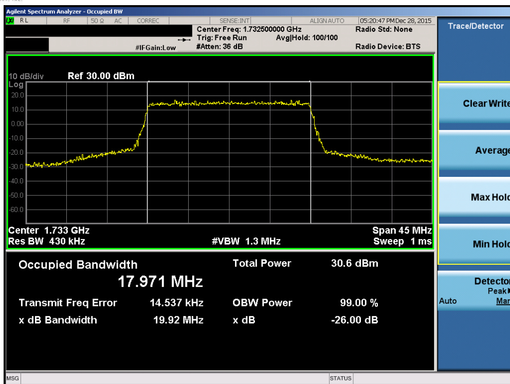
Plot 7-41. Occupied Bandwidth Plot (Band 4 – 20.0MHz QPSK – RB Size 100)
