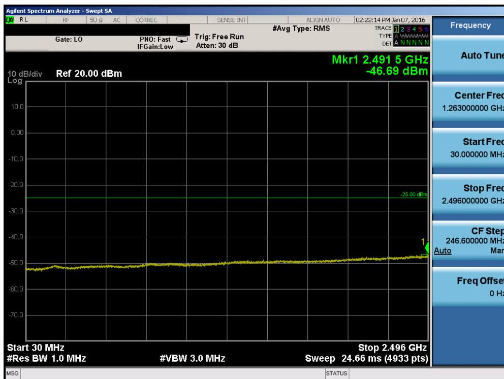
Plot 7-120. Conducted Spurious Plot (Band 41 – 15.0MHz QPSK – RB Size 1, RB Offset 0 – Mid Channel)
