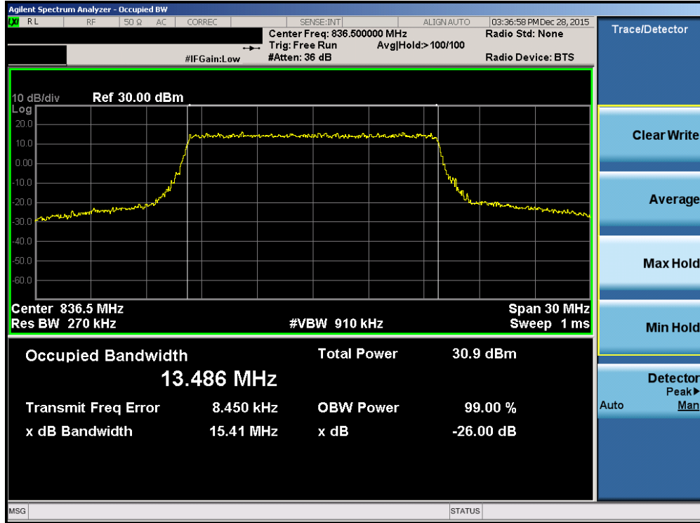
Plot 7-29. Occupied Bandwidth Plot (Band 26 – 15.0MHz QPSK – RB Size 75)
