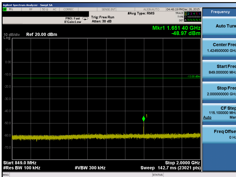
Plot 7-82. Conducted Spurious Plot (Band 5 – 3.0MHz QPSK – RB Size 1, RB Offset 0 – Low Channel)
