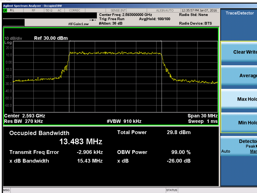
Plot 7-59. Occupied Bandwidth Plot (Band 41 – 15.0MHz QPSK – RB Size 75)
