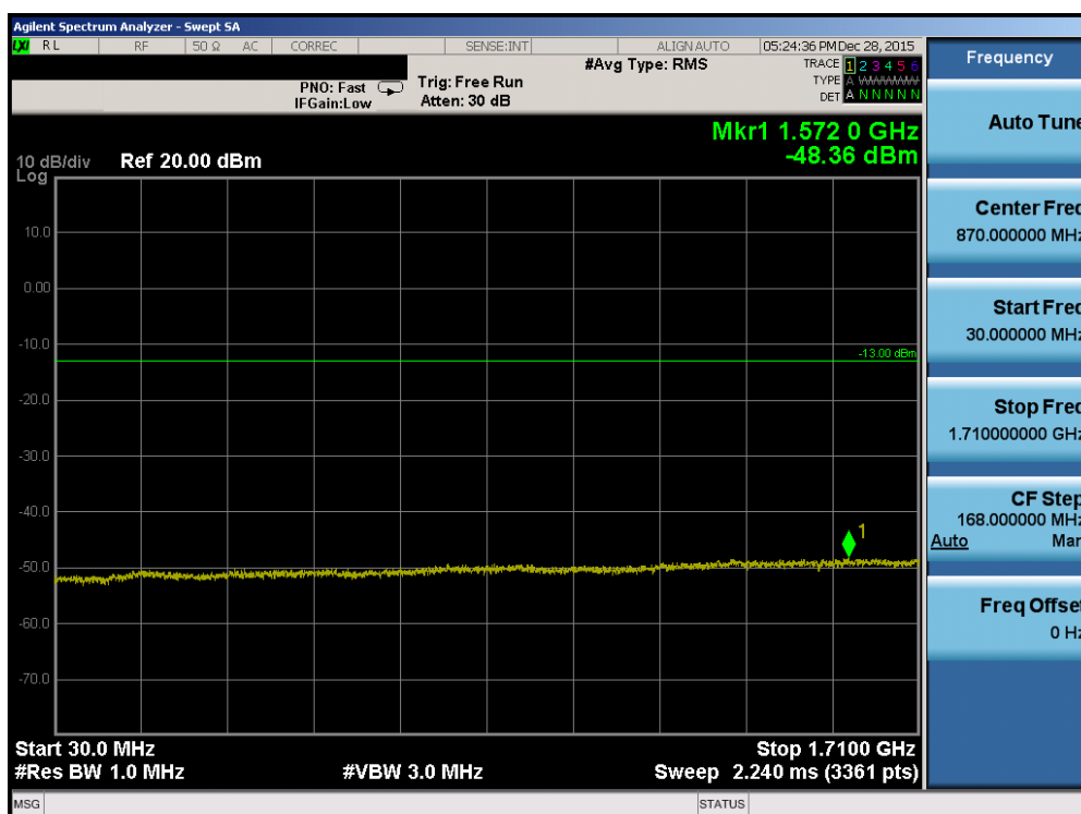
Plot 7-102. Conducted Spurious Plot (Band 4 – 10.0MHz QPSK – RB Size 1, RB Offset 0 – Mid Channel)
