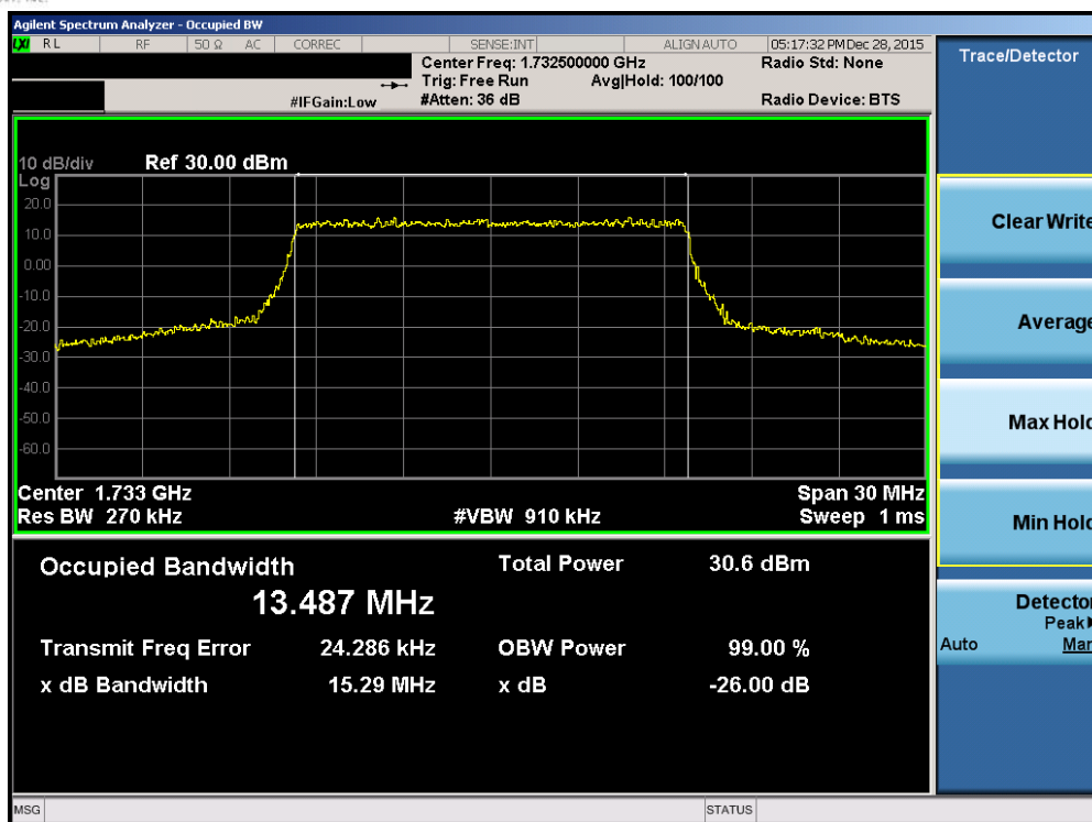
Plot 7-39. Occupied Bandwidth Plot (Band 4 – 15.0MHz QPSK – RB Size 75)
