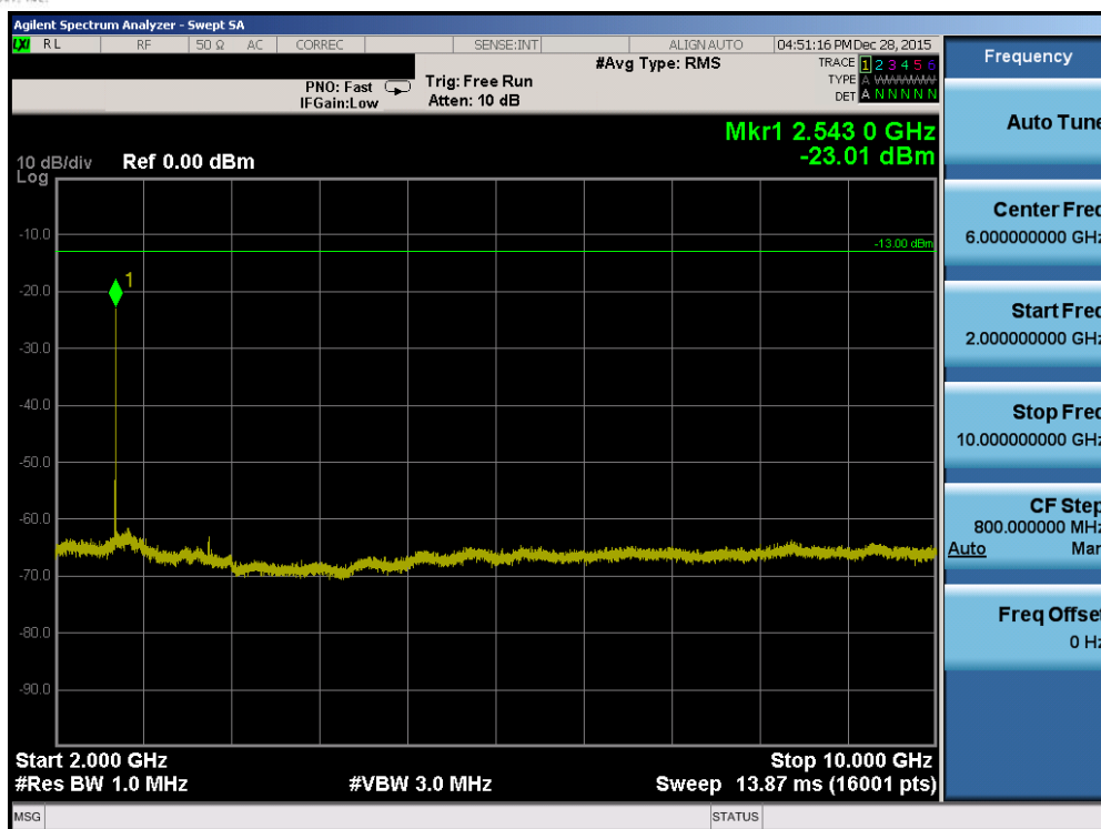
Plot 7-89. Conducted Spurious Plot (Band 5 – 3.0MHz QPSK – RB Size 1, RB Offset 0 – High Channel)
