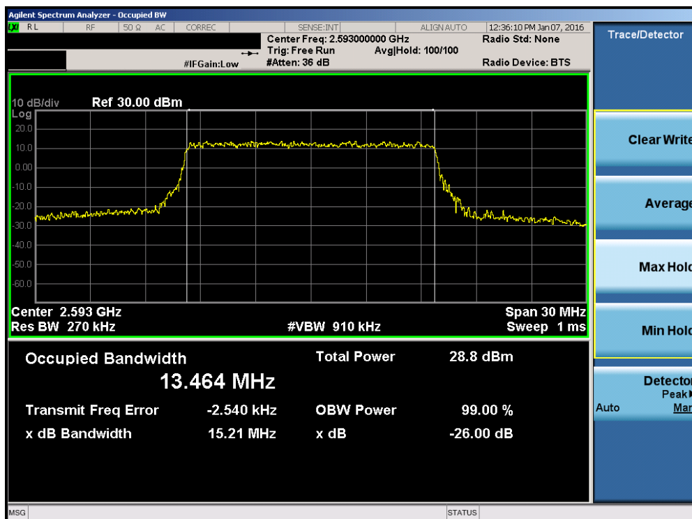
Plot 7-60. Occupied Bandwidth Plot (Band 41 – 15.0MHz 16-QAM – RB Size 75)
