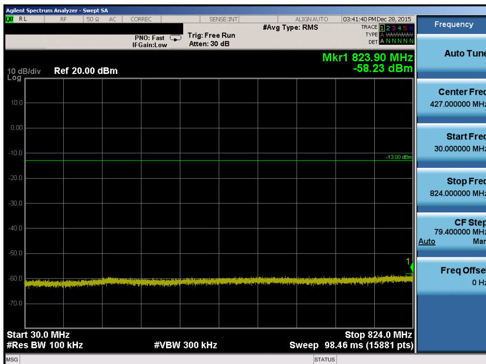
Plot 7-96. Conducted Spurious Plot (Band 26 – 5.0MHz QPSK – RB Size 1, RB Offset 0 – High Channel)
