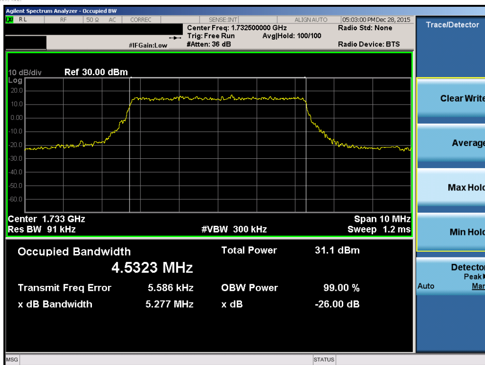
Plot 7-35. Occupied Bandwidth Plot (Band 4 – 5.0MHz QPSK – RB Size 25)
