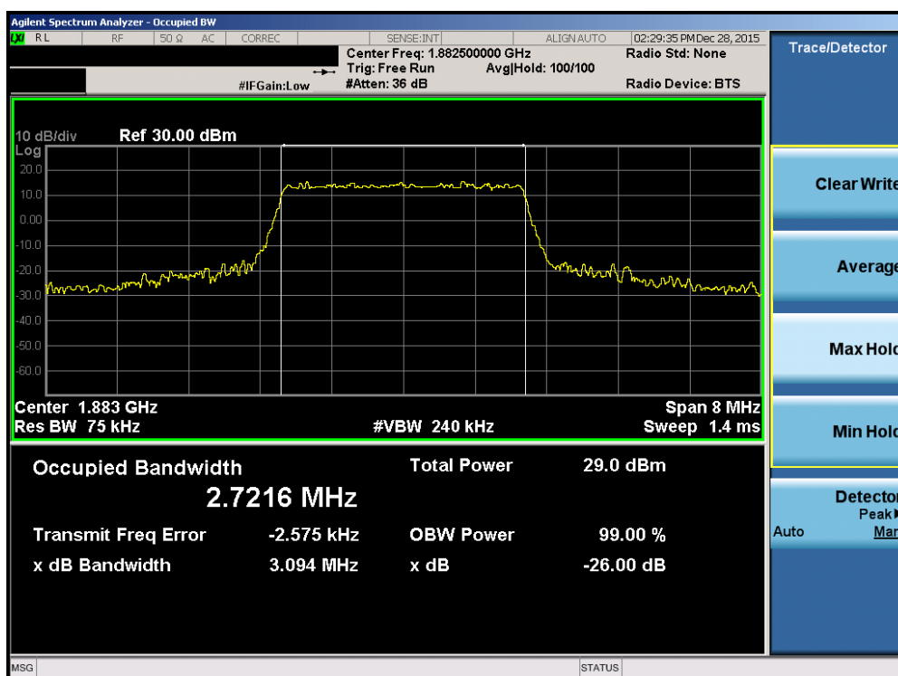
Plot 7-46. Occupied Bandwidth Plot (Band 2/25 – 3.0MHz 16-QAM – RB Size 15)
