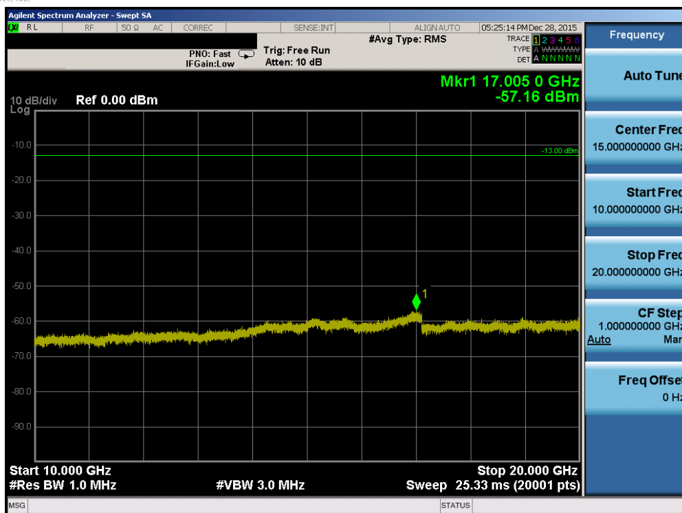
Plot 7-101. Conducted Spurious Plot (Band 4 – 10.0MHz QPSK – RB Size 1, RB Offset 0 – Low Channel)
