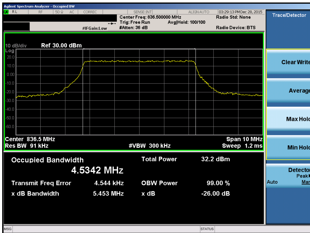
Plot 7-25. Occupied Bandwidth Plot (Band 26 – 5.0MHz QPSK – RB Size 25)
