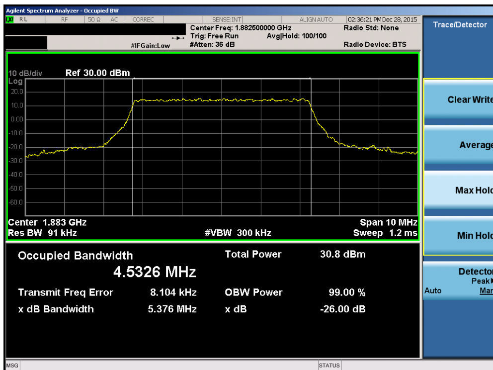
Plot 7-48. Occupied Bandwidth Plot (Band 2/25 – 5.0MHz 16-QAM – RB Size 25)
