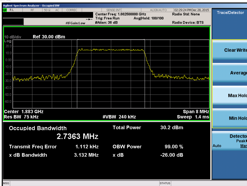
Plot 7-45. Occupied Bandwidth Plot (Band 2/25 – 3.0MHz QPSK – RB Size 15)
