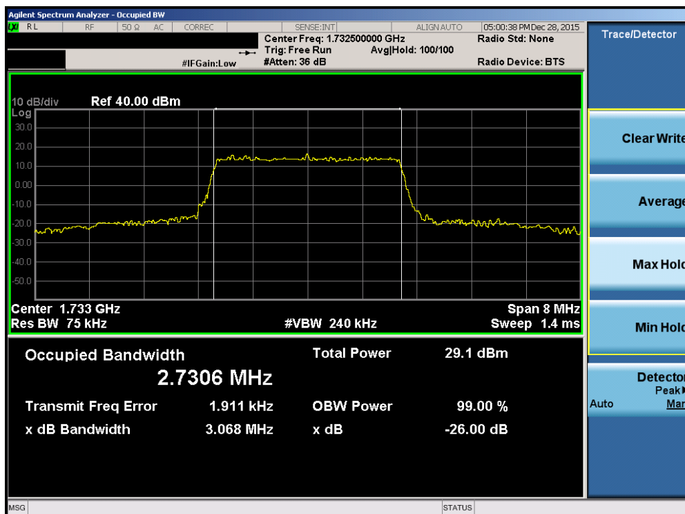
Plot 7-34. Occupied Bandwidth Plot (Band 4 – 3.0MHz 16-QAM – RB Size 15)
