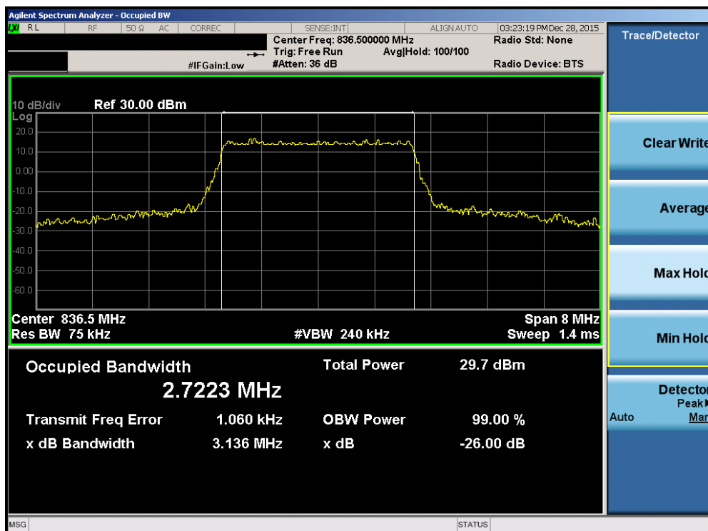
Plot 7-24. Occupied Bandwidth Plot (Band 26 – 3.0MHz 16-QAM – RB Size 15)
