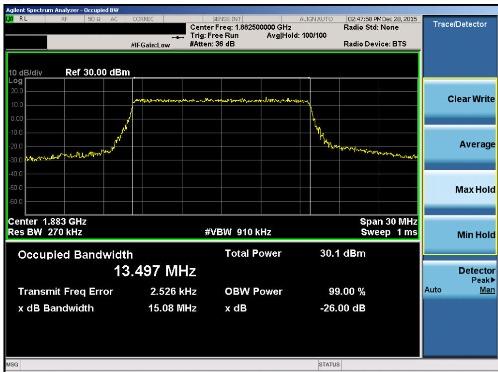
Plot 7-51. Occupied Bandwidth Plot (Band 2/25 – 15.0MHz QPSK – RB Size 75)
