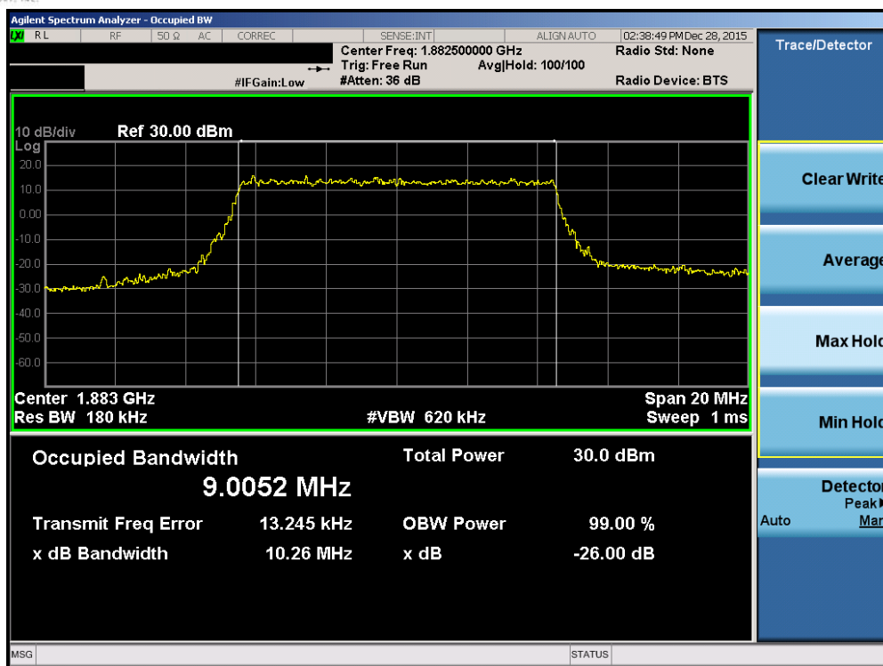
Plot 7-49. Occupied Bandwidth Plot (Band 2/25 – 10.0MHz QPSK – RB Size 50)
