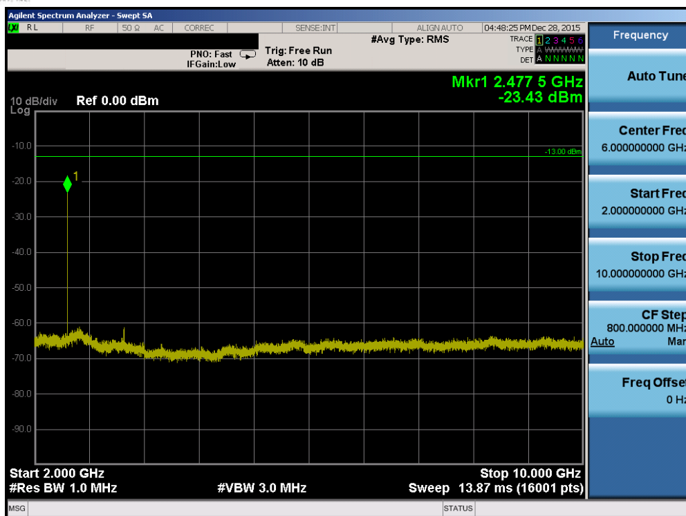
Plot 7-83. Conducted Spurious Plot (Band 5 – 3.0MHz QPSK – RB Size 1, RB Offset 0 – Low Channel)
