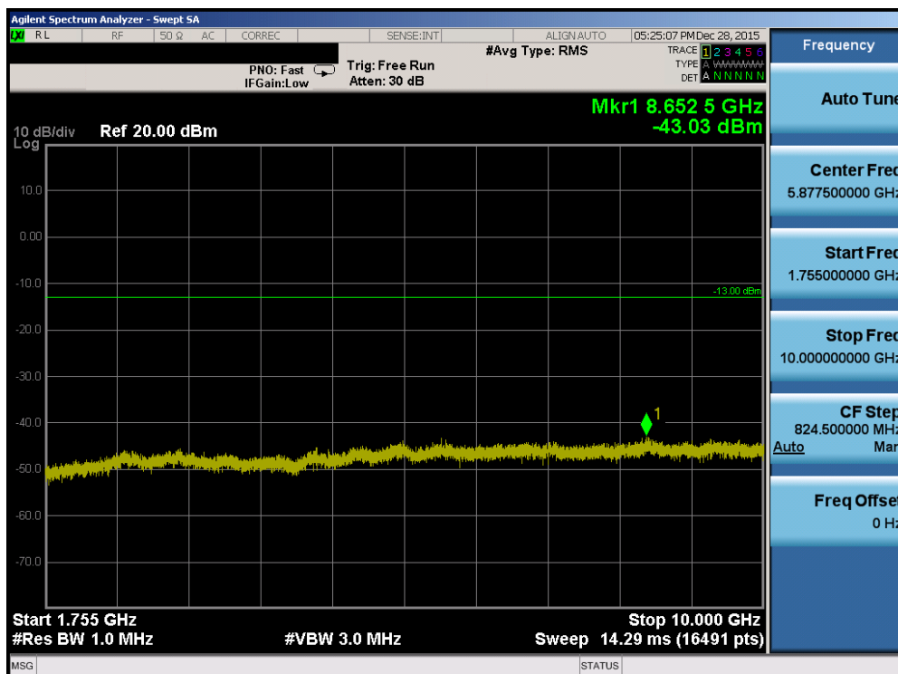
Plot 7-100. Conducted Spurious Plot (Band 4 – 10.0MHz QPSK – RB Size 1, RB Offset 0 – Low Channel)
