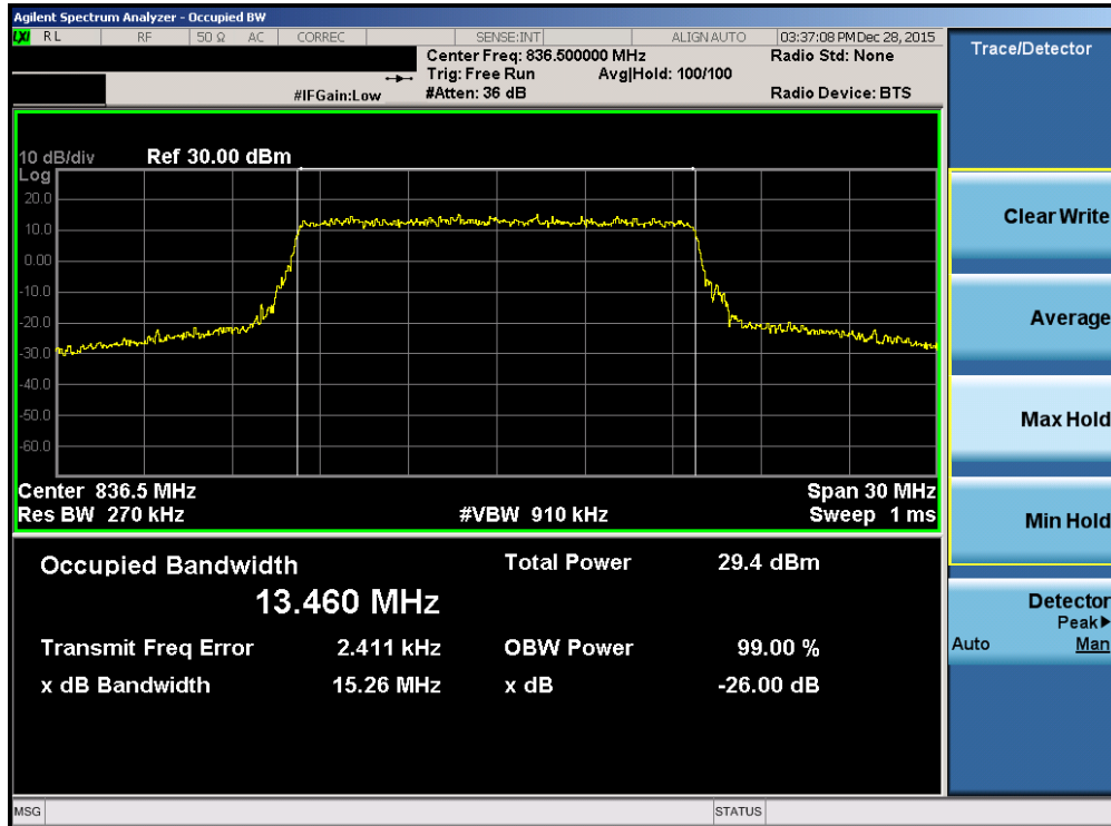
Plot 7-30. Occupied Bandwidth Plot (Band 26 – 15.0MHz 16-QAM – RB Size 75)
