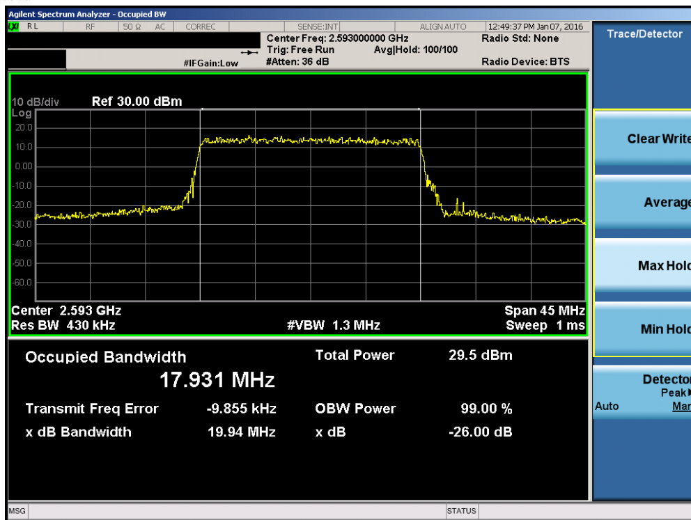
Plot 7-61. Occupied Bandwidth Plot (Band 41 – 20.0MHz QPSK – RB Size 100)
