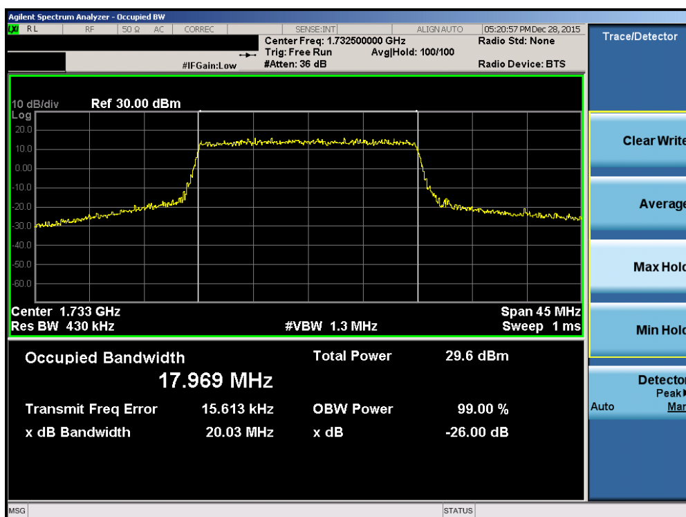
Plot 7-42. Occupied Bandwidth Plot (Band 4 – 20.0MHz 16-QAM – RB Size 100)
