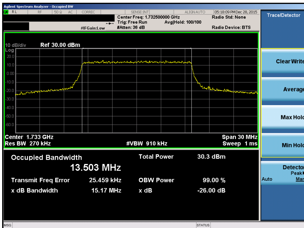
Plot 7-40. Occupied Bandwidth Plot (Band 4 – 15.0MHz 16-QAM – RB Size 75)
