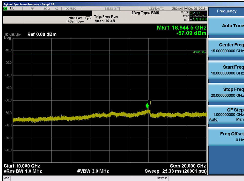
Plot 7-104. Conducted Spurious Plot (Band 4 – 10.0MHz QPSK – RB Size 1, RB Offset 0 – Mid Channel)
