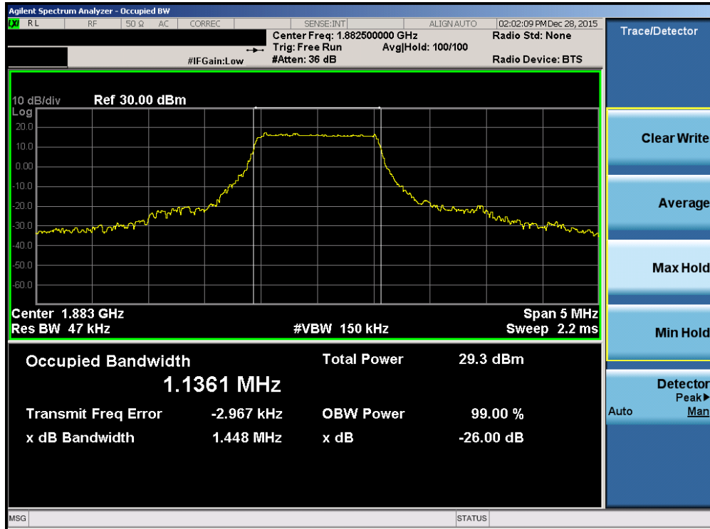
Plot 7-43. Occupied Bandwidth Plot (Band 2/25 – 1.4MHz QPSK – RB Size 6)
