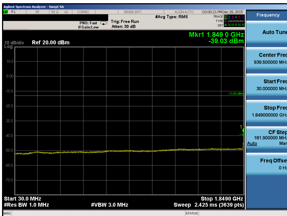
Plot 7-108. Conducted Spurious Plot (Band 2/25 – 5.0MHz QPSK – RB Size 1, RB Offset 0 – Low Channel)
