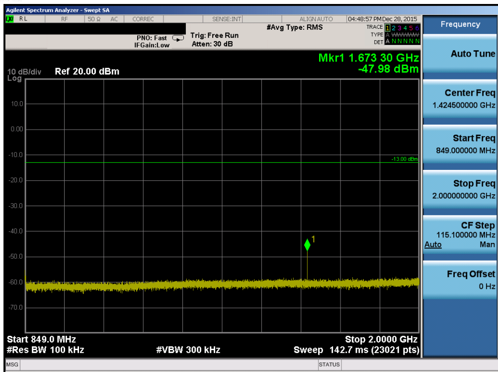
Plot 7-85. Conducted Spurious Plot (Band 5 – 3.0MHz QPSK – RB Size 1, RB Offset 0 – Mid Channel)
