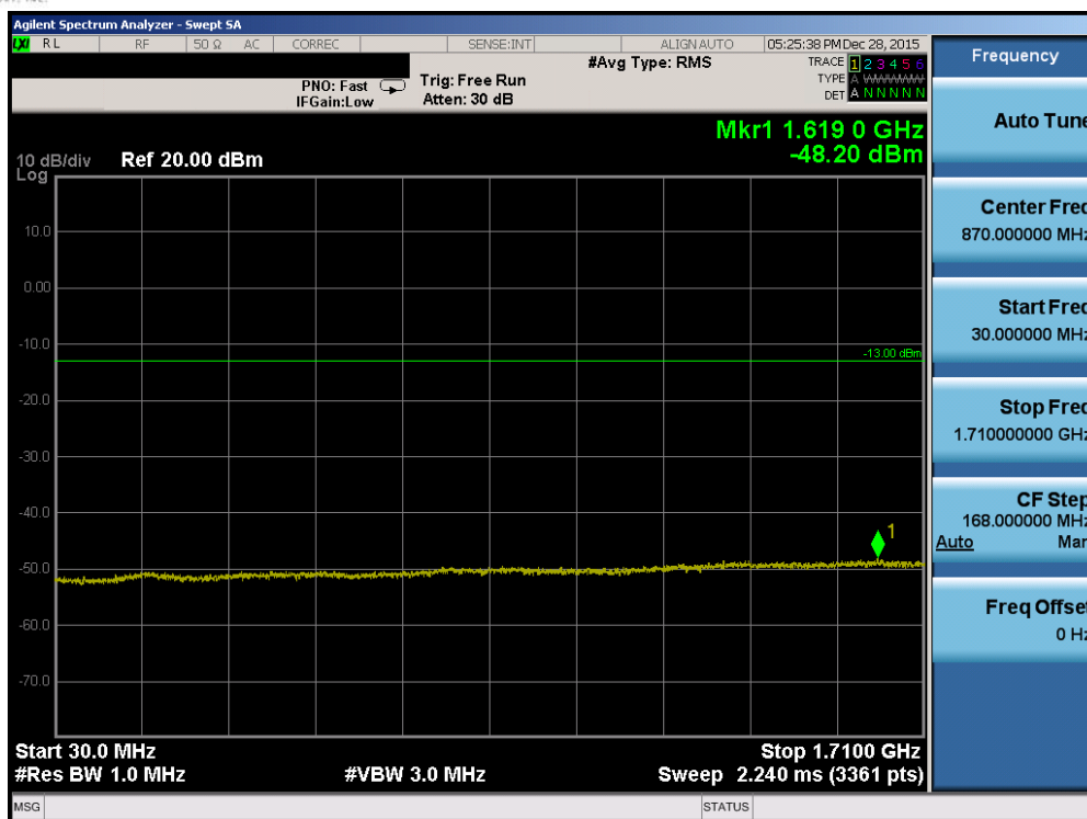
Plot 7-105. Conducted Spurious Plot (Band 4 – 10.0MHz QPSK – RB Size 1, RB Offset 0 – High Channel)
