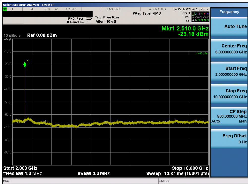
Plot 7-86. Conducted Spurious Plot (Band 5 – 3.0MHz QPSK – RB Size 1, RB Offset 0 – Mid Channel)
