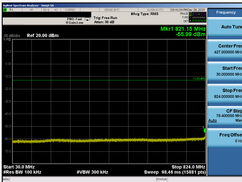
Plot 7-93. Conducted Spurious Plot (Band 26 – 5.0MHz QPSK – RB Size 1, RB Offset 0 – Mid Channel)
