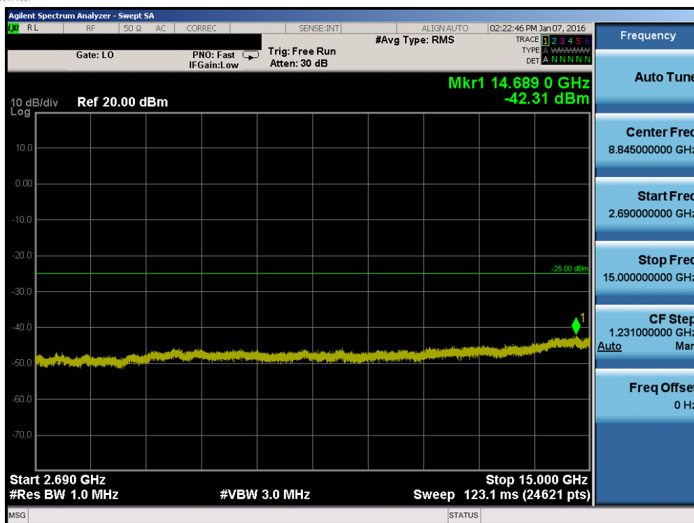
Plot 7-121. Conducted Spurious Plot (Band 41 – 15.0MHz QPSK – RB Size 1, RB Offset 0 – Mid Channel)
