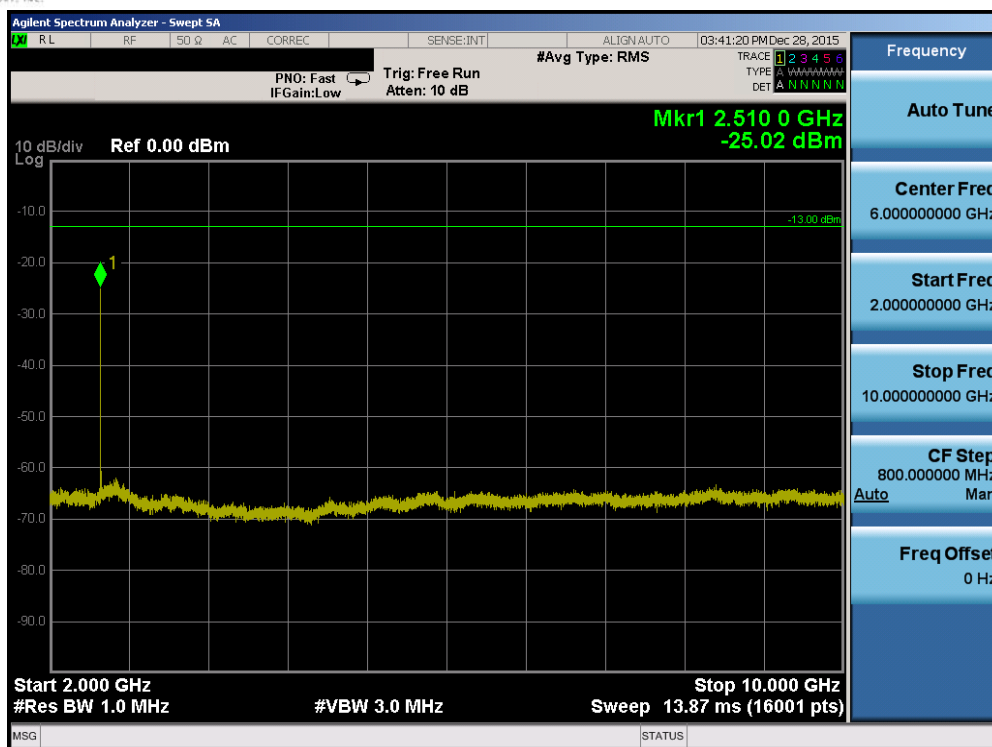
Plot 7-95. Conducted Spurious Plot (Band 26 – 5.0MHz QPSK – RB Size 1, RB Offset 0 – Mid Channel)
