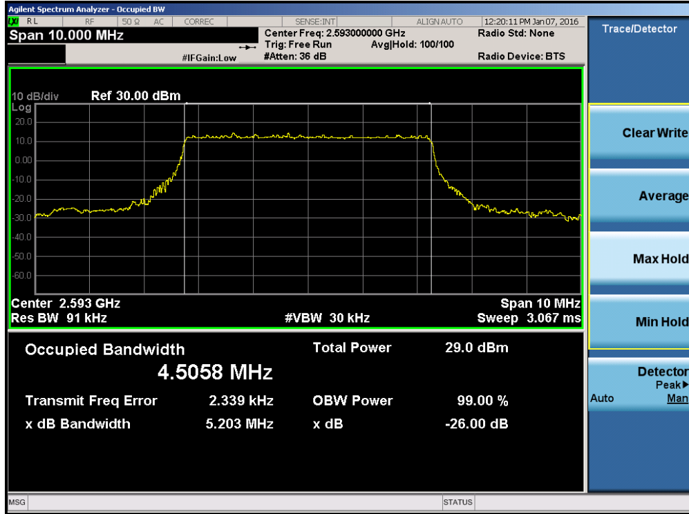
Plot 7-55. Occupied Bandwidth Plot (Band 41 – 5.0MHz QPSK – RB Size 25)
