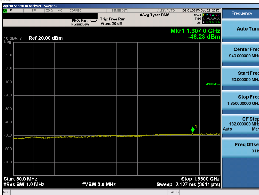
Plot 7-111. Conducted Spurious Plot (Band 2/25 – 5.0MHz QPSK – RB Size 1, RB Offset 0 – Mid Channel)
