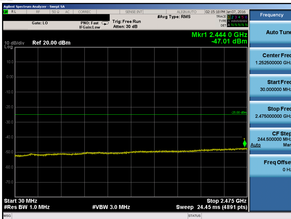
Plot 7-117. Conducted Spurious Plot (Band 41 – 15.0MHz QPSK – RB Size 1, RB Offset 0 – Low Channel)
