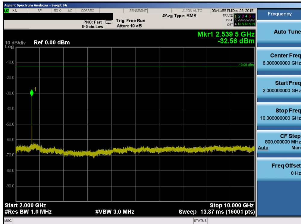
Plot 7-98. Conducted Spurious Plot (Band 26 – 5.0MHz QPSK – RB Size 1, RB Offset 0 – High Channel)
