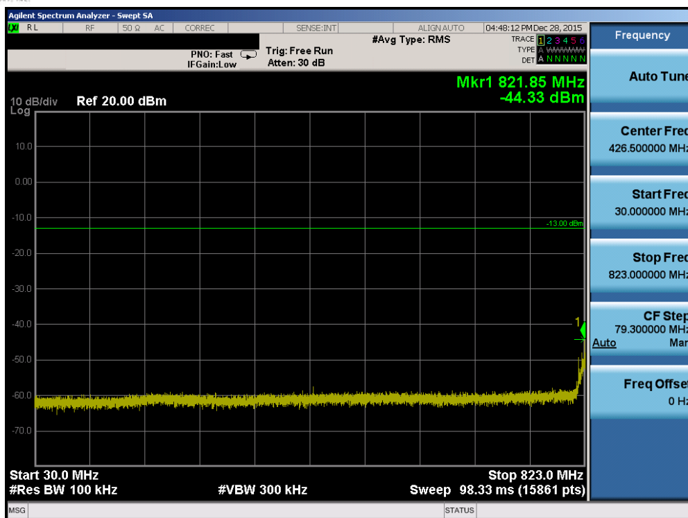
Plot 7-81. Conducted Spurious Plot (Band 5 – 3.0MHz QPSK – RB Size 1, RB Offset 0 – Low Channel)
