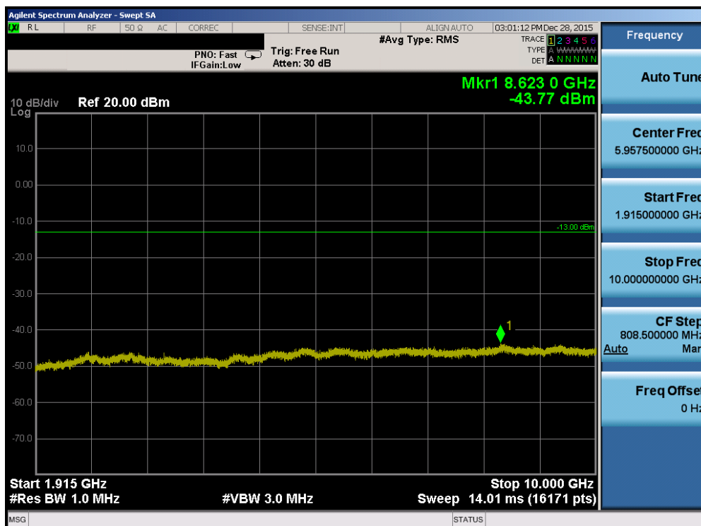
Plot 7-112. Conducted Spurious Plot (Band 2/25 – 5.0MHz QPSK – RB Size 1, RB Offset 0 – Mid Channel)
