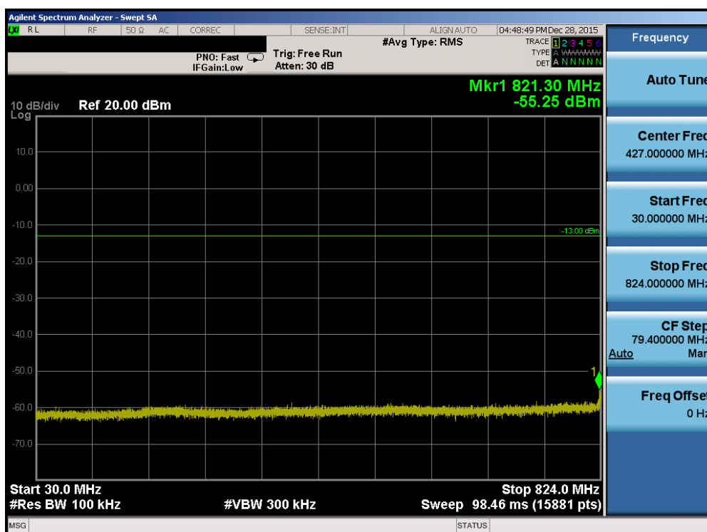
Plot 7-84. Conducted Spurious Plot (Band 5 – 3.0MHz QPSK – RB Size 1, RB Offset 0 – Mid Channel)
