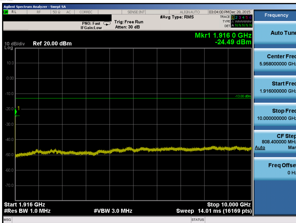
Plot 7-115. Conducted Spurious Plot (Band 2/25 – 5.0MHz QPSK – RB Size 1, RB Offset 0 – High Channel)
