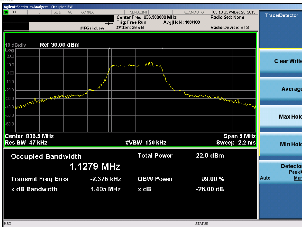
Plot 7-21. Occupied Bandwidth Plot (Band 26 – 1.4MHz QPSK – RB Size 6)
