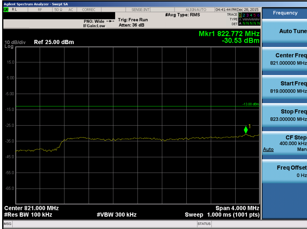
Plot 7-161. Lower Extended Band Edge Plot (Band 5 – 5.0MHz QPSK – RB Size 25)
