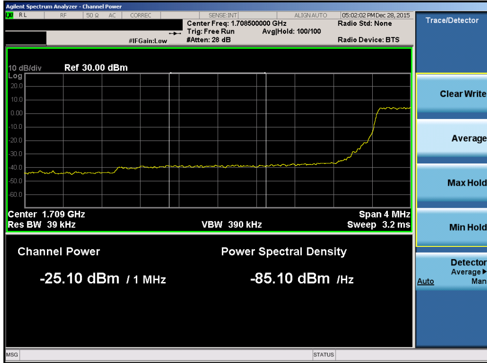
Plot 7-187. Lower Extended Band Edge Plot (Band 4 – 3.0MHz QPSK – RB Size 15)
