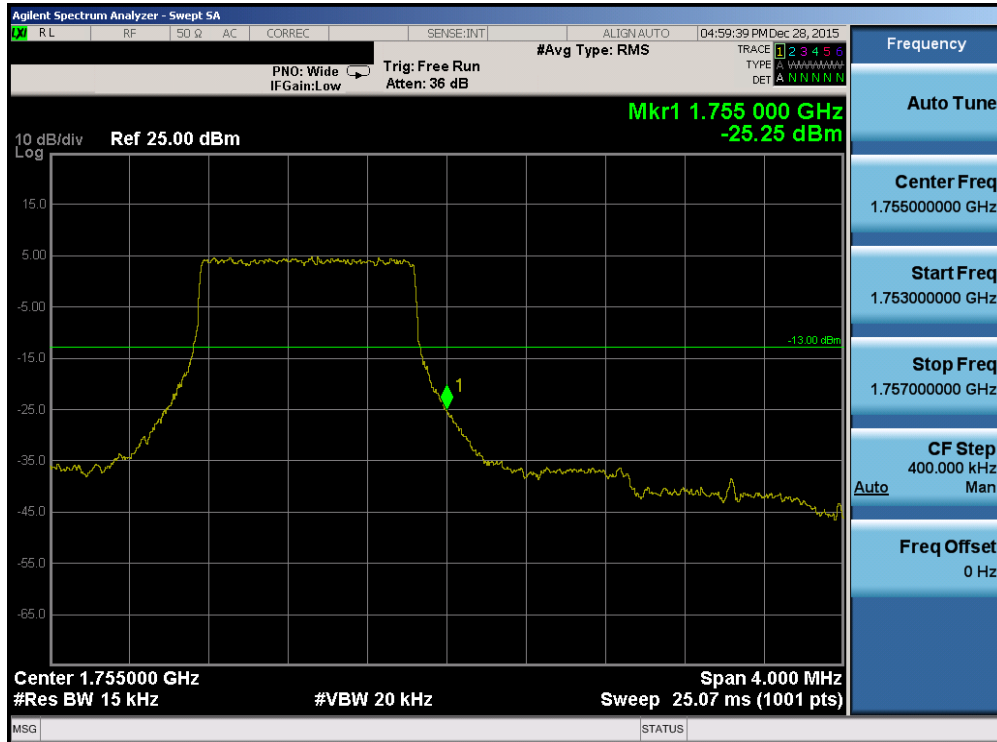
Plot 7-184. Upper Band Edge Plot (Band 4 – 1.4MHz QPSK – RB Size 6)
