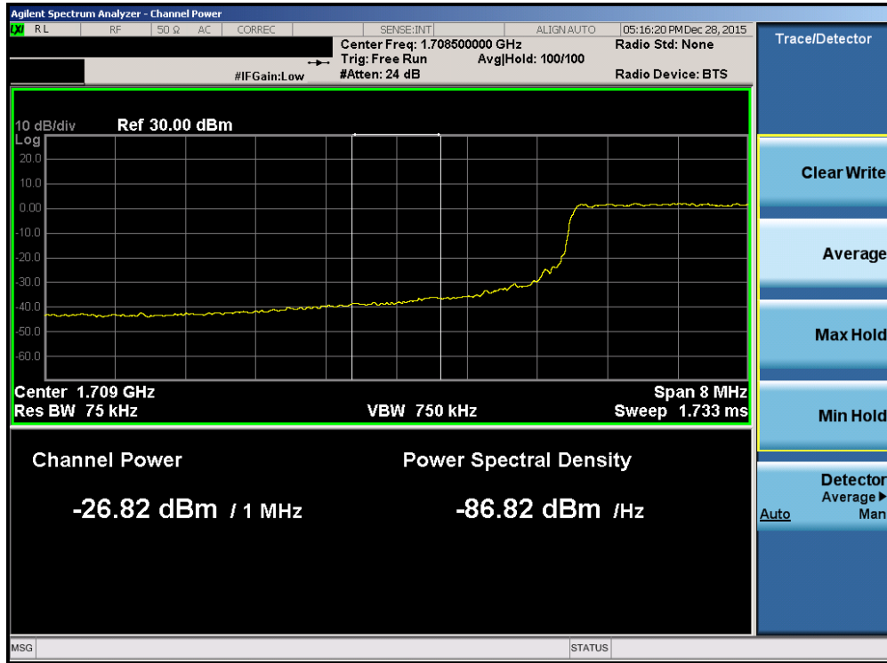
Plot 7-195. Lower Extended Band Edge Plot (Band 4 – 10.0MHz QPSK – RB Size 50)
