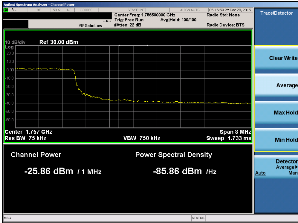
Plot 7-197. Upper Extended Band Edge Plot (Band 4 – 10.0MHz QPSK – RB Size 50)
