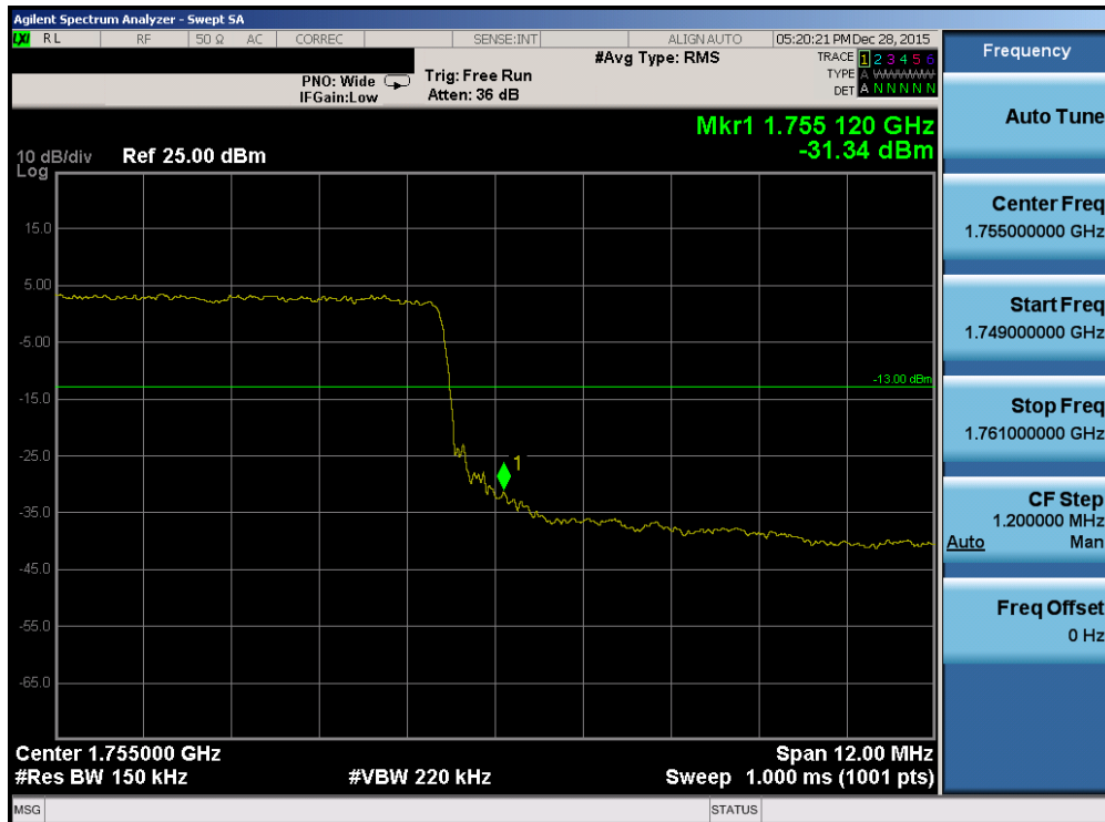
Plot 7-200. Upper Band Edge Plot (Band 4 – 15.0MHz QPSK – RB Size 75)
