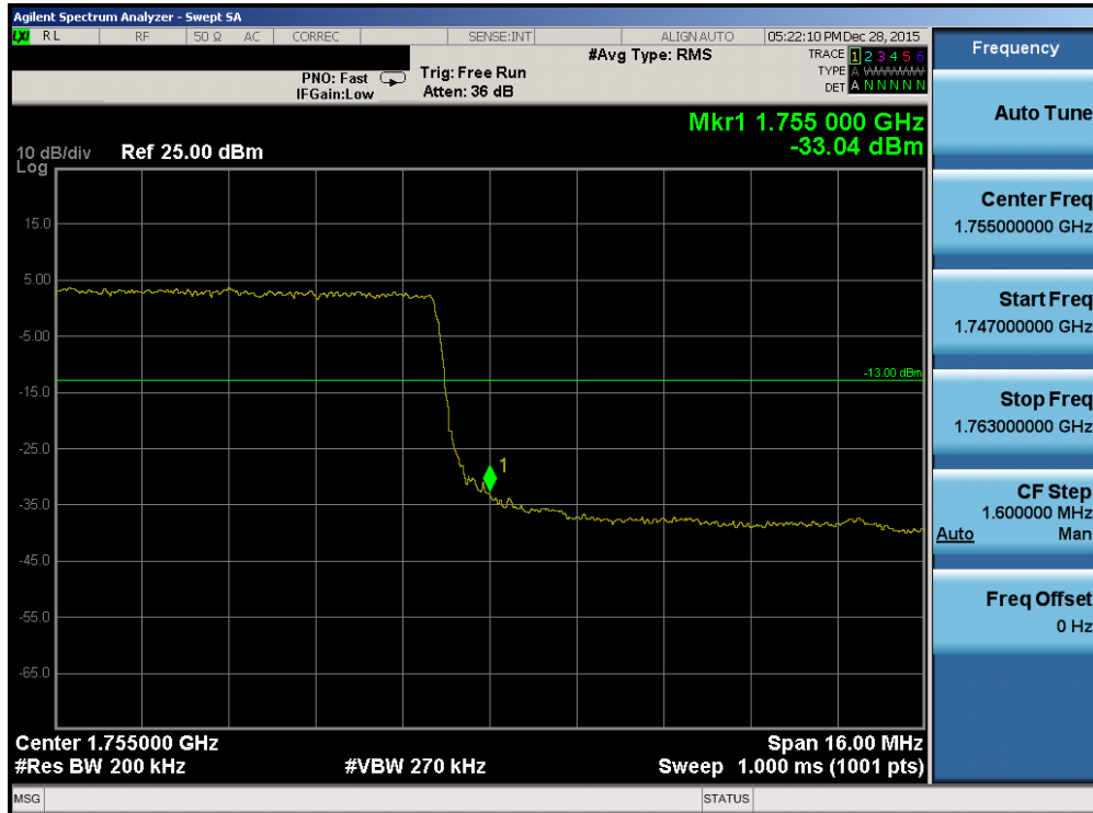
Plot 7-204. Upper Band Edge Plot (Band 4 – 20.0MHz QPSK – RB Size 100)
