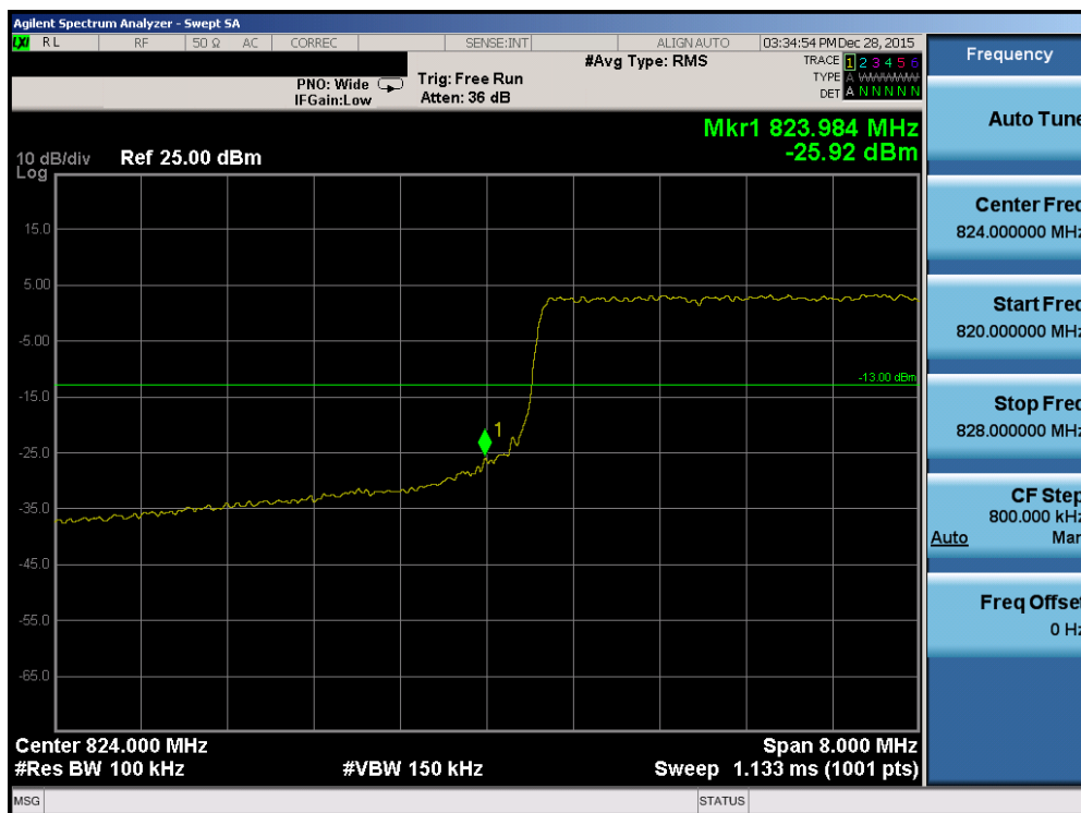
Plot 7-178. Lower Band Edge Plot (Band 26 - 10.0MHz QPSK - RB Size 50)
