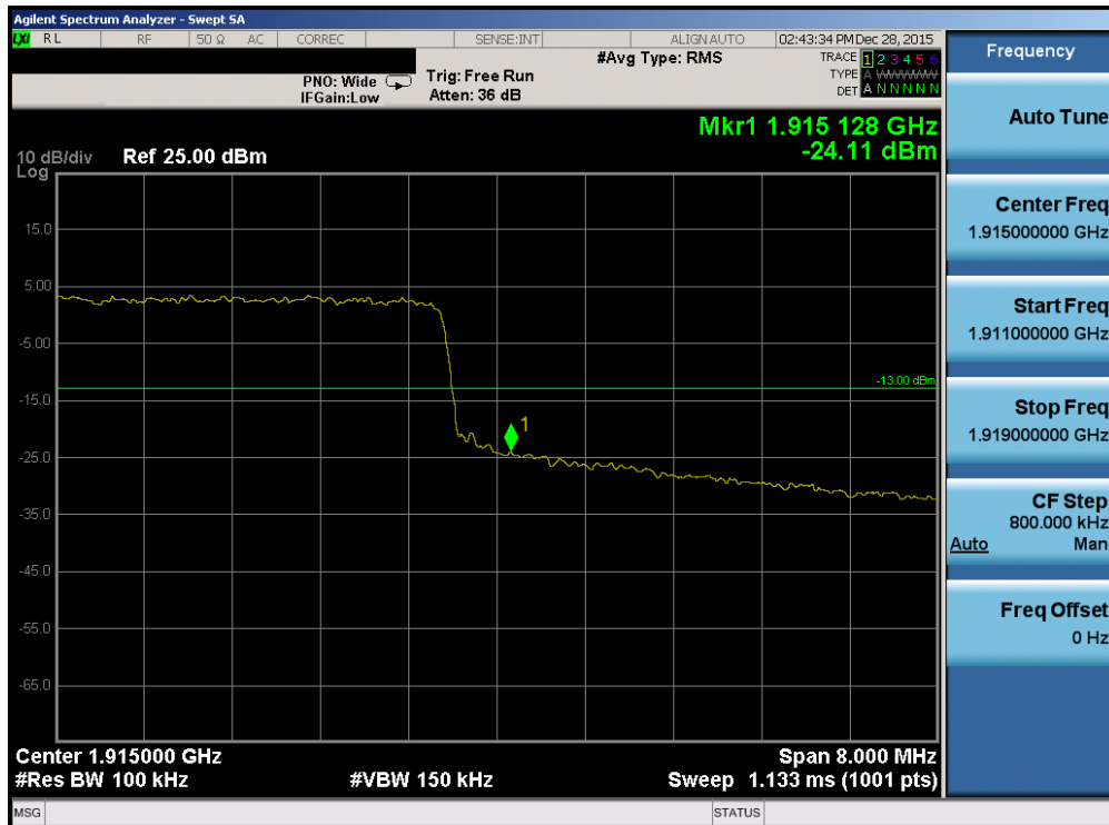
Plot 7-220. Upper Band Edge Plot (Band 2/25 – 10.0MHz QPSK – RB Size 50)
