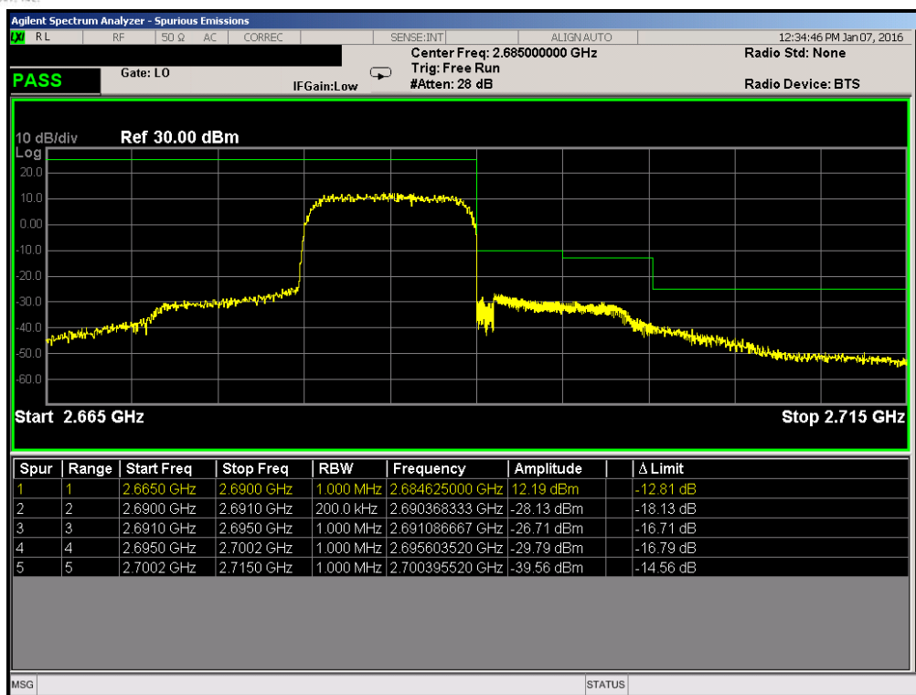
Plot 7-233. Upper ACP Plot (Band 41 – 10.0MHz QPSK – RB Size 50)
