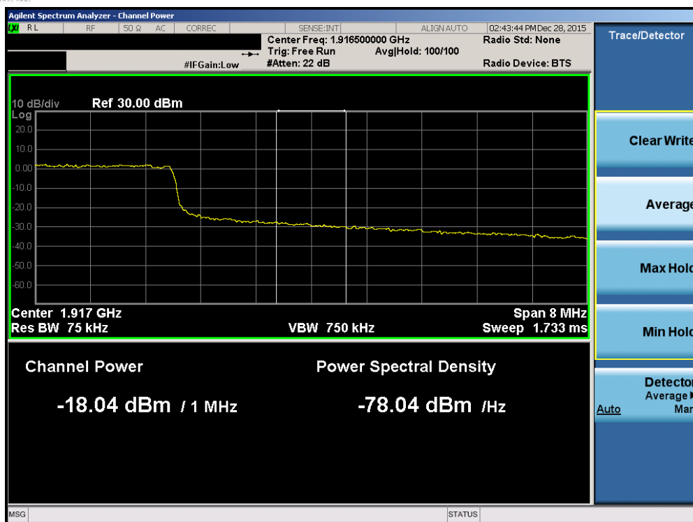
Plot 7-221. Upper Extended Band Edge Plot (Band 2/25 – 10.0MHz QPSK – RB Size 50)
