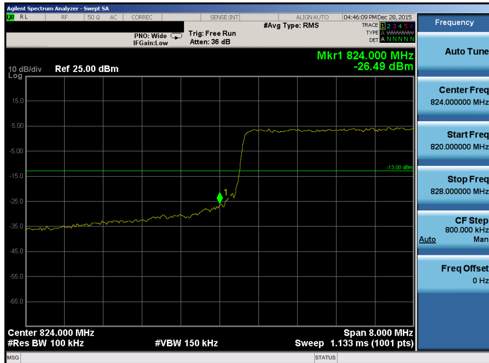
Plot 7-164. Lower Band Edge Plot (Band 5 - 10.0MHz QPSK - RB Size 50)
