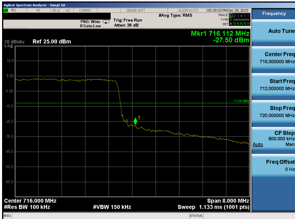
Plot 7-140. Upper Band Edge Plot (Band 12/17 – 10.0MHz QPSK – RB Size 50)
