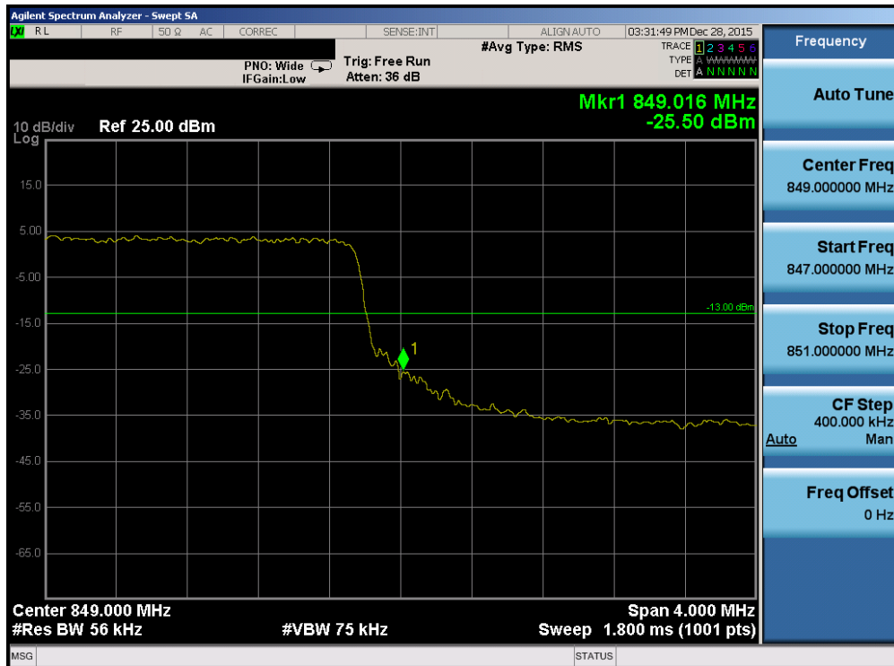
Plot 7-176. Upper Band Edge Plot (Band 26 – 5.0MHz QPSK – RB Size 25)
