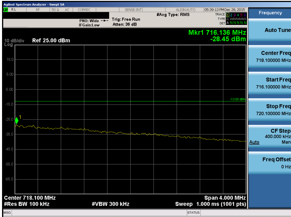
Plot 7-141. Upper Extended Band Edge Plot (Band 12/17 – 10.0MHz QPSK – RB Size 50)
