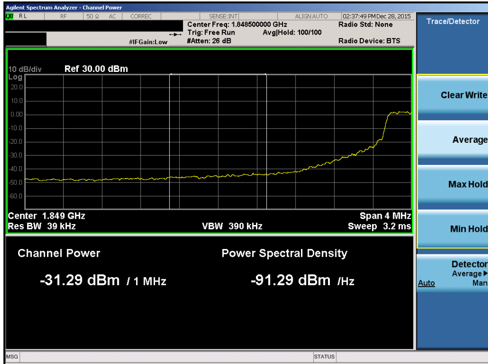
Plot 7-215. Lower Extended Band Edge Plot (Band 2/25 – 5.0MHz QPSK – RB Size 25)
