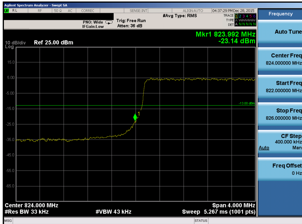
Plot 7-156. Lower Band Edge Plot (Band 5 - 3.0MHz QPSK - RB Size 15)
