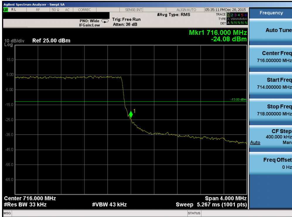
Plot 7-132. Upper Band Edge Plot (Band 12 – 3.0MHz QPSK – RB Size 15)
