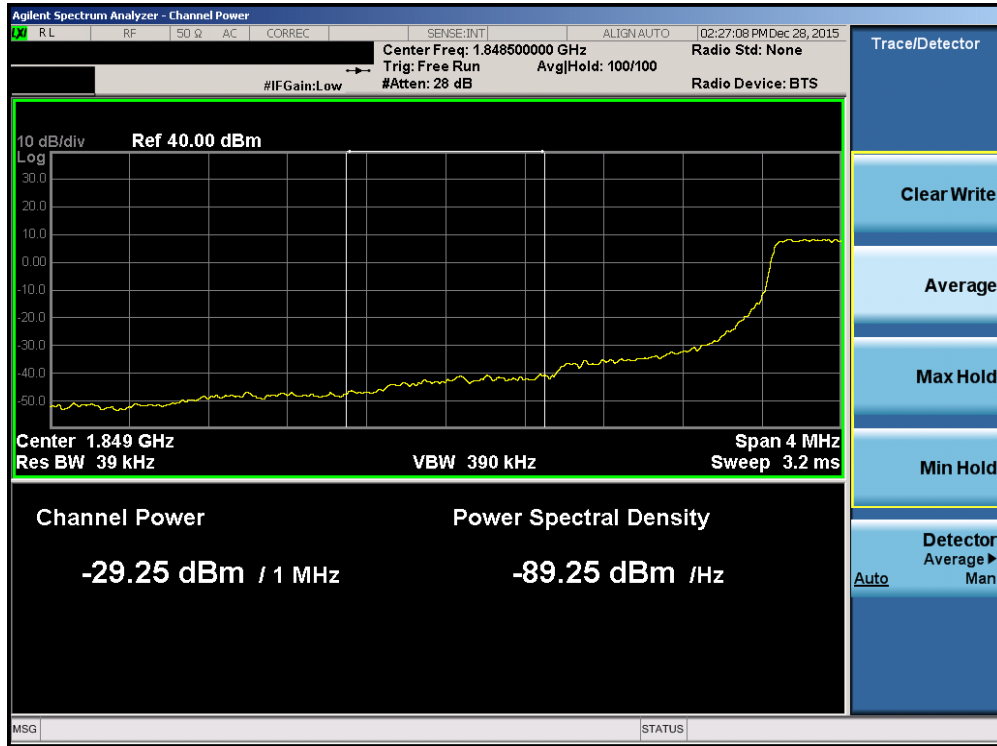
Plot 7-207. Lower Extended Band Edge Plot (Band 2/25 – 1.4MHz QPSK – RB Size 6)
