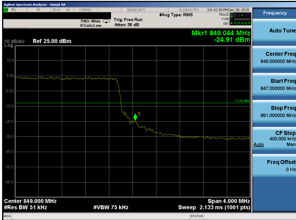
Plot 7-162. Upper Band Edge Plot (Band 5 – 5.0MHz QPSK – RB Size 25)
