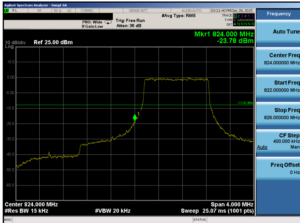
Plot 7-166. Lower Band Edge Plot (Band 26 – 1.4MHz QPSK – RB Size 6)
