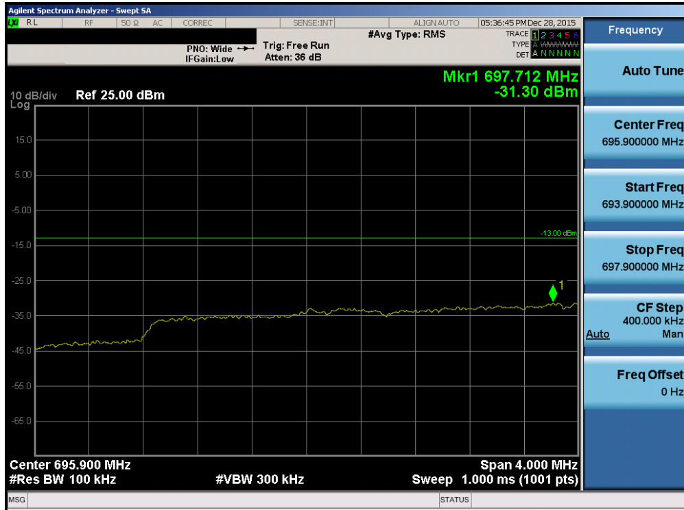
Plot 7-135. Lower Extended Band Edge Plot (Band 12/17 – 5.0MHz QPSK – RB Size 25)
