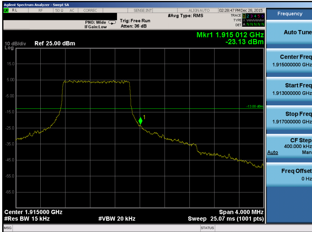
Plot 7-208. Upper Band Edge Plot (Band 2/25 – 1.4MHz QPSK – RB Size 6)
