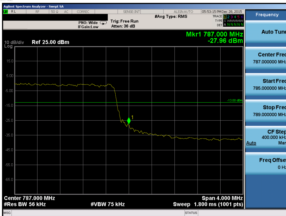
Plot 7-145. Upper Band Edge Plot (Band 13 – 5.0MHz QPSK – RB Size 25)
