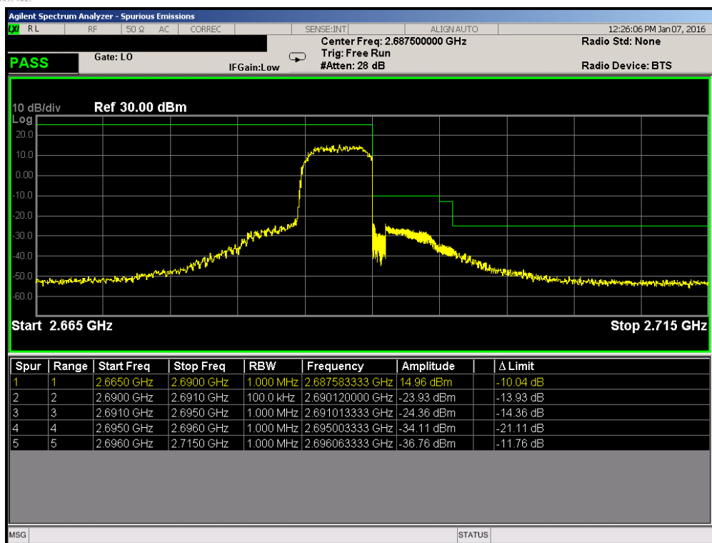
Plot 7-231. Upper ACP Plot (Band 41 – 5.0MHz QPSK – RB Size 25)
