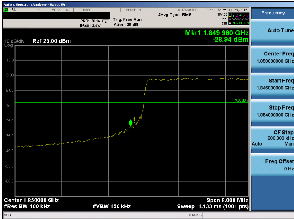
Plot 7-218. Lower Band Edge Plot (Band 2/25 – 10.0MHz QPSK – RB Size 50)
