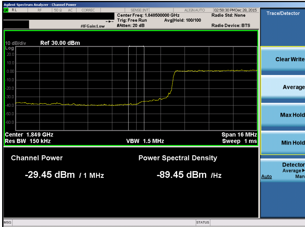
Plot 7-227. Lower Extended Band Edge Plot (Band 2/25 – 20.0MHz QPSK – RB Size 100)
