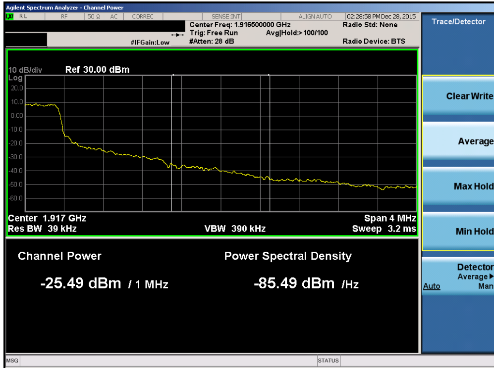
Plot 7-209. Upper Extended Band Edge Plot (Band 2/25 – 1.4MHz QPSK – RB Size 6)
