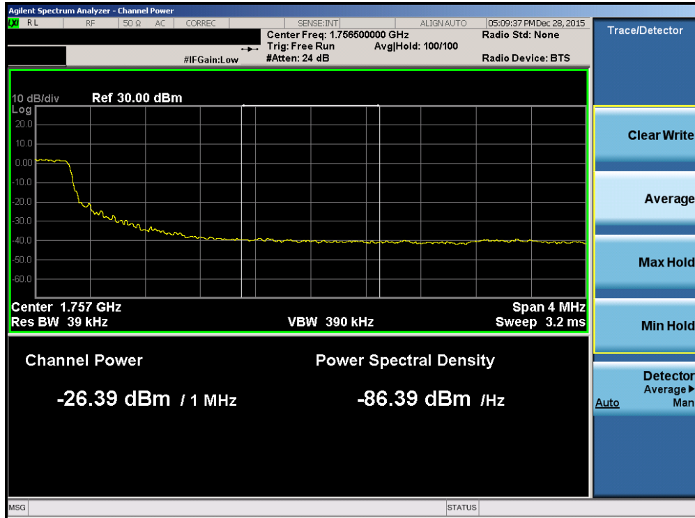
Plot 7-193. Upper Extended Band Edge Plot (Band 4 – 5.0MHz QPSK – RB Size 25)
