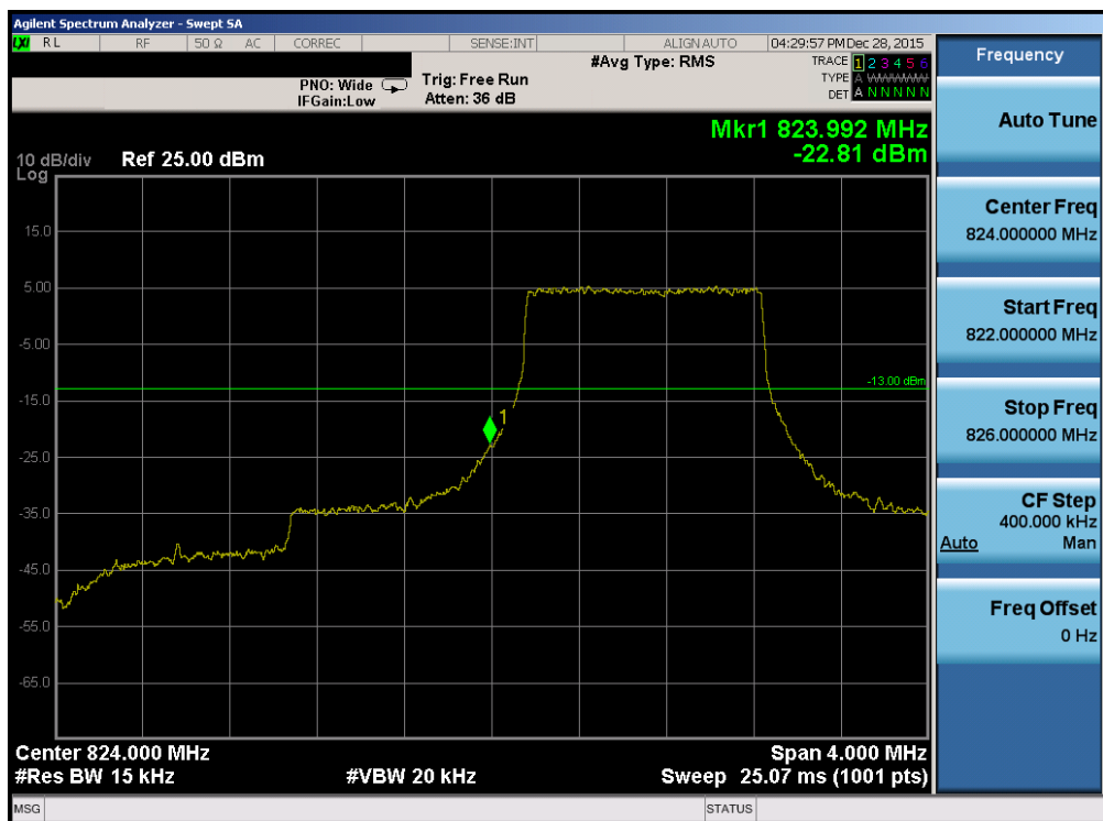
Plot 7-152. Lower Band Edge Plot (Band 5 – 1.4MHz QPSK – RB Size 6)
