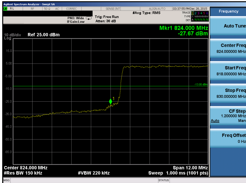
Plot 7-180. Lower Band Edge Plot (Band 26 – 15.0MHz QPSK – RB Size 75)
