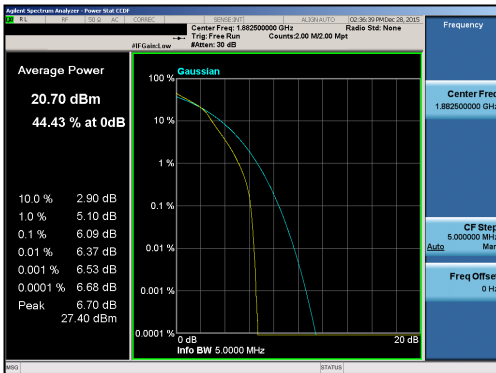
Plot 7-243. PAR Plot (Band 2/25 – 5.0MHz 16-QAM – RB Size 25)
