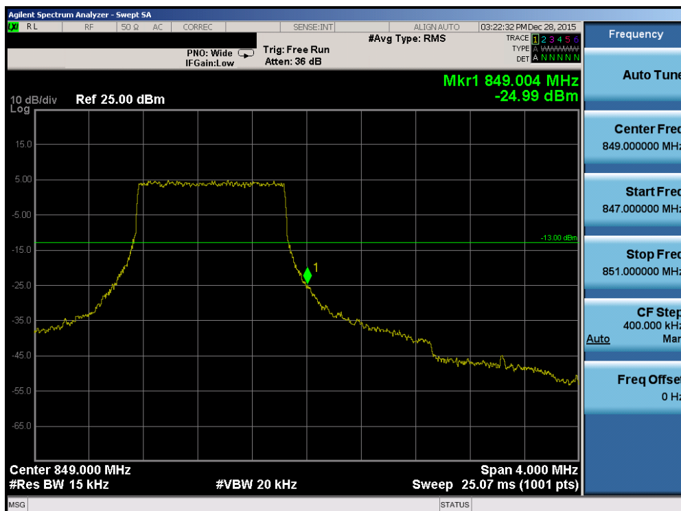
Plot 7-168. Upper Band Edge Plot (Band 26 – 1.4MHz QPSK – RB Size 6)
