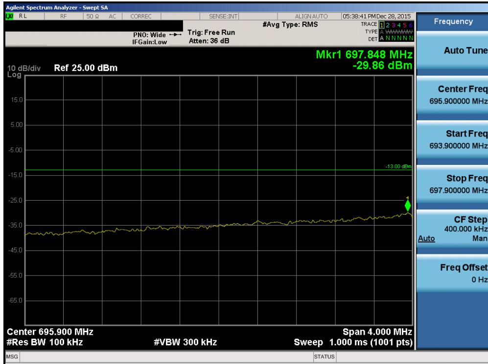
Plot 7-139. Lower Extended Band Edge Plot (Band 12/17 – 10.0MHz QPSK – RB Size 50)
