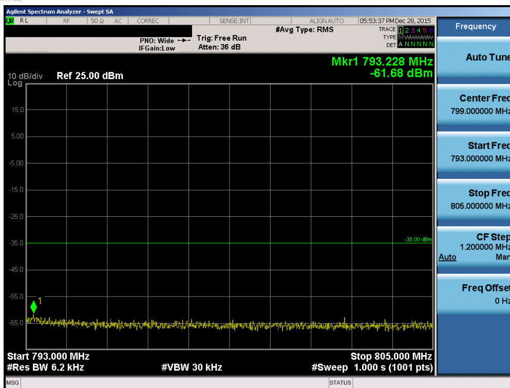
Plot 7-147. Upper Emission Mask Edge Plot (Band 13 – 5.0MHz QPSK – RB Size 25)
