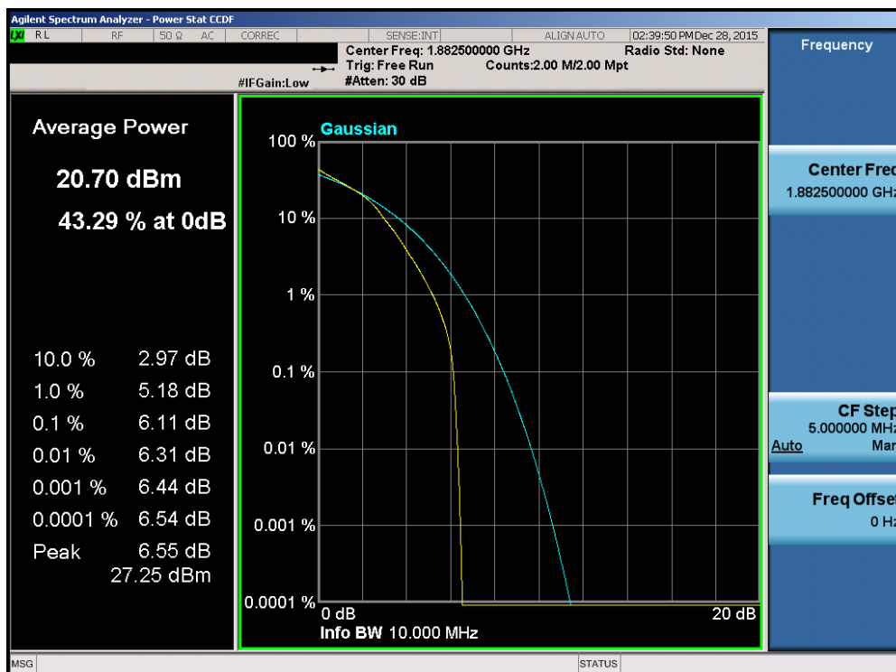
Plot 7-245. PAR Plot (Band 2/25 – 10.0MHz 16-QAM – RB Size 50)
