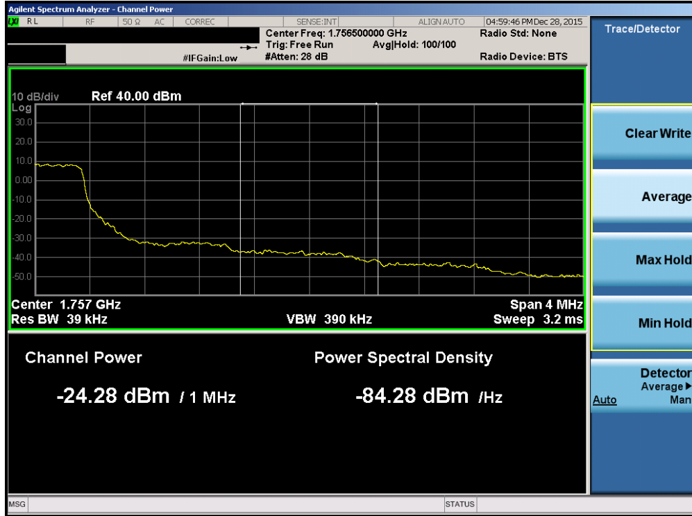
Plot 7-185. Upper Extended Band Edge Plot (Band 4 – 1.4MHz QPSK – RB Size 6)
