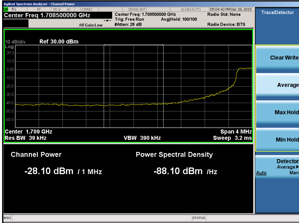
Plot 7-191. Lower Extended Band Edge Plot (Band 4 – 5.0MHz QPSK – RB Size 25)
