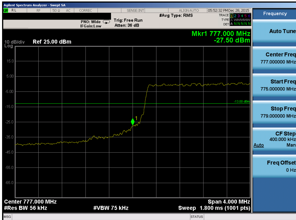
Plot 7-142. Lower Band Edge Plot (Band 13 – 5.0MHz QPSK – RB Size 25)
