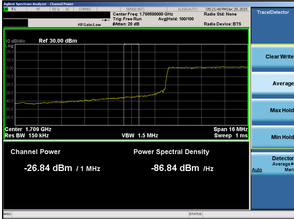
Plot 7-203. Lower Extended Band Edge Plot (Band 4 – 20.0MHz QPSK – RB Size 100)
