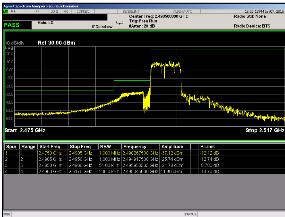
Plot 7-230. Lower ACP Plot (Band 41 – 5.0MHz QPSK – RB Size 25)
