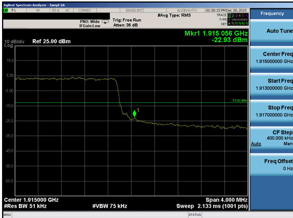
Plot 7-216. Upper Band Edge Plot (Band 2/25 – 5.0MHz QPSK – RB Size 25)
