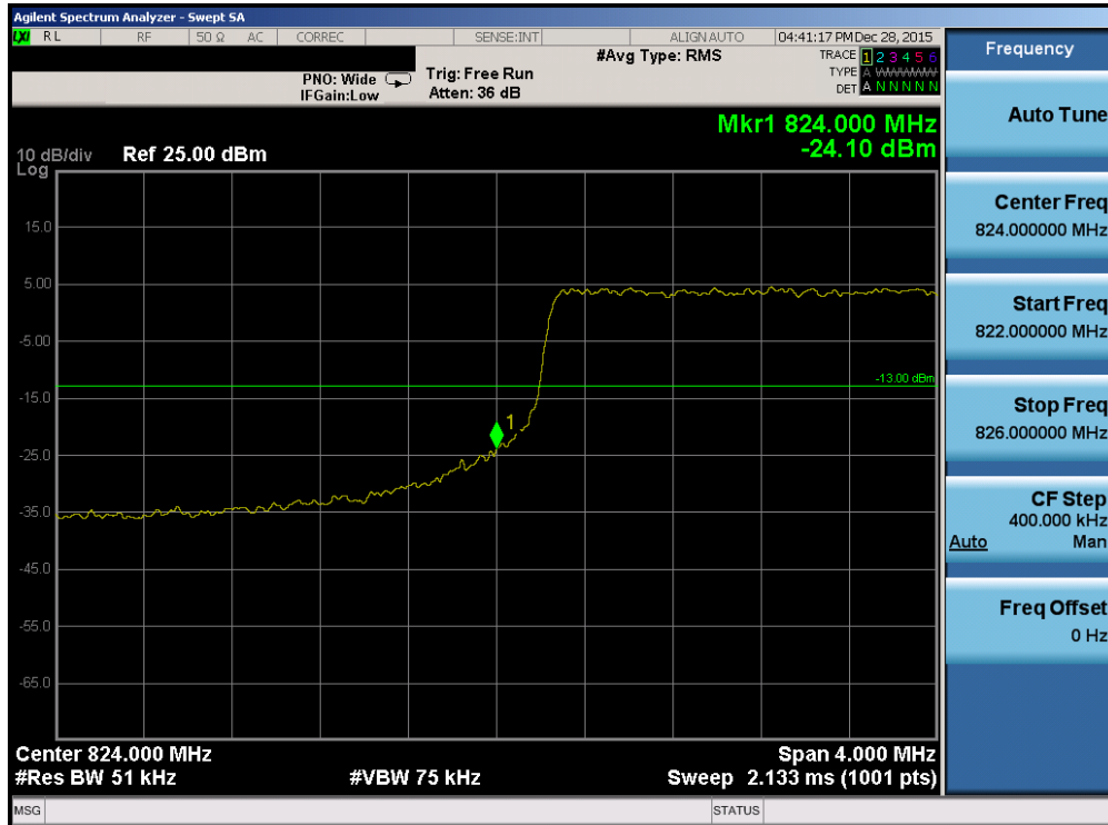
Plot 7-160. Lower Band Edge Plot (Band 5 – 5.0MHz QPSK – RB Size 25)
