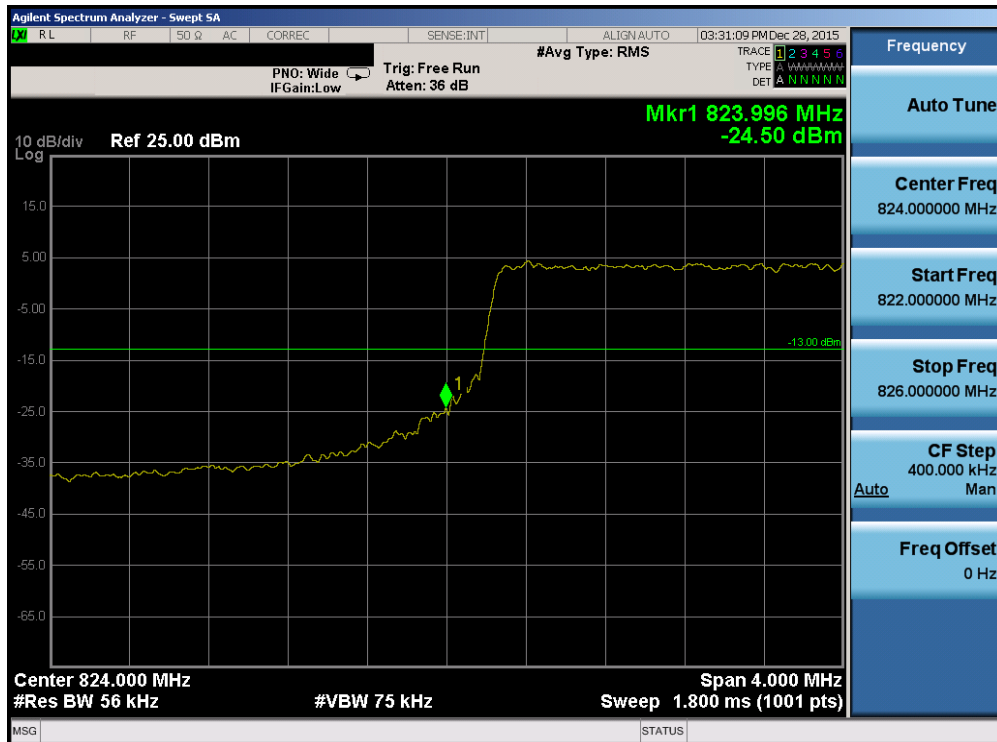
Plot 7-174. Lower Band Edge Plot (Band 26 – 5.0MHz QPSK – RB Size 25)
