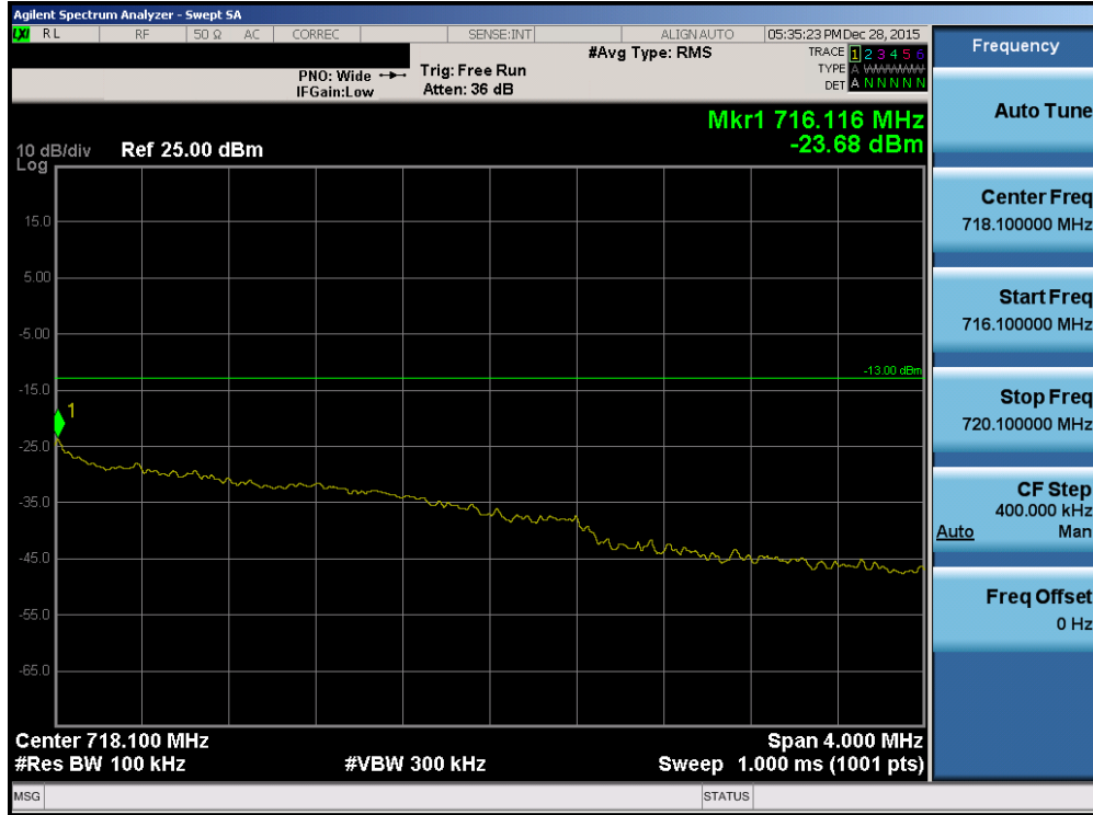
Plot 7-133. Upper Extended Band Edge Plot (Band 12 – 3.0MHz QPSK – RB Size 15)
