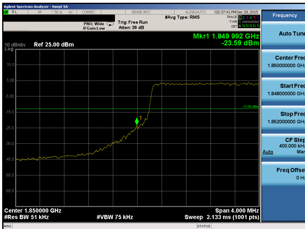
Plot 7-214. Lower Band Edge Plot (Band 2/25 – 5.0MHz QPSK – RB Size 25)
