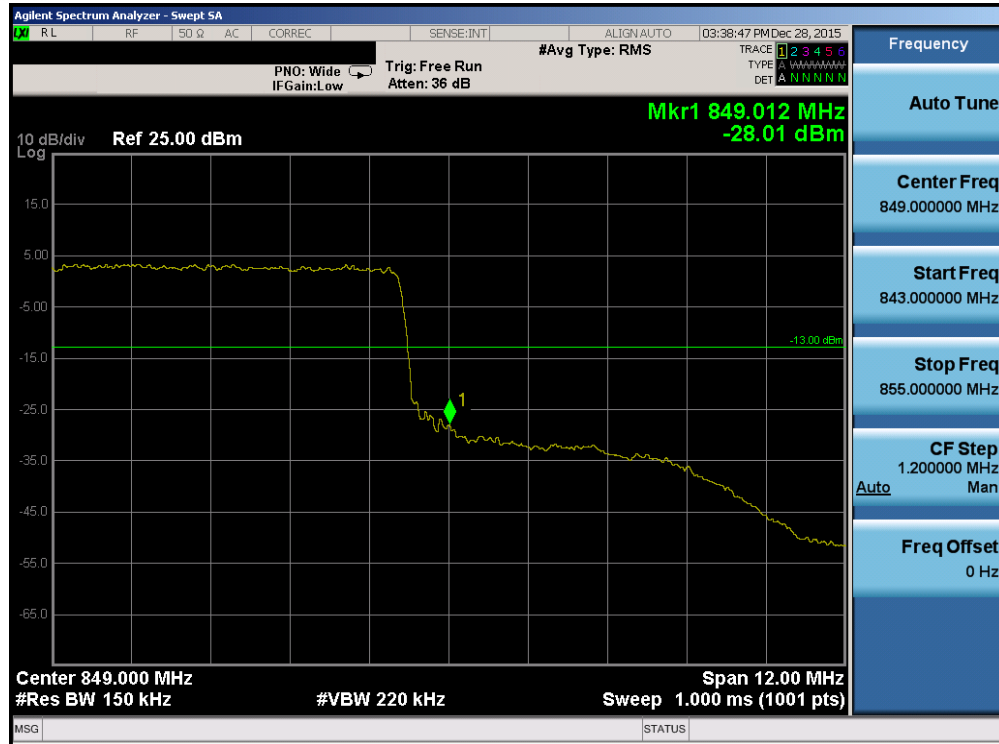
Plot 7-181. Upper Band Edge Plot (Band 26 – 15.0MHz QPSK – RB Size 75)
