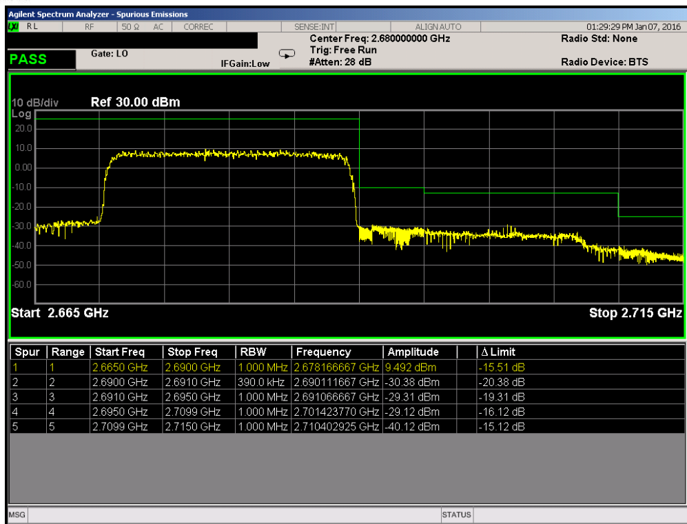
Plot 7-237. Upper ACP Plot (Band 41 – 20.0MHz QPSK – RB Size 100)
