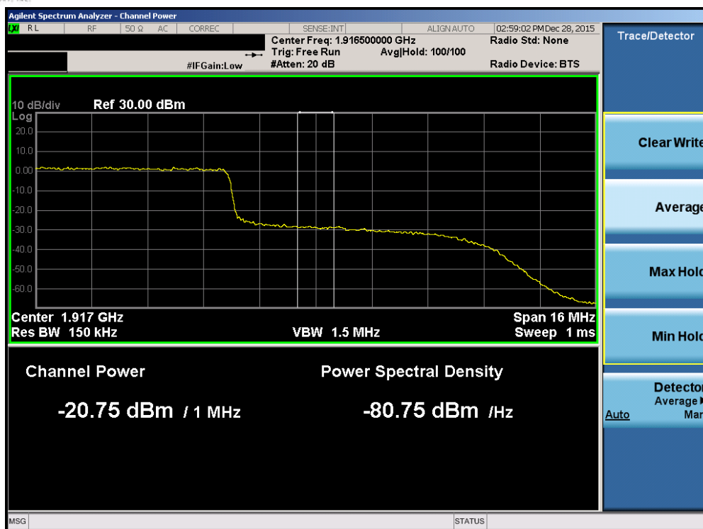
Plot 7-229. Upper Extended Band Edge Plot (Band 2/25 – 20.0MHz QPSK – RB Size 100)
