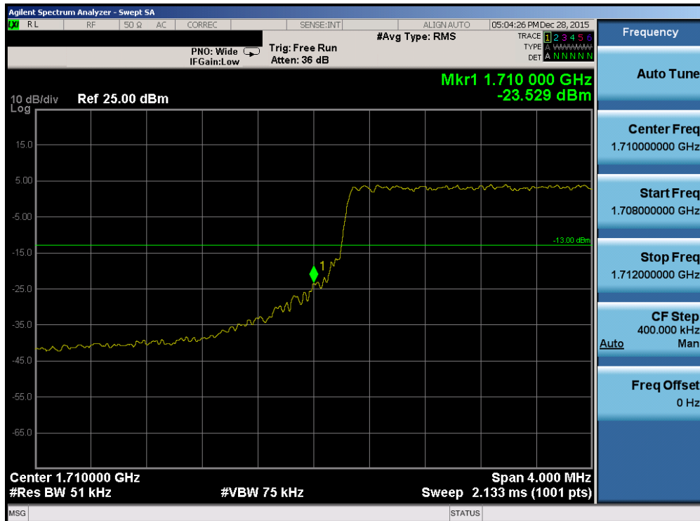
Plot 7-190. Lower Band Edge Plot (Band 4 – 5.0MHz QPSK – RB Size 25)
