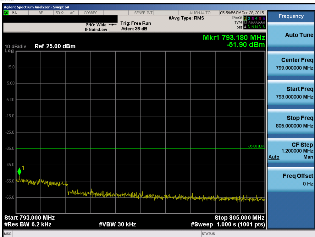
Plot 7-151. Upper Emission Mask Edge Plot (Band 13 – 10.0MHz QPSK – RB Size 50)
