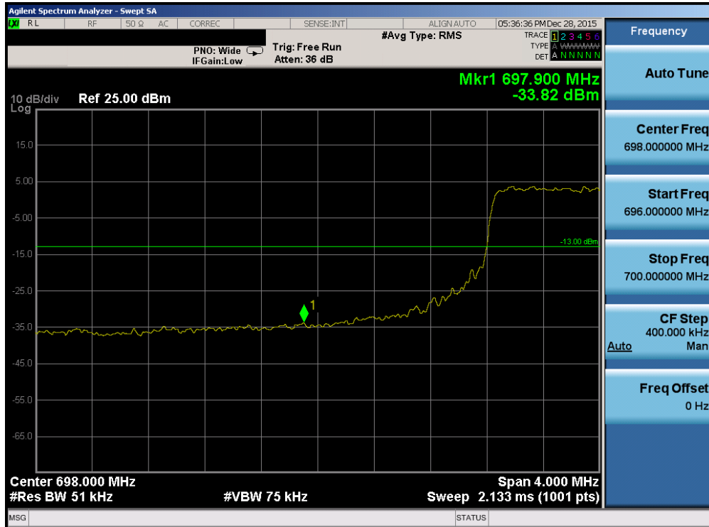
Plot 7-134. Lower Band Edge Plot (Band 12/17 – 5.0MHz QPSK – RB Size 25)
