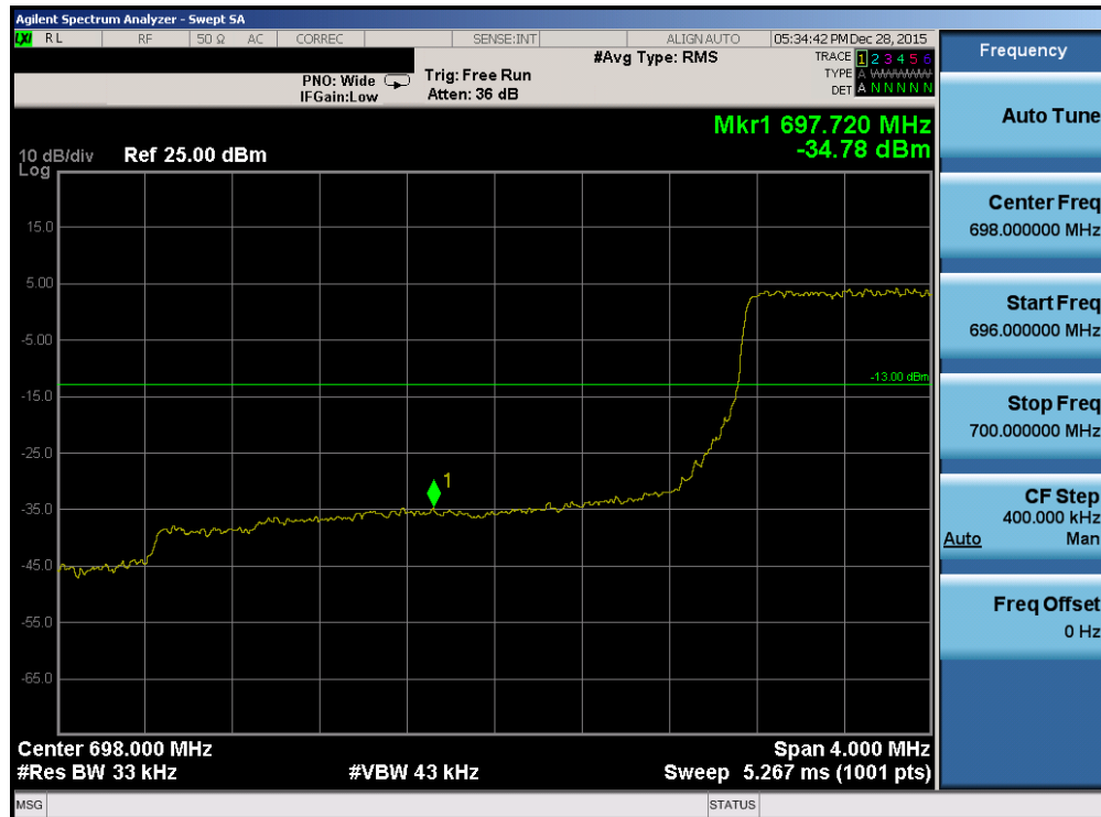
Plot 7-130. Lower Band Edge Plot (Band 12 – 3.0MHz QPSK – RB Size 15)
