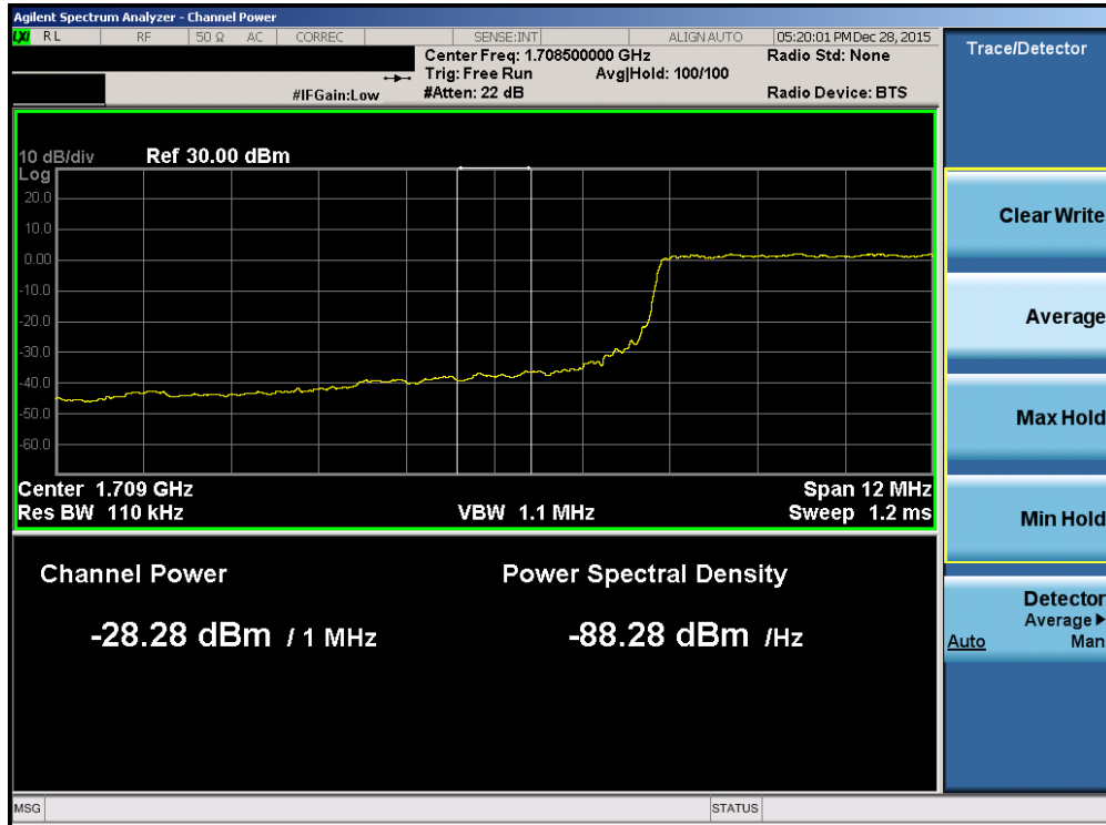
Plot 7-199. Lower Extended Band Edge Plot (Band 4 – 15.0MHz QPSK – RB Size 75)
