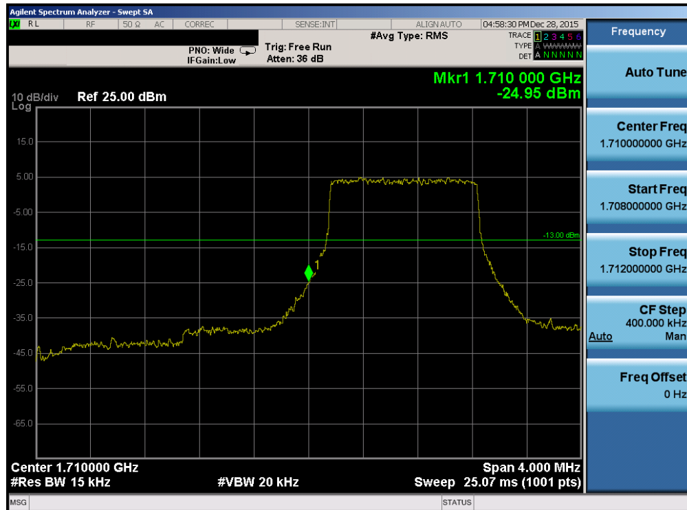
Plot 7-182. Lower Band Edge Plot (Band 4 – 1.4MHz QPSK – RB Size 6)
