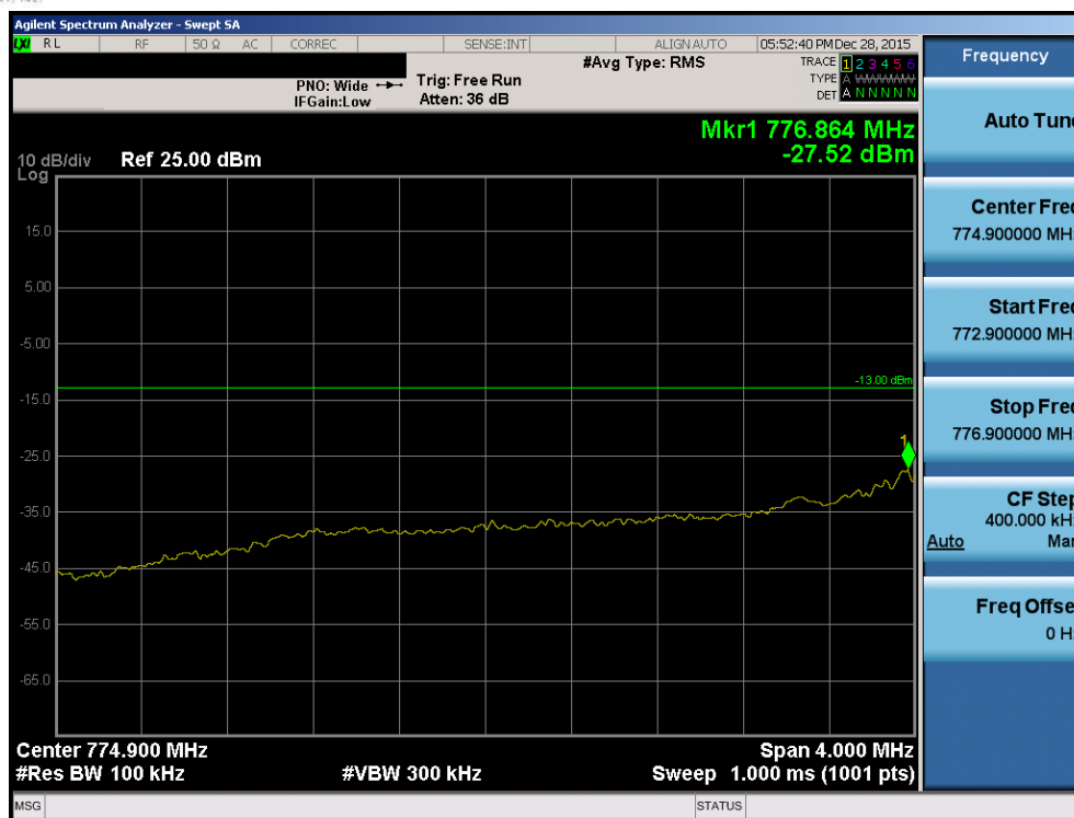
Plot 7-143. Lower Extended Band Edge Plot (Band 13 – 5.0MHz QPSK – RB Size 25)
