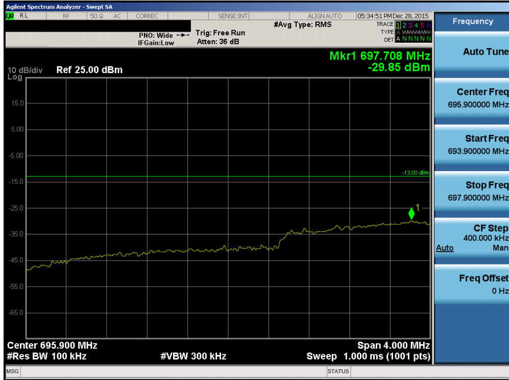
Plot 7-131. Lower Extended Band Edge Plot (Band 12 – 3.0MHz QPSK – RB Size 15)
