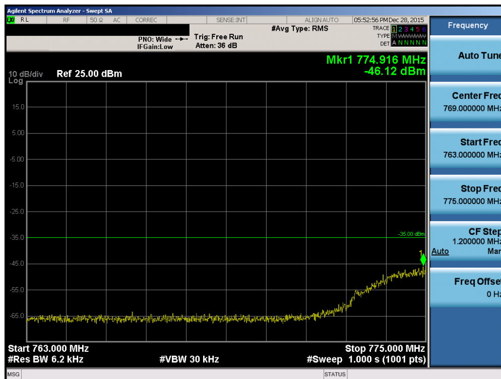
Plot 7-144. Lower Emission Mask Edge Plot (Band 13 – 5.0MHz QPSK – RB Size 25)
