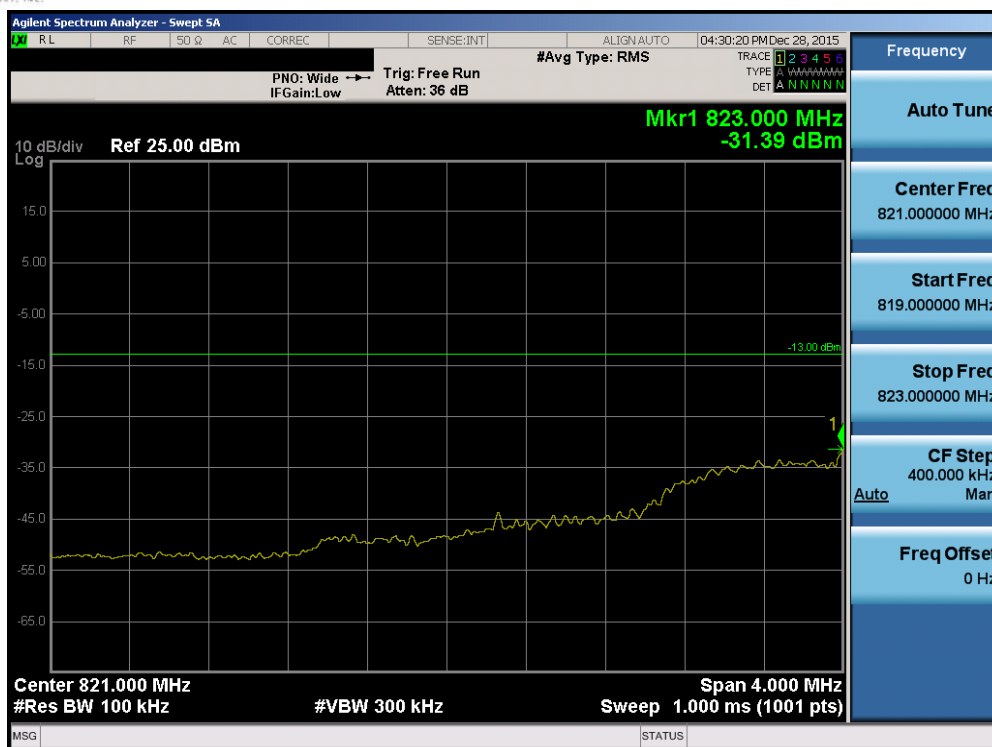
Plot 7-153. Lower Extended Band Edge Plot (Band 5 - 1.4MHz QPSK - RB Size 6)
