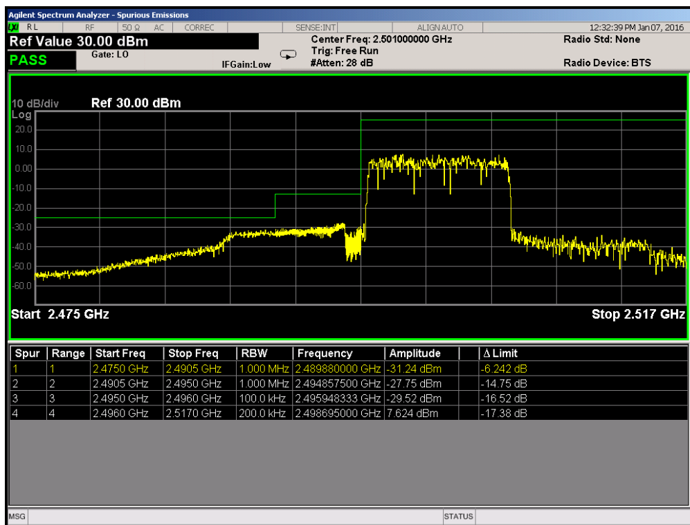
Plot 7-232. Lower ACP Plot (Band 41 – 10.0MHz QPSK – RB Size 50)
