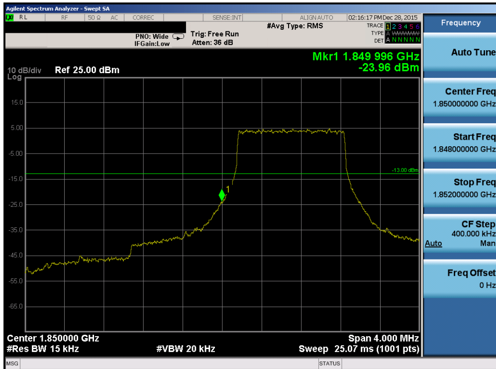
Plot 7-206. Lower Band Edge Plot (Band 2/25 – 1.4MHz QPSK – RB Size 6)
