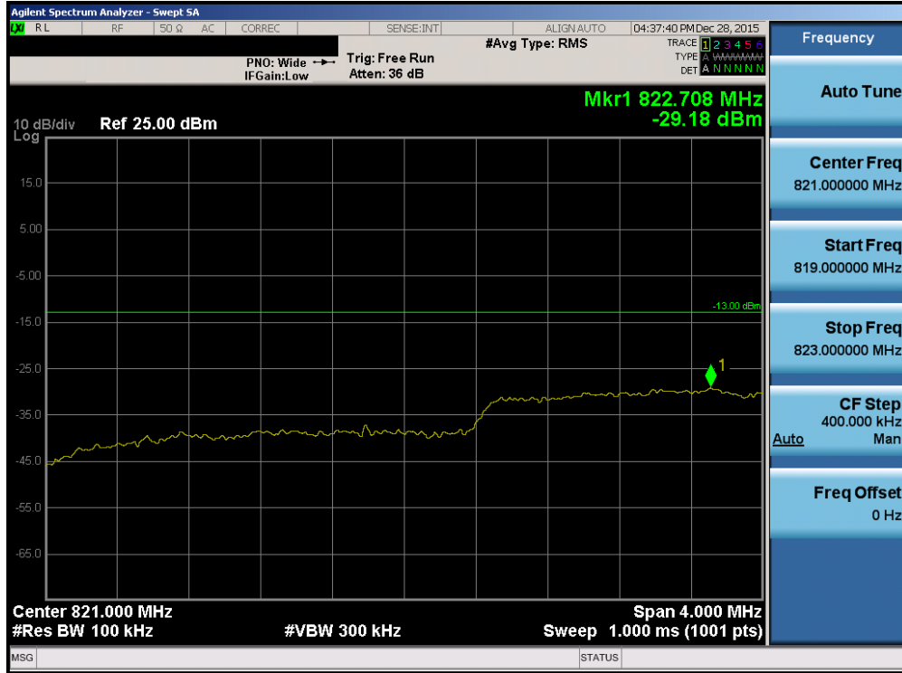
Plot 7-157. Lower Extended Band Edge Plot (Band 5 – 3.0MHz QPSK – RB Size 15)
