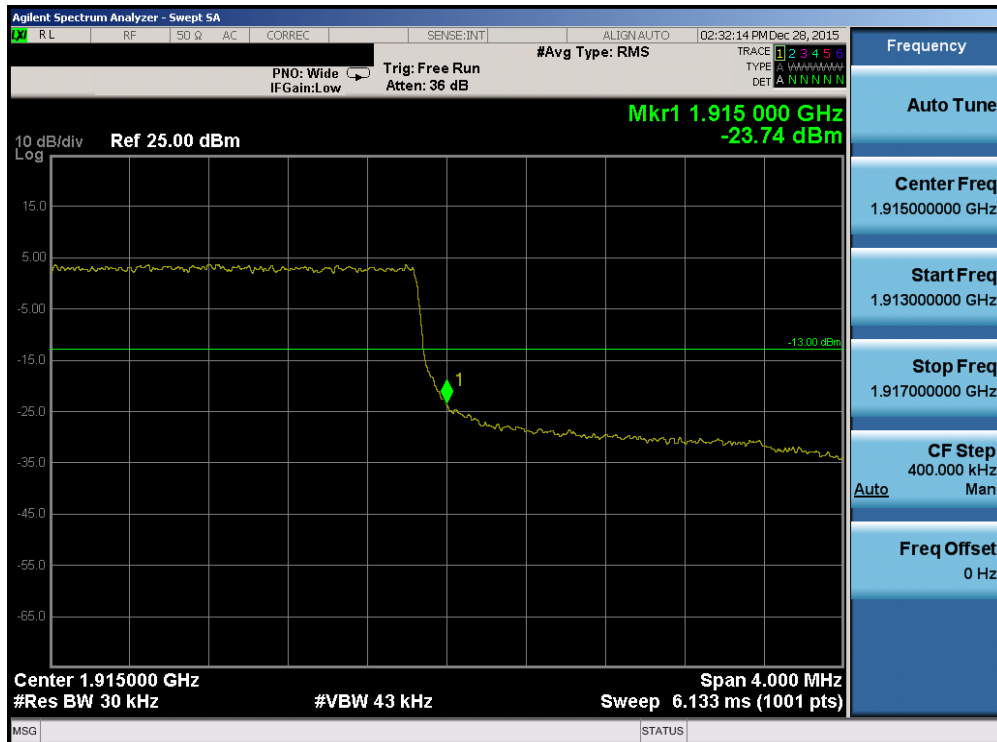
Plot 7-212. Upper Band Edge Plot (Band 2/25 – 3.0MHz QPSK – RB Size 15)
