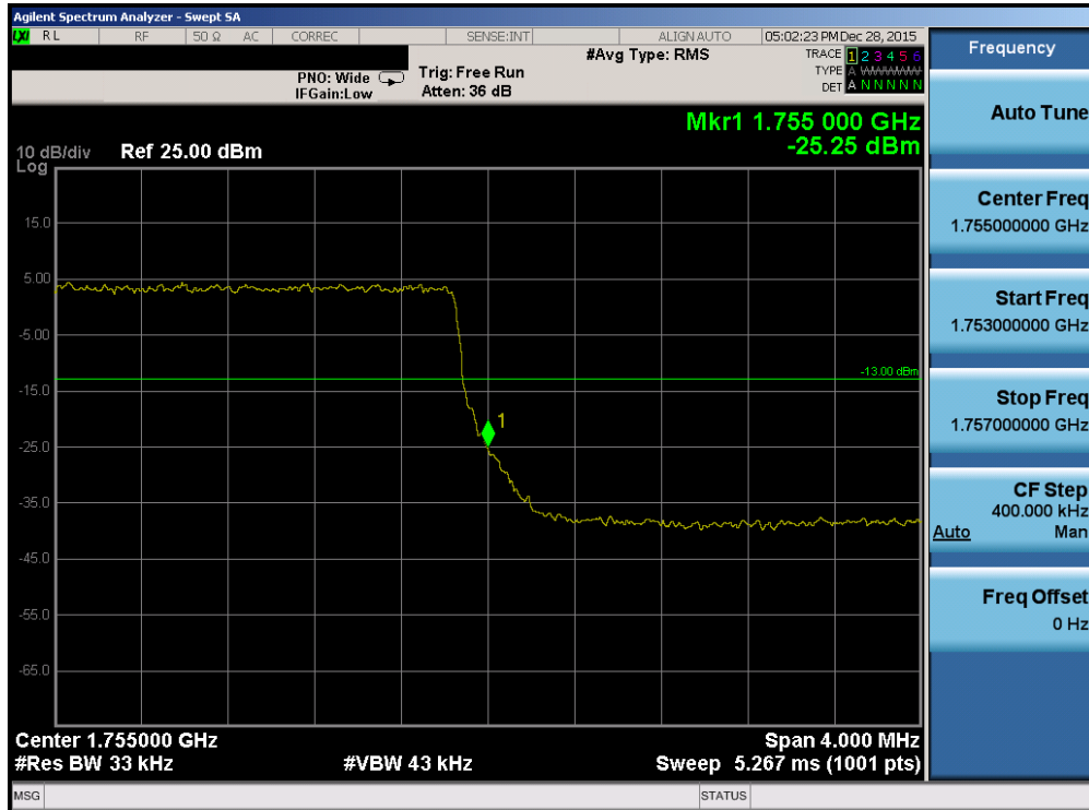
Plot 7-188. Upper Band Edge Plot (Band 4 – 3.0MHz QPSK – RB Size 15)
