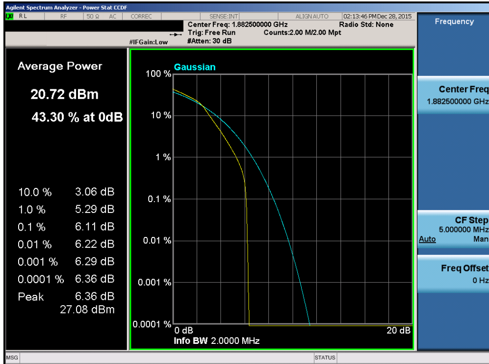
Plot 7-239. PAR Plot (Band 2/25 – 1.4MHz 16-QAM – RB Size 6)
