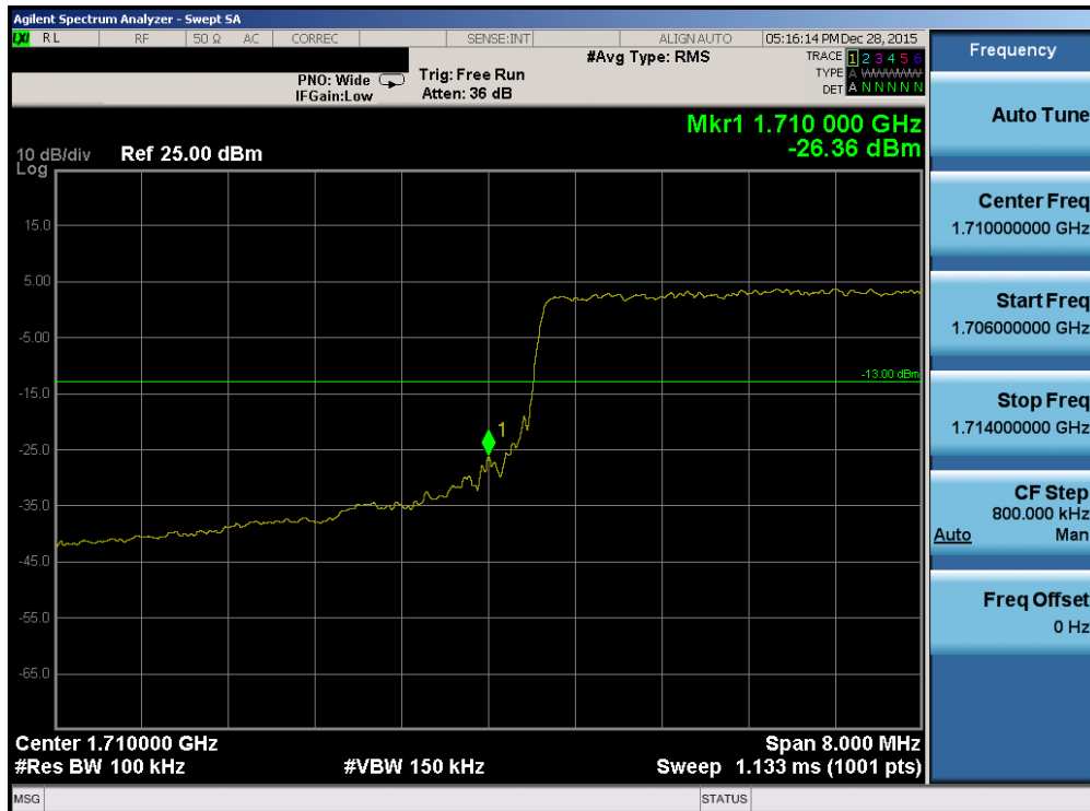
Plot 7-194. Lower Band Edge Plot (Band 4 – 10.0MHz QPSK – RB Size 50)
