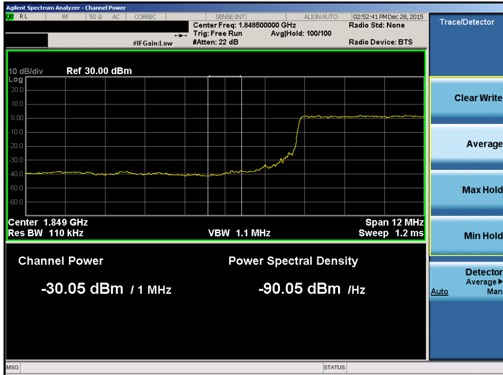
Plot 7-223. Lower Extended Band Edge Plot (Band 2/25 – 15.0MHz QPSK – RB Size 75)
