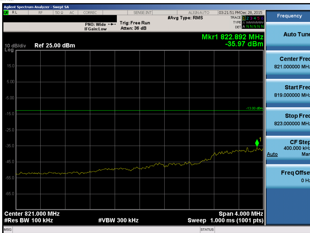
Plot 7-167. Lower Extended Band Edge Plot (Band 26 – 1.4MHz QPSK – RB Size 6)
