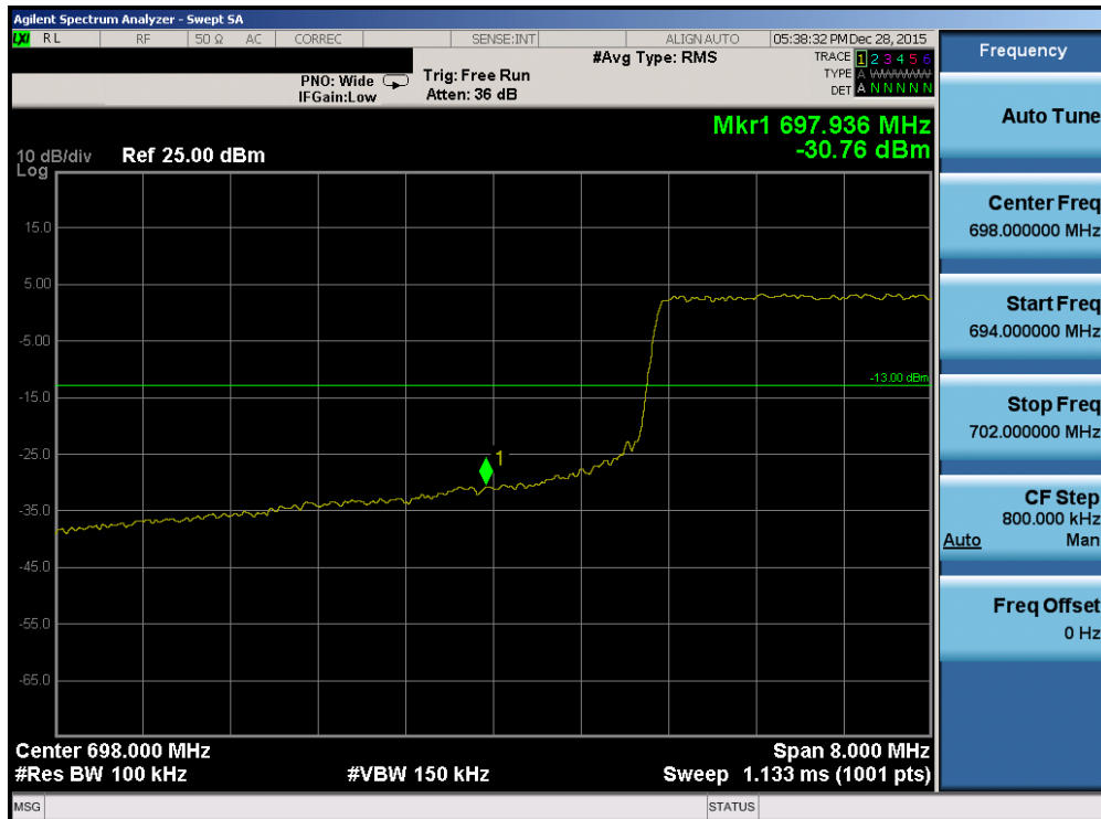
Plot 7-138. Lower Band Edge Plot (Band 12/17 – 10.0MHz QPSK – RB Size 50)
