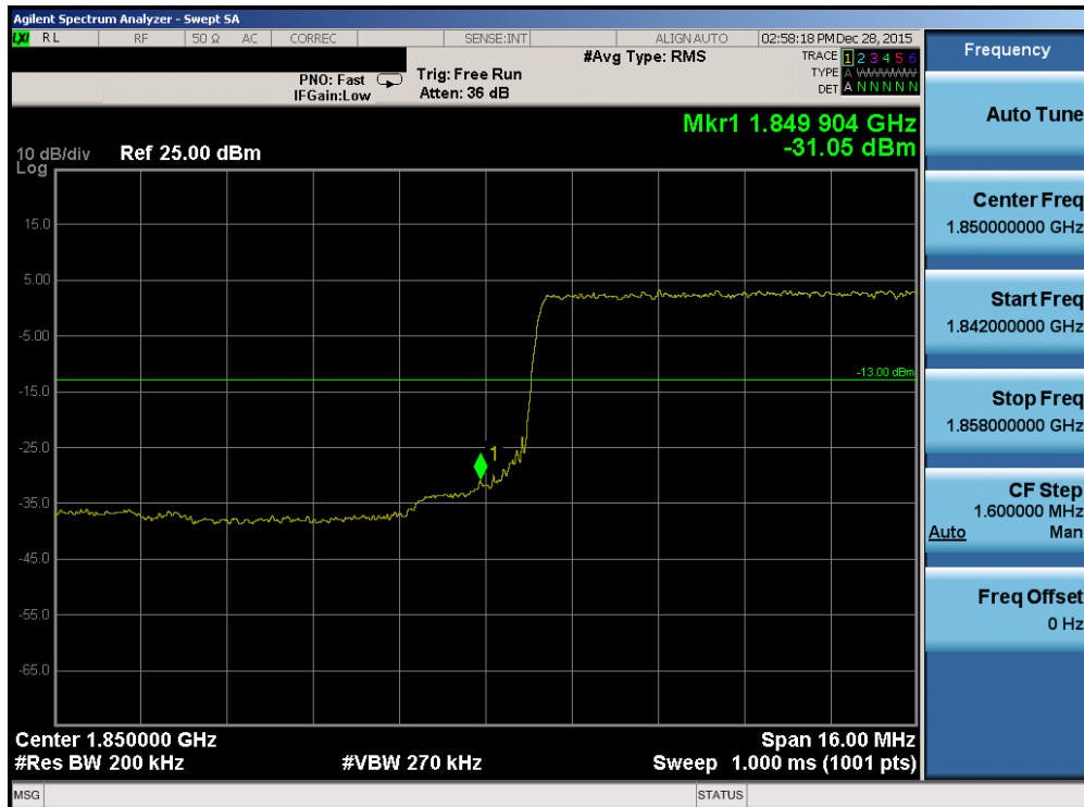
Plot 7-226. Lower Band Edge Plot (Band 2/25 – 20.0MHz QPSK – RB Size 100)
