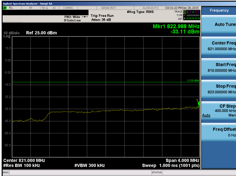
Plot 7-175. Lower Extended Band Edge Plot (Band 26 – 5.0MHz QPSK – RB Size 25)
