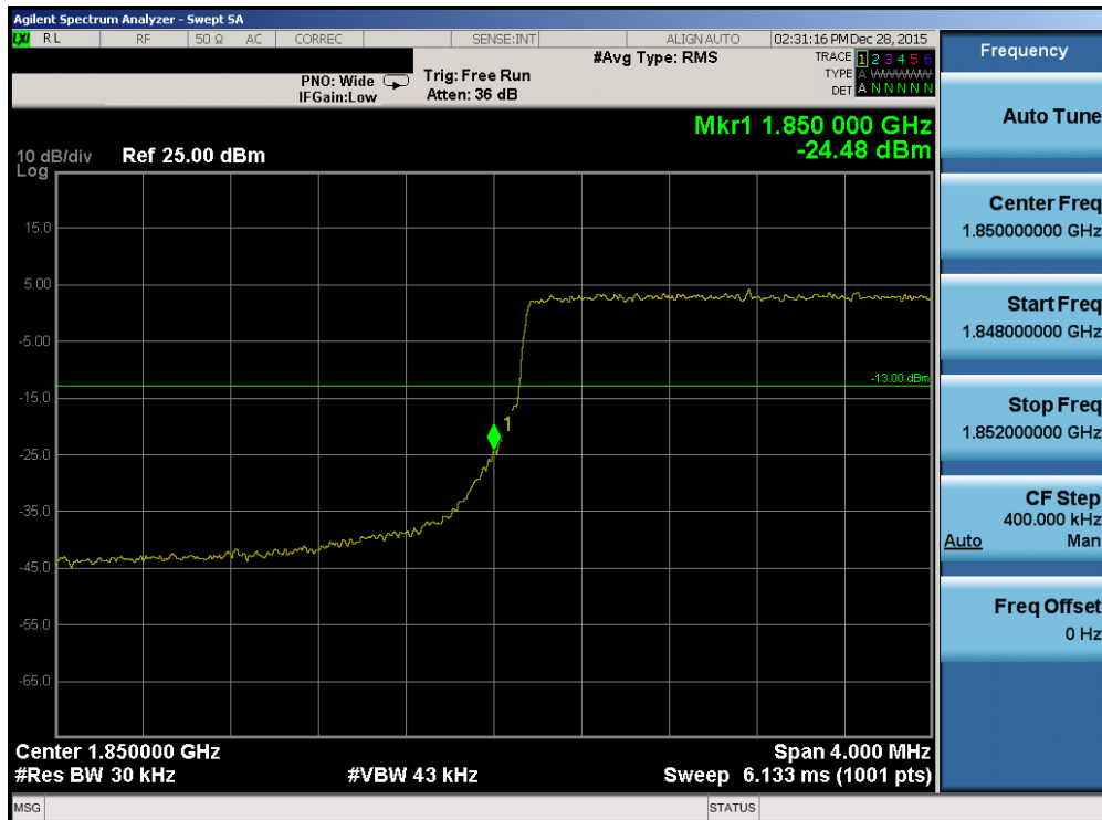
Plot 7-210. Lower Band Edge Plot (Band 2/25 – 3.0MHz QPSK – RB Size 15)
