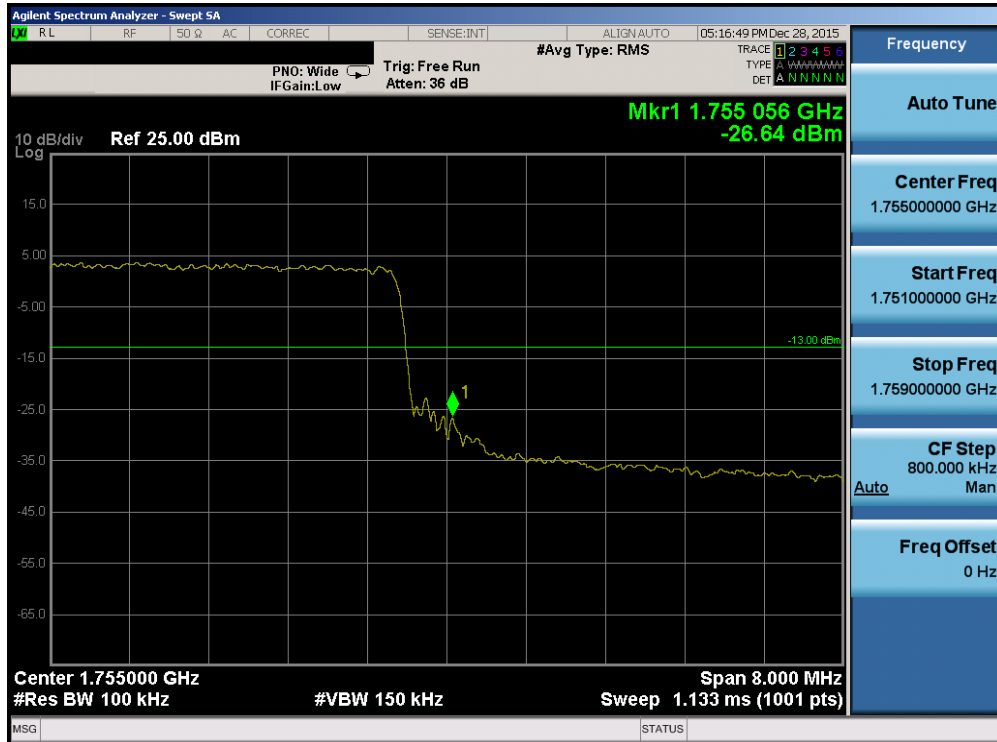
Plot 7-196. Upper Band Edge Plot (Band 4 – 10.0MHz QPSK – RB Size 50)
