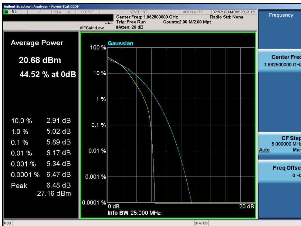
Plot 7-249. PAR Plot (Band 2/25 – 20.0MHz 16-QAM – RB Size 100)
