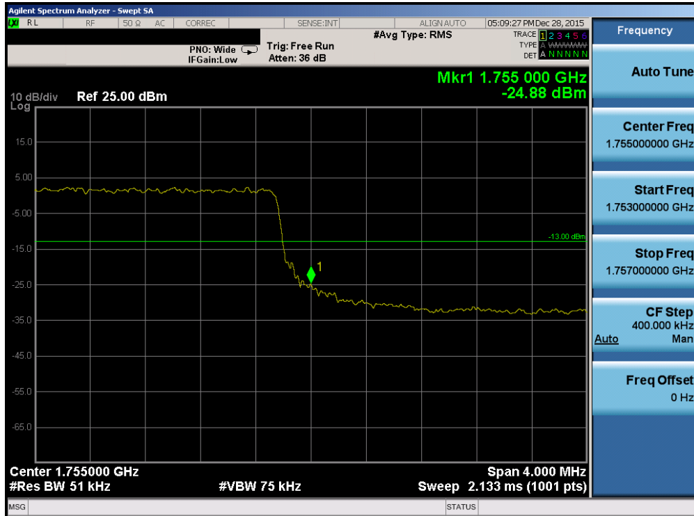
Plot 7-192. Upper Band Edge Plot (Band 4 – 5.0MHz QPSK – RB Size 25)
