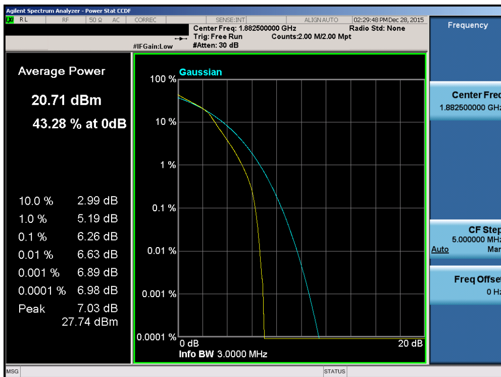
Plot 7-241. PAR Plot (Band 2/25 – 3.0MHz 16-QAM – RB Size 15)
