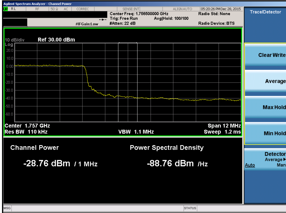
Plot 7-201. Upper Extended Band Edge Plot (Band 4 – 15.0MHz QPSK – RB Size 75)
