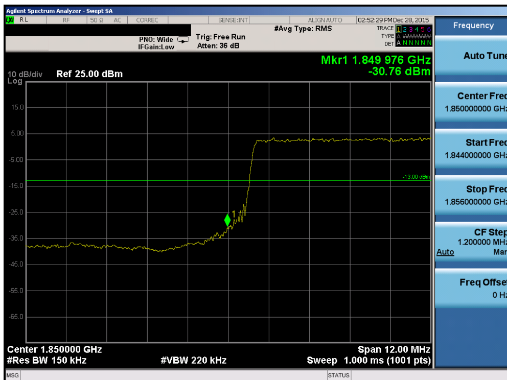
Plot 7-222. Lower Band Edge Plot (Band 2/25 – 15.0MHz QPSK – RB Size 75)
