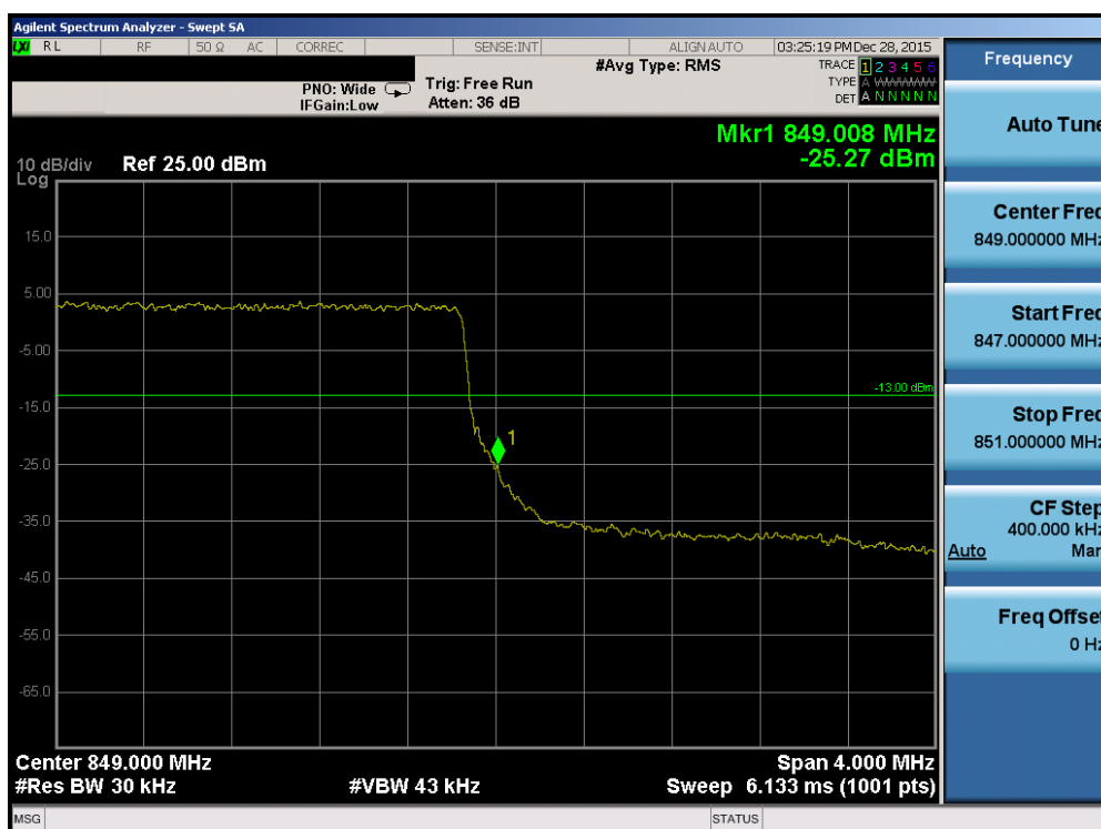
Plot 7-172. Upper Band Edge Plot (Band 26 – 3.0MHz QPSK – RB Size 15)
