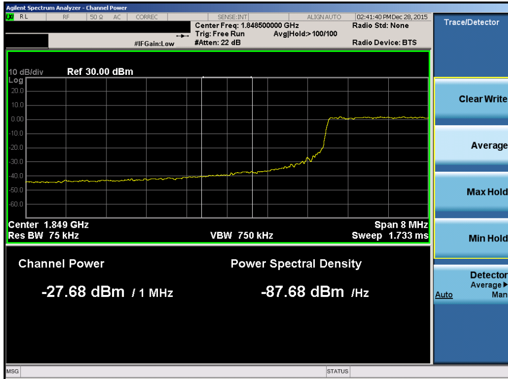
Plot 7-219. Lower Extended Band Edge Plot (Band 2/25 – 10.0MHz QPSK – RB Size 50)
