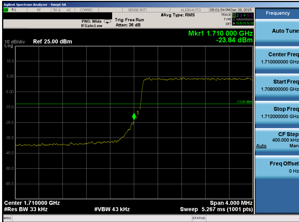
Plot 7-186. Lower Band Edge Plot (Band 4 – 3.0MHz QPSK – RB Size 15)
