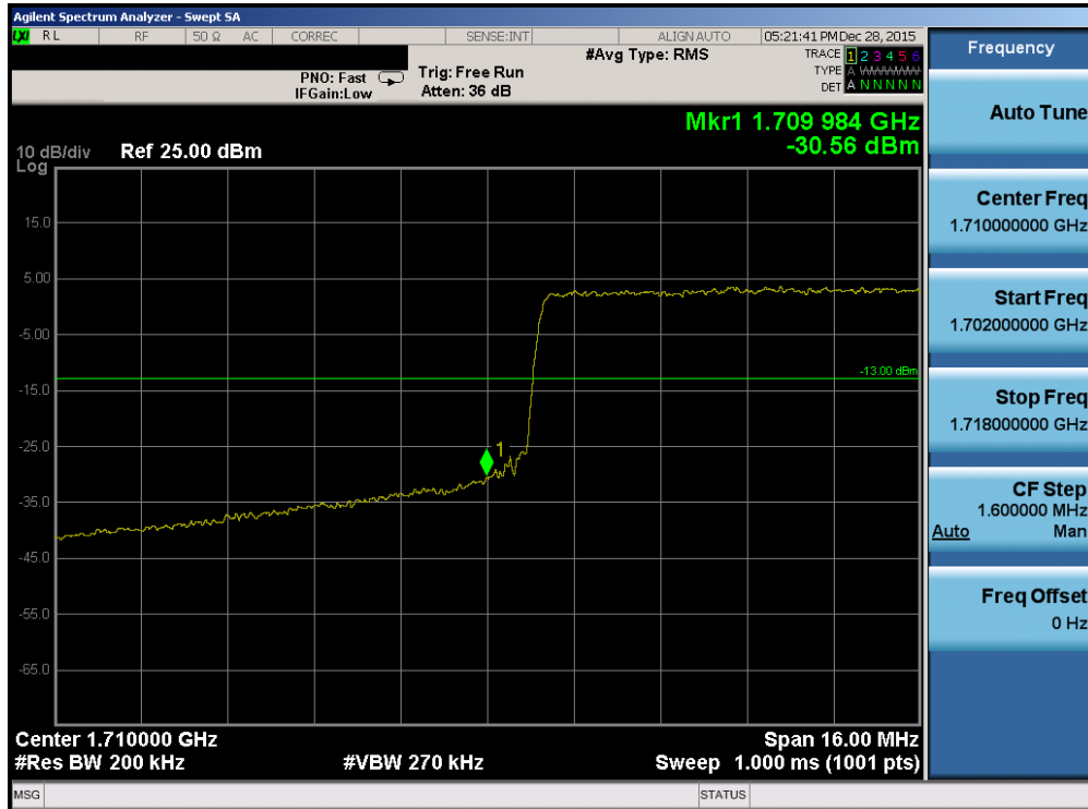
Plot 7-202. Lower Band Edge Plot (Band 4 – 20.0MHz QPSK – RB Size 100)
