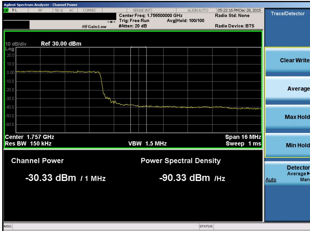
Plot 7-205. Upper Extended Band Edge Plot (Band 4 – 20.0MHz QPSK – RB Size 100)
