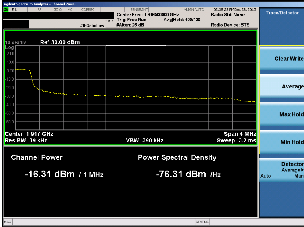
Plot 7-217. Upper Extended Band Edge Plot (Band 2/25 – 5.0MHz QPSK – RB Size 25)
