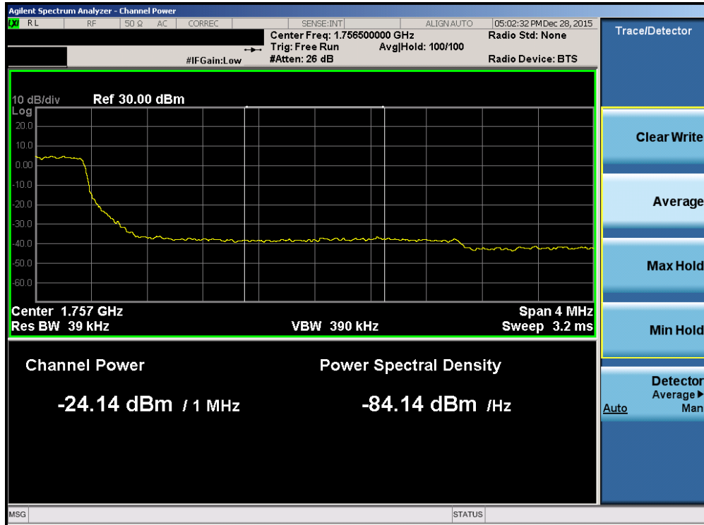
Plot 7-189. Upper Extended Band Edge Plot (Band 4 – 3.0MHz QPSK – RB Size 15)
