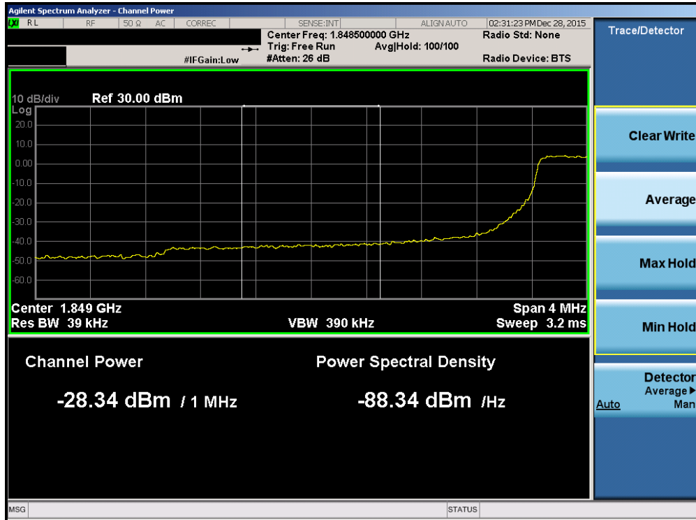
Plot 7-211. Lower Extended Band Edge Plot (Band 2/25 – 3.0MHz QPSK – RB Size 15)
