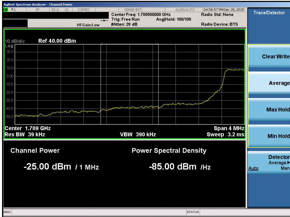
Plot 7-183. Lower Extended Band Edge Plot (Band 4 – 1.4MHz QPSK – RB Size 6)
