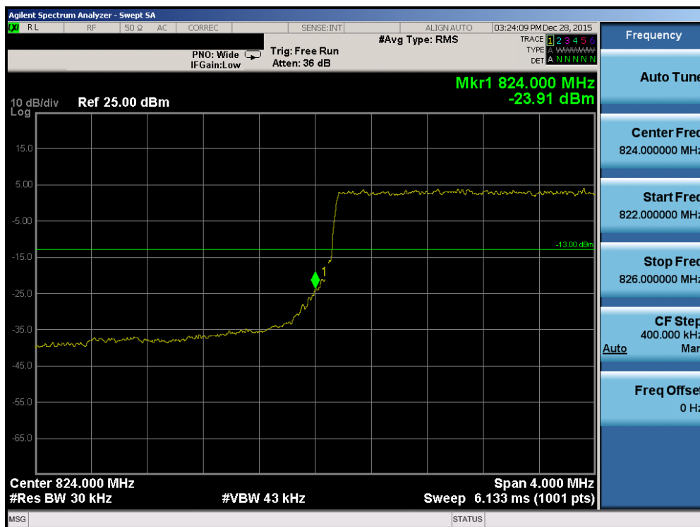
Plot 7-170. Lower Band Edge Plot (Band 26 – 3.0MHz QPSK – RB Size 15)
