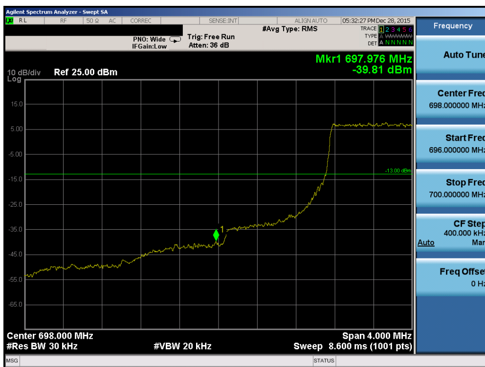
Plot 7-126. Lower Band Edge Plot (Band 12 – 1.4MHz QPSK – RB Size 6)
