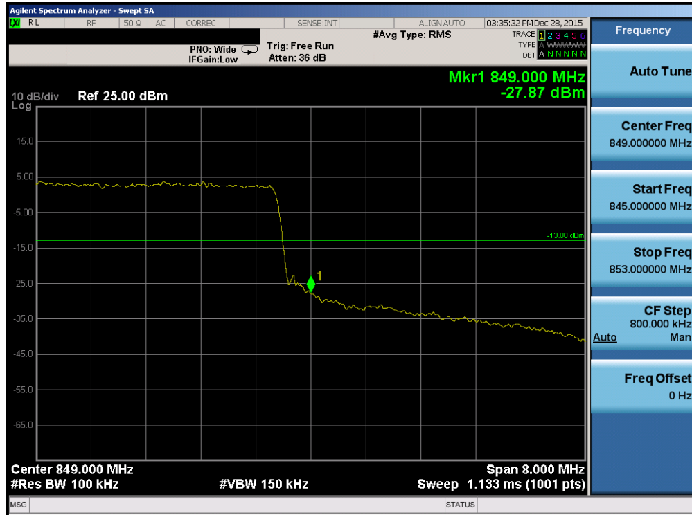
Plot 7-179. Upper Band Edge Plot (Band 26 – 10.0MHz QPSK – RB Size 50)
