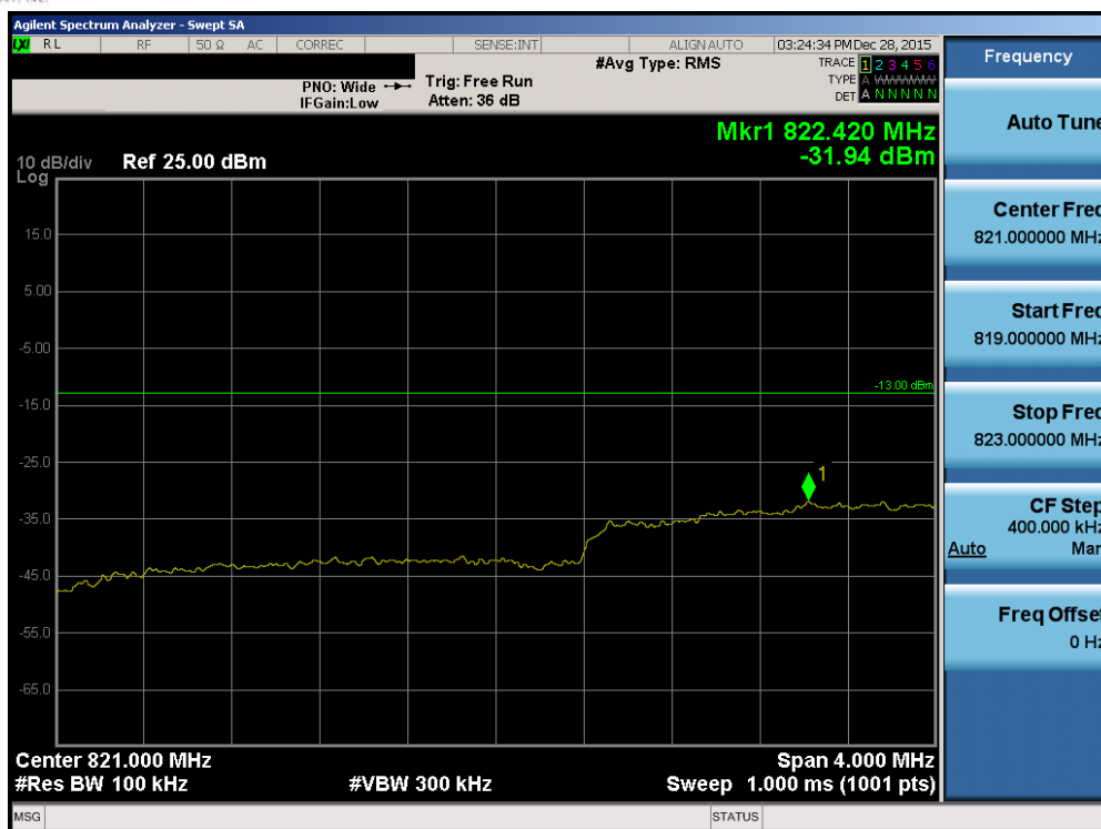
Plot 7-171. Lower Extended Band Edge Plot (Band 26 – 3.0MHz QPSK – RB Size 15)
