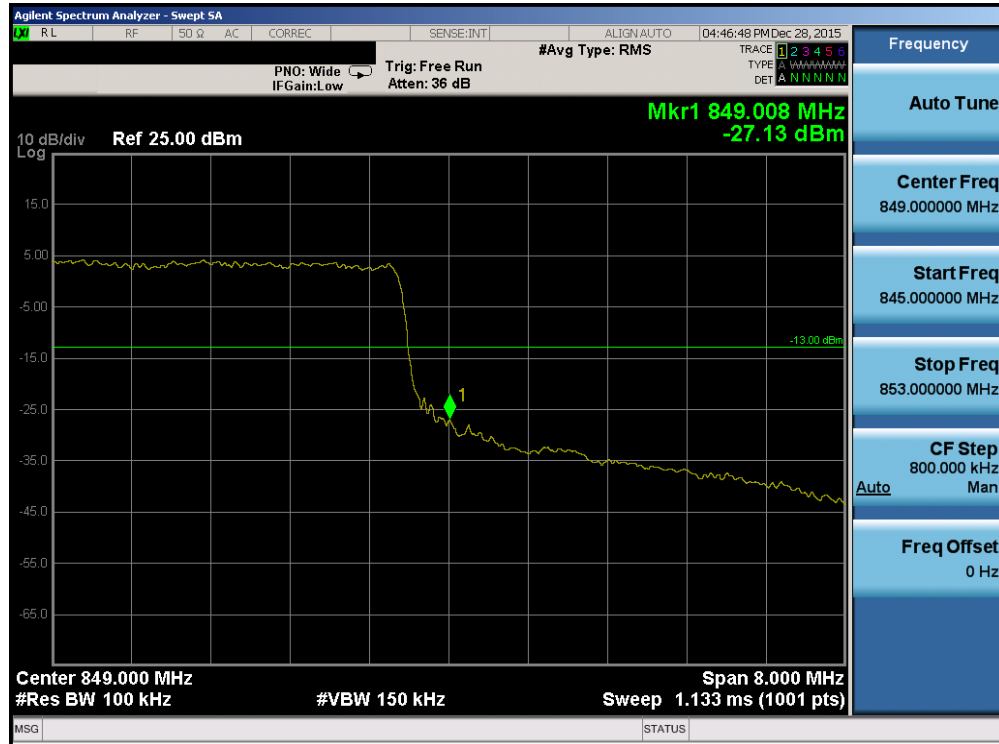
Plot 7-165. Upper Band Edge Plot (Band 5 – 10.0MHz QPSK – RB Size 50)
