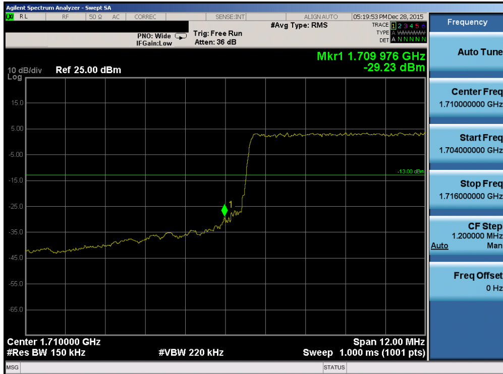
Plot 7-198. Lower Band Edge Plot (Band 4 – 15.0MHz QPSK – RB Size 75)
