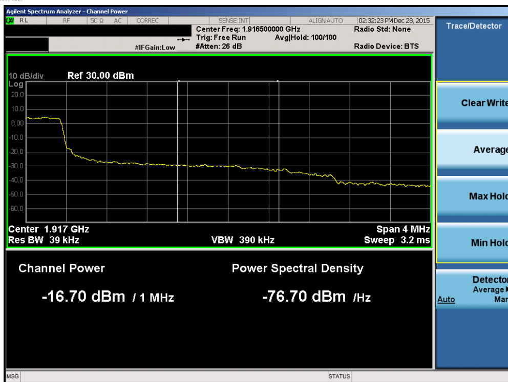
Plot 7-213. Upper Extended Band Edge Plot (Band 2/25 – 3.0MHz QPSK – RB Size 15)
