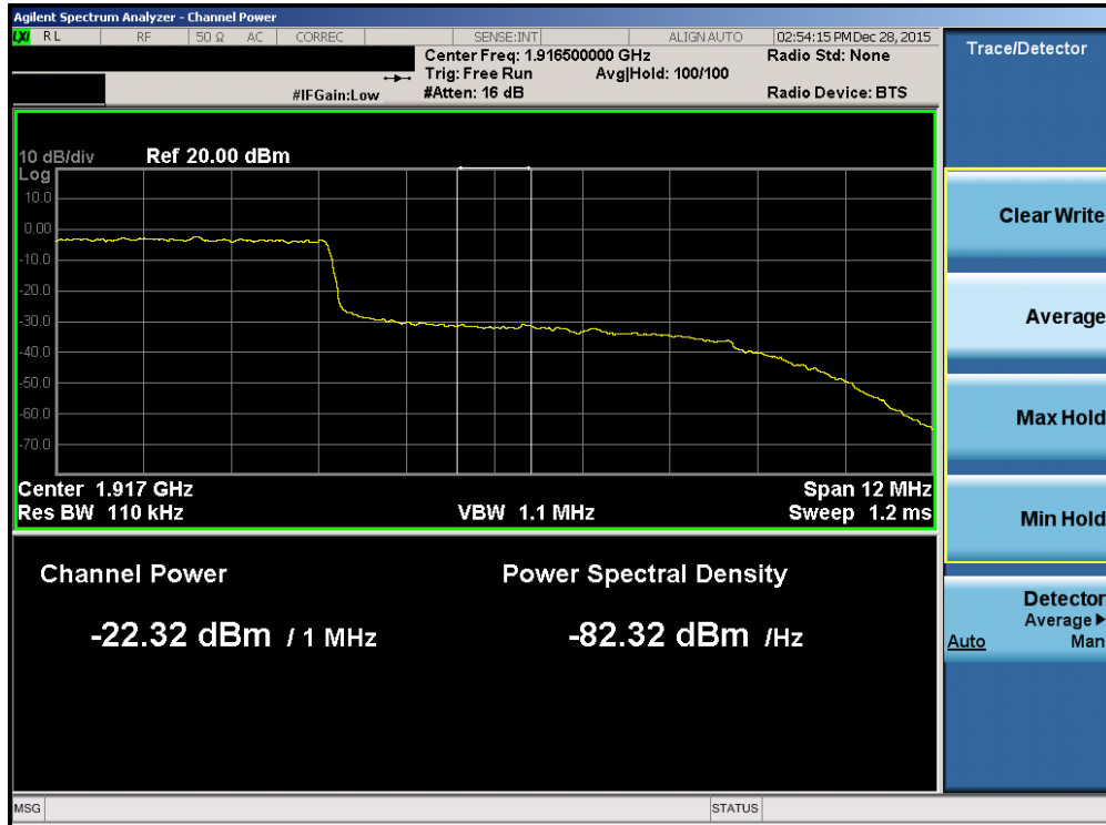
Plot 7-225. Upper Extended Band Edge Plot (Band 2/25 – 15.0MHz QPSK – RB Size 75)
