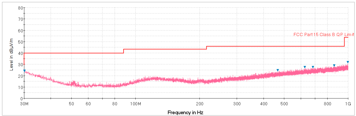
Plot 7-136. Radiated Spurious Plot below 1GHz (Pol. V)
