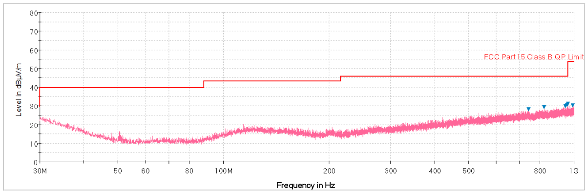
Plot 7-138. Radiated Spurious Plot below 1GHz (Pol. V)
