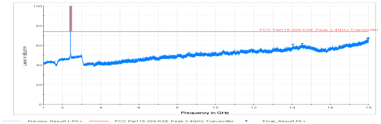
Plot 7-74. Radiated Spurious Plot above 1GHz (802.11b – Ch. 1, Ant. Pol. V)
