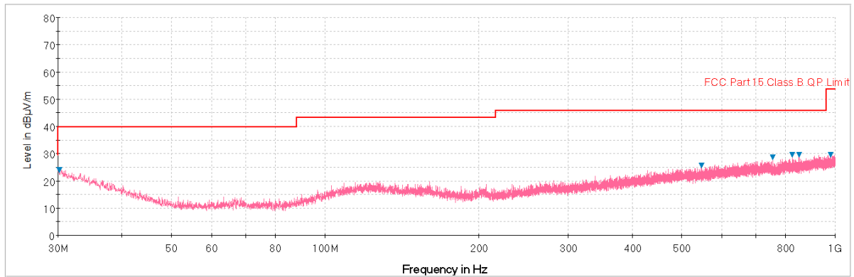
Plot 7-135. Radiated Spurious Plot below 1GHz (Pol. H)
