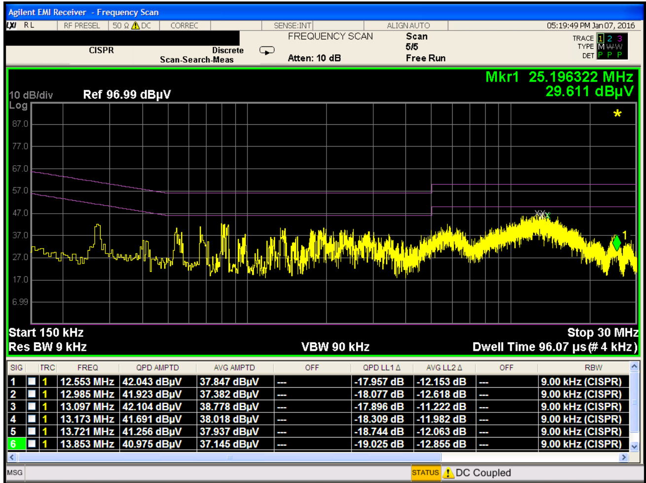
Plot 7-139. Line Conducted Plot with 802.11b (L1)
