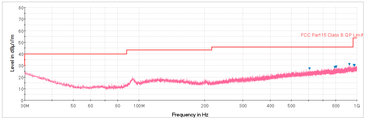
Plot 7-137. Radiated Spurious Plot below 1GHz (Pol. H)
