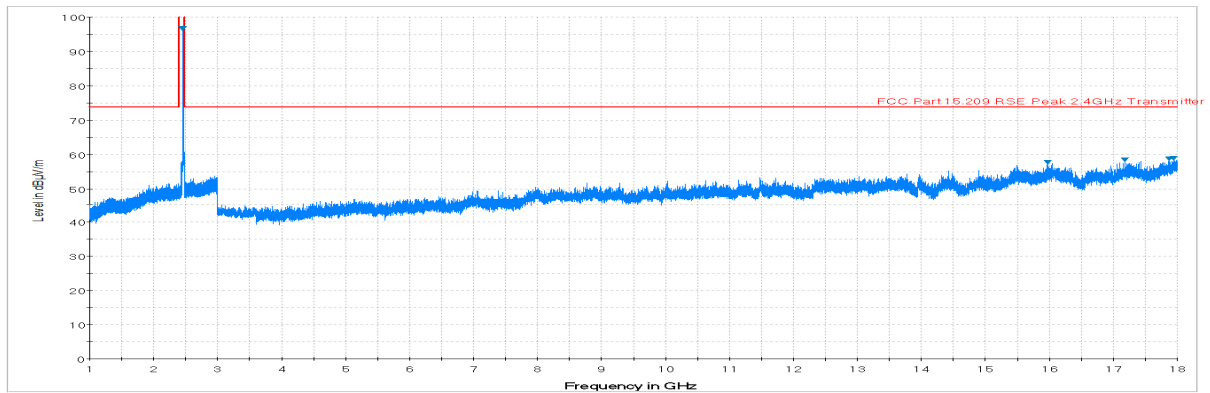
Plot 7-86. Radiated Spurious Plot above 1GHz (802.11b – Ch. 11, Ant. Pol. V)
