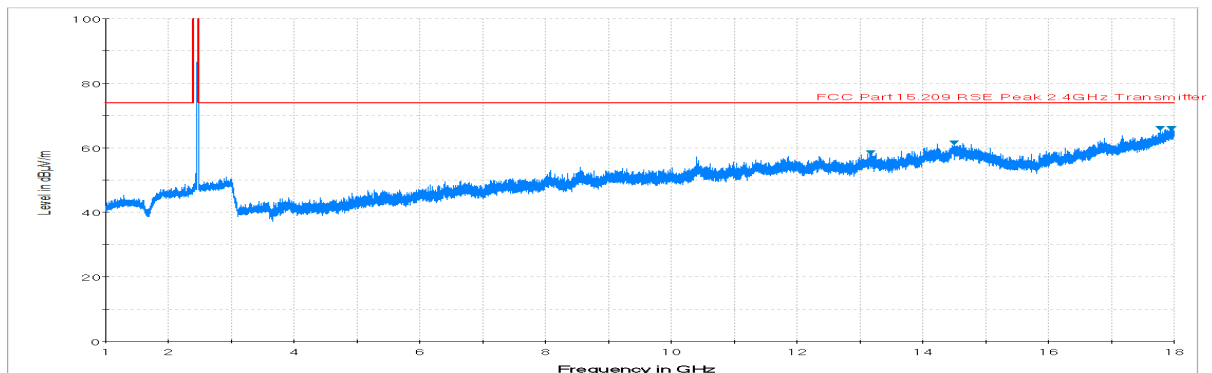
Plot 7-77. Radiated Spurious Plot above 1GHz (802.11b – Ch. 11, Ant. Pol. H)
