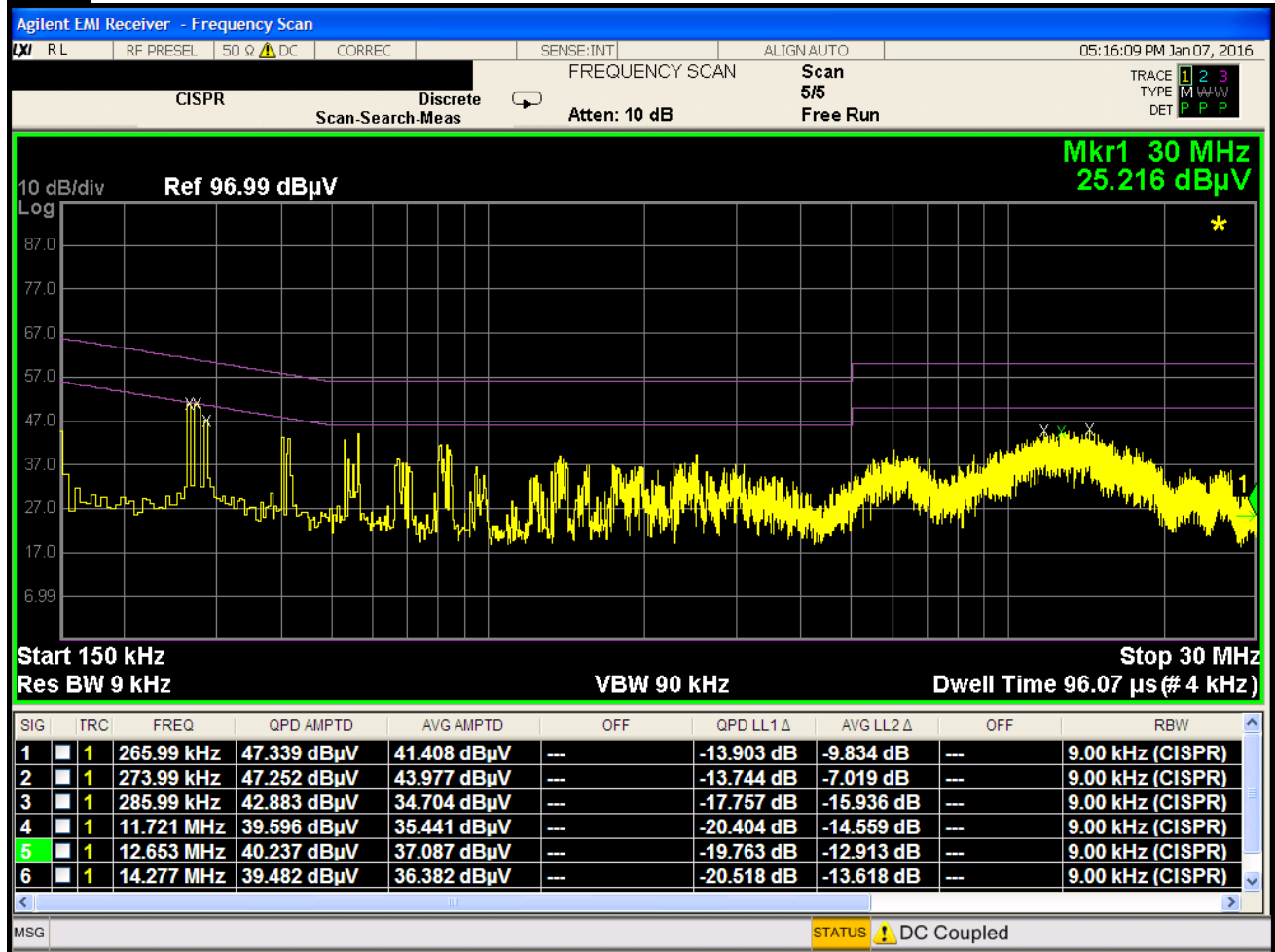
Plot 7-140. Line Conducted Plot with 802.11b (N)
