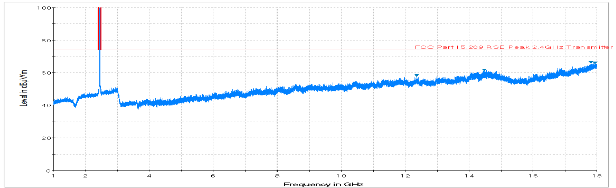
Plot 7-76. Radiated Spurious Plot above 1GHz (802.11b – Ch. 6, Ant. Pol. V)
