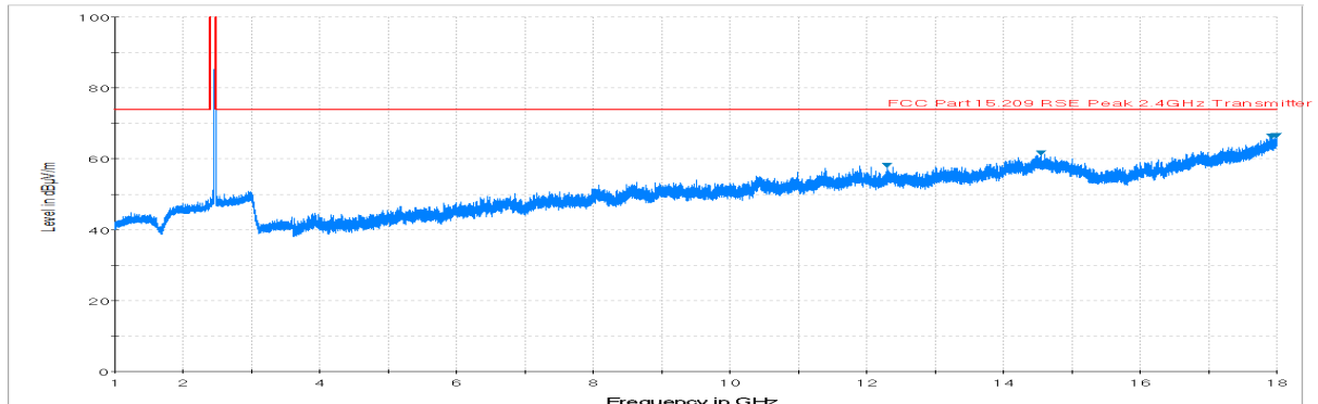
Plot 7-78. Radiated Spurious Plot above 1GHz (802.11b – Ch. 11, Ant. Pol. V)
