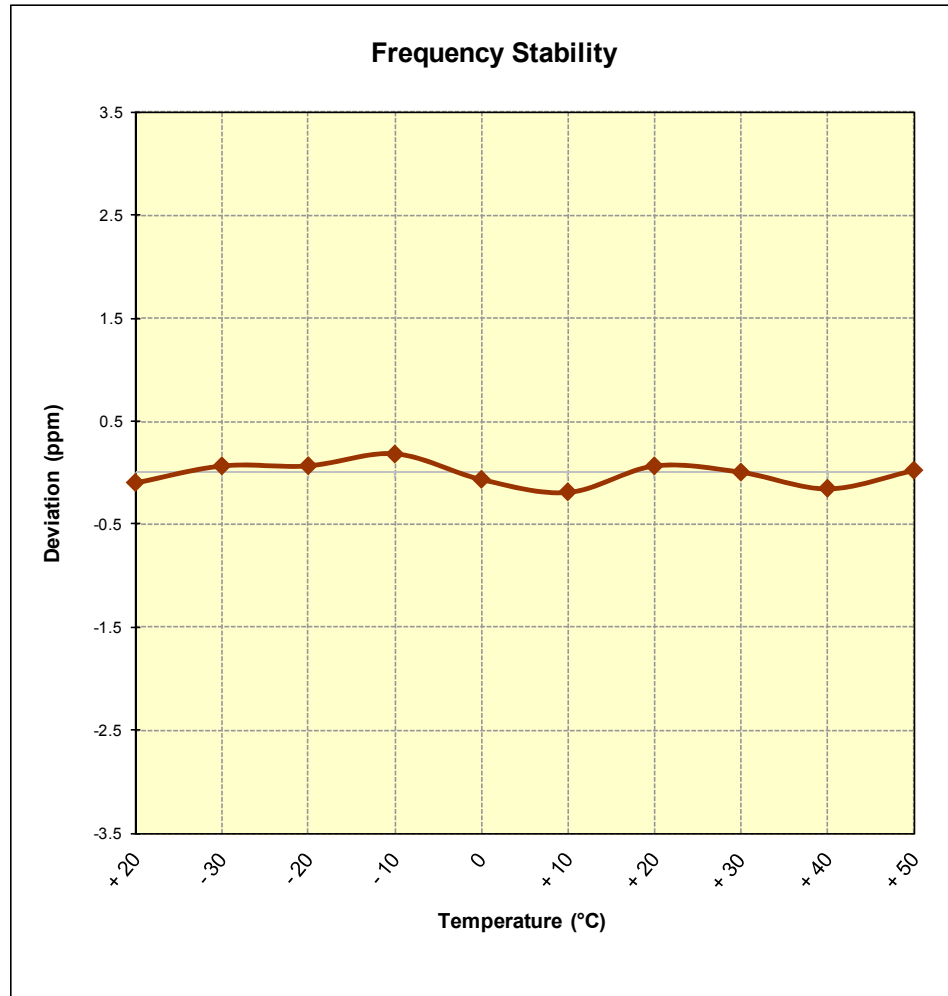
Figure 7-9. Frequency Stability Graph (PCS GPRS Mode – Ch. 661)
