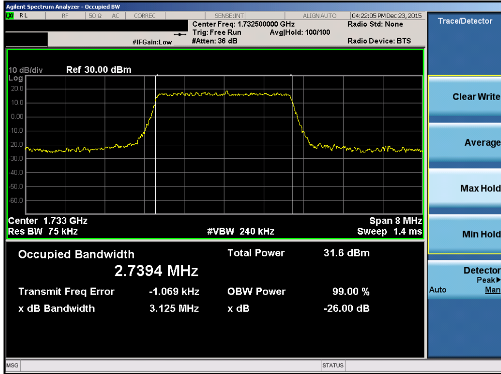
Plot 7-29. Occupied Bandwidth Plot (Band 4 – 3.0MHz QPSK – RB Size 15)
