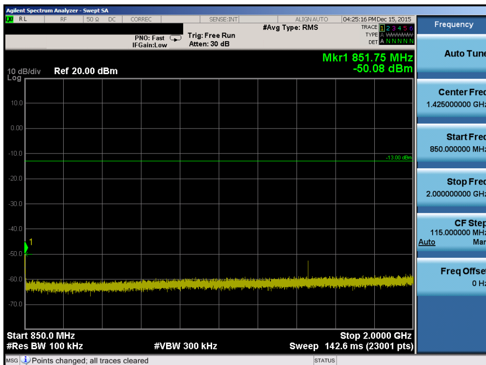
Plot 7-84. Conducted Spurious Plot (Band 26 – 10.0MHz QPSK – RB Size 1, RB Offset 0 – High Channel)
