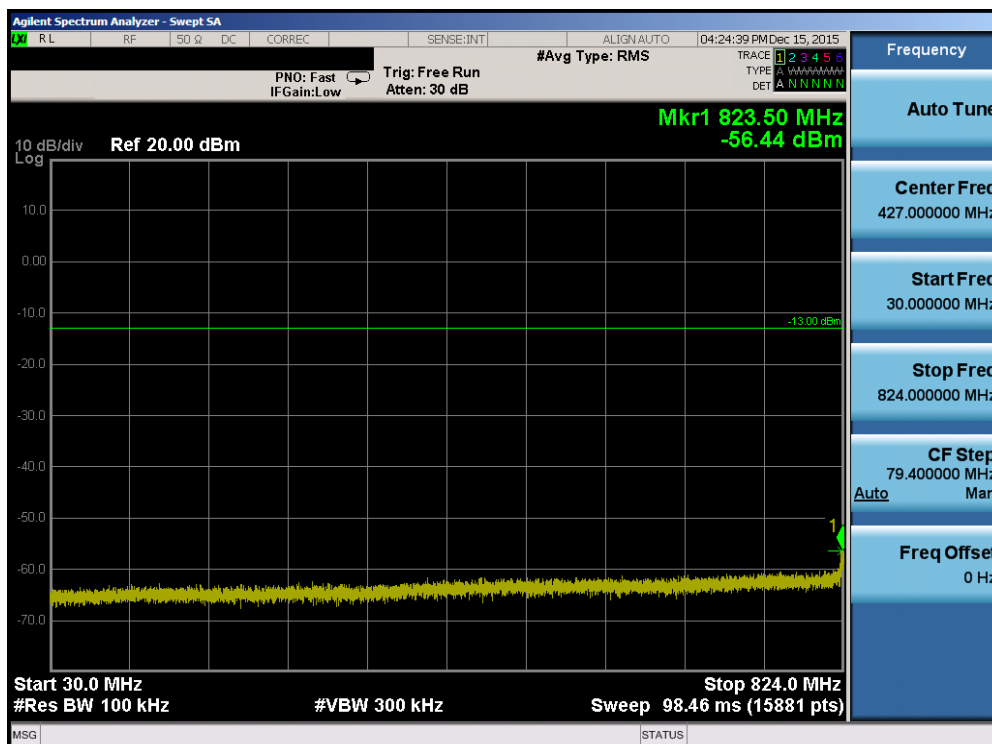
Plot 7-80. Conducted Spurious Plot (Band 26 – 10.0MHz QPSK – RB Size 1, RB Offset 0 – Mid Channel)
