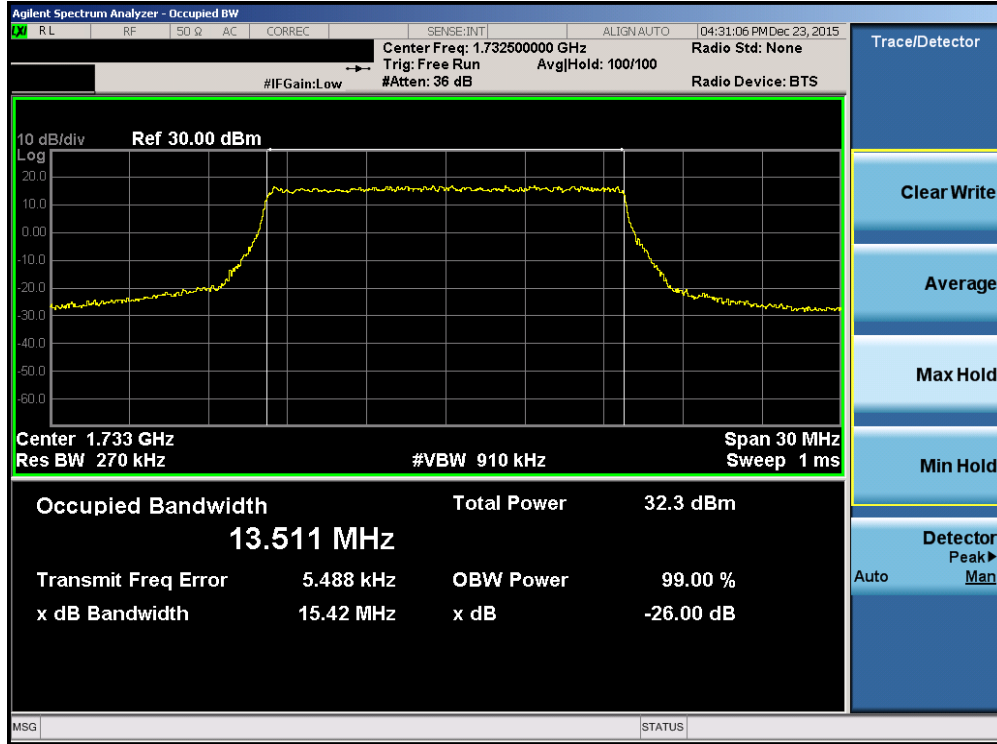
Plot 7-35. Occupied Bandwidth Plot (Band 4 – 15.0MHz QPSK – RB Size 75)
