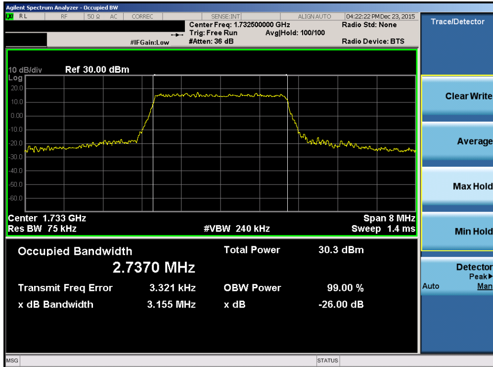
Plot 7-30. Occupied Bandwidth Plot (Band 4 – 3.0MHz 16-QAM – RB Size 15)
