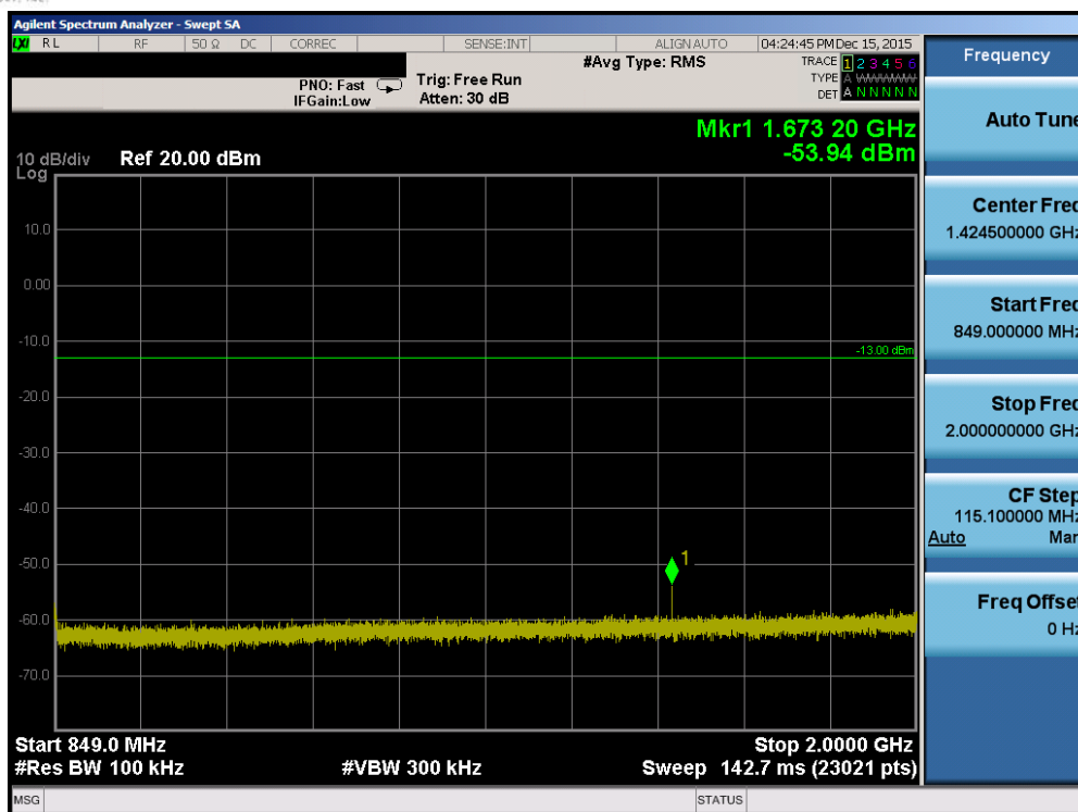
Plot 7-81. Conducted Spurious Plot (Band 26 – 10.0MHz QPSK – RB Size 1, RB Offset 0 – Mid Channel)
