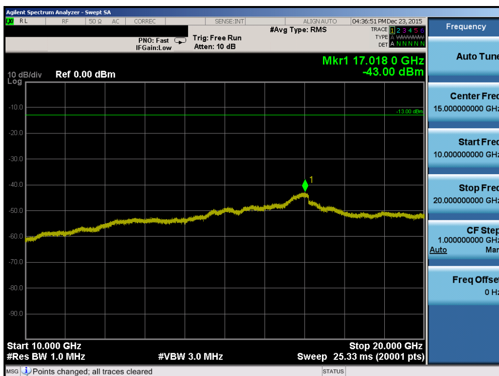
Plot 7-88. Conducted Spurious Plot (Band 4 – 20.0MHz QPSK – RB Size 1, RB Offset 0 – Low Channel)
