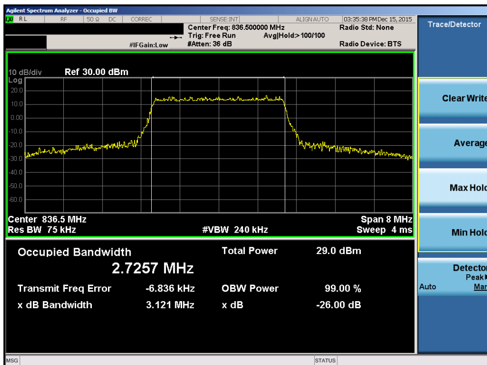
Plot 7-20. Occupied Bandwidth Plot (Band 26 – 3.0MHz 16-QAM – RB Size 15)
