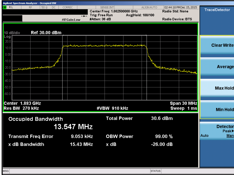
Plot 7-47. Occupied Bandwidth Plot (Band2/25 – 15.0MHz QPSK – RB Size 75)
