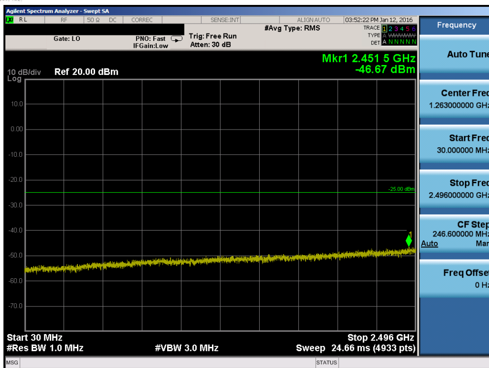
Plot 7-107. Conducted Spurious Plot (Band 41 – 20.0MHz QPSK – RB Size 1, RB Offset 0 – Mid Channel)
