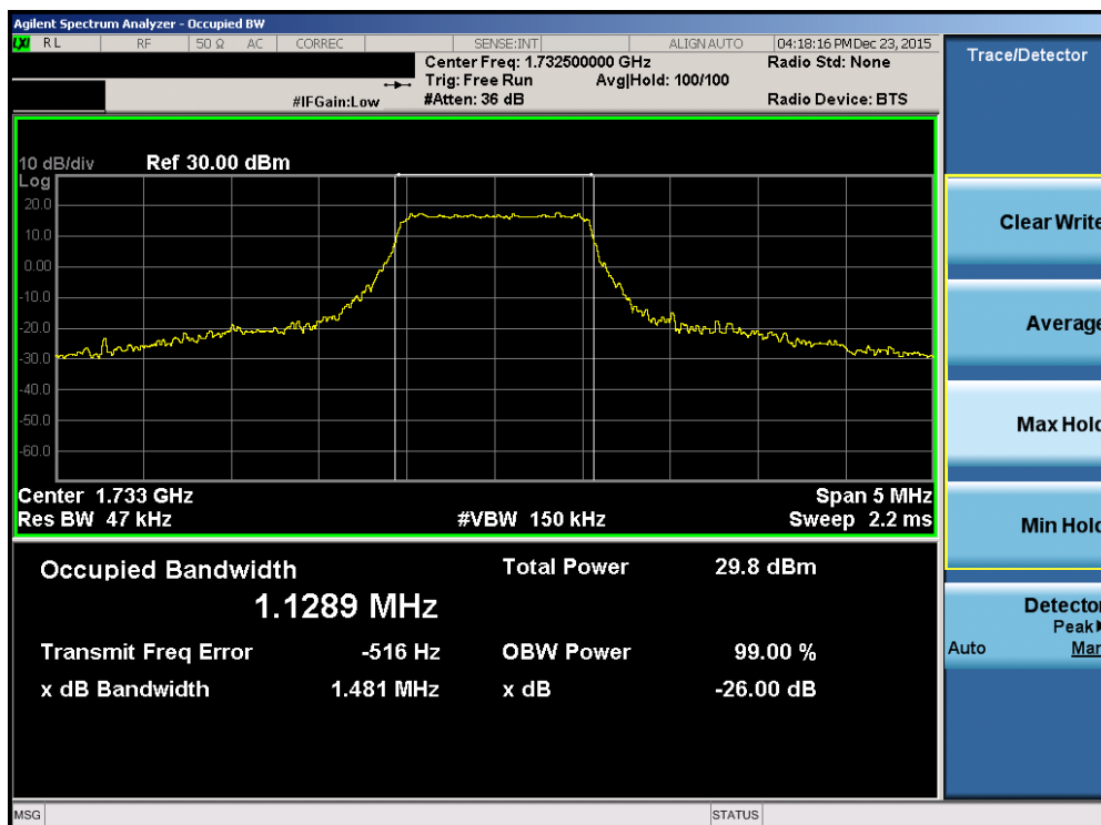
Plot 7-28. Occupied Bandwidth Plot (Band 4 – 1.4MHz 16-QAM – RB Size 6)
