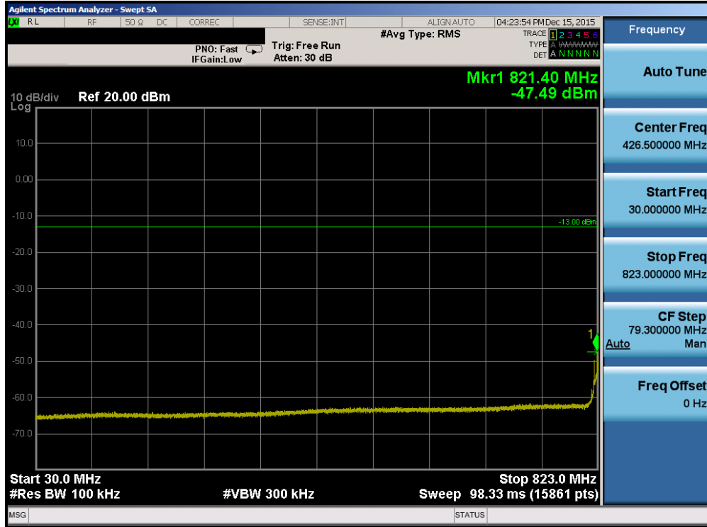
Plot 7-77. Conducted Spurious Plot (Band 26 – 10.0MHz QPSK – RB Size 1, RB Offset 0– Low Channel)
