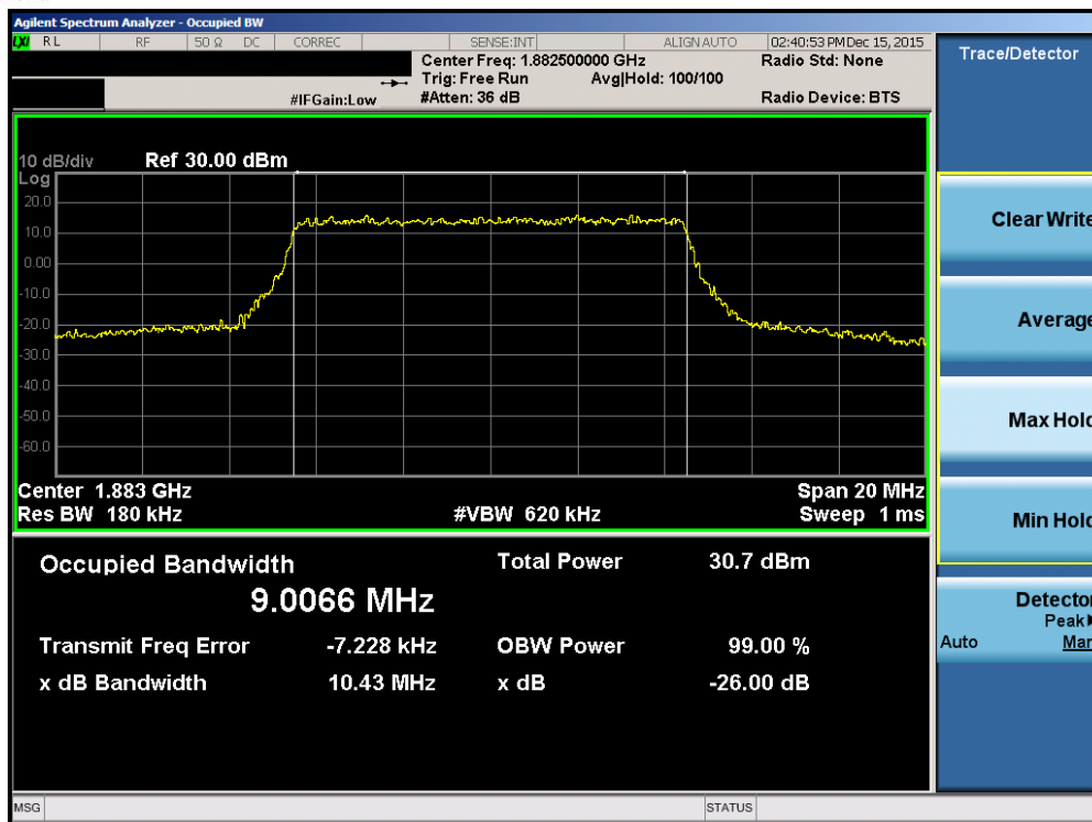
Plot 7-45. Occupied Bandwidth Plot (Band2/25 – 10.0MHz QPSK – RB Size 50)
