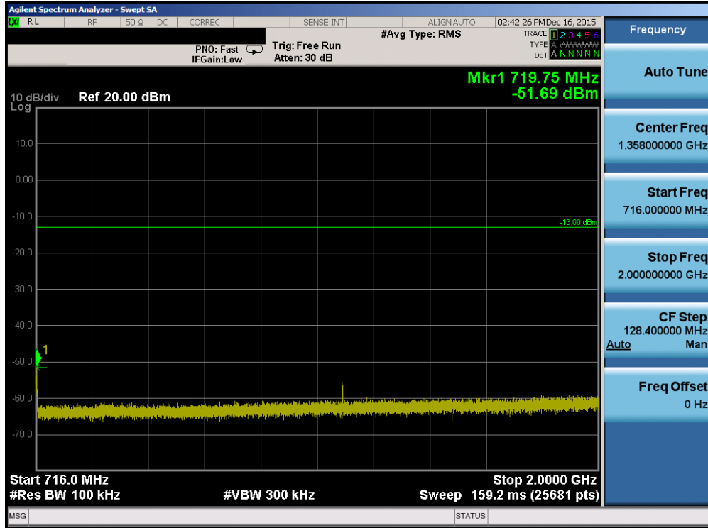
Plot 7-63. Conducted Spurious Plot (Band 12/17 – 10.0MHz QPSK – RB Size 1, RB Offset 0 – Mid Channel)
