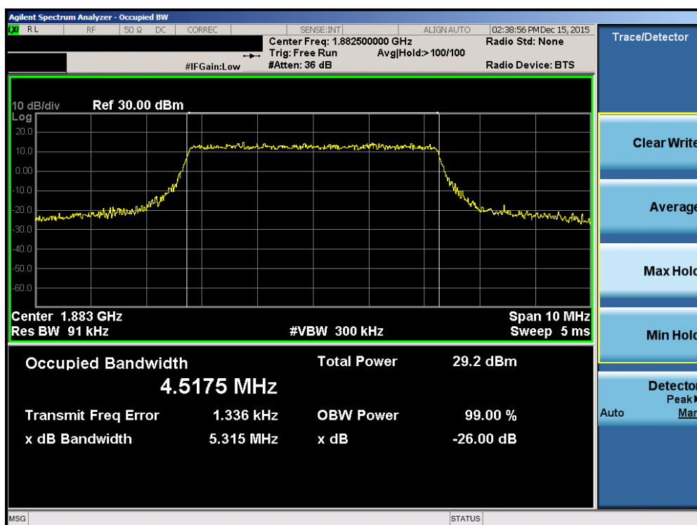
Plot 7-44. Occupied Bandwidth Plot (Band2/25 – 5.0MHz 16-QAM – RB Size 25)
