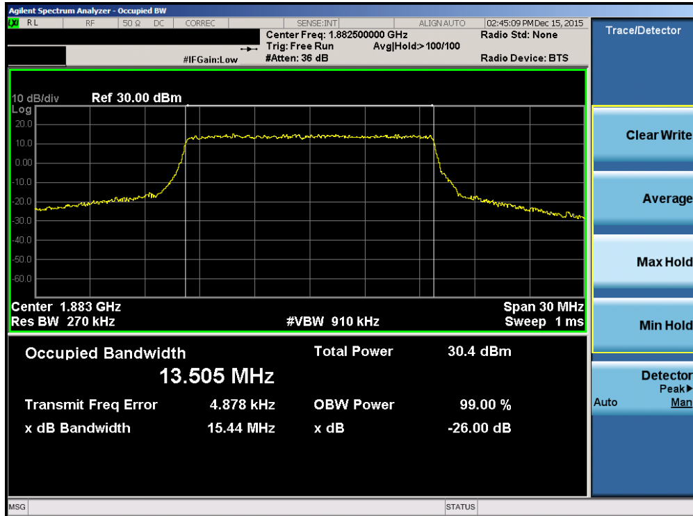
Plot 7-48. Occupied Bandwidth Plot (Band2/25 – 15.0MHz 16-QAM – RB Size 75)
