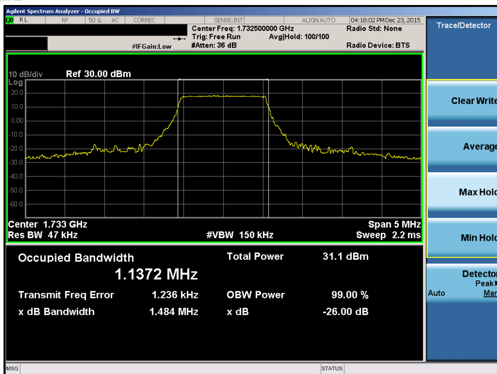
Plot 7-27. Occupied Bandwidth Plot (Band 4 – 1.4MHz QPSK – RB Size 6)
