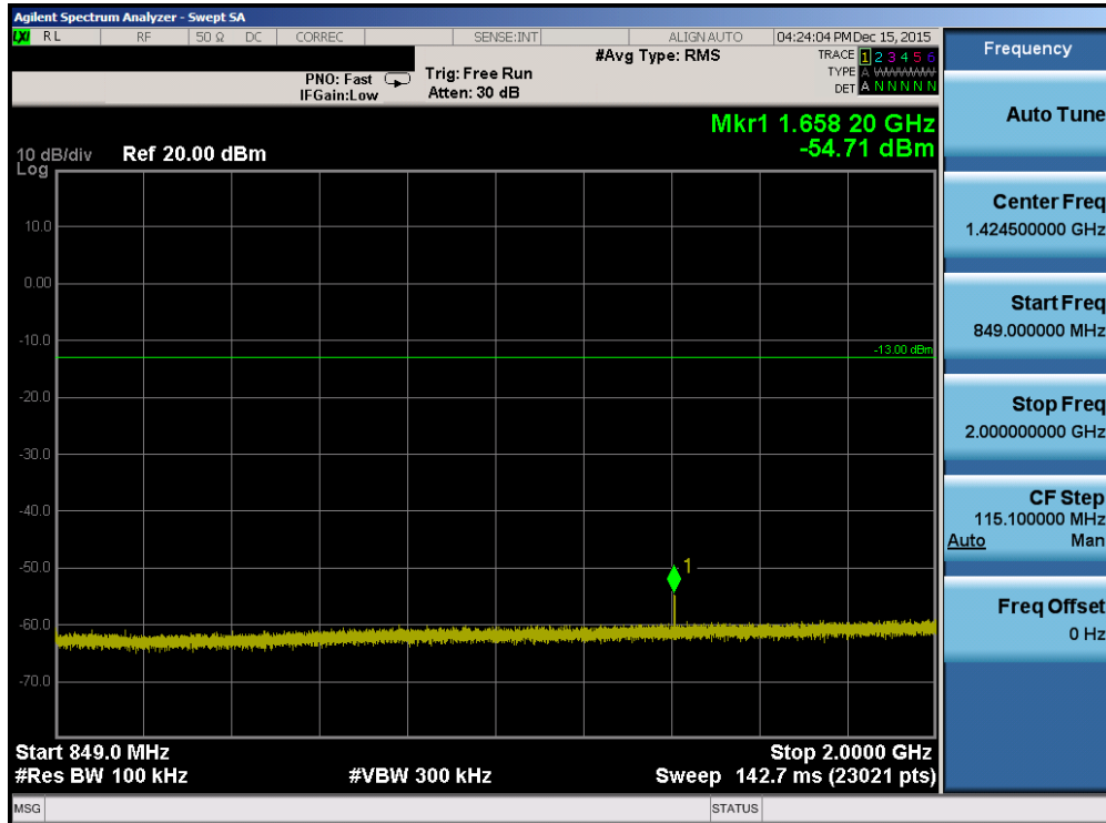
Plot 7-78. Conducted Spurious Plot (Band 26 – 10.0MHz QPSK – RB Size 1, RB Offset 0 – Low Channel)
