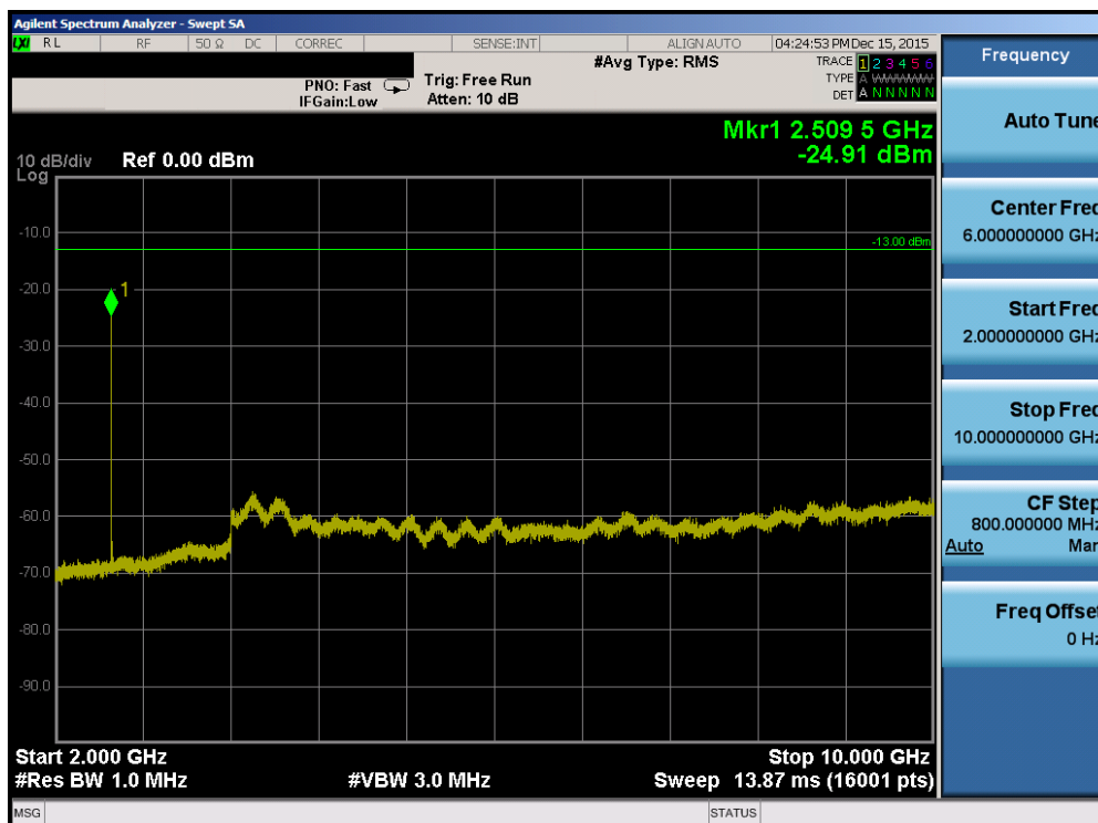
Plot 7-82. Conducted Spurious Plot (Band 26 – 10.0MHz QPSK – RB Size 1, RB Offset 0 – Mid Channel)
