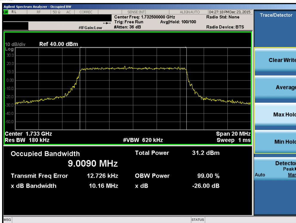
Plot 7-33. Occupied Bandwidth Plot (Band 4 – 10.0MHz QPSK – RB Size 50)
