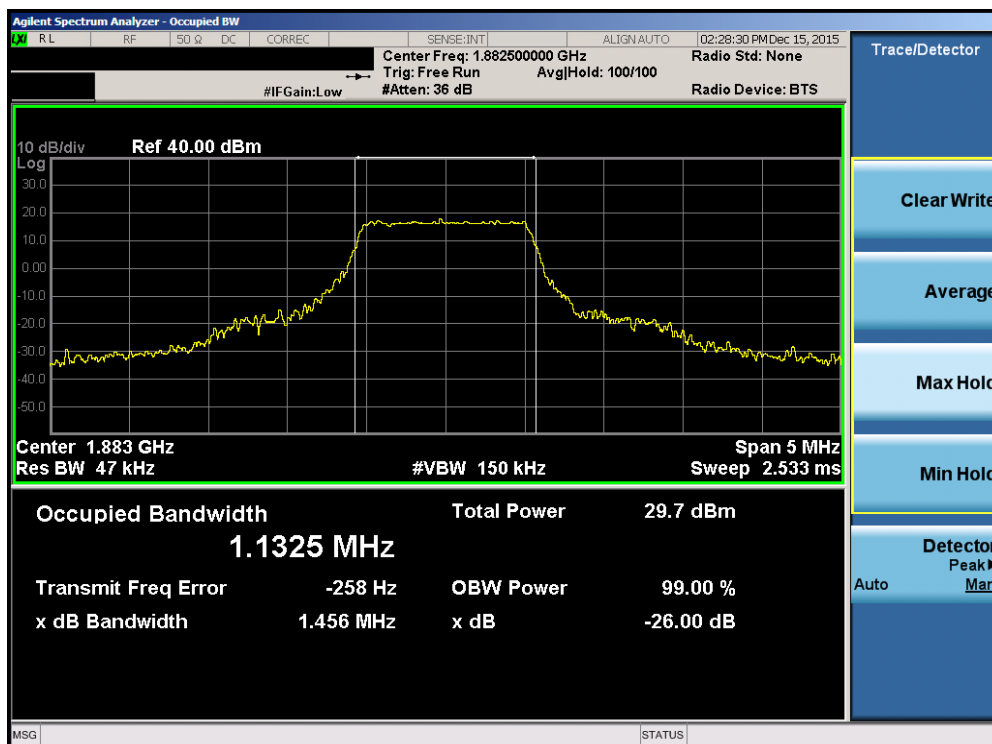
Plot 7-40. Occupied Bandwidth Plot (Band2/25 – 1.4MHz 16-QAM – RB Size 6)
