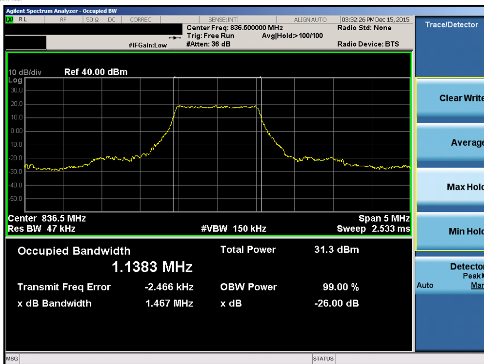
Plot 7-17. Occupied Bandwidth Plot (Band 26 – 1.4MHz QPSK – RB Size 6)
