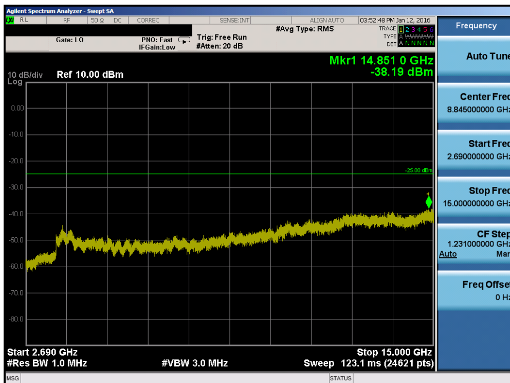
Plot 7-108. Conducted Spurious Plot (Band 41 – 20.0MHz QPSK – RB Size 1, RB Offset 0 – Mid Channel)
