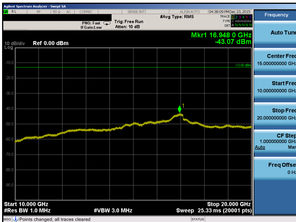
Plot 7-94. Conducted Spurious Plot (Band 4 – 20.0MHz QPSK – RB Size 1, RB Offset 0 – High Channel)
