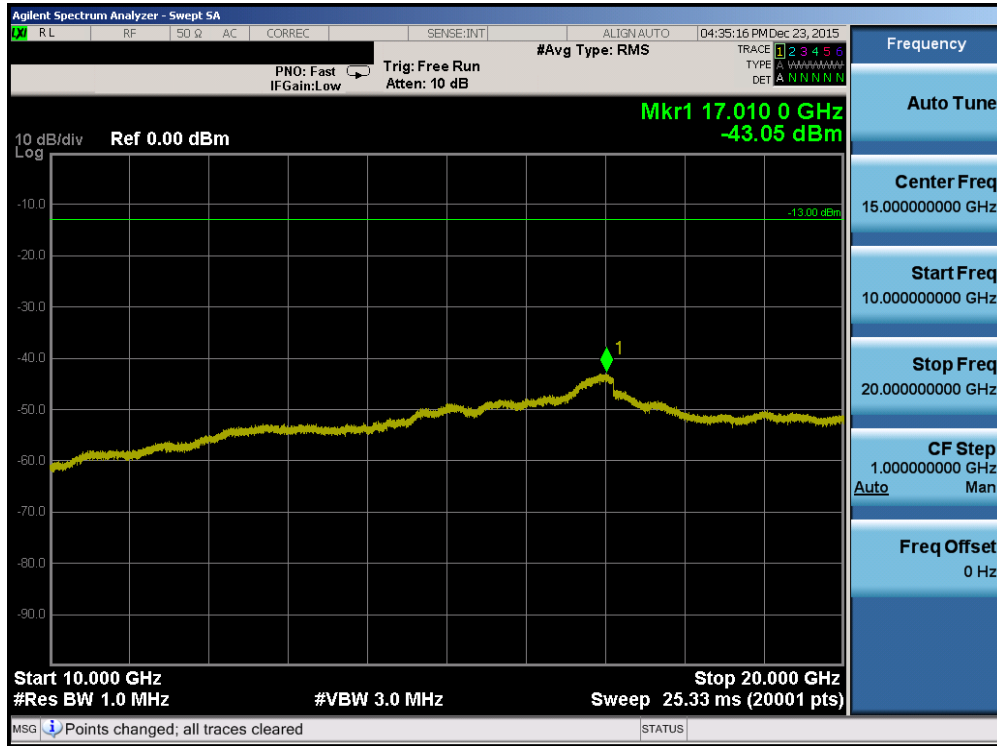
Plot 7-91. Conducted Spurious Plot (Band 4 – 20.0MHz QPSK – RB Size 1, RB Offset 0 – Mid Channel)
