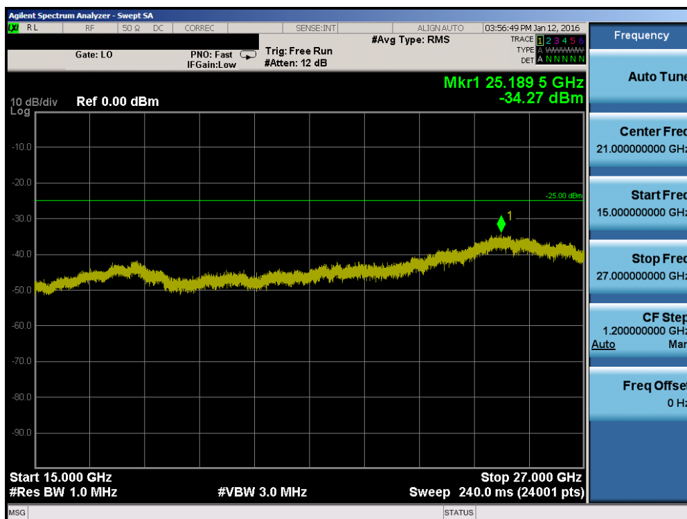
Plot 7-112. Conducted Spurious Plot (Band 41 – 20.0MHz QPSK – RB Size 1, RB Offset 0 – High Channel)
