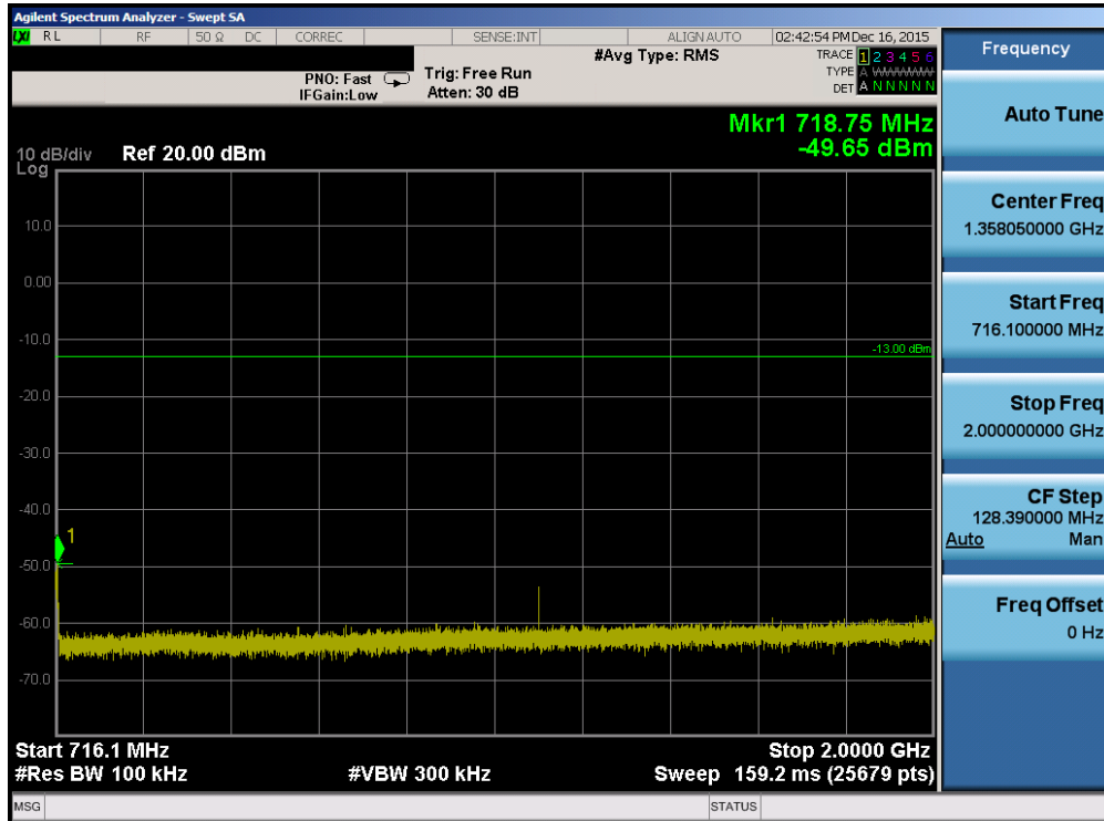
Plot 7-66. Conducted Spurious Plot (Band 12/17 – 10.0MHz QPSK – RB Size 1, RB Offset 0 – High Channel)
