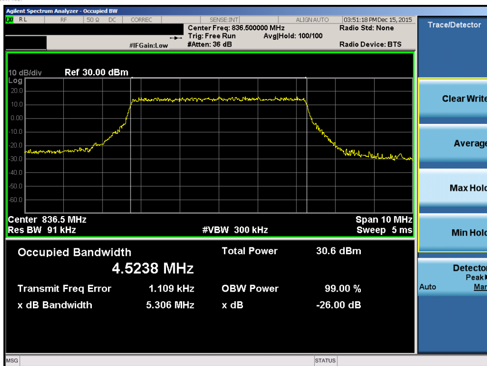
Plot 7-21. Occupied Bandwidth Plot (Band 26 – 5.0MHz QPSK – RB Size 25)
