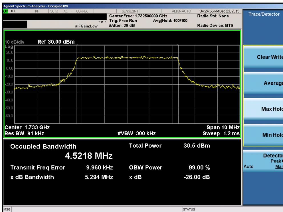
Plot 7-32. Occupied Bandwidth Plot (Band 4 – 5.0MHz 16-QAM – RB Size 25)
