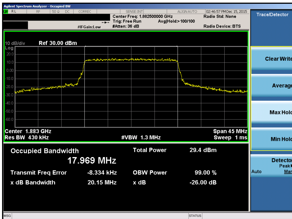
Plot 7-50. Occupied Bandwidth Plot (Band2/25 – 20.0MHz 16-QAM – RB Size 100)
