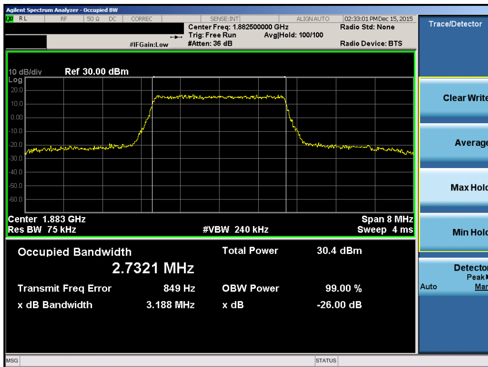
Plot 7-41. Occupied Bandwidth Plot (Band2/25 – 3.0MHz QPSK – RB Size 15)
