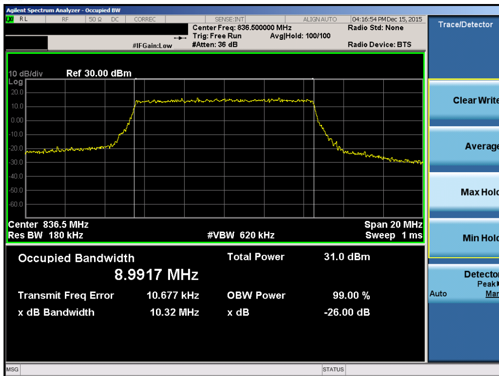
Plot 7-23. Occupied Bandwidth Plot (Band 26 – 10.0MHz QPSK – RB Size 50)
