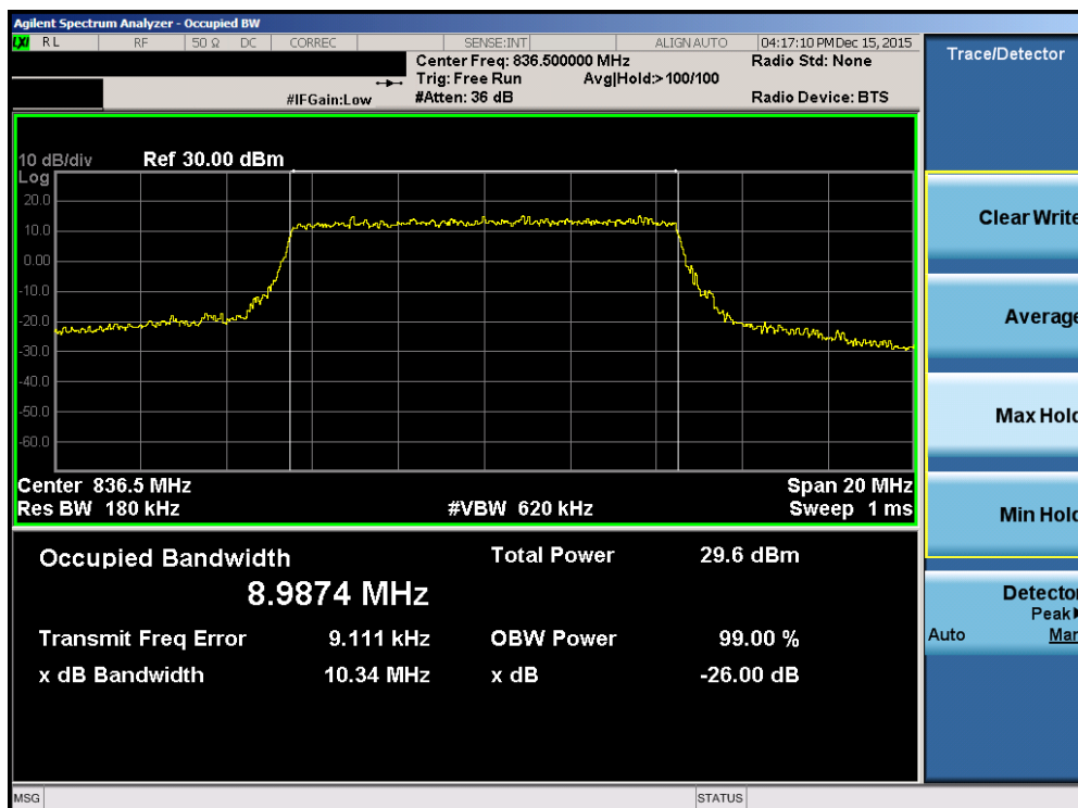
Plot 7-24. Occupied Bandwidth Plot (Band 26 – 10.0MHz 16-QAM – RB Size 50)
