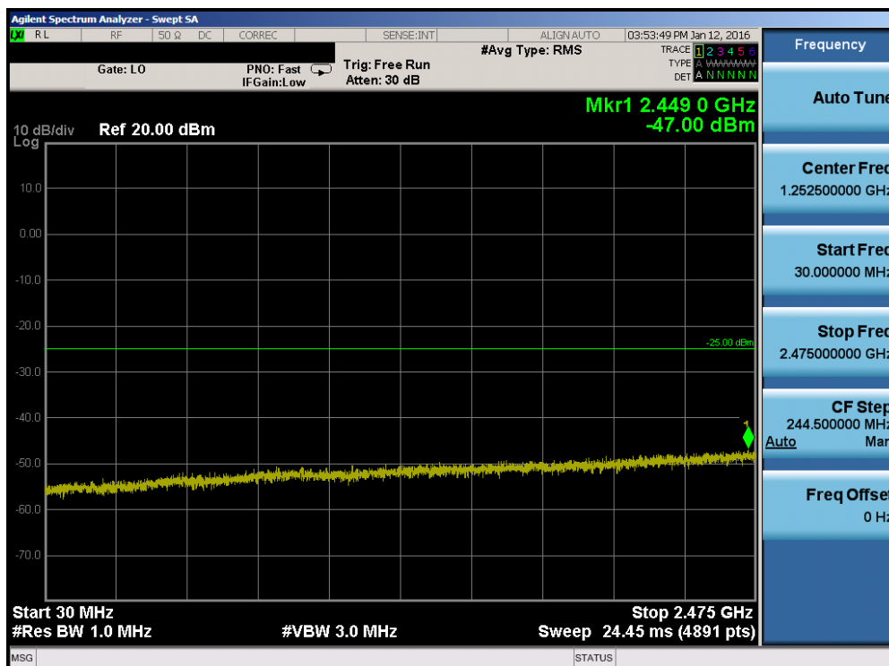
Plot 7-104. Conducted Spurious Plot (Band 41 – 20.0MHz QPSK – RB Size 1, RB Offset 0– Low Channel)
