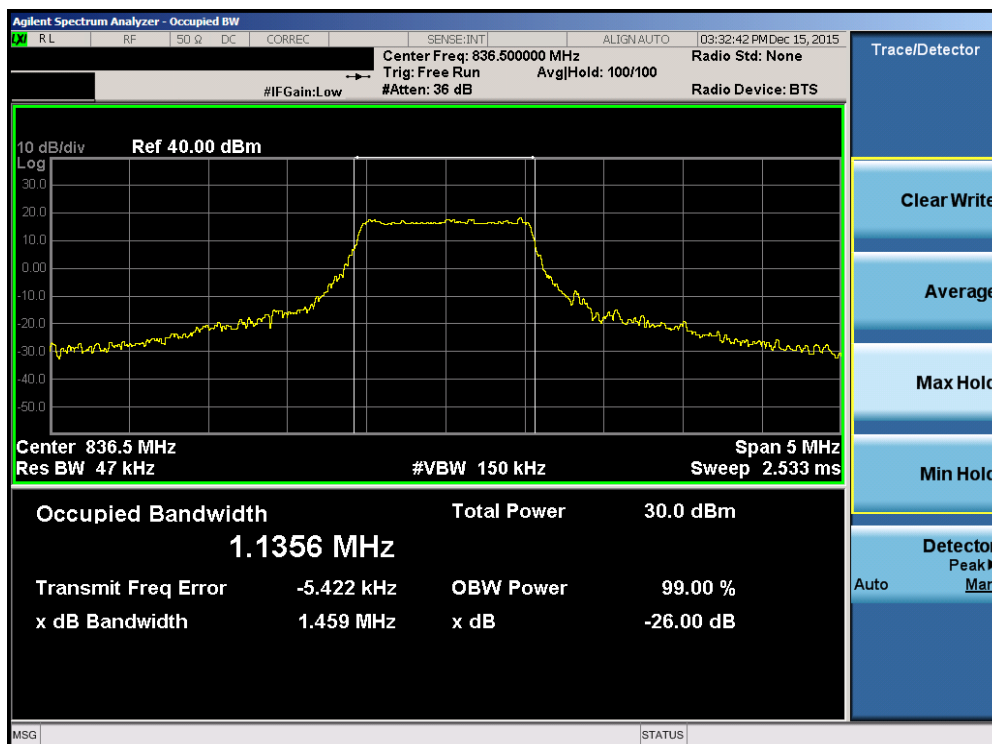
Plot 7-18. Occupied Bandwidth Plot (Band 26 – 1.4MHz 16-QAM – RB Size 6)
