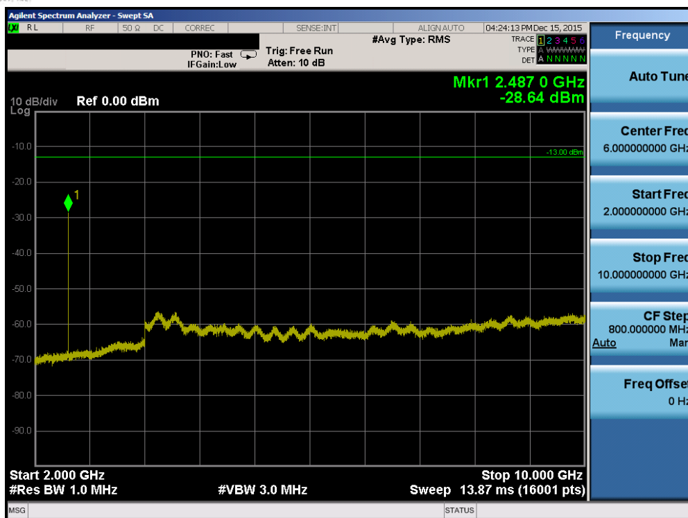
Plot 7-79. Conducted Spurious Plot (Band 26 – 10.0MHz QPSK – RB Size 1, RB Offset 0 – Low Channel)
