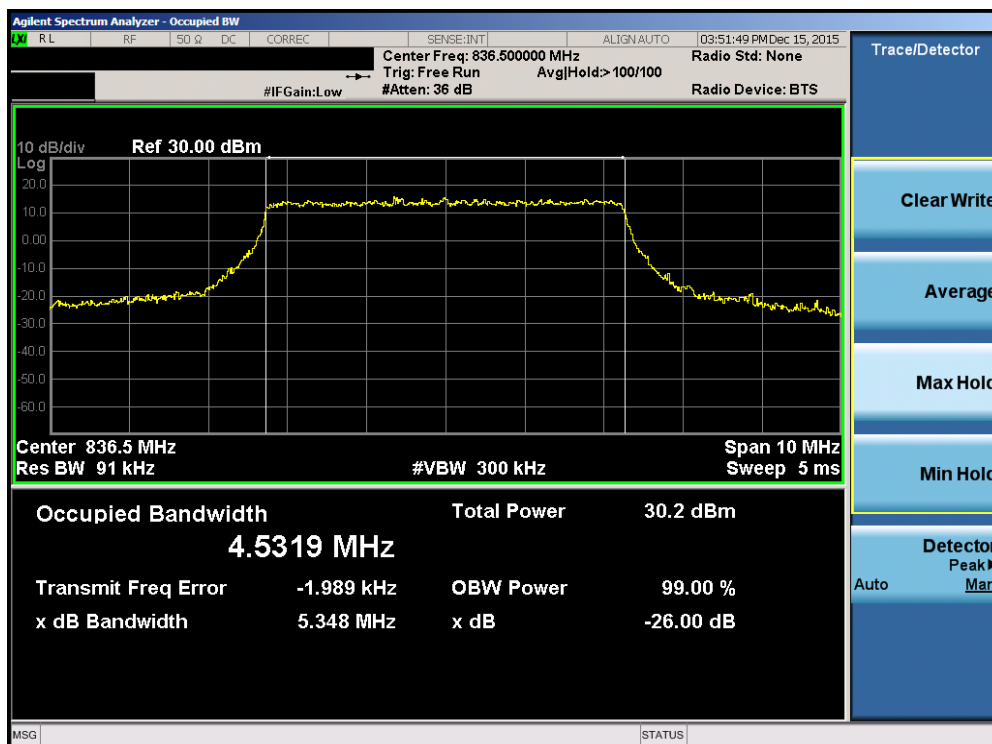
Plot 7-22. Occupied Bandwidth Plot (Band 26 – 5.0MHz 16-QAM – RB Size 25)
