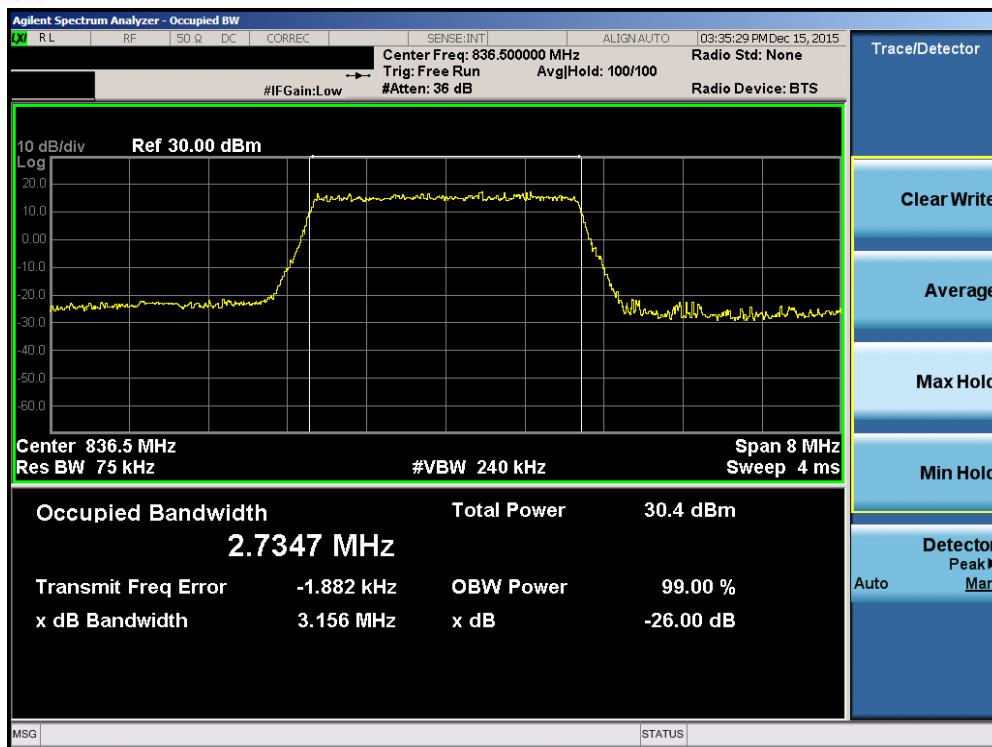
Plot 7-19. Occupied Bandwidth Plot (Band 26 – 3.0MHz QPSK – RB Size 15)
