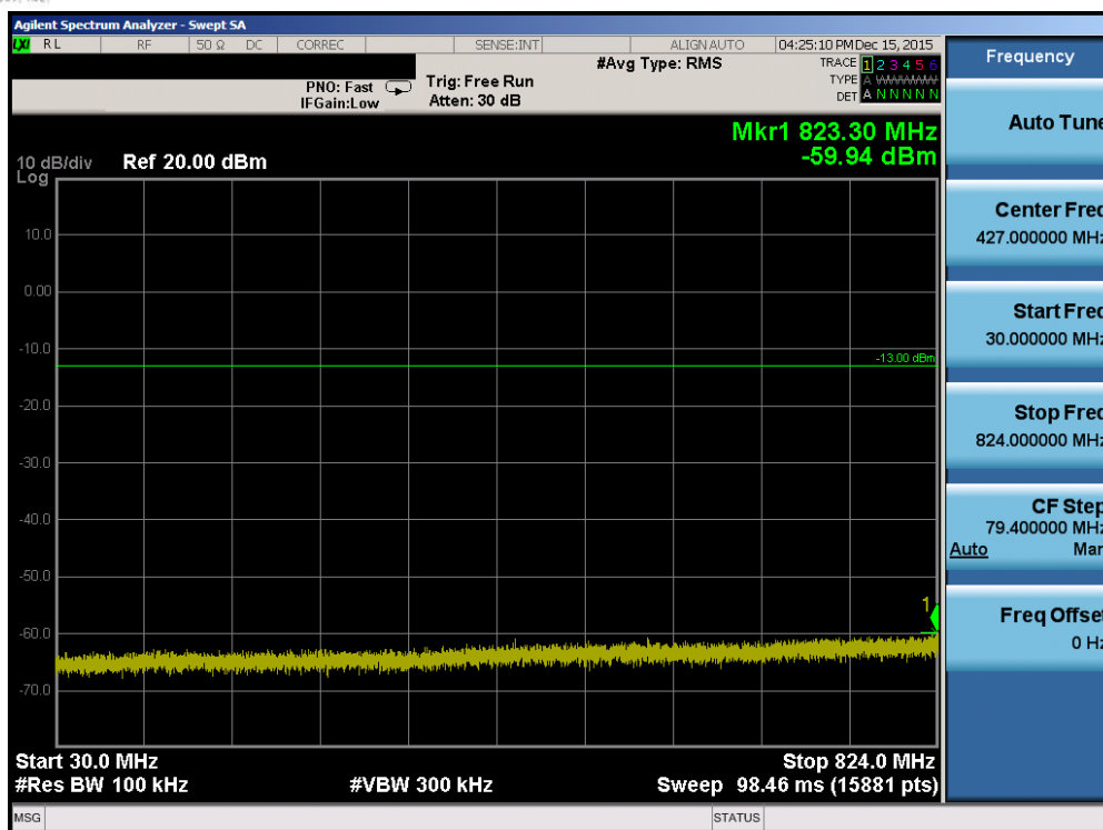
Plot 7-83. Conducted Spurious Plot (Band 26 – 10.0MHz QPSK – RB Size 1, RB Offset 0 – High Channel)
