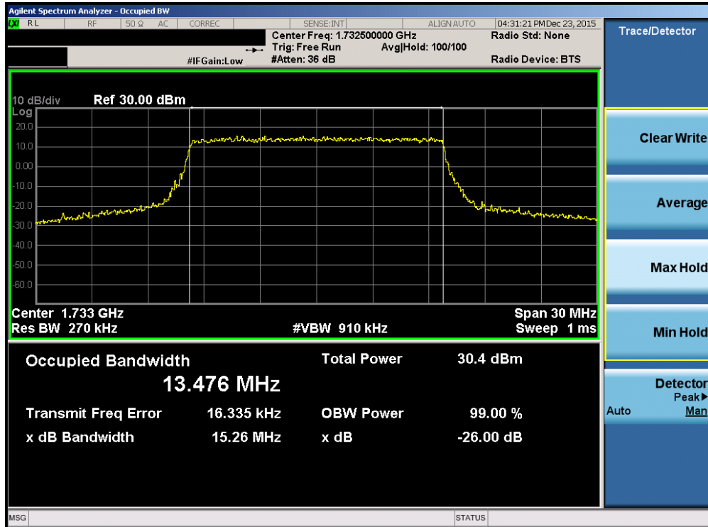
Plot 7-36. Occupied Bandwidth Plot (Band 4 – 15.0MHz 16-QAM – RB Size 75)
