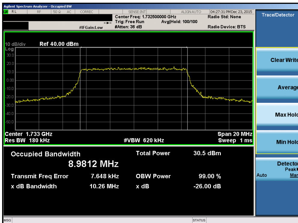
Plot 7-34. Occupied Bandwidth Plot (Band 4 – 10.0MHz 16-QAM – RB Size 50)
