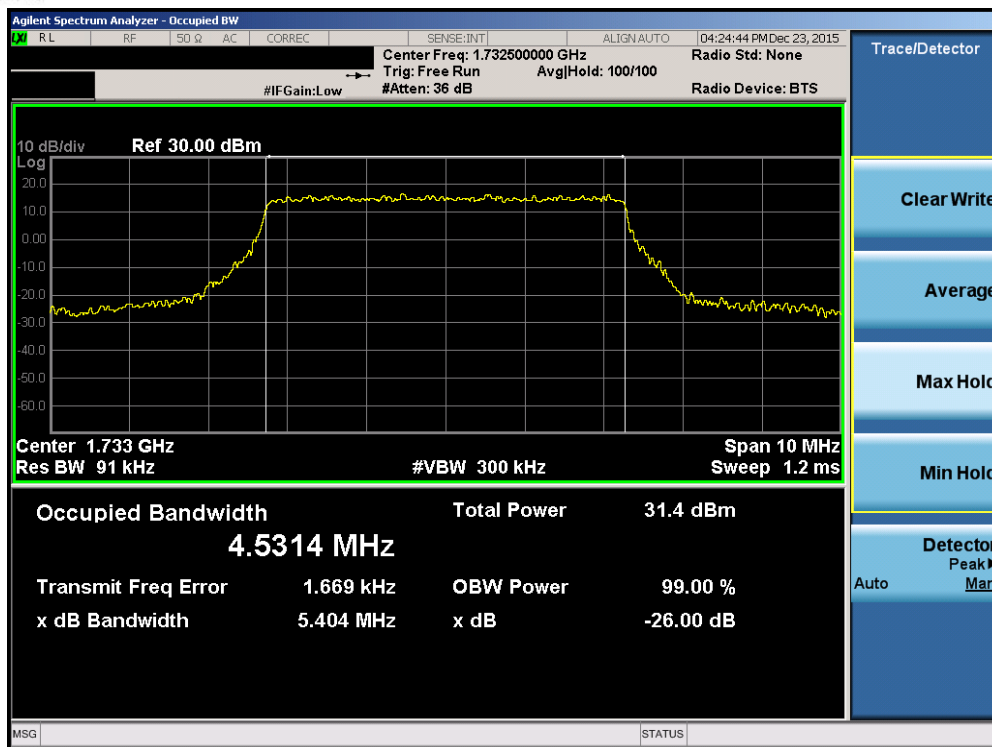
Plot 7-31. Occupied Bandwidth Plot (Band 4 – 5.0MHz QPSK – RB Size 25)
