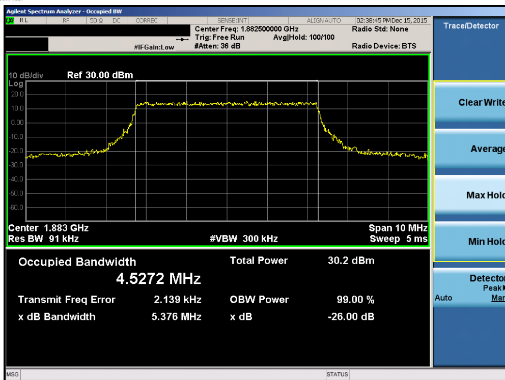
Plot 7-43. Occupied Bandwidth Plot (Band2/25 – 5.0MHz QPSK – RB Size 25)
