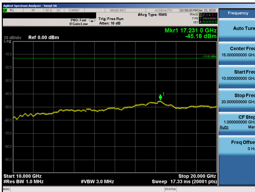
Plot 7-97. Conducted Spurious Plot (Band2/25 – 1.4MHz QPSK – RB Size 1, RB Offset 0 – Low Channel)
