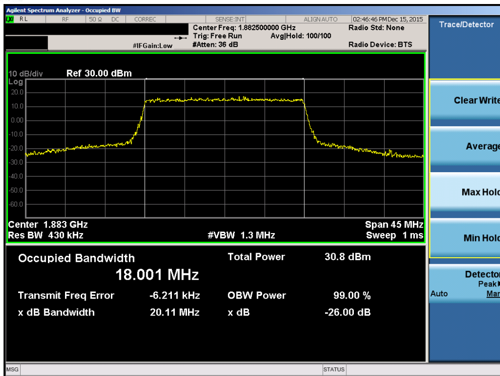
Plot 7-49. Occupied Bandwidth Plot (Band2/25 – 20.0MHz QPSK – RB Size 100)
