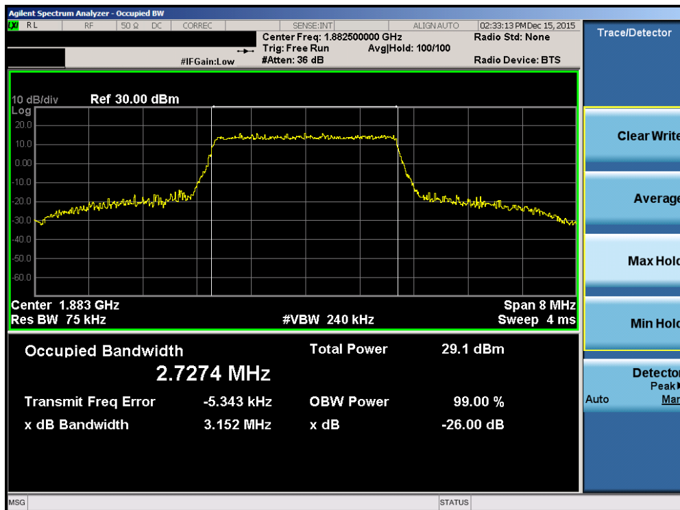
Plot 7-42. Occupied Bandwidth Plot (Band2/25 – 3.0MHz 16-QAM – RB Size 15)
