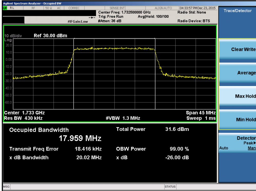
Plot 7-37. Occupied Bandwidth Plot (Band 4 – 20.0MHz QPSK – RB Size 100)
