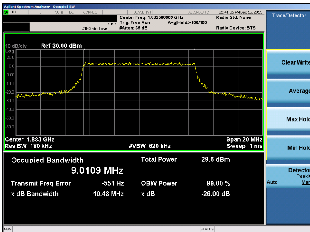
Plot 7-46. Occupied Bandwidth Plot (Band2/25 – 10.0MHz 16-QAM – RB Size 50)
