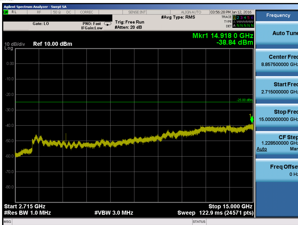
Plot 7-111. Conducted Spurious Plot (Band 41 – 20.0MHz QPSK – RB Size 1, RB Offset 0 – High Channel)
