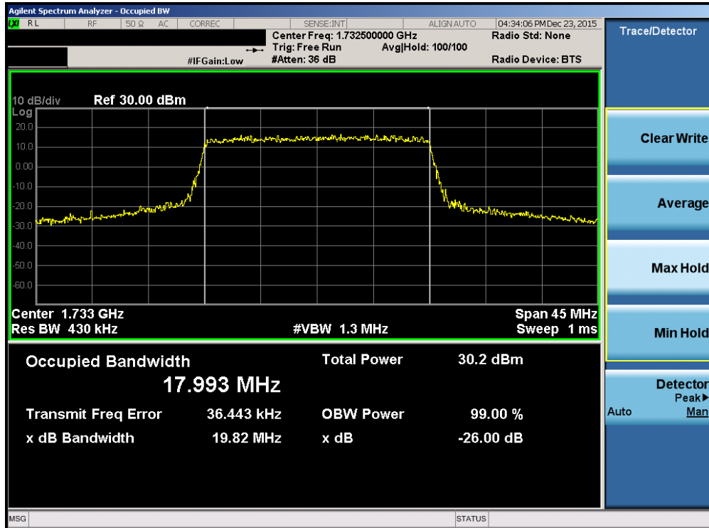
Plot 7-38. Occupied Bandwidth Plot (Band 4 – 20.0MHz 16-QAM – RB Size 100)
