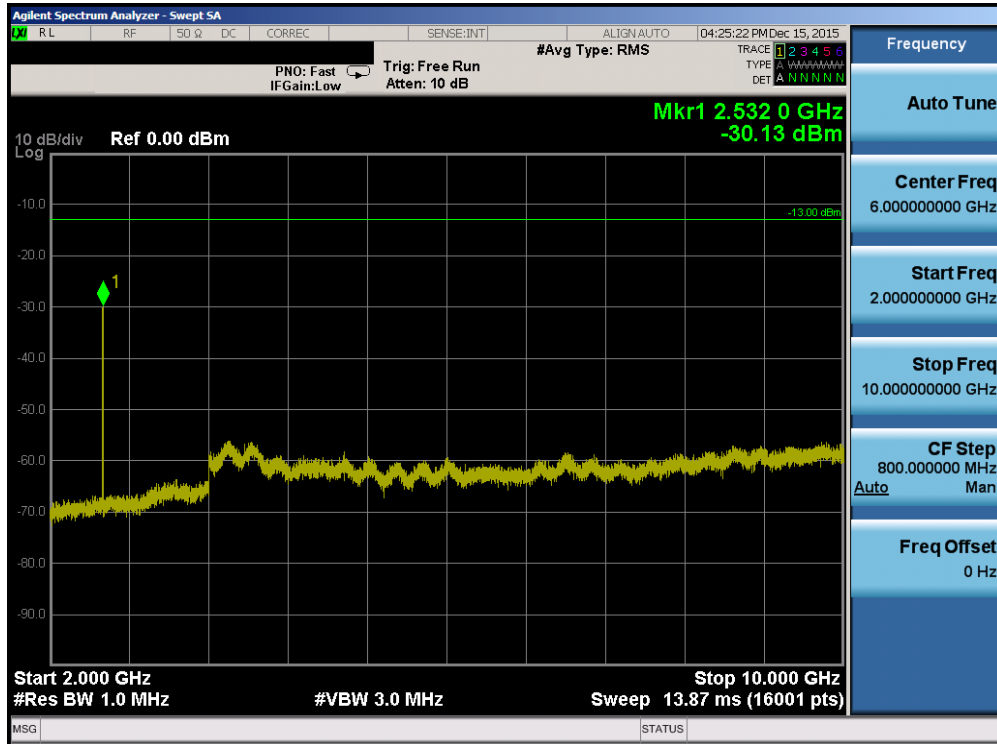
Plot 7-85. Conducted Spurious Plot (Band 26 – 10.0MHz QPSK – RB Size 1, RB Offset 0 – High Channel)
