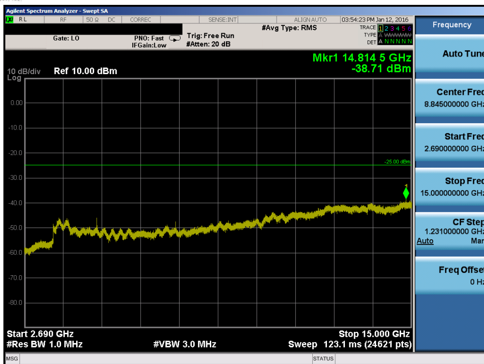
Plot 7-105. Conducted Spurious Plot (Band 41 – 20.0MHz QPSK – RB Size 1, RB Offset 0 – Low Channel)
