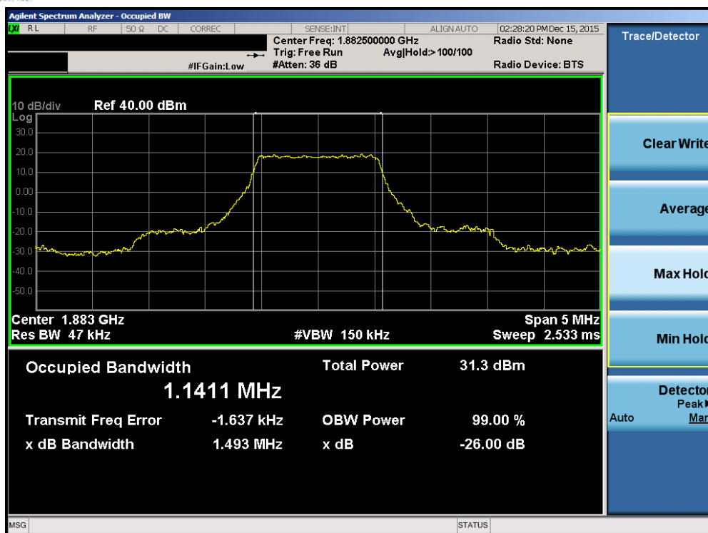
Plot 7-39. Occupied Bandwidth Plot (Band2/25 – 1.4MHz QPSK – RB Size 6)
