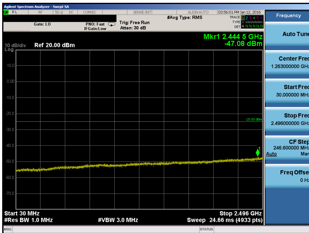
Plot 7-110. Conducted Spurious Plot (Band 41 – 20.0MHz QPSK – RB Size 1, RB Offset 0 – High Channel)
