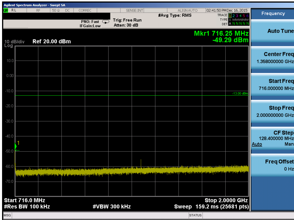
Plot 7-60. Conducted Spurious Plot (Band 12/17 – 10.0MHz QPSK – RB Size 1, RB Offset 0 – Low Channel)
