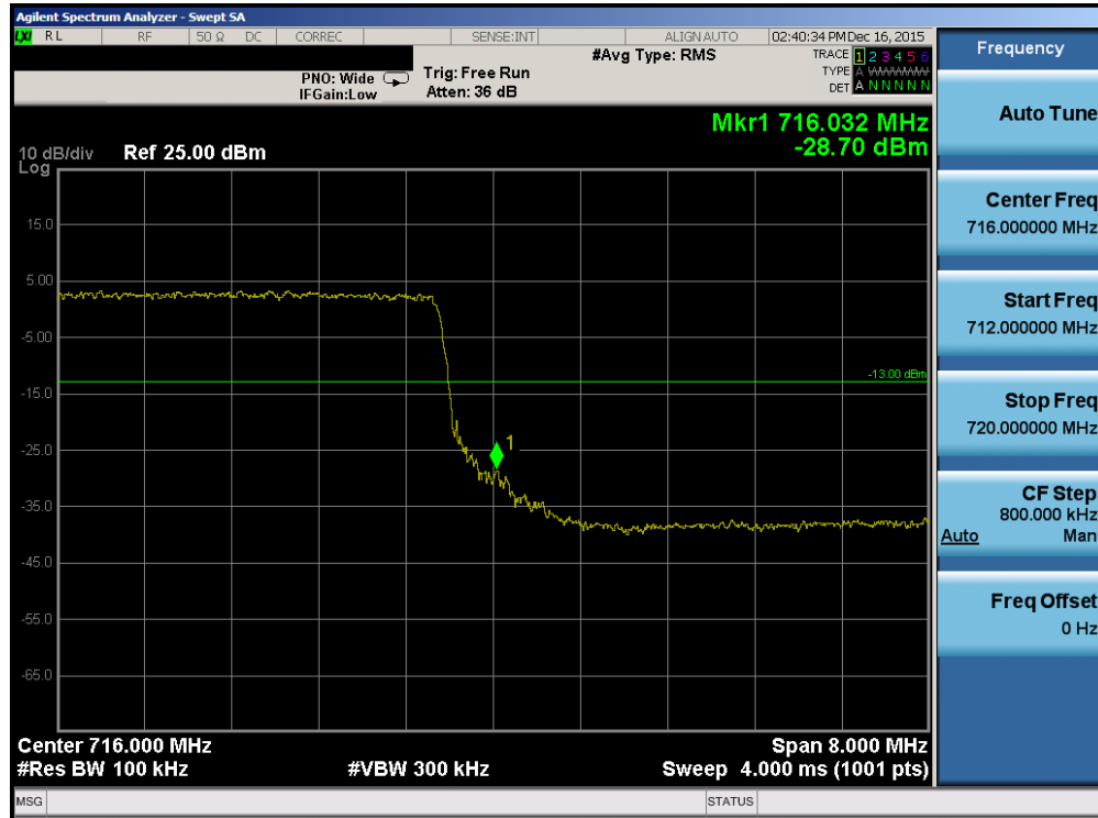
Plot 7-126. Upper Band Edge Plot (Band 12/17 – 10.0MHz QPSK – RB Size 50)
