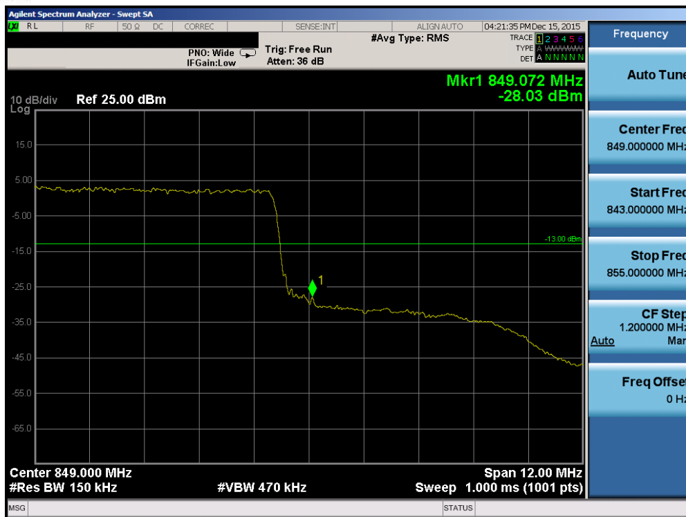
Plot 7-156. Upper Band Edge Plot (Band 26 – 15.0MHz QPSK – RB Size 75)
