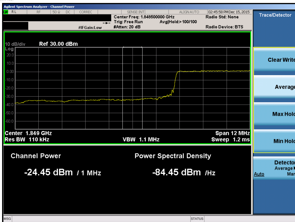
Plot 7-198. Lower Extended Band Edge Plot (Band2/25 – 15.0MHz QPSK – RB Size 75)
