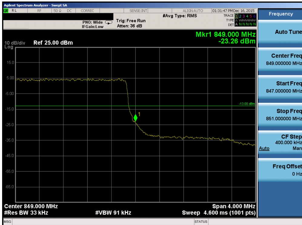
Plot 7-133. Upper Band Edge Plot (Band 5 – 3.0MHz QPSK – RB Size 15)
