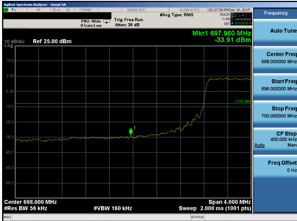
Plot 7-121. Lower Band Edge Plot (Band 12/17 – 5.0MHz QPSK – RB Size 25)
