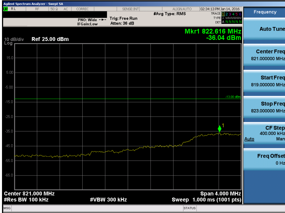
Plot 7-128. Lower Extended Band Edge Plot (Band 5 – 1.4MHz QPSK – RB Size 6)
