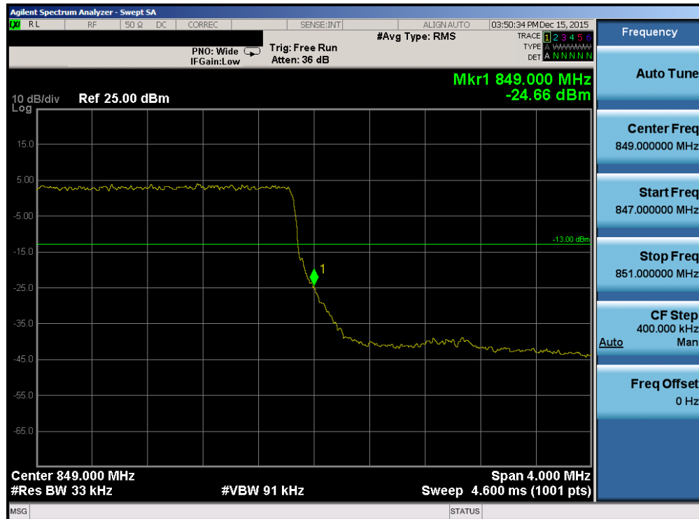
Plot 7-147. Upper Band Edge Plot (Band 26 – 3.0MHz QPSK – RB Size 15)
