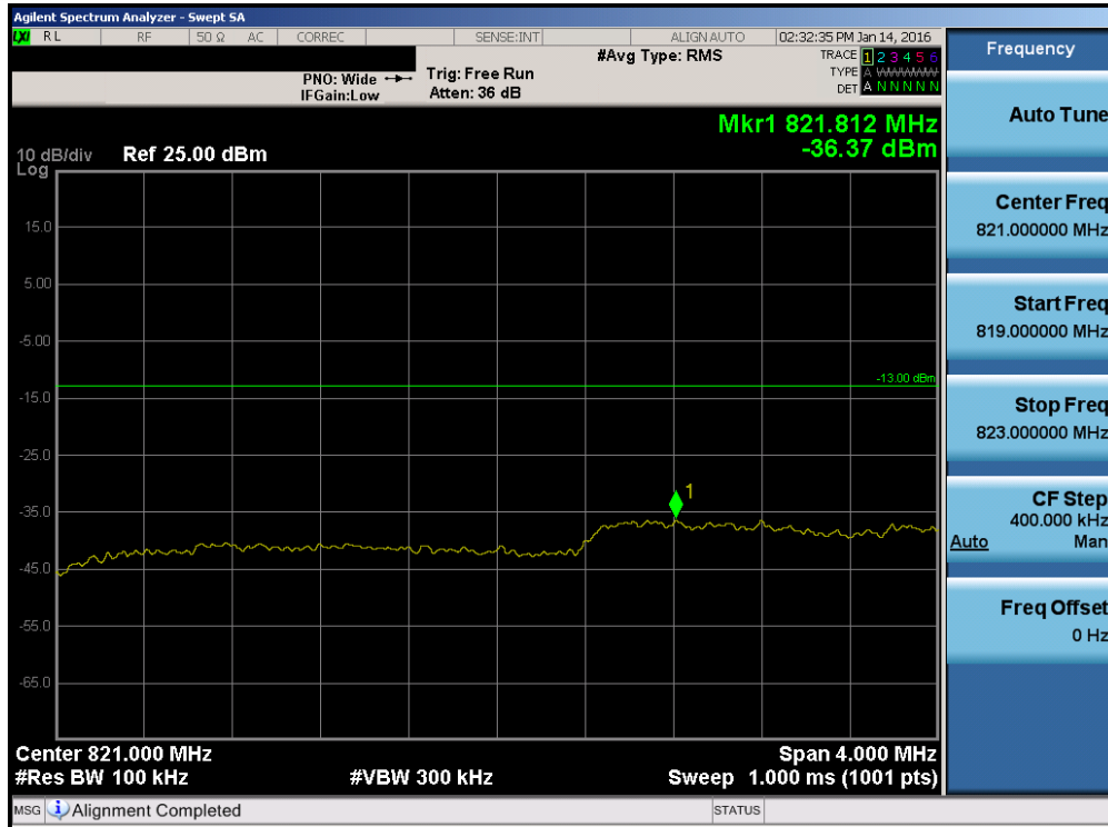
Plot 7-132. Lower Extended Band Edge Plot (Band 5 – 3.0MHz QPSK – RB Size 15)
