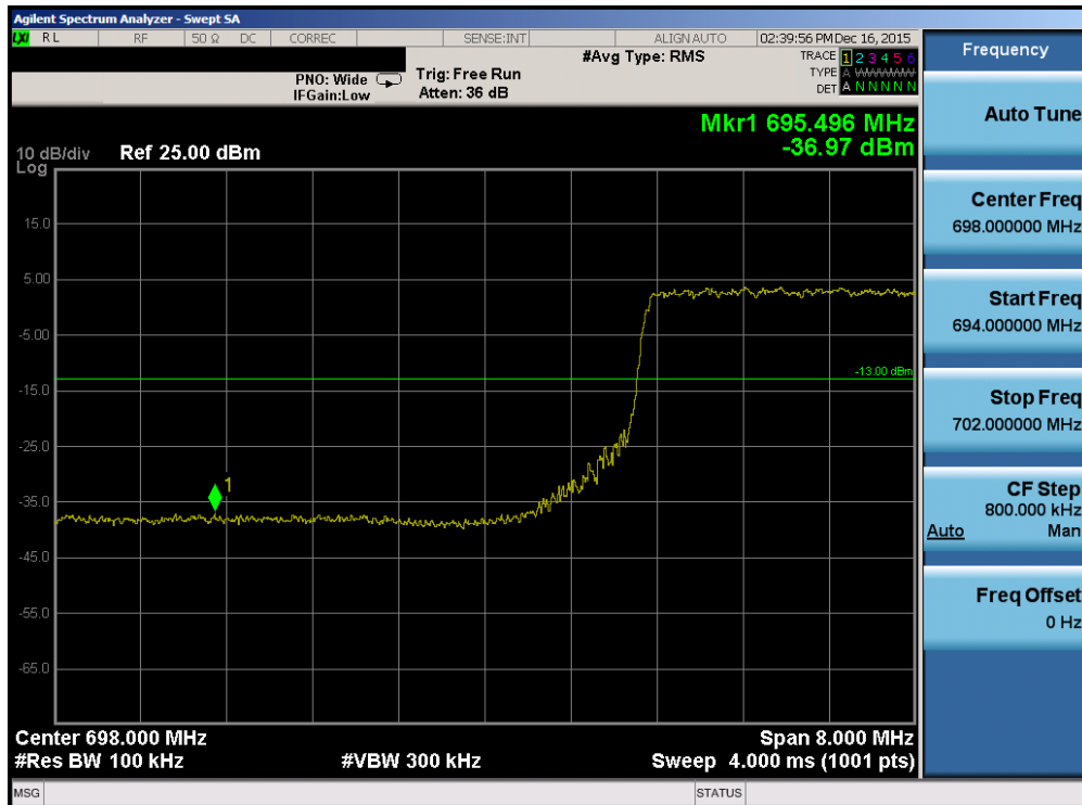
Plot 7-125. Lower Band Edge Plot (Band 12/17 – 10.0MHz QPSK – RB Size 50)
