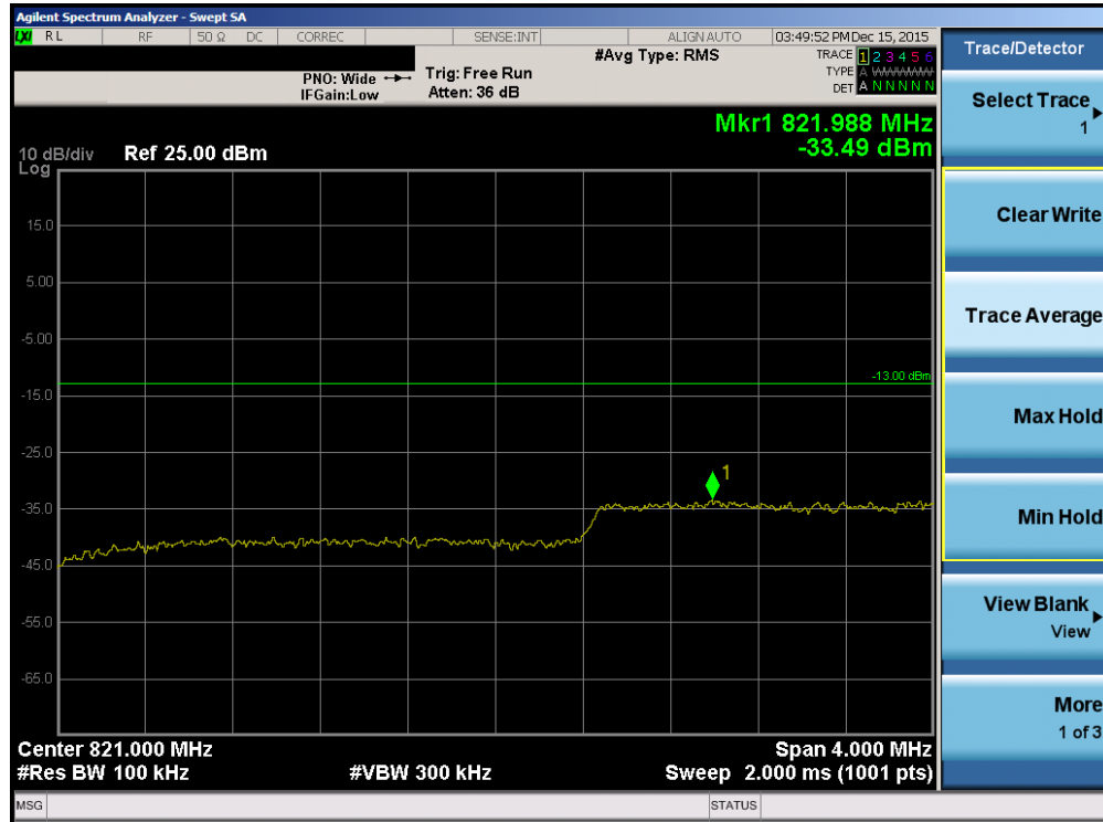
Plot 7-146. Lower Extended Band Edge Plot (Band 26 – 3.0MHz QPSK – RB Size 15)
