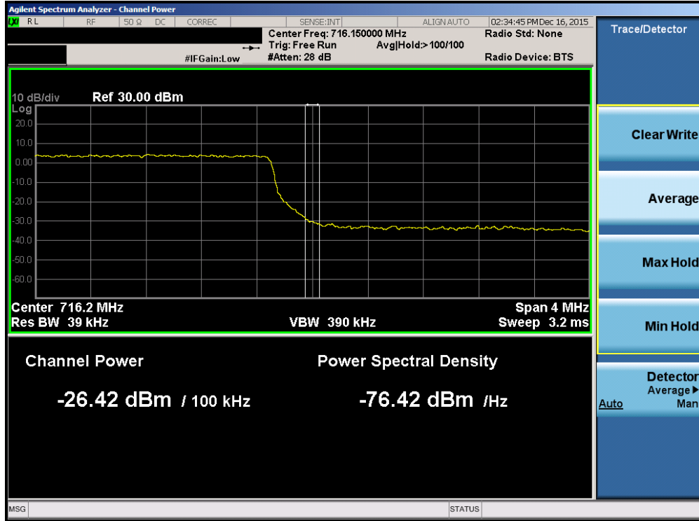
Plot 7-120. Upper Extended Band Edge Plot (Band 12 – 3.0MHz QPSK – RB Size 15)
