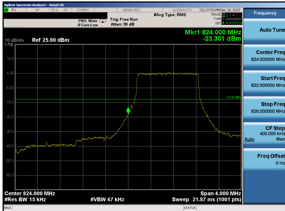
Plot 7-127. Lower Band Edge Plot (Band 5 – 1.4MHz QPSK – RB Size 6)
