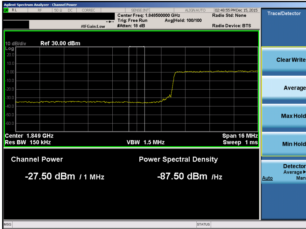
Plot 7-202. Lower Extended Band Edge Plot (Band2/25 – 20.0MHz QPSK – RB Size 100)
