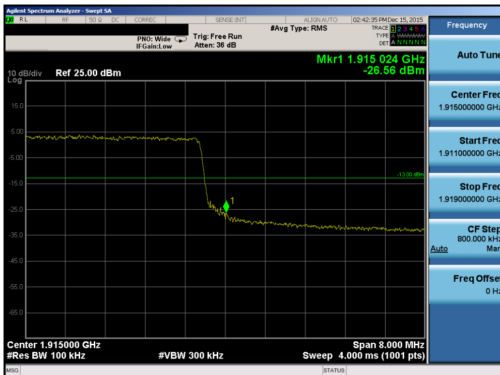
Plot 7-195. Upper Band Edge Plot (Band2/25 – 10.0MHz QPSK – RB Size 50)
