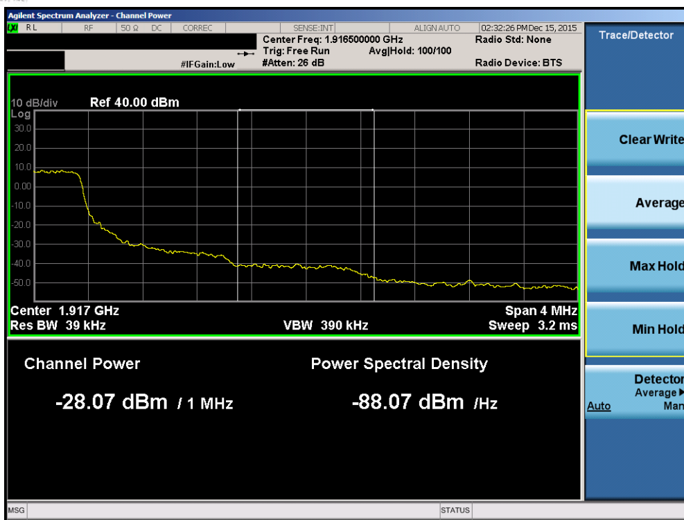
Plot 7-184. Upper Extended Band Edge Plot (Band2/25 – 1.4MHz QPSK – RB Size 6)
