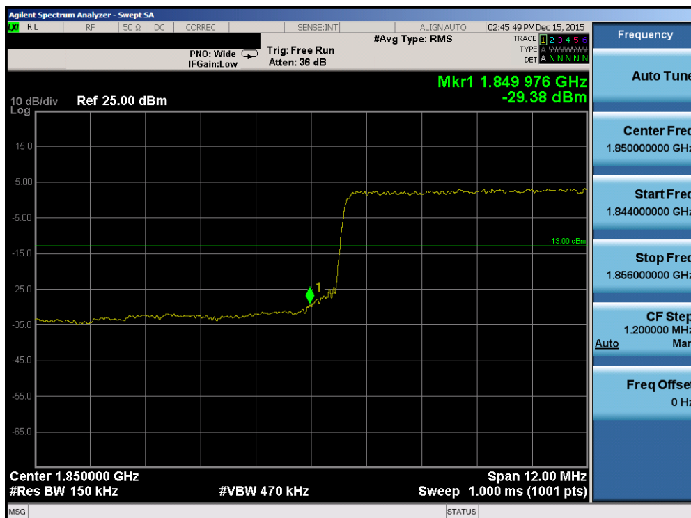
Plot 7-197. Lower Band Edge Plot (Band2/25 – 15.0MHz QPSK – RB Size 75)
