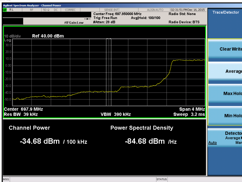
Plot 7-114. Lower Extended Band Edge Plot (Band 12 – 1.4MHz QPSK – RB Size 6)
