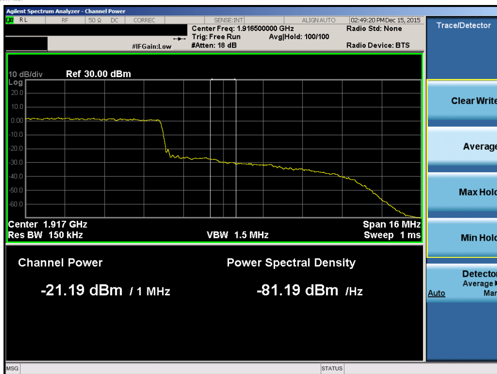
Plot 7-204. Upper Extended Band Edge Plot (Band2/25 – 20.0MHz QPSK – RB Size 100)
