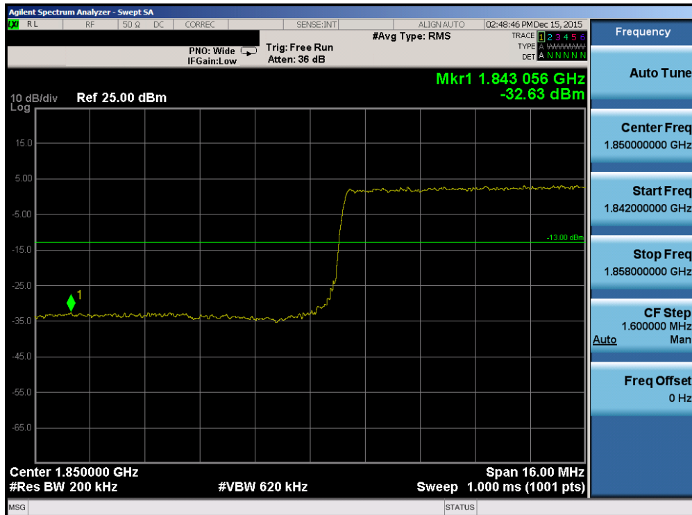
Plot 7-201. Lower Band Edge Plot (Band2/25 – 20.0MHz QPSK – RB Size 100)
