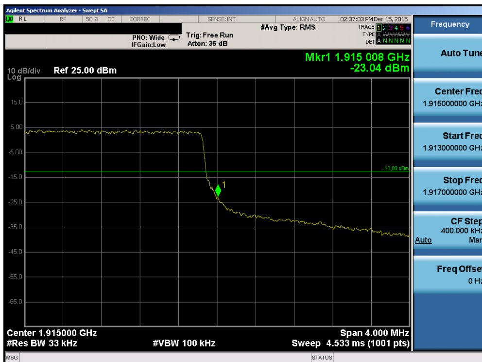
Plot 7-187. Upper Band Edge Plot (Band2/25 – 3.0MHz QPSK – RB Size 15)
