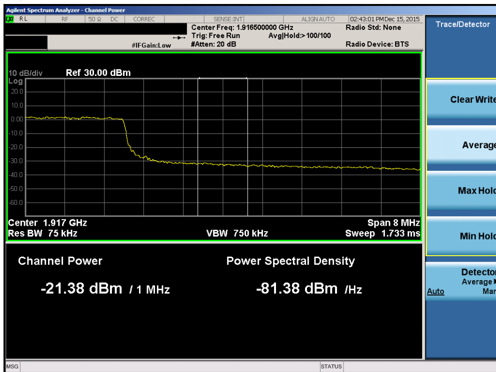
Plot 7-196. Upper Extended Band Edge Plot (Band2/25 – 10.0MHz QPSK – RB Size 50)
