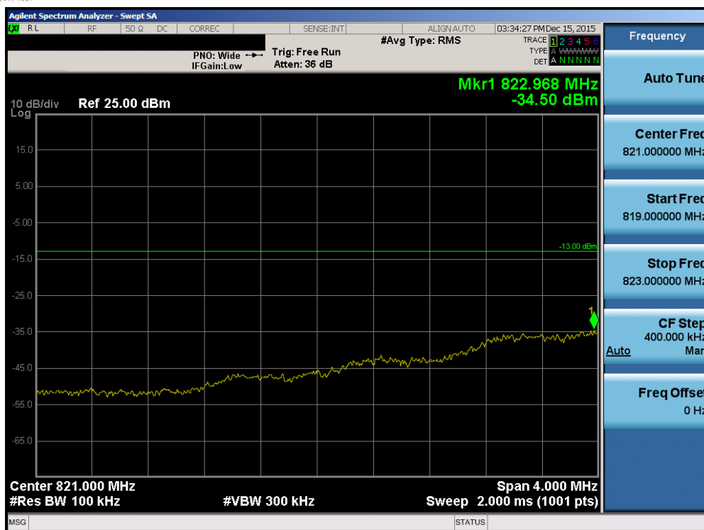
Plot 7-142. Lower Extended Band Edge Plot (Band 26 – 1.4MHz QPSK – RB Size 6)
