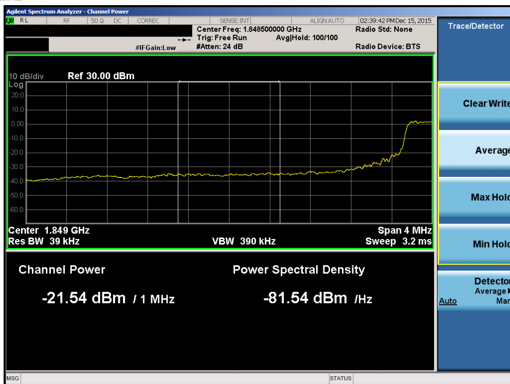
Plot 7-190. Lower Extended Band Edge Plot (Band2/25 – 5.0MHz QPSK – RB Size 25)
