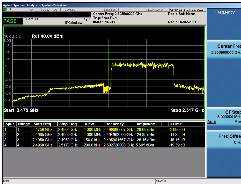
Plot 7-209. Lower ACP Plot (Band 41 – 15.0MHz QPSK – RB Size 75)
