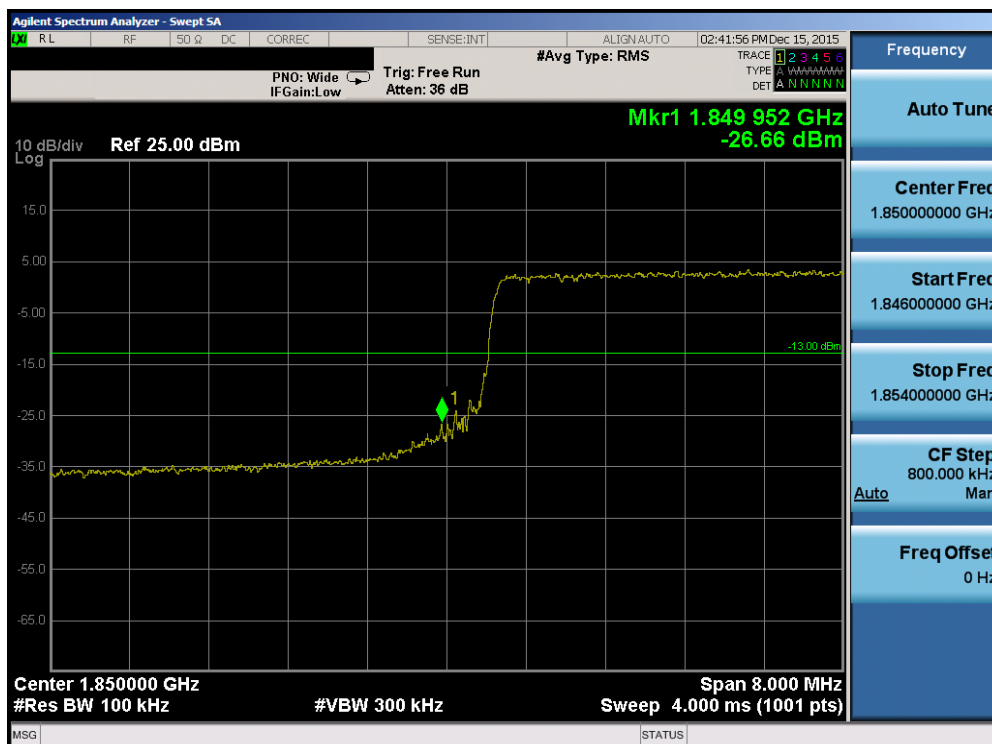
Plot 7-193. Lower Band Edge Plot (Band2/25 – 10.0MHz QPSK – RB Size 50)
