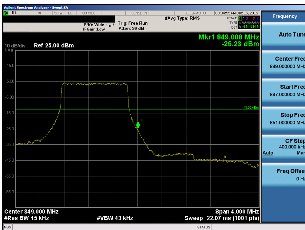
Plot 7-143. Upper Band Edge Plot (Band 26 – 1.4MHz QPSK – RB Size 6)
