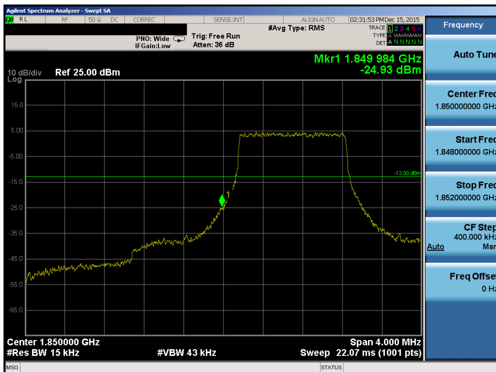
Plot 7-181. Lower Band Edge Plot (Band2/25 – 1.4MHz QPSK – RB Size 6)
