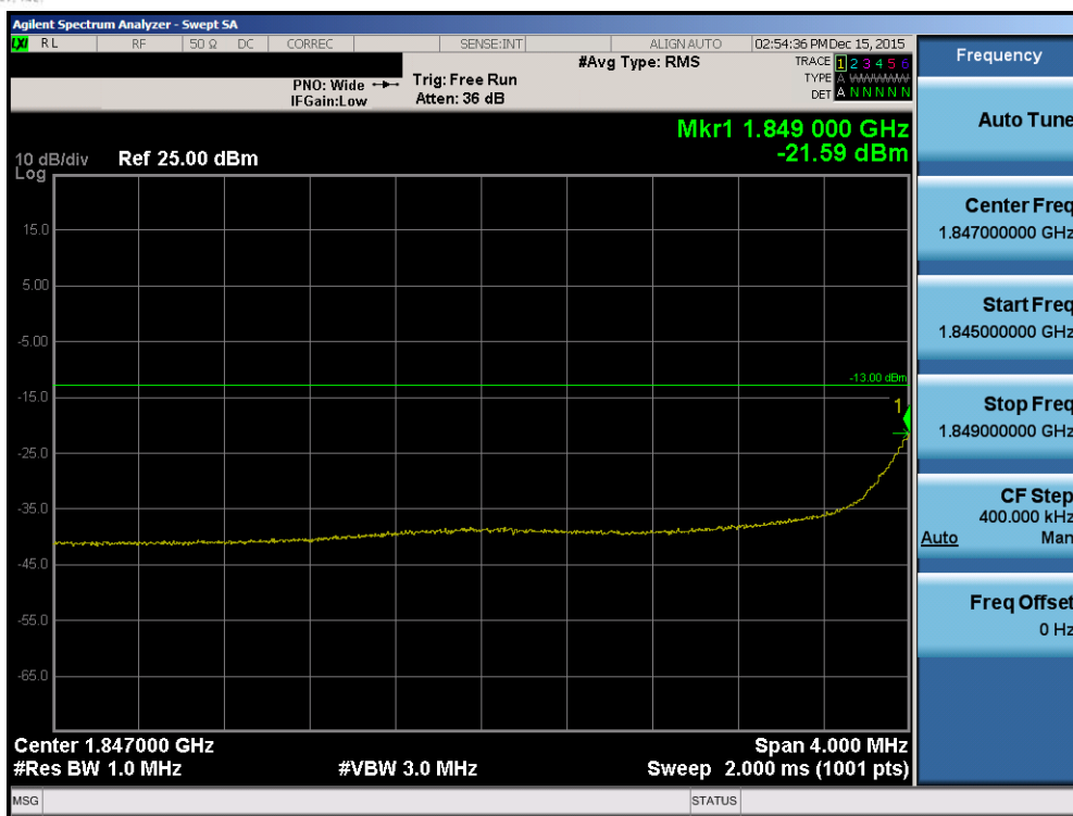
Plot 7-182. Lower Extended Band Edge Plot (Band2/25 – 1.4MHz QPSK – RB Size 6)
