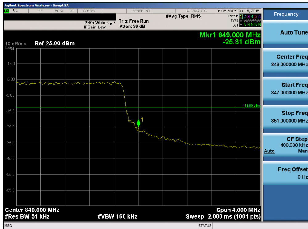
Plot 7-151. Upper Band Edge Plot (Band 26 – 5.0MHz QPSK – RB Size 25)
