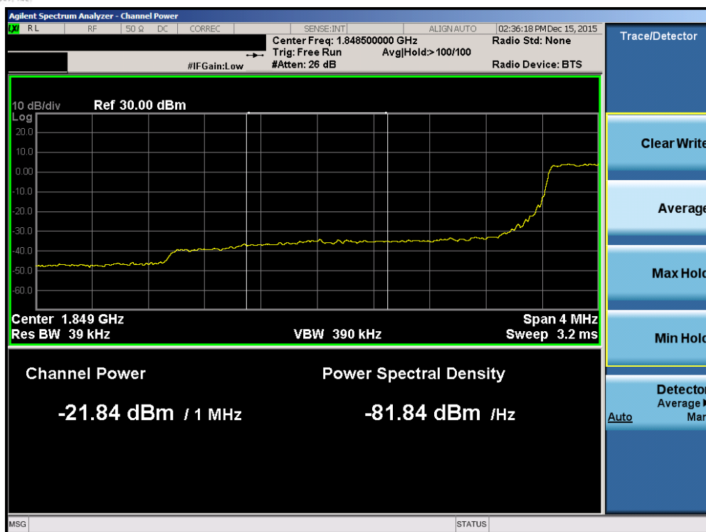
Plot 7-186. Lower Extended Band Edge Plot (Band2/25 – 3.0MHz QPSK – RB Size 15)
