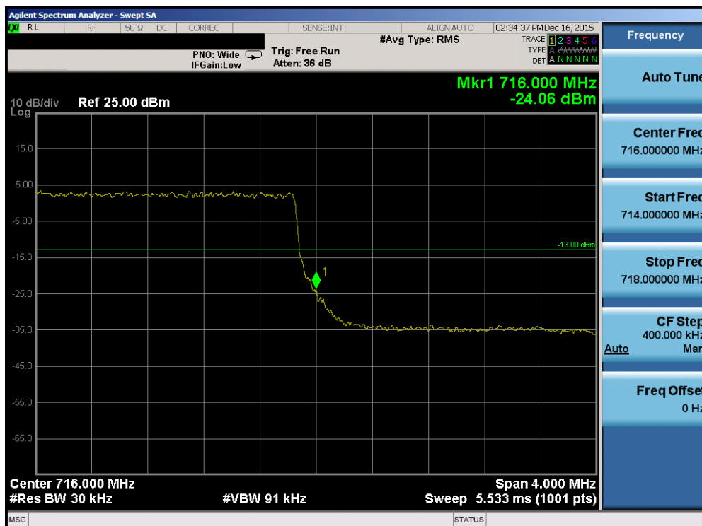
Plot 7-119. Upper Band Edge Plot (Band 12 – 3.0MHz QPSK – RB Size 15)
