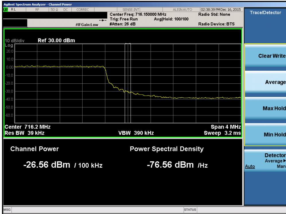
Plot 7-124. Upper Extended Band Edge Plot (Band 12/17 – 5.0MHz QPSK – RB Size 25)
