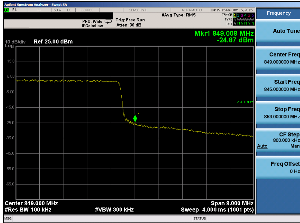
Plot 7-154. Upper Band Edge Plot (Band 26 – 10.0MHz QPSK – RB Size 50)
