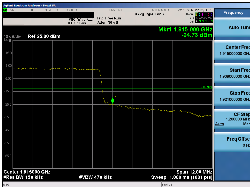
Plot 7-199. Upper Band Edge Plot (Band2/25 – 15.0MHz QPSK – RB Size 75)
