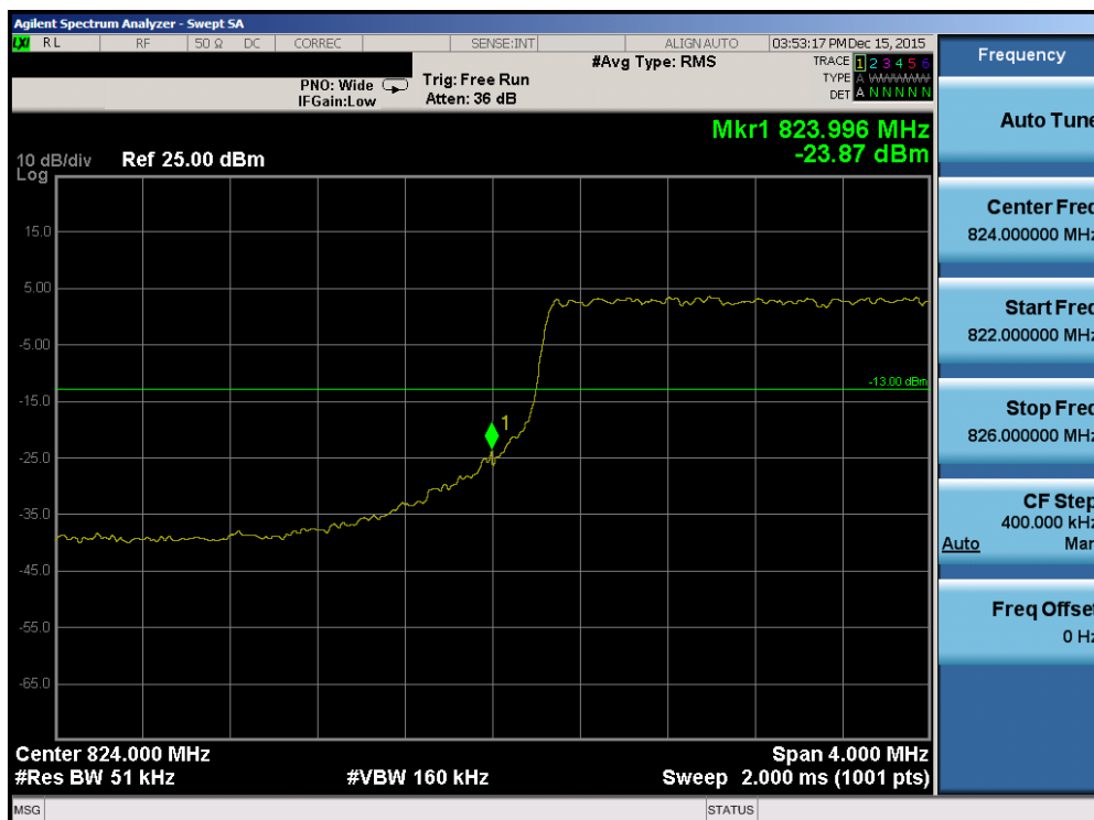
Plot 7-149. Lower Band Edge Plot (Band 26 – 5.0MHz QPSK – RB Size 25)
