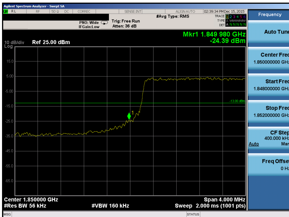
Plot 7-189. Lower Band Edge Plot (Band2/25 – 5.0MHz QPSK – RB Size 25)
