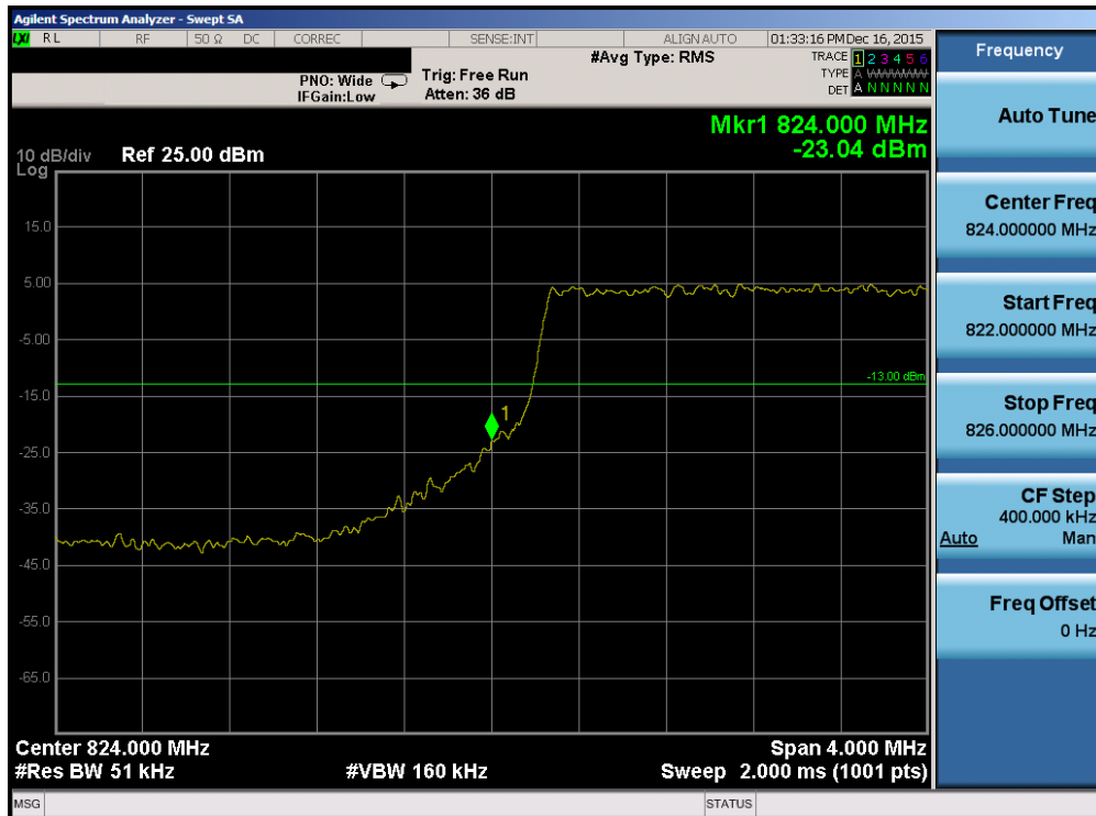
Plot 7-135. Lower Band Edge Plot (Band 5 – 5.0MHz QPSK – RB Size 25)
