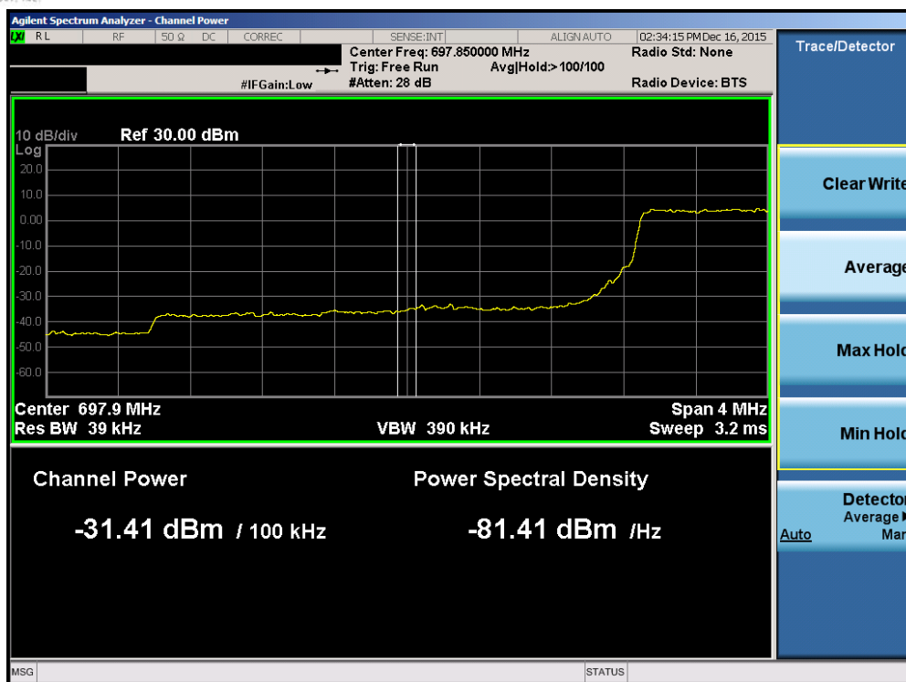
Plot 7-118. Lower Extended Band Edge Plot (Band 12 – 3.0MHz QPSK – RB Size 15)
