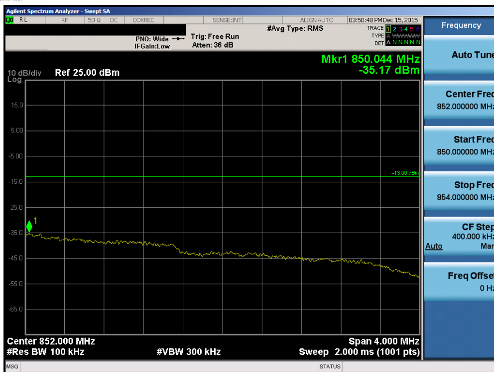
Plot 7-148. Upper Extended Band Edge Plot (Band 26 – Band 5 – 3.0MHz QPSK – RB Size 15)
