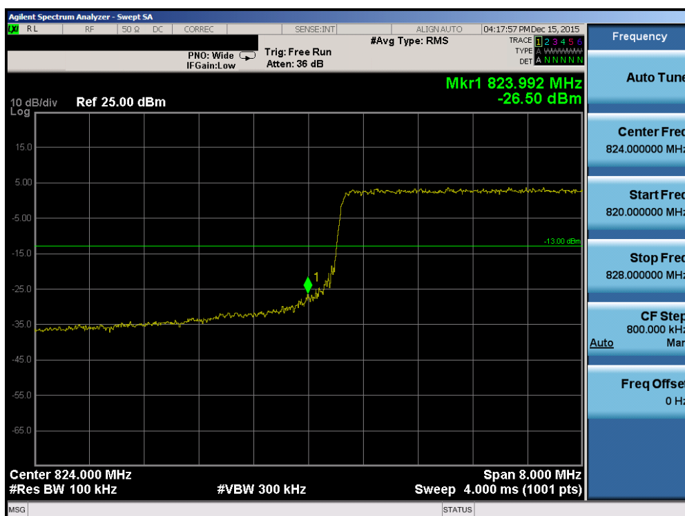
Plot 7-153. Lower Band Edge Plot (Band 26 – 10.0MHz QPSK – RB Size 50)
