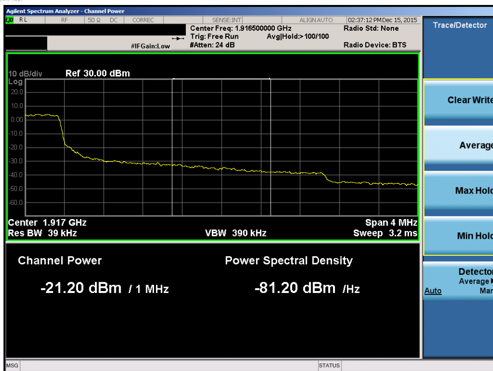
Plot 7-188. Upper Extended Band Edge Plot (Band2/25 – 3.0MHz QPSK – RB Size 15)
