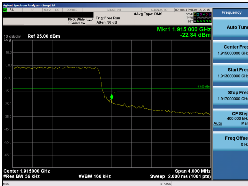
Plot 7-191. Upper Band Edge Plot (Band2/25 – 5.0MHz QPSK – RB Size 25)
