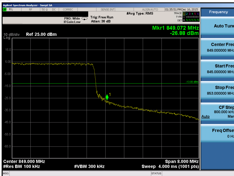
Plot 7-140. Upper Band Edge Plot (Band 5 – 10.0MHz QPSK – RB Size 50)
