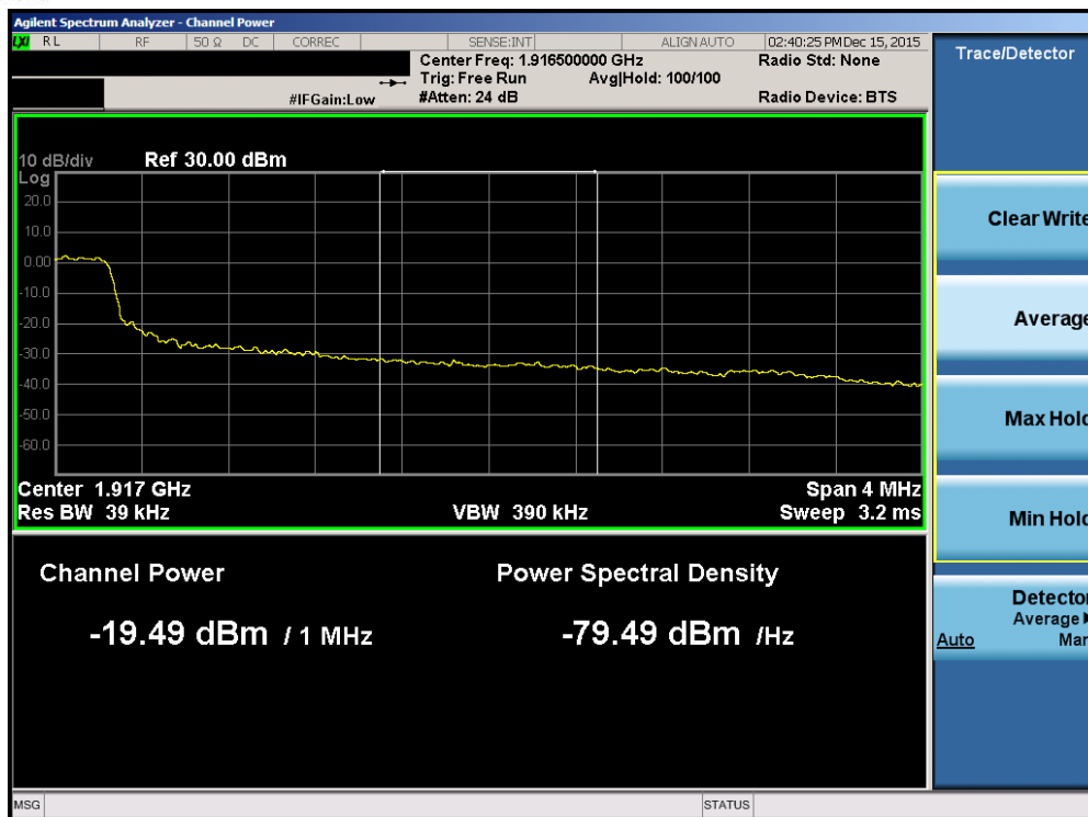
Plot 7-192. Upper Extended Band Edge Plot (Band2/25 – 5.0MHz QPSK – RB Size 25)
