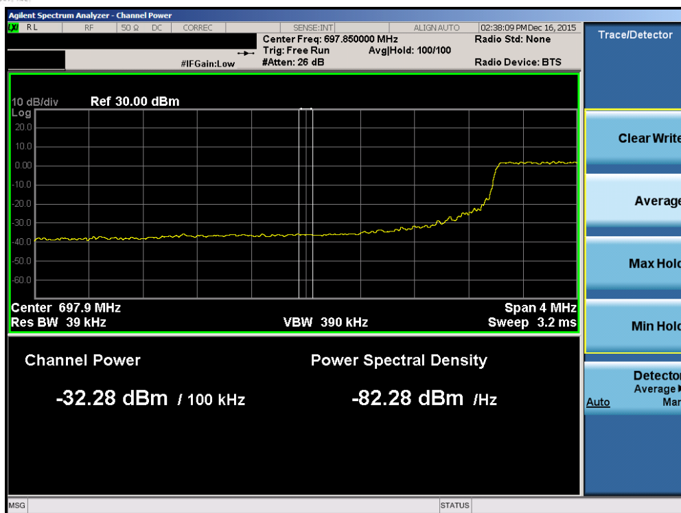
Plot 7-122. Lower Extended Band Edge Plot (Band 12/17 – 5.0MHz QPSK – RB Size 25)
