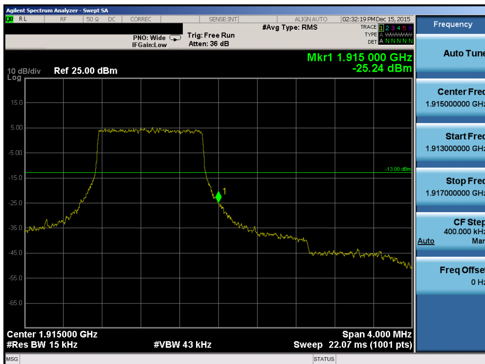
Plot 7-183. Upper Band Edge Plot (Band2/25 – 1.4MHz QPSK – RB Size 6)
