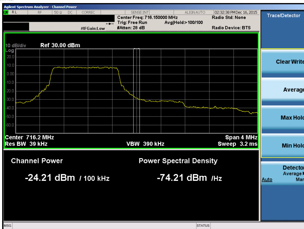
Plot 7-116. Upper Extended Band Edge Plot (Band 12 – 1.4MHz QPSK – RB Size 6)
