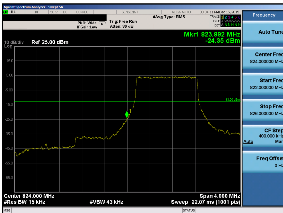
Plot 7-141. Lower Band Edge Plot (Band 26 – 1.4MHz QPSK – RB Size 6)
