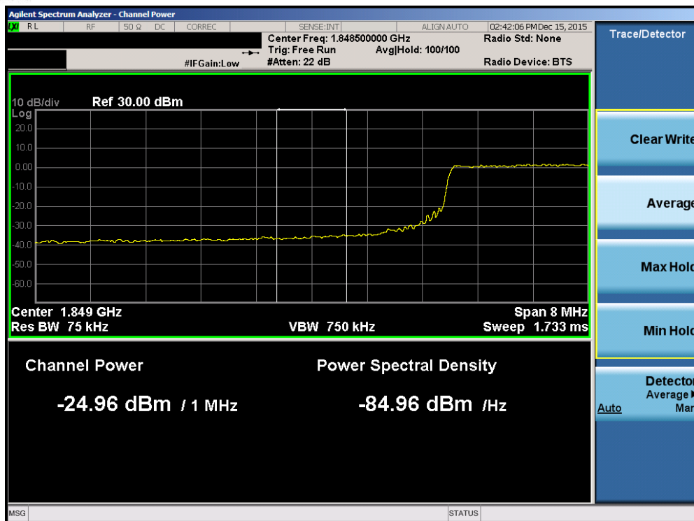
Plot 7-194. Lower Extended Band Edge Plot (Band2/25 – 10.0MHz QPSK – RB Size 50)
