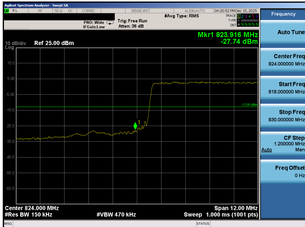
Plot 7-155. Lower Band Edge Plot (Band 26 – 15.0MHz QPSK – RB Size 75)
