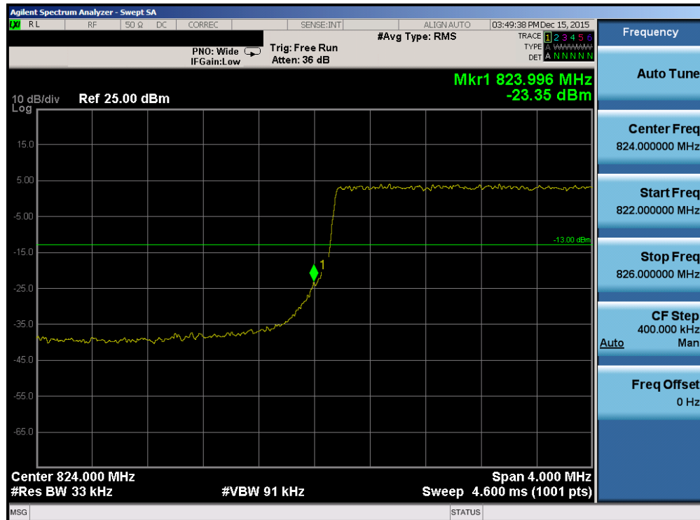
Plot 7-145. Lower Band Edge Plot (Band 26 – 3.0MHz QPSK – RB Size 15)
