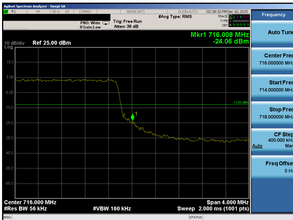
Plot 7-123. Upper Band Edge Plot (Band 12/17 – 5.0MHz QPSK – RB Size 25)
