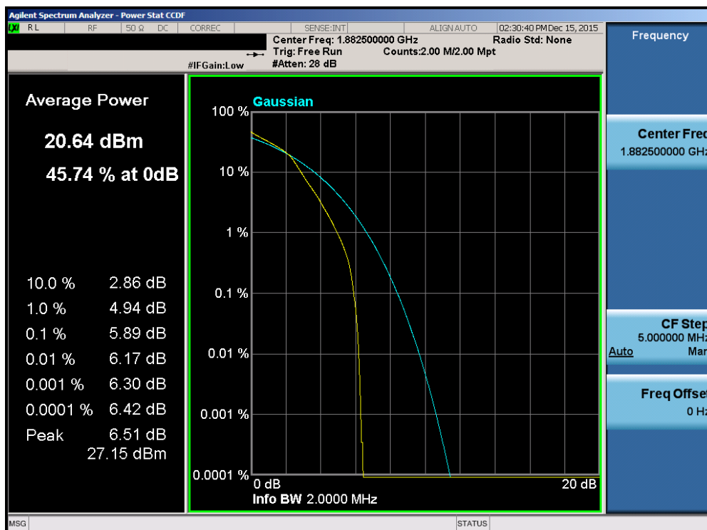
Plot 7-214. PAR Plot (Band2/25 – 1.4MHz 16-QAM – RB Size 6)
