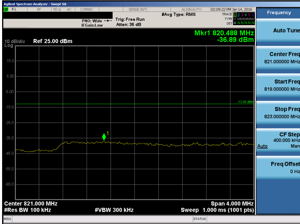
Plot 7-136. Lower Extended Band Edge Plot (Band 5 – 5.0MHz QPSK – RB Size 25)
