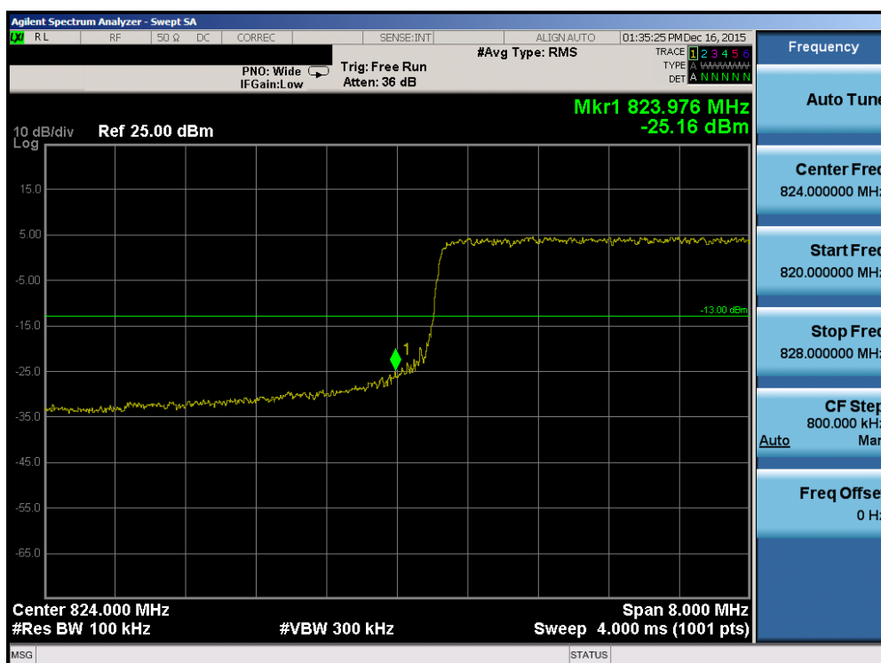
Plot 7-139. Lower Band Edge Plot (Band 5 – 10.0MHz QPSK – RB Size 50)
