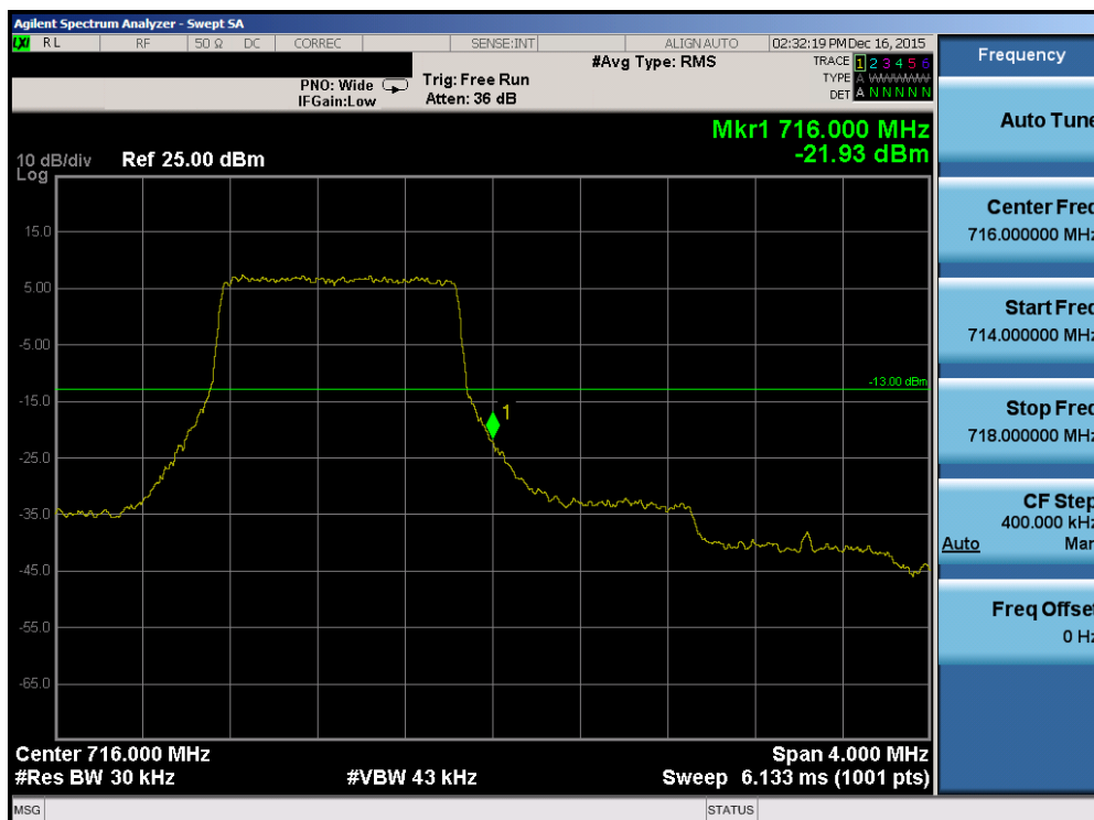
Plot 7-115. Upper Band Edge Plot (Band 12 – 1.4MHz QPSK – RB Size 6)
