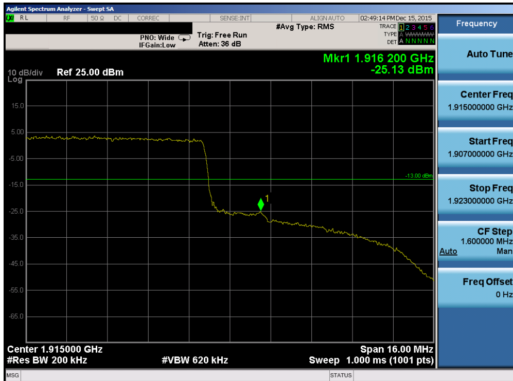
Plot 7-203. Upper Band Edge Plot (Band2/25 – 20.0MHz QPSK – RB Size 100)
