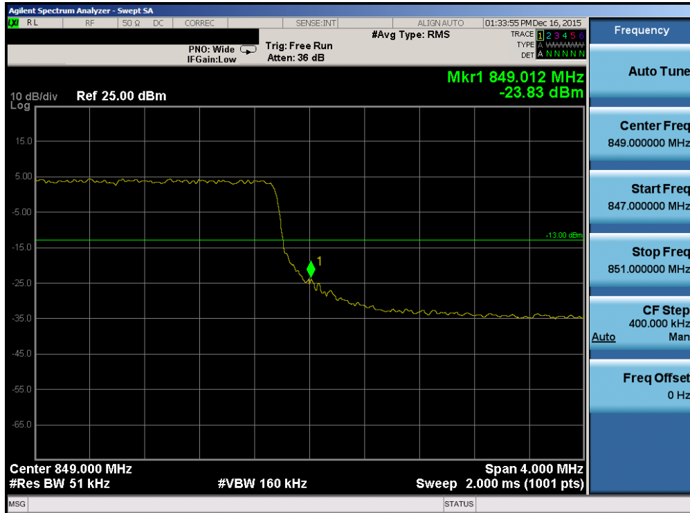
Plot 7-137. Upper Band Edge Plot (Band 5 – 5.0MHz QPSK – RB Size 25)
