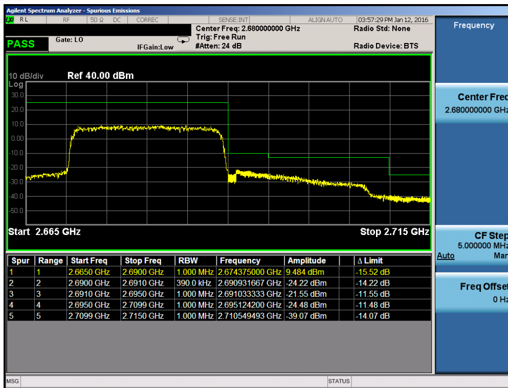
Plot 7-212. Upper ACP Plot (Band 41 – 20.0MHz QPSK – RB Size 100)
