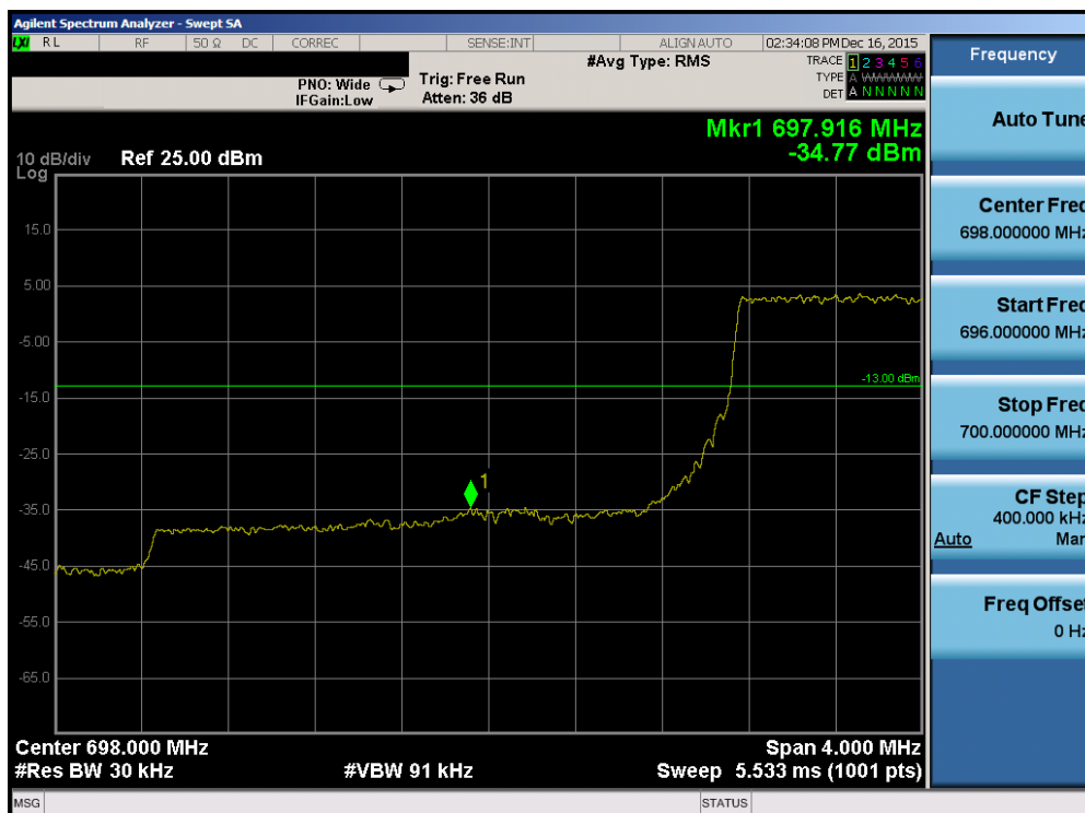
Plot 7-117. Lower Band Edge Plot (Band 12 – 3.0MHz QPSK – RB Size 15)
