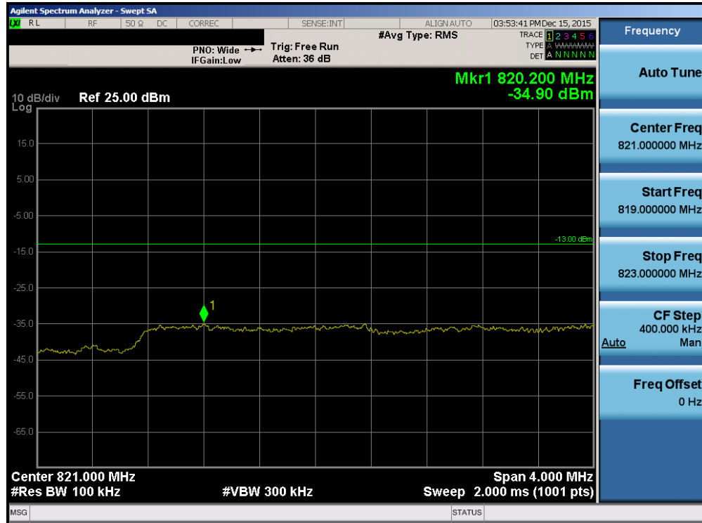
Plot 7-150. Lower Extended Band Edge Plot (Band 26 – 5.0MHz QPSK – RB Size 25)
