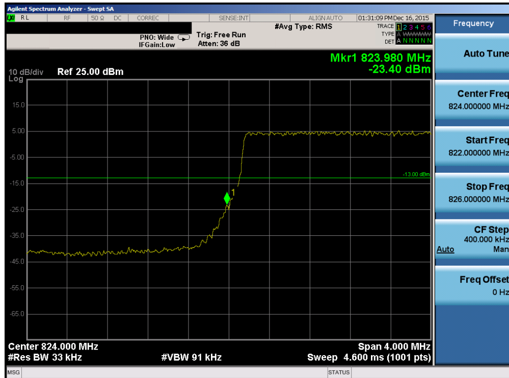
Plot 7-131. Lower Band Edge Plot (Band 5 – 3.0MHz QPSK – RB Size 15)
