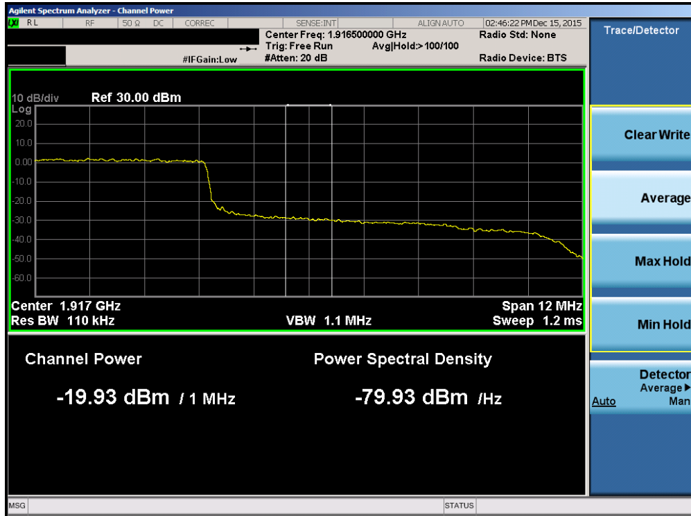
Plot 7-200. Upper Extended Band Edge Plot (Band2/25 – 15.0MHz QPSK – RB Size 75)
