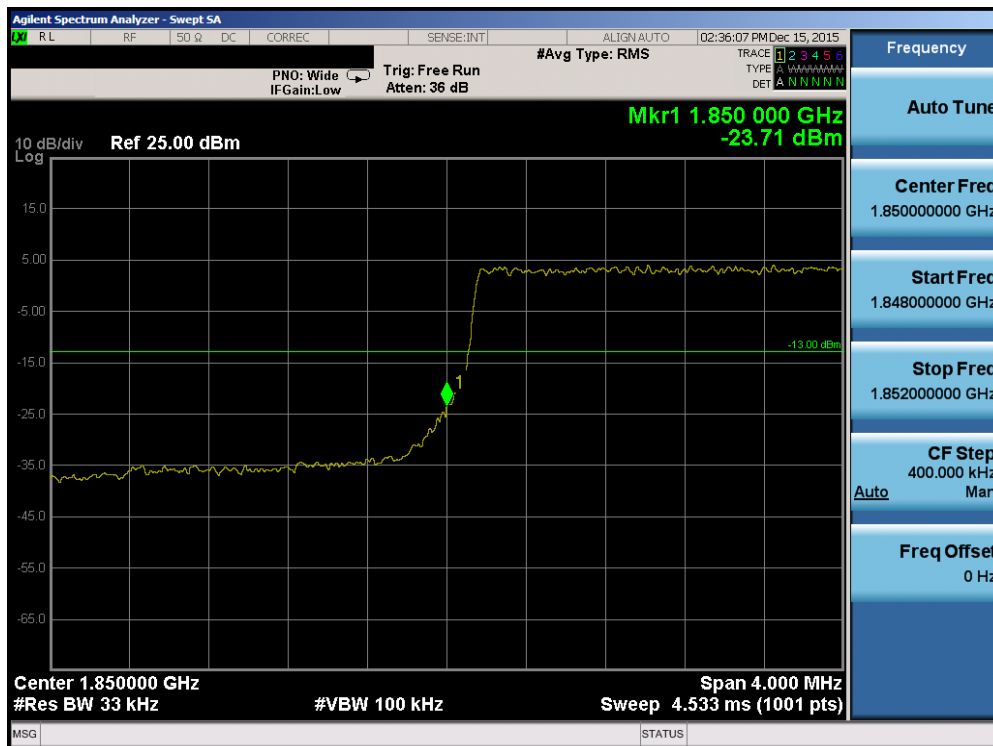
Plot 7-185. Lower Band Edge Plot (Band2/25 – 3.0MHz QPSK – RB Size 15)
