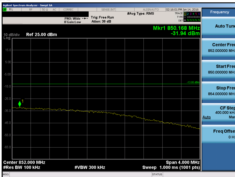
Plot 7-138. Upper Extended Band Edge Plot (Band 5 – 5.0MHz QPSK – RB Size 25)
