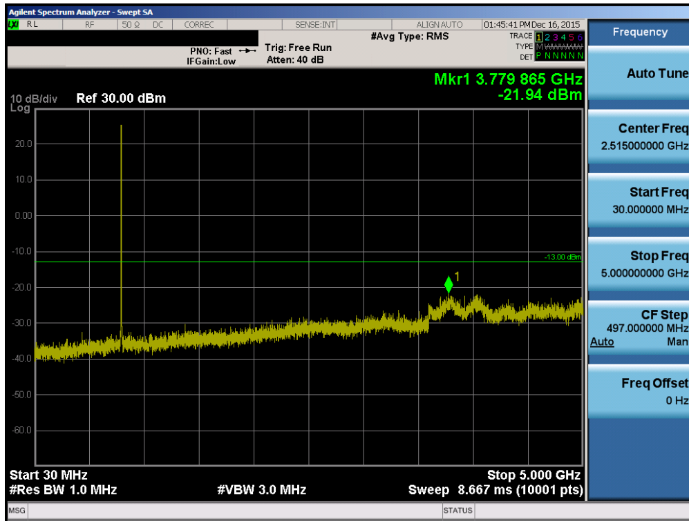
Plot 7-9. Conducted Spurious Plot ( 3MHz QPSK – RB Size 1, RB Offset 0 – Low Channel)
