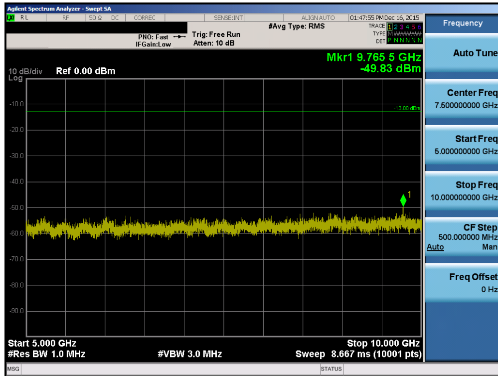
Plot 7-12. Conducted Spurious Plot ( 3MHz QPSK – RB Size 1, RB Offset 0 – High Channel)
