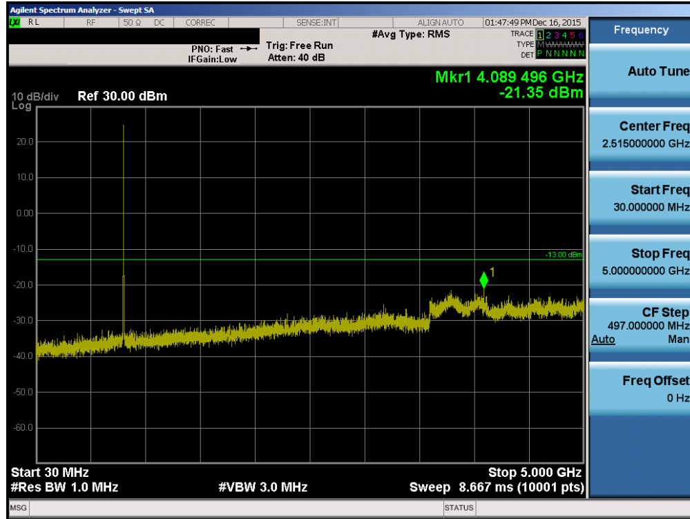
Plot 7-11. Conducted Spurious Plot ( 3MHz QPSK – RB Size 1, RB Offset 0 – High Channel)
