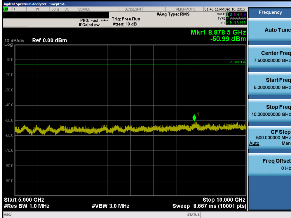
Plot 7-10. Conducted Spurious Plot ( 3MHz QPSK – RB Size 1, RB Offset 0 – Low Channel)
