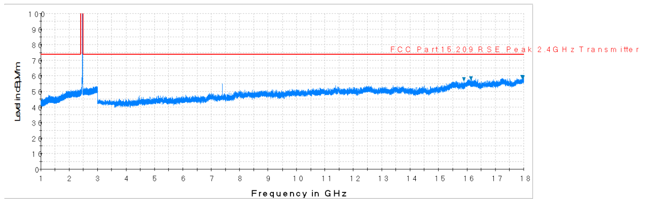
Plot 7-73. Radiated Spurious Plot above 1GHz (802.11b – Ch. 11, Ant. Pol. H)
