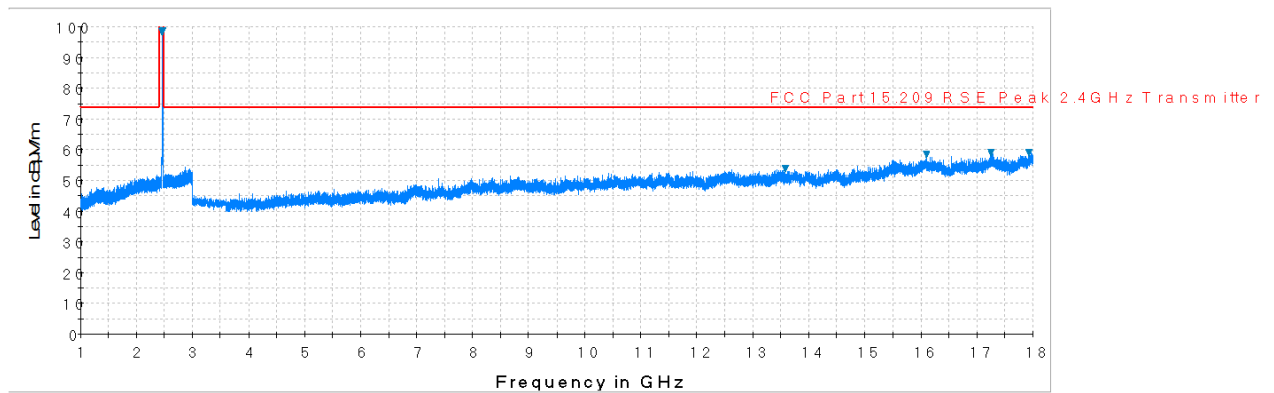
Plot 7-65. Radiated Spurious Plot above 1GHz (802.11b – Ch. 11, Ant. Pol. H)
