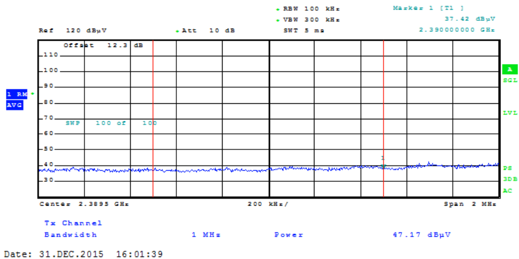
Plot A4-1. Radiated Restricted Lower Band Edge Measurement (Average)
