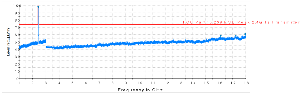
Plot 7-64. Radiated Spurious Plot above 1GHz (802.11b – Ch. 6, Ant. Pol. V)
