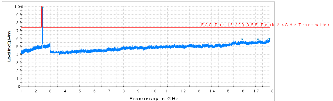
Plot 7-66. Radiated Spurious Plot above 1GHz (802.11b – Ch. 11, Ant. Pol. V)
