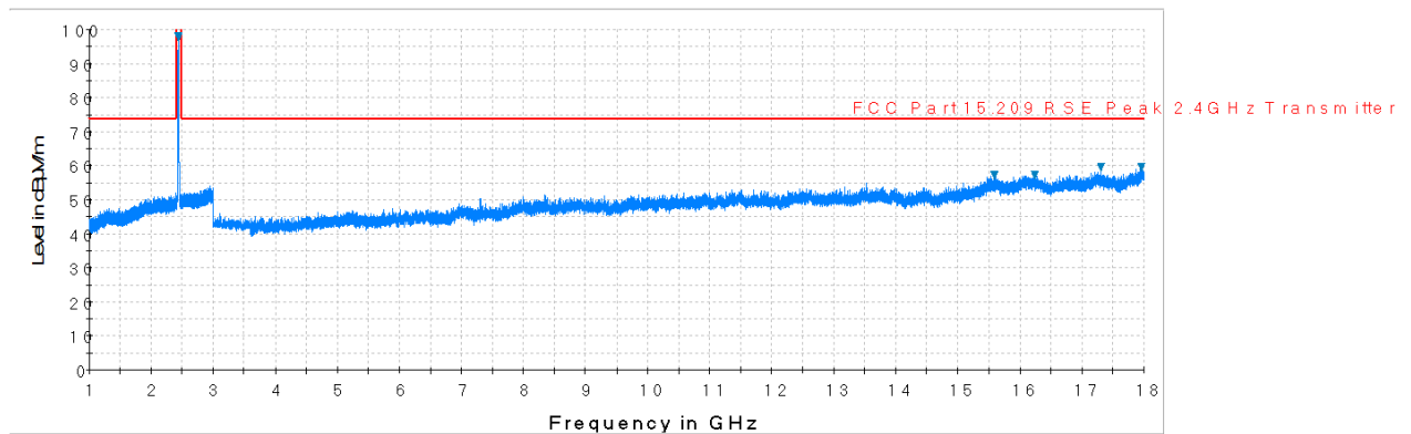
Plot 7-63. Radiated Spurious Plot above 1GHz (802.11b – Ch. 6, Ant. Pol. H)
