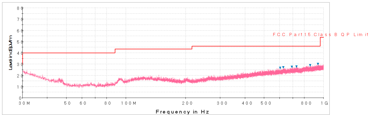
Plot 7-98. Radiated Spurious Plot below 1GHz (Pol. V)
