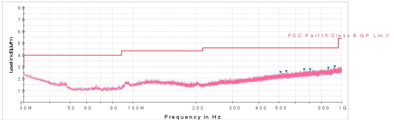
Plot 7-97. Radiated Spurious Plot below 1GHz (Pol. H)
