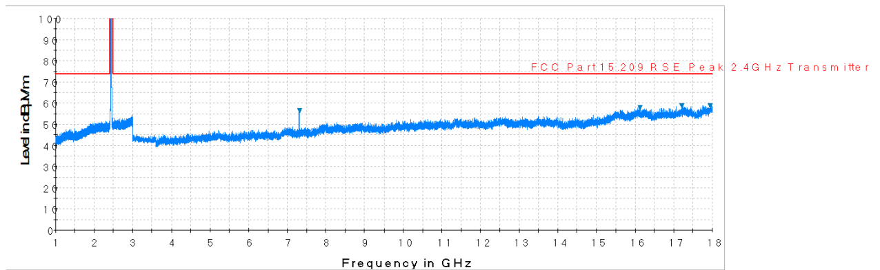
Plot 7-71. Radiated Spurious Plot above 1GHz (802.11b – Ch. 6, Ant. Pol. H)
