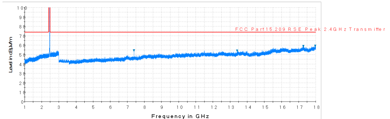
Plot 7-74. Radiated Spurious Plot above 1GHz (802.11b – Ch. 11, Ant. Pol. V)
