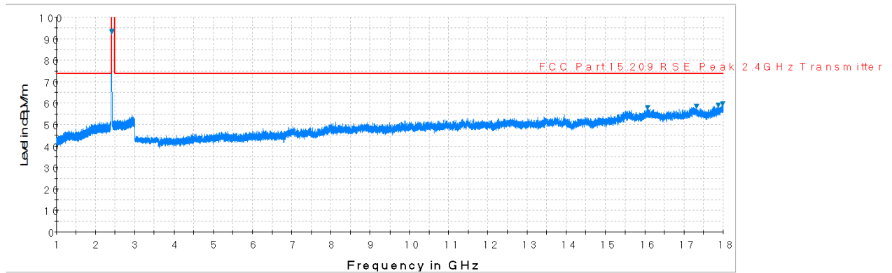
Plot 7-61. Radiated Spurious Plot above 1GHz (802.11b – Ch. 1, Ant. Pol. H)
