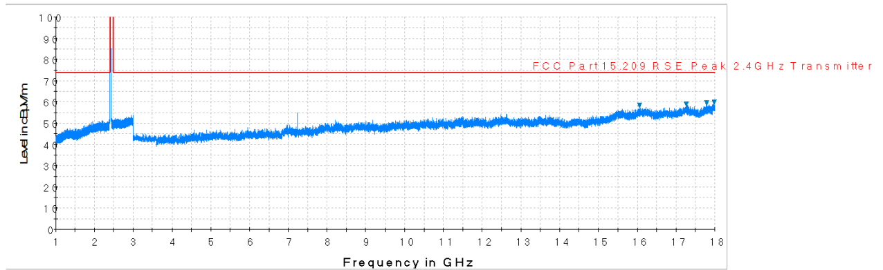
Plot 7-69. Radiated Spurious Plot above 1GHz (802.11b – Ch. 1, Ant. Pol. H)
