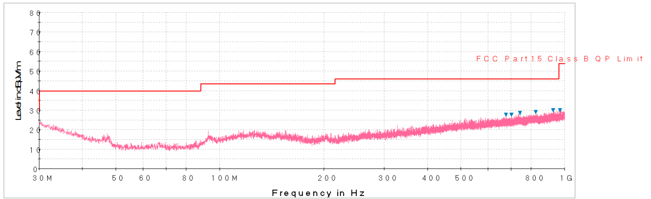
Plot 7-95. Radiated Spurious Plot below 1GHz (Pol. H)
