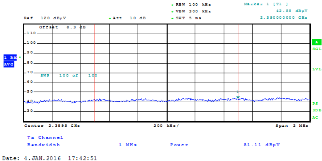
Plot 7-93. Radiated Restricted Band Edge Measurement with WCP (Average)
