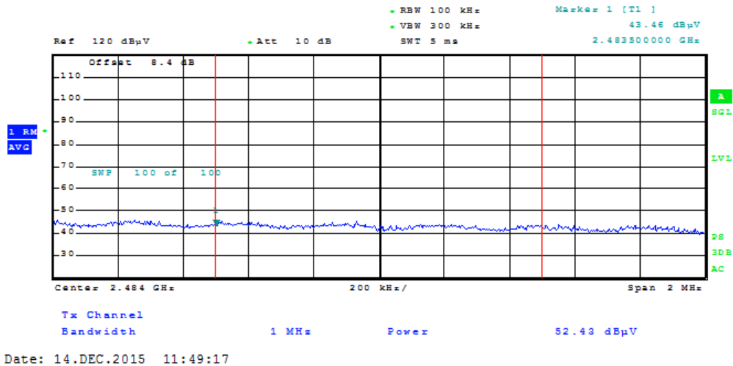
Plot 7-85. Radiated Restricted Upper Band Edge Measurement (Average)
