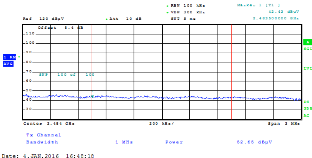
Plot 7-87. Radiated Restricted Band Edge Measurement with WCP (Average)
