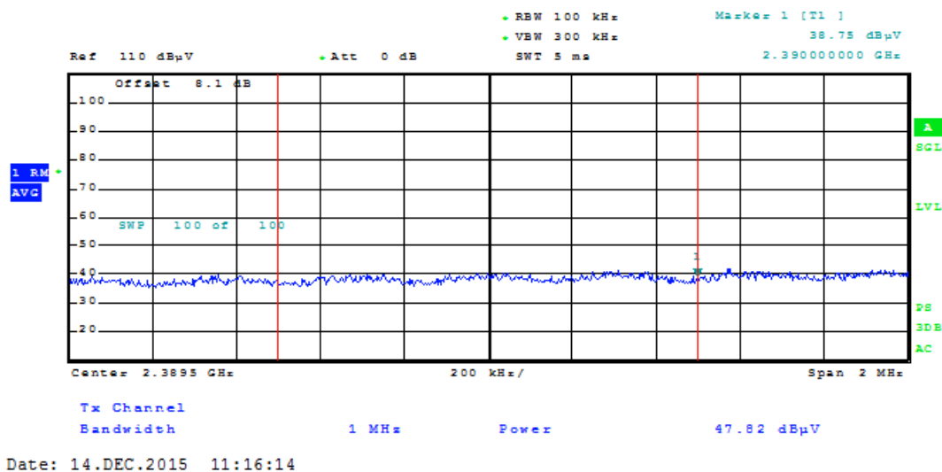
Plot 7-83. Radiated Restricted Lower Band Edge Measurement (Average)
