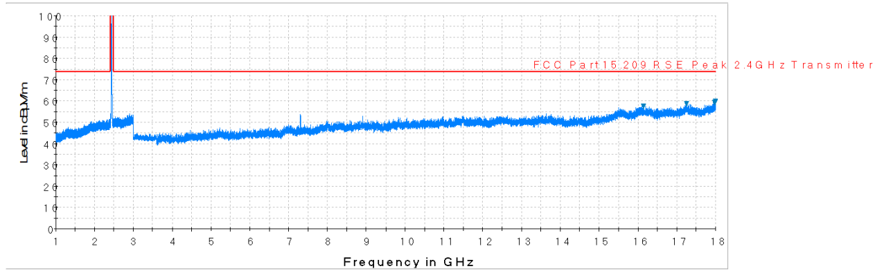
Plot 7-72. Radiated Spurious Plot above 1GHz (802.11b – Ch. 6, Ant. Pol. V)
