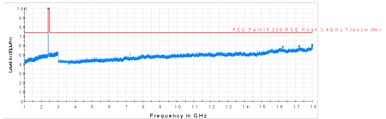
Plot 7-70. Radiated Spurious Plot above 1GHz (802.11b – Ch. 1, Ant. Pol. V)
