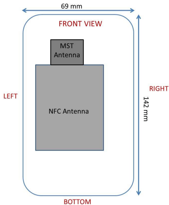
Figure F-1 DUT Antenna Locations
