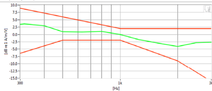
Frequency Response
