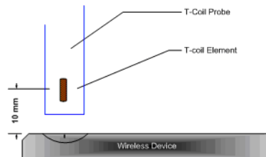
Figure 5-10 Measurement Distance
