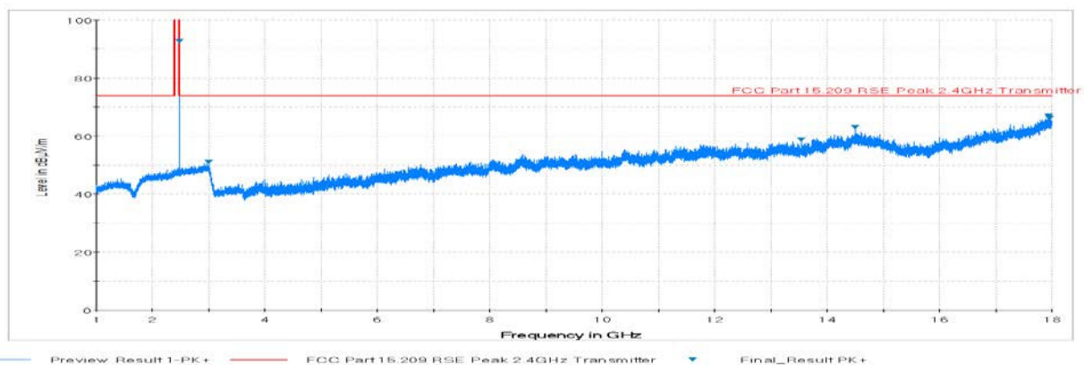
Plot 22. Radiated Spurious Plot above 1GHz (BT LE – Ch. 39, Ant. Pol. H)
