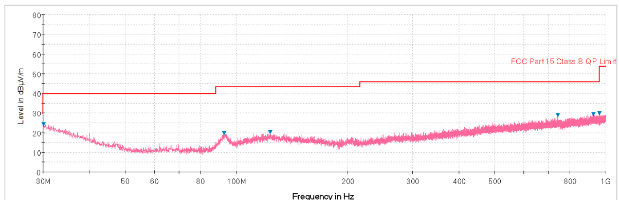
Plot 30. Radiated Spurious Plot below 1GHz (Pol. H)
