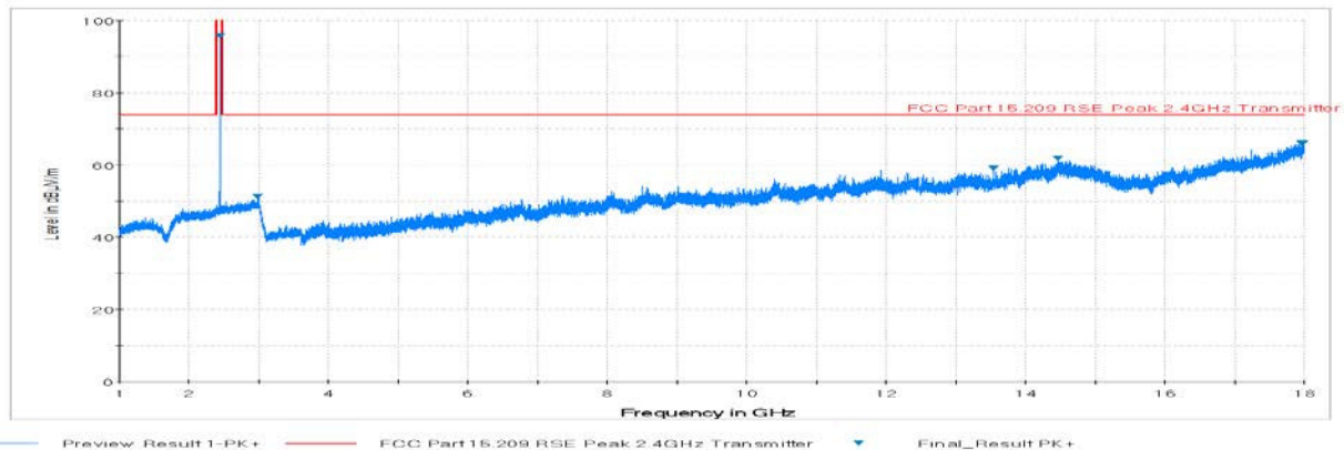
Plot 21. Radiated Spurious Plot above 1GHz (BT LE – Ch. 19, Ant. Pol. V)
