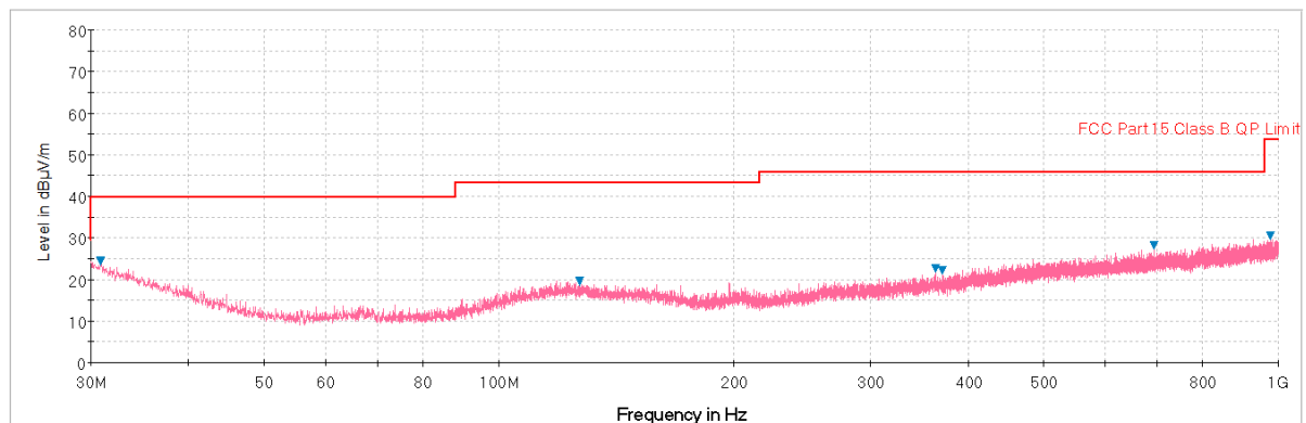
Plot 31. Radiated Spurious Plot below 1GHz (Pol. V)
