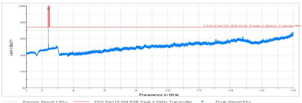
Plot 19. Radiated Spurious Plot above 1GHz (BT LE – Ch. 0, Ant. Pol. V)
