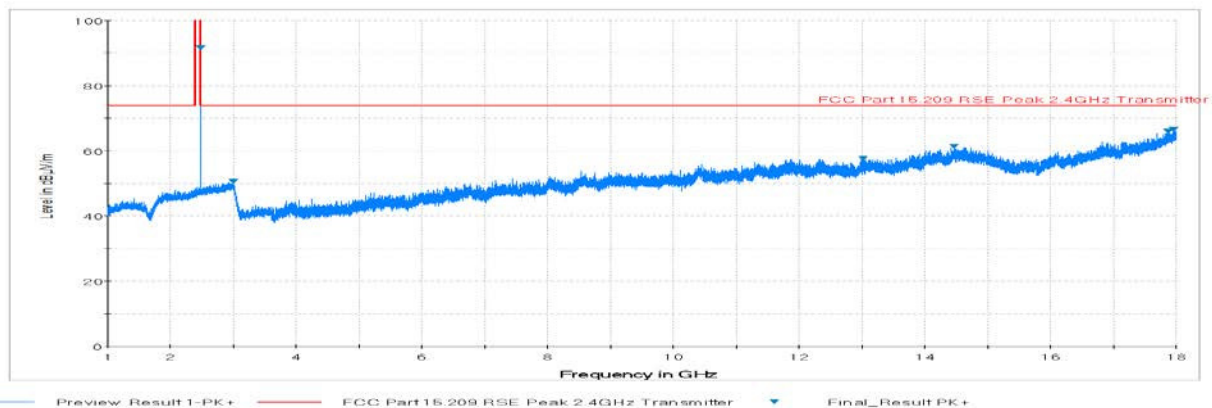
Plot 23. Radiated Spurious Plot above 1GHz (BT LE - Ch. 39, Ant. Pol. V)
