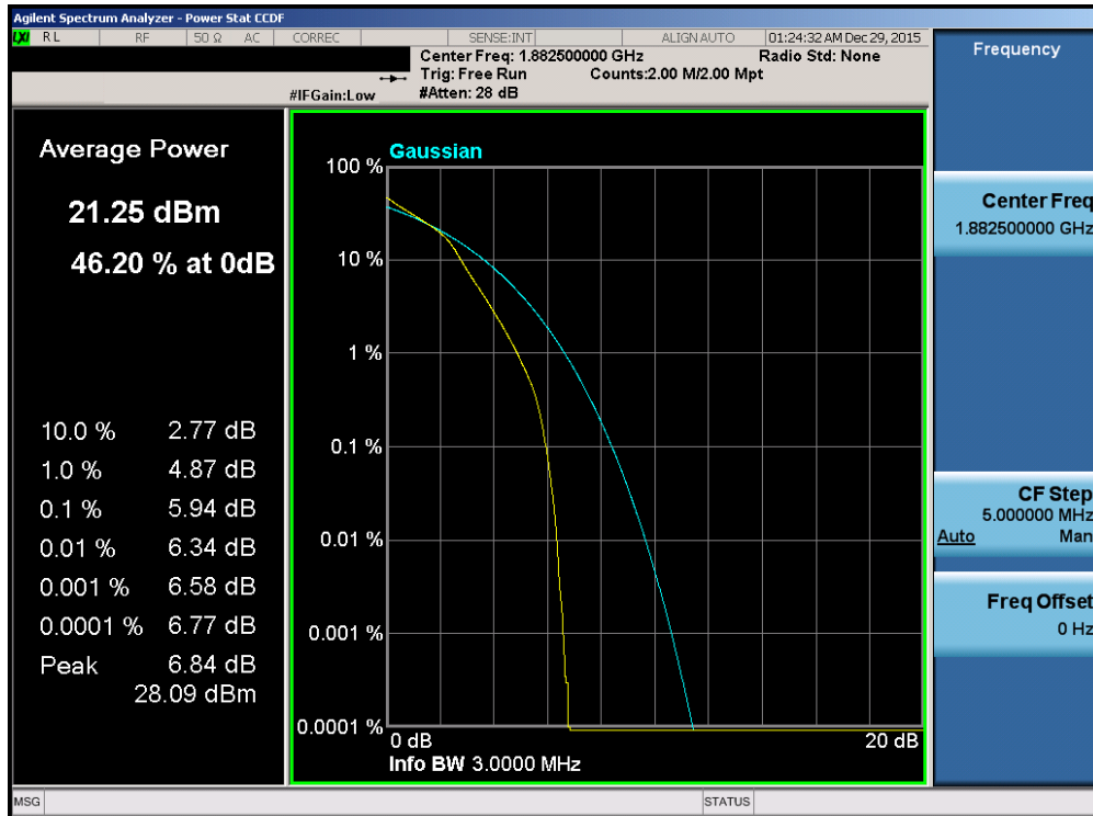
Plot 7-239. PAR Plot (Band 2/25 – 3.0MHz 16-QAM – RB Size 15)
