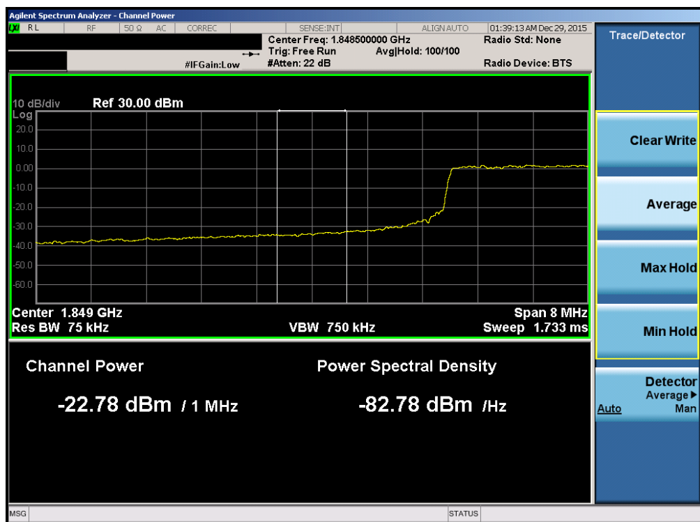
Plot 7-208. Lower Extended Band Edge Plot (Band 2/25 – 10.0MHz QPSK – RB Size 50)
