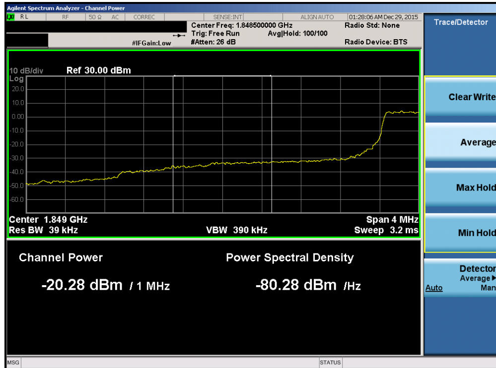
Plot 7-200. Lower Extended Band Edge Plot (Band 2/25 – 3.0MHz QPSK – RB Size 15)
