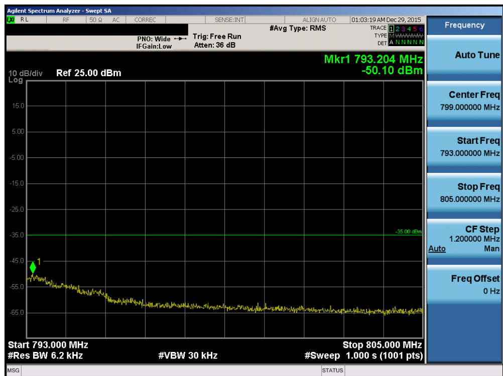
Plot 7-156. Upper Emission Mask Edge Plot (Band 13 – 10.0MHz QPSK – RB Size 50)
