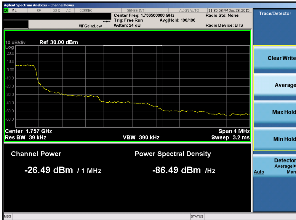
Plot 7-174. Upper Extended Band Edge Plot (Band 4 – 1.4MHz QPSK – RB Size 6)
