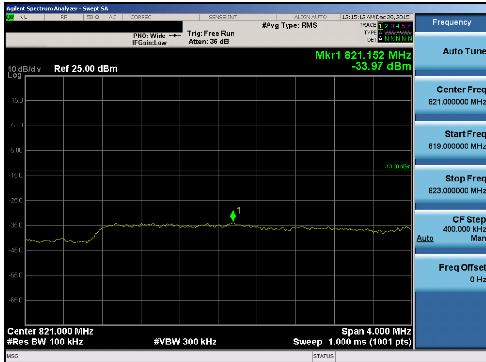
Plot 7-166. Lower Extended Band Edge Plot (Band 5 - 5.0MHz QPSK - RB Size 25)
