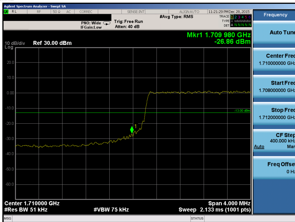
Plot 7-179. Lower Band Edge Plot (Band 4 – 5.0MHz QPSK – RB Size 25)
