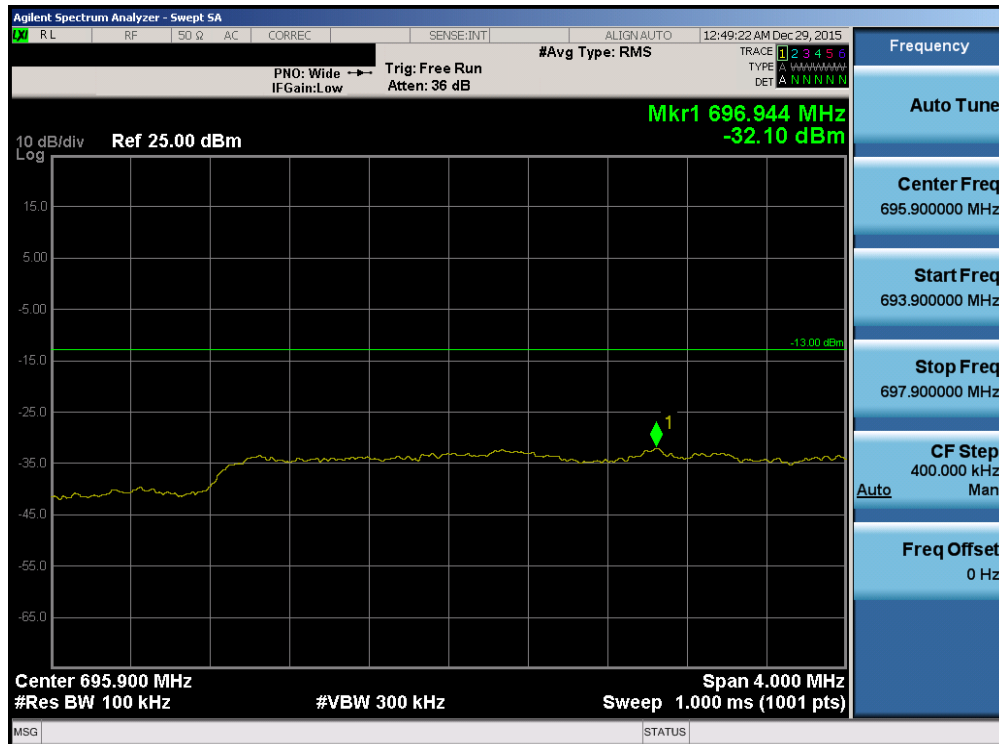
Plot 7-136. Lower Extended Band Edge Plot (Band 12 – 5.0MHz QPSK – RB Size 25)
