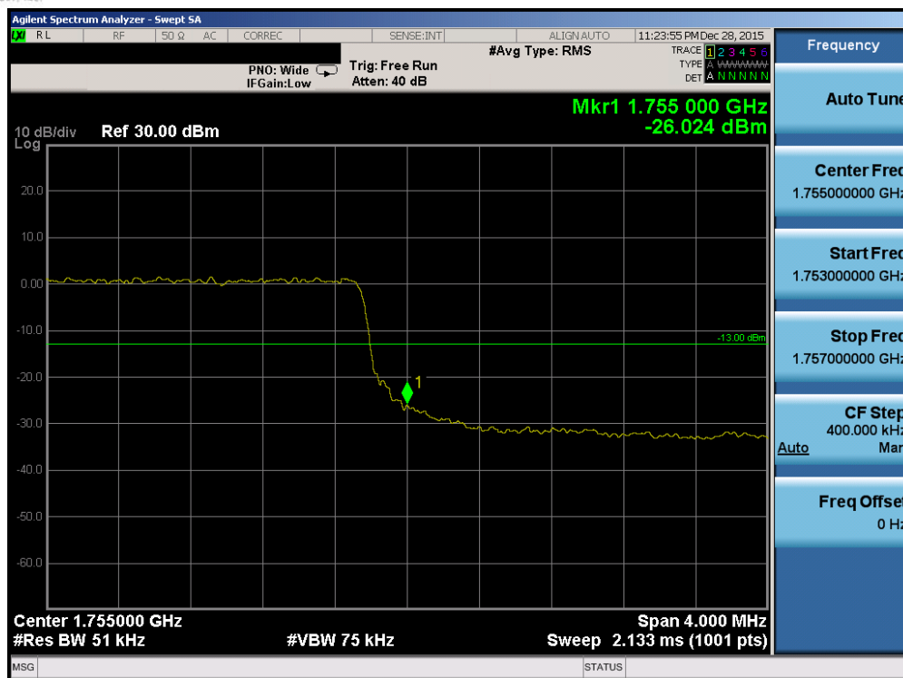
Plot 7-181. Upper Band Edge Plot (Band 4 – 5.0MHz QPSK – RB Size 25)
