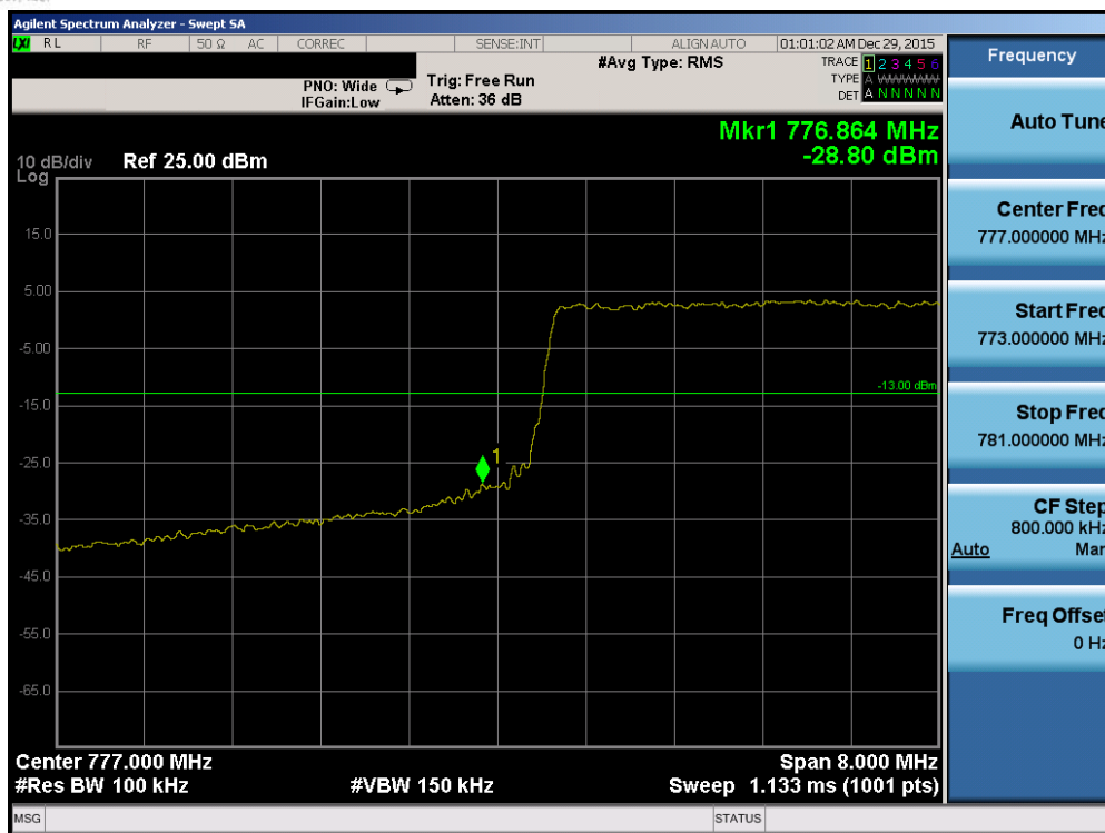
Plot 7-153. Lower Band Edge Plot (Band 13 – 10.0MHz QPSK – RB Size 50)
