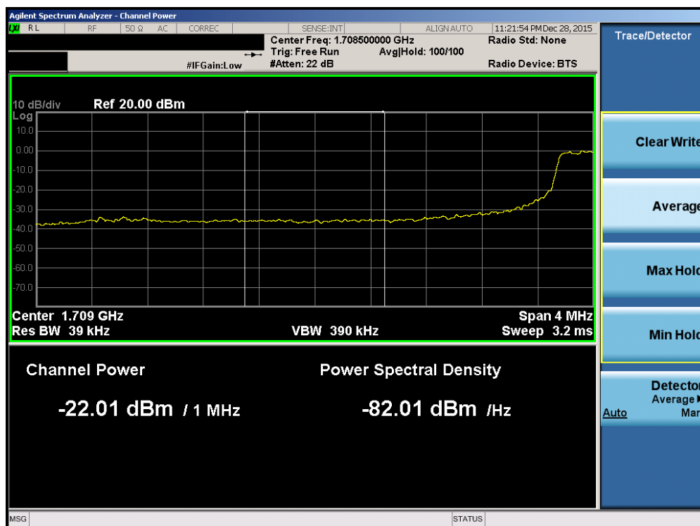
Plot 7-180. Lower Extended Band Edge Plot (Band 4 – 5.0MHz QPSK – RB Size 25)
