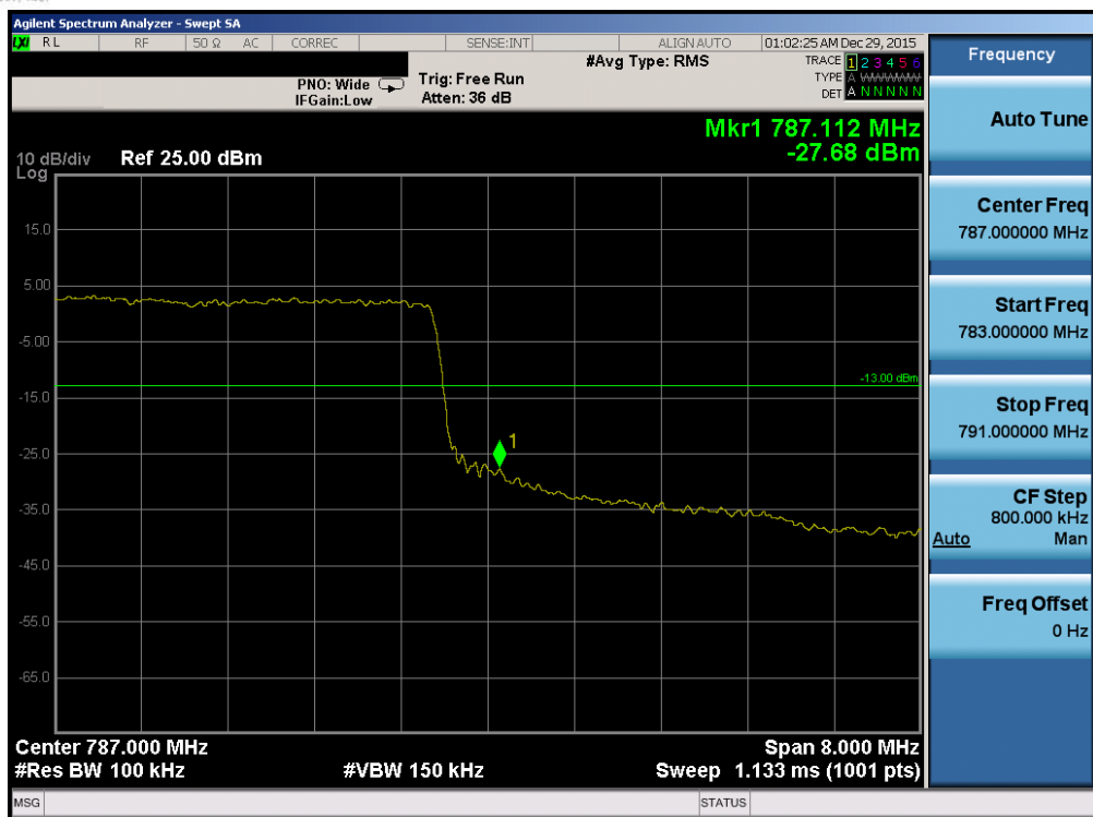
Plot 7-155. Upper Band Edge Plot (Band 13 – 10.0MHz QPSK – RB Size 50)
