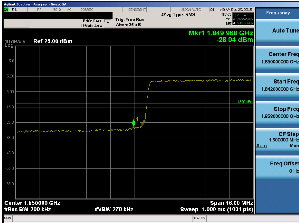
Plot 7-215. Lower Band Edge Plot (Band 2/25 – 20.0MHz QPSK – RB Size 100)
