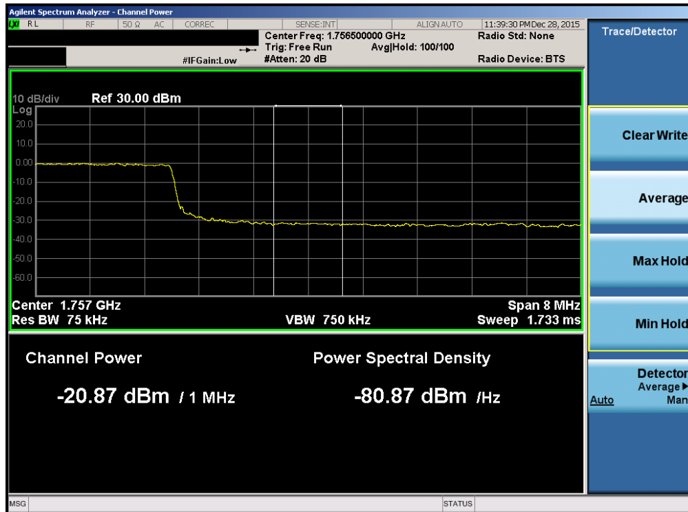
Plot 7-186. Upper Extended Band Edge Plot (Band 4 – 10.0MHz QPSK – RB Size 50)
