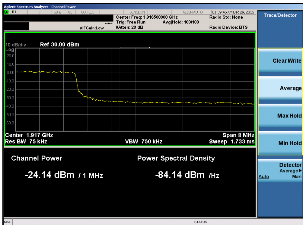
Plot 7-210. Upper Extended Band Edge Plot (Band 2/25 – 10.0MHz QPSK – RB Size 50)
