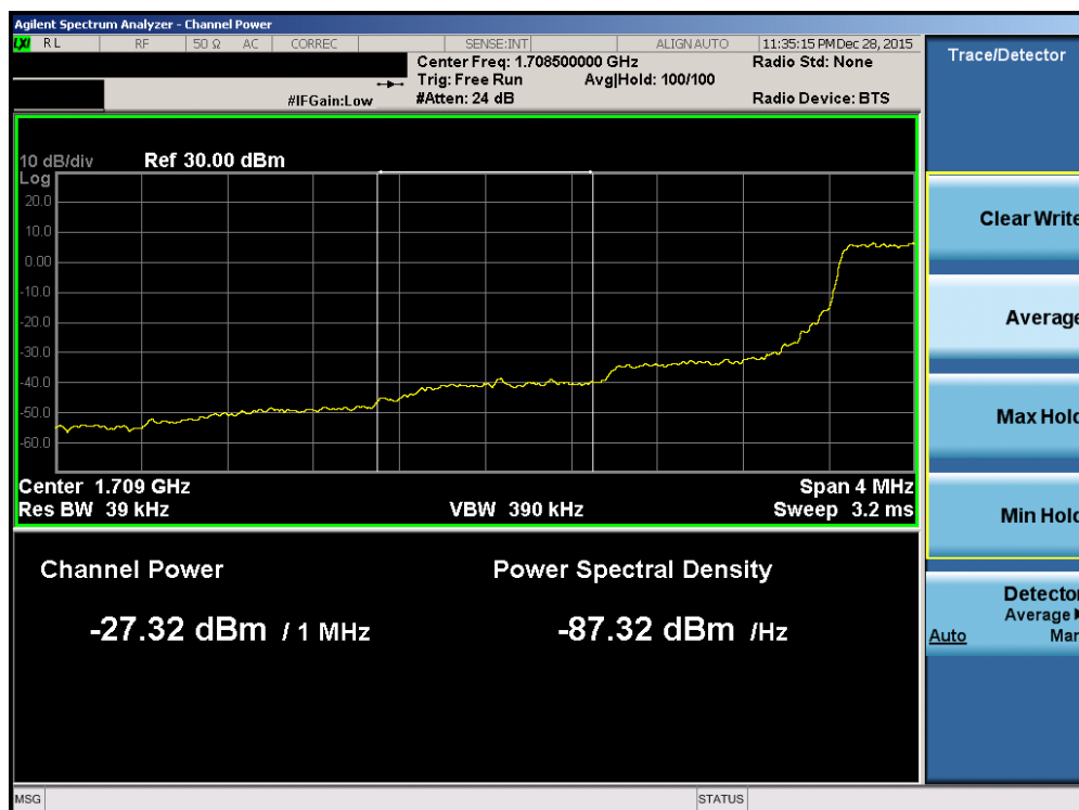
Plot 7-172. Lower Extended Band Edge Plot (Band 4 – 1.4MHz QPSK – RB Size 6)
