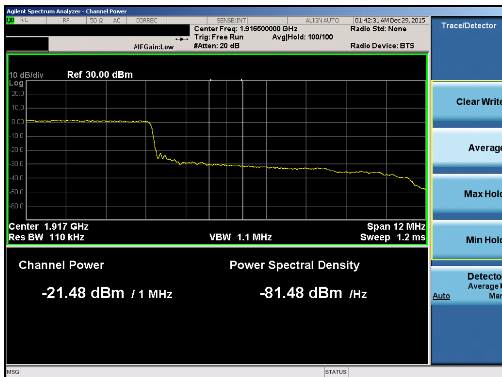
Plot 7-214. Upper Extended Band Edge Plot (Band 2/25 – 15.0MHz QPSK – RB Size 75)
