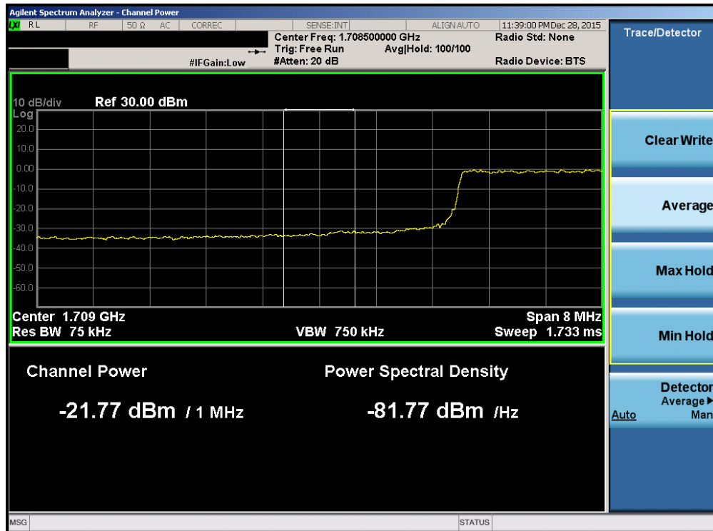
Plot 7-184. Lower Extended Band Edge Plot (Band 4 – 10.0MHz QPSK – RB Size 50)
