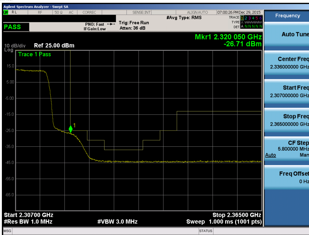
Plot 7-227. Upper Extended Band Edge Plot (Band 30 – 10.0MHz QPSK – RB Size 50)
