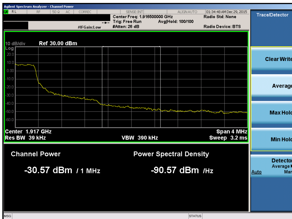
Plot 7-198. Upper Extended Band Edge Plot (Band 2/25 – 1.4MHz QPSK – RB Size 6)
