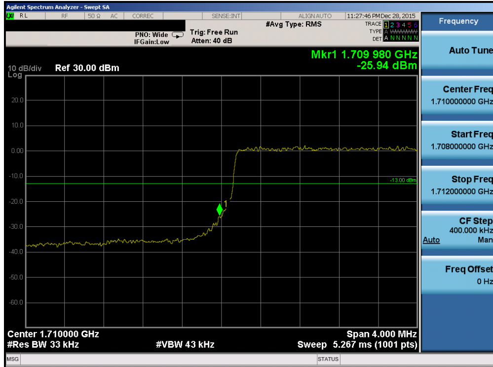
Plot 7-175. Lower Band Edge Plot (Band 4 – 3.0MHz QPSK – RB Size 15)
