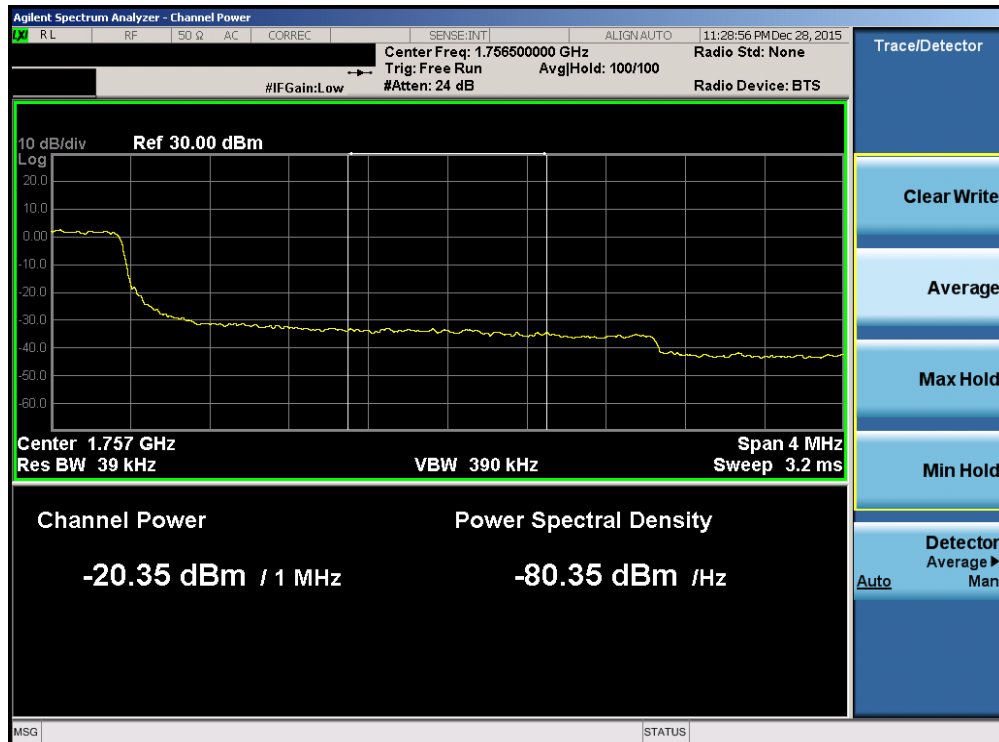
Plot 7-178. Upper Extended Band Edge Plot (Band 4 – 3.0MHz QPSK – RB Size 15)
