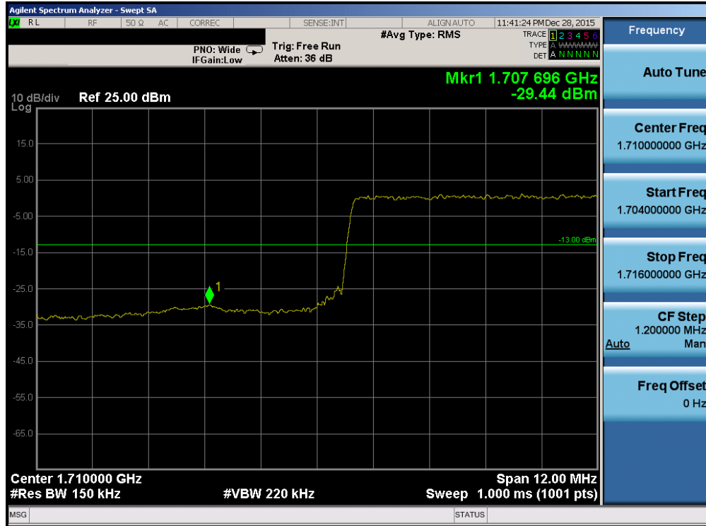
Plot 7-187. Lower Band Edge Plot (Band 4 – 15.0MHz QPSK – RB Size 75)
