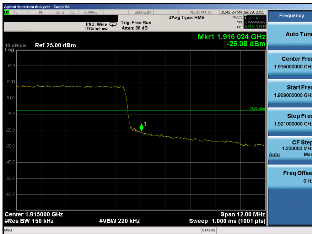
Plot 7-213. Upper Band Edge Plot (Band 2/25 – 15.0MHz QPSK – RB Size 75)
