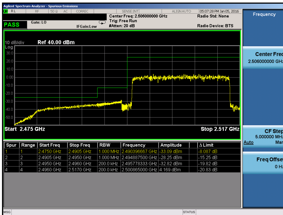
Plot 7-234. Lower ACP Plot (Band 41 – 20.0MHz QPSK – RB Size 100)
