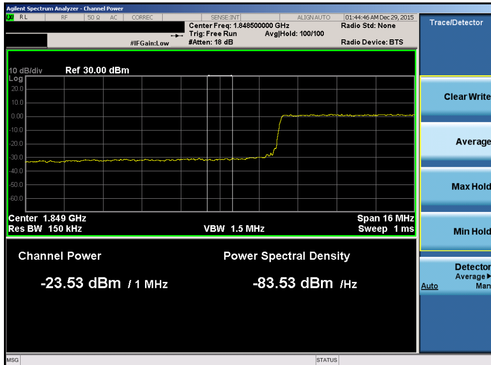
Plot 7-216. Lower Extended Band Edge Plot (Band 2/25 – 20.0MHz QPSK – RB Size 100)
