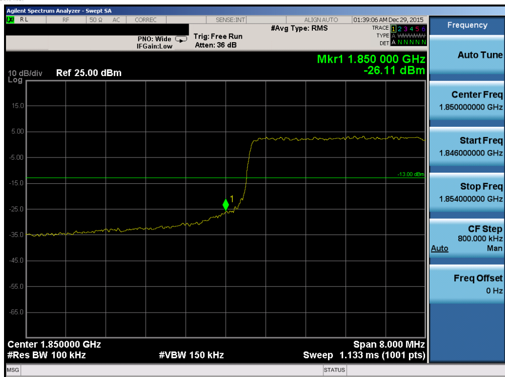
Plot 7-207. Lower Band Edge Plot (Band 2/25 – 10.0MHz QPSK – RB Size 50)
