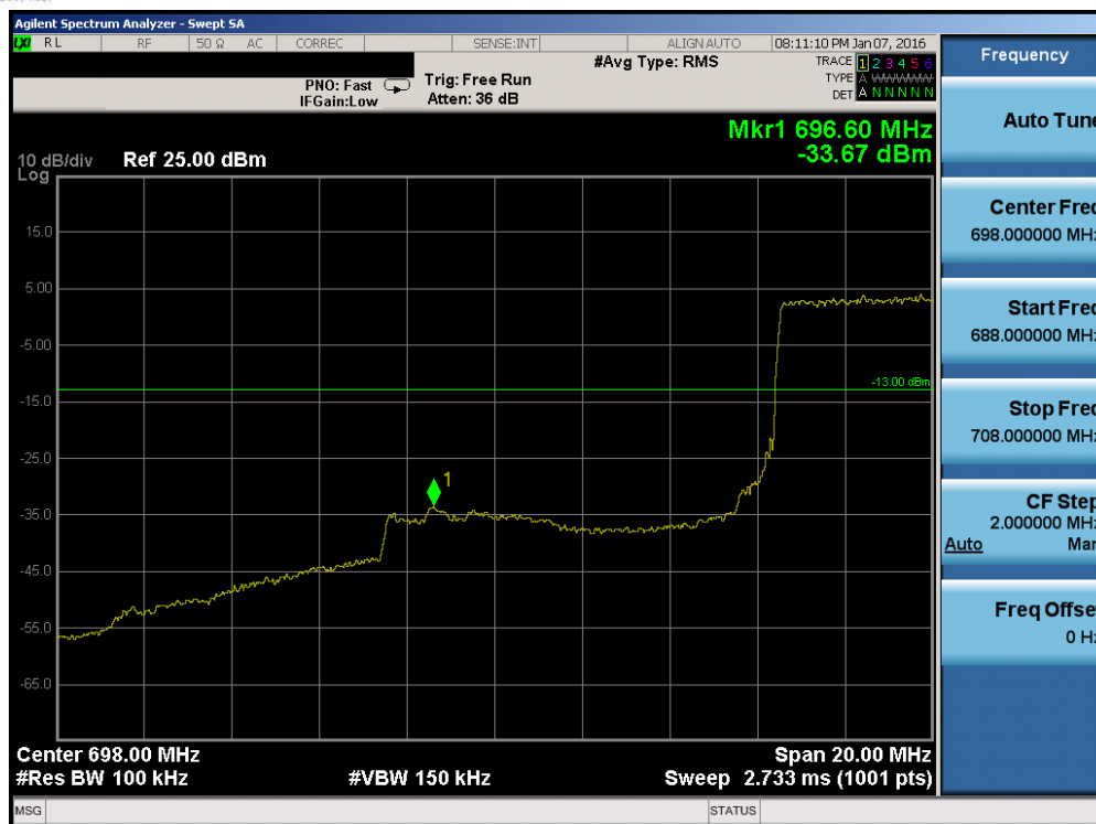
Plot 7-145. Lower Band Edge Plot (Band 17 – 10.0MHz QPSK – RB Size 50)
