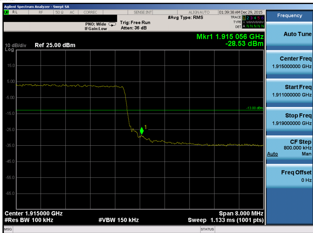
Plot 7-209. Upper Band Edge Plot (Band 2/25 – 10.0MHz QPSK – RB Size 50)
