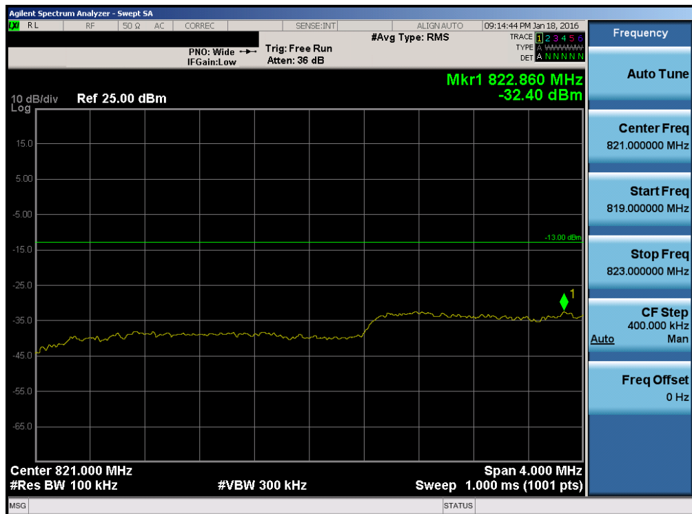
Plot 7-162. Lower Extended Band Edge Plot (Band 5 – 3.0MHz QPSK – RB Size 15)
