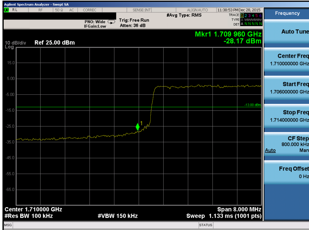
Plot 7-183. Lower Band Edge Plot (Band 4 – 10.0MHz QPSK – RB Size 50)
