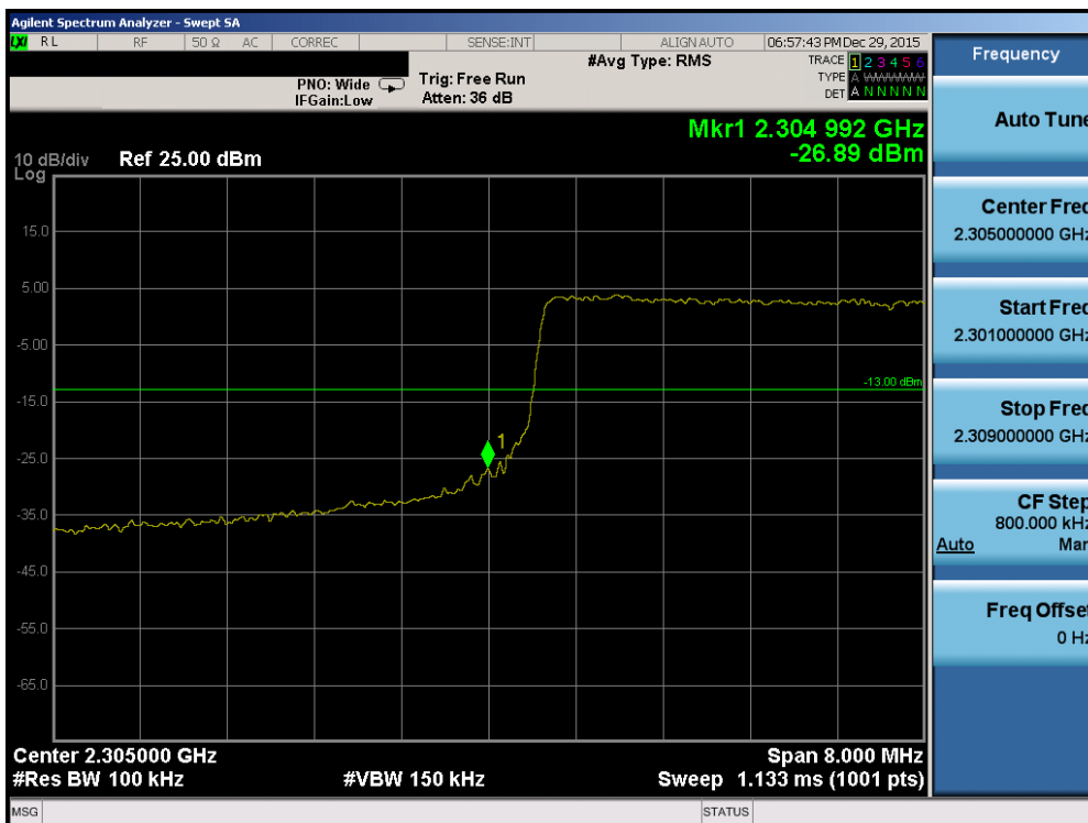
Plot 7-224. Lower Band Edge Plot (Band 30 – 10.0MHz QPSK – RB Size 50)
