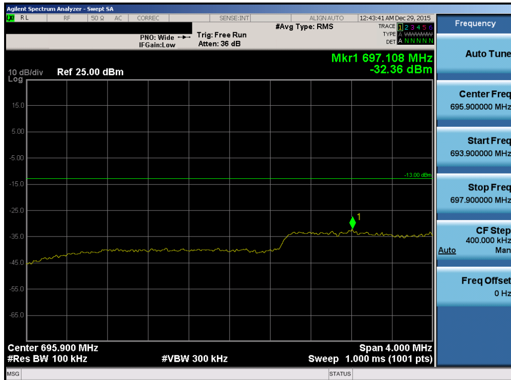
Plot 7-132. Lower Extended Band Edge Plot (Band 12 – 3.0MHz QPSK – RB Size 15)
