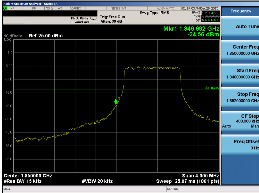
Plot 7-195. Lower Band Edge Plot (Band 2/25 – 1.4MHz QPSK – RB Size 6)
