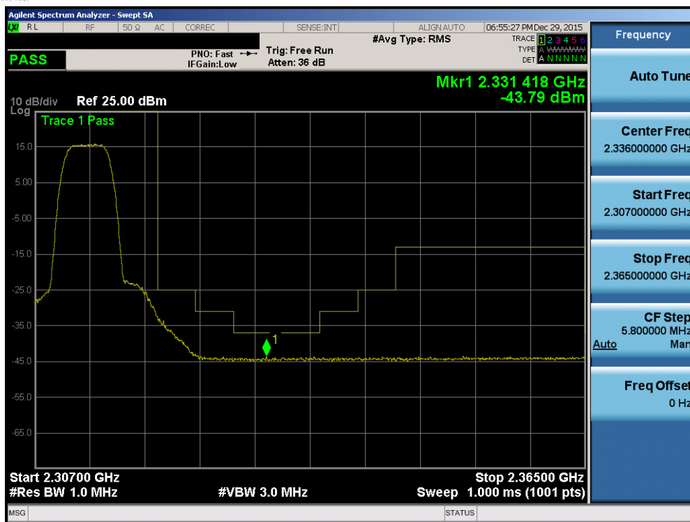
Plot 7-223. Upper Extended Band Edge Plot (Band 30 – 5.0MHz QPSK – RB Size 25)
