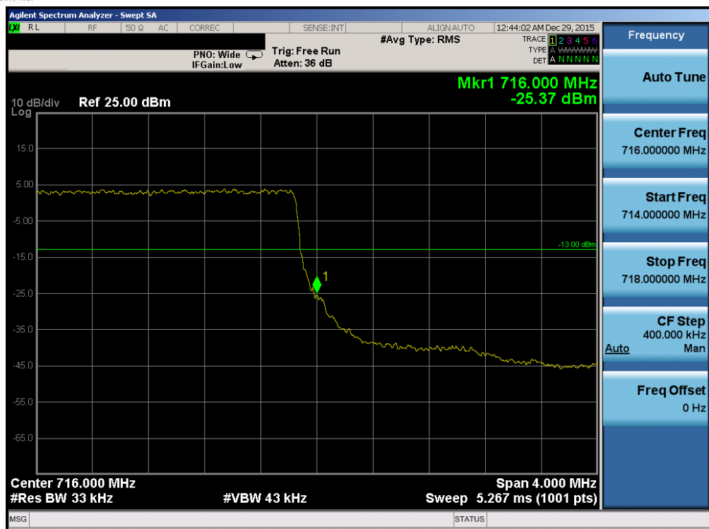
Plot 7-133. Upper Band Edge Plot (Band 12 – 3.0MHz QPSK – RB Size 15)
