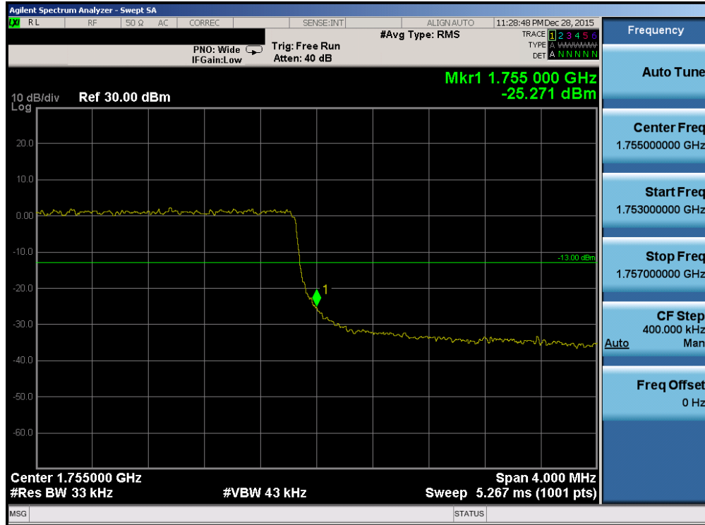
Plot 7-177. Upper Band Edge Plot (Band 4 – 3.0MHz QPSK – RB Size 15)
