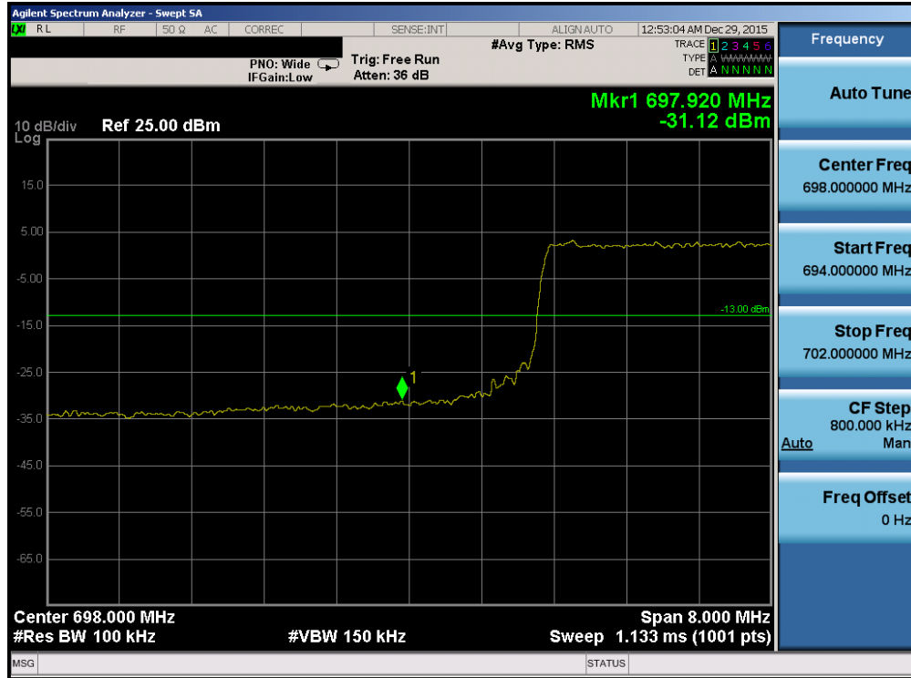
Plot 7-139. Lower Band Edge Plot (Band 12 – 10.0MHz QPSK – RB Size 50)
