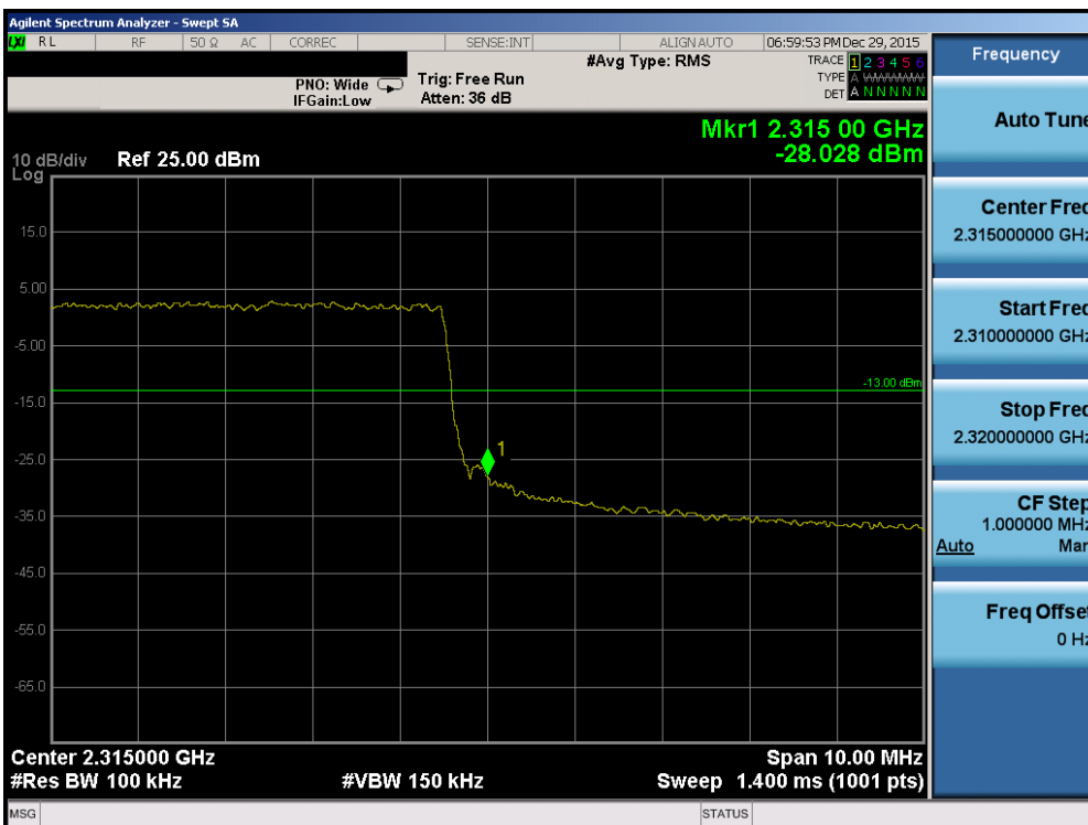
Plot 7-226. Upper Band Edge Plot (Band 30 – 10.0MHz QPSK – RB Size 50)
