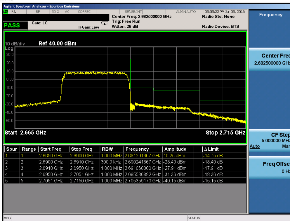
Plot 7-233. Upper ACP Plot (Band 41 – 15.0MHz QPSK – RB Size 75)
