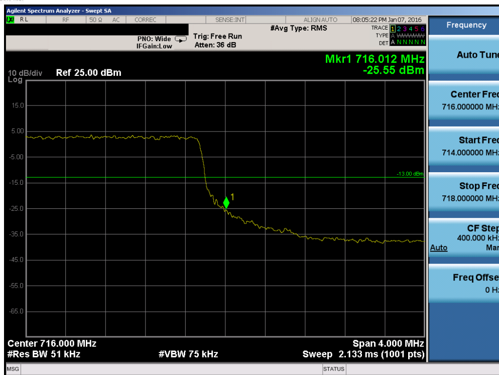
Plot 7-143. Upper Band Edge Plot (Band 17 – 5.0MHz QPSK – RB Size 25)
