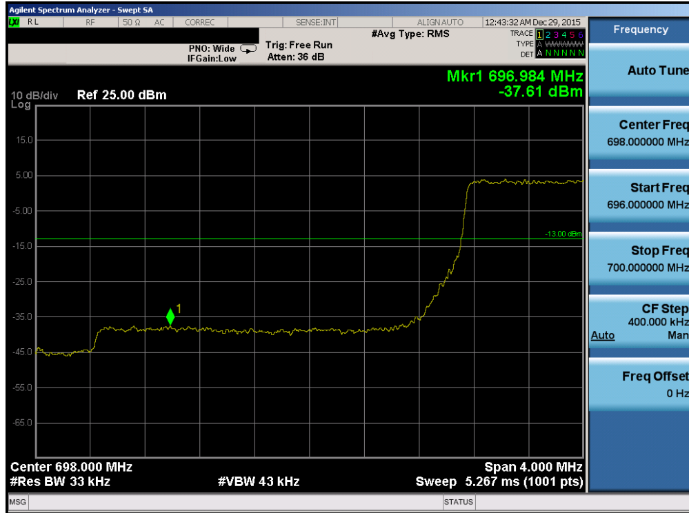
Plot 7-131. Lower Band Edge Plot (Band 12 – 3.0MHz QPSK – RB Size 15)
