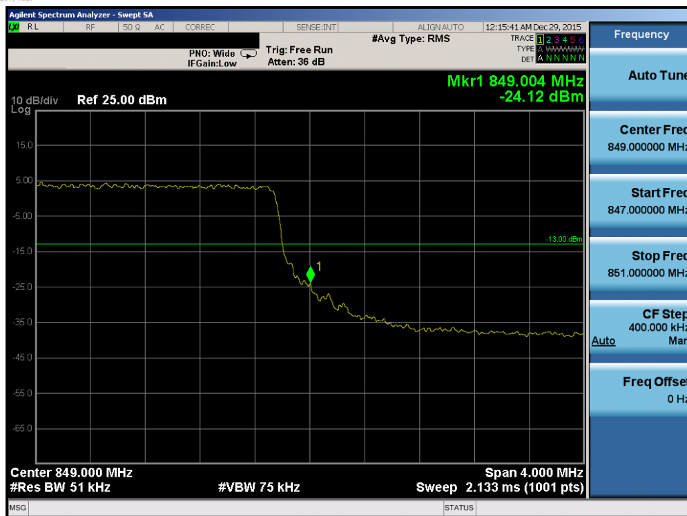
Plot 7-167. Upper Band Edge Plot (Band 5 – 5.0MHz QPSK – RB Size 25)
