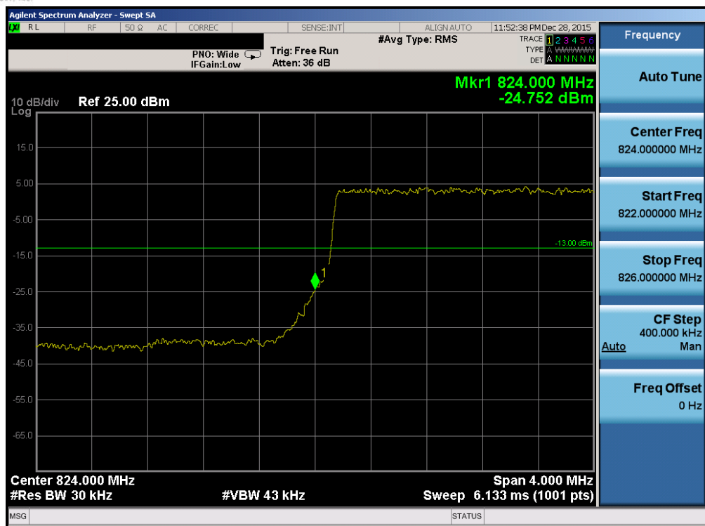
Plot 7-161. Lower Band Edge Plot (Band 5 – 3.0MHz QPSK – RB Size 15)
