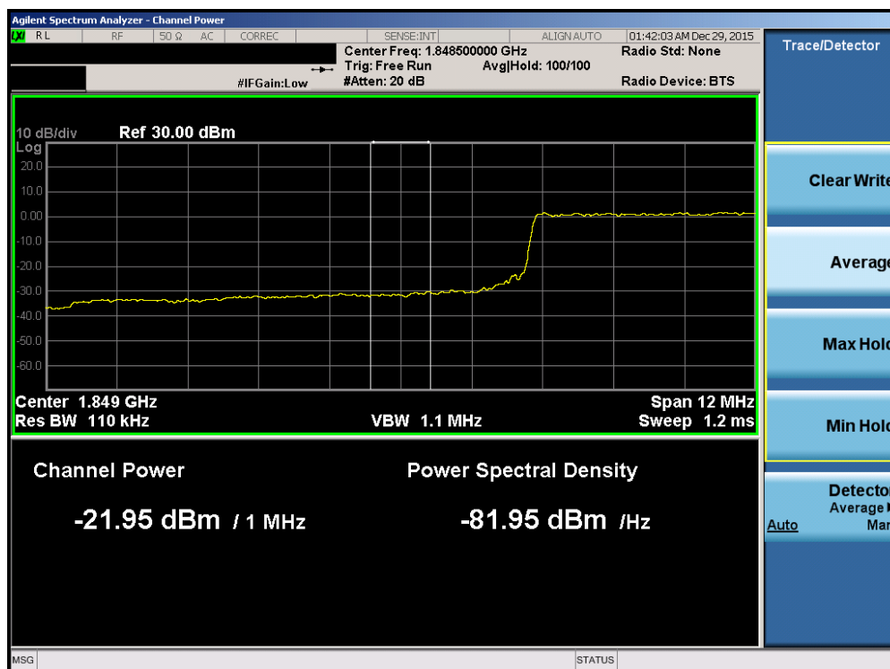
Plot 7-212. Lower Extended Band Edge Plot (Band 2/25 – 15.0MHz QPSK – RB Size 75)
