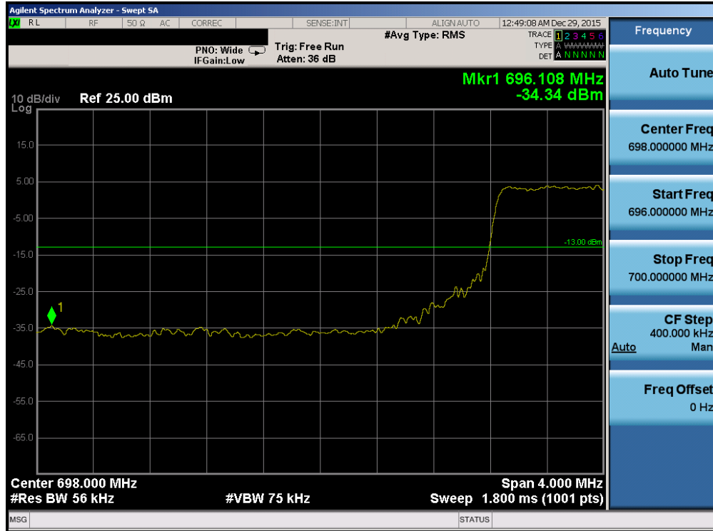
Plot 7-135. Lower Band Edge Plot (Band 12 – 5.0MHz QPSK – RB Size 25)
