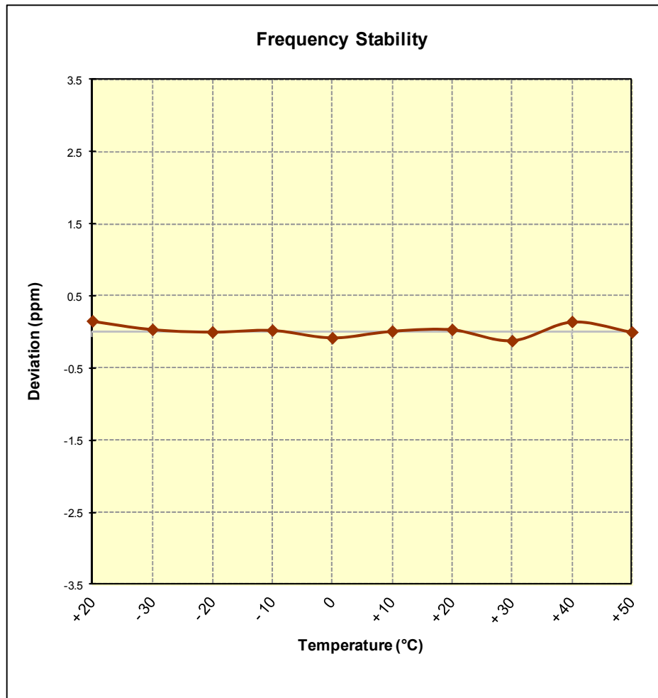
Figure 7-13. Frequency Stability Graph (Band 2/25)
