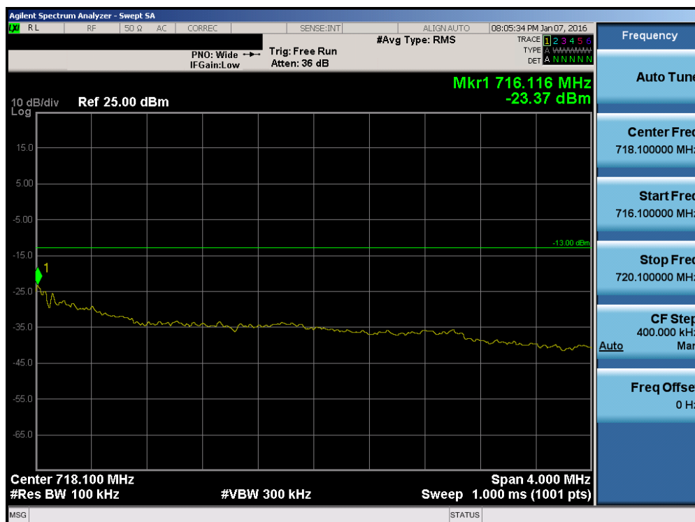
Plot 7-144. Upper Extended Band Edge Plot (Band 17 – 5.0MHz QPSK – RB Size 25)
