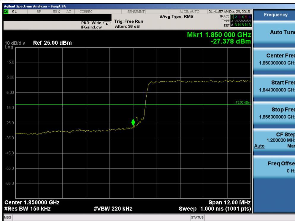
Plot 7-211. Lower Band Edge Plot (Band 2/25 – 15.0MHz QPSK – RB Size 75)
