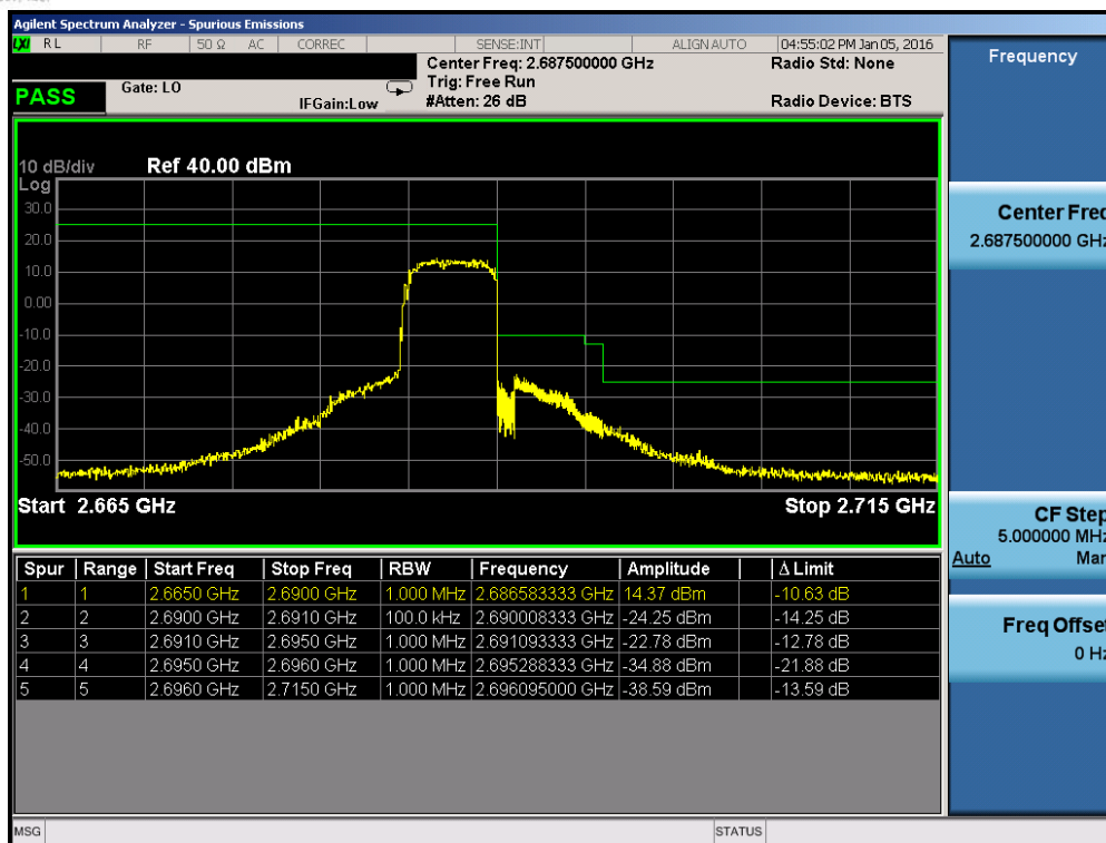
Plot 7-229. Upper ACP Plot (Band 41 – 5.0MHz QPSK – RB Size 25)
