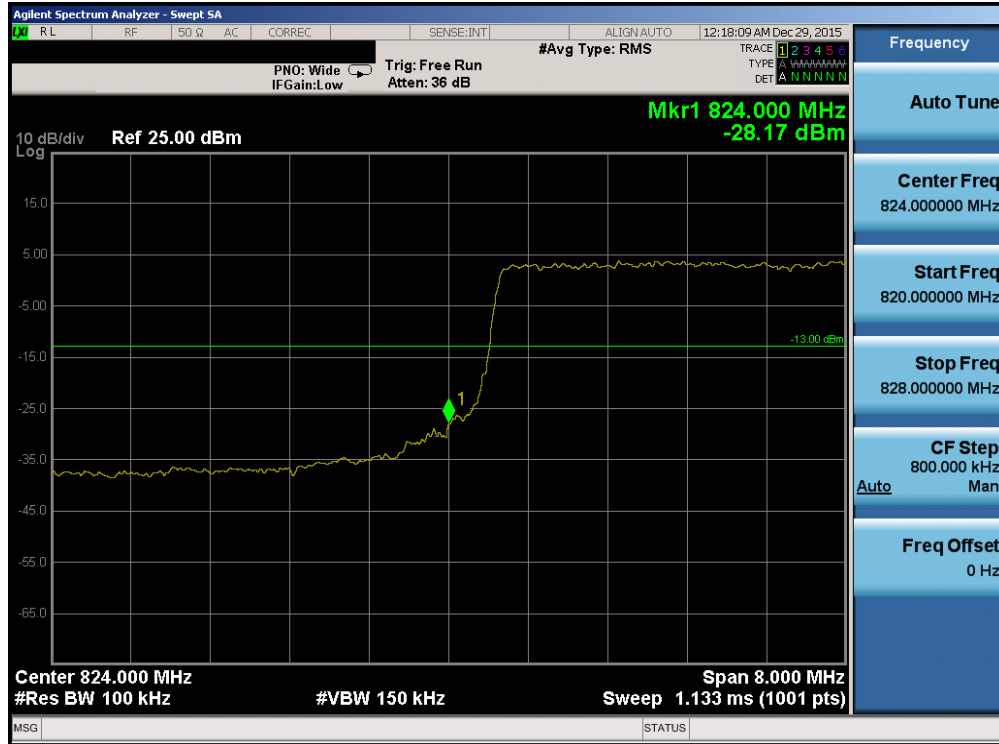
Plot 7-169. Lower Band Edge Plot (Band 5 – 10.0MHz QPSK – RB Size 50)
