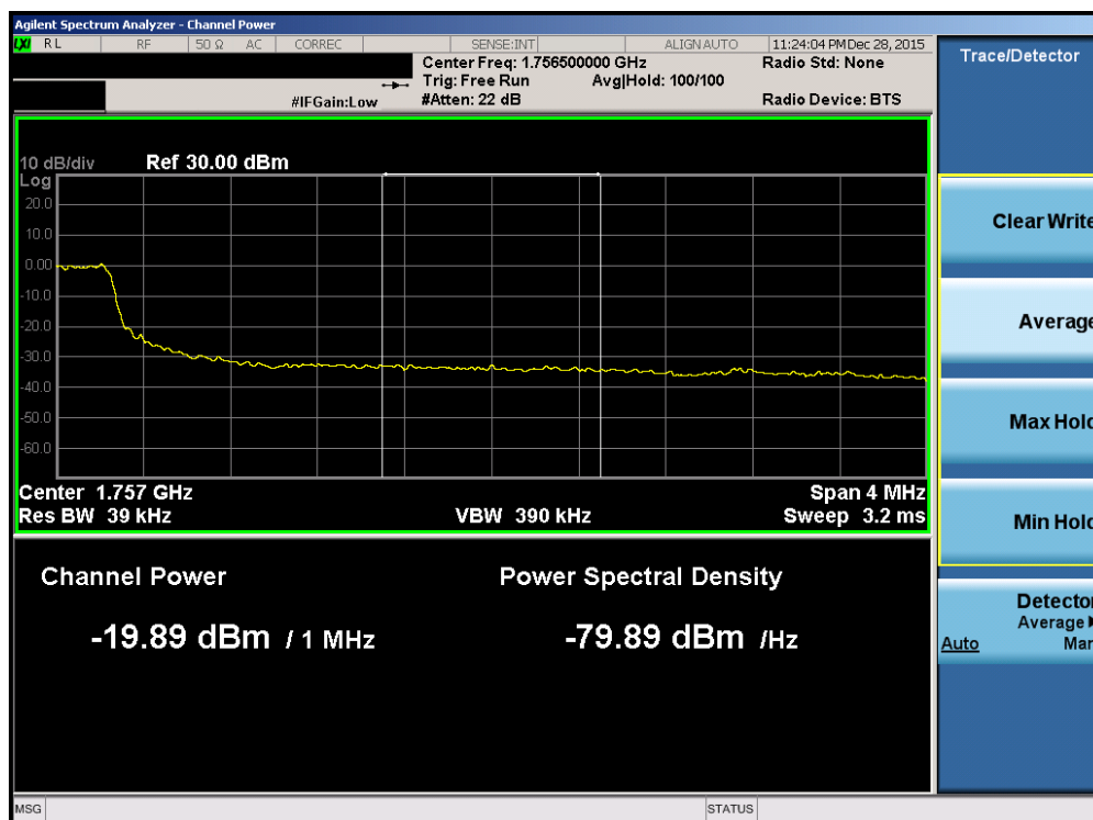
Plot 7-182. Upper Extended Band Edge Plot (Band 4 – 5.0MHz QPSK – RB Size 25)
