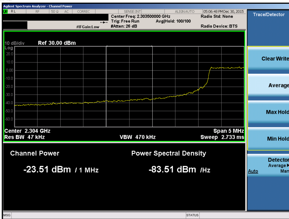
Plot 7-221. Lower Extended Band Edge Plot (Band 30 – 5.0MHz QPSK – RB Size 25)
