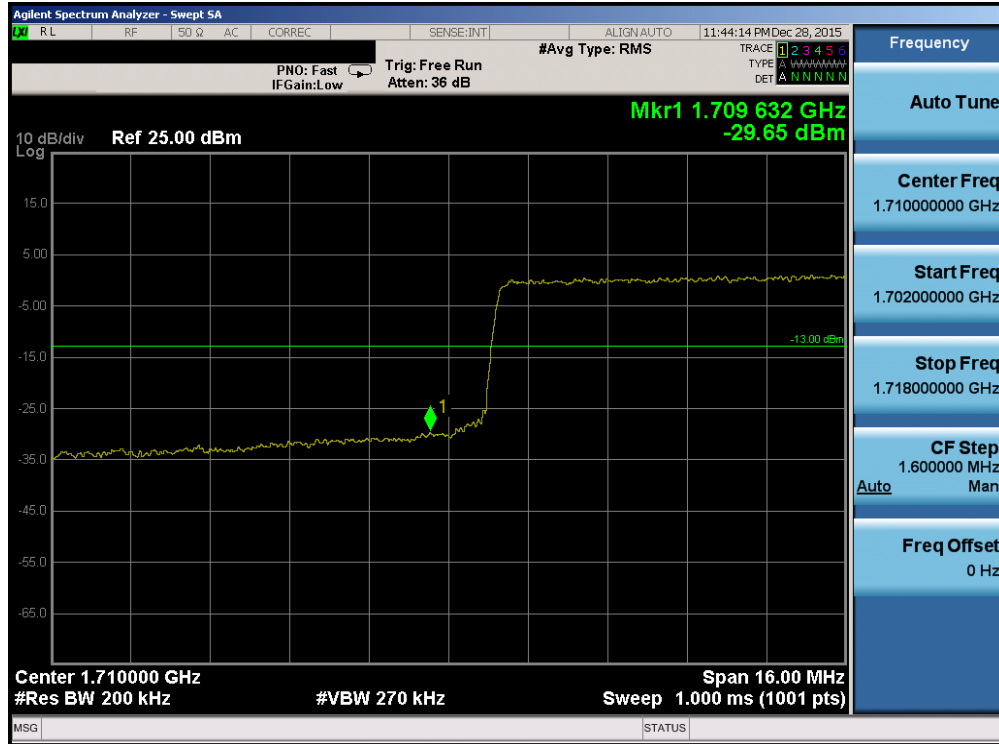
Plot 7-191. Lower Band Edge Plot (Band 4 – 20.0MHz QPSK – RB Size 100)
