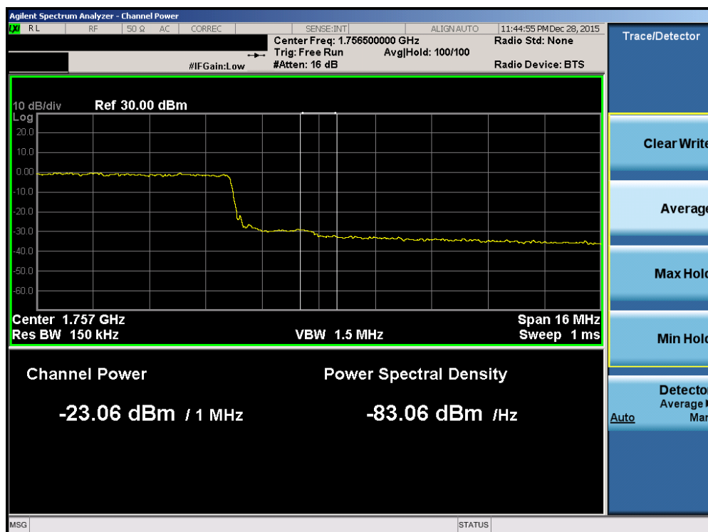
Plot 7-194. Upper Extended Band Edge Plot (Band 4 – 20.0MHz QPSK – RB Size 100)
