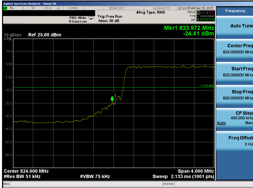
Plot 7-165. Lower Band Edge Plot (Band 5 - 5.0MHz QPSK - RB Size 25)
