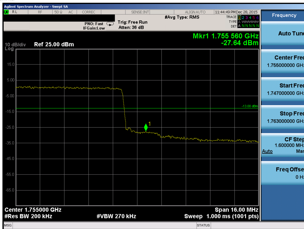
Plot 7-193. Upper Band Edge Plot (Band 4 – 20.0MHz QPSK – RB Size 100)
