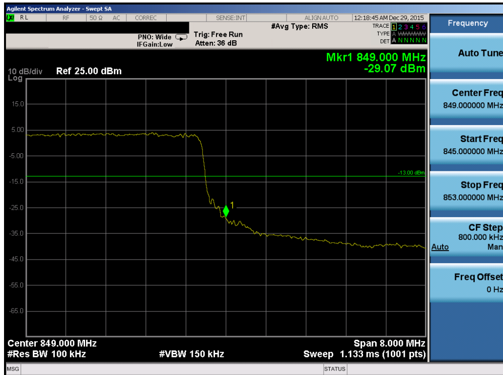
Plot 7-170. Upper Band Edge Plot (Band 5 – 10.0MHz QPSK – RB Size 50)
