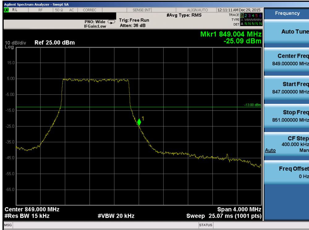
Plot 7-159. Upper Band Edge Plot (Band 5 – 1.4MHz QPSK – RB Size 6)
