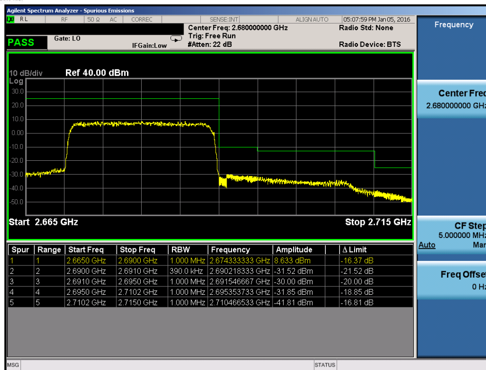
Plot 7-235. Upper ACP Plot (Band 41 – 20.0MHz QPSK – RB Size 100)
