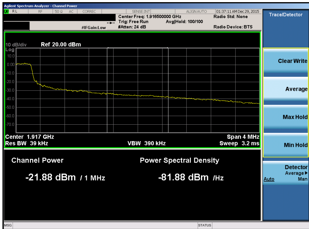
Plot 7-206. Upper Extended Band Edge Plot (Band 2/25 – 5.0MHz QPSK – RB Size 25)
