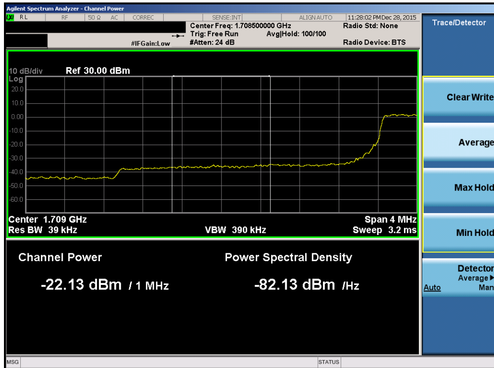
Plot 7-176. Lower Extended Band Edge Plot (Band 4 – 3.0MHz QPSK – RB Size 15)
