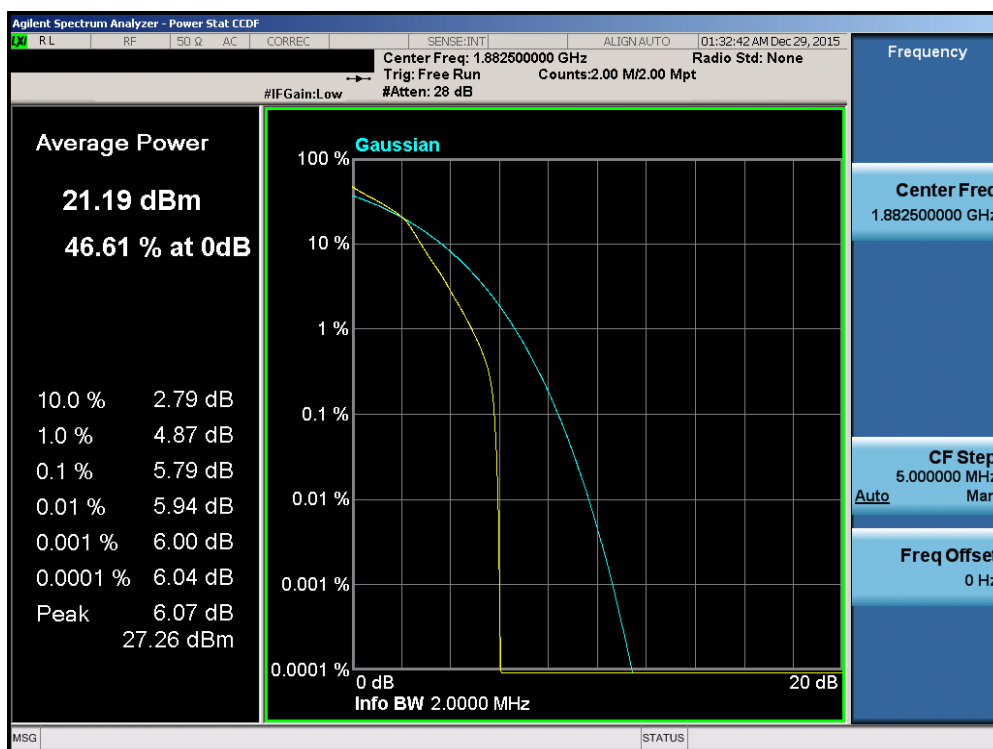
Plot 7-237. PAR Plot (Band 2/25 - 1.4MHz 16-QAM - RB Size 6)
