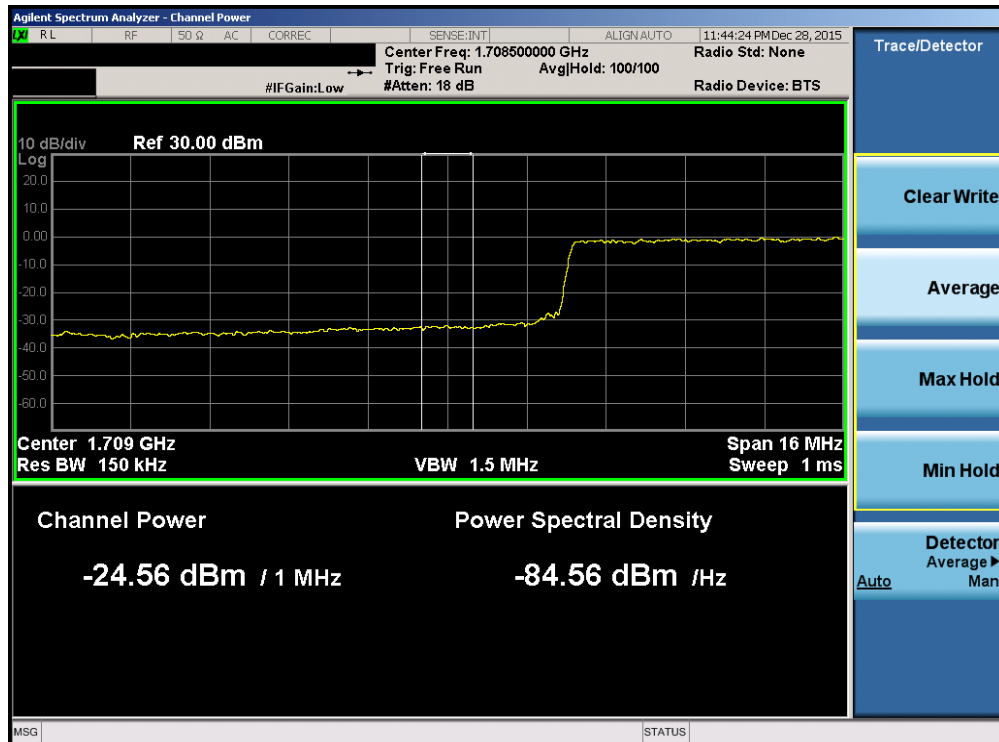
Plot 7-192. Lower Extended Band Edge Plot (Band 4 – 20.0MHz QPSK – RB Size 100)
