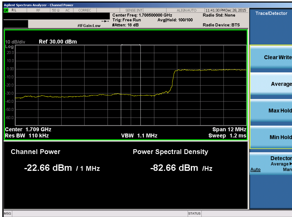
Plot 7-188. Lower Extended Band Edge Plot (Band 4 – 15.0MHz QPSK – RB Size 75)
