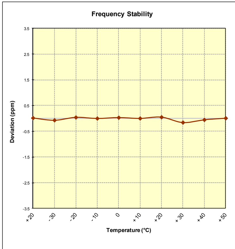
Figure 7-14. Frequency Stability Graph (Band 30)
