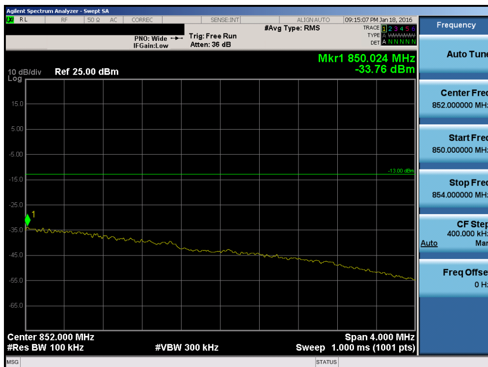
Plot 7-164. Upper Extended Band Edge Plot (Band 5 - Band 5 - 3.0MHz QPSK - RB Size 15)
