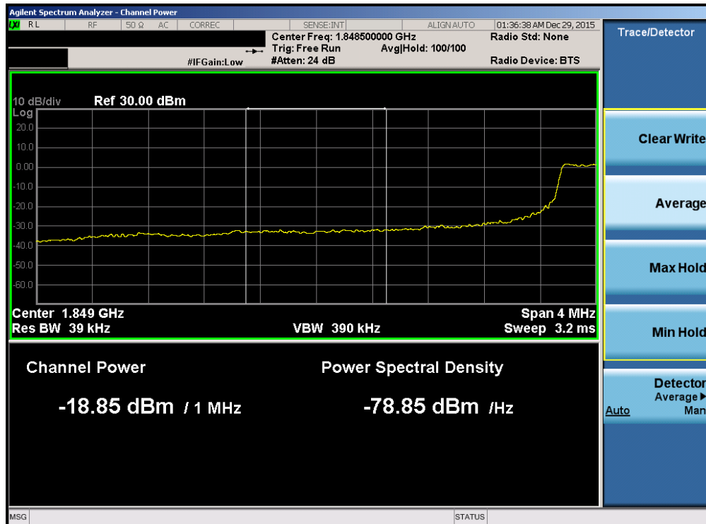
Plot 7-204. Lower Extended Band Edge Plot (Band 2/25 – 5.0MHz QPSK – RB Size 25)
