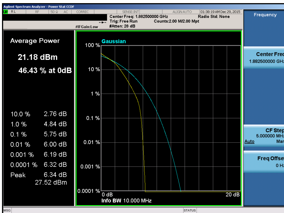
Plot 7-243. PAR Plot (Band 2/25 - 10.0MHz 16-QAM - RB Size 50)
