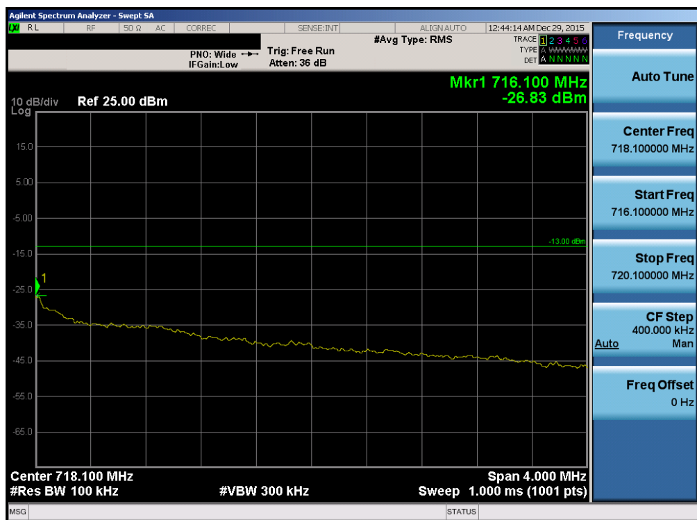
Plot 7-134. Upper Extended Band Edge Plot (Band 12 – 3.0MHz QPSK – RB Size 15)
