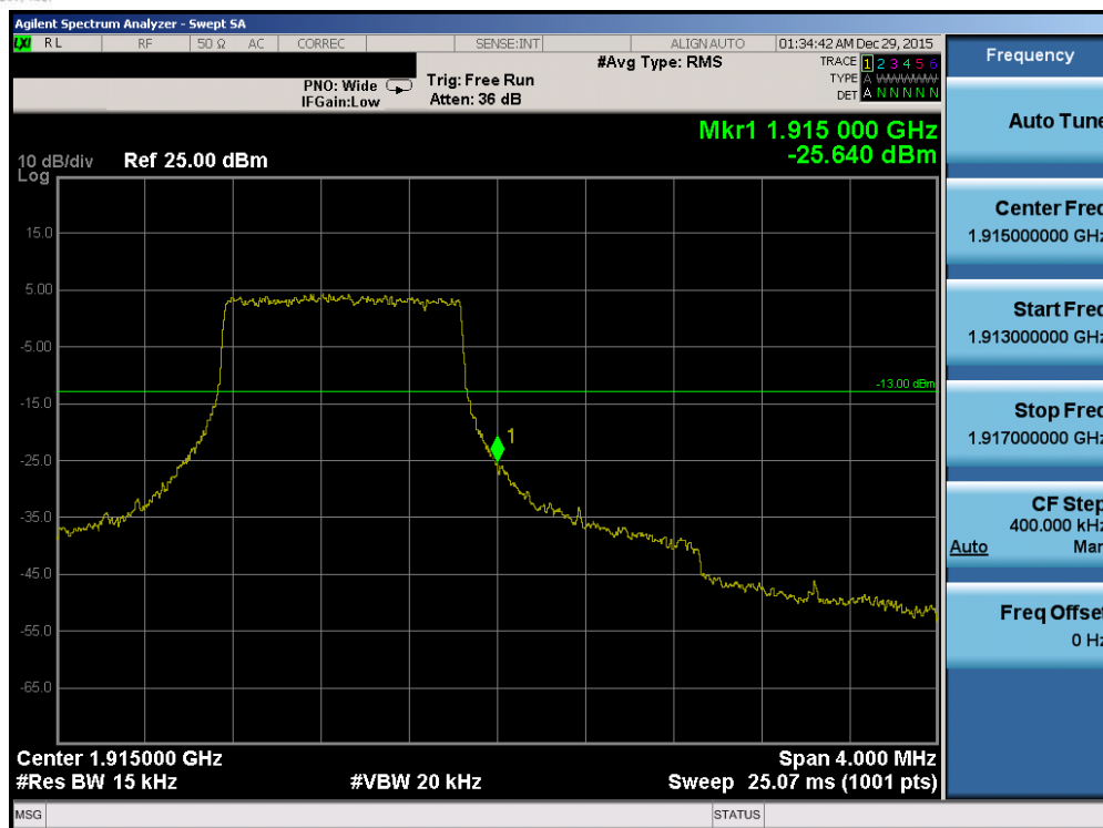
Plot 7-197. Upper Band Edge Plot (Band 2/25 – 1.4MHz QPSK – RB Size 6)
