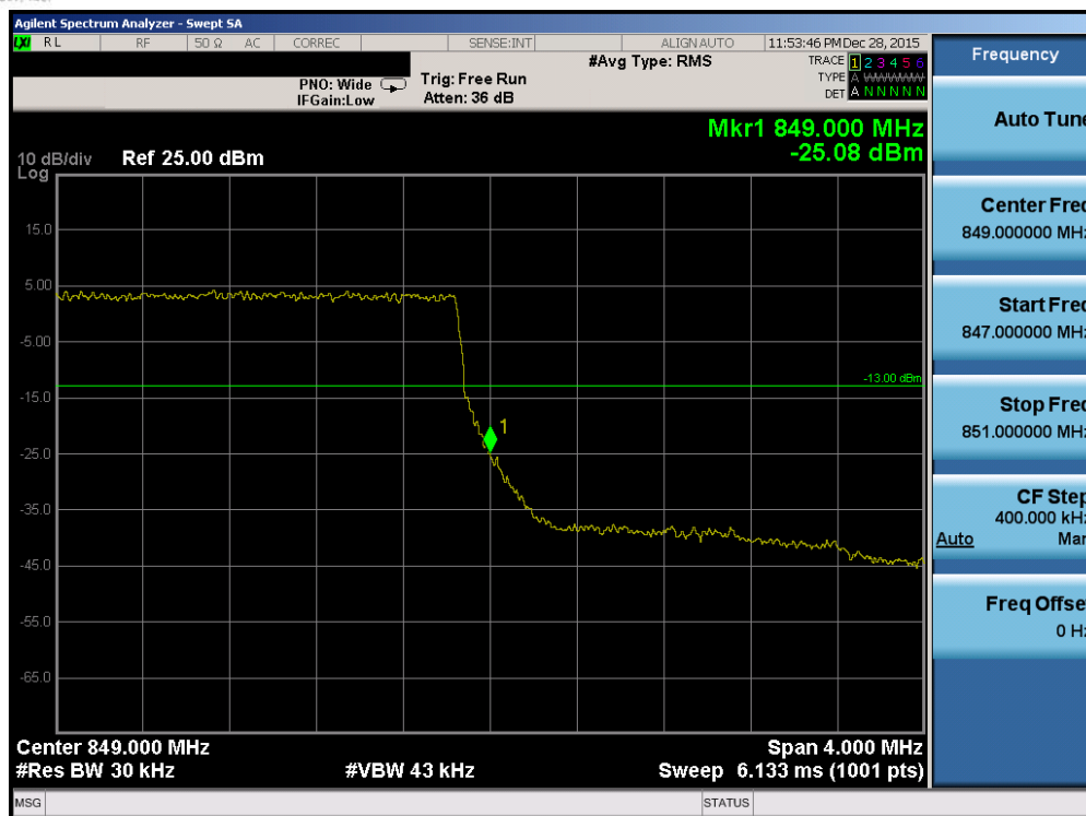
Plot 7-163. Upper Band Edge Plot (Band 5 - 3.0MHz QPSK - RB Size 15)
