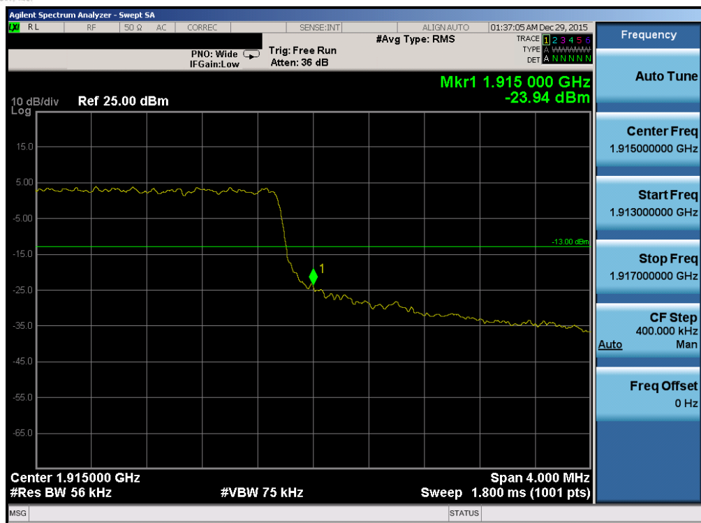
Plot 7-205. Upper Band Edge Plot (Band 2/25 – 5.0MHz QPSK – RB Size 25)
