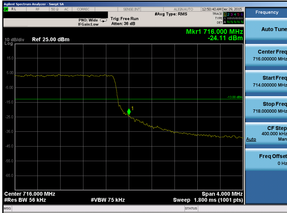
Plot 7-137. Upper Band Edge Plot (Band 12 – 5.0MHz QPSK – RB Size 25)
