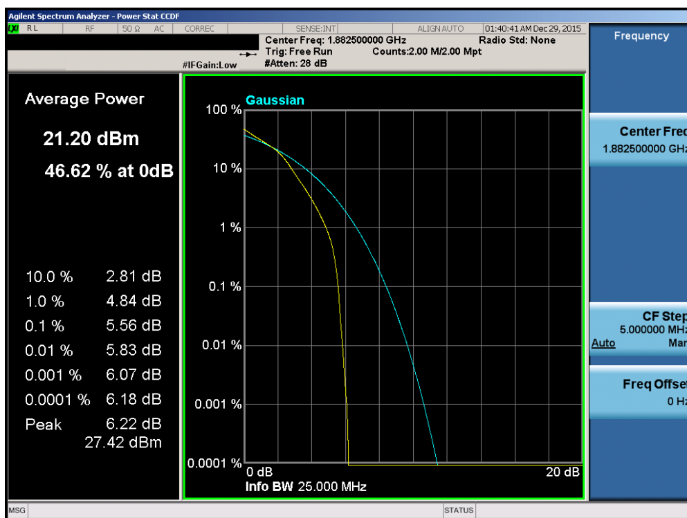
Plot 7-245. PAR Plot (Band 2/25 – 15.0MHz 16-QAM – RB Size 75)
