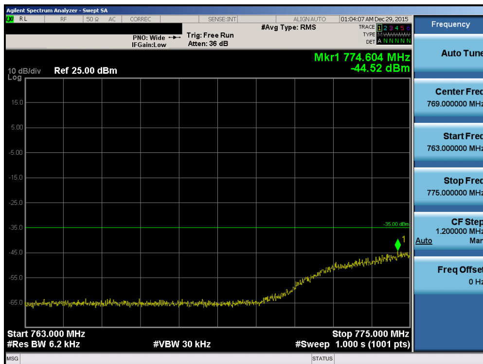
Plot 7-154. Lower Emission Mask Edge Plot (Band 13 – 10.0MHz QPSK – RB Size 50)
