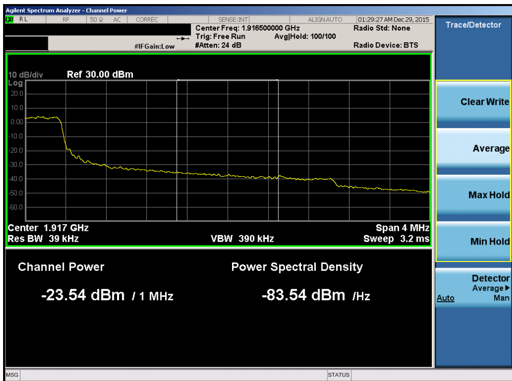
Plot 7-202. Upper Extended Band Edge Plot (Band 2/25 – 3.0MHz QPSK – RB Size 15)
