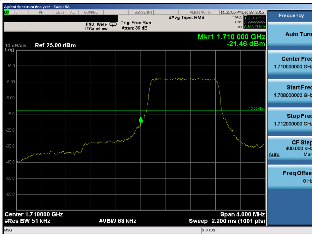
Plot 7-171. Lower Band Edge Plot (Band 4 – 1.4MHz QPSK – RB Size 6)
