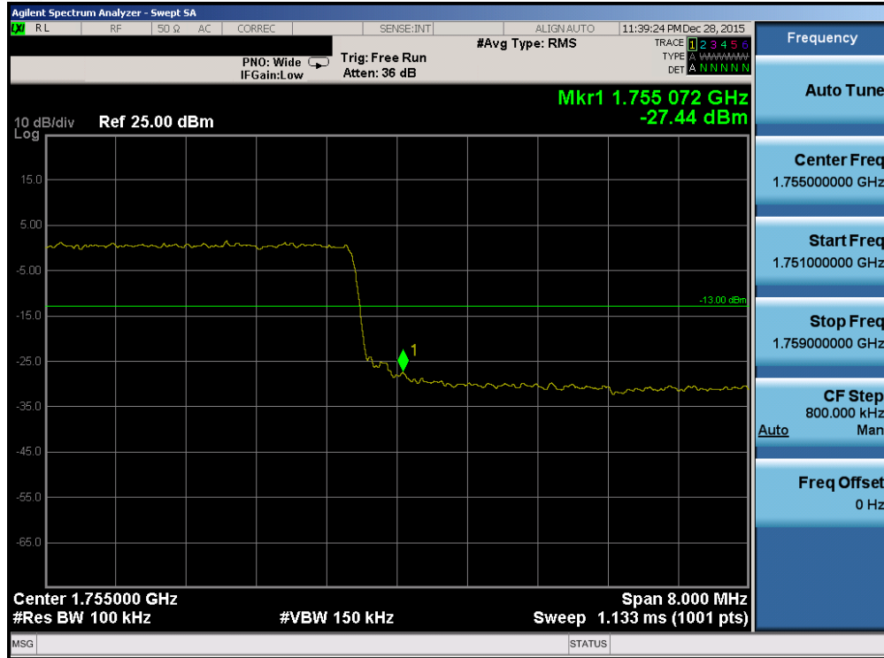
Plot 7-185. Upper Band Edge Plot (Band 4 – 10.0MHz QPSK – RB Size 50)
