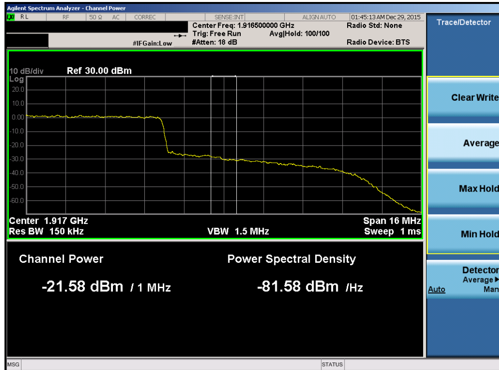
Plot 7-218. Upper Extended Band Edge Plot (Band 2/25 – 20.0MHz QPSK – RB Size 100)
