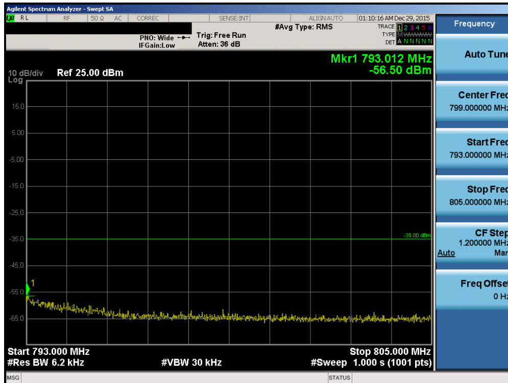
Plot 7-152. Upper Emission Mask Edge Plot (Band 13 – 5.0MHz QPSK – RB Size 25)
