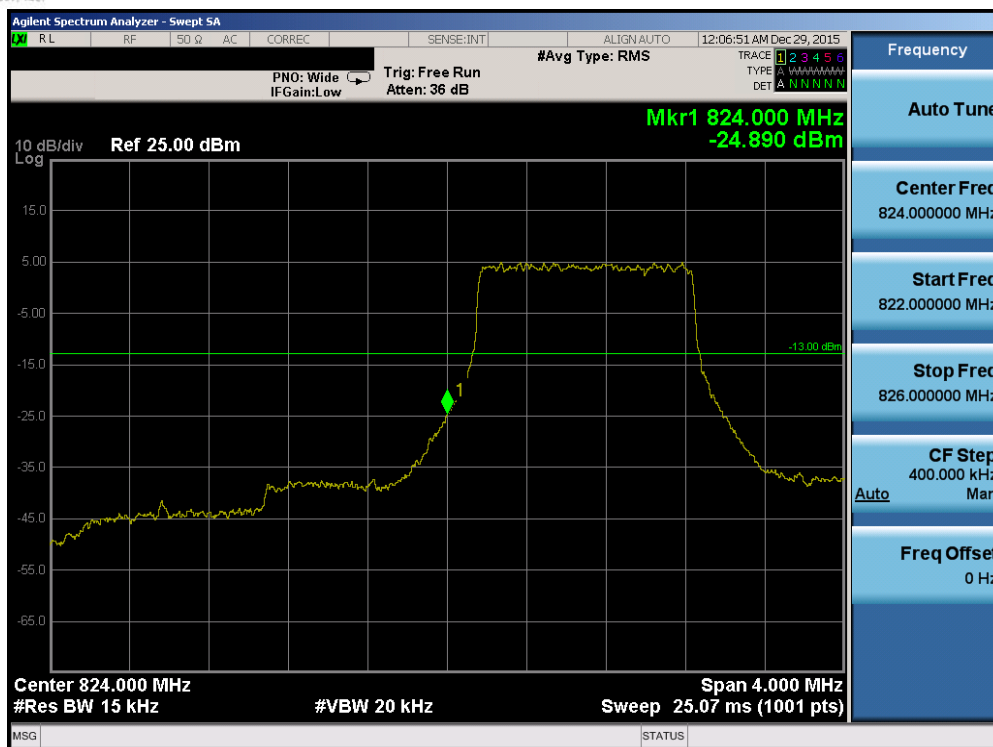
Plot 7-157. Lower Band Edge Plot (Band 5 – 1.4MHz QPSK – RB Size 6)
