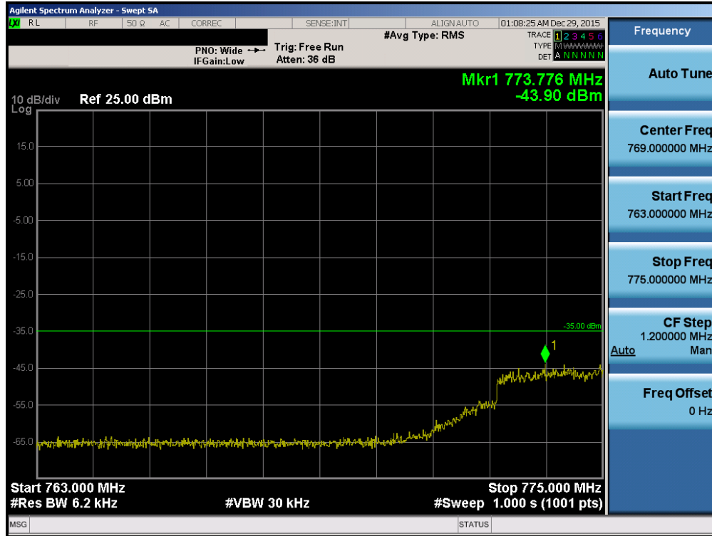
Plot 7-149. Lower Emission Mask Edge Plot (Band 13 – 5.0MHz QPSK – RB Size 25)
