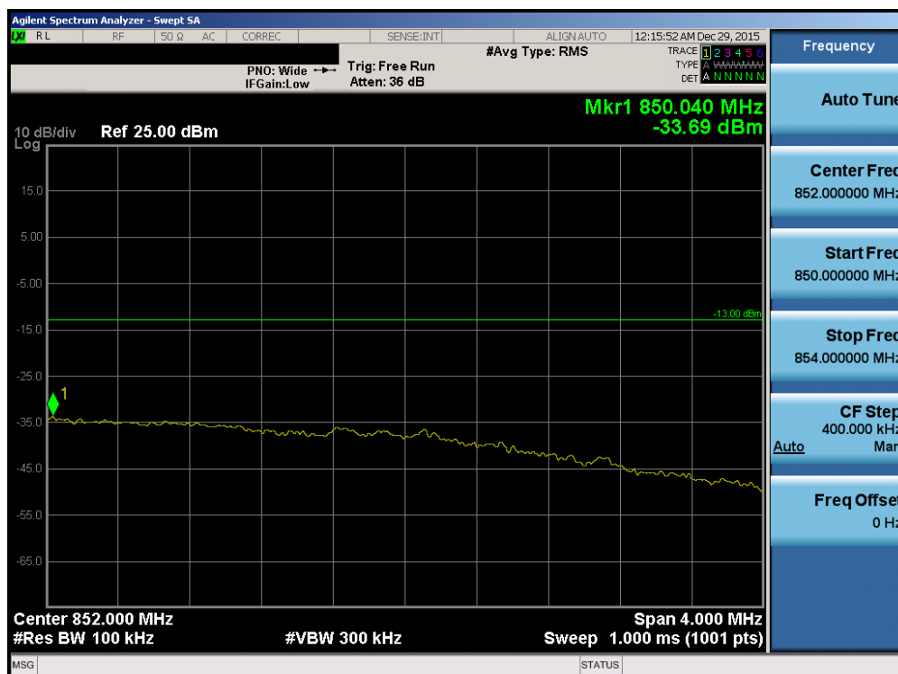
Plot 7-168. Upper Extended Band Edge Plot (Band 5 – 5.0MHz QPSK – RB Size 25)
