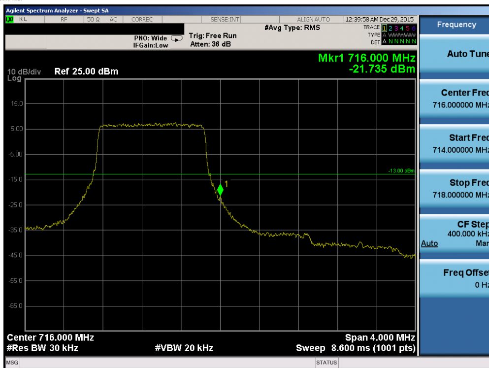
Plot 7-129. Upper Band Edge Plot (Band 12 – 1.4MHz QPSK – RB Size 6)
