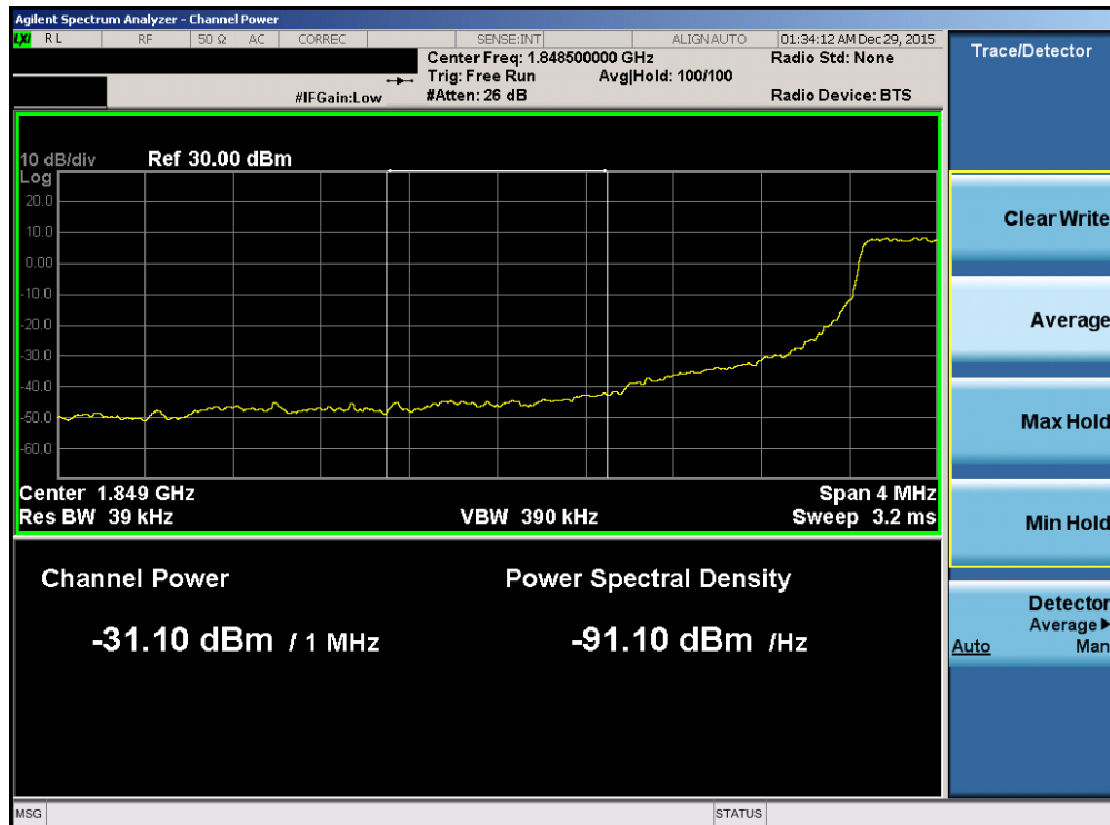
Plot 7-196. Lower Extended Band Edge Plot (Band 2/25 – 1.4MHz QPSK – RB Size 6)
