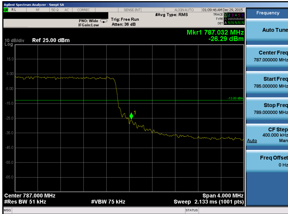
Plot 7-150. Upper Band Edge Plot (Band 13 – 5.0MHz QPSK – RB Size 25)
