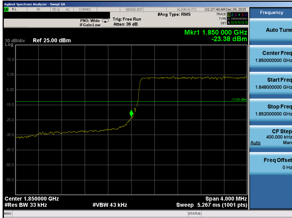
Plot 7-199. Lower Band Edge Plot (Band 2/25 – 3.0MHz QPSK – RB Size 15)
