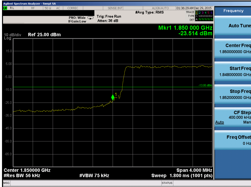
Plot 7-203. Lower Band Edge Plot (Band 2/25 – 5.0MHz QPSK – RB Size 25)
