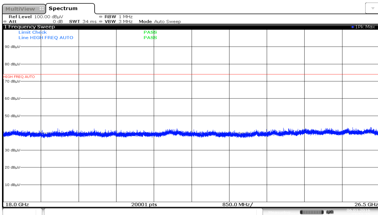
Plot 7-76. Radiated Spurious Plot above 18GHz (Pol. V)
