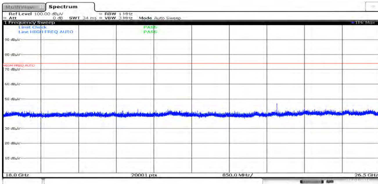
Plot 7-68. Radiated Spurious Plot above 18GHz (Pol. V)
