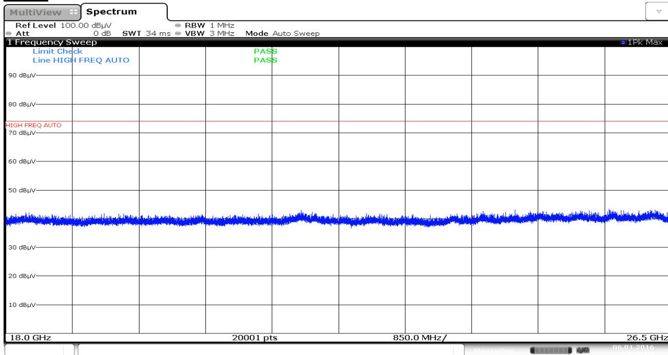
Plot 7-67. Radiated Spurious Plot above 18GHz (Pol. H)
