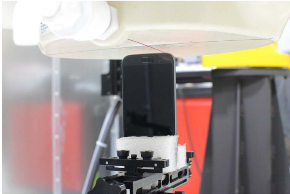
SAR Test Setup Photo 9: Bottom at 1.0 cm
