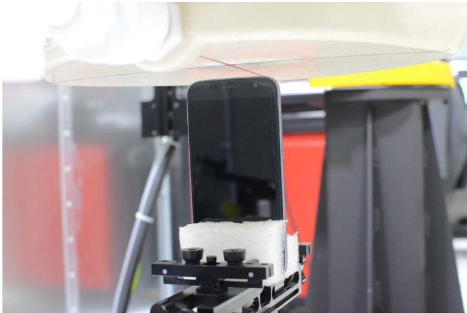
SAR Test Setup Photo 8: Top at 1.0 cm
