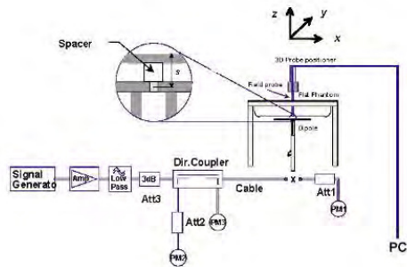
Figure 9-1 System Verification Setup Diagram
