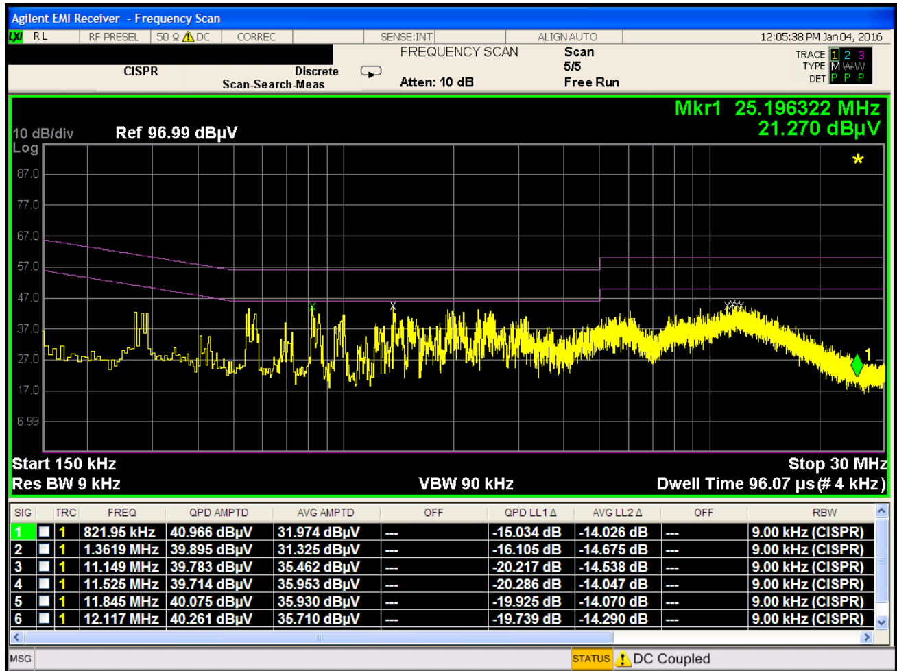
Plot 7-32. Line Conducted Plot with Bluetooth LE (L1)
