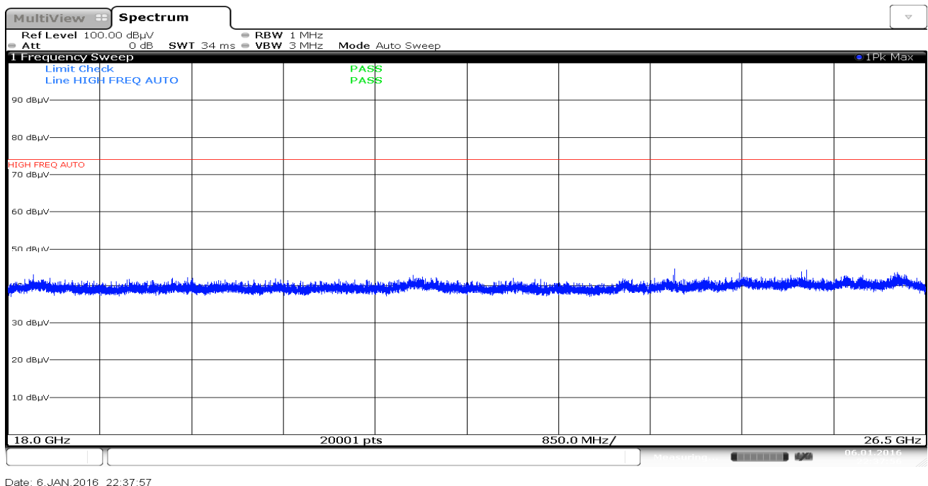
Plot 25. Radiated Spurious Plot above 18GHz (Pol. V)
