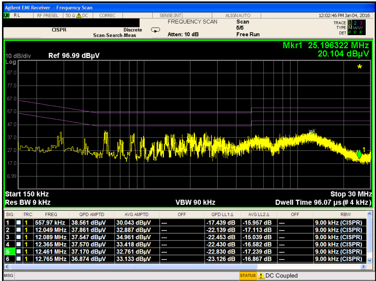
Plot 7-33. Line Conducted Plot with Bluetooth LE (N)
