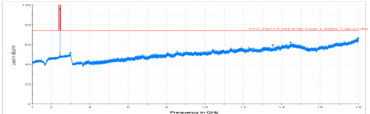
Plot 21. Radiated Spurious Plot above 1GHz (BT LE – Ch. 19, Ant. Pol. V)
