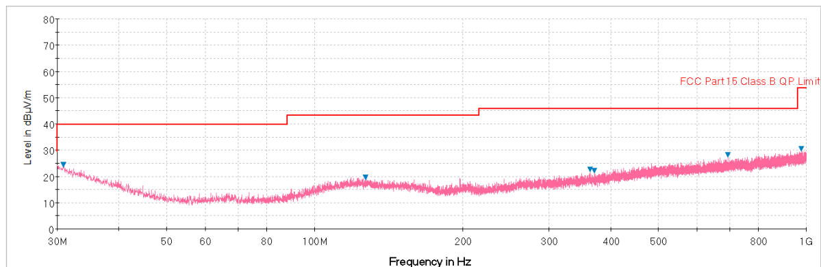
Plot 31. Radiated Spurious Plot below 1GHz (Pol. V)
