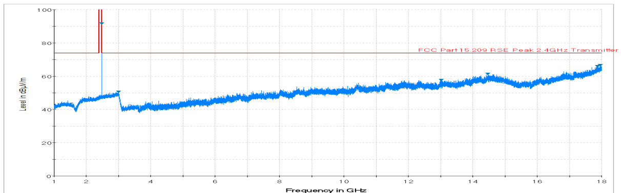
Plot 23. Radiated Spurious Plot above 1GHz (BT LE - Ch. 39, Ant. Pol. V)
