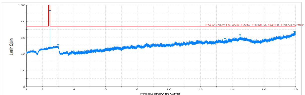
Plot 22. Radiated Spurious Plot above 1GHz (BT LE – Ch. 39, Ant. Pol. H)
