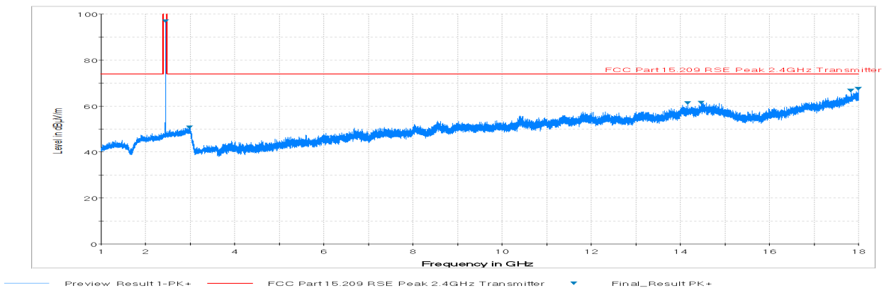
Plot 20. Radiated Spurious Plot above 1GHz (BT LE – Ch. 19, Ant. Pol. H)
