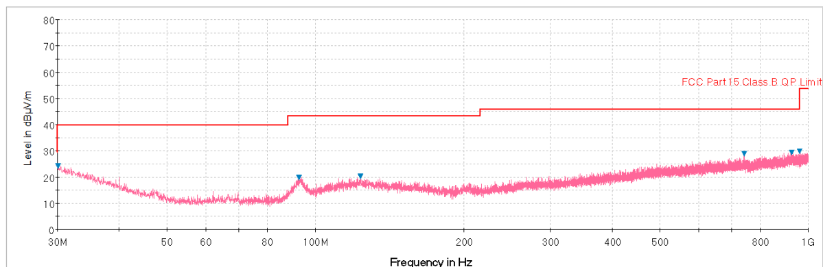
Plot 30. Radiated Spurious Plot below 1GHz (Pol. H)
