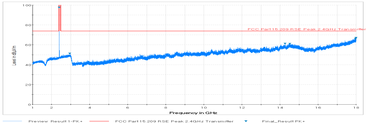
Plot 18. Radiated Spurious Plot above 1GHz (BT LE – Ch. 0, Ant. Pol. H)
