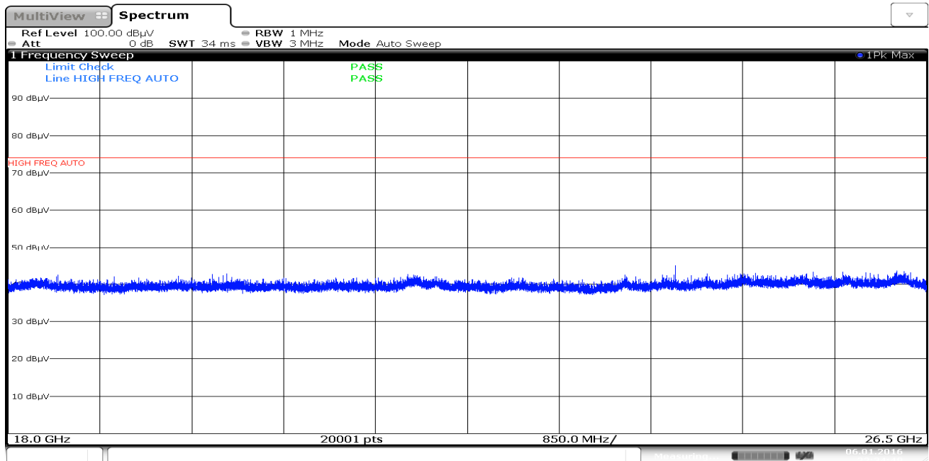
Plot 24. Radiated Spurious Plot above 18GHz (Pol. H)
