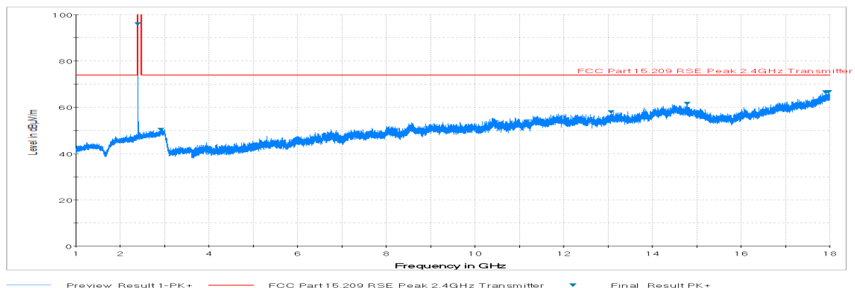
Plot 19. Radiated Spurious Plot above 1GHz (BT LE – Ch. 0, Ant. Pol. V)
