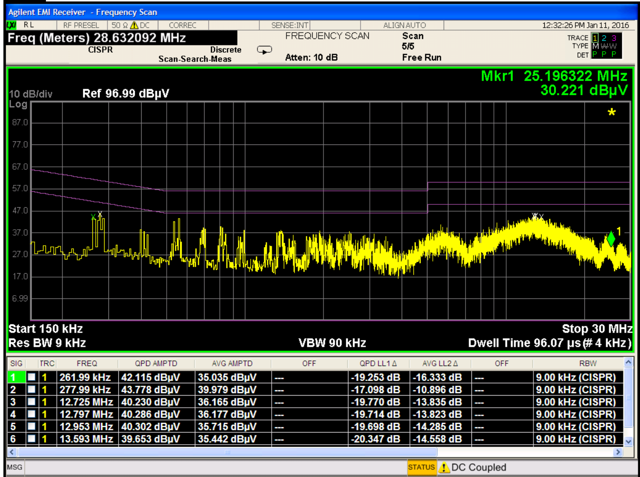
Plot 8-4. Line-Conducted Test Plot (N) – Antenna Terminated in 50Ohms
