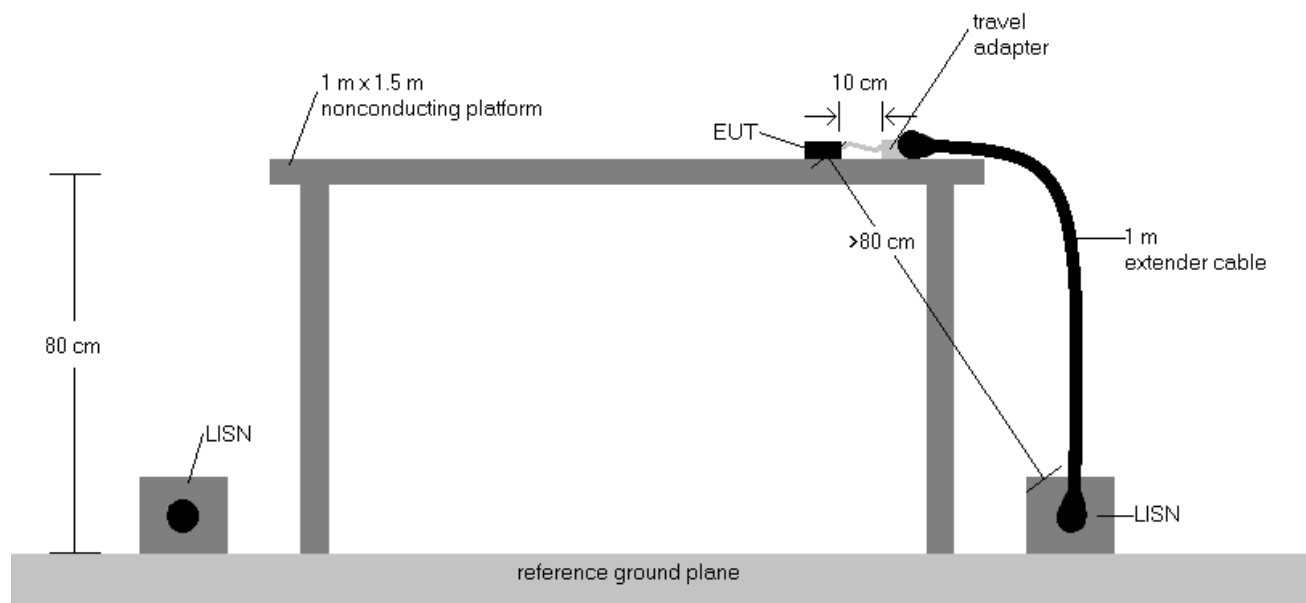
Figure 8-8. Test Instrument & Measurement Setup
