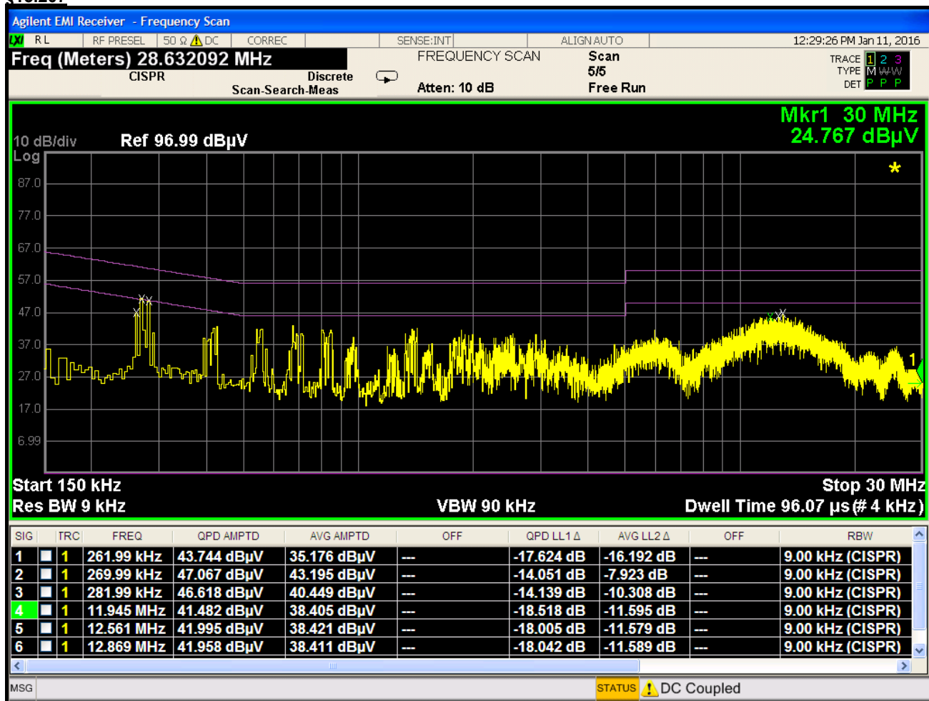
Plot 8-3. Line-Conducted Test Plot (L1) – Antenna Terminated in 50 Ohms
