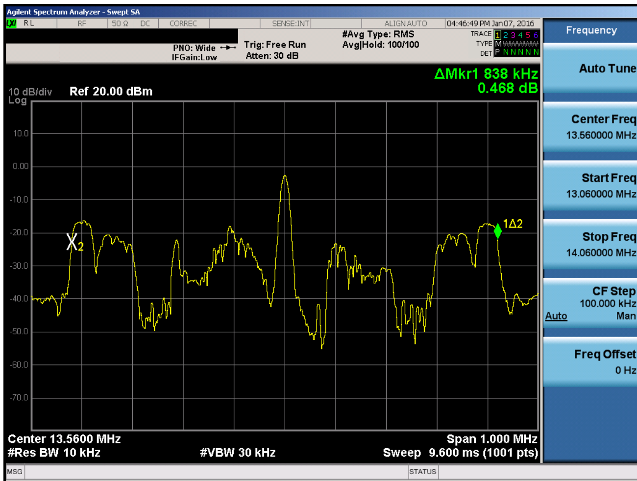
Figure 8-3. 20dB Bandwidth Plot with WCP
