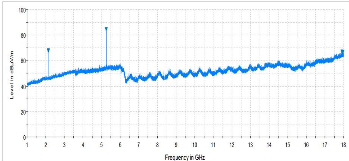
Plot 7-184. Radiated Spurious Plot above 1GHz (5GHz – 2.4 GHz, Ant. Pol. V)
