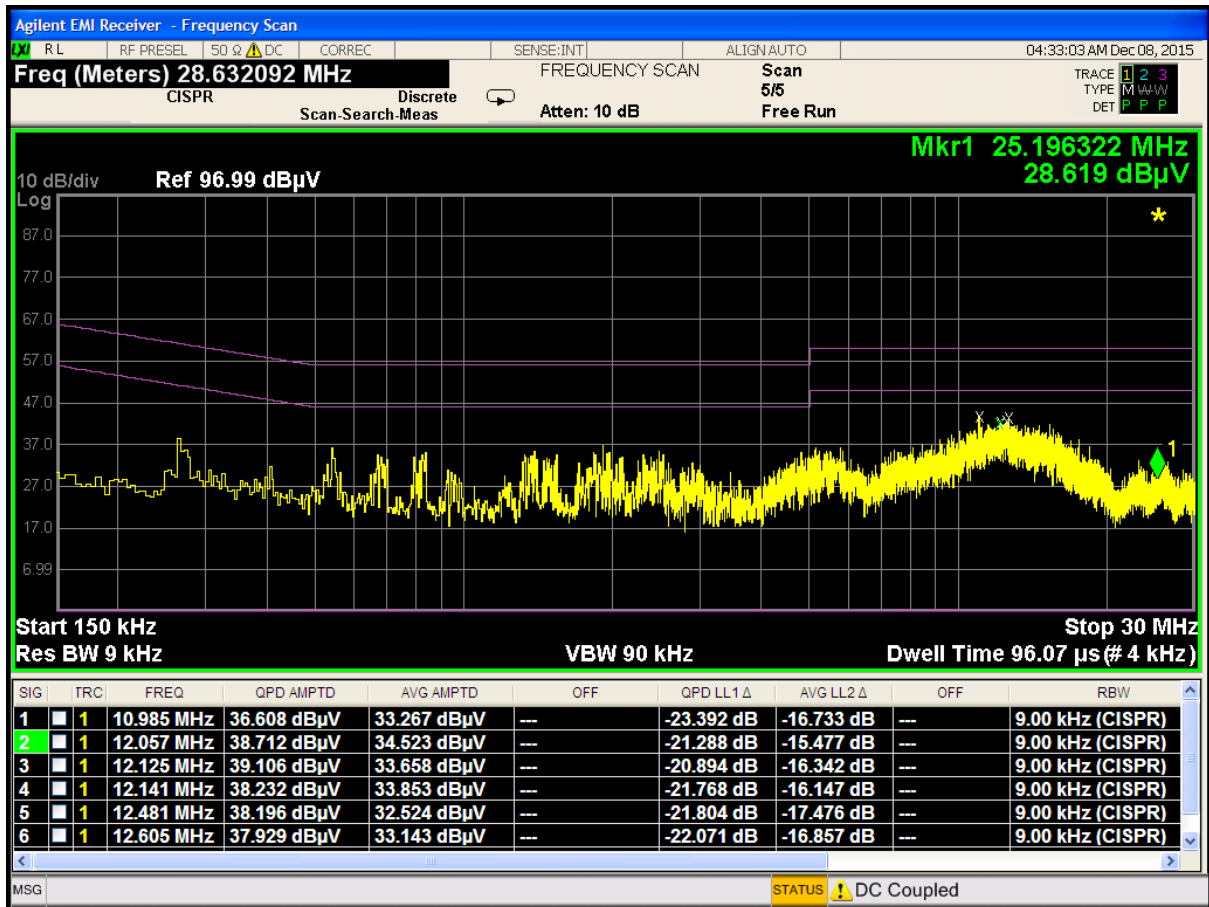
Plot 7-9. Line-Conducted Test Plot (N)
