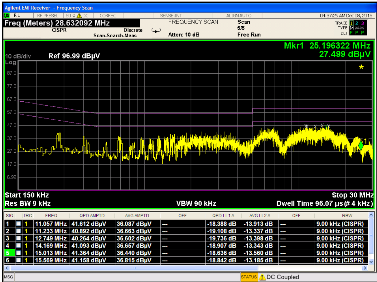
Plot 7-8. Line-Conducted Test Plot (L1)
