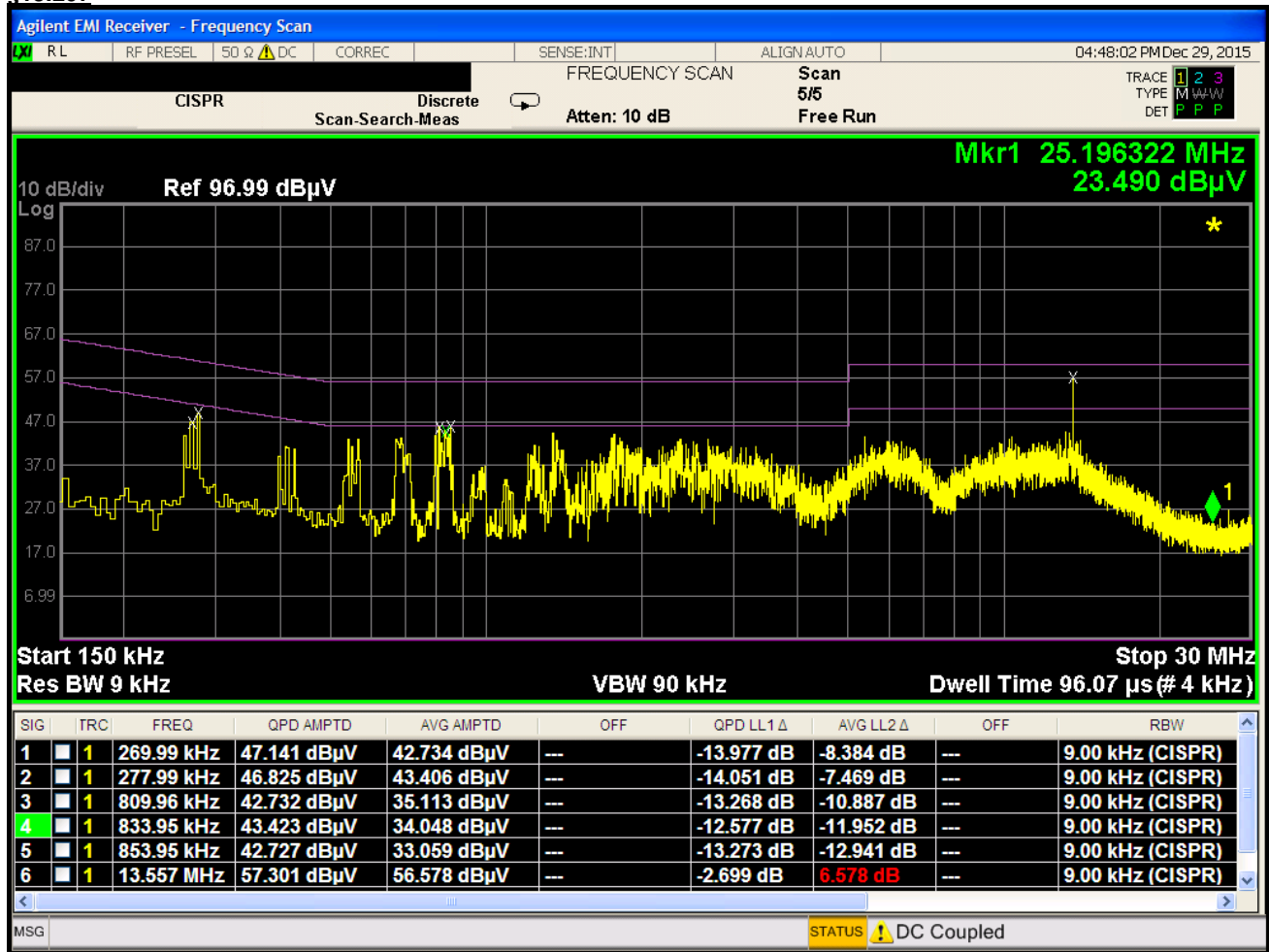
Plot 8-1. Line-Conducted Test Plot with RFID Antenna Attached(L1)
