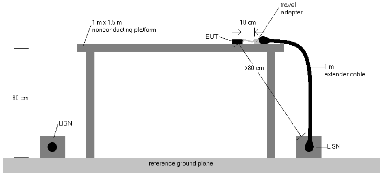
Figure 8-8. Test Instrument & Measurement Setup
