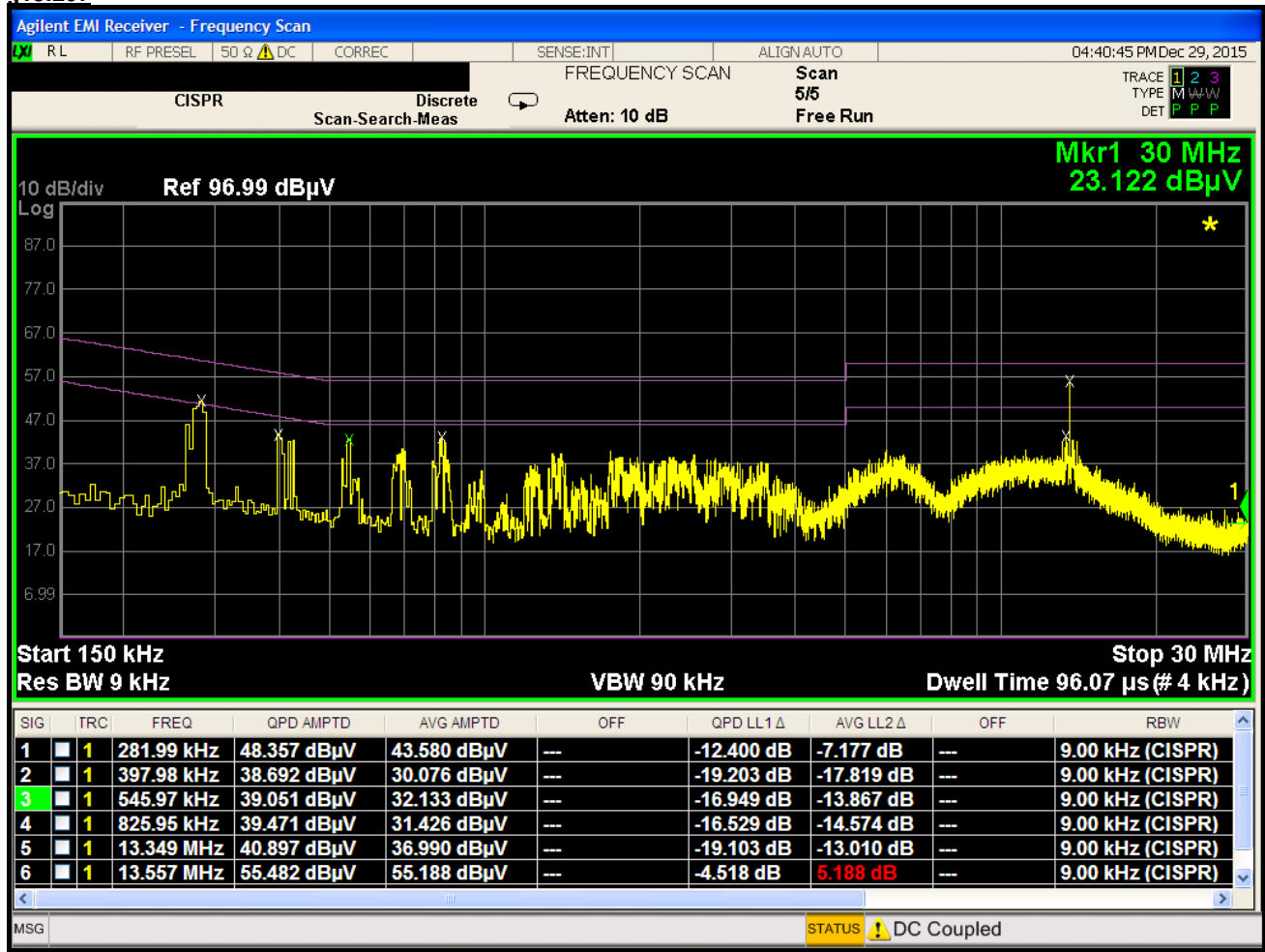
Plot 8-2. Line-Conducted Test Plot with RFID Antenna Attached(N)
