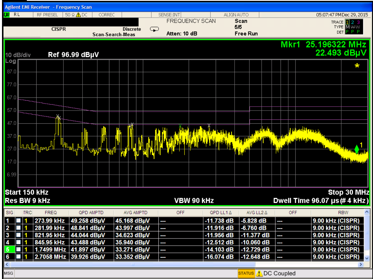
Plot 8-3. Line-Conducted Test Plot with RFID Antenna Terminated in 50 Ohms (L1)
