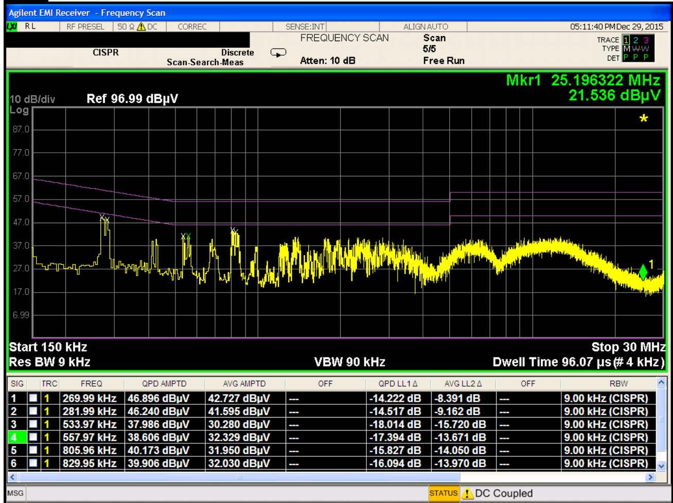
Plot 8-4. Line-Conducted Test Plot with RFID Antenna Terminated in 50 Ohms (N)
