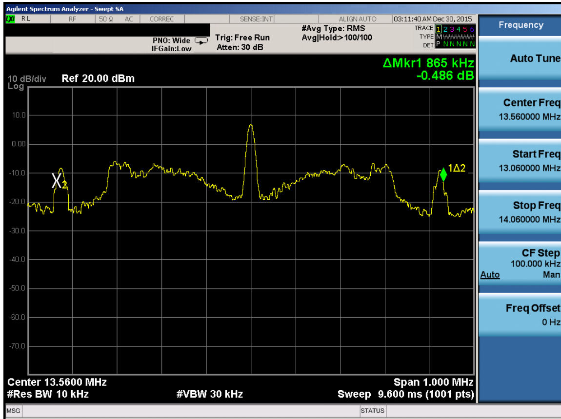
Figure 8-3. 20dB Bandwidth Plot with WCP
