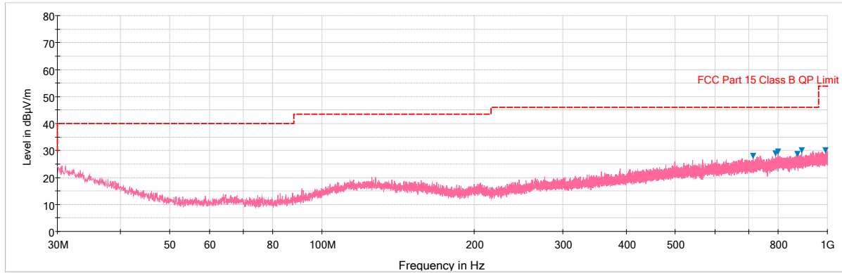
Plot 7-281. Radiated Spurious Plot below 1GHz (Simultaneous Transmission Config-2, Ant. Pol. V)
