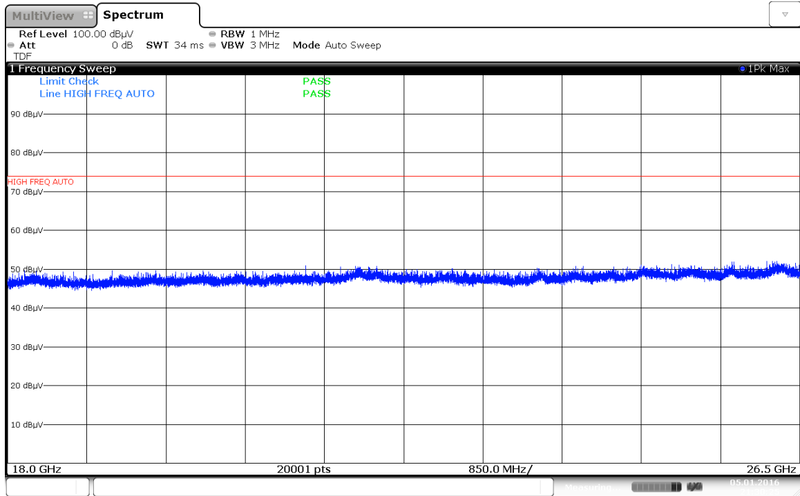
Plot 7-189. Radiated Spurious Plot 18GHz – 26.5GHz (Simultaneous Transmission Config-2 Ant. Pol. H)
