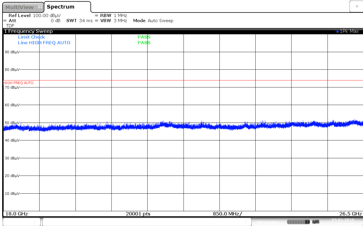
Plot 7-183. Radiated Spurious Plot 18GHz – 26.5GHz (Simultaneous Transmission Config-1 Ant. Pol. H)
