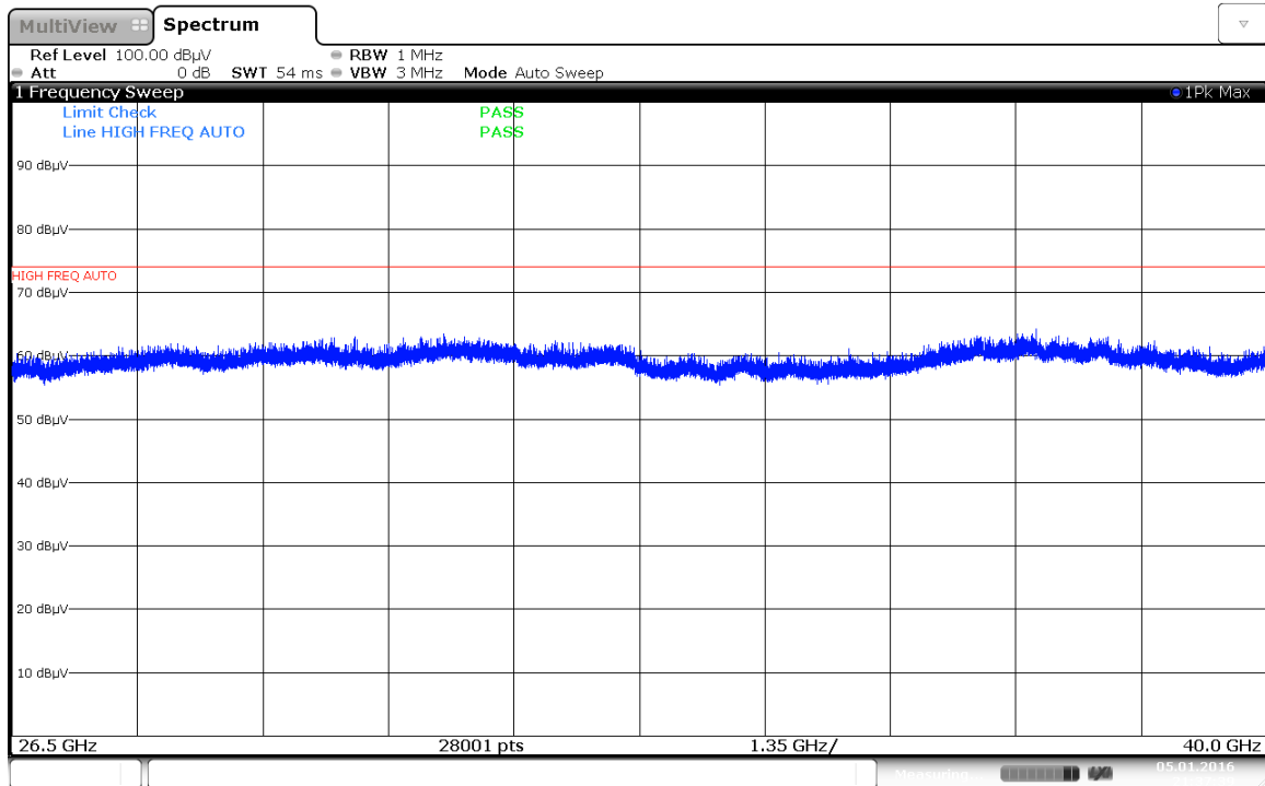
Plot 7-184. Radiated Spurious Plot above 26.5GHz (Simultaneous Transmission Config-1 Ant. Pol. H)
