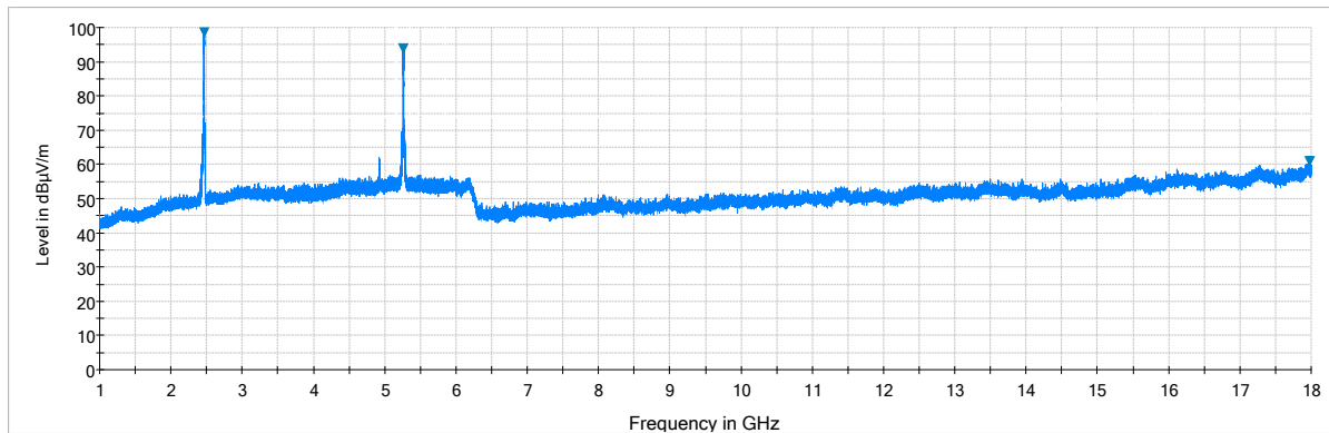
Plot 7-188. Radiated Spurious Plot above 1GHz (Simultaneous Transmission Config-2, Ant. Pol. V)
