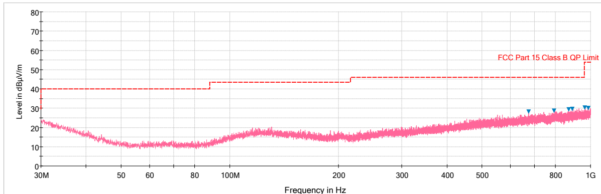
Plot 7-279. Radiated Spurious Plot below 1GHz (Simultaneous Transmission Config-1, Ant. Pol. V)
