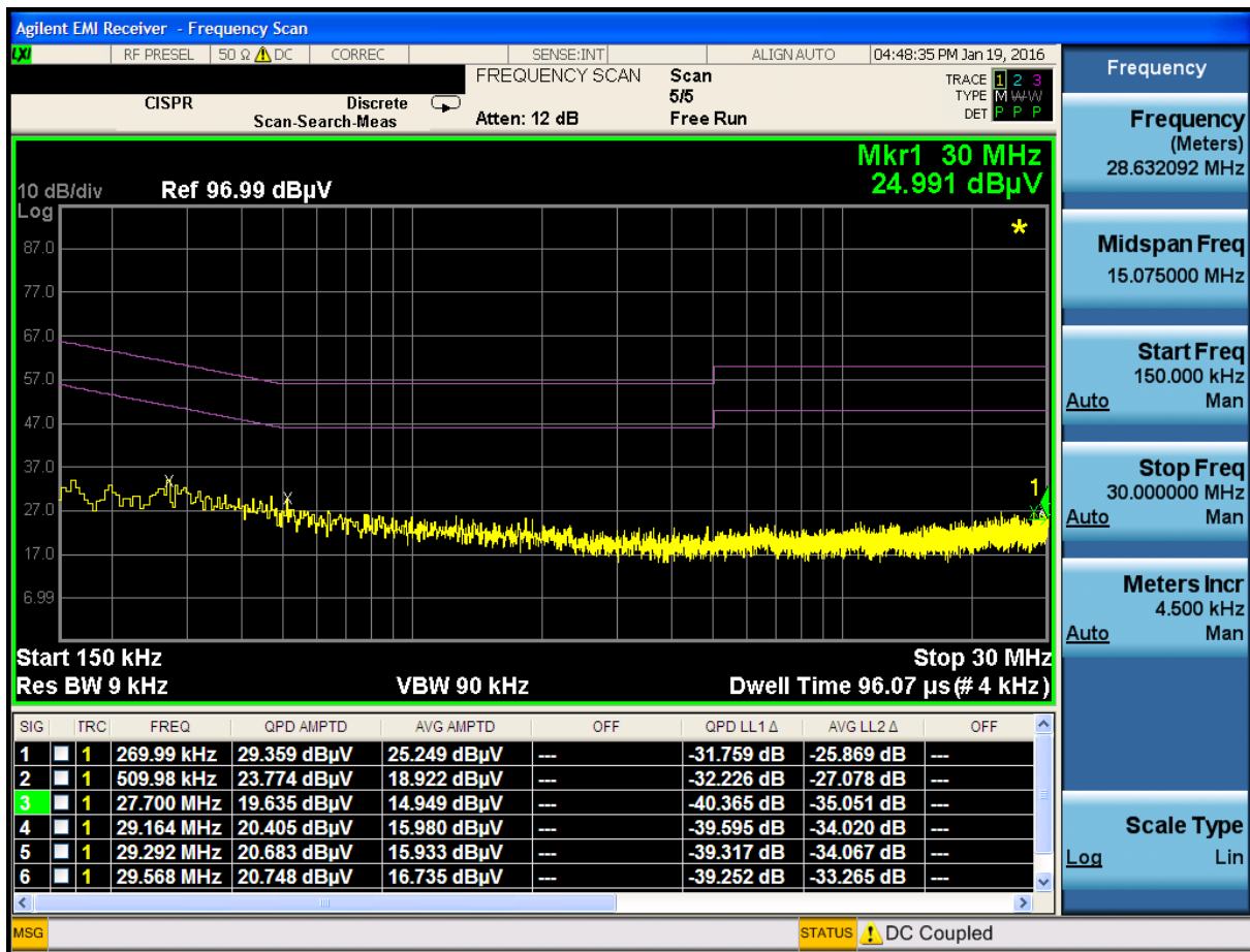
Plot 7-2. Line Conducted Plot (LN)
