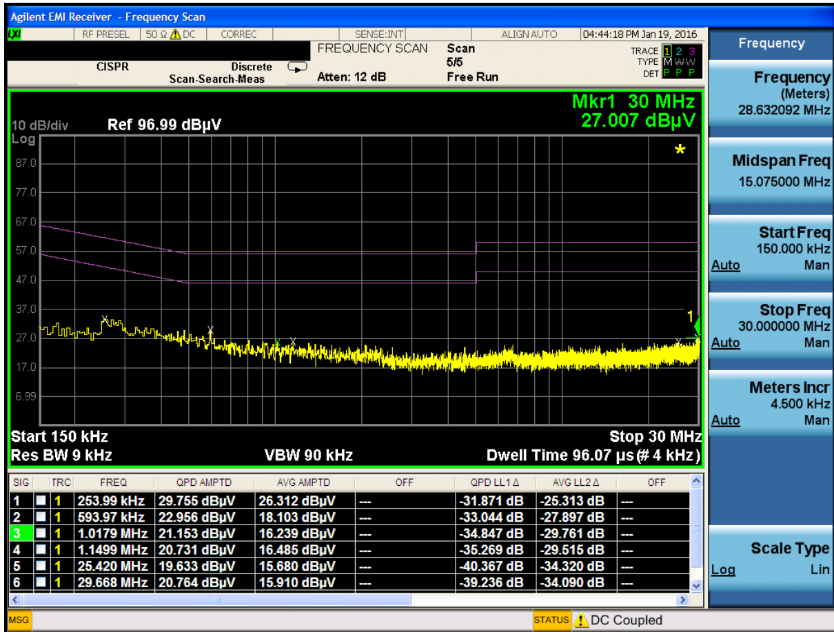
Plot 7-1. Line Conducted Plot (L1)
